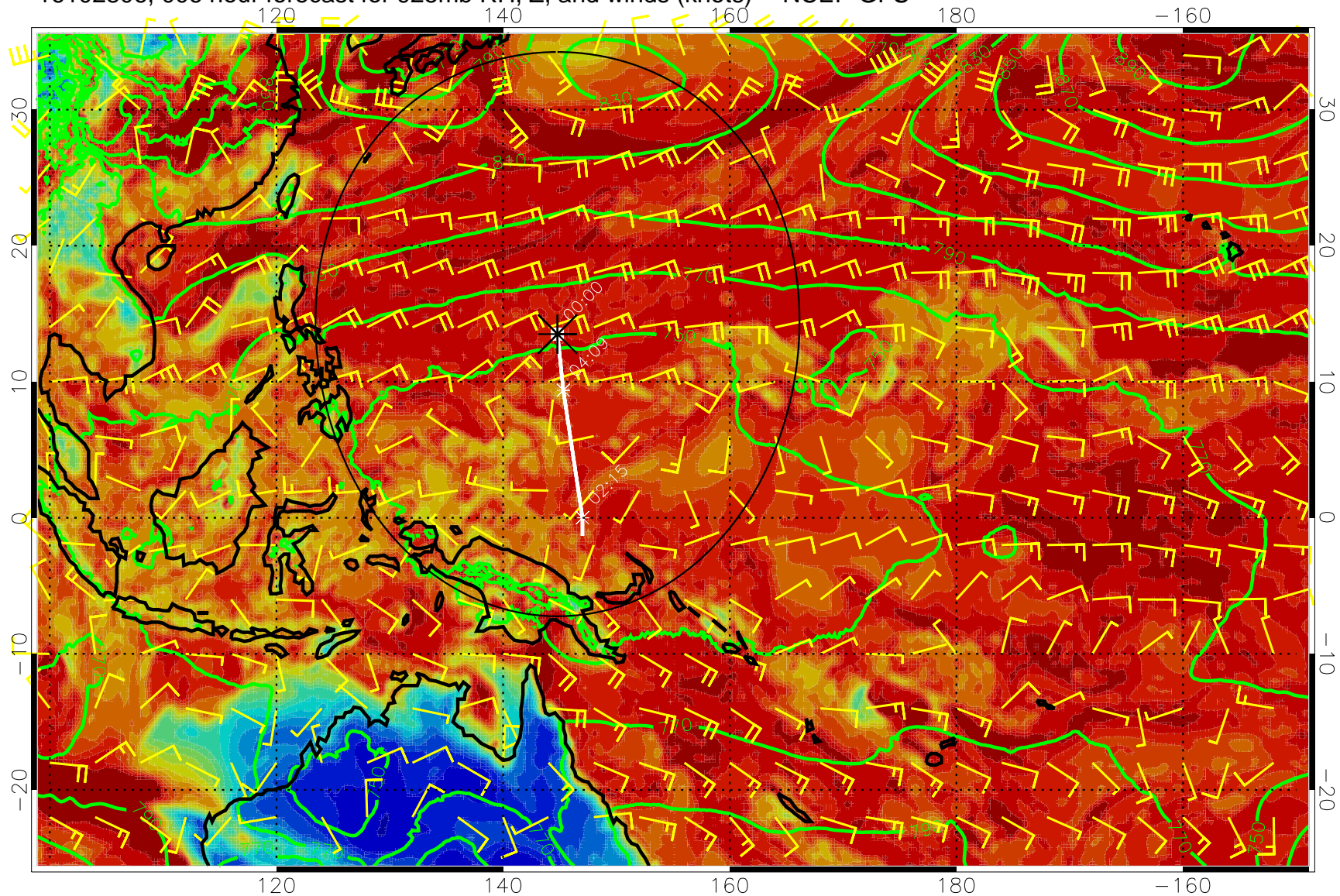
16102806, 006 hour forecast for 925mb RH, Z, and winds (knots) -- NCEP GFS
