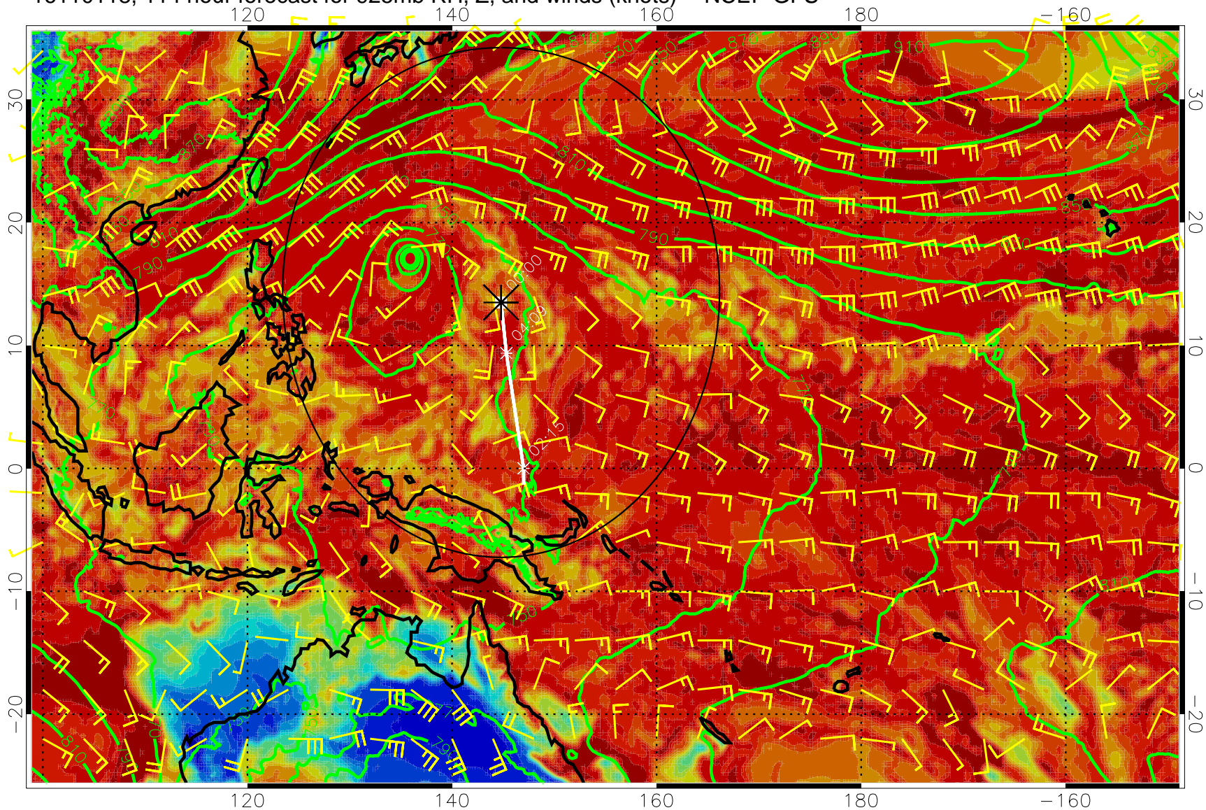
16110118, 114 hour forecast for 925mb RH, Z, and winds (knots) -- NCEP GFS
