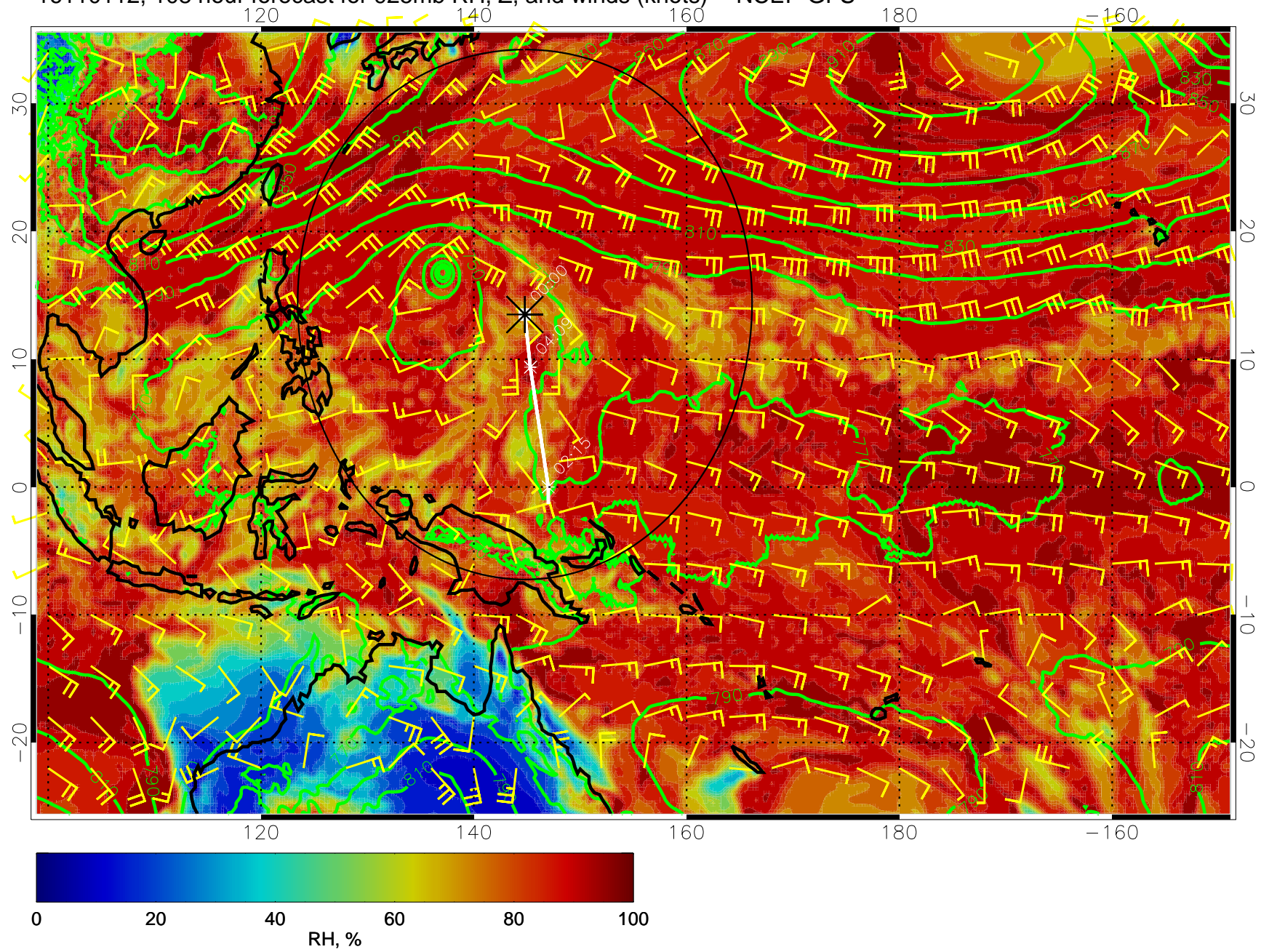
16110112, 108 hour forecast for 925mb RH, Z, and winds (knots) -- NCEP GFS
