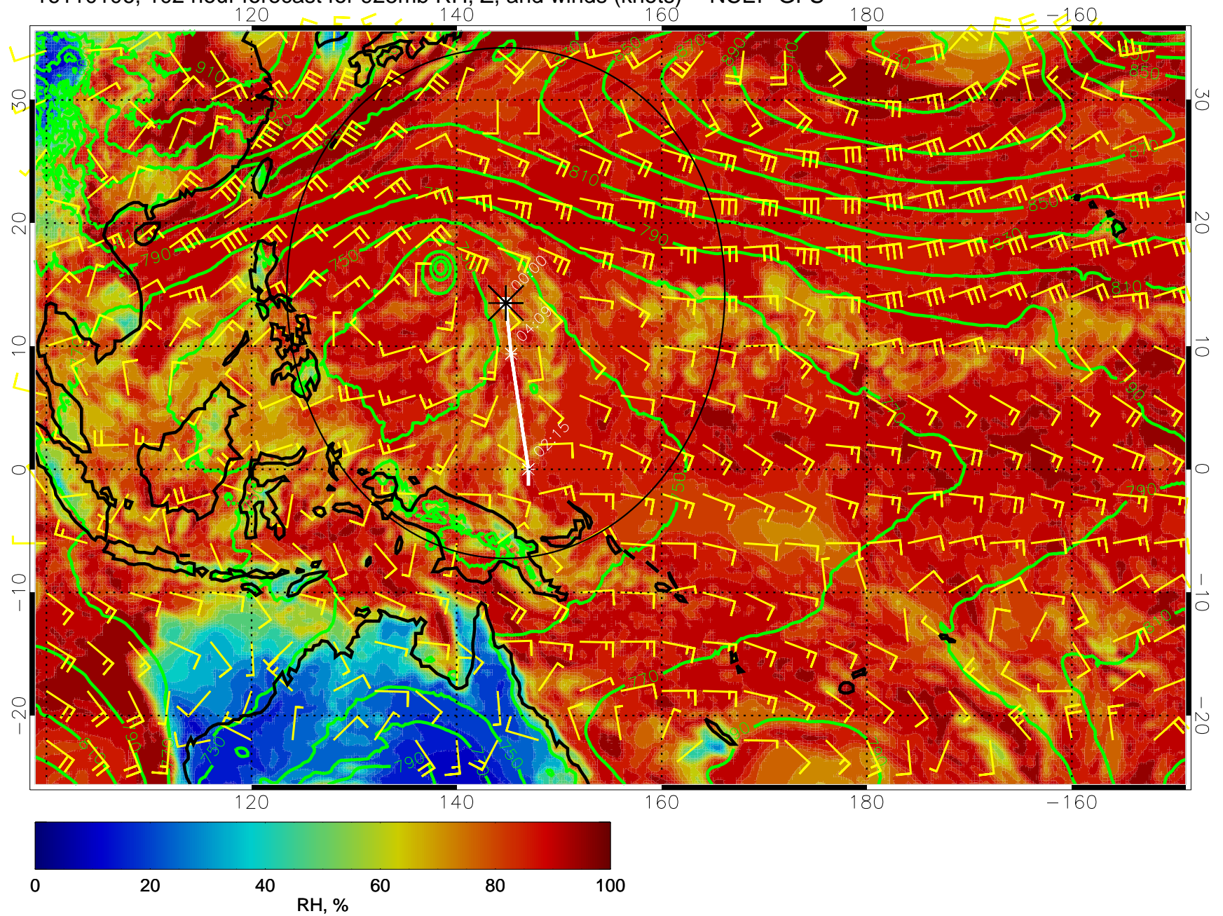
16110106, 102 hour forecast for 925mb RH, Z, and winds (knots) -- NCEP GFS
