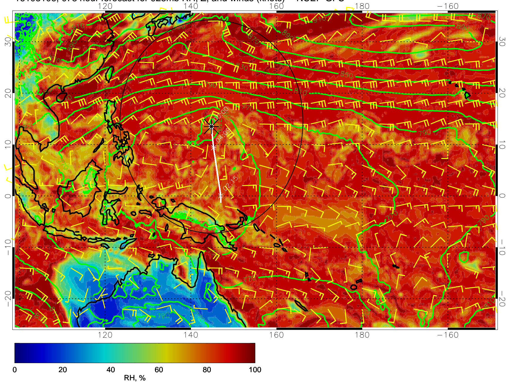
16103106, 078 hour forecast for 925mb RH, Z, and winds (knots) -- NCEP GFS
