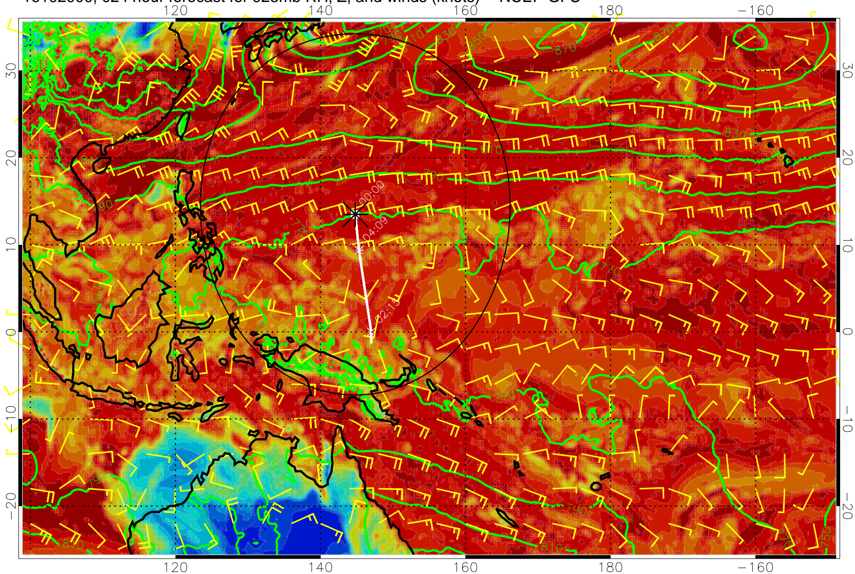
16102900, 024 hour forecast for 925mb RH, Z, and winds (knots) -- NCEP GFS
