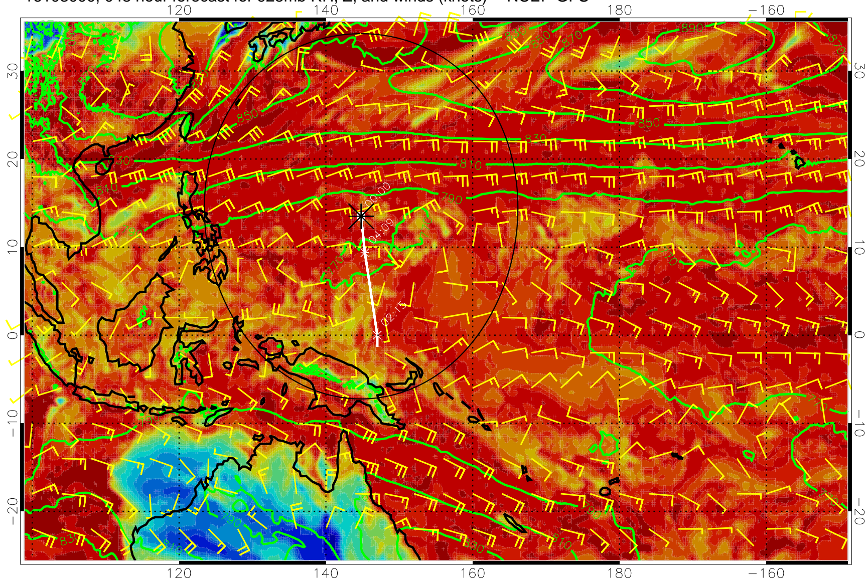
16103000, 048 hour forecast for 925mb RH, Z, and winds (knots) -- NCEP GFS
