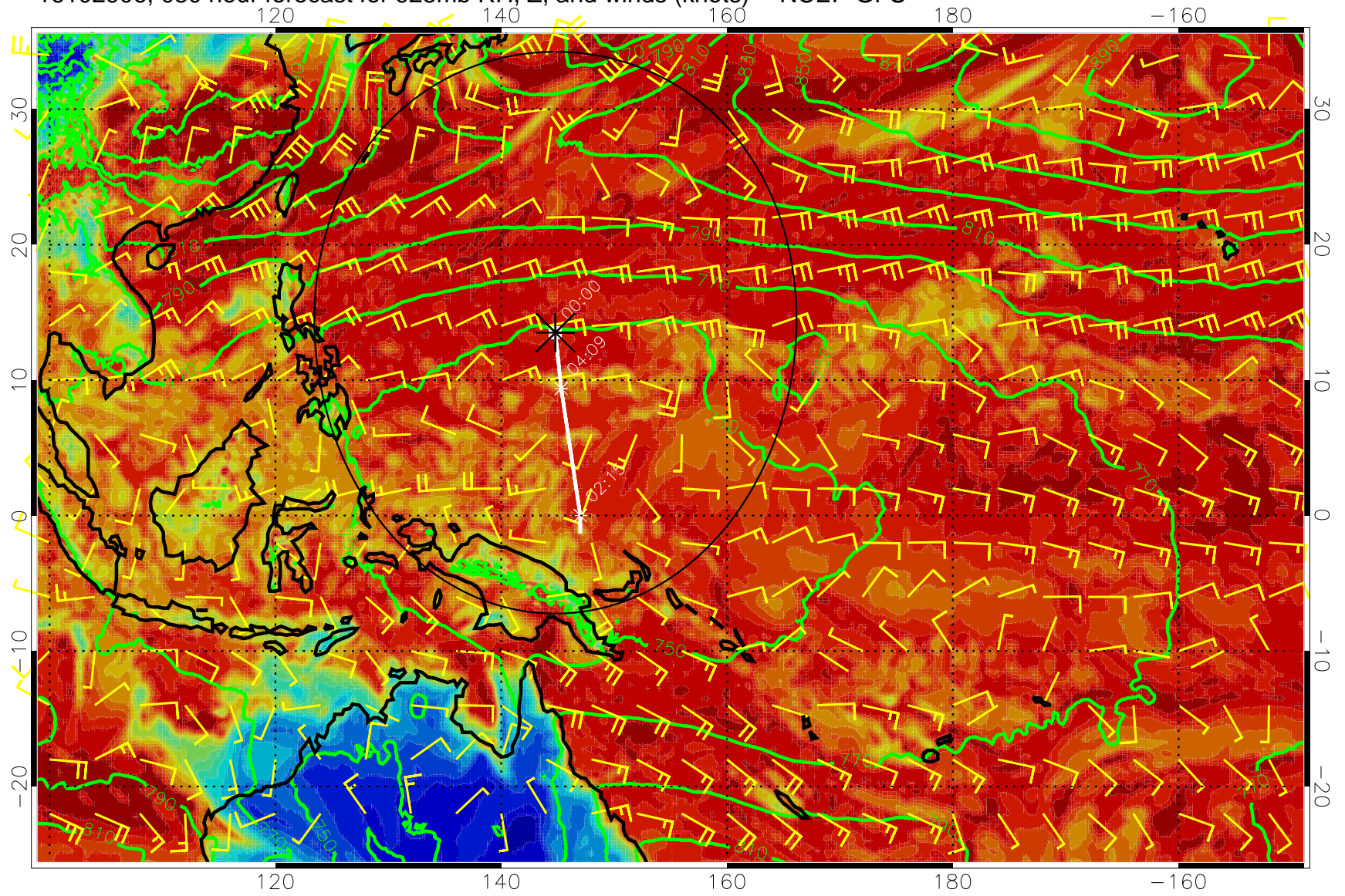
16102906, 030 hour forecast for 925mb RH, Z, and winds (knots) -- NCEP GFS
