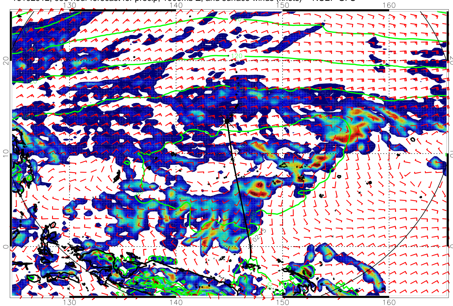
16102912, 036 hour forecast for precip, 1000mb Z, and surface winds (knots) -- NCEP GFS
