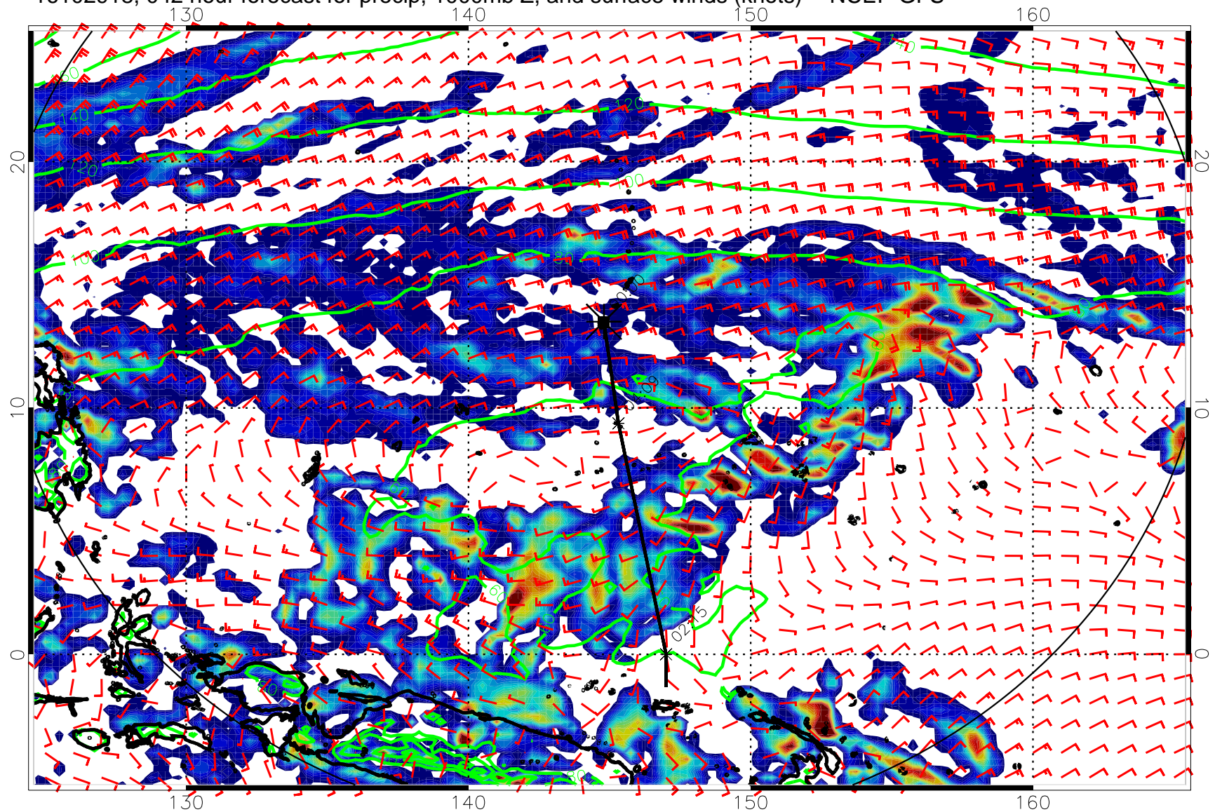
16102918, 042 hour forecast for precip, 1000mb Z, and surface winds (knots) -- NCEP GFS
