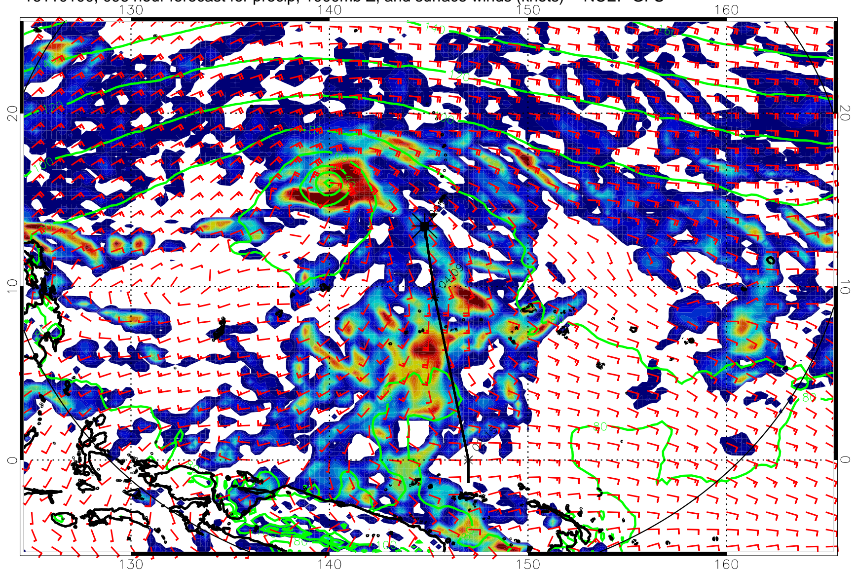
16110100, 096 hour forecast for precip, 1000mb Z, and surface winds (knots) -- NCEP GFS
