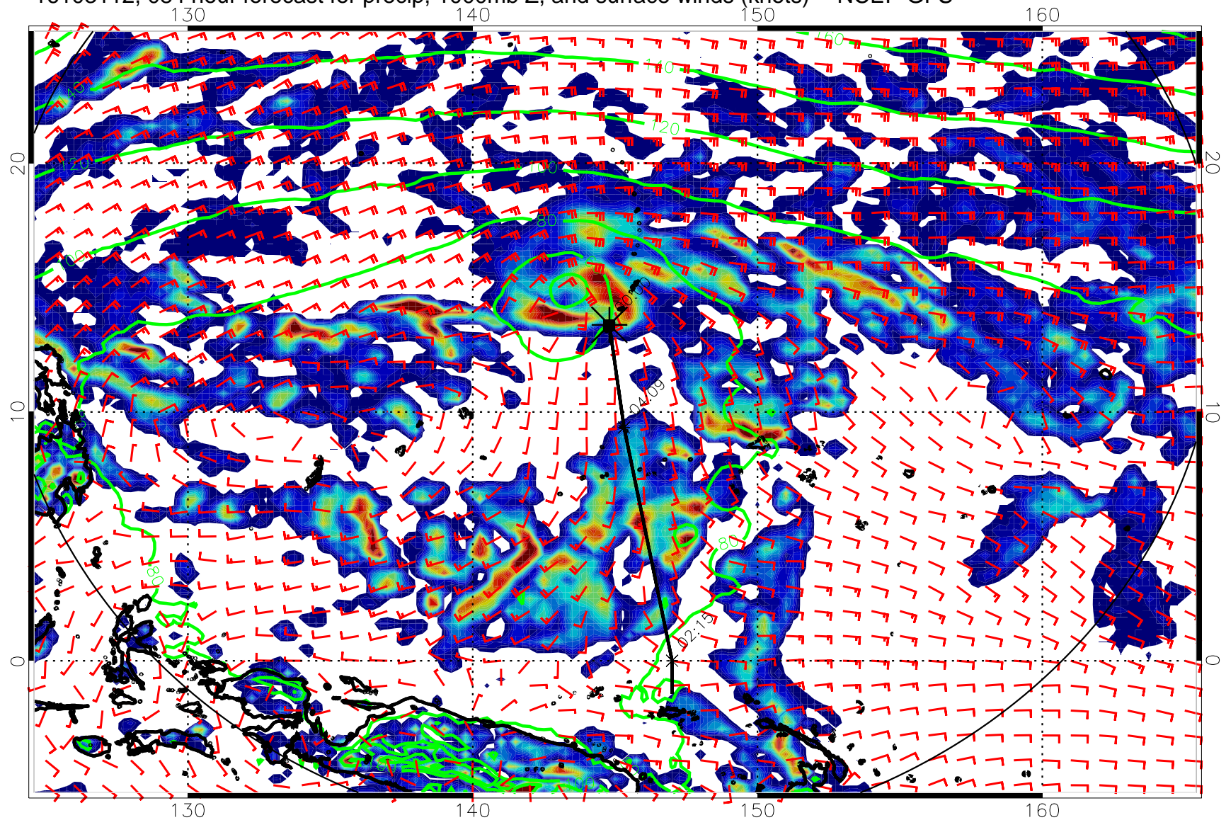
16103112, 084 hour forecast for precip, 1000mb Z, and surface winds (knots) -- NCEP GFS
