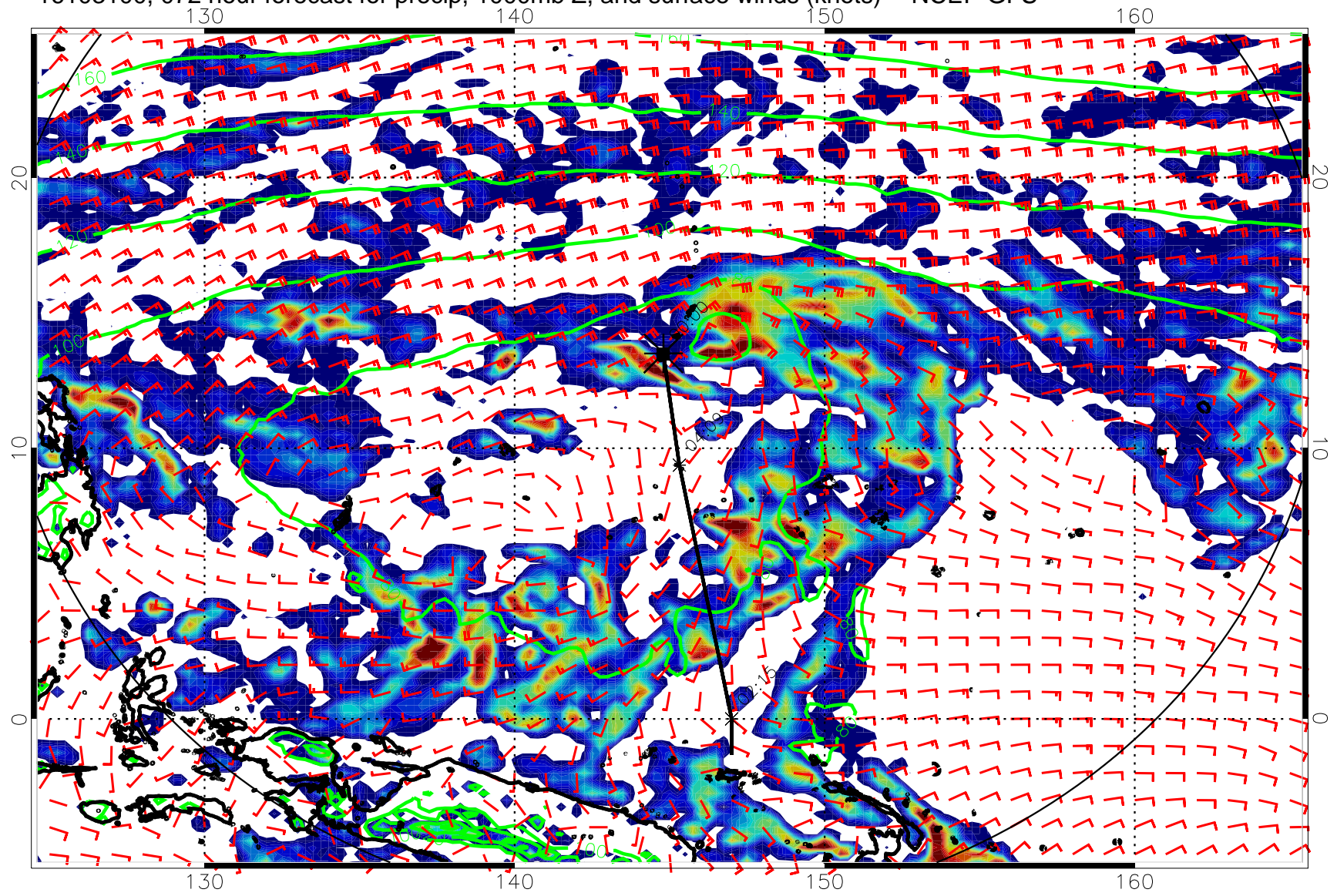
16103100, 072 hour forecast for precip, 1000mb Z, and surface winds (knots) -- NCEP GFS
