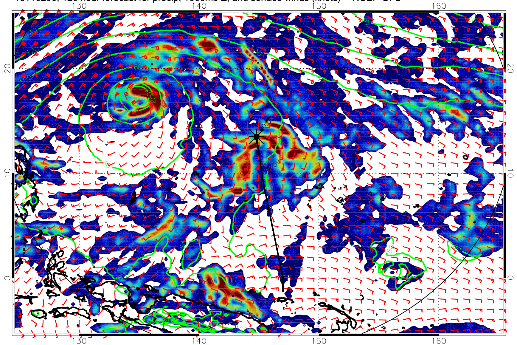
16110200, 120 hour forecast for precip, 1000mb Z, and surface winds (knots) -- NCEP GFS
