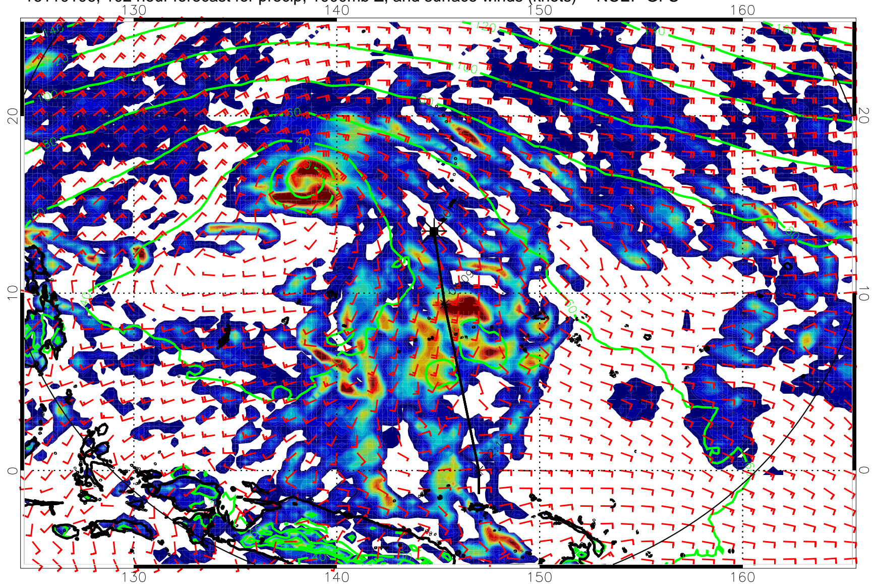
16110106, 102 hour forecast for precip, 1000mb Z, and surface winds (knots) -- NCEP GFS
