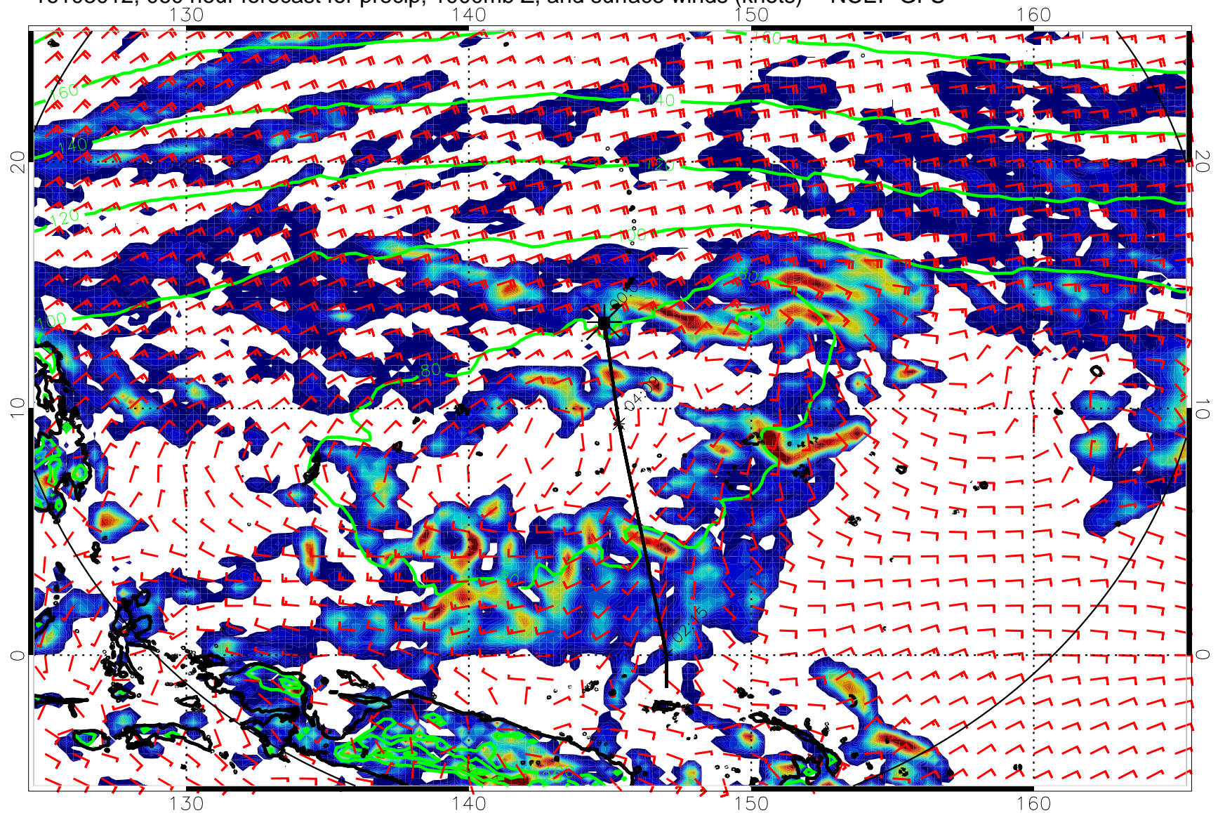
16103012, 060 hour forecast for precip, 1000mb Z, and surface winds (knots) -- NCEP GFS
