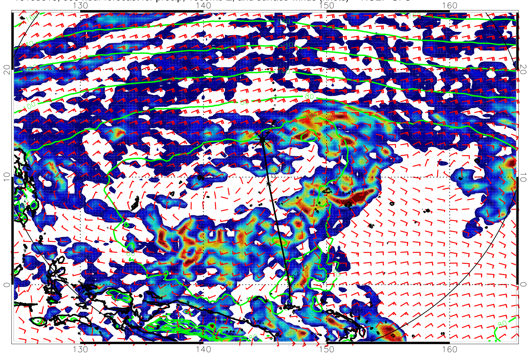
16103018, 066 hour forecast for precip, 1000mb Z, and surface winds (knots) -- NCEP GFS
