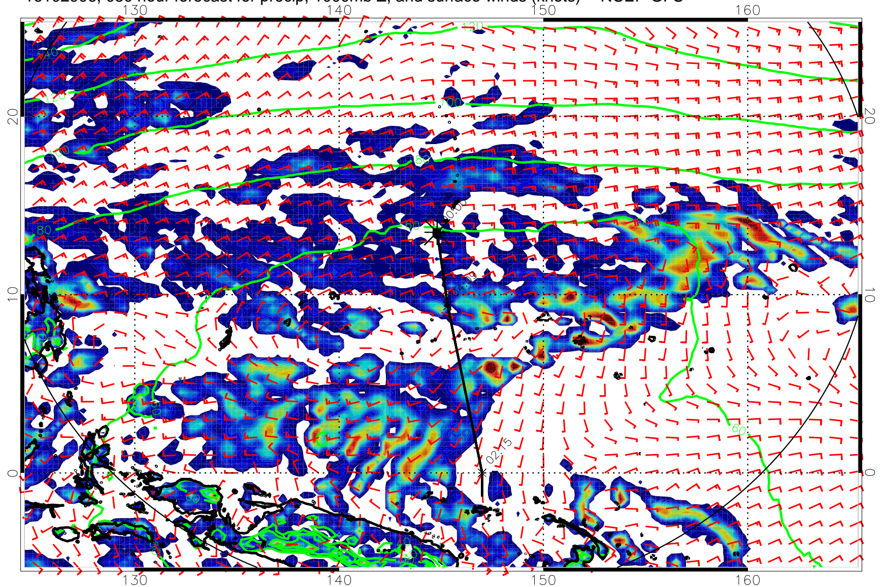
16102906, 030 hour forecast for precip, 1000mb Z, and surface winds (knots) -- NCEP GFS
