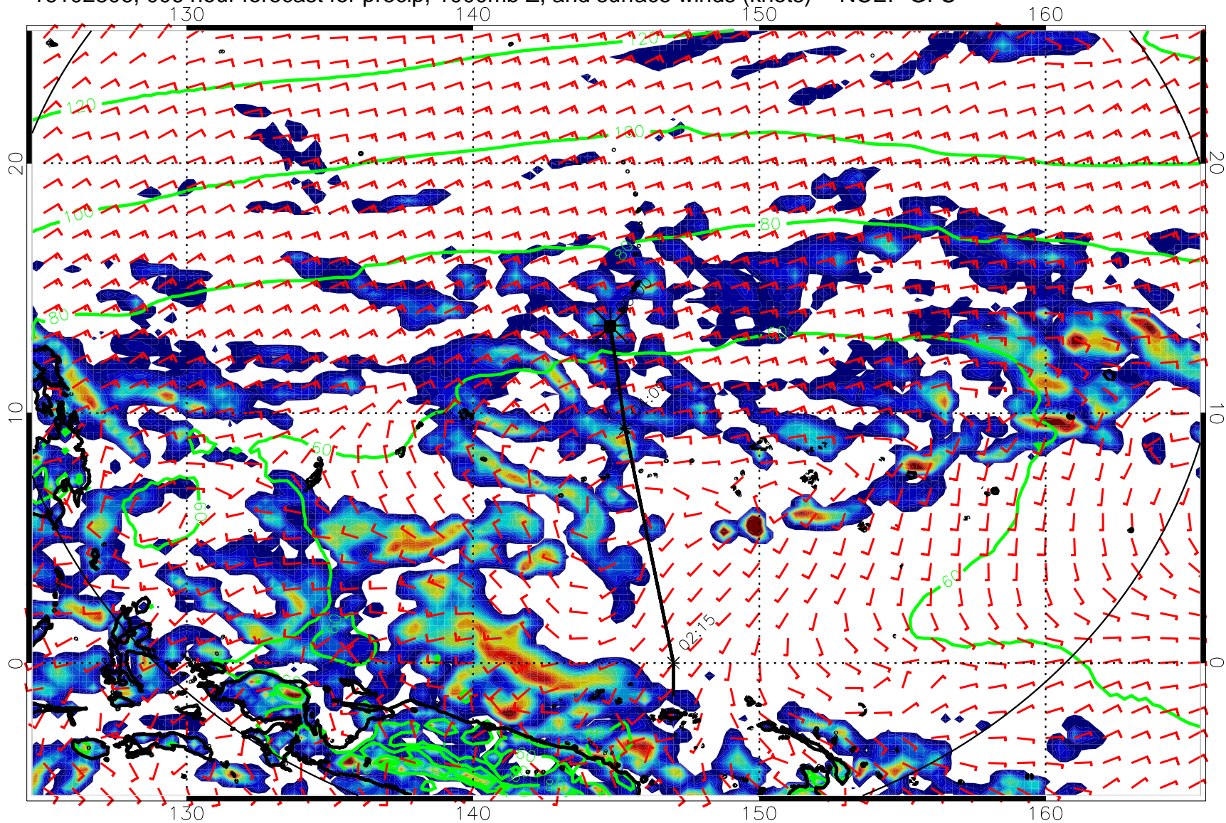
16102806, 006 hour forecast for precip, 1000mb Z, and surface winds (knots) -- NCEP GFS
