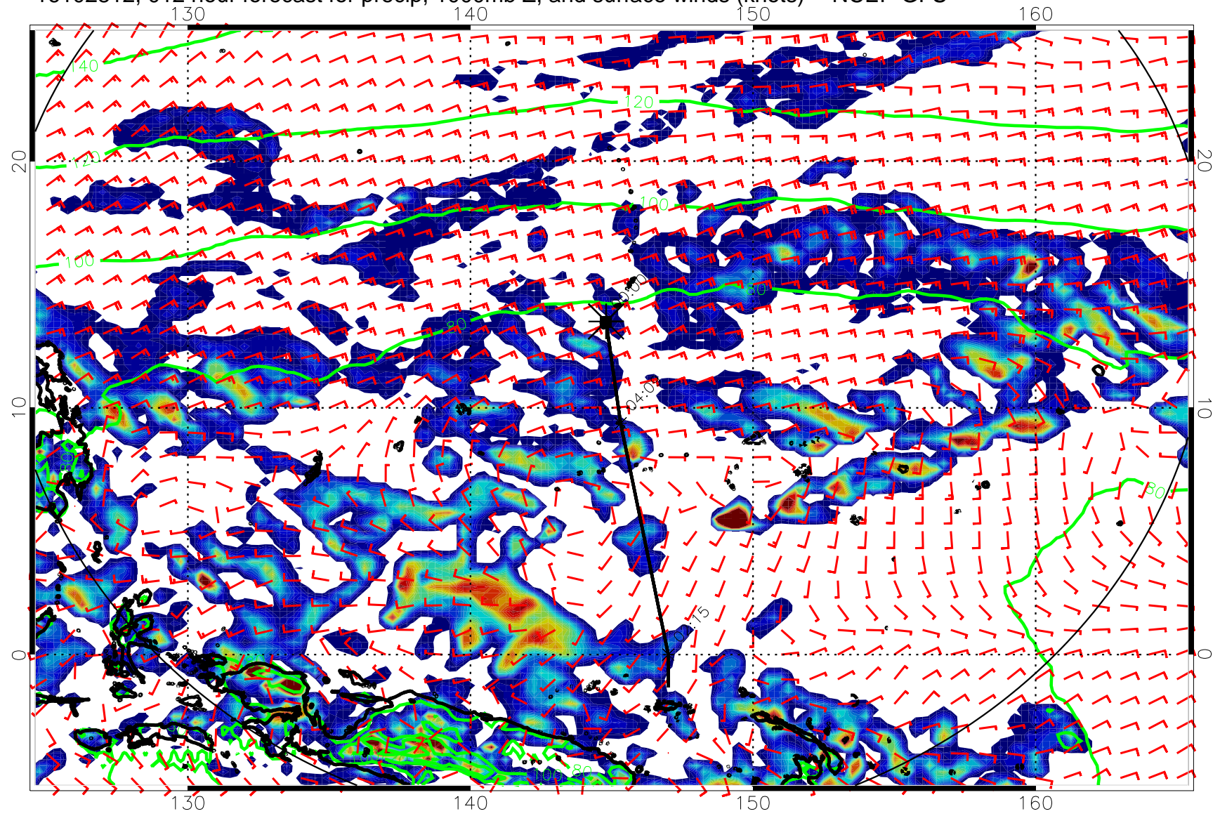
16102812, 012 hour forecast for precip, 1000mb Z, and surface winds (knots) -- NCEP GFS
