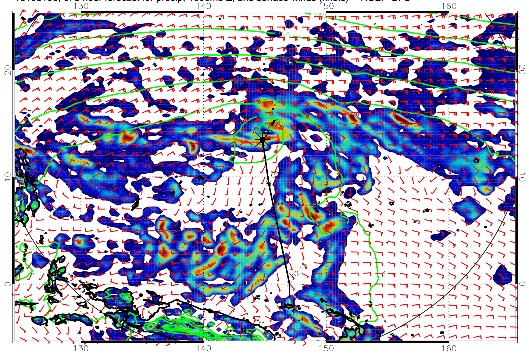
16103106, 078 hour forecast for precip, 1000mb Z, and surface winds (knots) -- NCEP GFS
