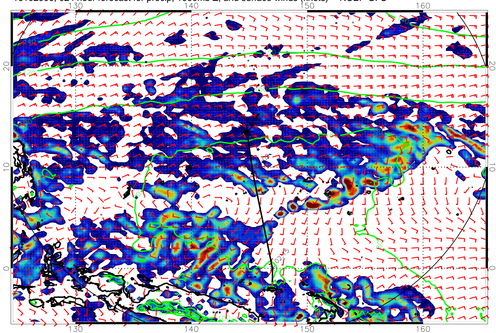
16102900, 024 hour forecast for precip, 1000mb Z, and surface winds (knots) -- NCEP GFS
