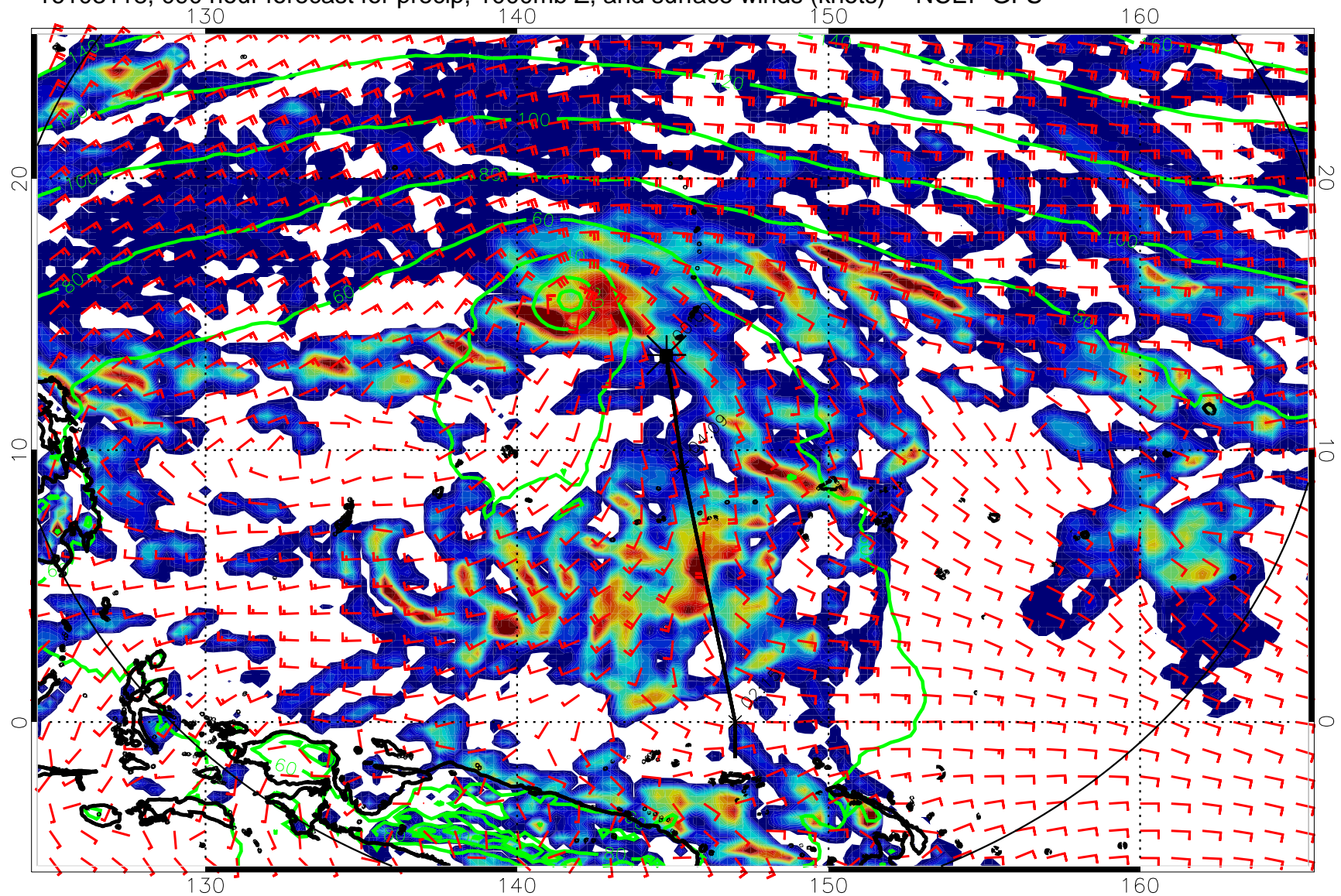
16103118, 090 hour forecast for precip, 1000mb Z, and surface winds (knots) -- NCEP GFS
