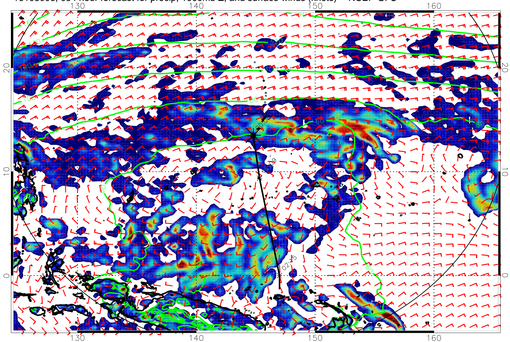
16103006, 054 hour forecast for precip, 1000mb Z, and surface winds (knots) -- NCEP GFS
