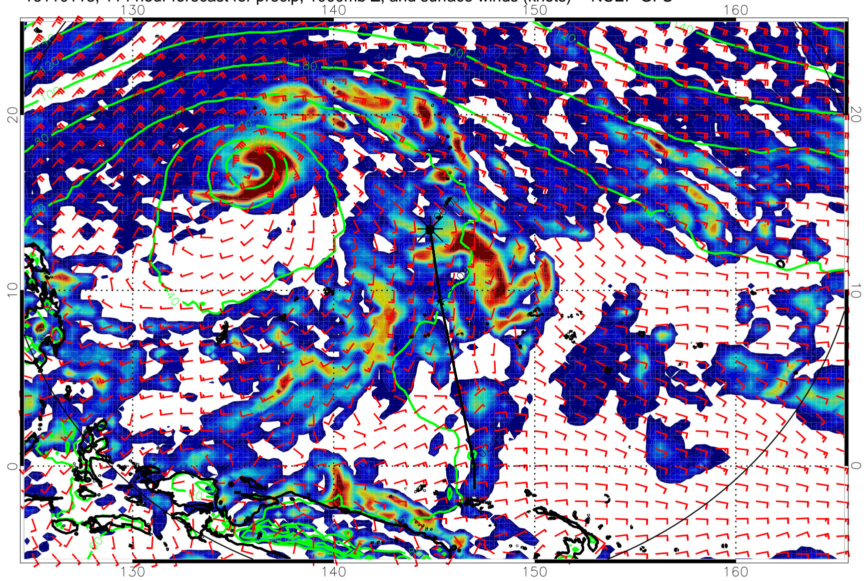
16110118, 114 hour forecast for precip, 1000mb Z, and surface winds (knots) -- NCEP GFS
