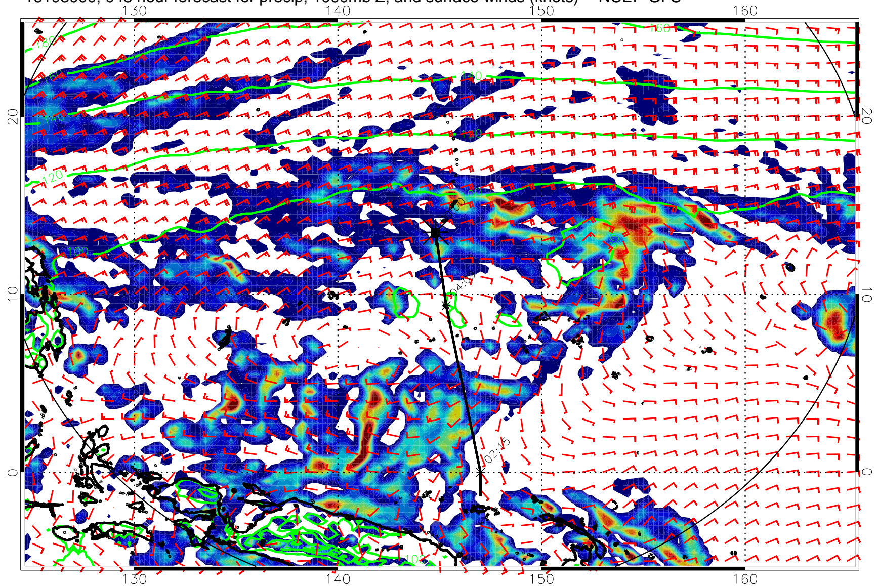
16103000, 048 hour forecast for precip, 1000mb Z, and surface winds (knots) -- NCEP GFS
