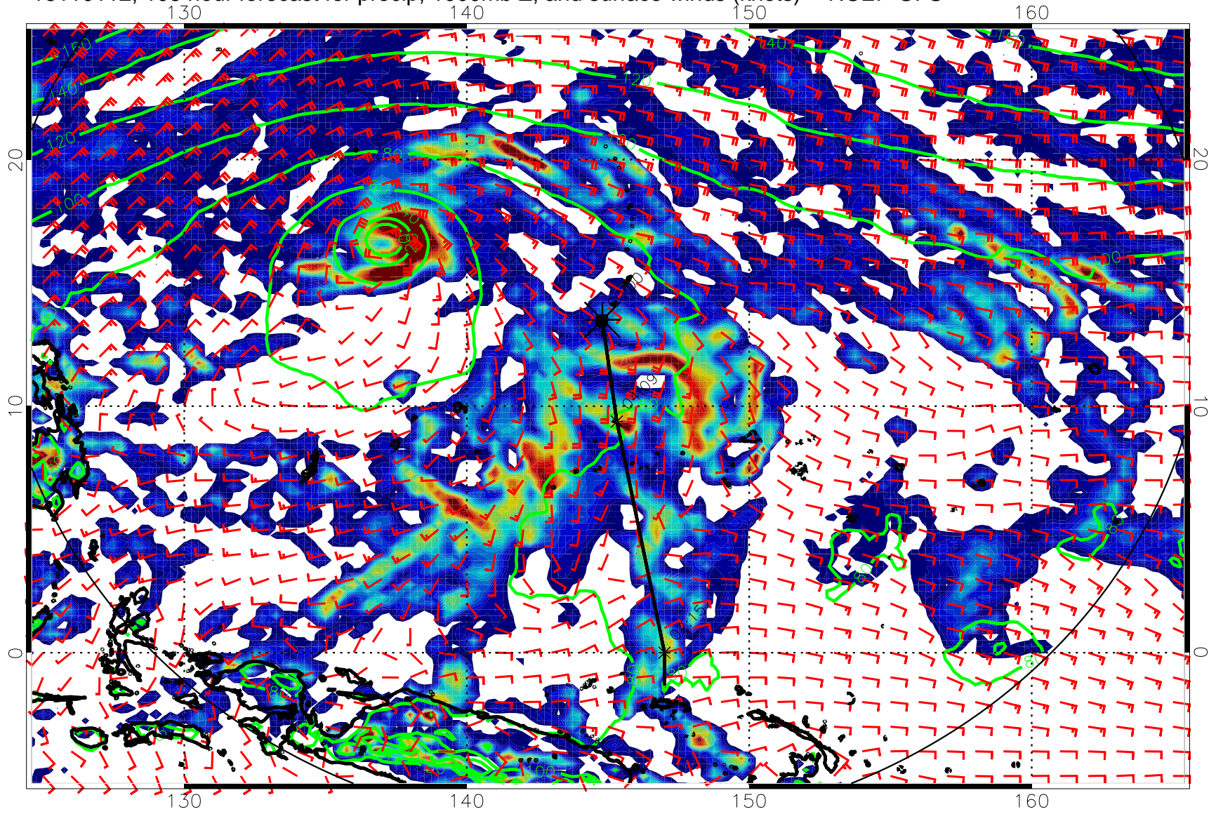
16110112, 108 hour forecast for precip, 1000mb Z, and surface winds (knots) -- NCEP GFS
