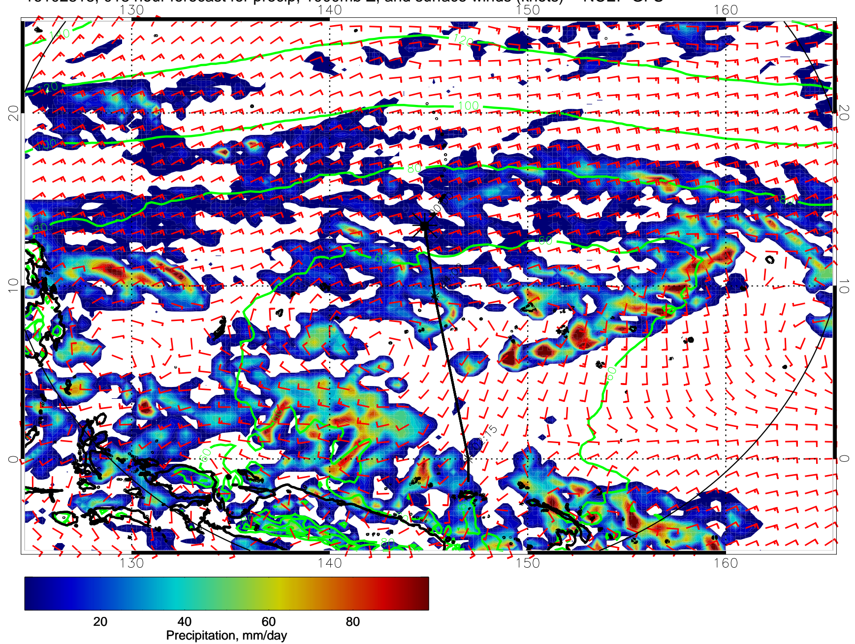
16102818, 018 hour forecast for precip, 1000mb Z, and surface winds (knots) -- NCEP GFS
