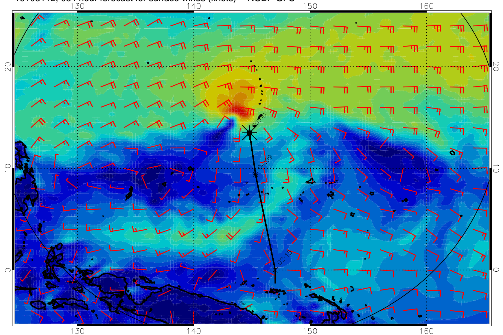
16103112, 084 hour forecast for surface winds (knots) -- NCEP GFS
