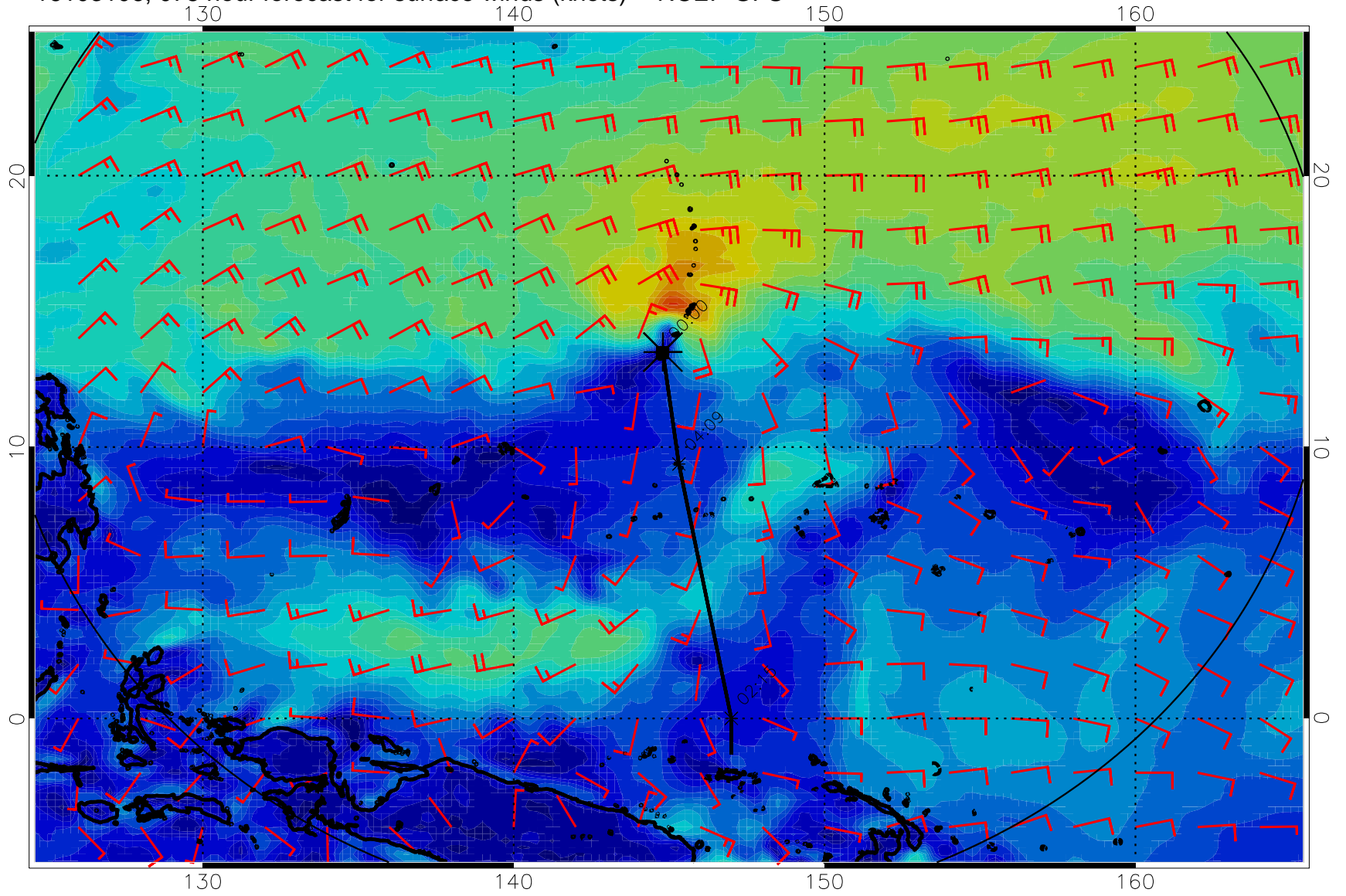
16103106, 078 hour forecast for surface winds (knots) -- NCEP GFS
