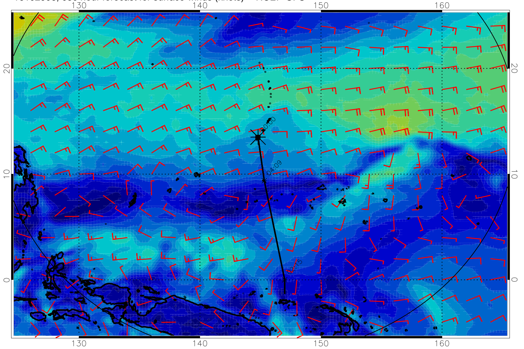
16102906, 030 hour forecast for surface winds (knots) -- NCEP GFS
