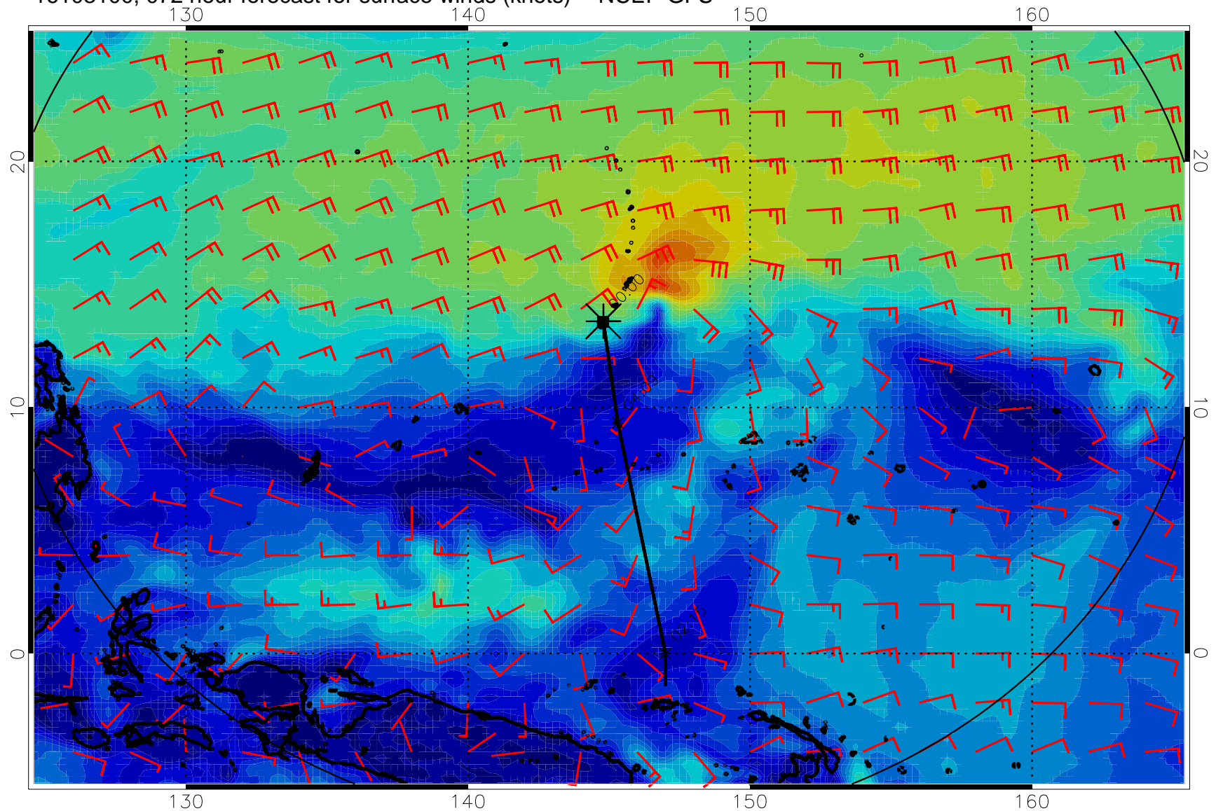
16103100, 072 hour forecast for surface winds (knots) -- NCEP GFS
