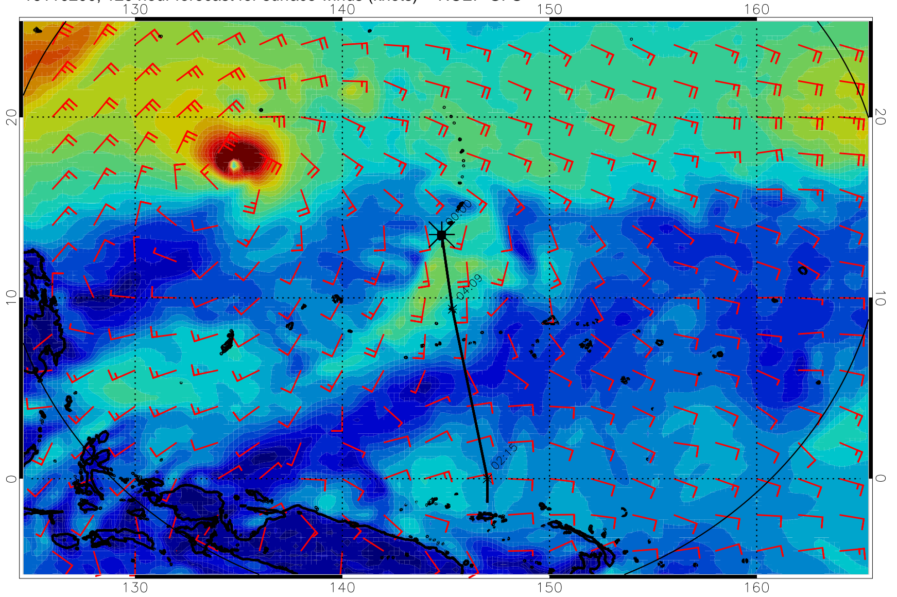
16110200, 120 hour forecast for surface winds (knots) -- NCEP GFS
