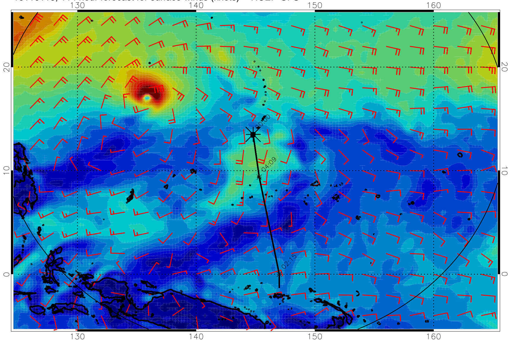
16110118, 114 hour forecast for surface winds (knots) -- NCEP GFS
