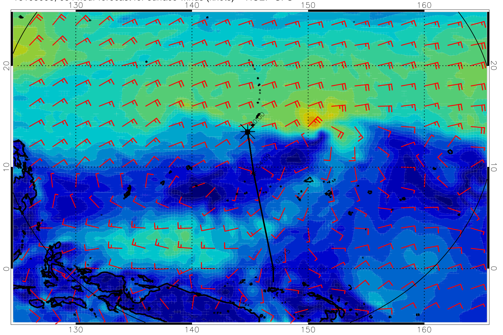
16103006, 054 hour forecast for surface winds (knots) -- NCEP GFS
