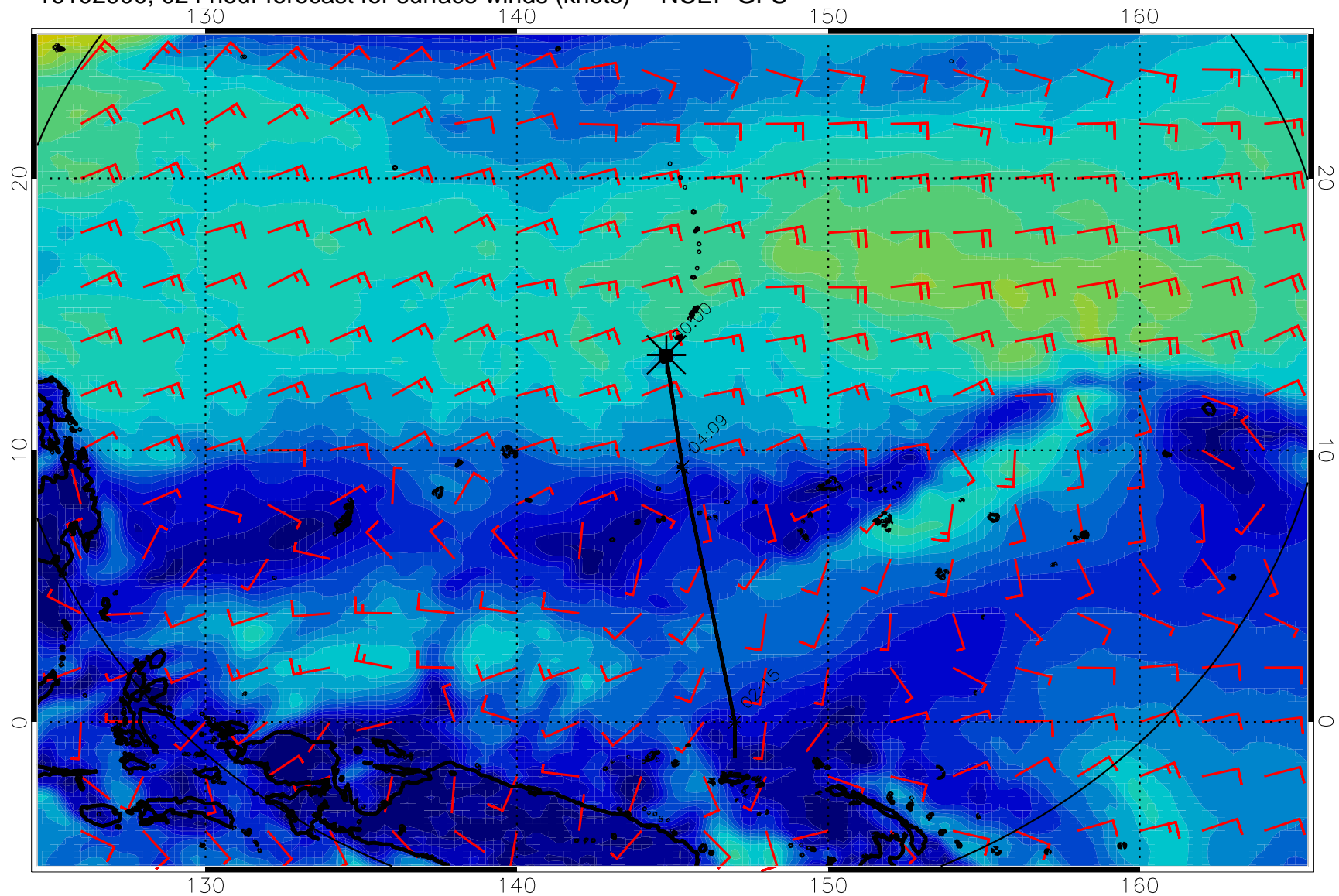
16102900, 024 hour forecast for surface winds (knots) -- NCEP GFS
