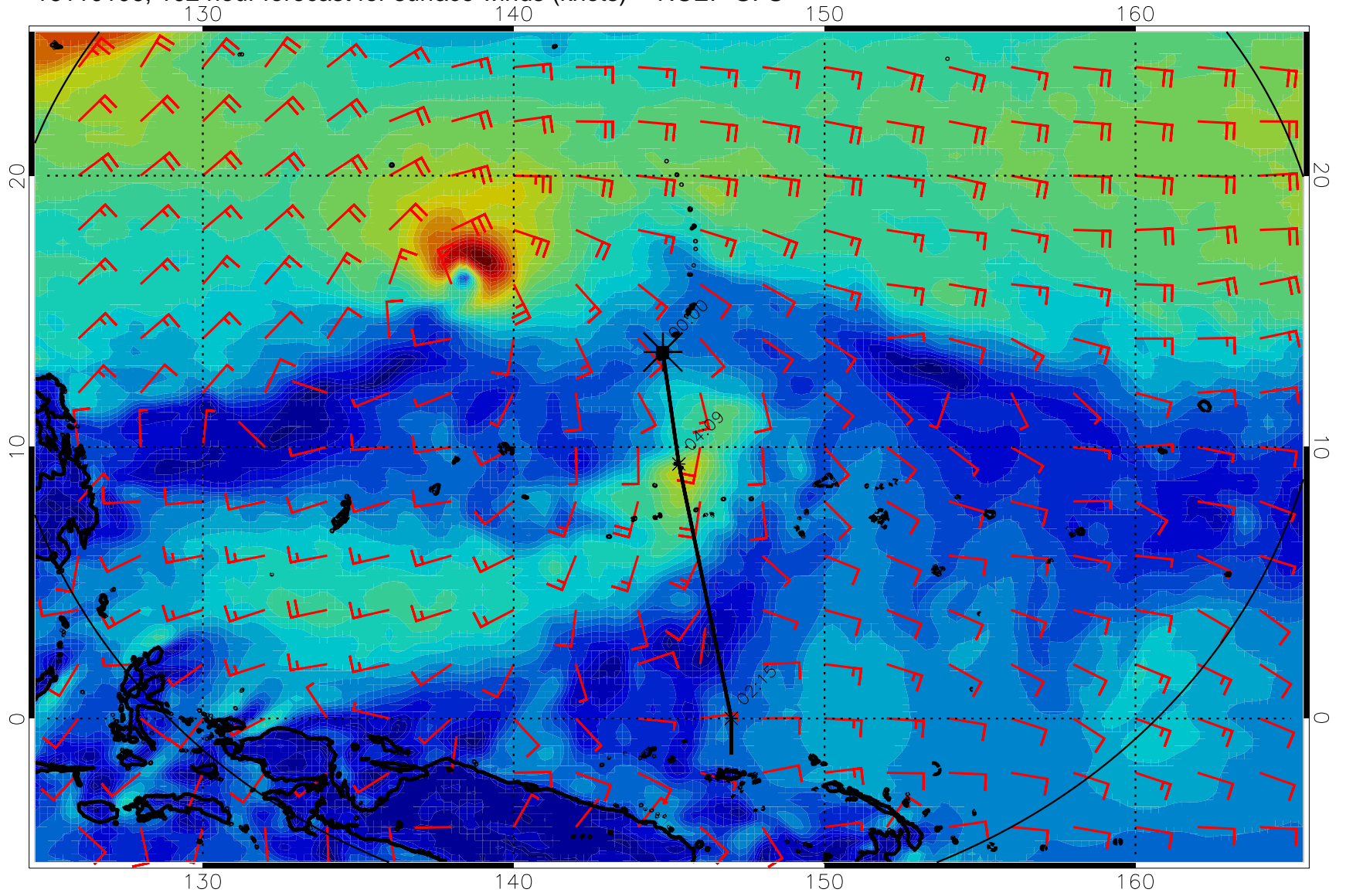
16110106, 102 hour forecast for surface winds (knots) -- NCEP GFS
