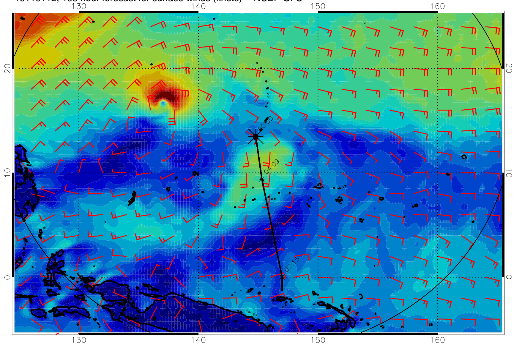
16110112, 108 hour forecast for surface winds (knots) -- NCEP GFS
