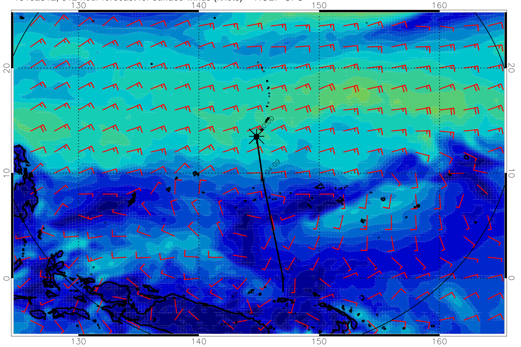
16102812, 012 hour forecast for surface winds (knots) -- NCEP GFS
