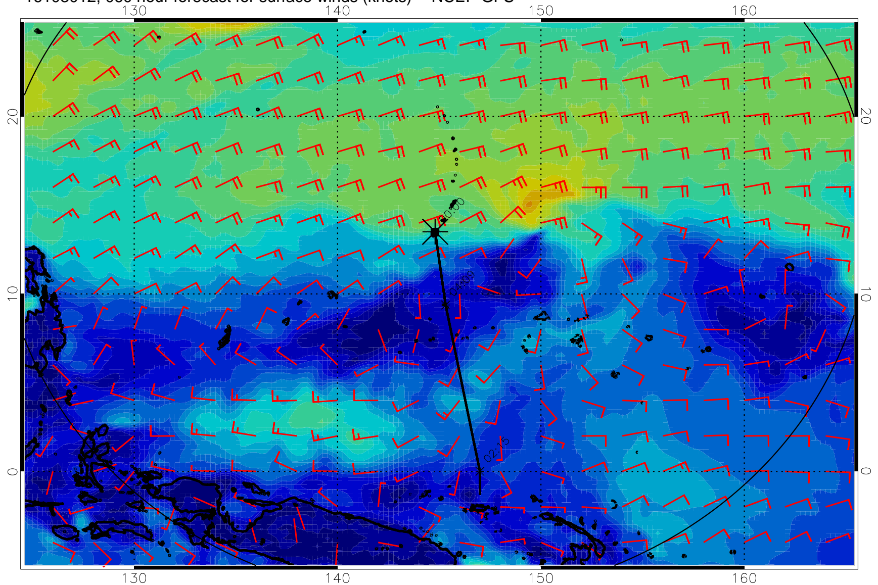
16103012, 060 hour forecast for surface winds (knots) -- NCEP GFS
