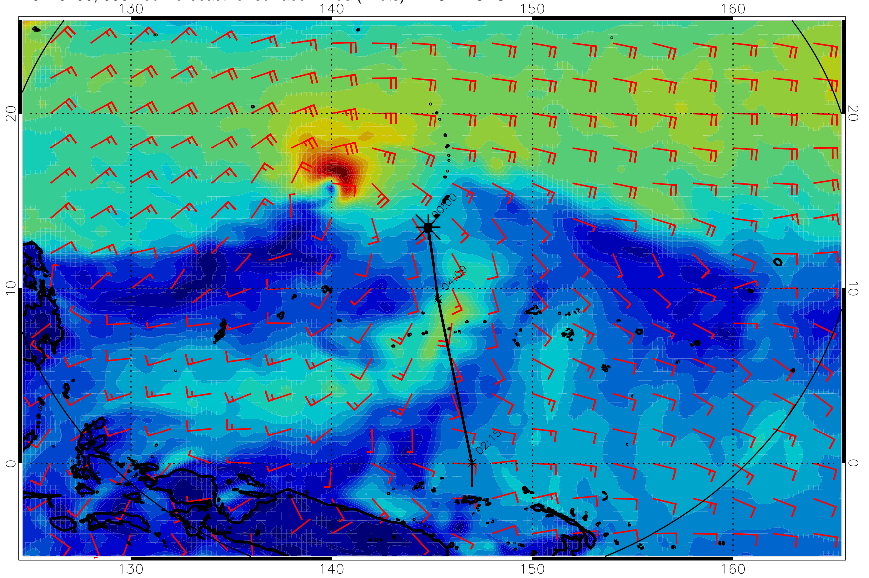
16110100, 096 hour forecast for surface winds (knots) -- NCEP GFS
