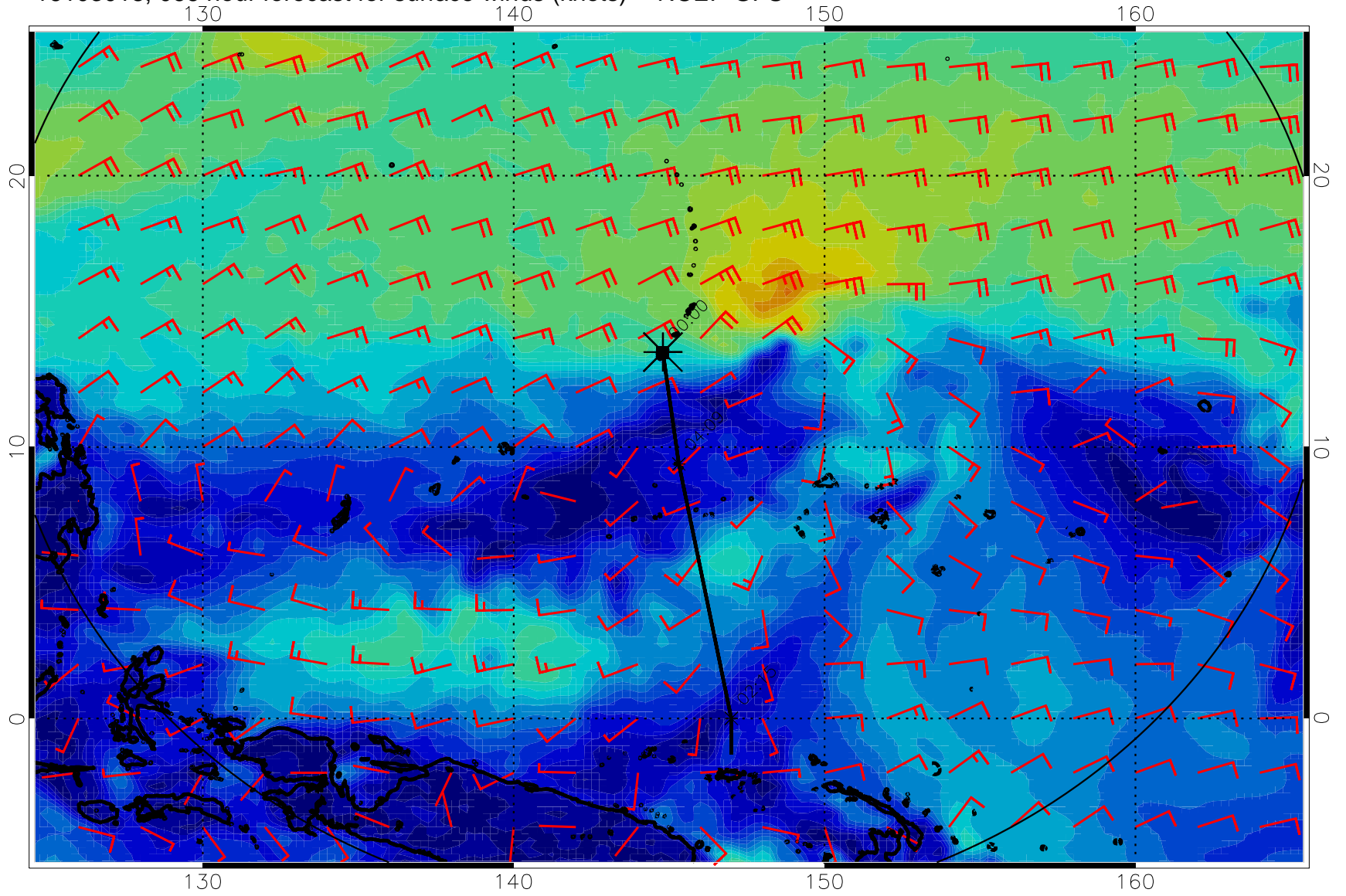
16103018, 066 hour forecast for surface winds (knots) -- NCEP GFS
