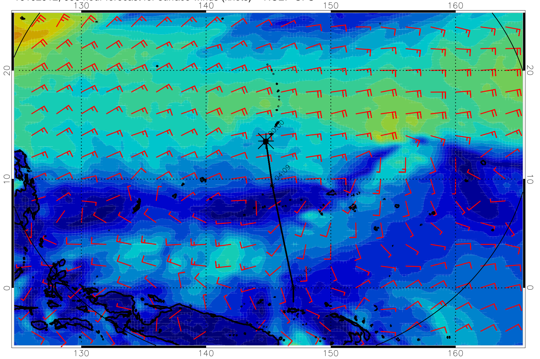
16102912, 036 hour forecast for surface winds (knots) -- NCEP GFS
