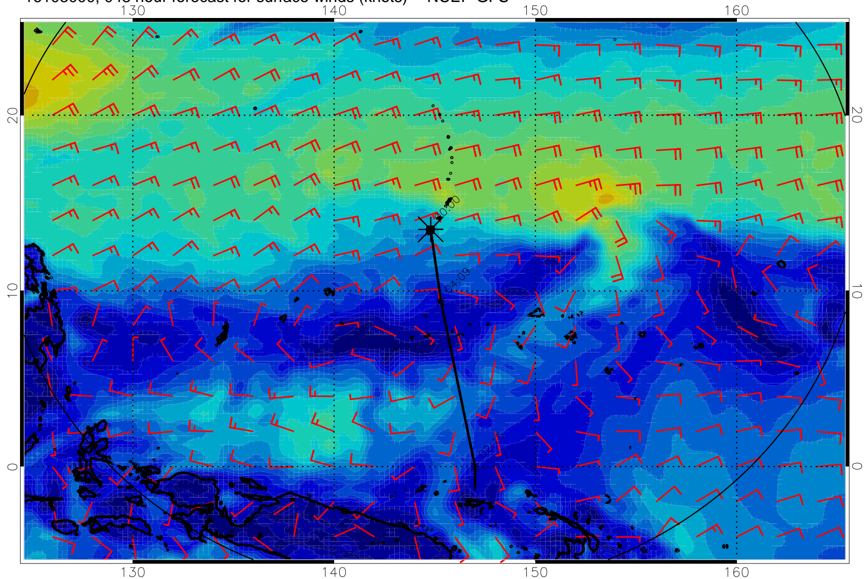
16103000, 048 hour forecast for surface winds (knots) -- NCEP GFS
