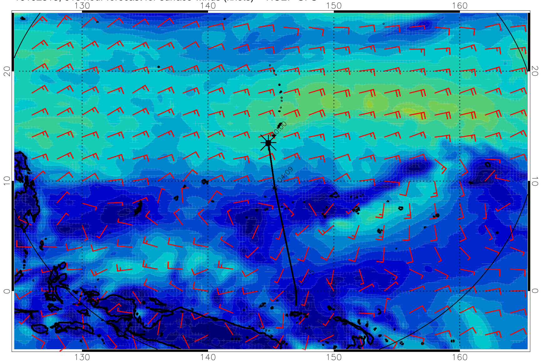
16102818, 018 hour forecast for surface winds (knots) -- NCEP GFS
