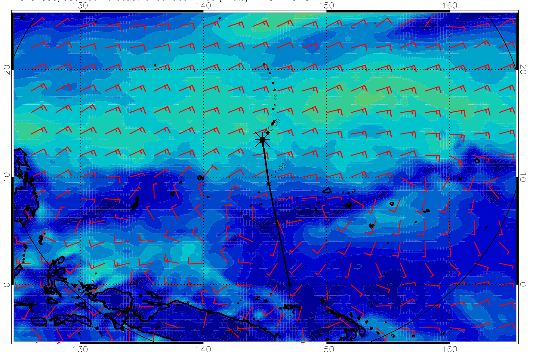
16102806, 006 hour forecast for surface winds (knots) -- NCEP GFS
