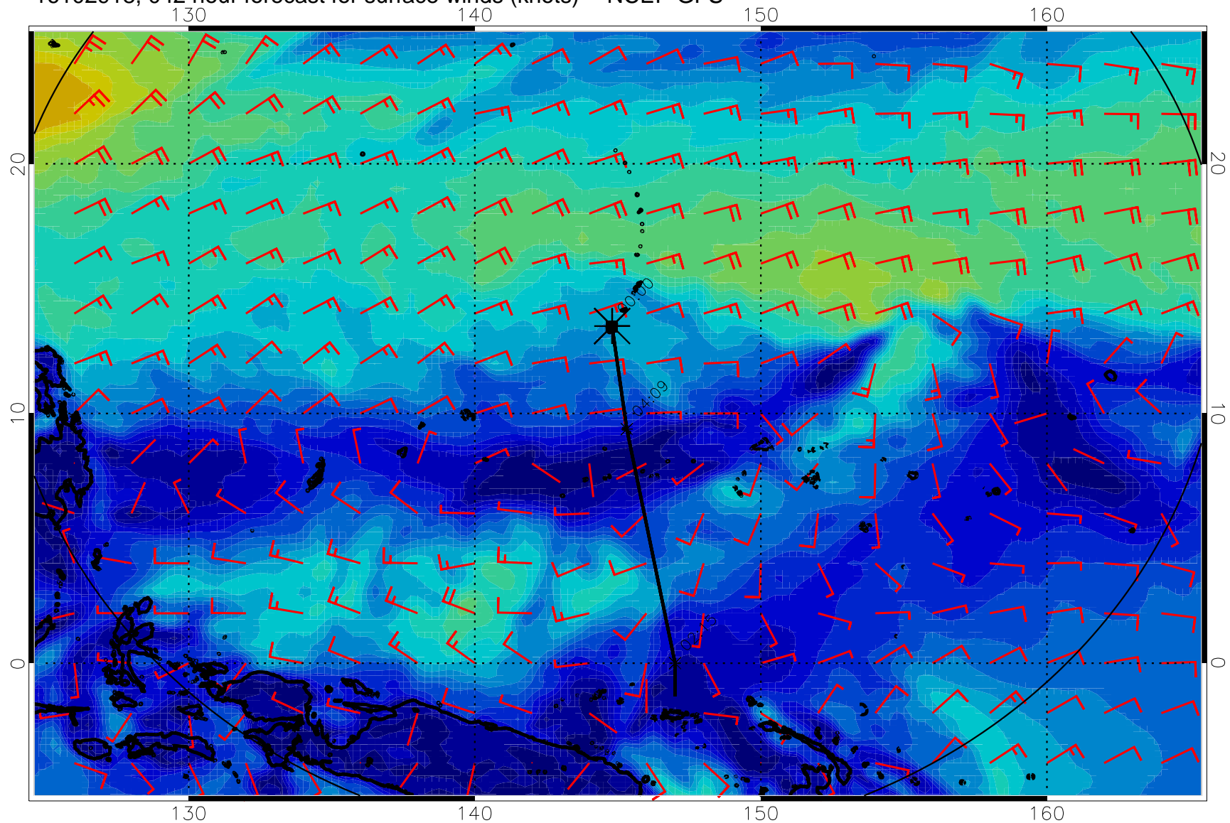
16102918, 042 hour forecast for surface winds (knots) -- NCEP GFS
