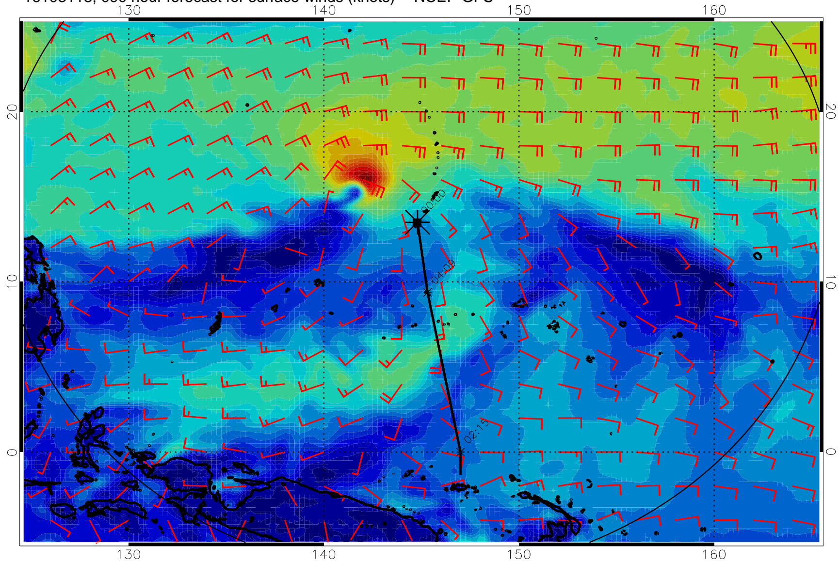
16103118, 090 hour forecast for surface winds (knots) -- NCEP GFS
