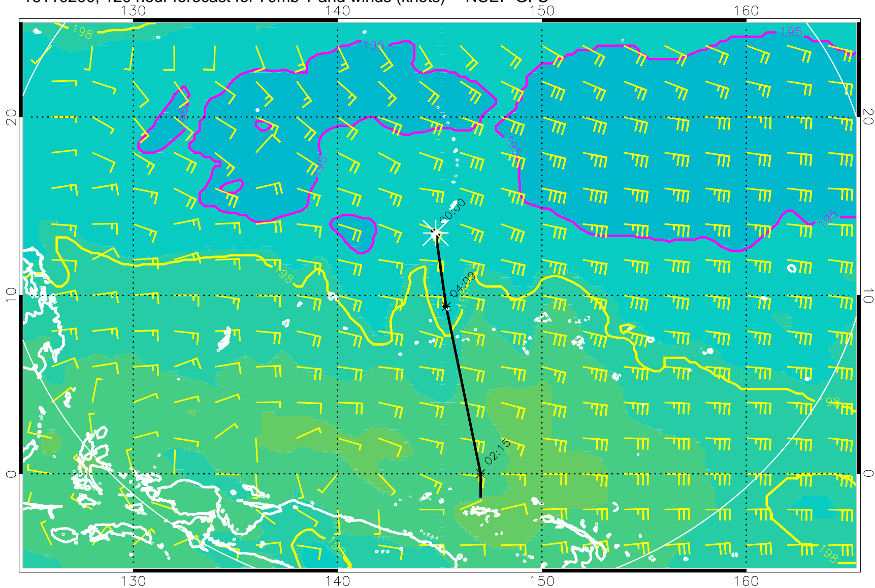
16110200, 120 hour forecast for 70mb T and winds (knots) -- NCEP GFS
