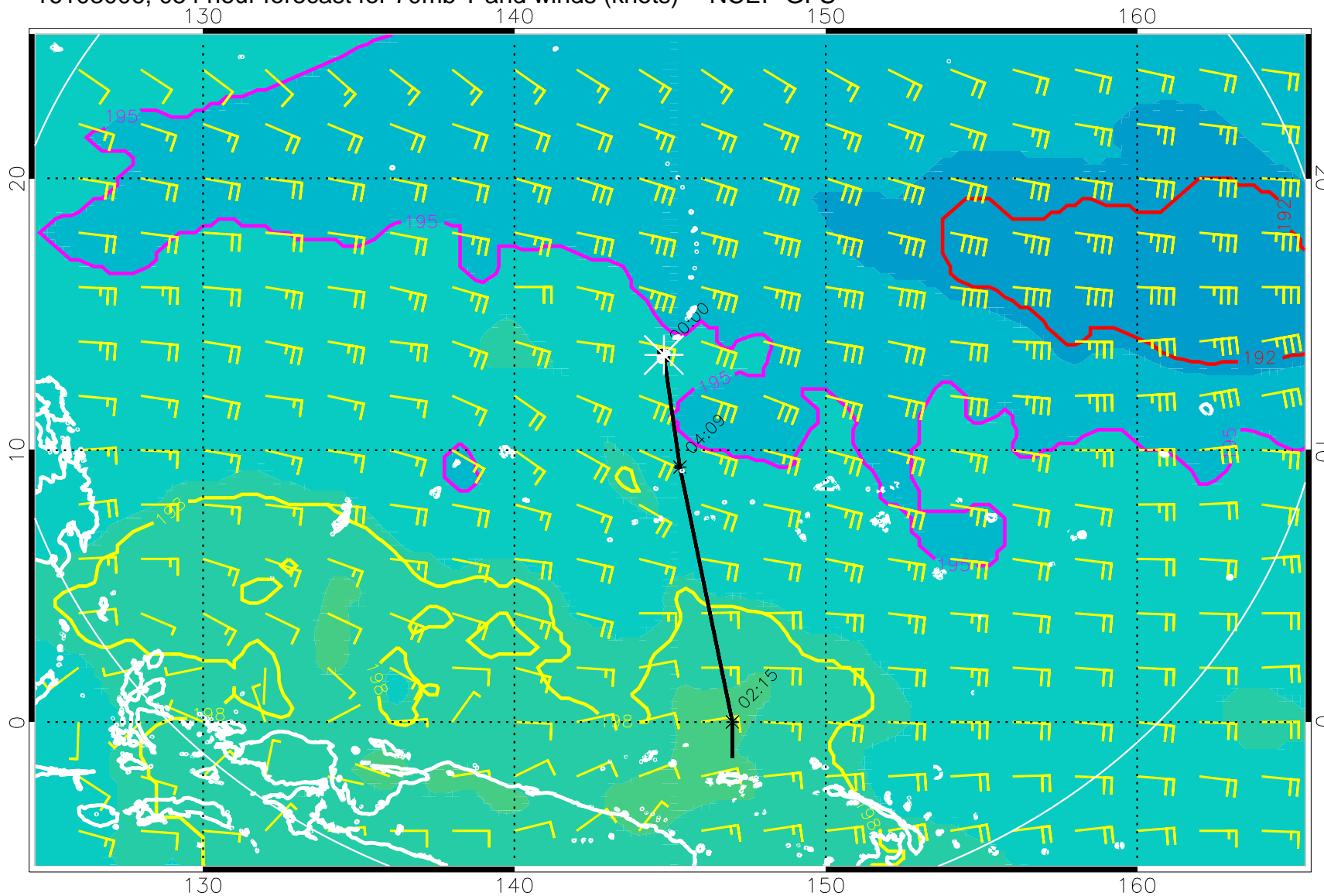
16103006, 054 hour forecast for 70mb T and winds (knots) -- NCEP GFS
