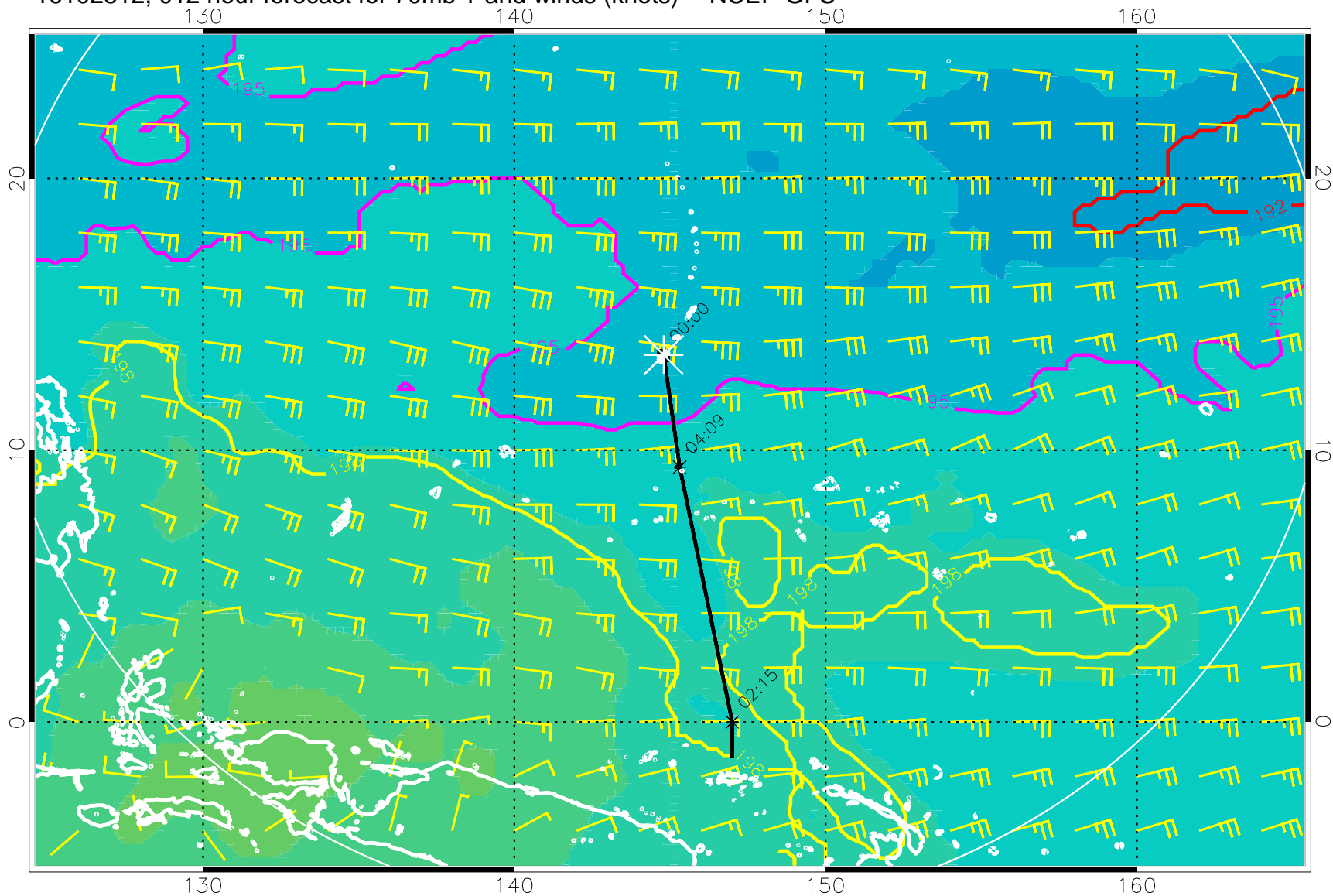
16102812, 012 hour forecast for 70mb T and winds (knots) -- NCEP GFS
