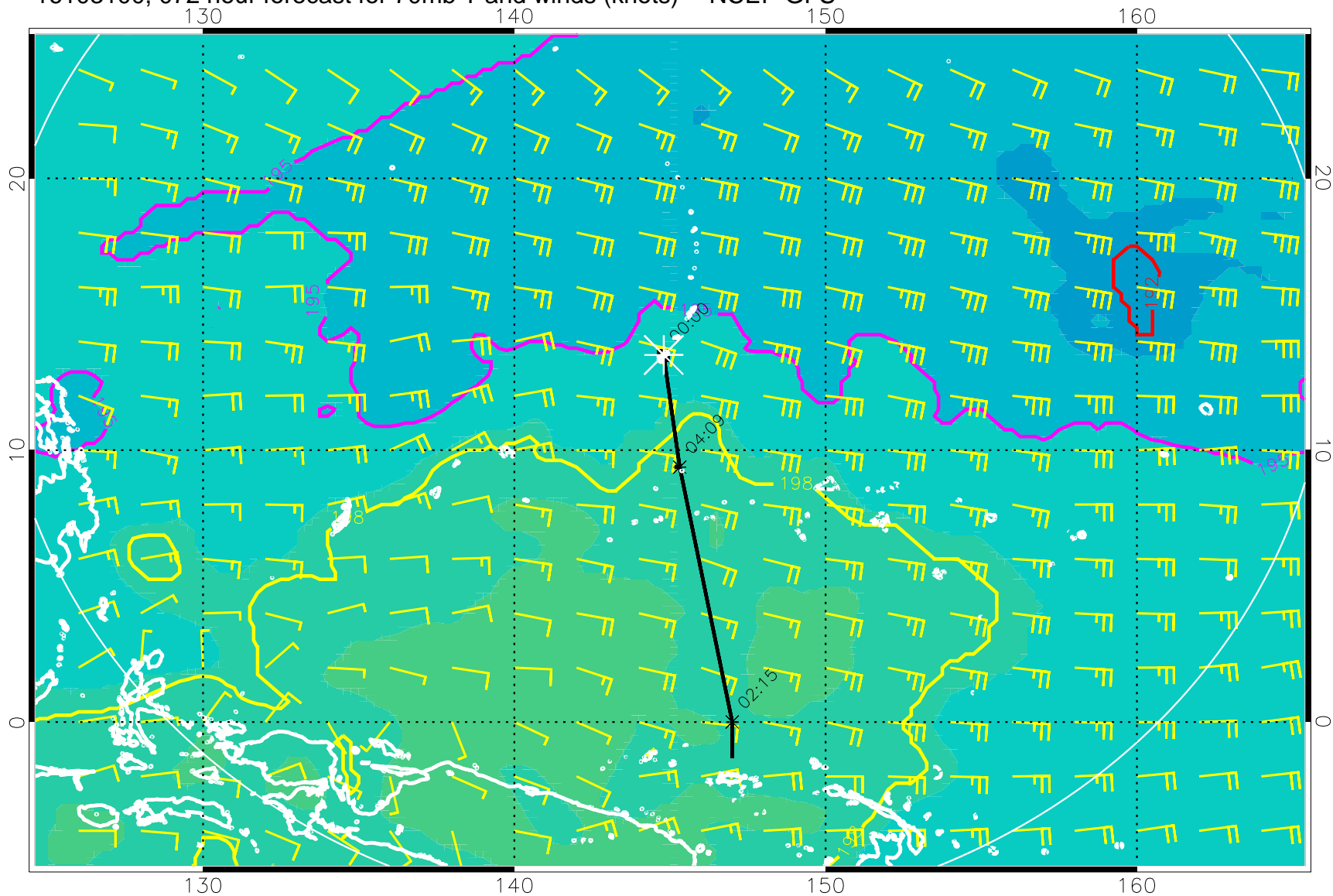
16103100, 072 hour forecast for 70mb T and winds (knots) -- NCEP GFS
