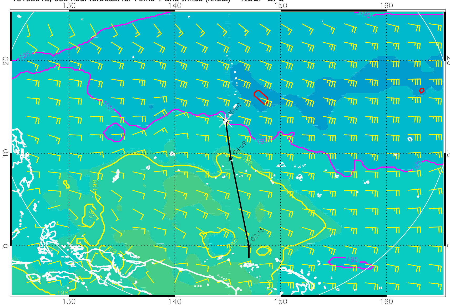
16103018, 066 hour forecast for 70mb T and winds (knots) -- NCEP GFS
