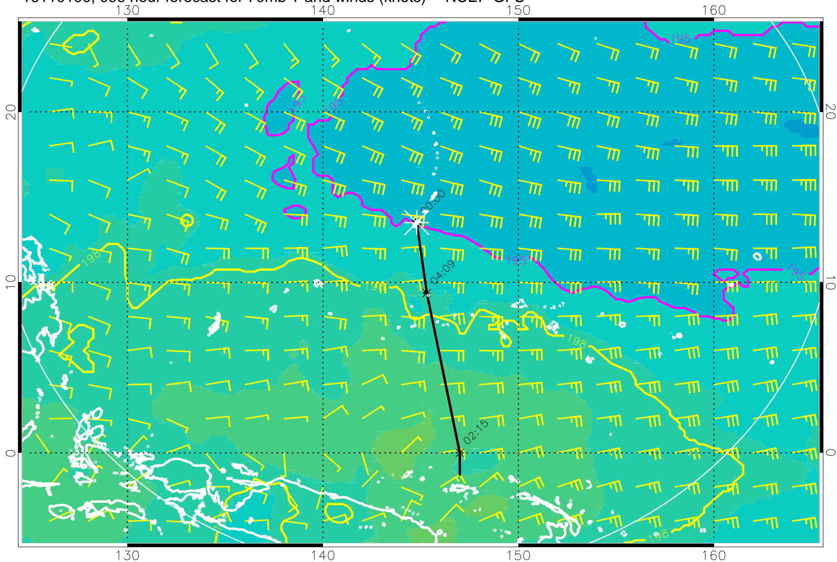
16110100, 096 hour forecast for 70mb T and winds (knots) -- NCEP GFS
