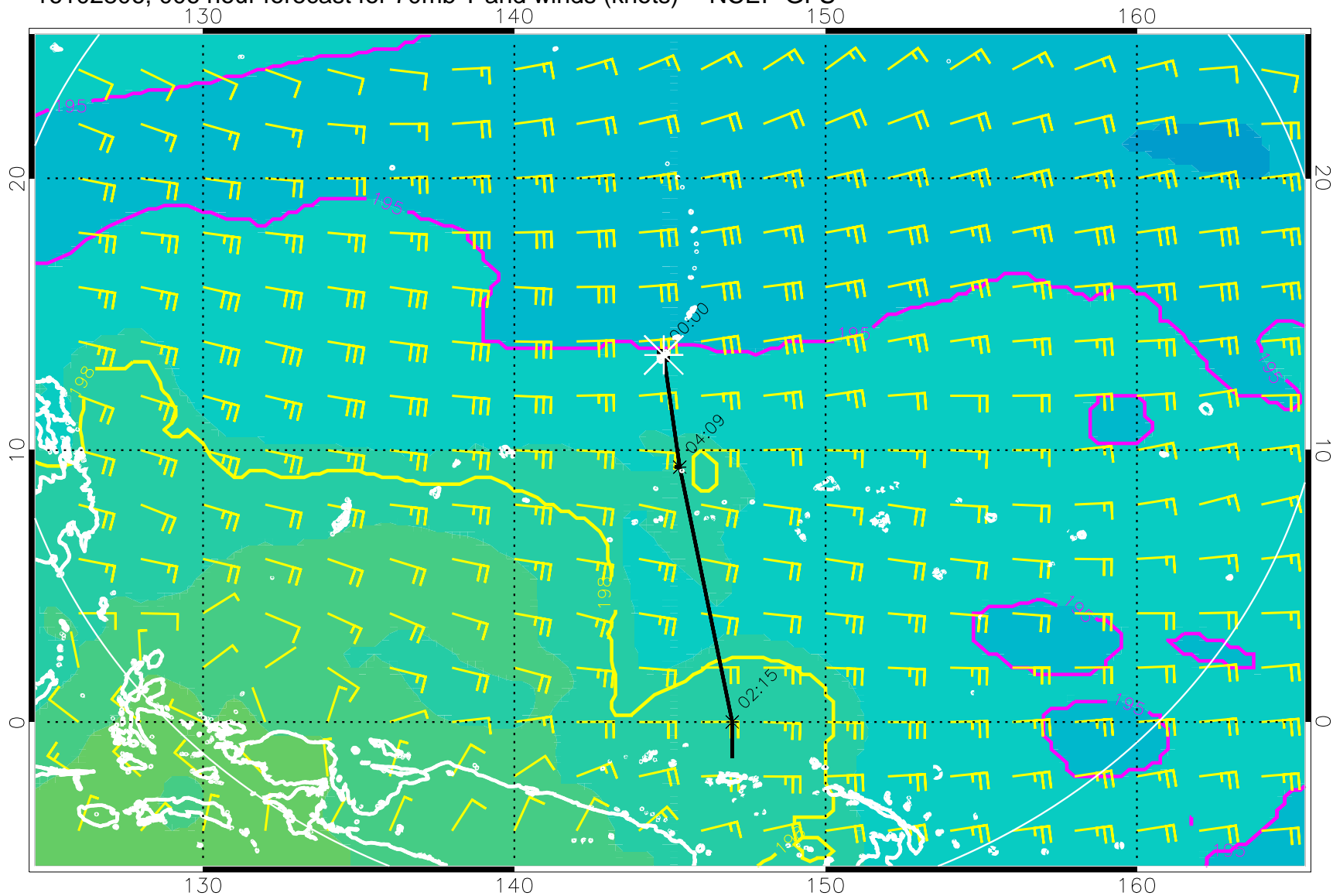
16102806, 006 hour forecast for 70mb T and winds (knots) -- NCEP GFS
