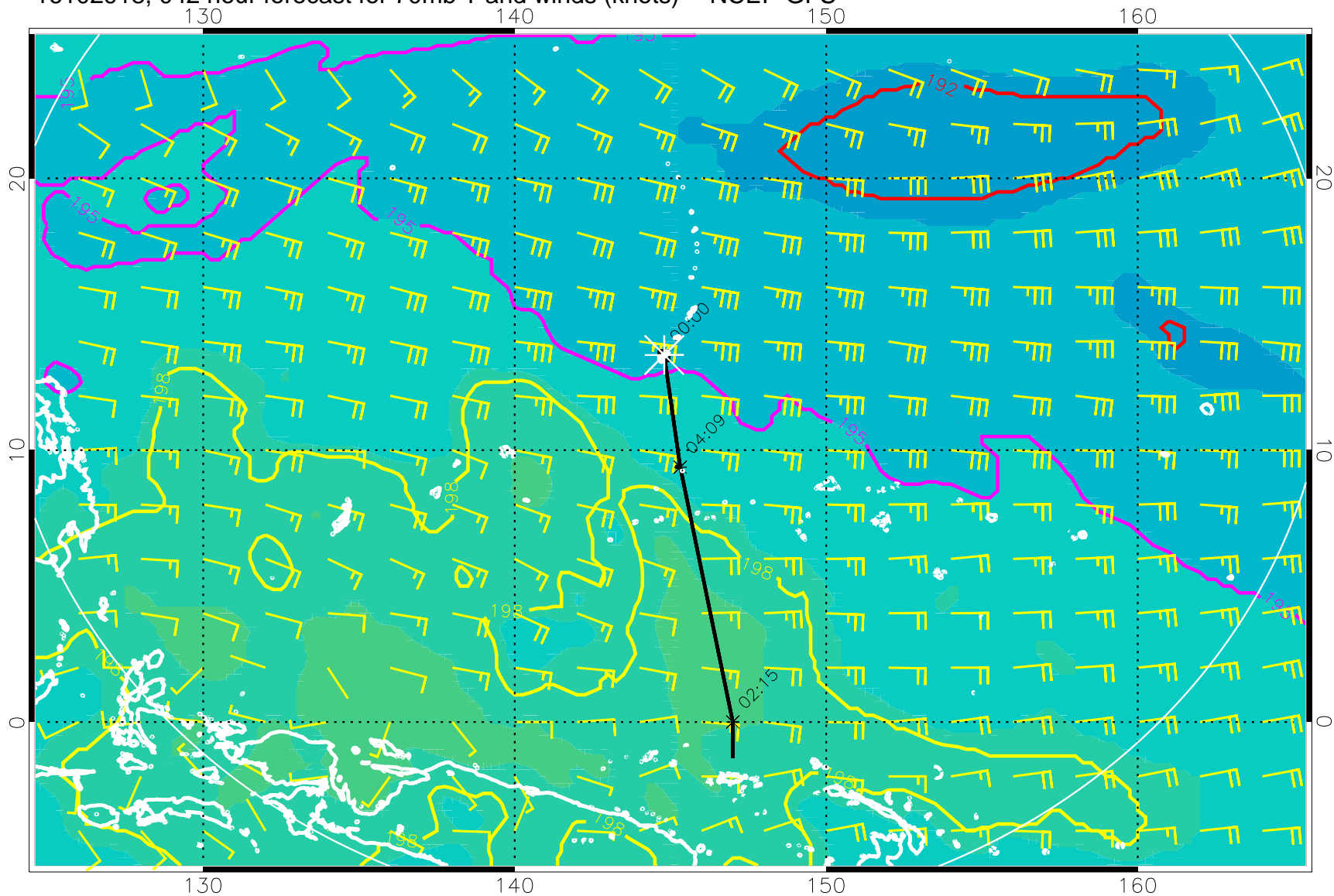
16102918, 042 hour forecast for 70mb T and winds (knots) -- NCEP GFS
