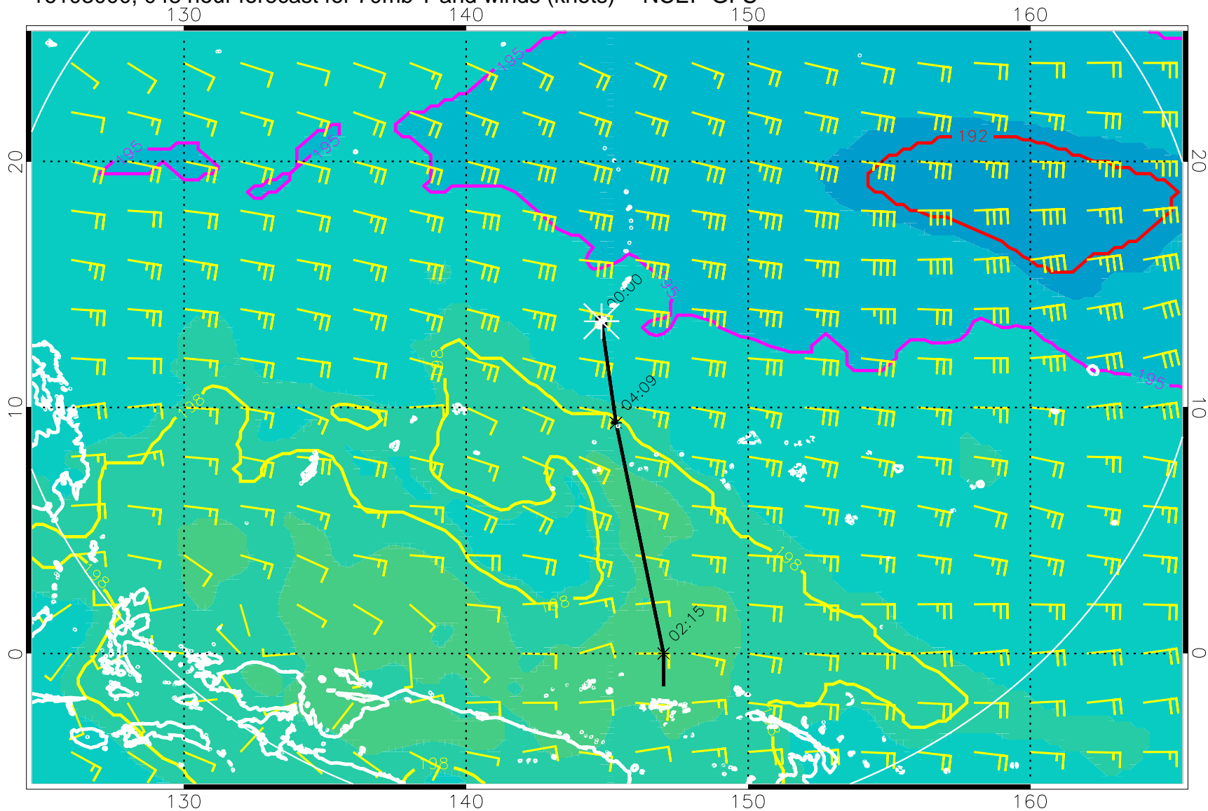
16103000, 048 hour forecast for 70mb T and winds (knots) -- NCEP GFS
