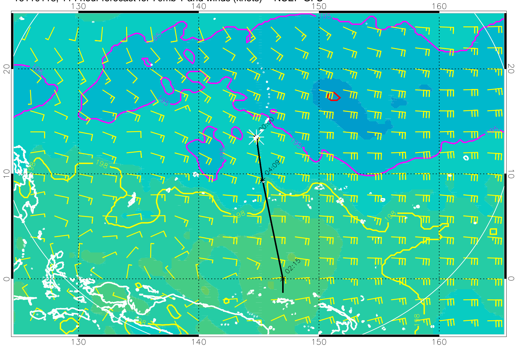
16110118, 114 hour forecast for 70mb T and winds (knots) -- NCEP GFS
