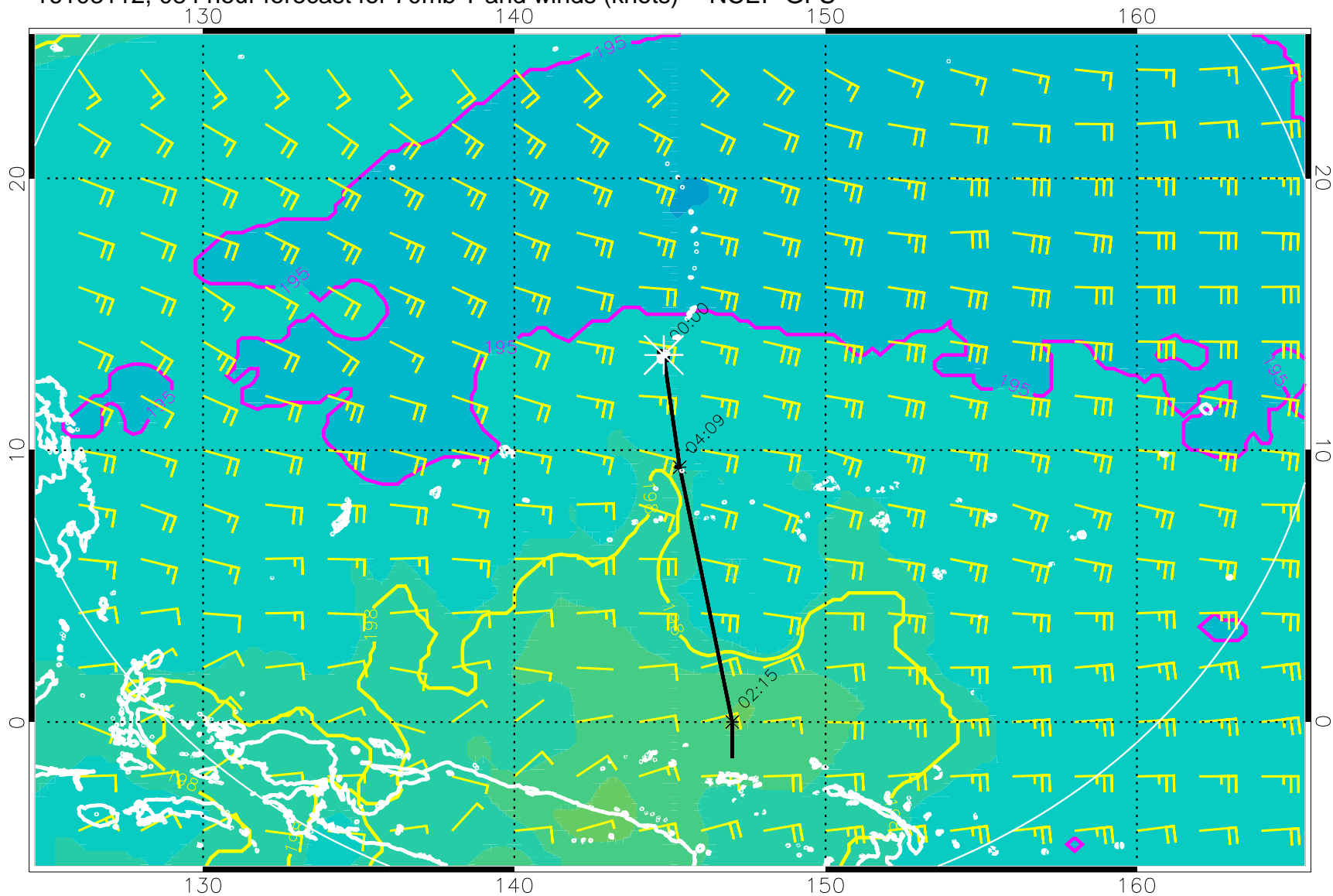
16103112, 084 hour forecast for 70mb T and winds (knots) -- NCEP GFS
