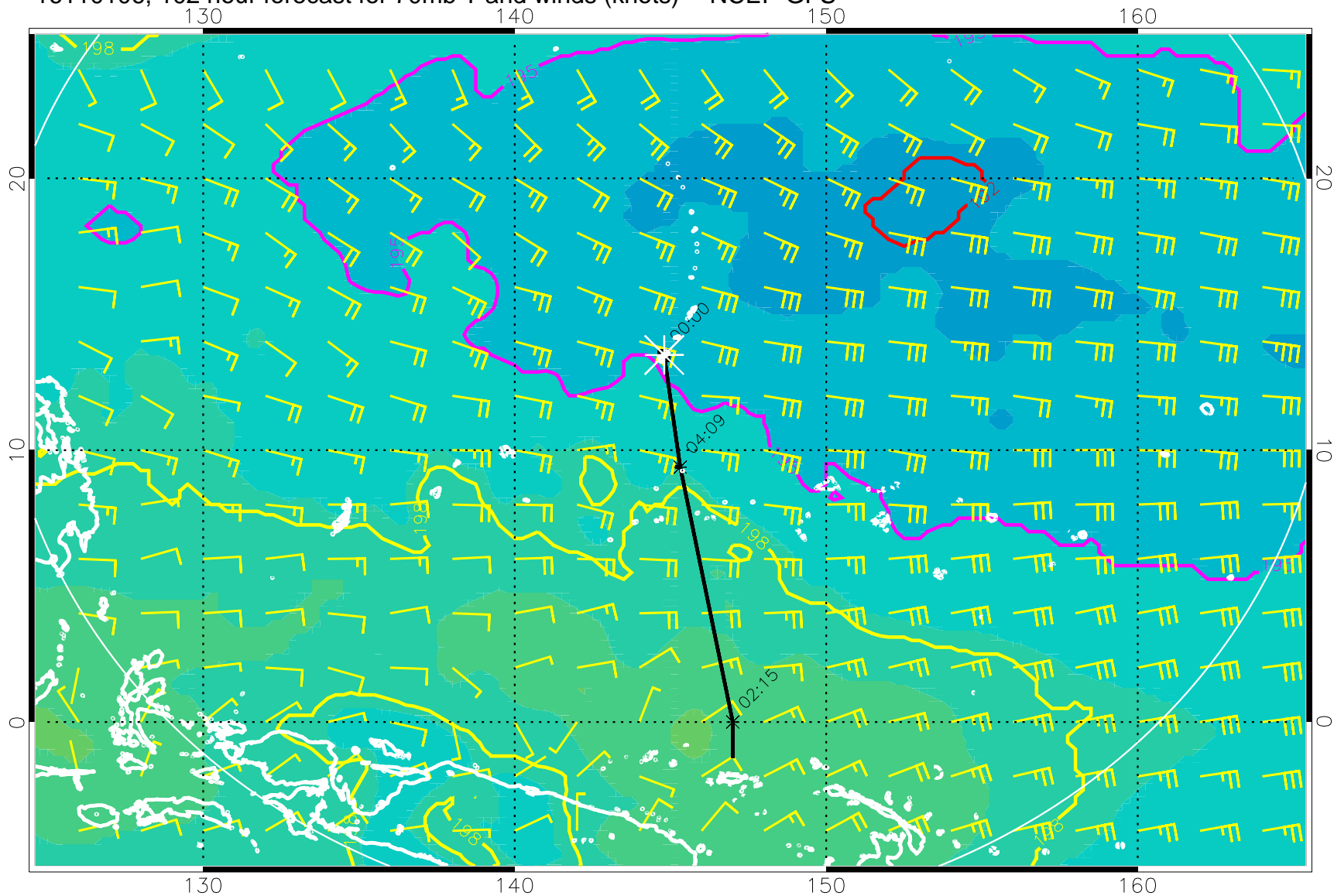
16110106, 102 hour forecast for 70mb T and winds (knots) -- NCEP GFS
