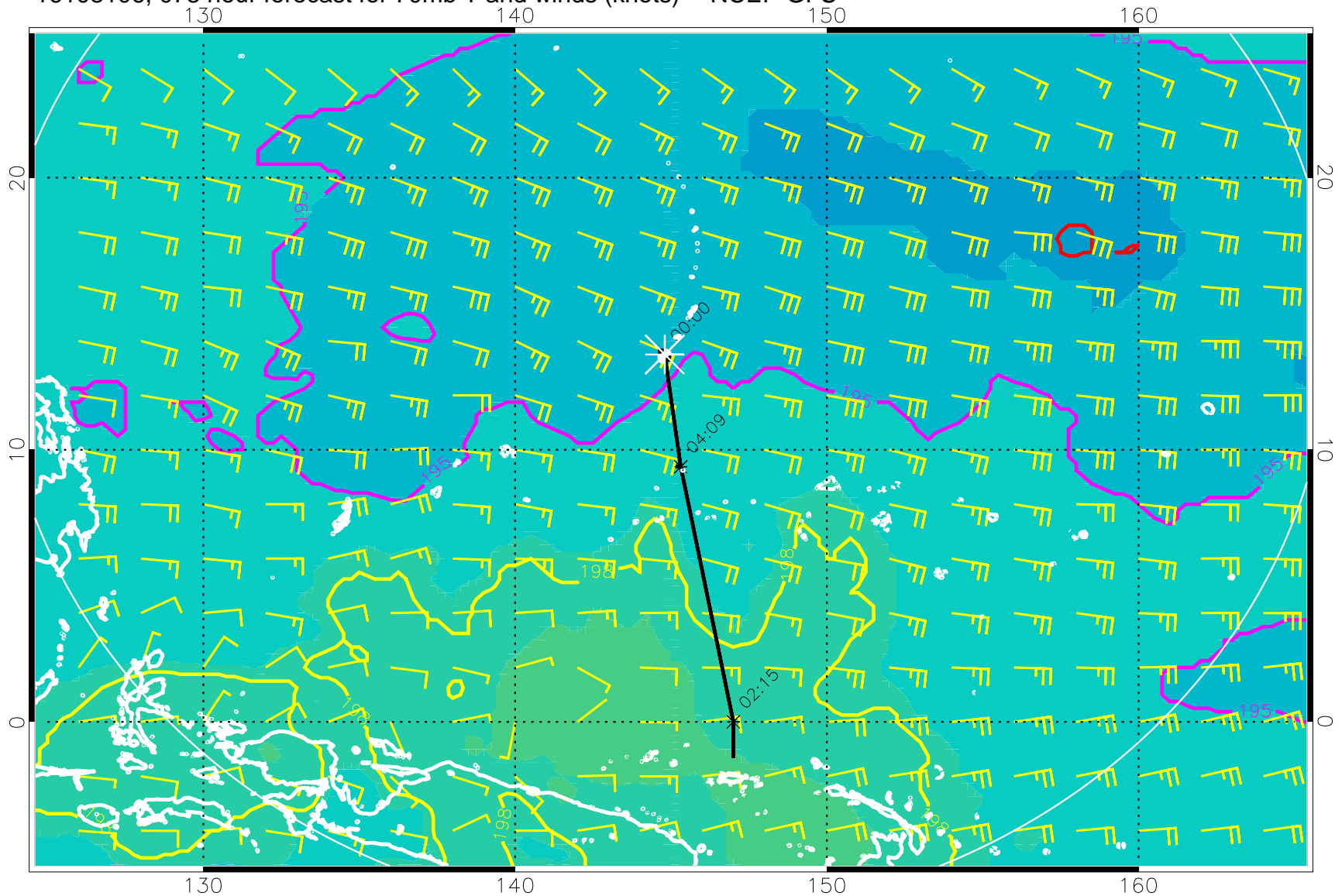
16103106, 078 hour forecast for 70mb T and winds (knots) -- NCEP GFS
