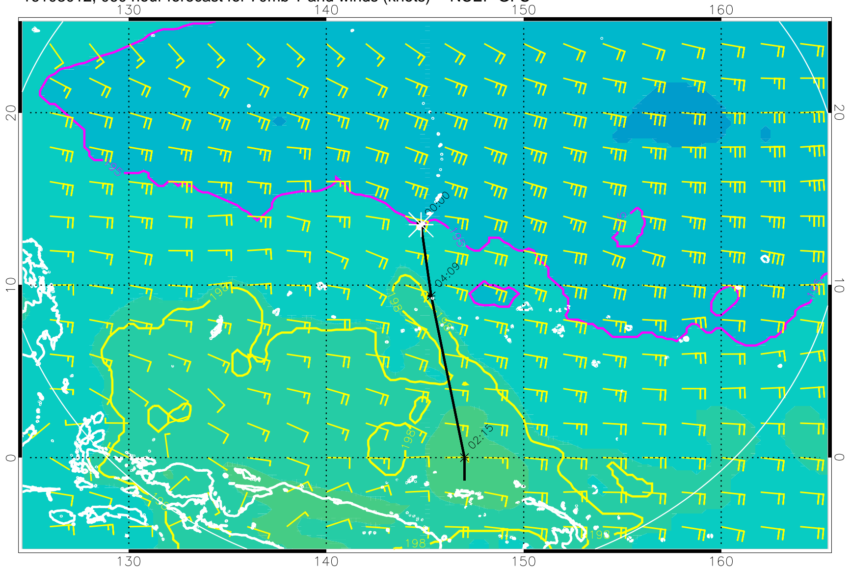
16103012, 060 hour forecast for 70mb T and winds (knots) -- NCEP GFS
