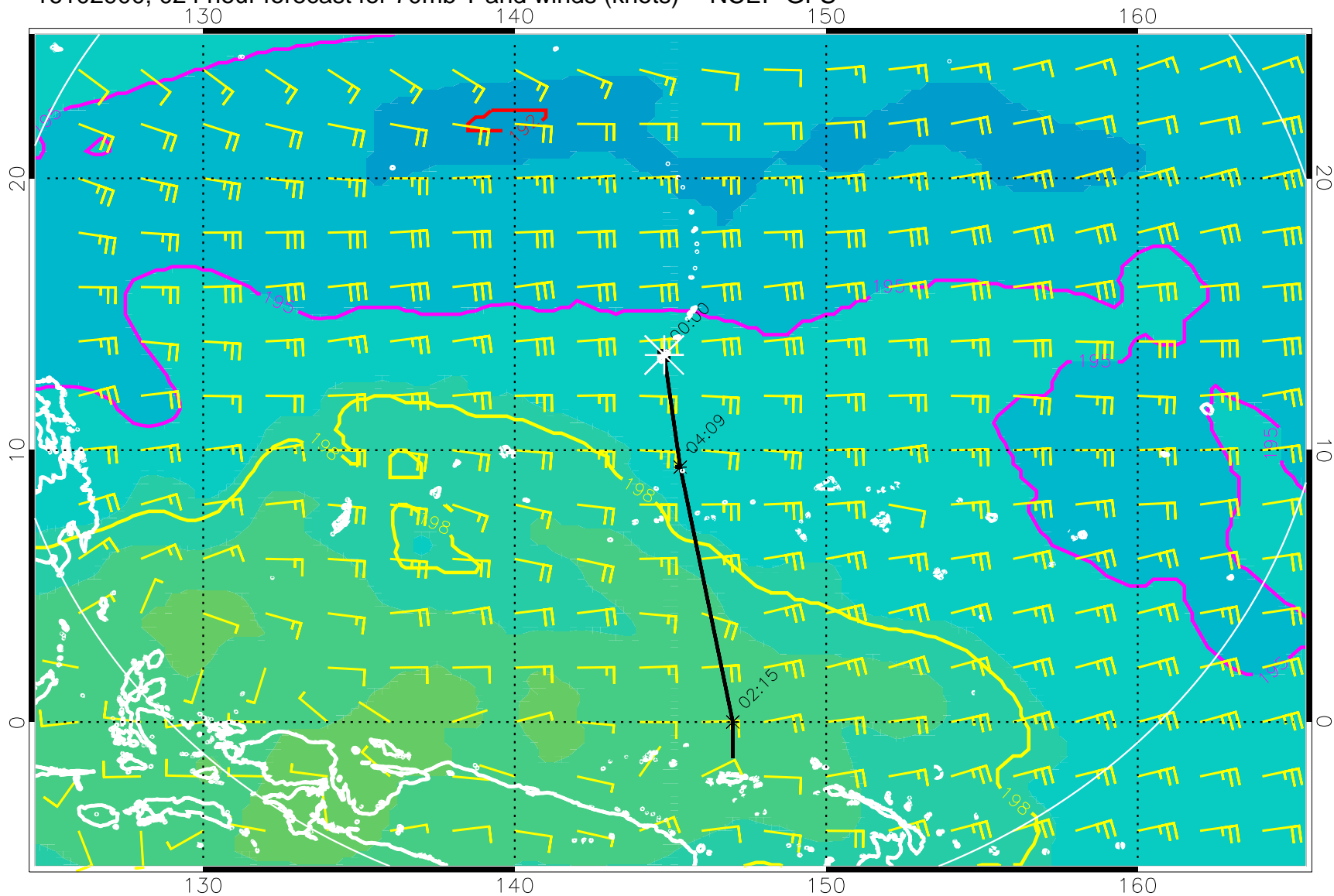
16102900, 024 hour forecast for 70mb T and winds (knots) -- NCEP GFS
