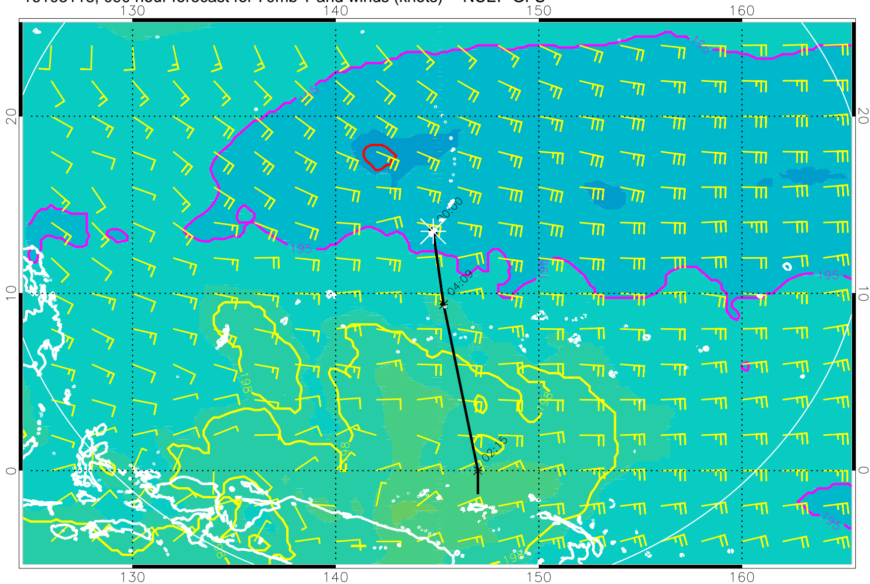
16103118, 090 hour forecast for 70mb T and winds (knots) -- NCEP GFS
