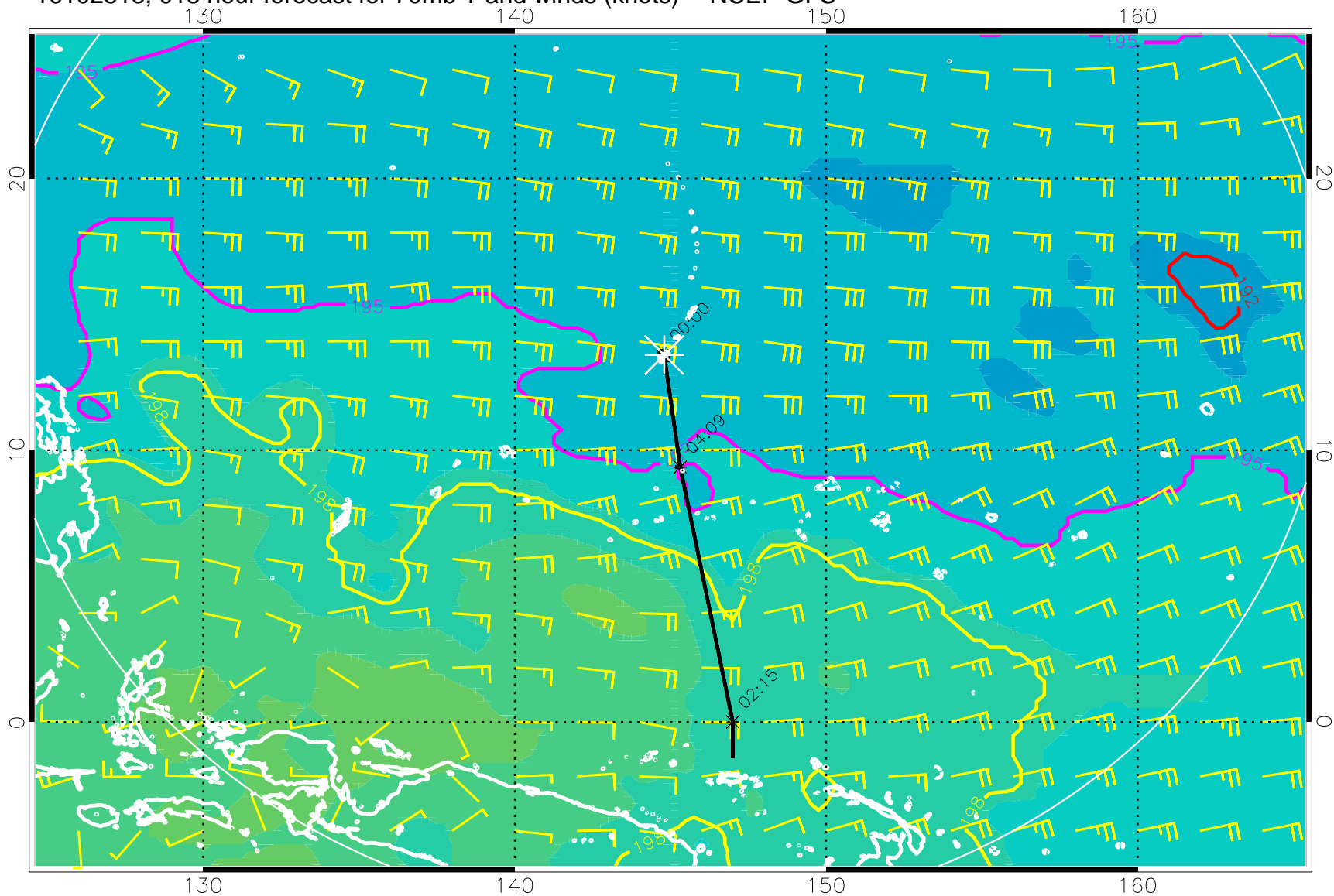
16102818, 018 hour forecast for 70mb T and winds (knots) -- NCEP GFS
