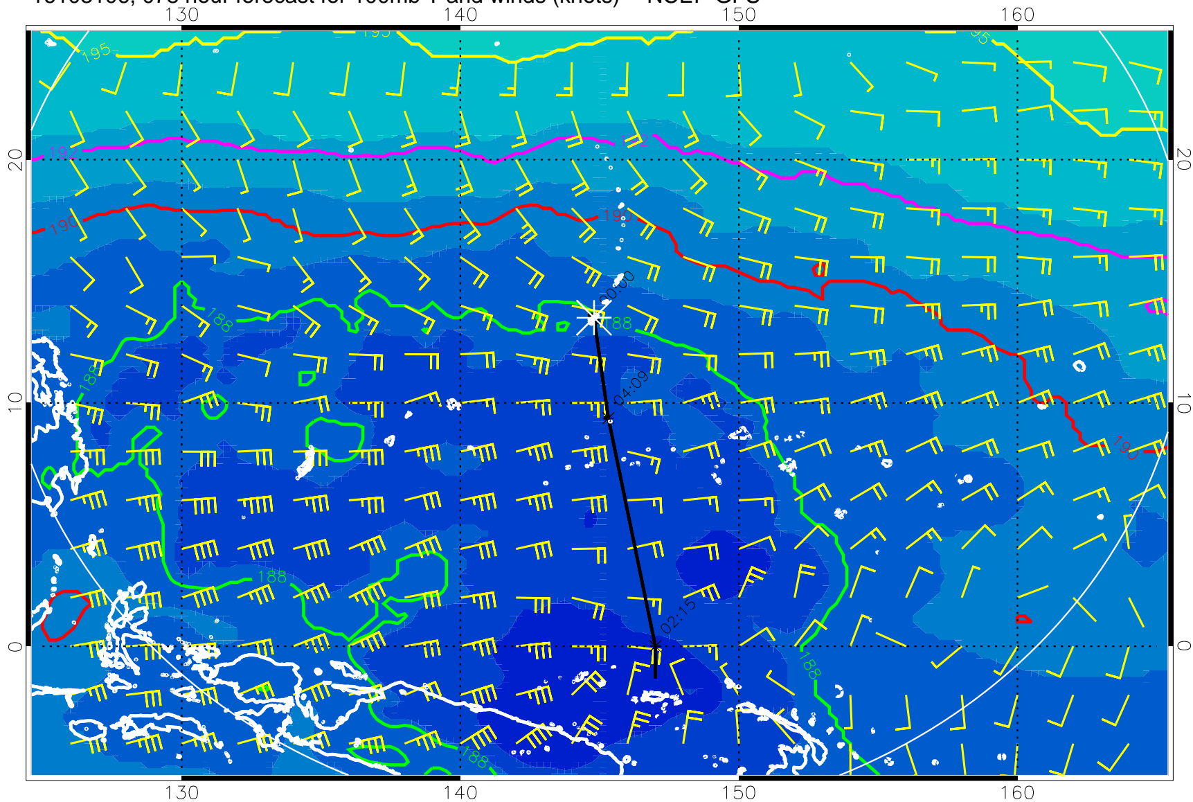
16103106, 078 hour forecast for 100mb T and winds (knots) -- NCEP GFS
