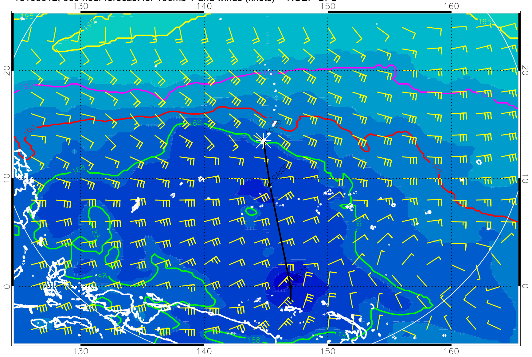
16103012, 060 hour forecast for 100mb T and winds (knots) -- NCEP GFS
