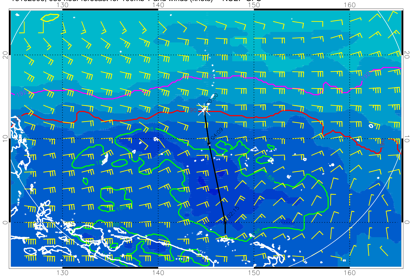
16102906, 030 hour forecast for 100mb T and winds (knots) -- NCEP GFS
