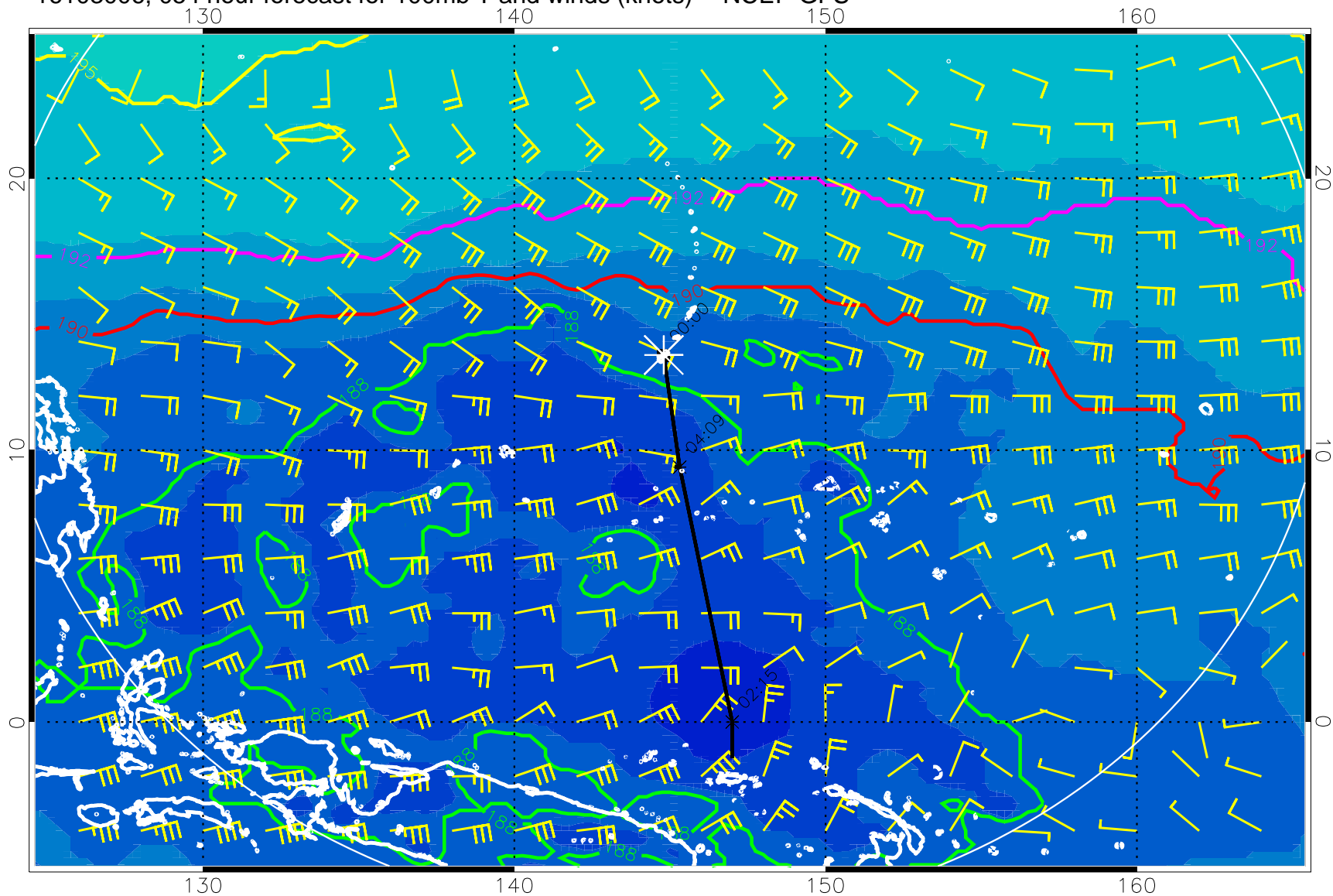
16103006, 054 hour forecast for 100mb T and winds (knots) -- NCEP GFS
