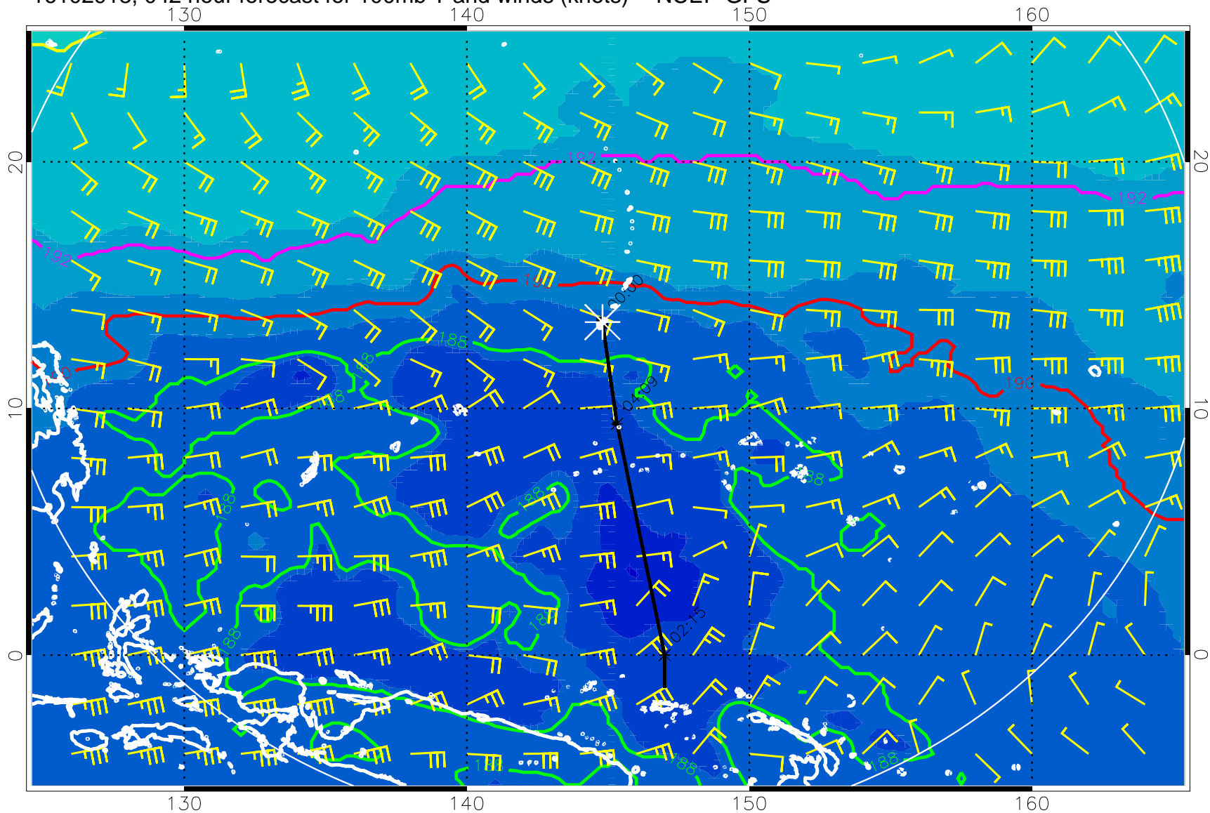
16102918, 042 hour forecast for 100mb T and winds (knots) -- NCEP GFS
