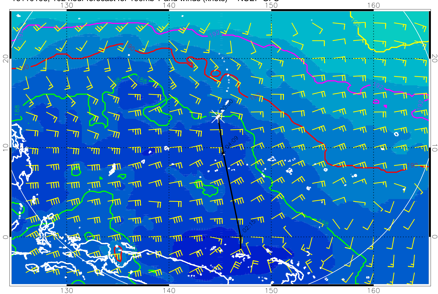
16110106, 102 hour forecast for 100mb T and winds (knots) -- NCEP GFS
