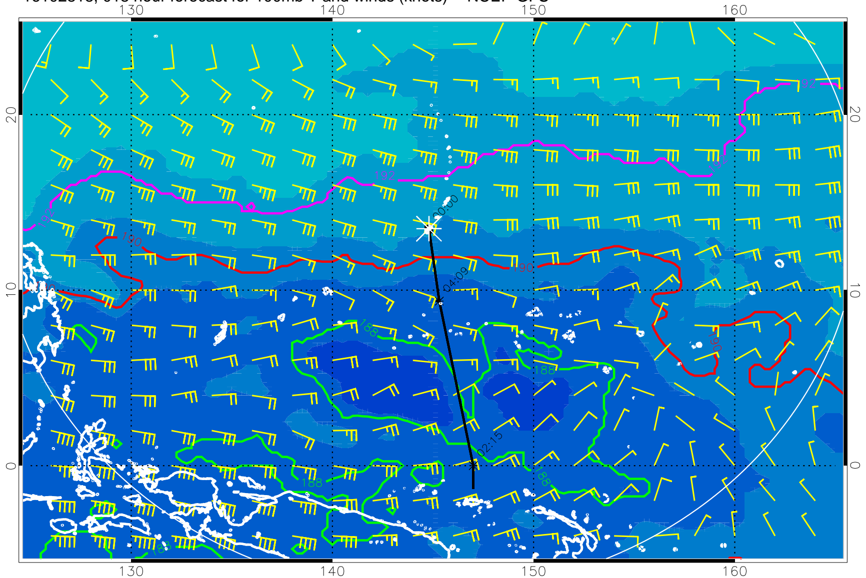
16102818, 018 hour forecast for 100mb T and winds (knots) -- NCEP GFS
