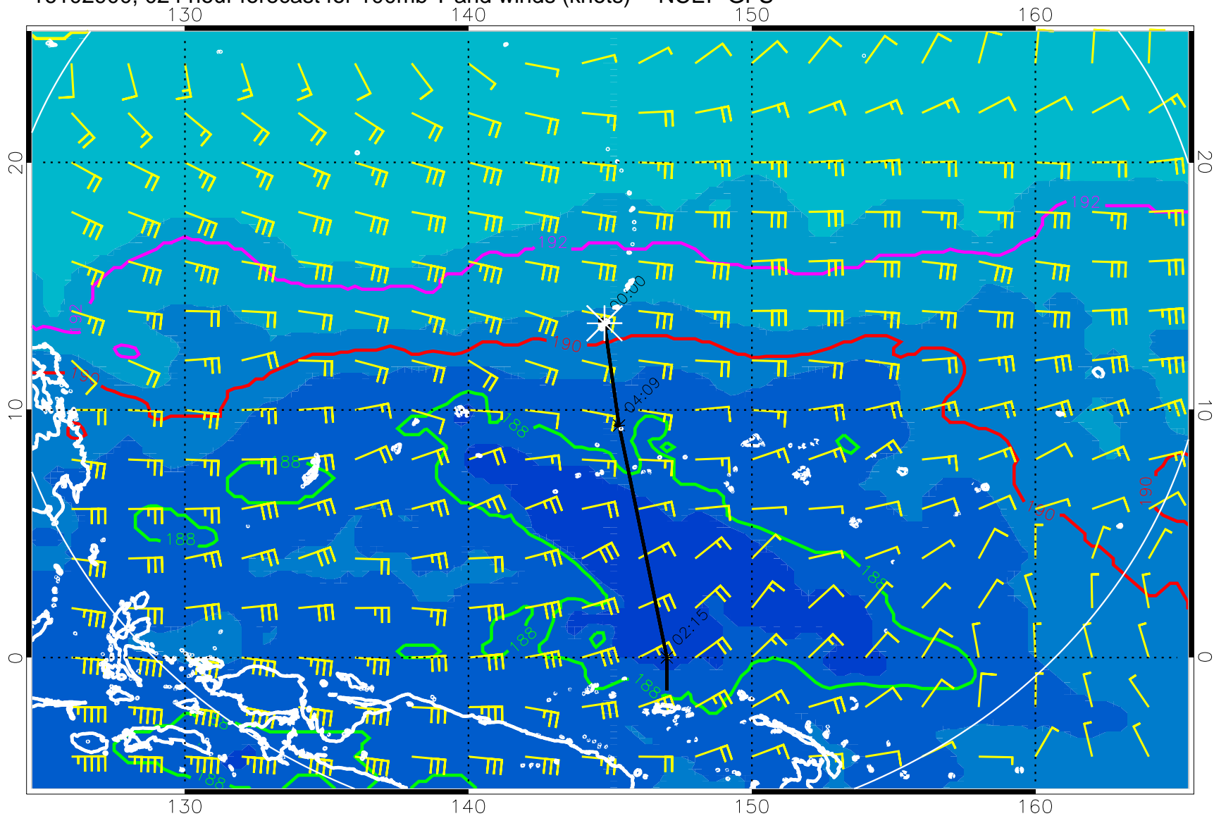
16102900, 024 hour forecast for 100mb T and winds (knots) -- NCEP GFS
