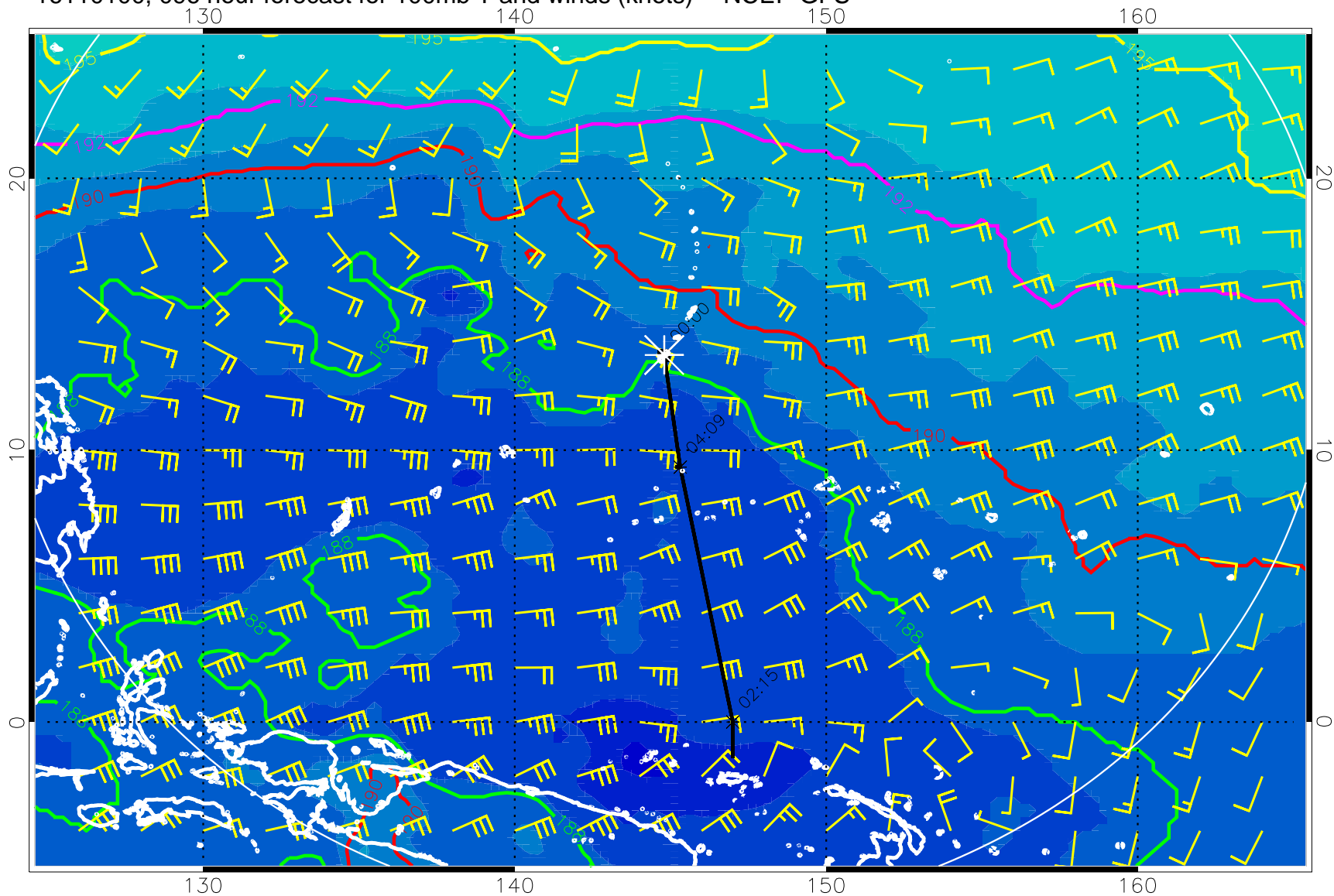
16110100, 096 hour forecast for 100mb T and winds (knots) -- NCEP GFS
