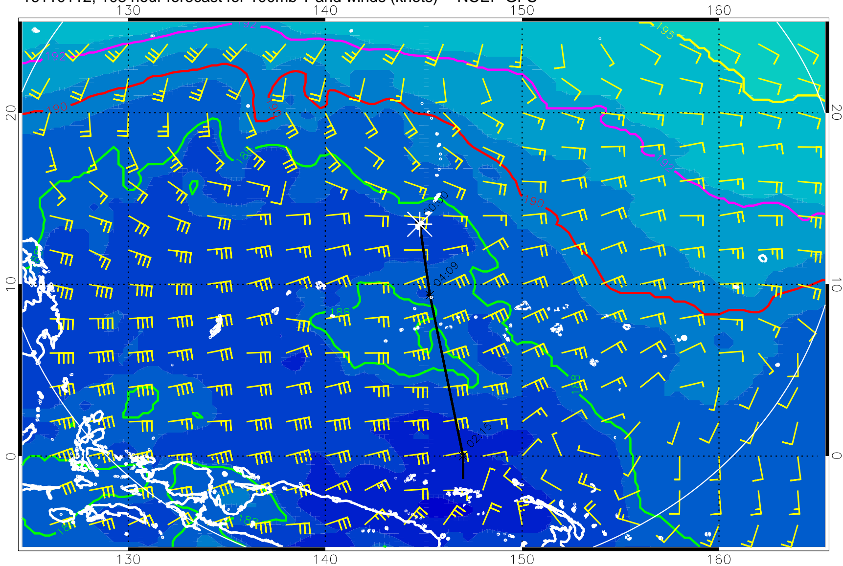
16110112, 108 hour forecast for 100mb T and winds (knots) -- NCEP GFS
