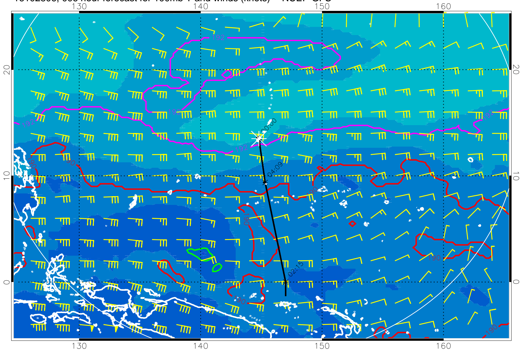
16102806, 006 hour forecast for 100mb T and winds (knots) -- NCEP GFS
