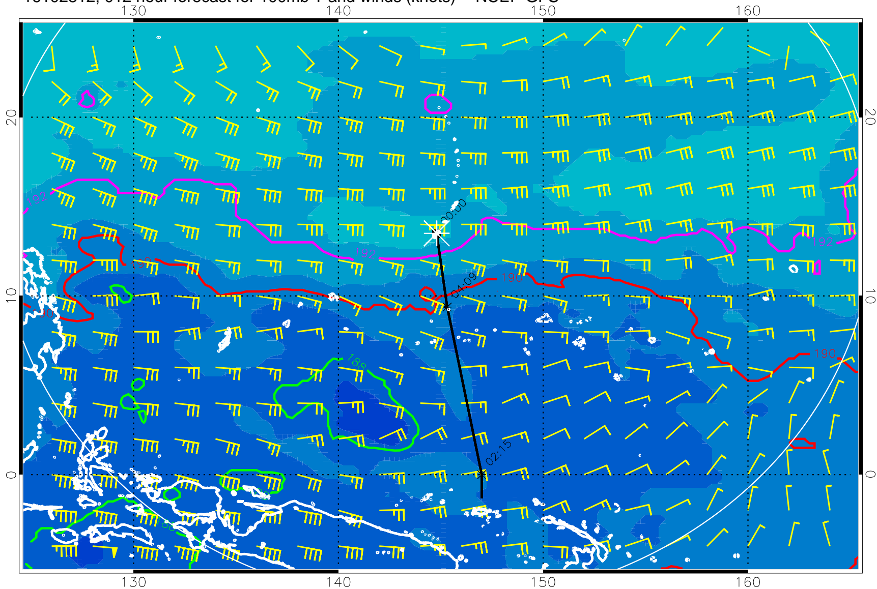
16102812, 012 hour forecast for 100mb T and winds (knots) -- NCEP GFS
