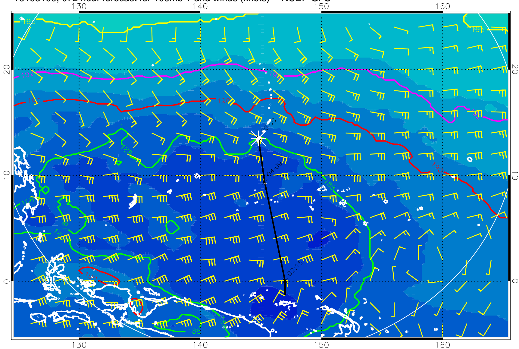
16103100, 072 hour forecast for 100mb T and winds (knots) -- NCEP GFS
