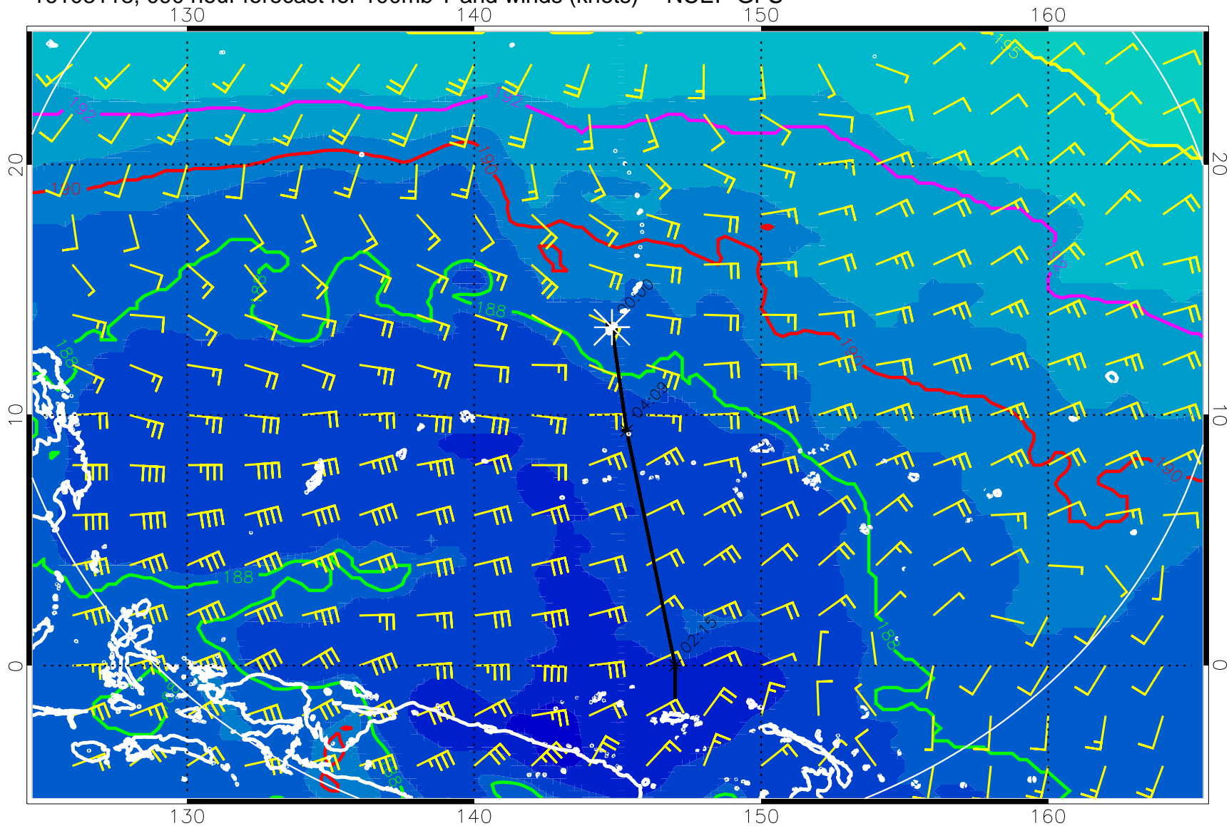
16103118, 090 hour forecast for 100mb T and winds (knots) -- NCEP GFS
