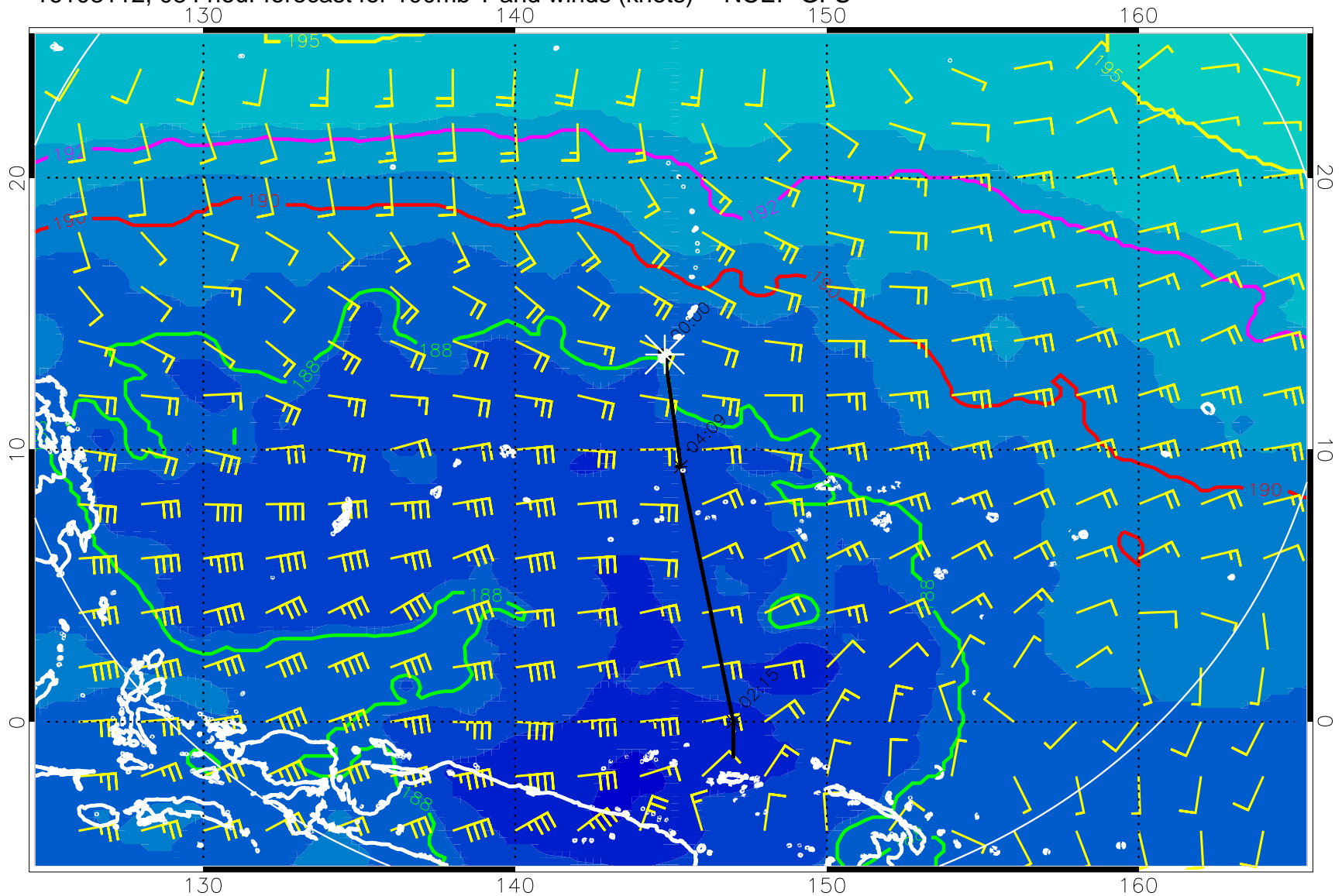
16103112, 084 hour forecast for 100mb T and winds (knots) -- NCEP GFS
