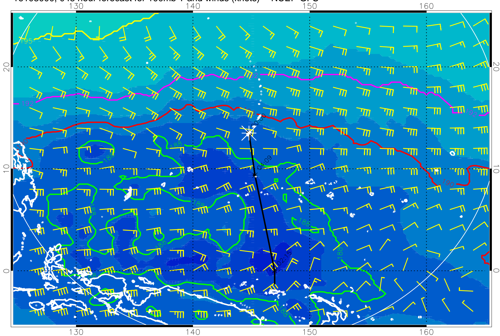
16103000, 048 hour forecast for 100mb T and winds (knots) -- NCEP GFS
