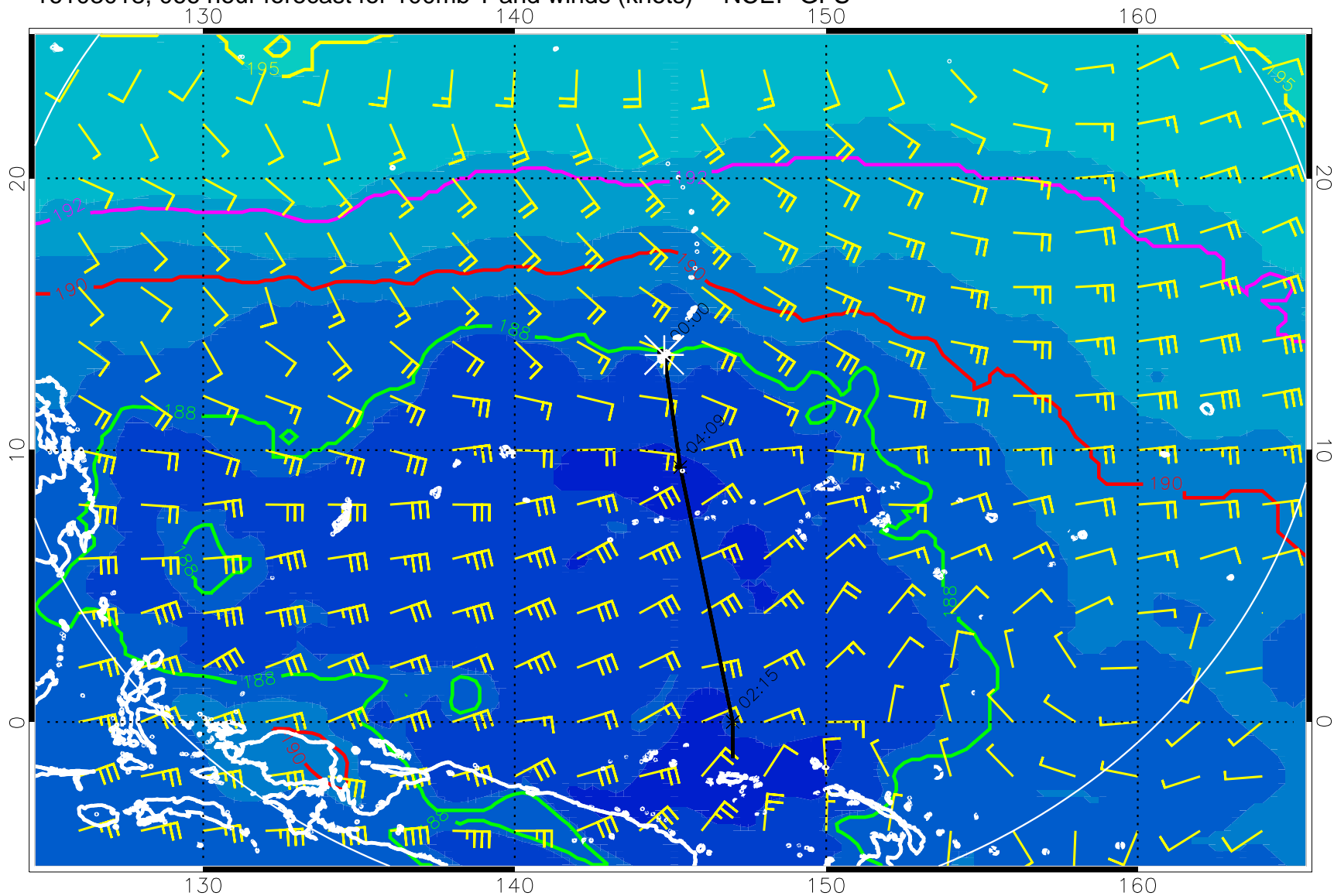
16103018, 066 hour forecast for 100mb T and winds (knots) -- NCEP GFS
