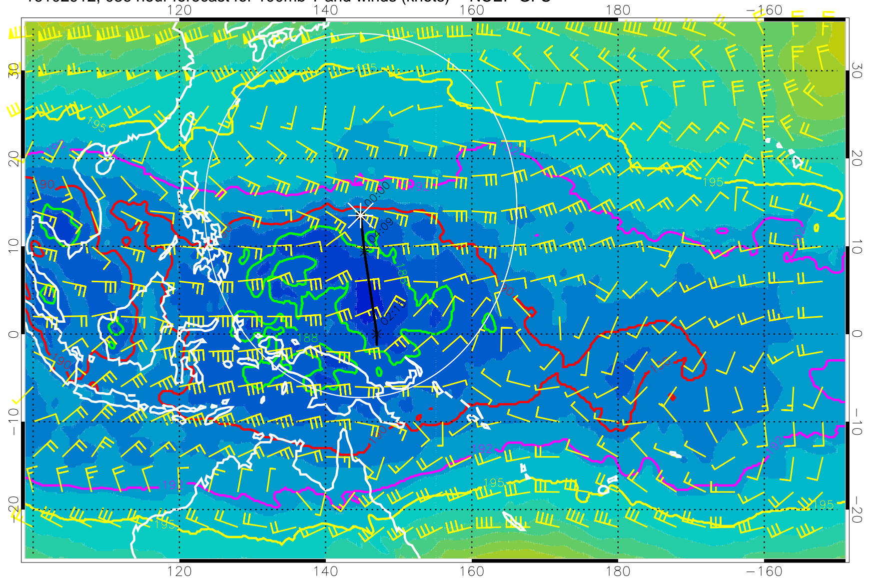
16102912, 036 hour forecast for 100mb T and winds (knots) -- NCEP GFS
