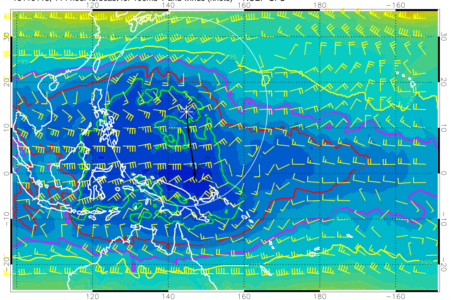
16110118, 114 hour forecast for 100mb T and winds (knots) -- NCEP GFS
