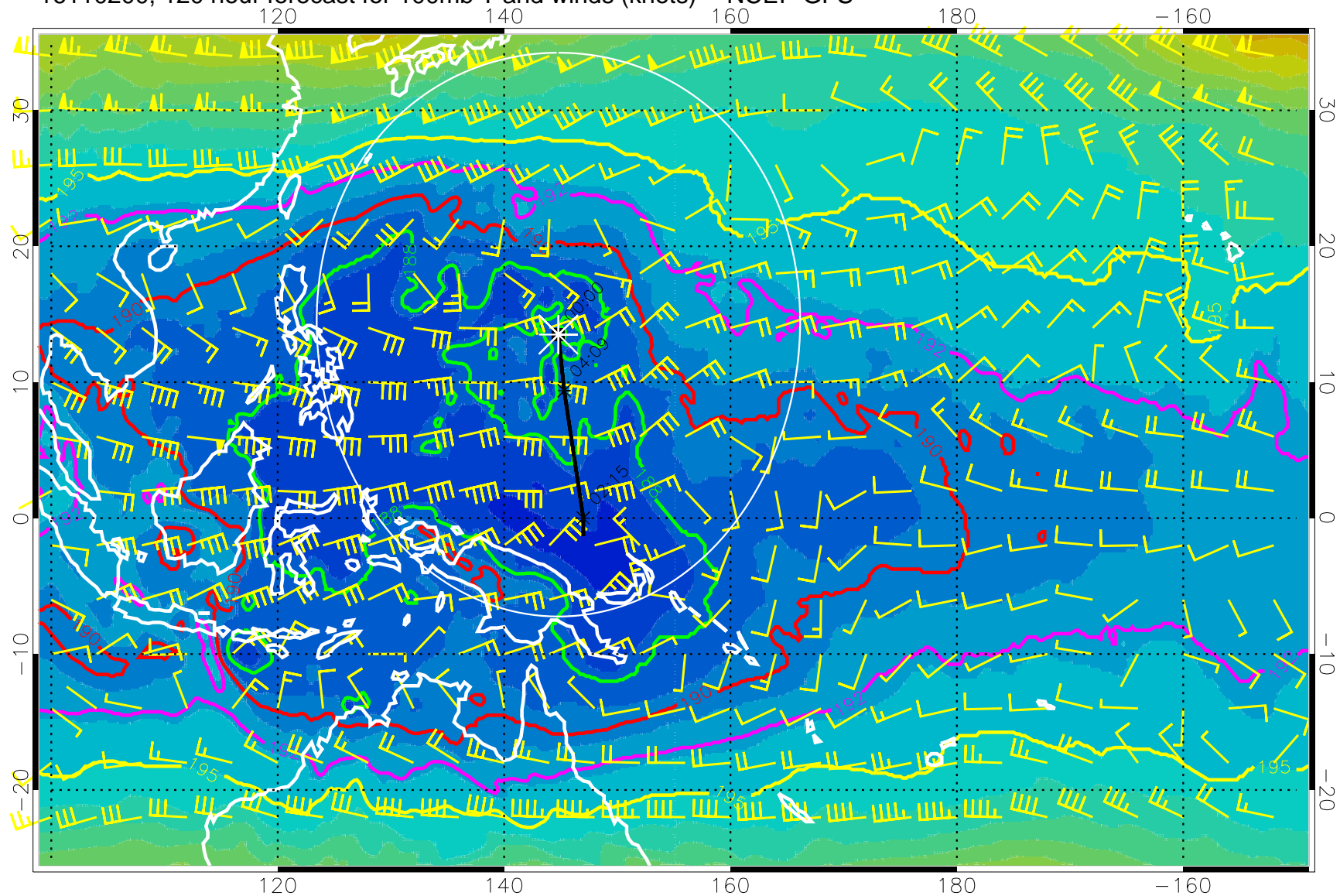
16110200, 120 hour forecast for 100mb T and winds (knots) -- NCEP GFS
