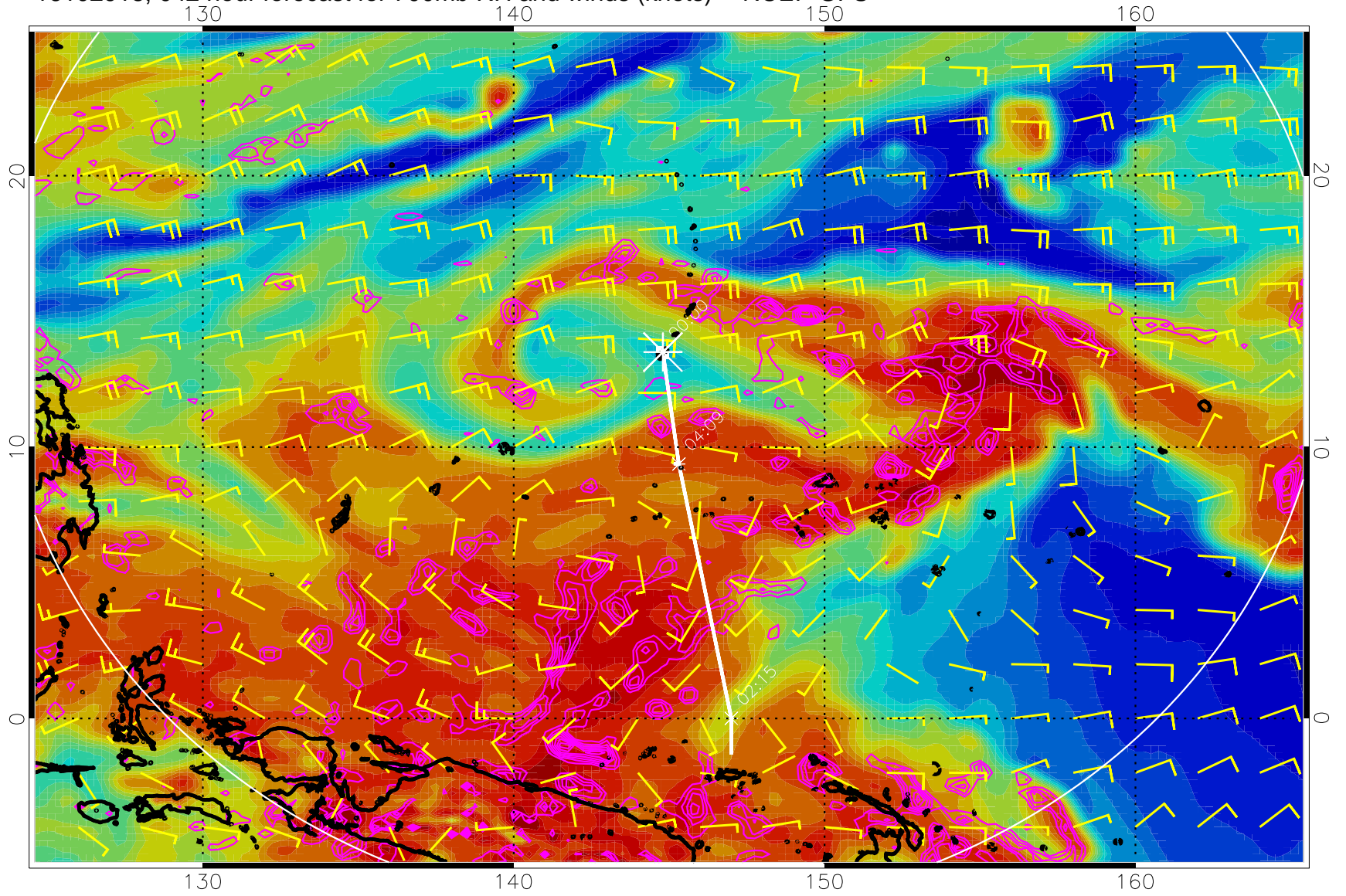
16102918, 042 hour forecast for 700mb RH and winds (knots) -- NCEP GFS
