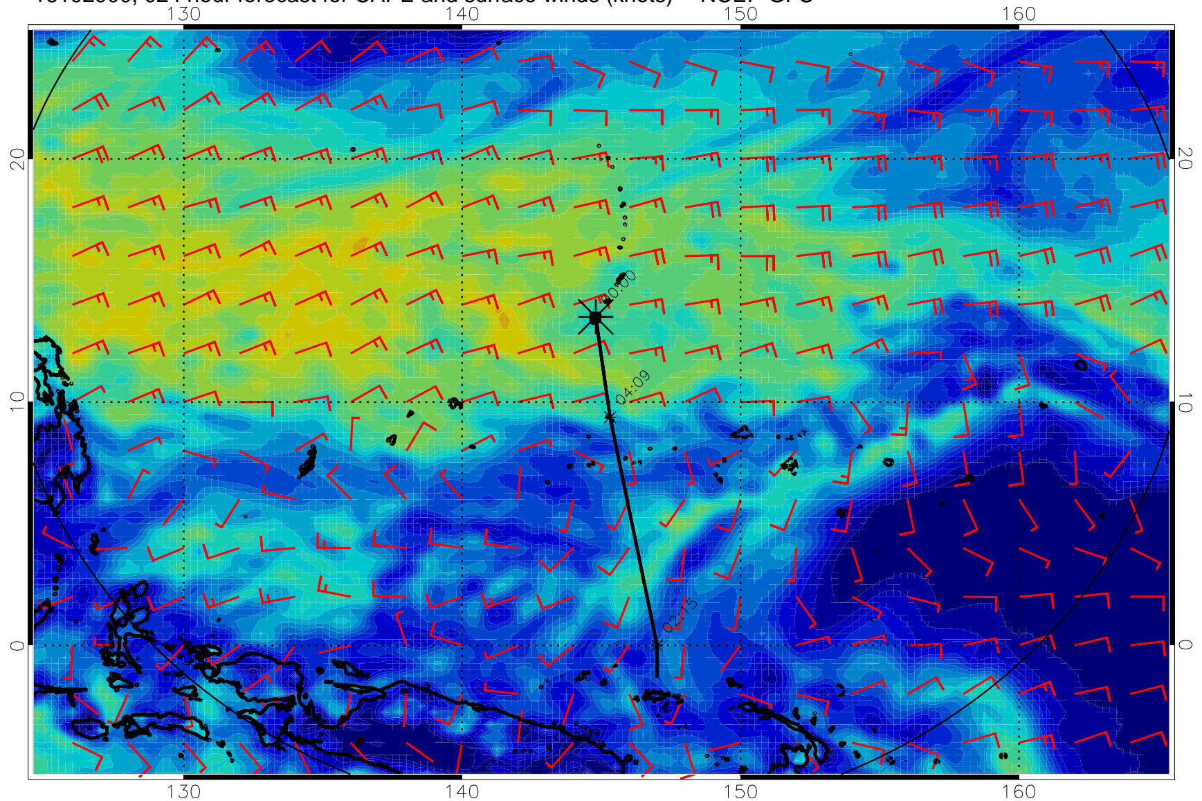
16102900, 024 hour forecast for CAPE and surface winds (knots) -- NCEP GFS
