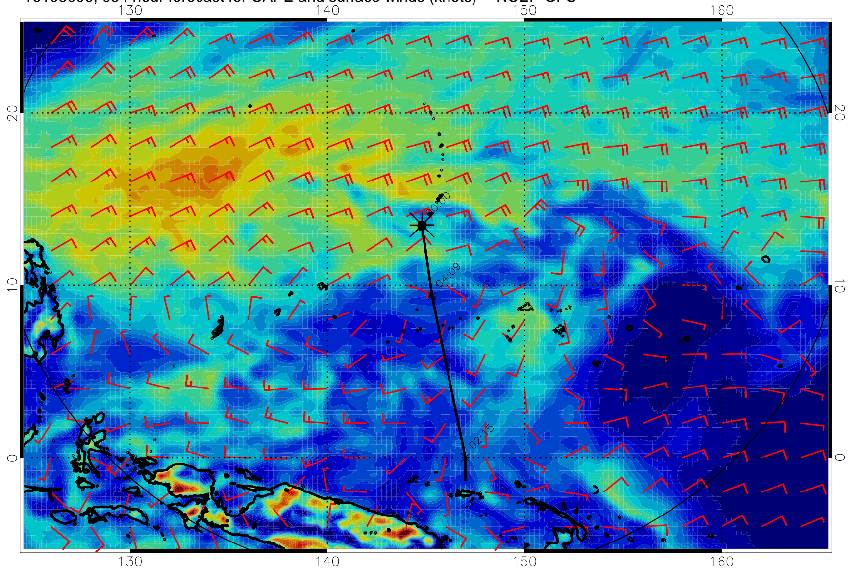
16103006, 054 hour forecast for CAPE and surface winds (knots) -- NCEP GFS
