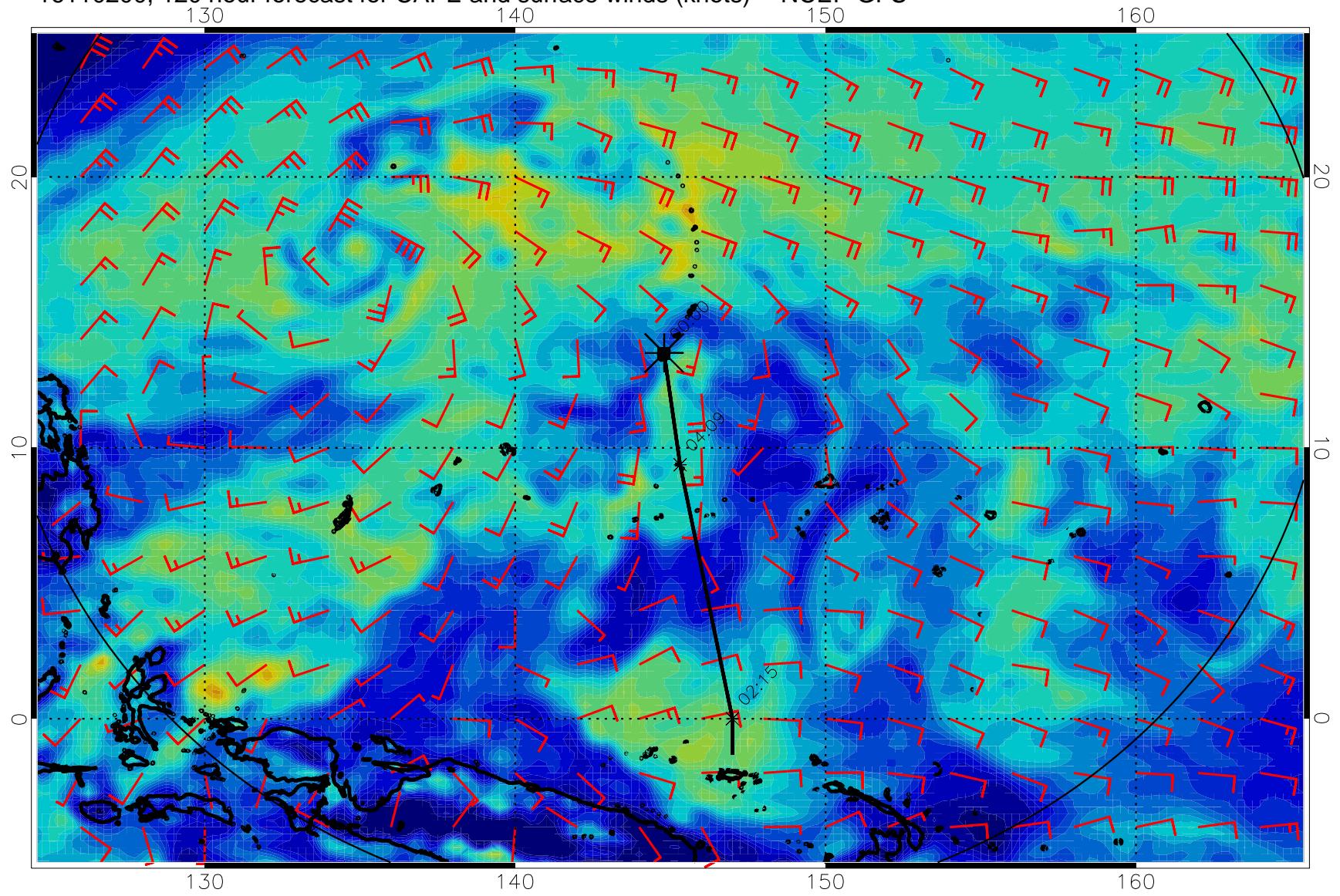
16110200, 120 hour forecast for CAPE and surface winds (knots) -- NCEP GFS
