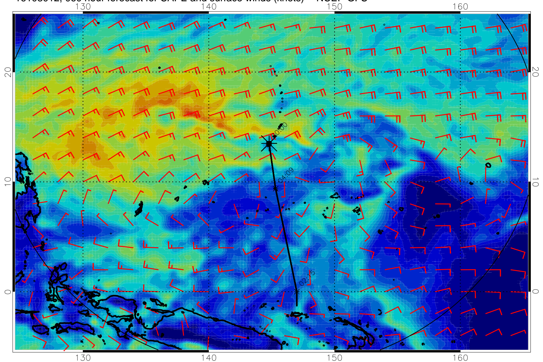
16103012, 060 hour forecast for CAPE and surface winds (knots) -- NCEP GFS
