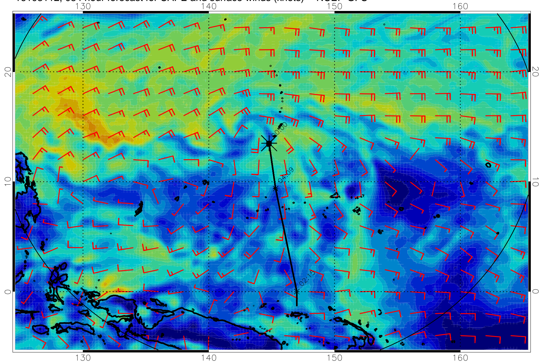
16103112, 084 hour forecast for CAPE and surface winds (knots) -- NCEP GFS
