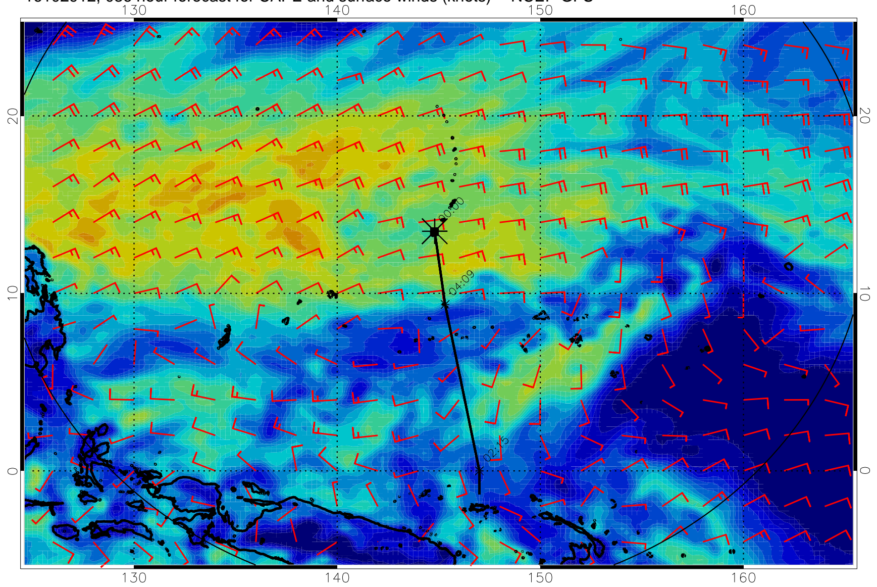
16102912, 036 hour forecast for CAPE and surface winds (knots) -- NCEP GFS
