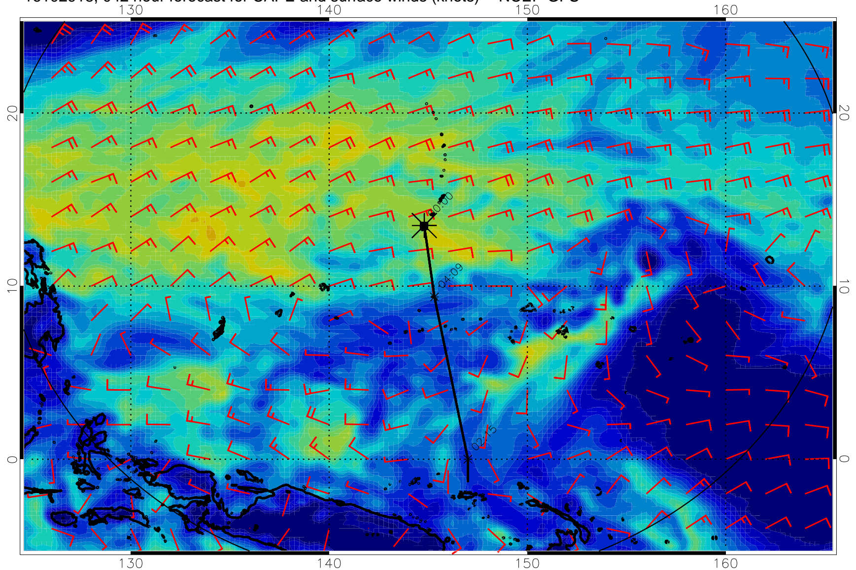
16102918, 042 hour forecast for CAPE and surface winds (knots) -- NCEP GFS
