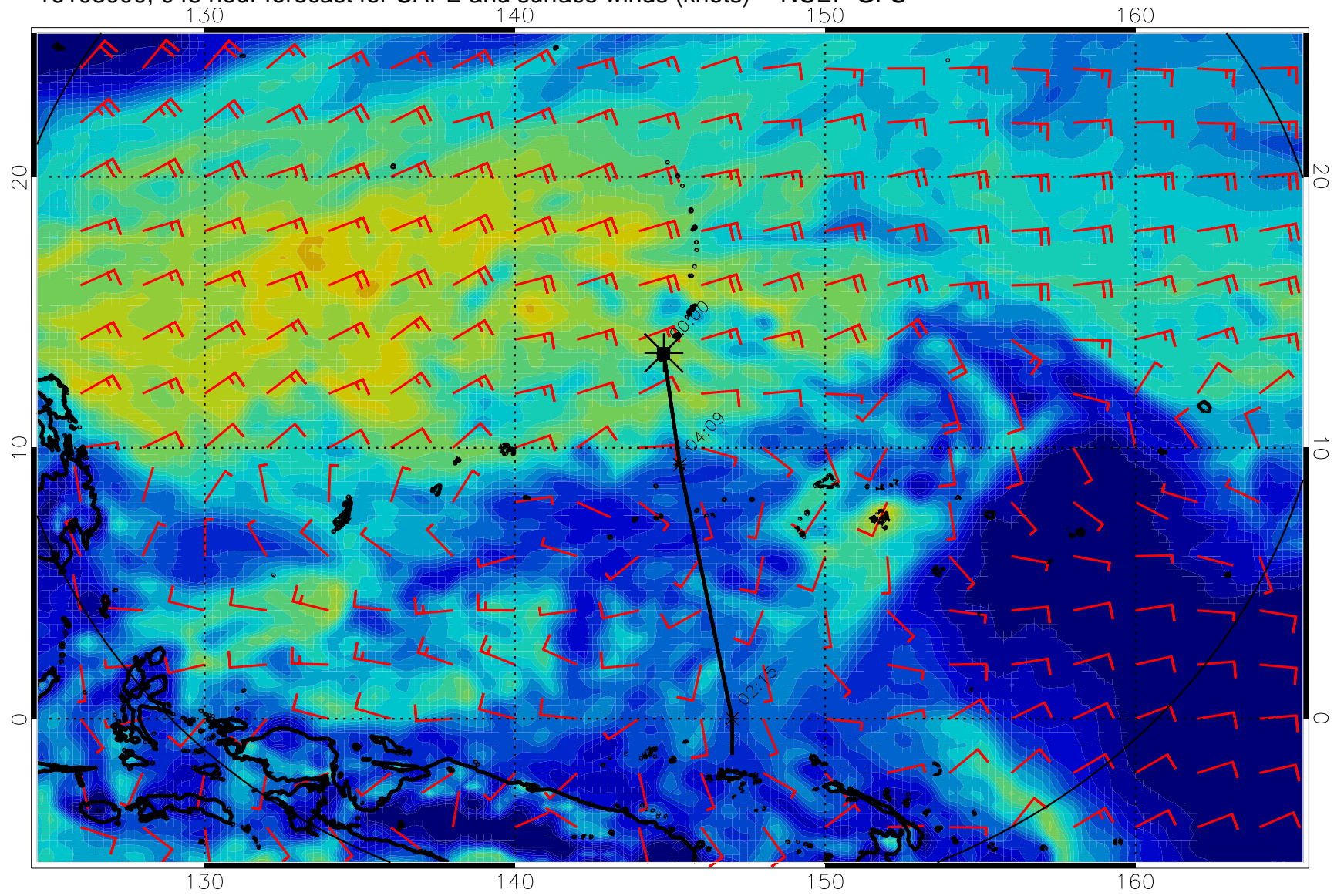
16103000, 048 hour forecast for CAPE and surface winds (knots) -- NCEP GFS
