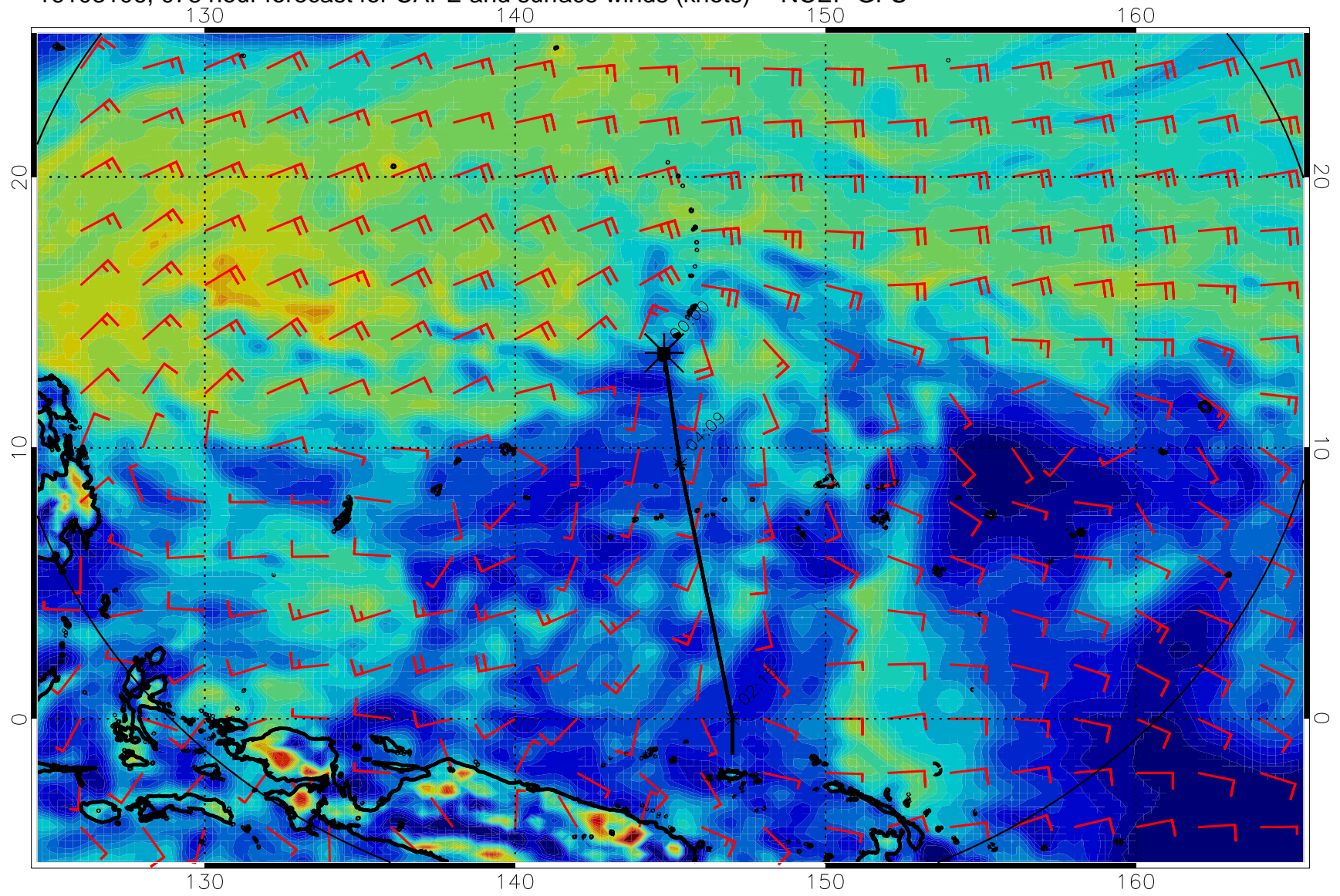
16103106, 078 hour forecast for CAPE and surface winds (knots) -- NCEP GFS
