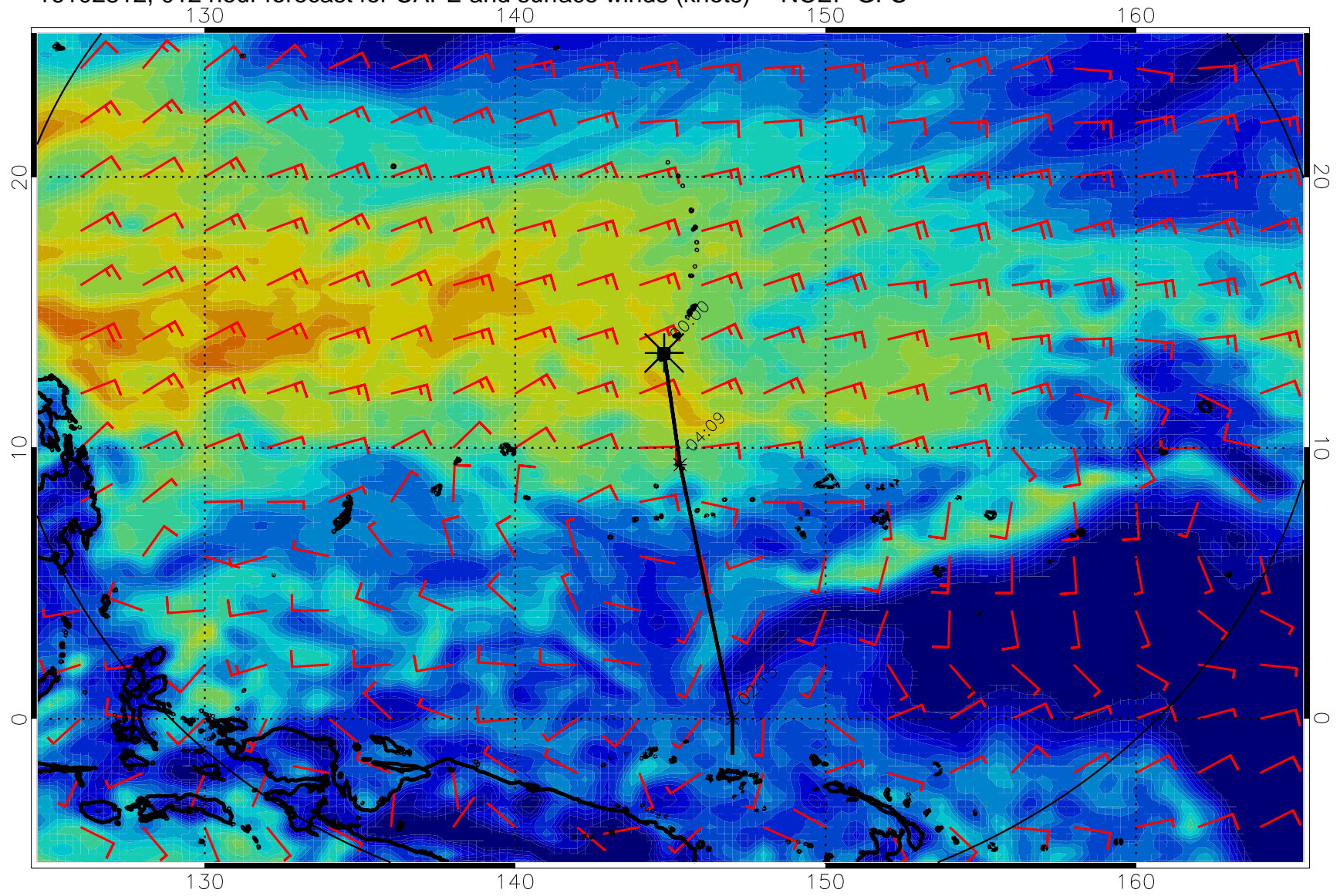
16102812, 012 hour forecast for CAPE and surface winds (knots) -- NCEP GFS
