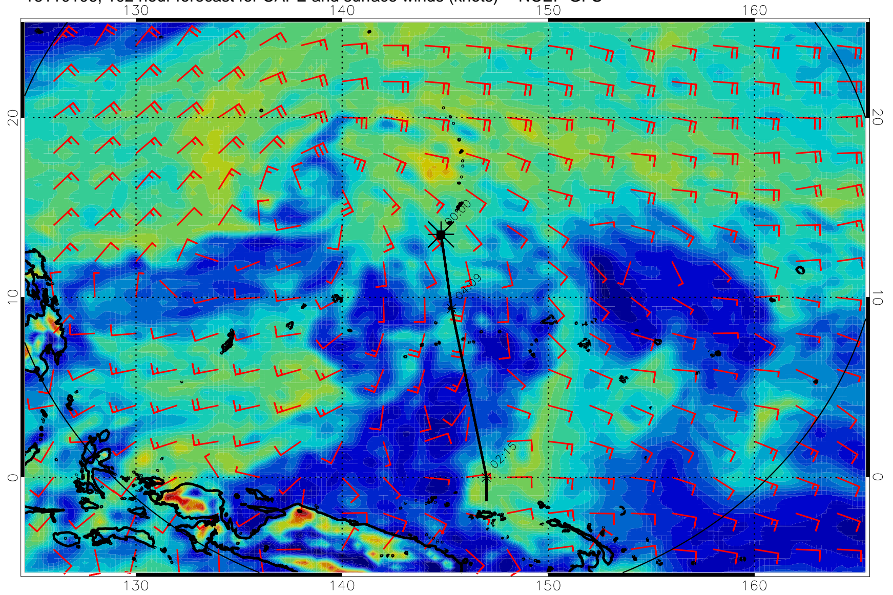
16110106, 102 hour forecast for CAPE and surface winds (knots) -- NCEP GFS
