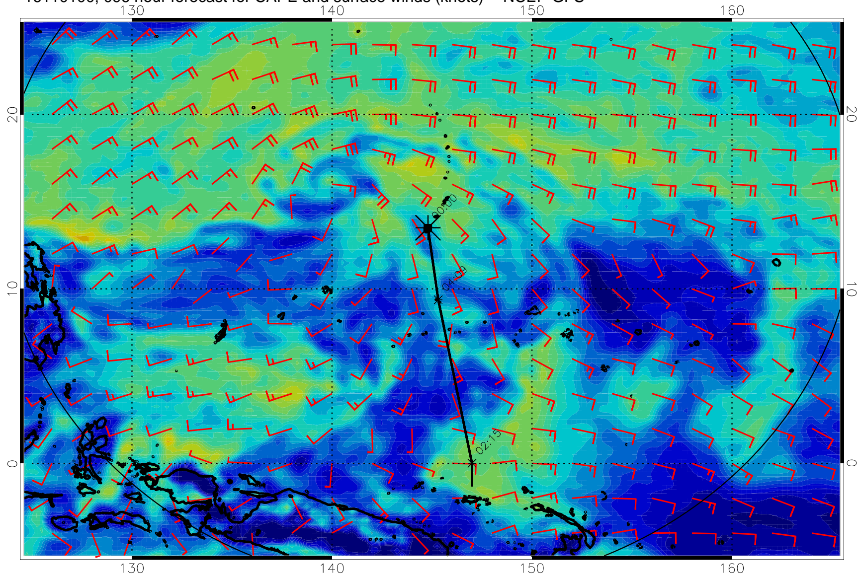
16110100, 096 hour forecast for CAPE and surface winds (knots) -- NCEP GFS
