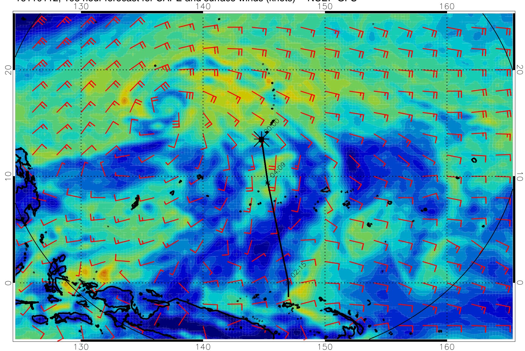
16110112, 108 hour forecast for CAPE and surface winds (knots) -- NCEP GFS
