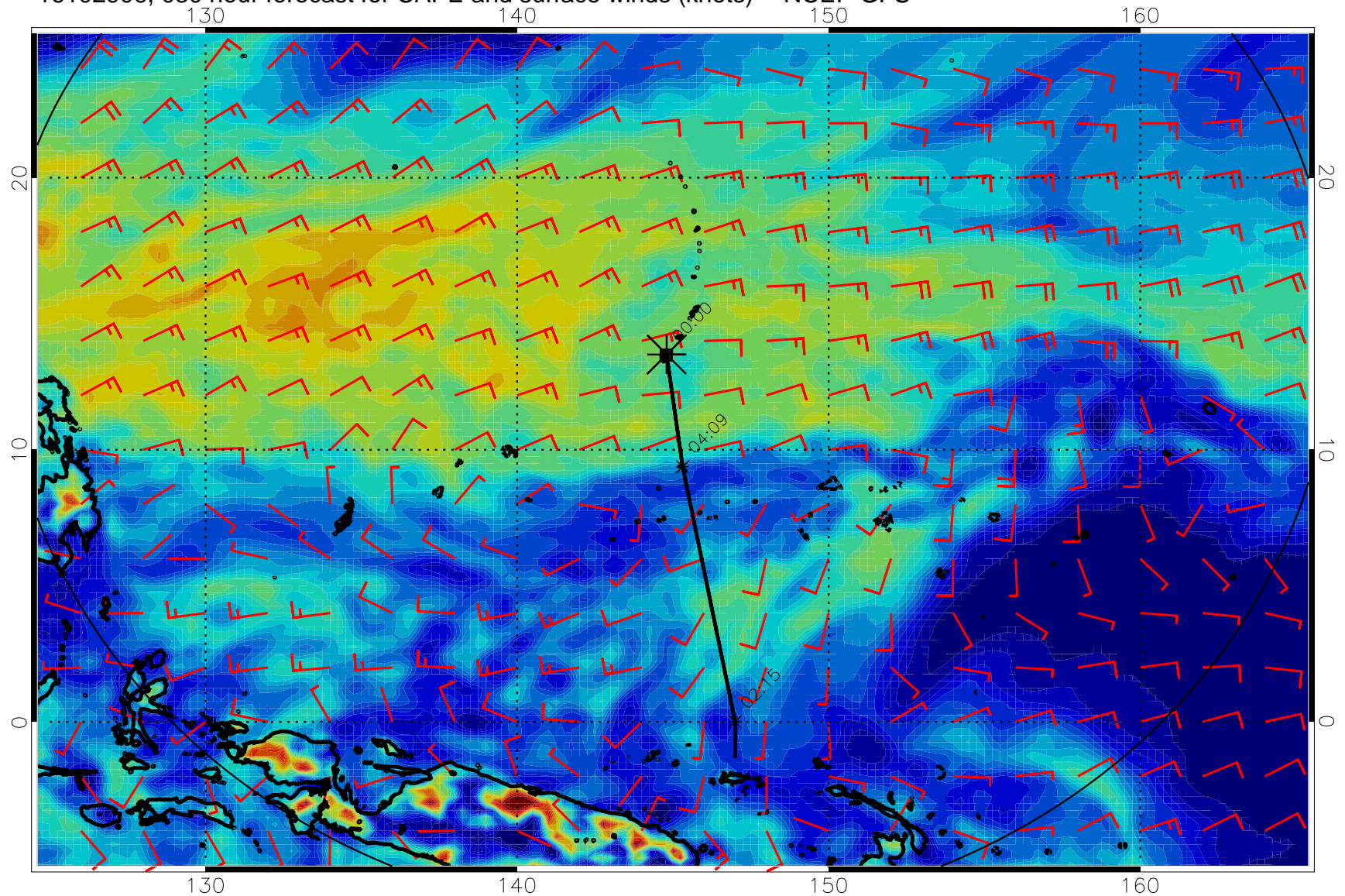
16102906, 030 hour forecast for CAPE and surface winds (knots) -- NCEP GFS
