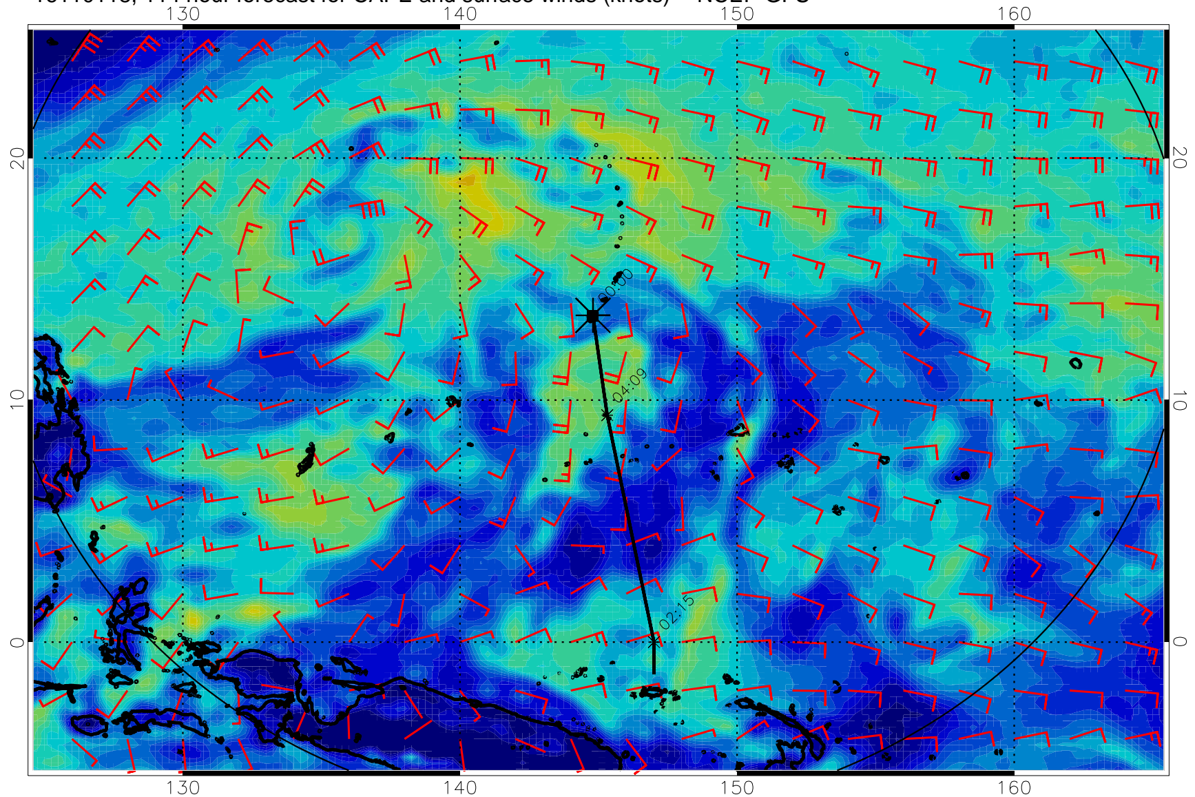
16110118, 114 hour forecast for CAPE and surface winds (knots) -- NCEP GFS
