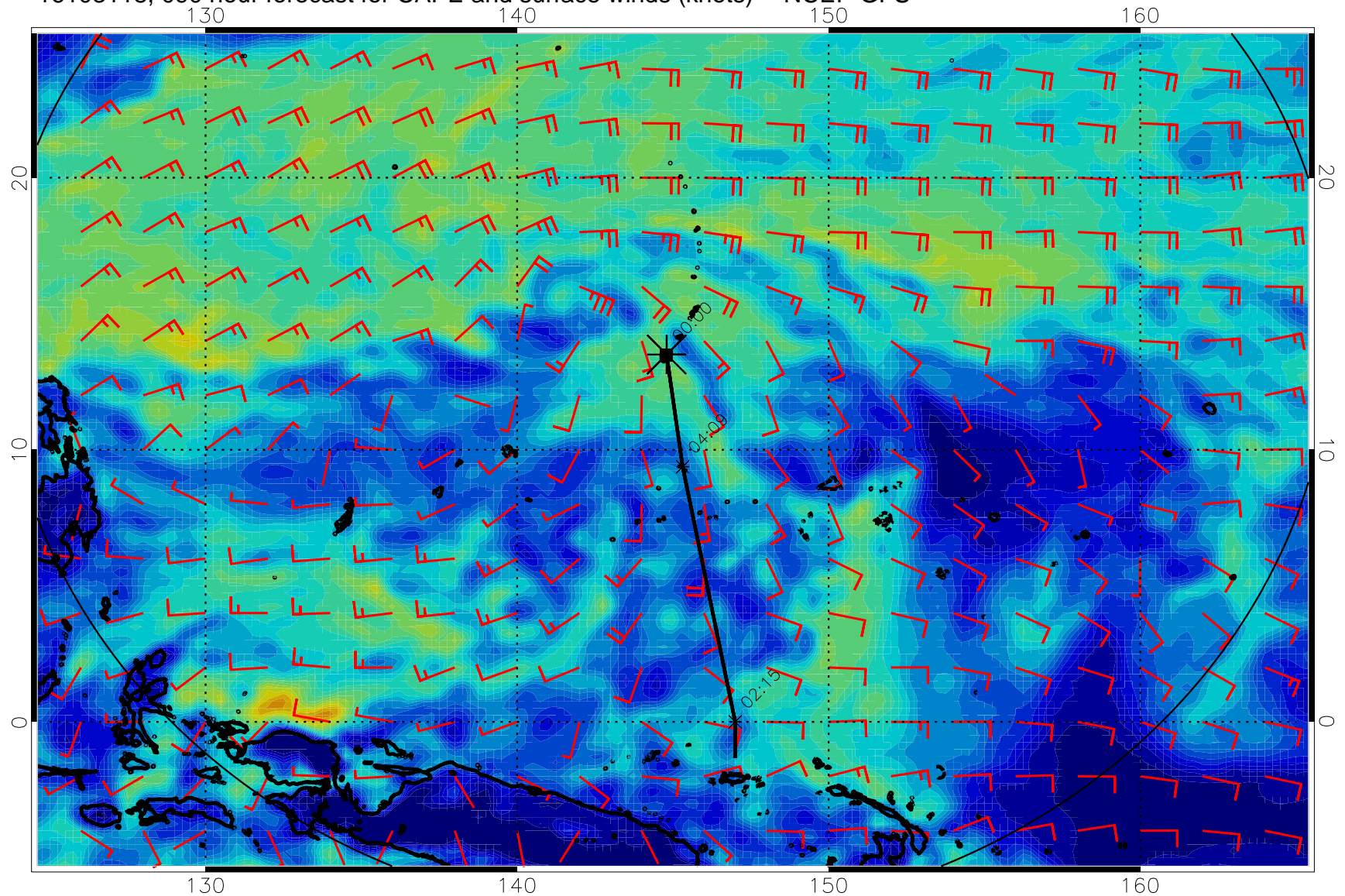
16103118, 090 hour forecast for CAPE and surface winds (knots) -- NCEP GFS
