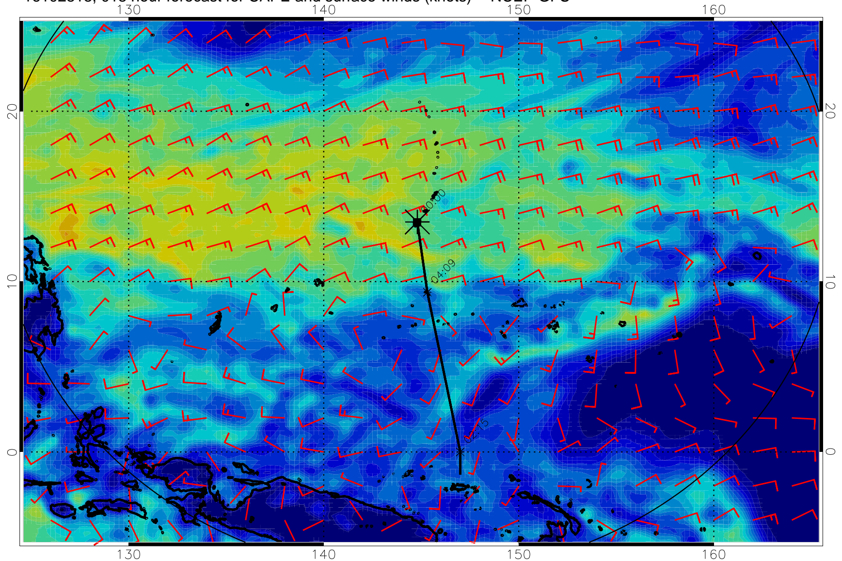
16102818, 018 hour forecast for CAPE and surface winds (knots) -- NCEP GFS
