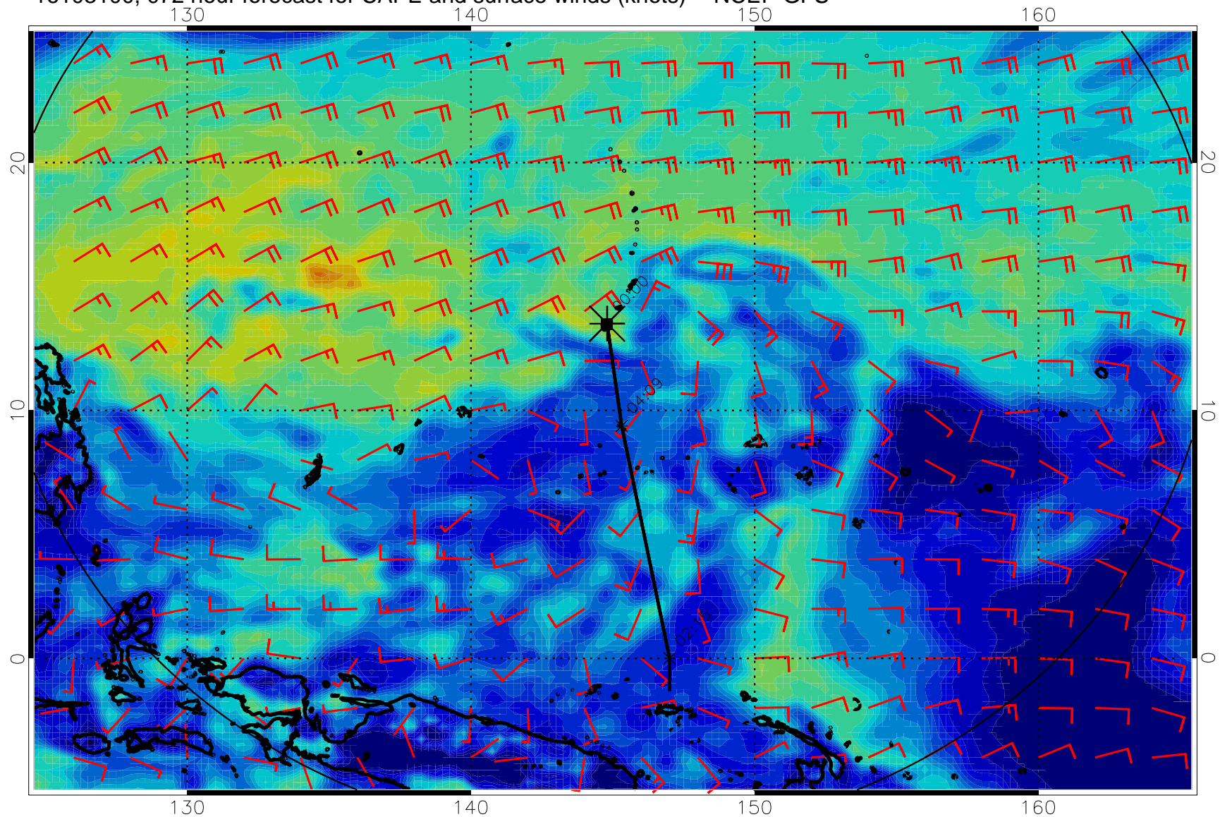
16103100, 072 hour forecast for CAPE and surface winds (knots) -- NCEP GFS
