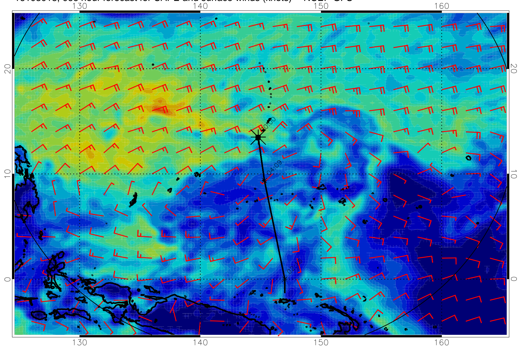
16103018, 066 hour forecast for CAPE and surface winds (knots) -- NCEP GFS
