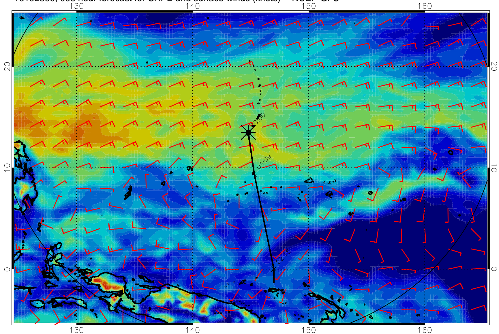
16102806, 006 hour forecast for CAPE and surface winds (knots) -- NCEP GFS
