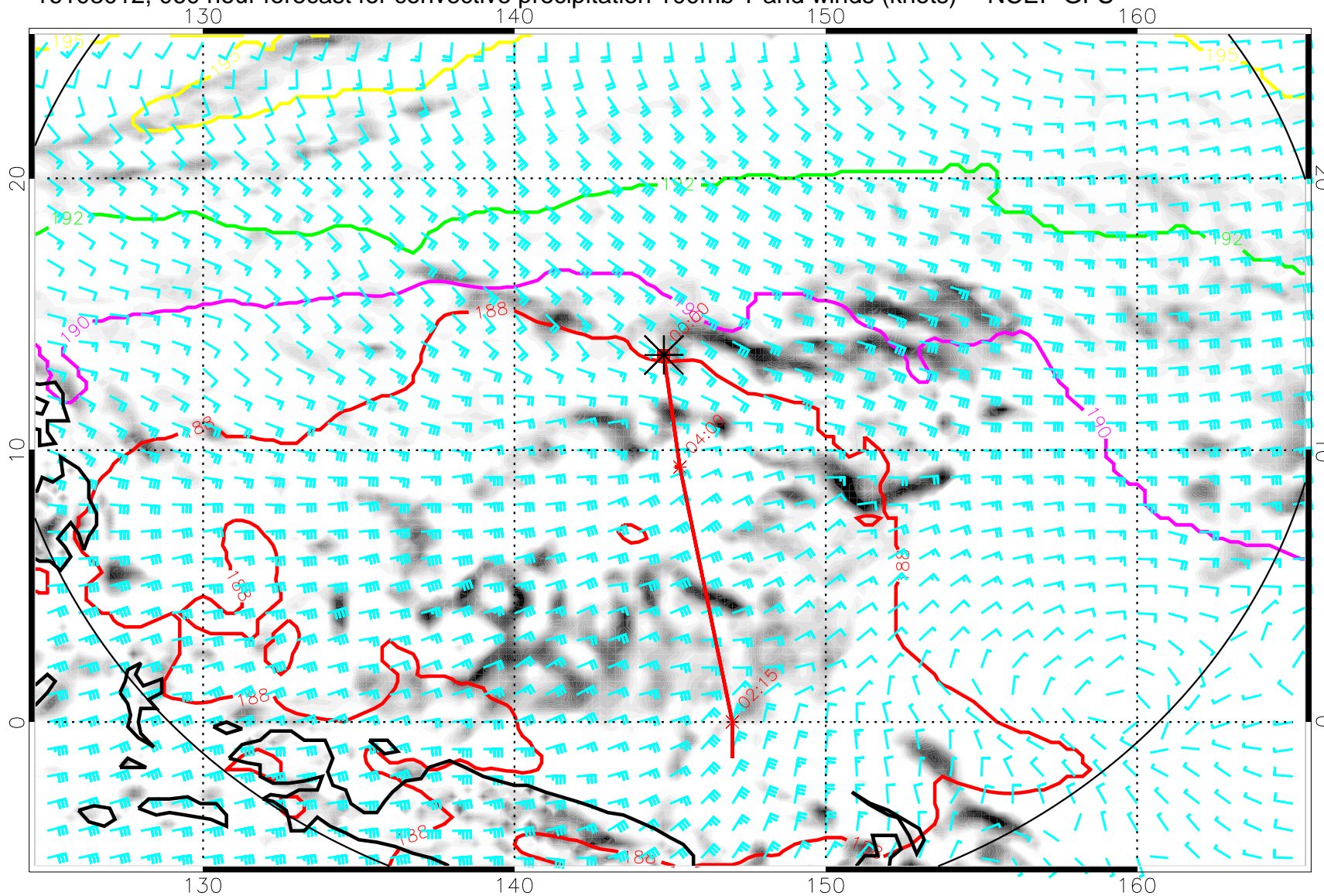
16103012, 060 hour forecast for convective precipitation 100mb T and winds (knots) -- NCEP GFS
