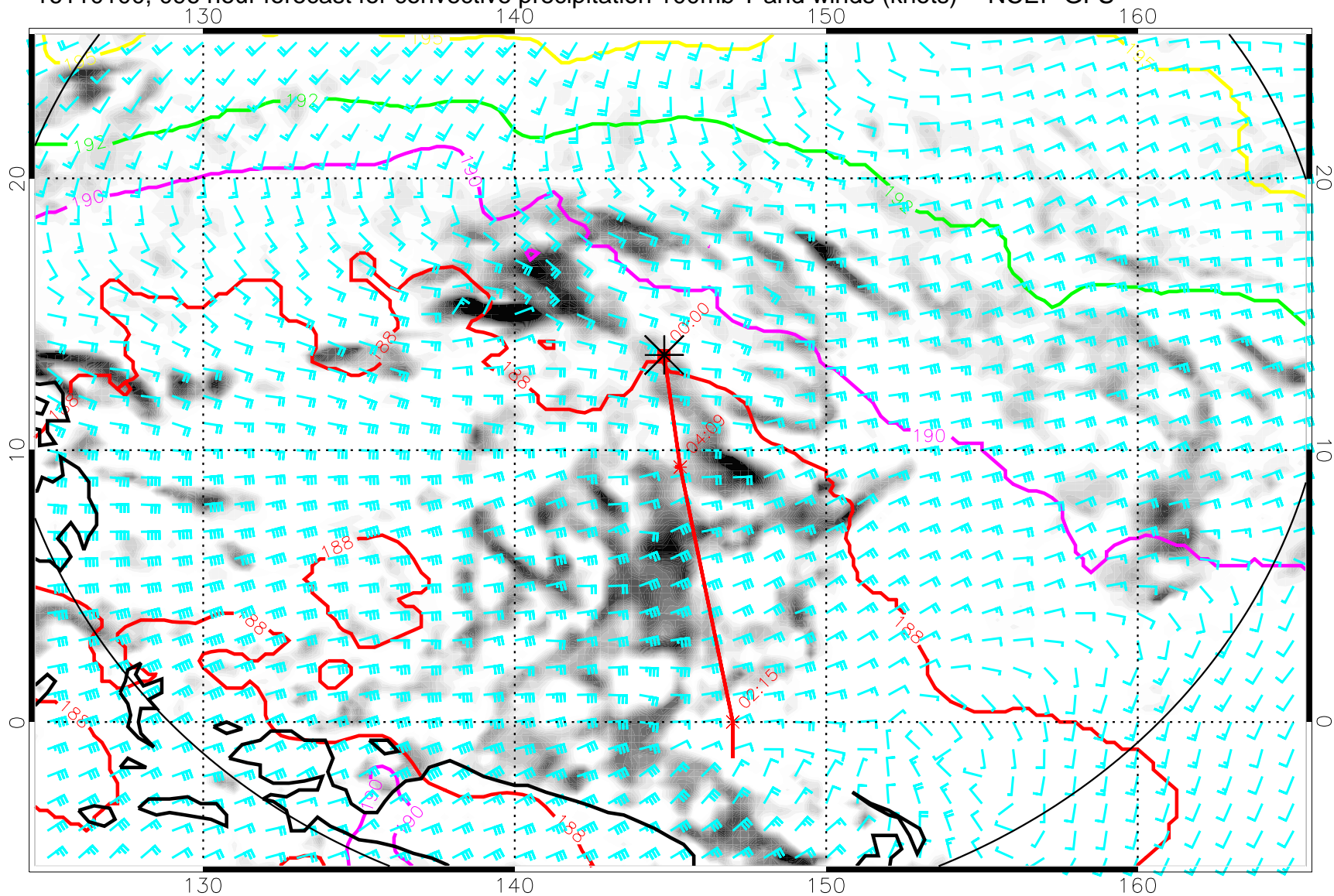
16110100, 096 hour forecast for convective precipitation 100mb T and winds (knots) -- NCEP GFS
