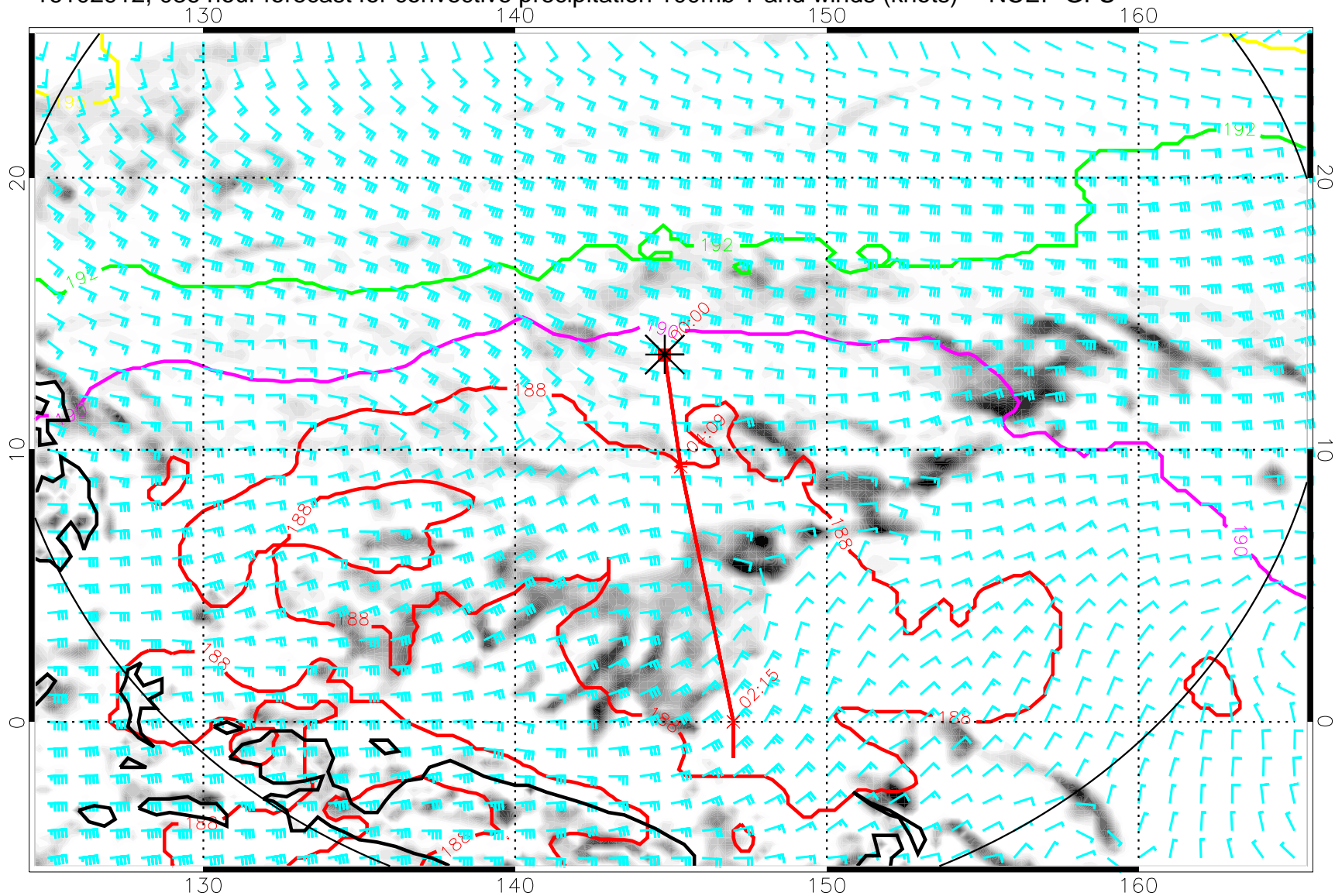
16102912, 036 hour forecast for convective precipitation 100mb T and winds (knots) -- NCEP GFS
