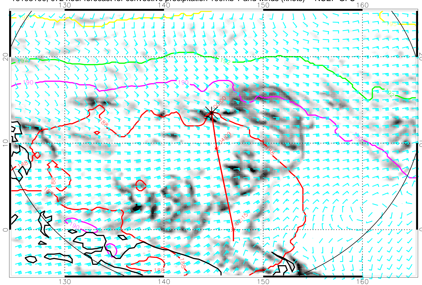
16103100, 072 hour forecast for convective precipitation 100mb T and winds (knots) -- NCEP GFS
