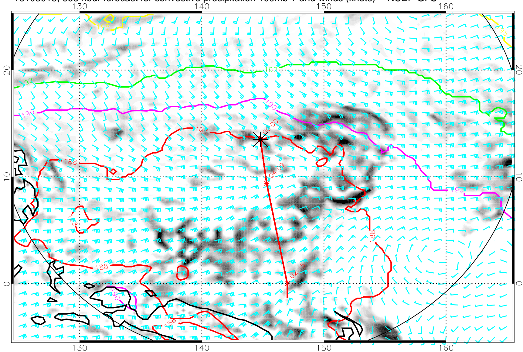
16103018, 066 hour forecast for convective precipitation 100mb T and winds (knots) -- NCEP GFS
