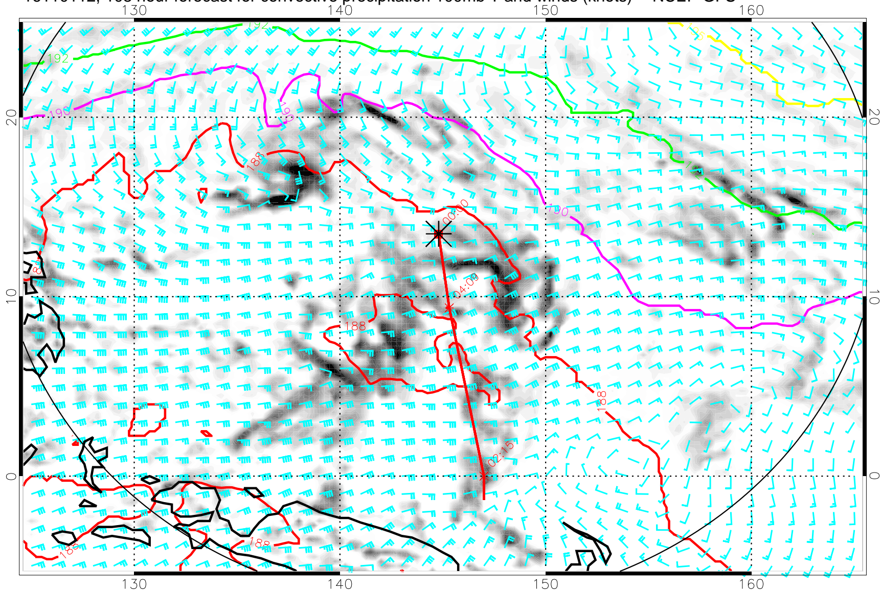
16110112, 108 hour forecast for convective precipitation 100mb T and winds (knots) -- NCEP GFS
