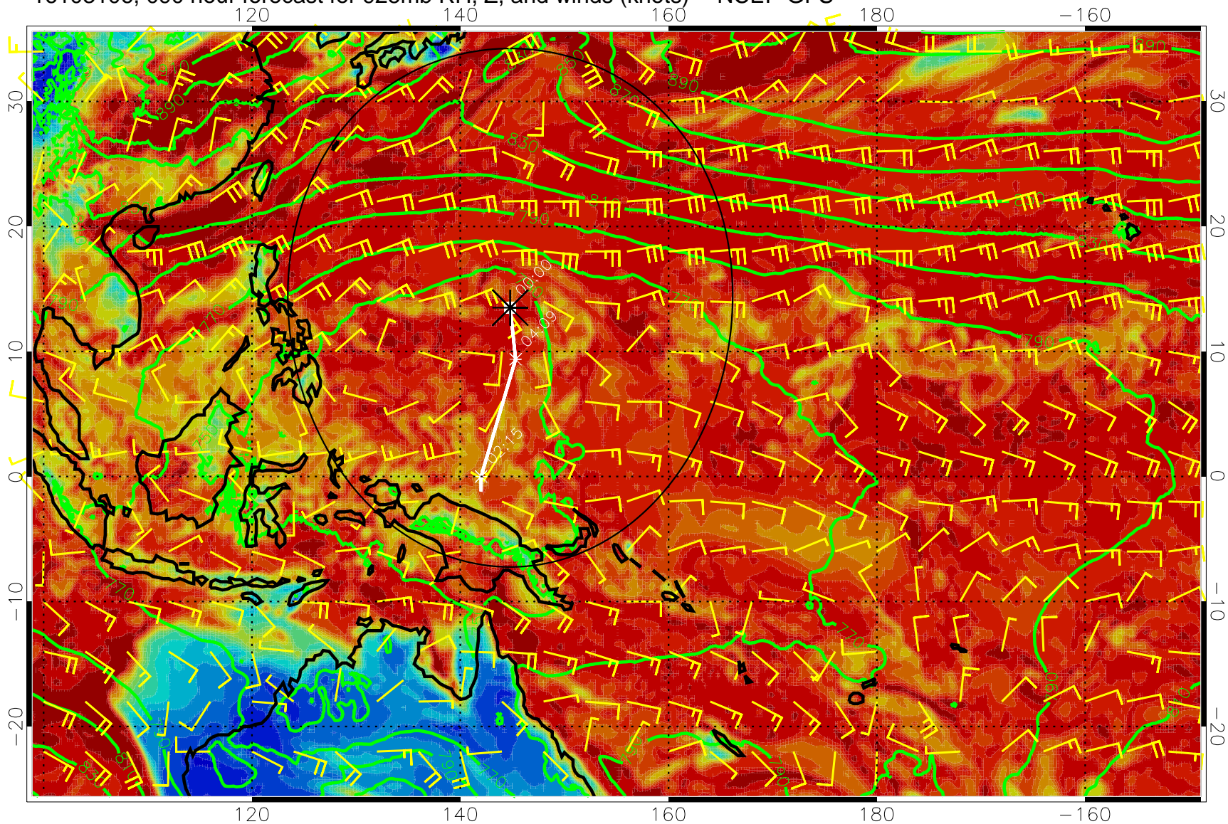
16103106, 090 hour forecast for 925mb RH, Z, and winds (knots) -- NCEP GFS
