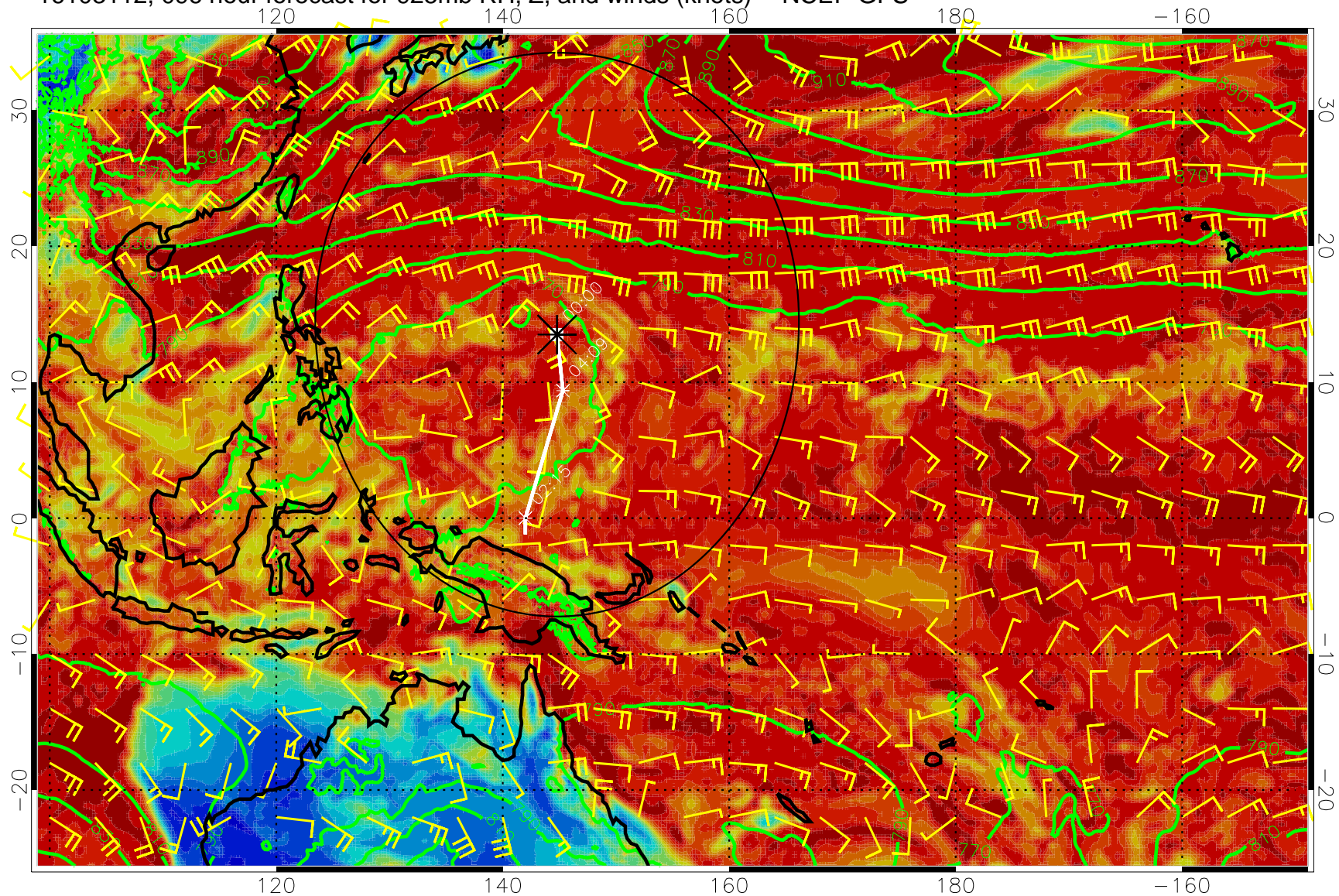
16103112, 096 hour forecast for 925mb RH, Z, and winds (knots) -- NCEP GFS
