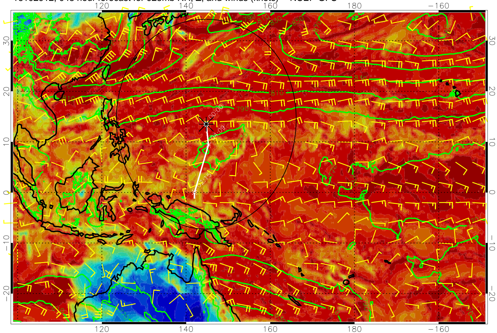
16102912, 048 hour forecast for 925mb RH, Z, and winds (knots) -- NCEP GFS
