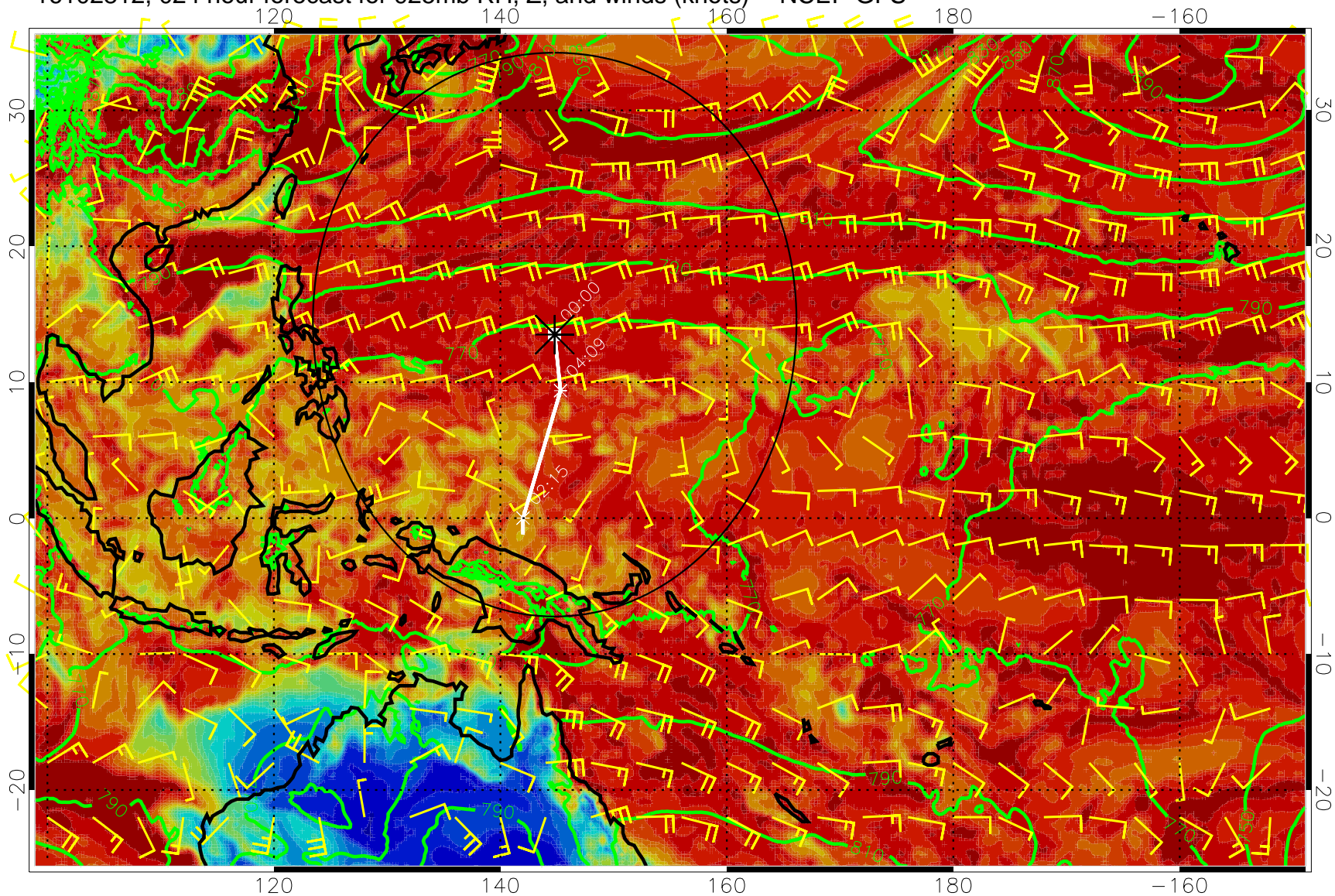
16102812, 024 hour forecast for 925mb RH, Z, and winds (knots) -- NCEP GFS
