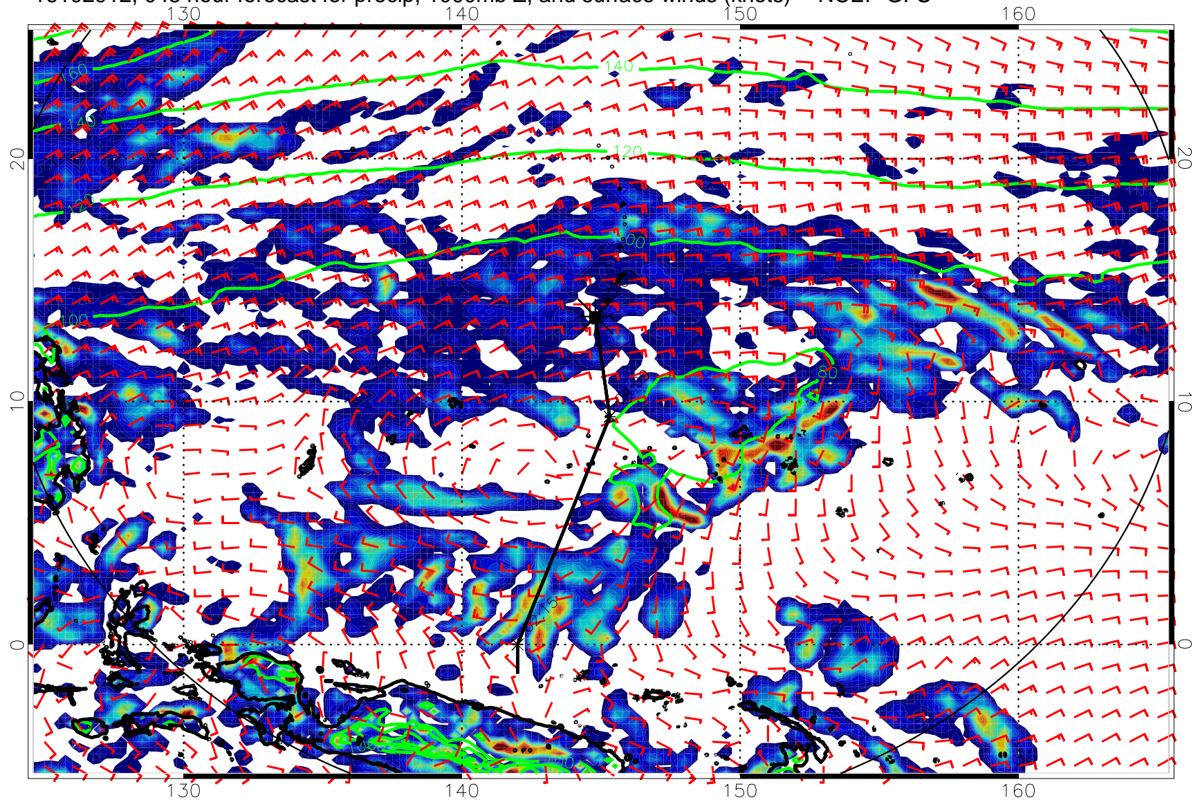
16102912, 048 hour forecast for precip, 1000mb Z, and surface winds (knots) -- NCEP GFS
