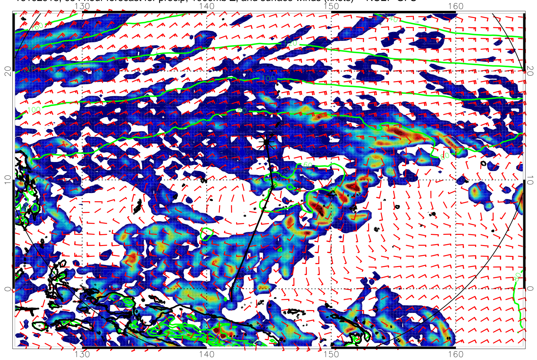
16102918, 054 hour forecast for precip, 1000mb Z, and surface winds (knots) -- NCEP GFS
