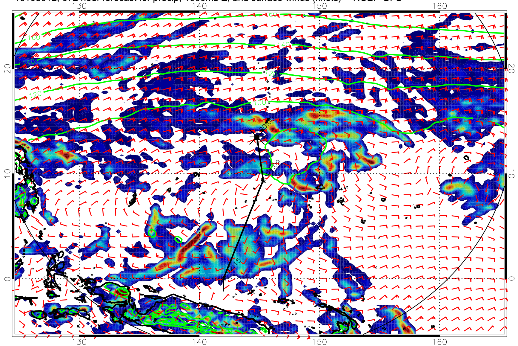
16103012, 072 hour forecast for precip, 1000mb Z, and surface winds (knots) -- NCEP GFS
