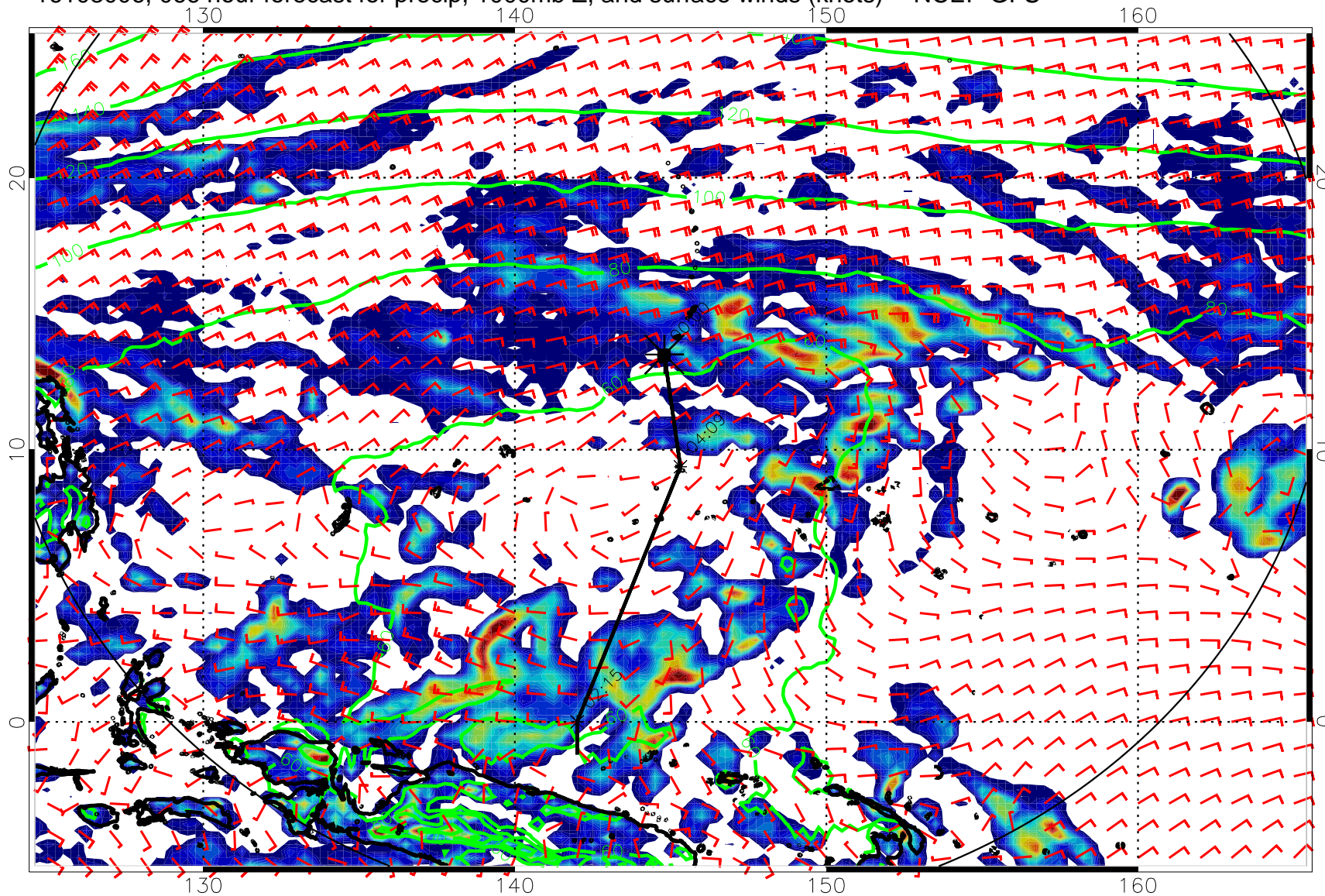
16103006, 066 hour forecast for precip, 1000mb Z, and surface winds (knots) -- NCEP GFS
