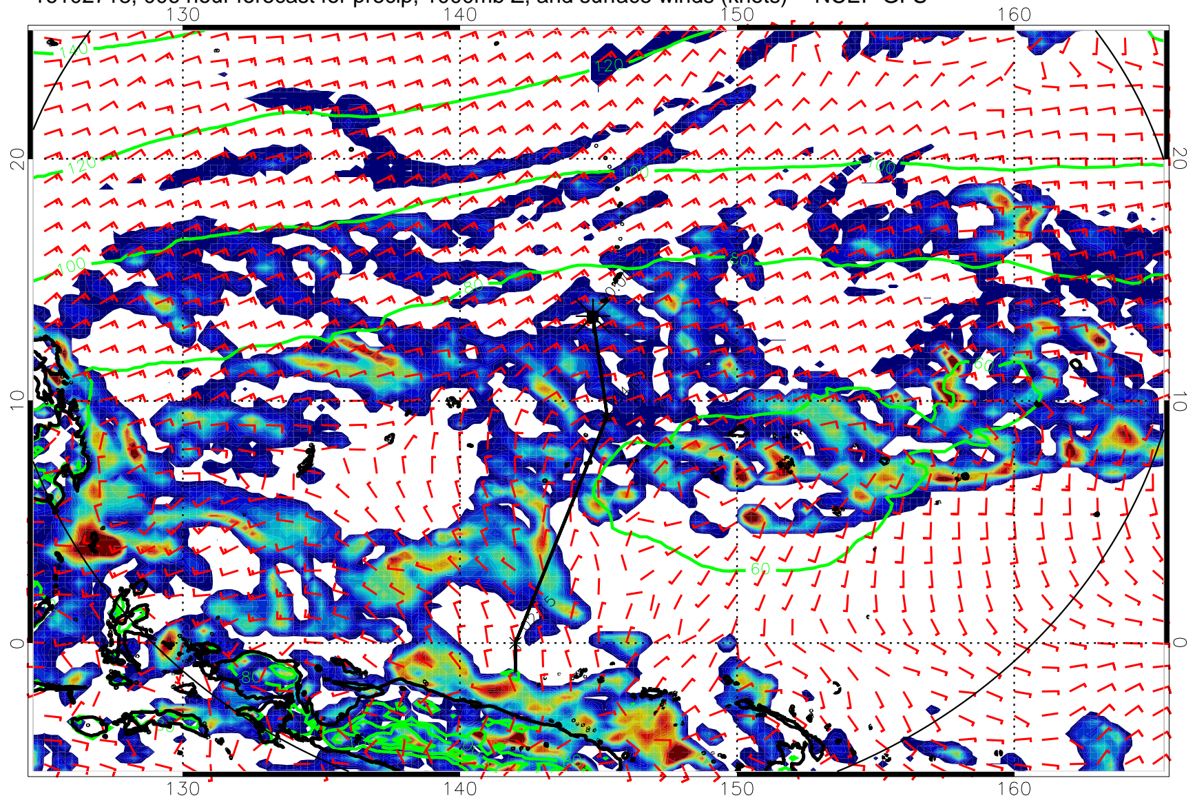
16102718, 006 hour forecast for precip, 1000mb Z, and surface winds (knots) -- NCEP GFS
