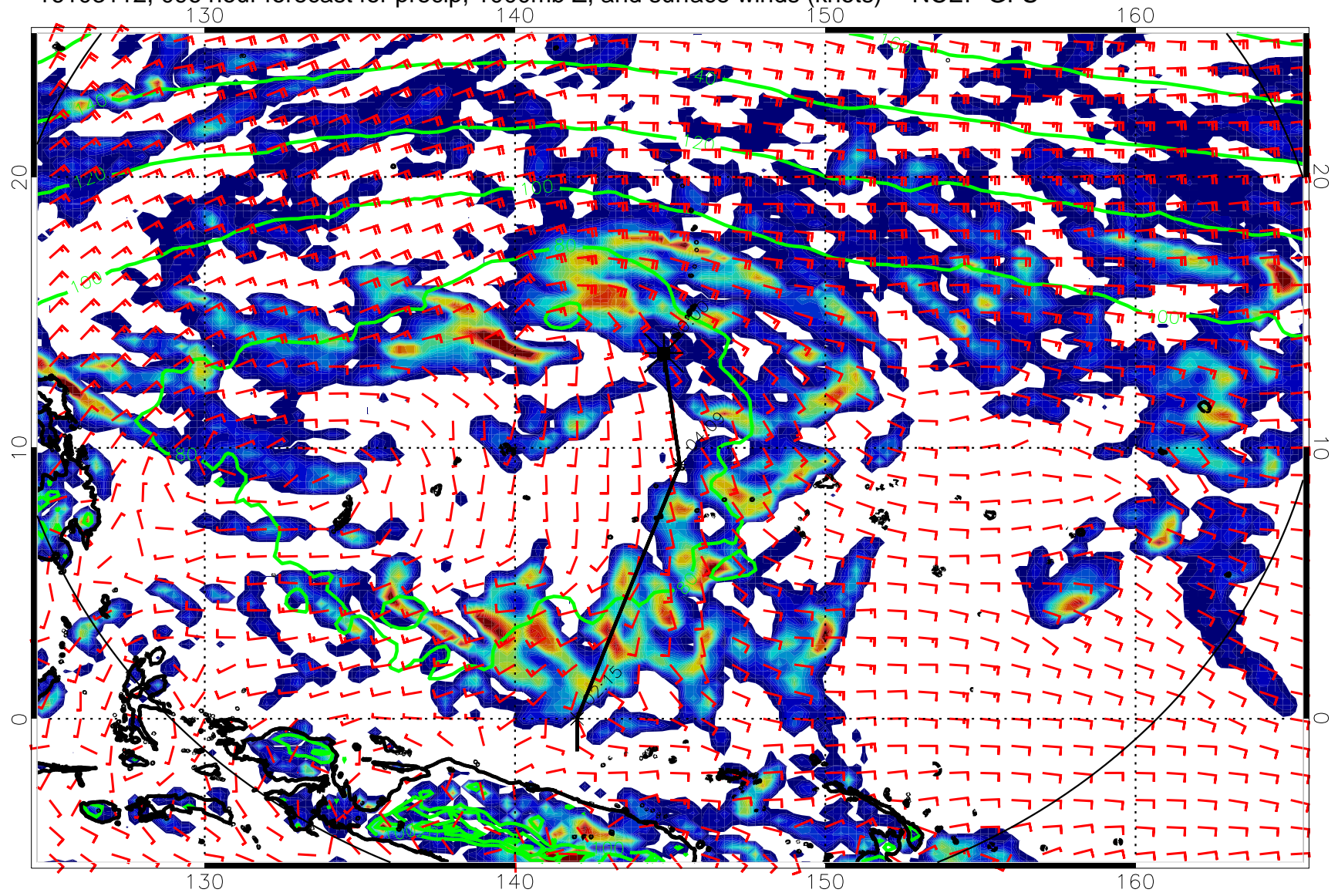
16103112, 096 hour forecast for precip, 1000mb Z, and surface winds (knots) -- NCEP GFS
