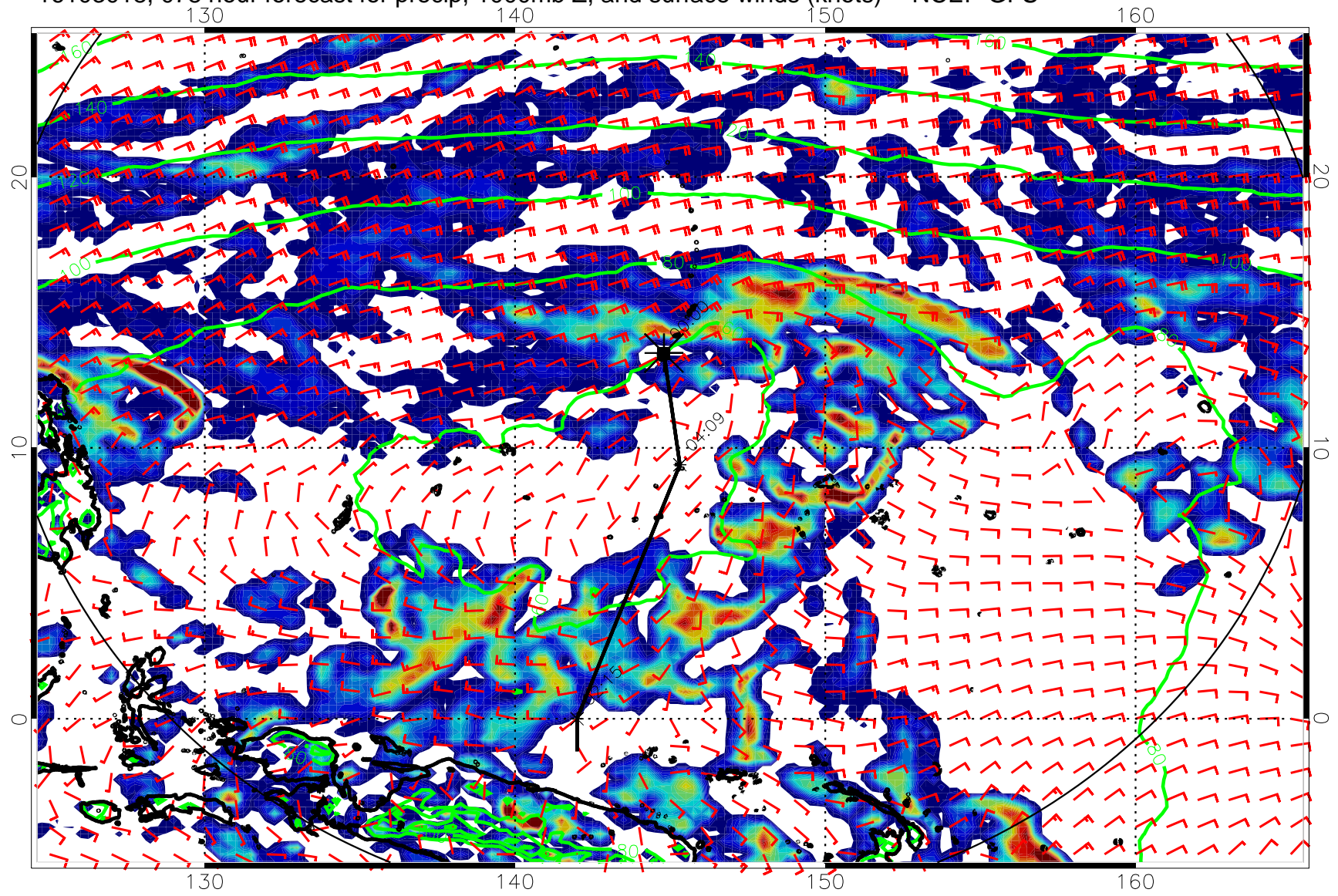
16103018, 078 hour forecast for precip, 1000mb Z, and surface winds (knots) -- NCEP GFS
