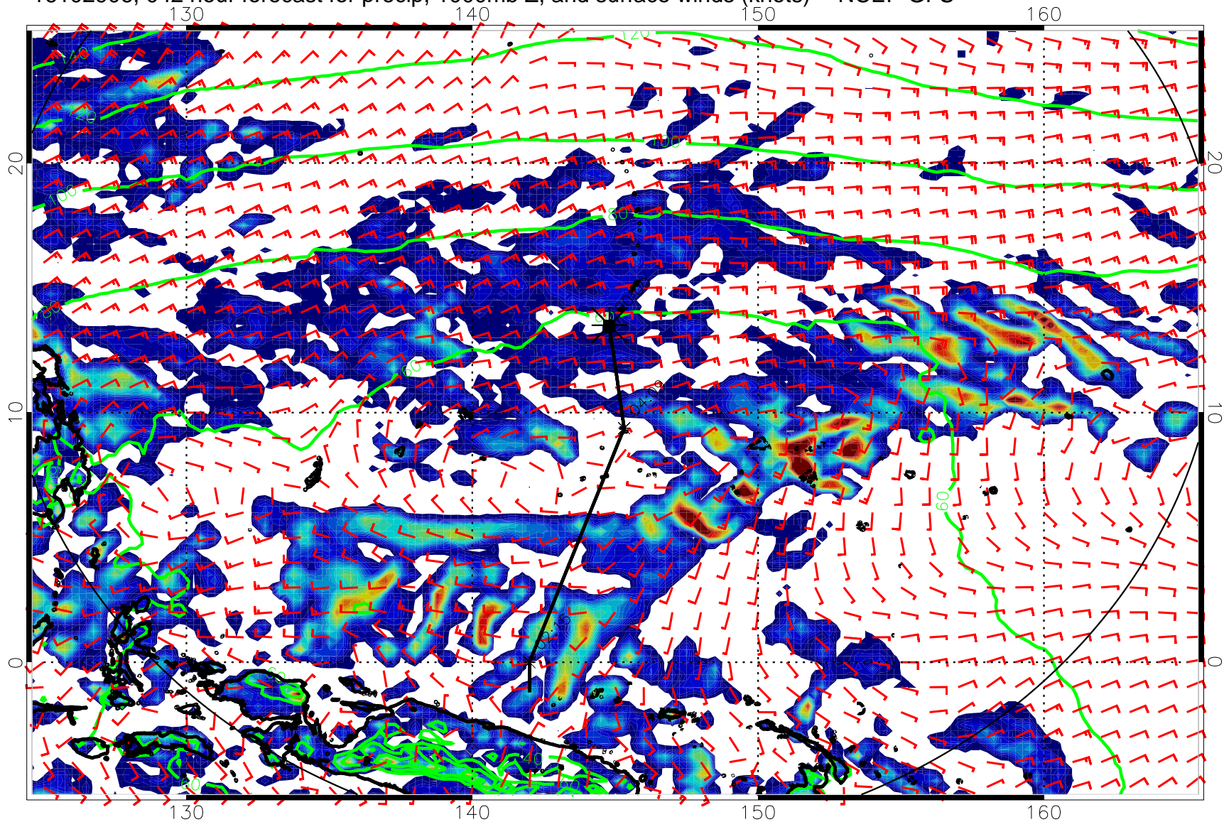
16102906, 042 hour forecast for precip, 1000mb Z, and surface winds (knots) -- NCEP GFS
