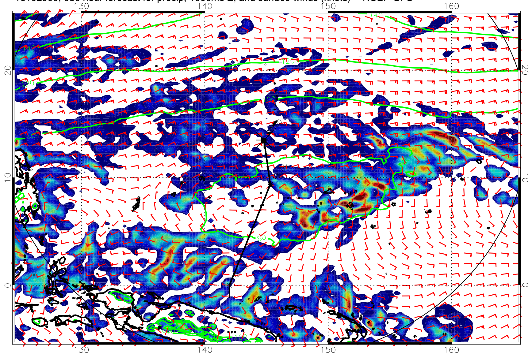
16102900, 036 hour forecast for precip, 1000mb Z, and surface winds (knots) -- NCEP GFS
