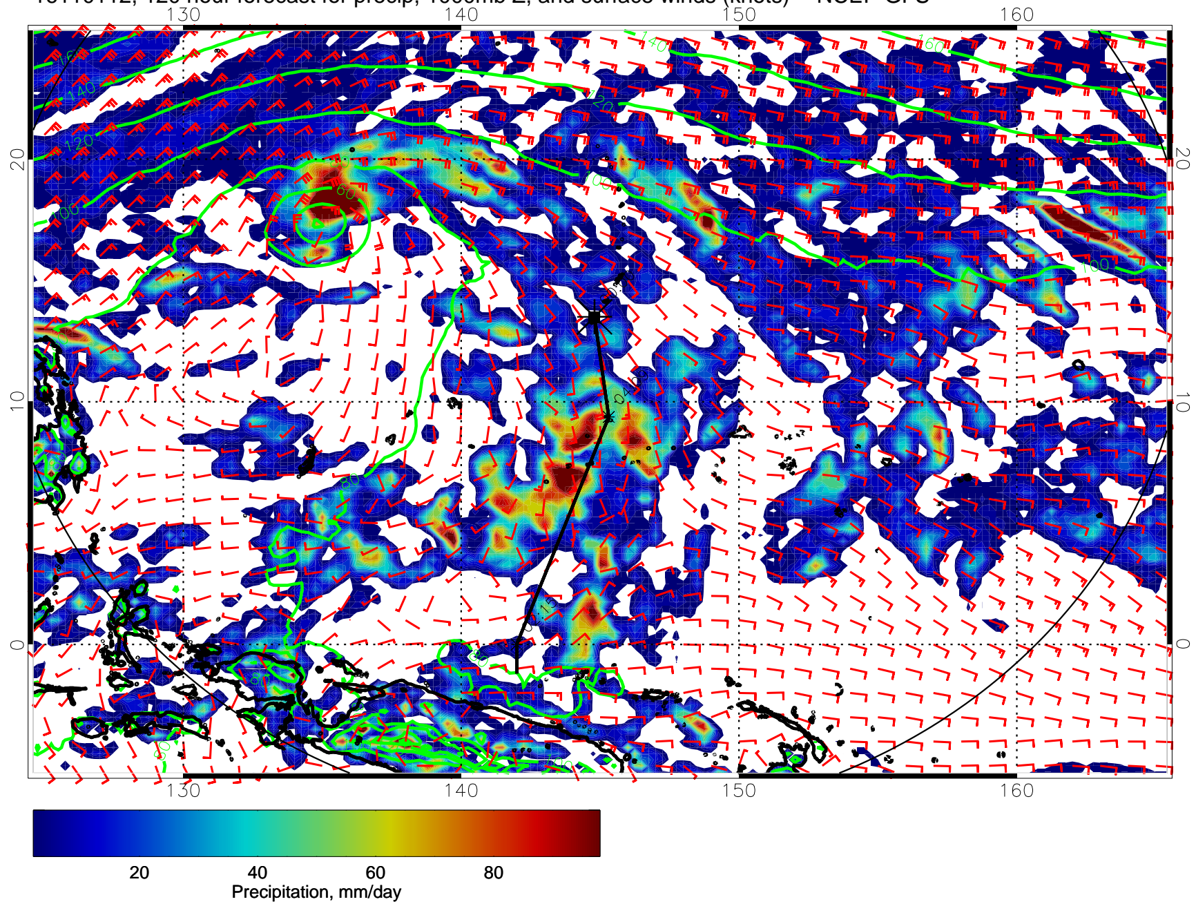
16110112, 120 hour forecast for precip, 1000mb Z, and surface winds (knots) -- NCEP GFS
