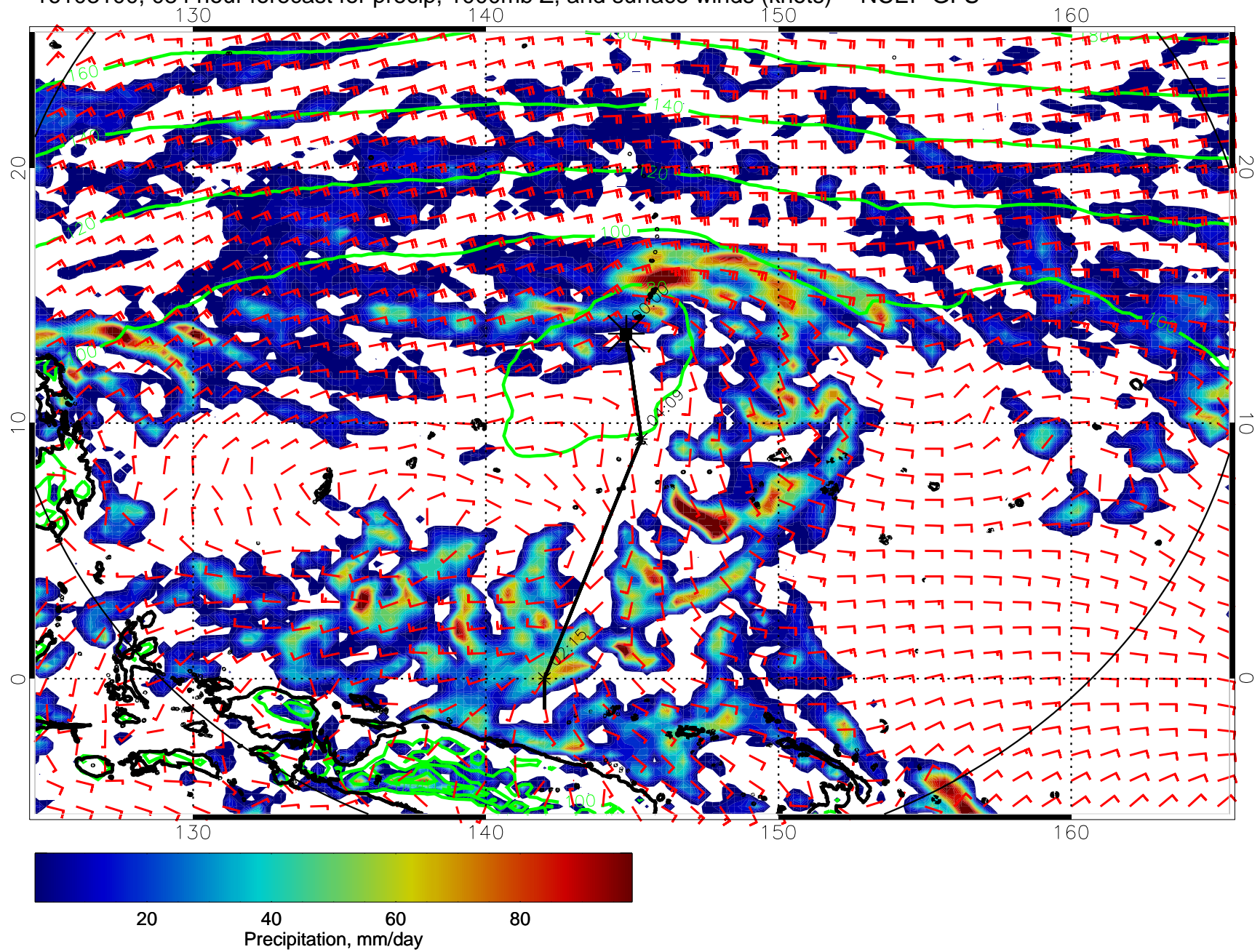
16103100, 084 hour forecast for precip, 1000mb Z, and surface winds (knots) -- NCEP GFS
