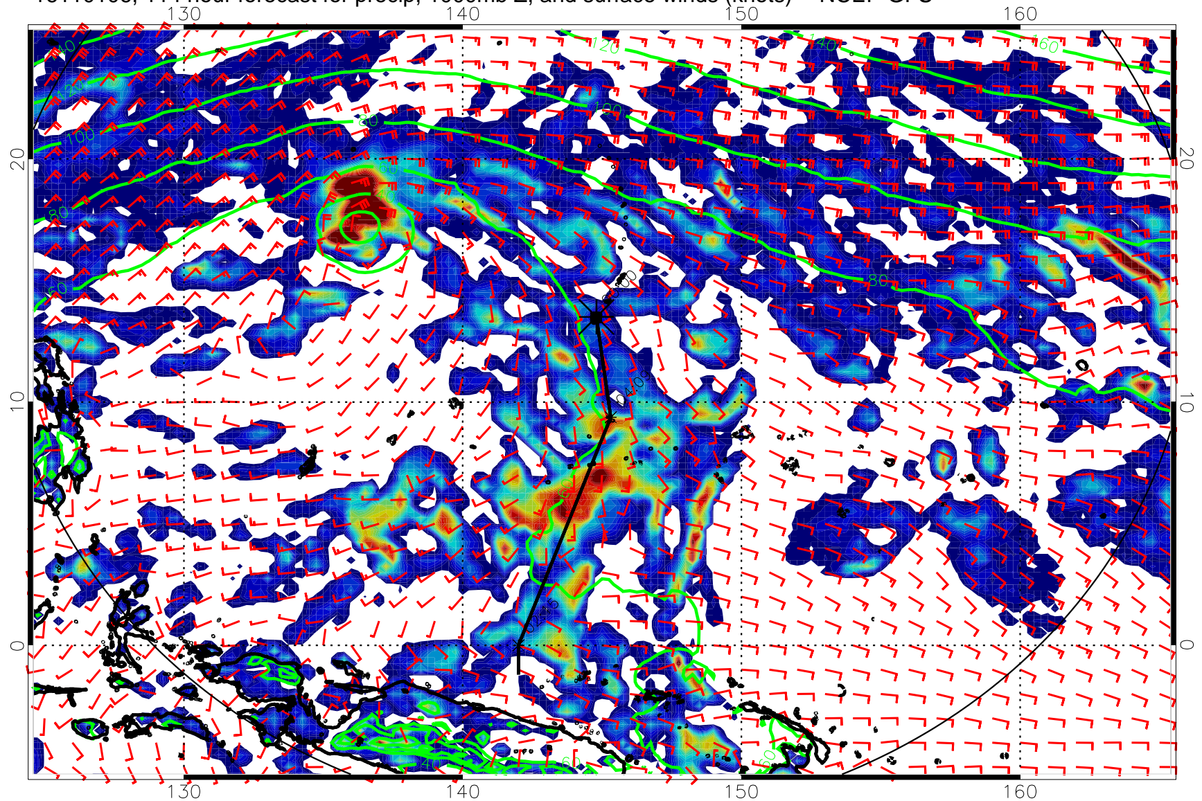
16110106, 114 hour forecast for precip, 1000mb Z, and surface winds (knots) -- NCEP GFS
