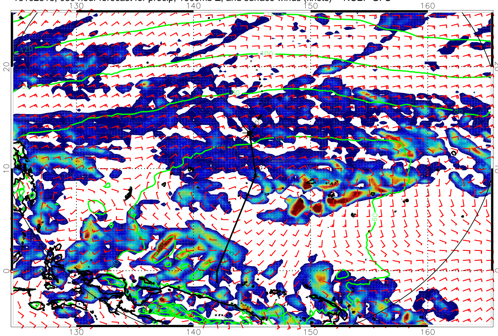
16102818, 030 hour forecast for precip, 1000mb Z, and surface winds (knots) -- NCEP GFS
