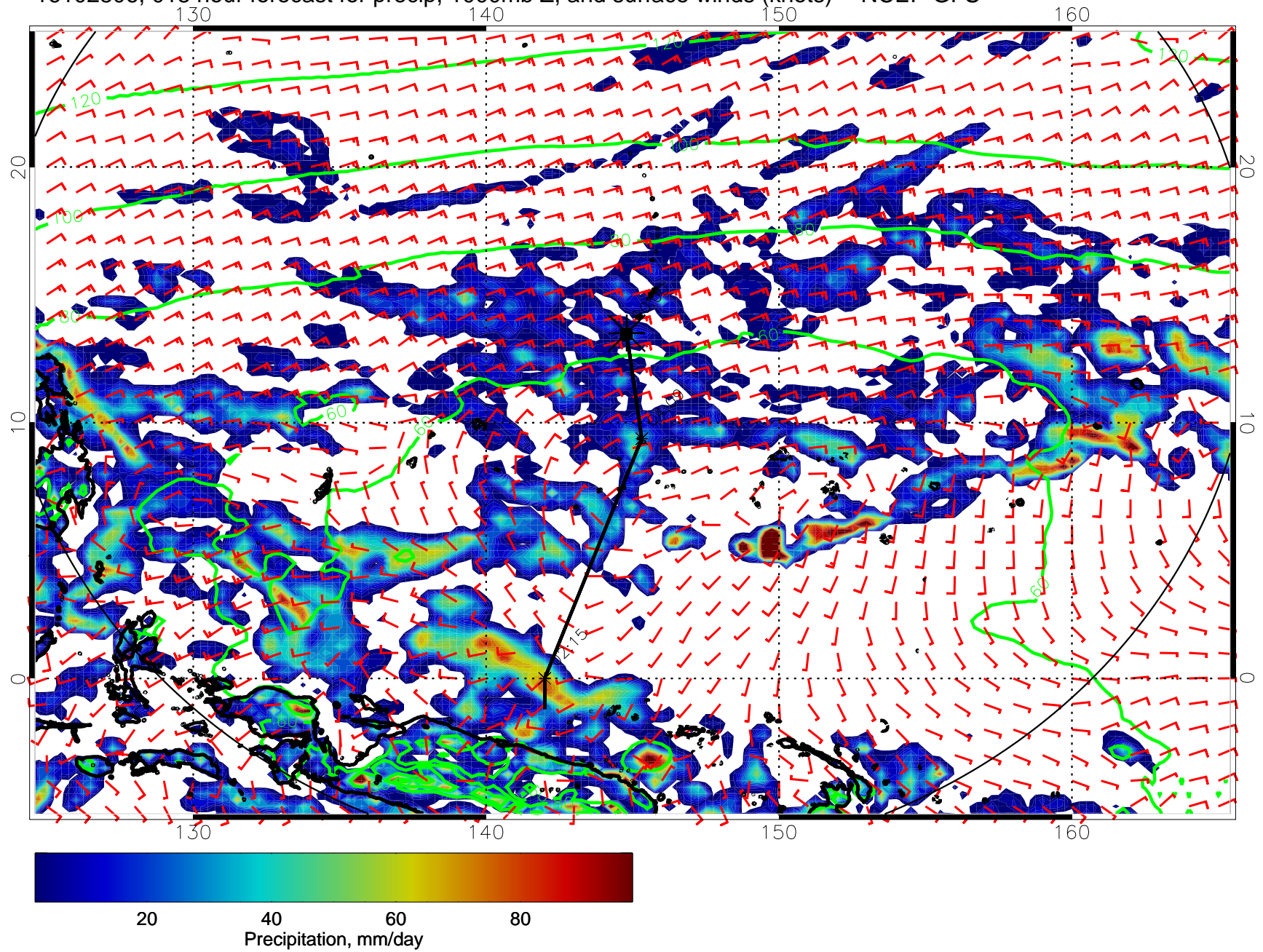
16102806, 018 hour forecast for precip, 1000mb Z, and surface winds (knots) -- NCEP GFS
