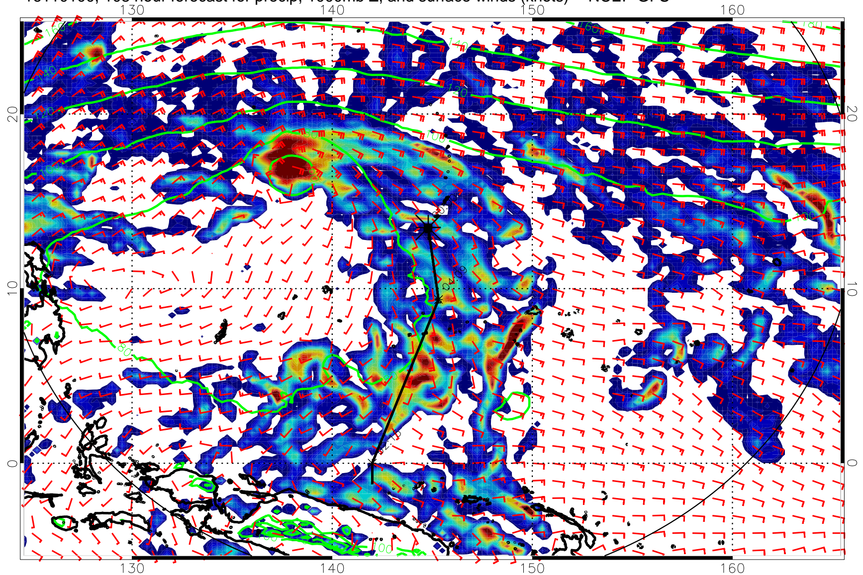
16110100, 108 hour forecast for precip, 1000mb Z, and surface winds (knots) -- NCEP GFS
