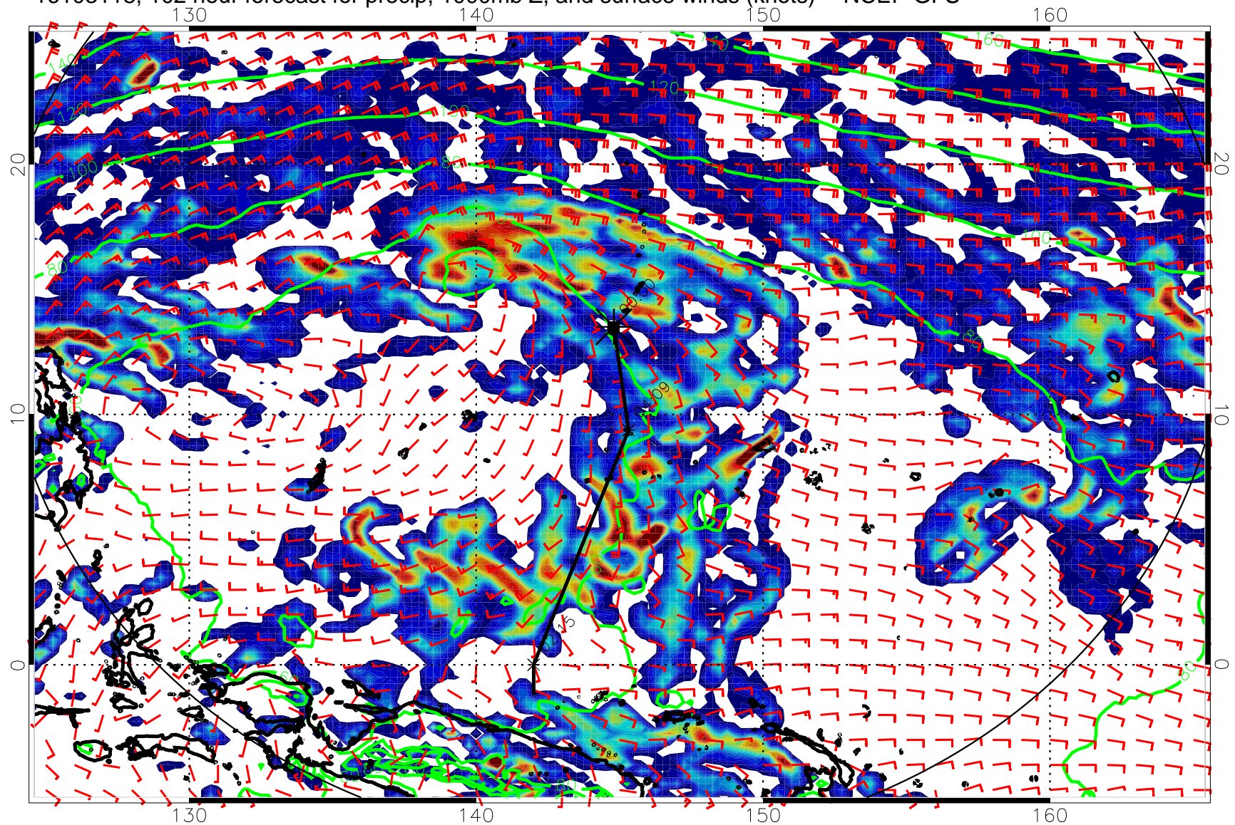
16103118, 102 hour forecast for precip, 1000mb Z, and surface winds (knots) -- NCEP GFS
