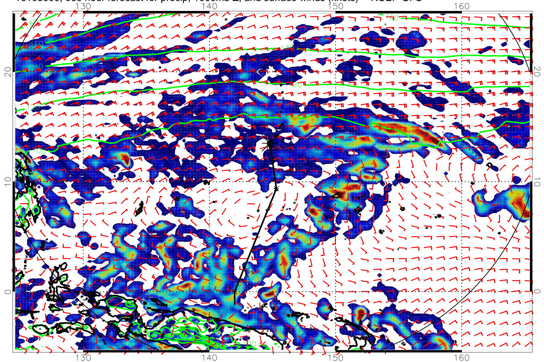
16103000, 060 hour forecast for precip, 1000mb Z, and surface winds (knots) -- NCEP GFS
