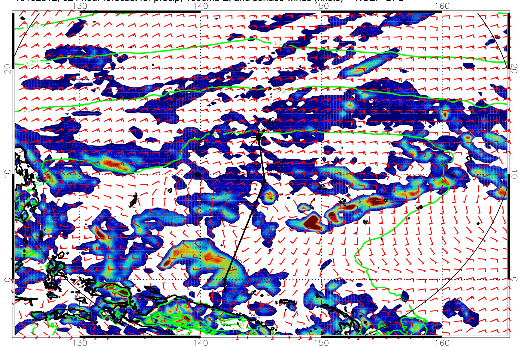
16102812, 024 hour forecast for precip, 1000mb Z, and surface winds (knots) -- NCEP GFS
