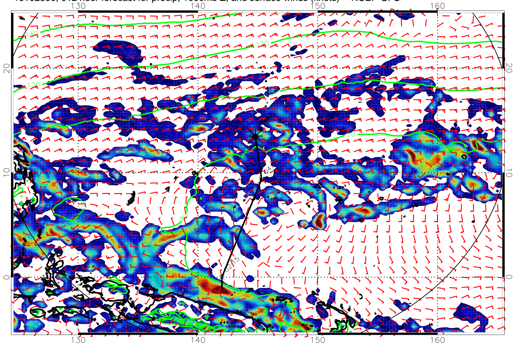
16102800, 012 hour forecast for precip, 1000mb Z, and surface winds (knots) -- NCEP GFS
