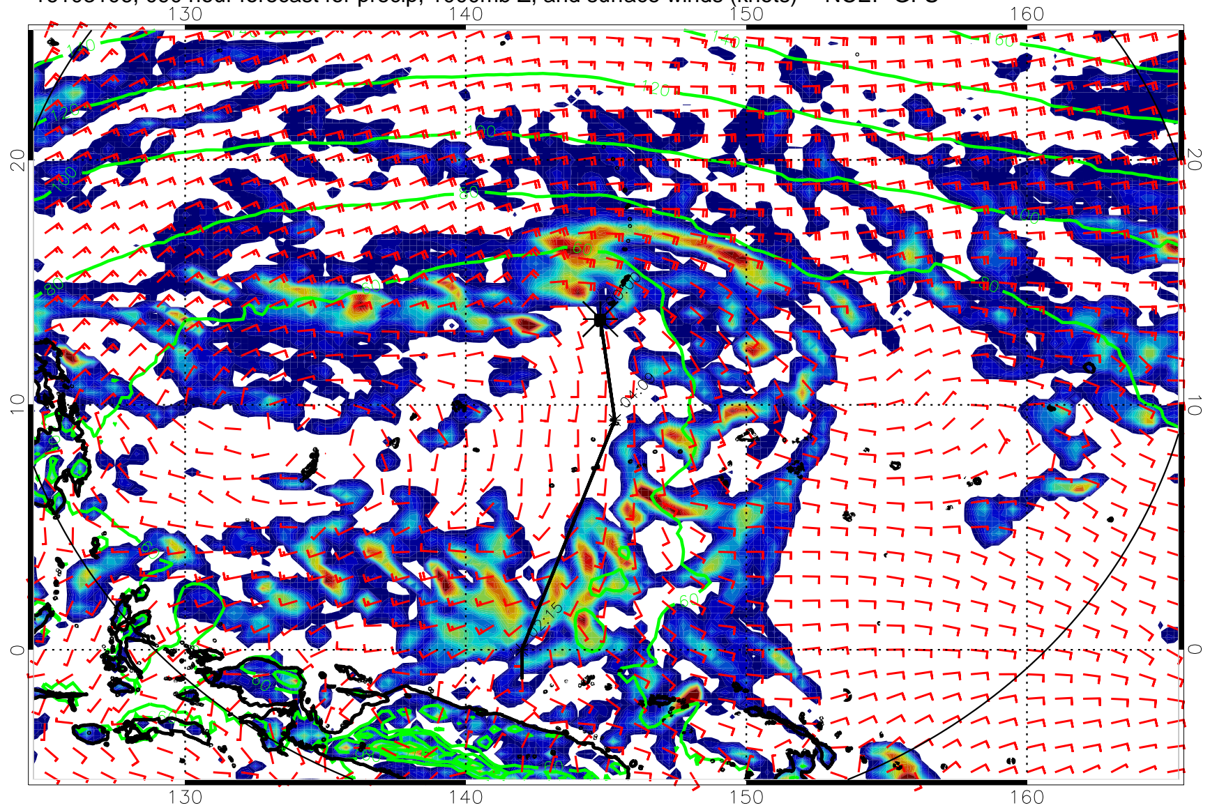
16103106, 090 hour forecast for precip, 1000mb Z, and surface winds (knots) -- NCEP GFS
