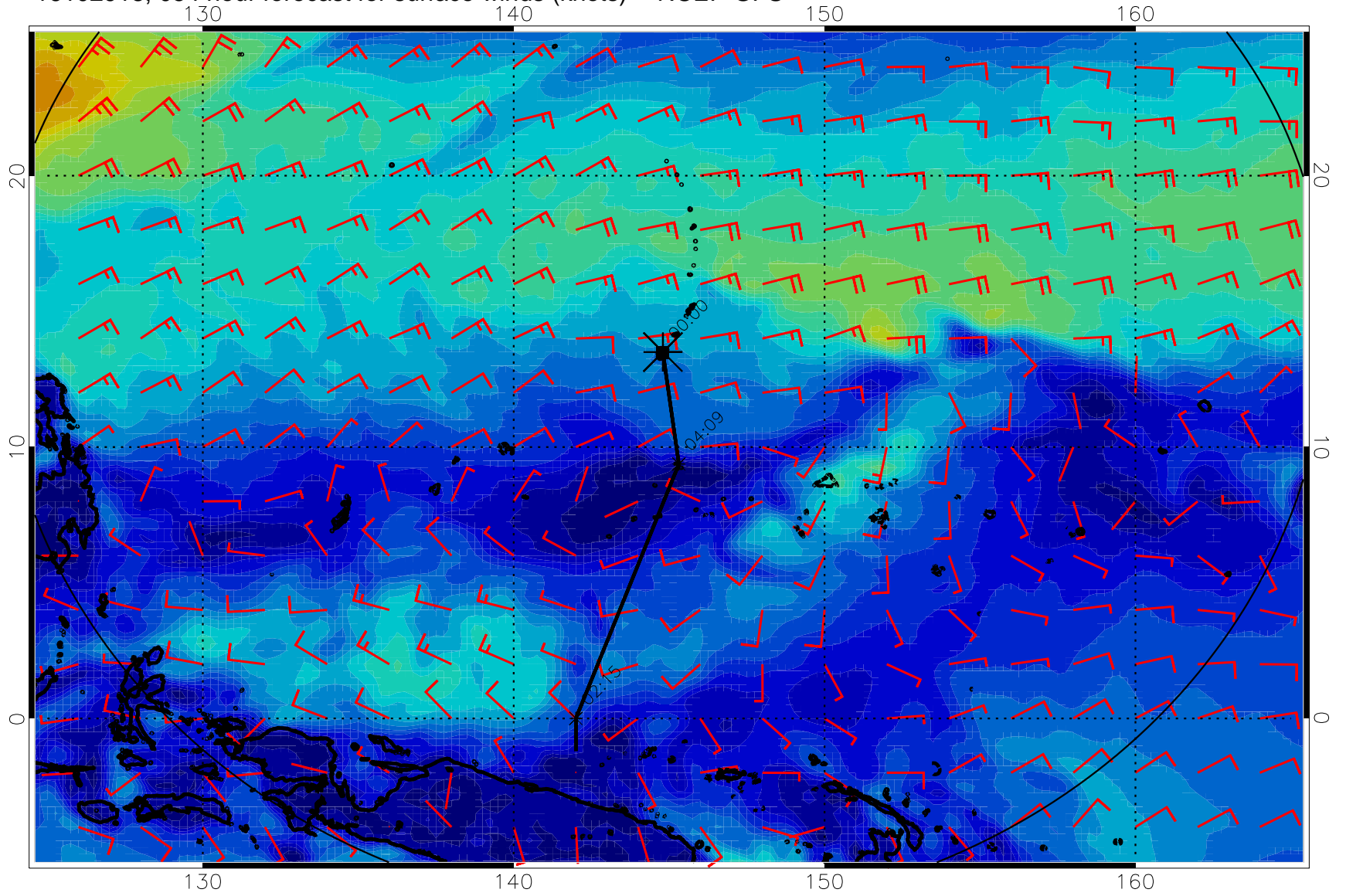
16102918, 054 hour forecast for surface winds (knots) -- NCEP GFS
