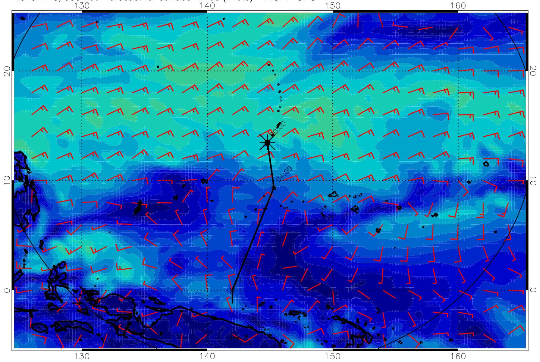
16102718, 006 hour forecast for surface winds (knots) -- NCEP GFS
