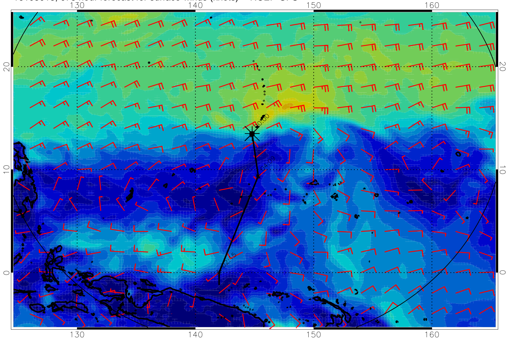
16103018, 078 hour forecast for surface winds (knots) -- NCEP GFS
