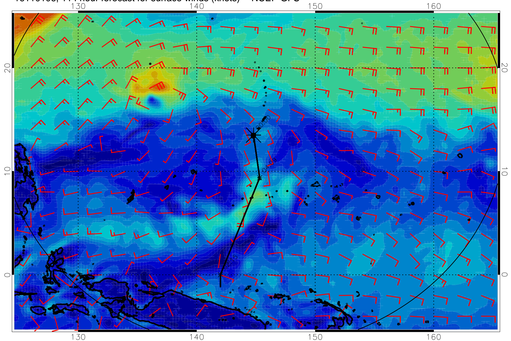
16110106, 114 hour forecast for surface winds (knots) -- NCEP GFS
