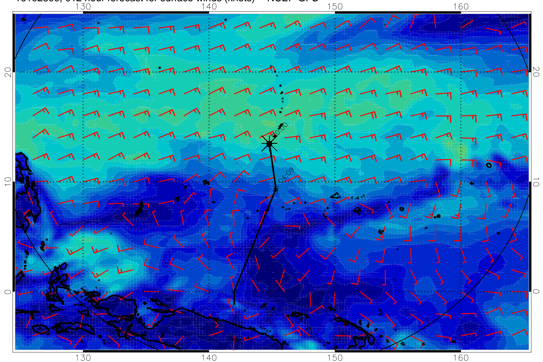
16102800, 012 hour forecast for surface winds (knots) -- NCEP GFS
