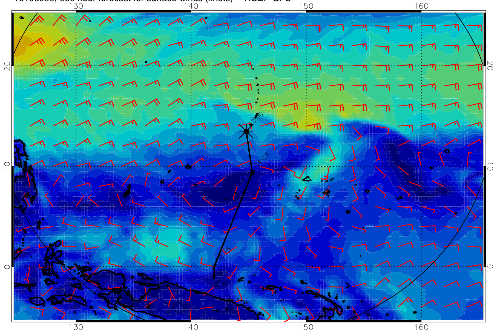
16103000, 060 hour forecast for surface winds (knots) -- NCEP GFS
