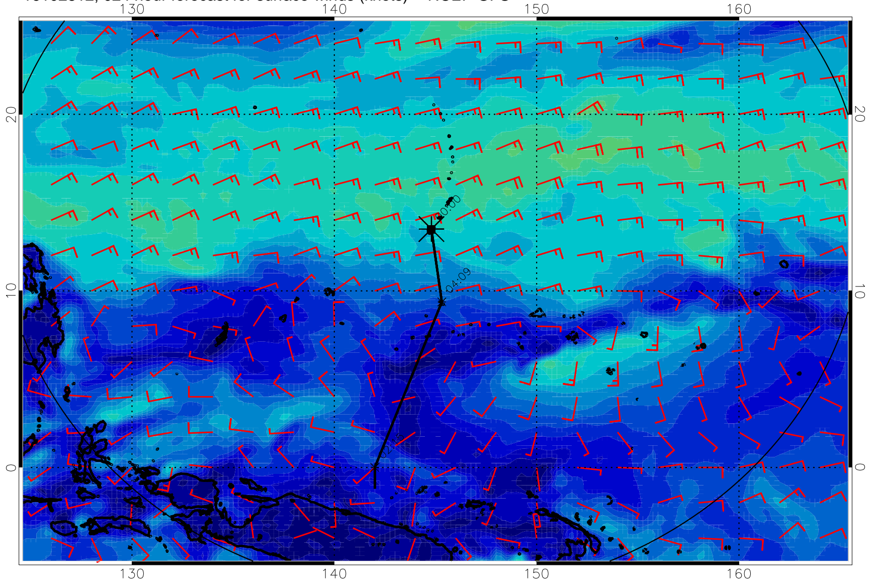
16102812, 024 hour forecast for surface winds (knots) -- NCEP GFS
