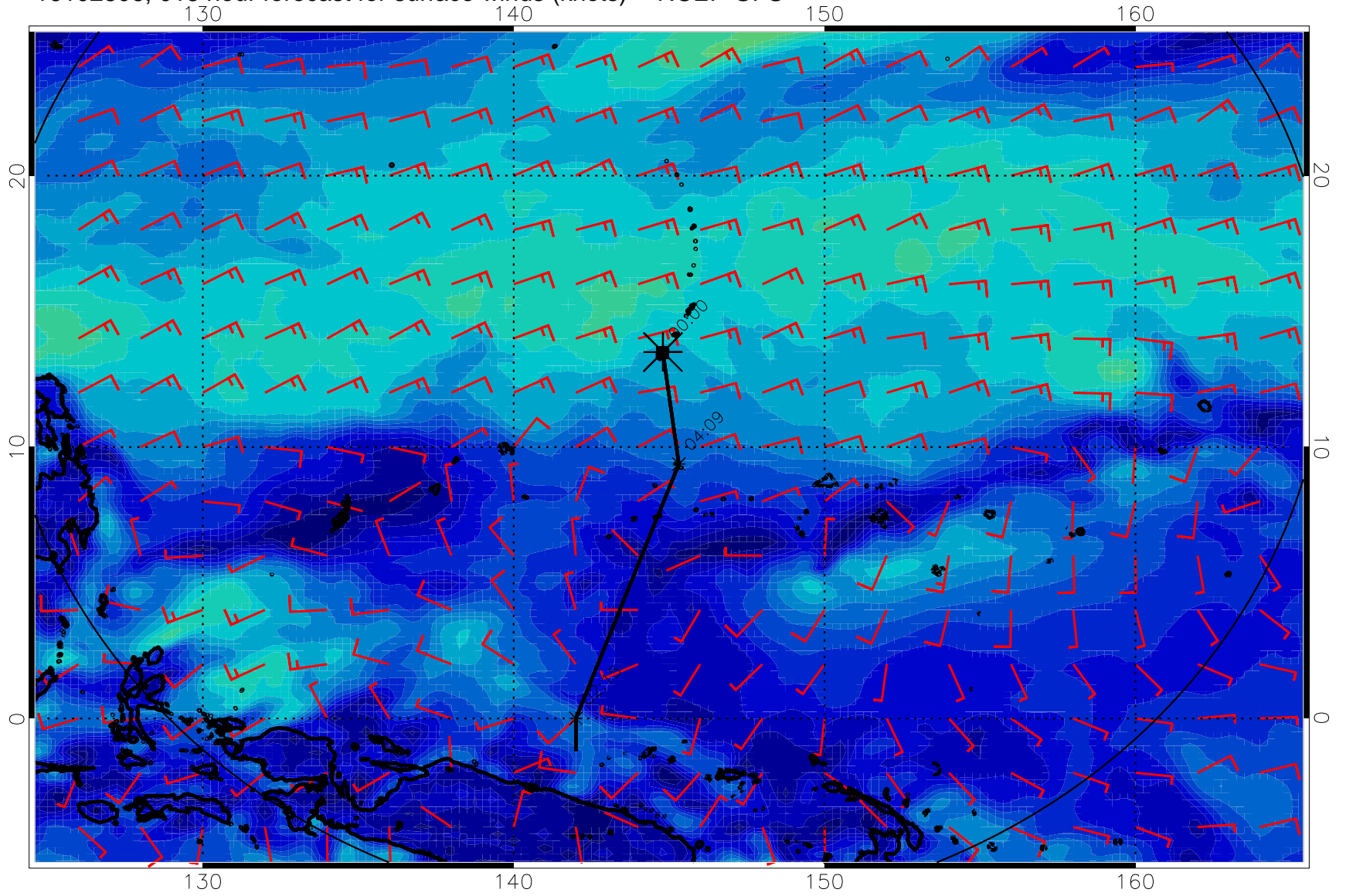
16102806, 018 hour forecast for surface winds (knots) -- NCEP GFS
