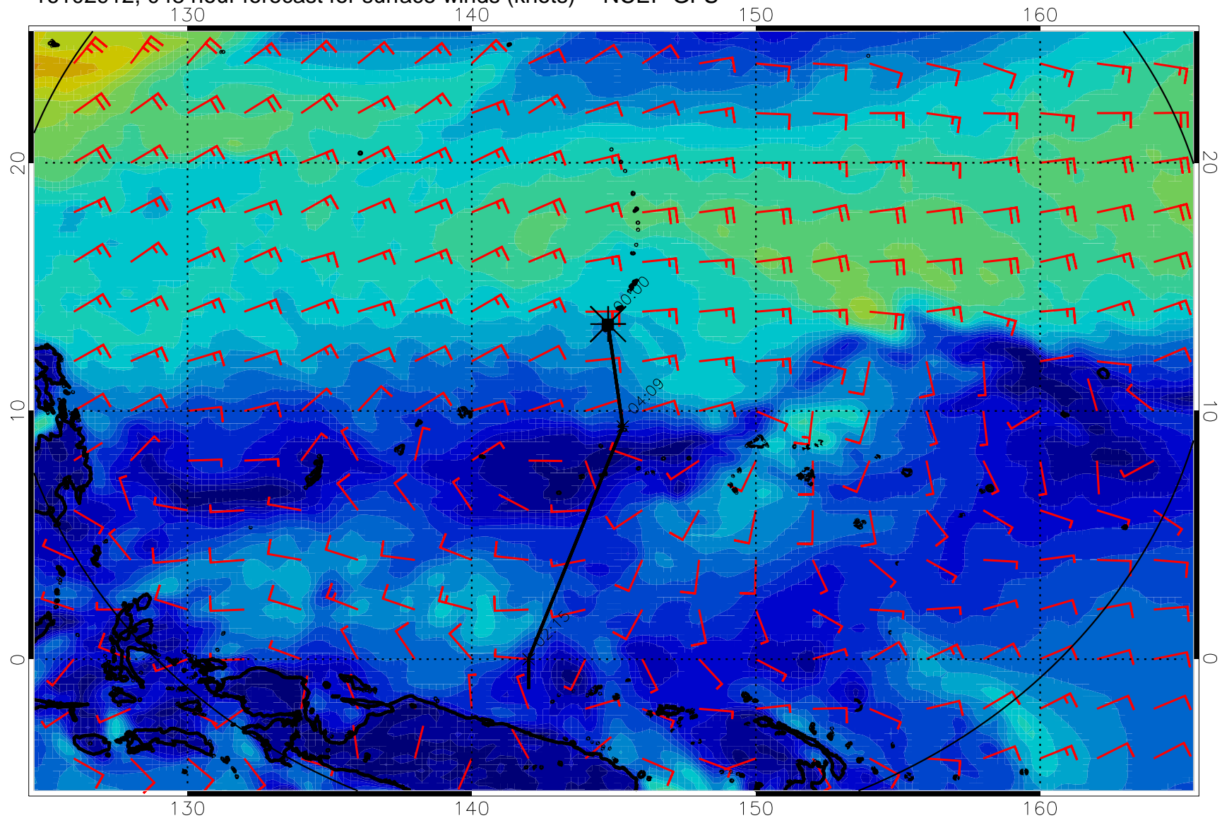
16102912, 048 hour forecast for surface winds (knots) -- NCEP GFS
