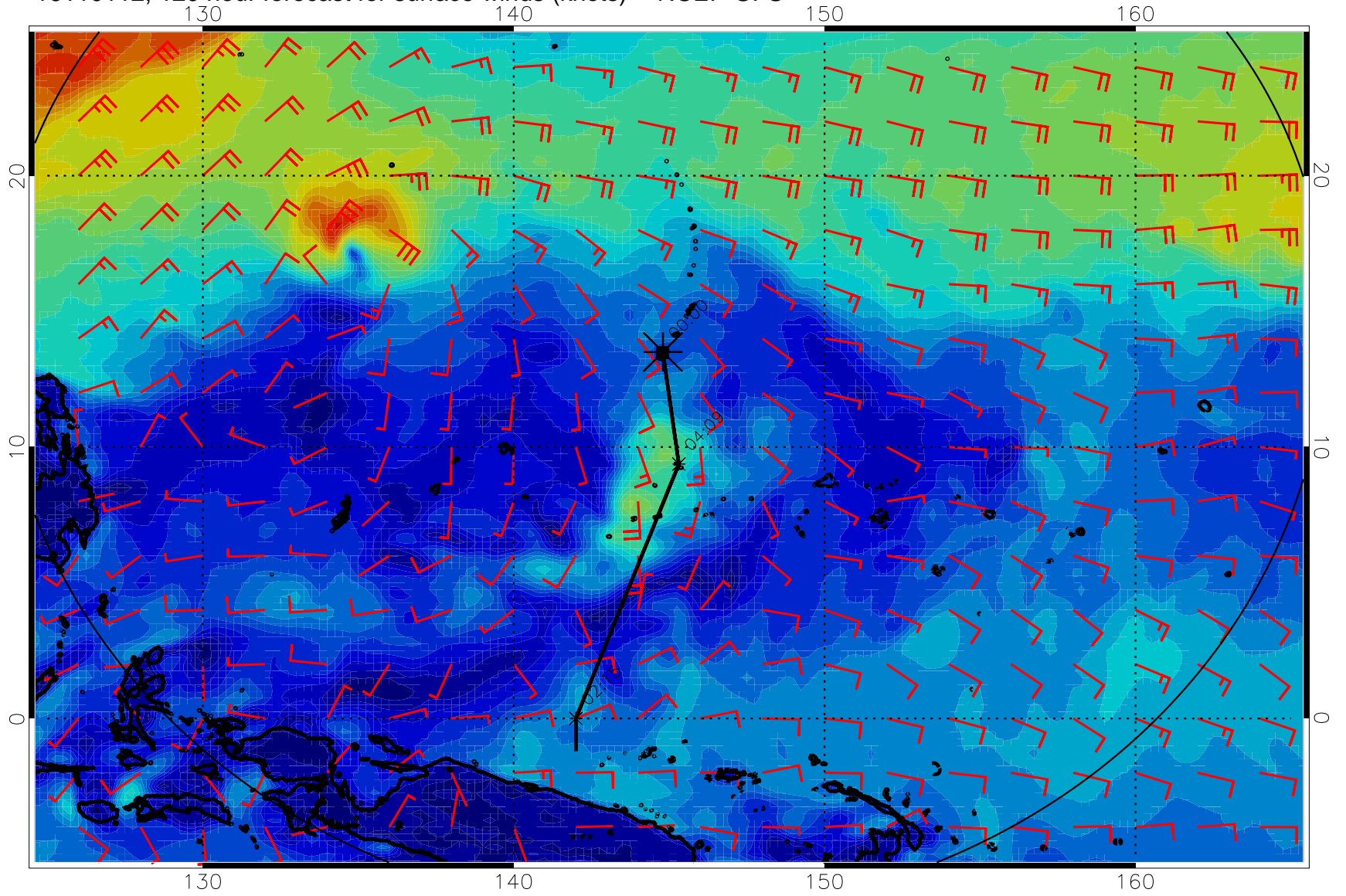
16110112, 120 hour forecast for surface winds (knots) -- NCEP GFS
