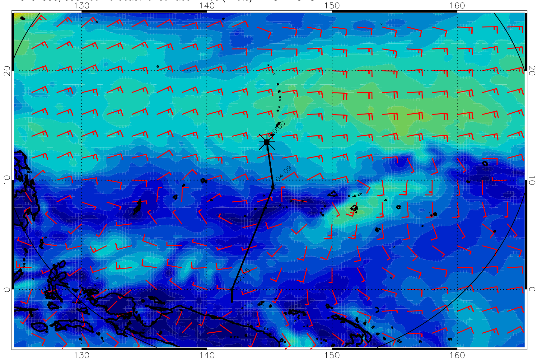
16102900, 036 hour forecast for surface winds (knots) -- NCEP GFS
