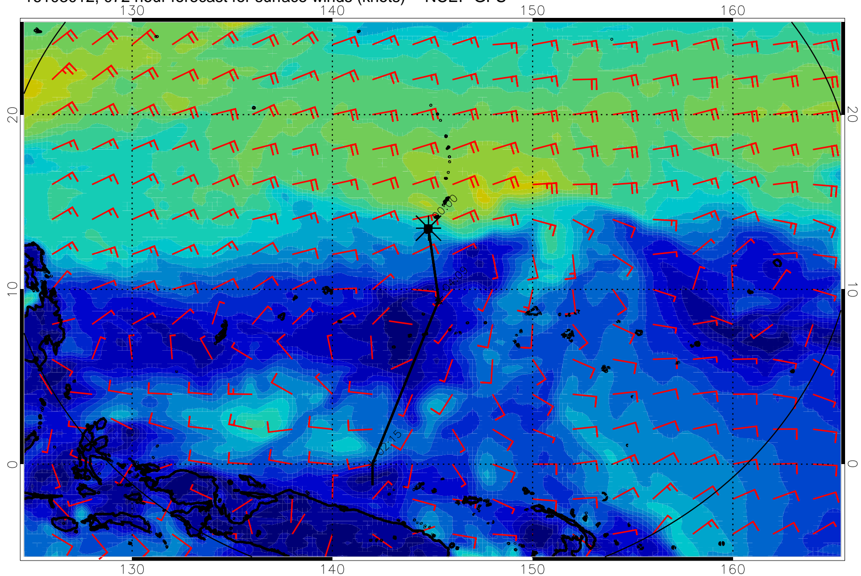
16103012, 072 hour forecast for surface winds (knots) -- NCEP GFS
