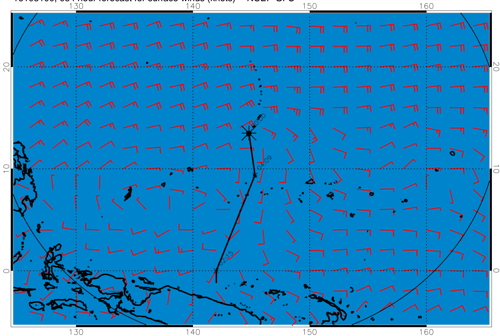
16103100, 084 hour forecast for surface winds (knots) -- NCEP GFS
