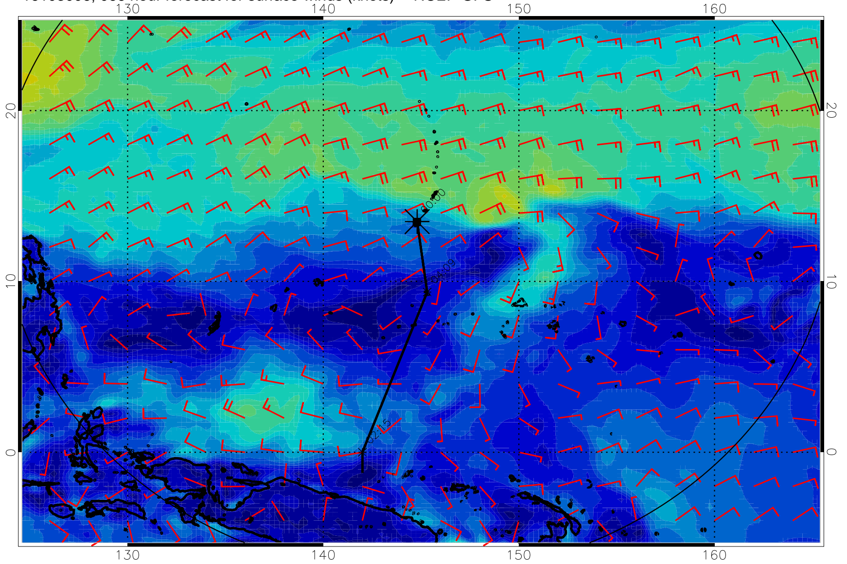
16103006, 066 hour forecast for surface winds (knots) -- NCEP GFS
