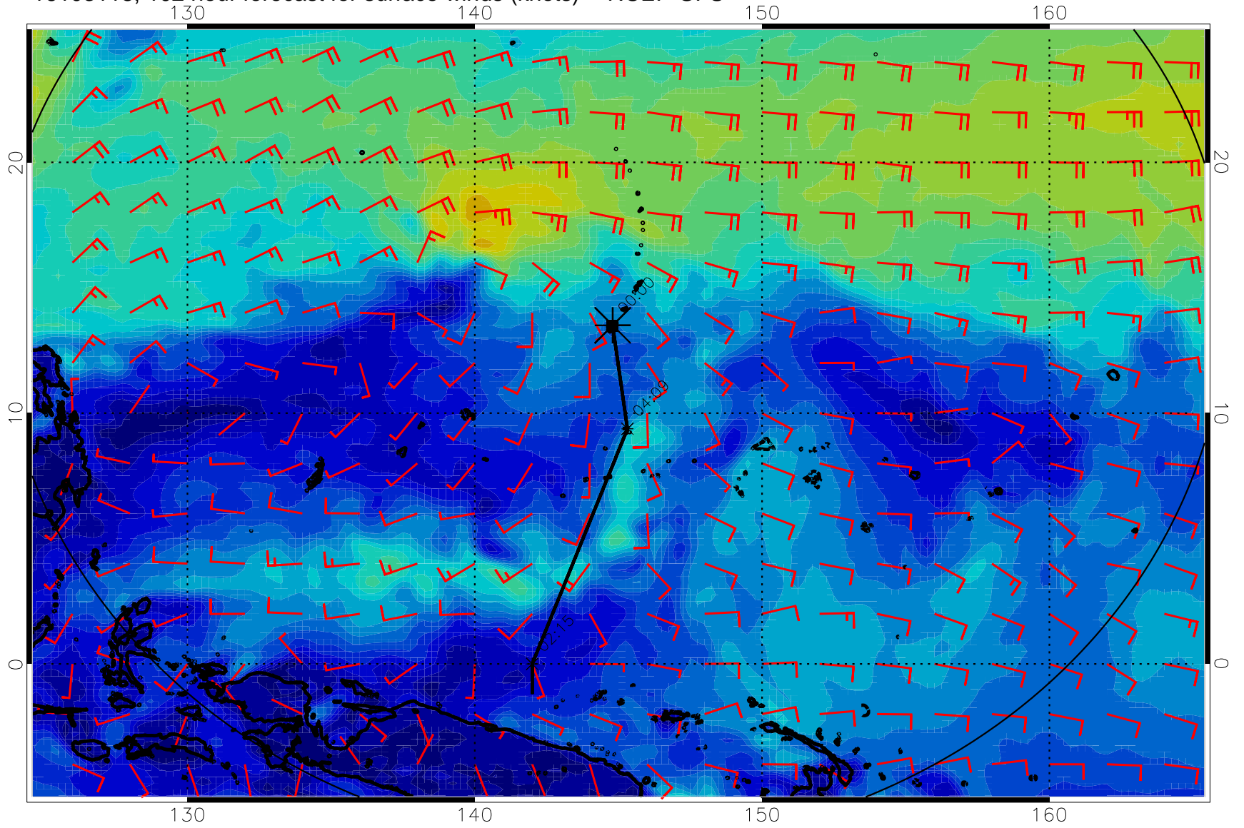
16103118, 102 hour forecast for surface winds (knots) -- NCEP GFS
