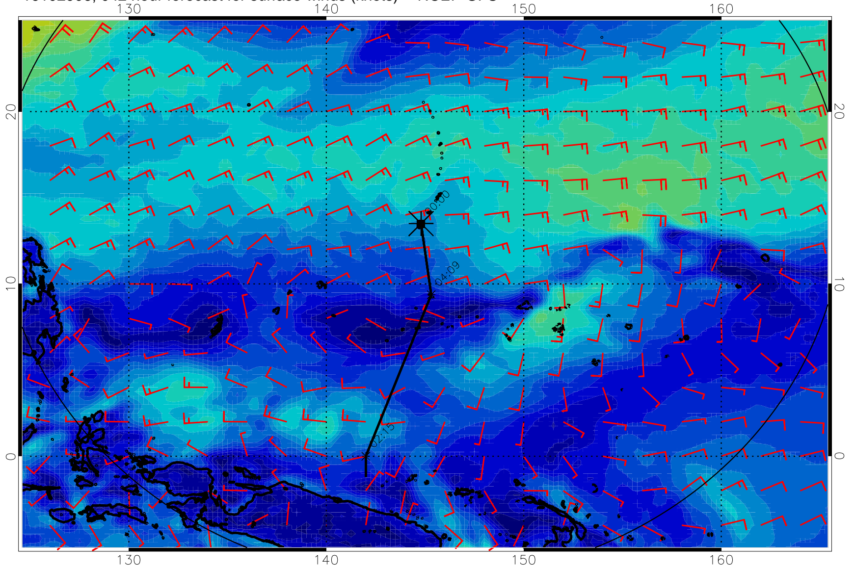
16102906, 042 hour forecast for surface winds (knots) -- NCEP GFS
