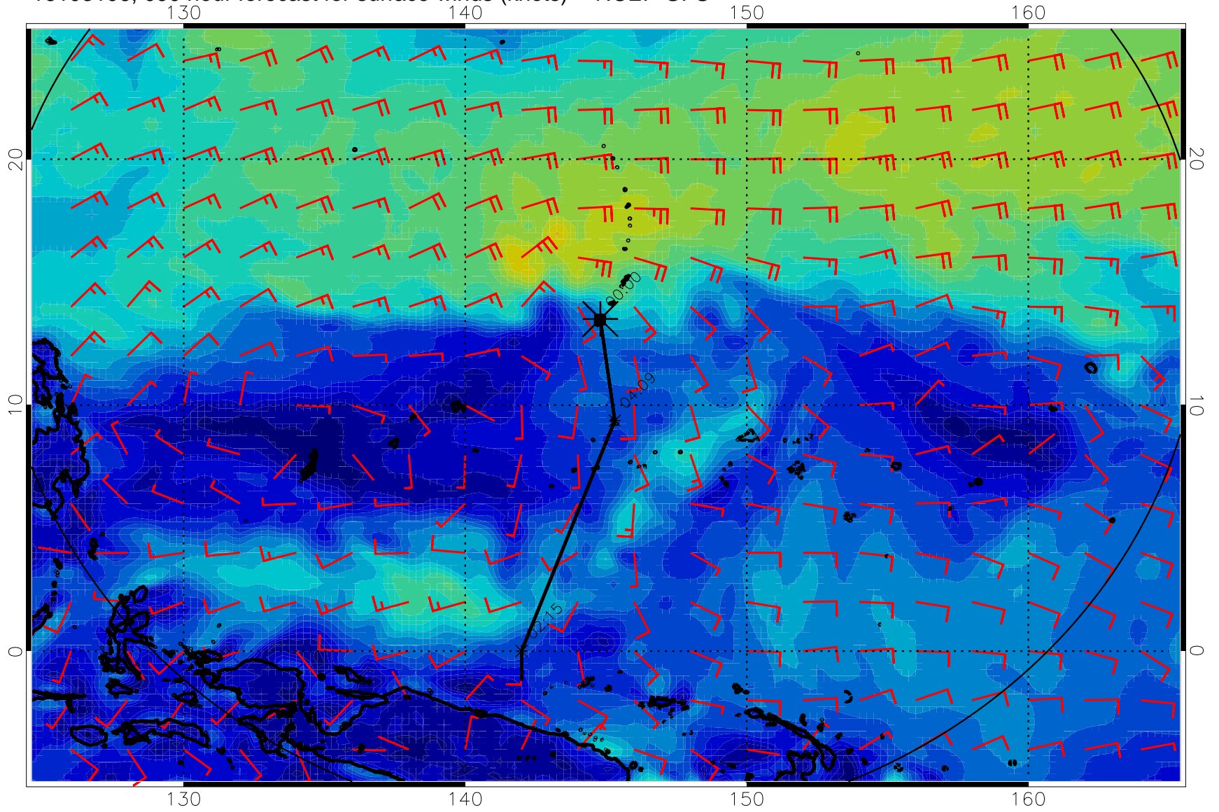
16103106, 090 hour forecast for surface winds (knots) -- NCEP GFS
