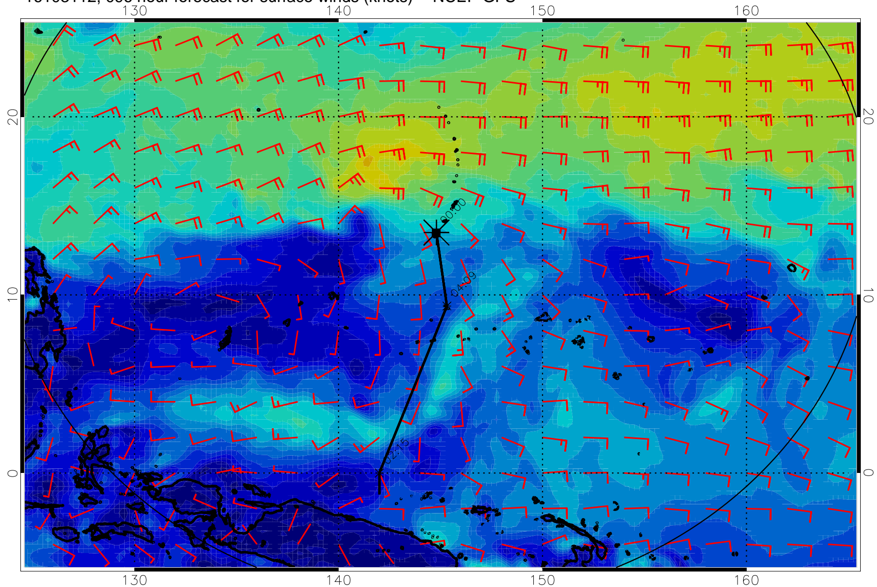
16103112, 096 hour forecast for surface winds (knots) -- NCEP GFS
