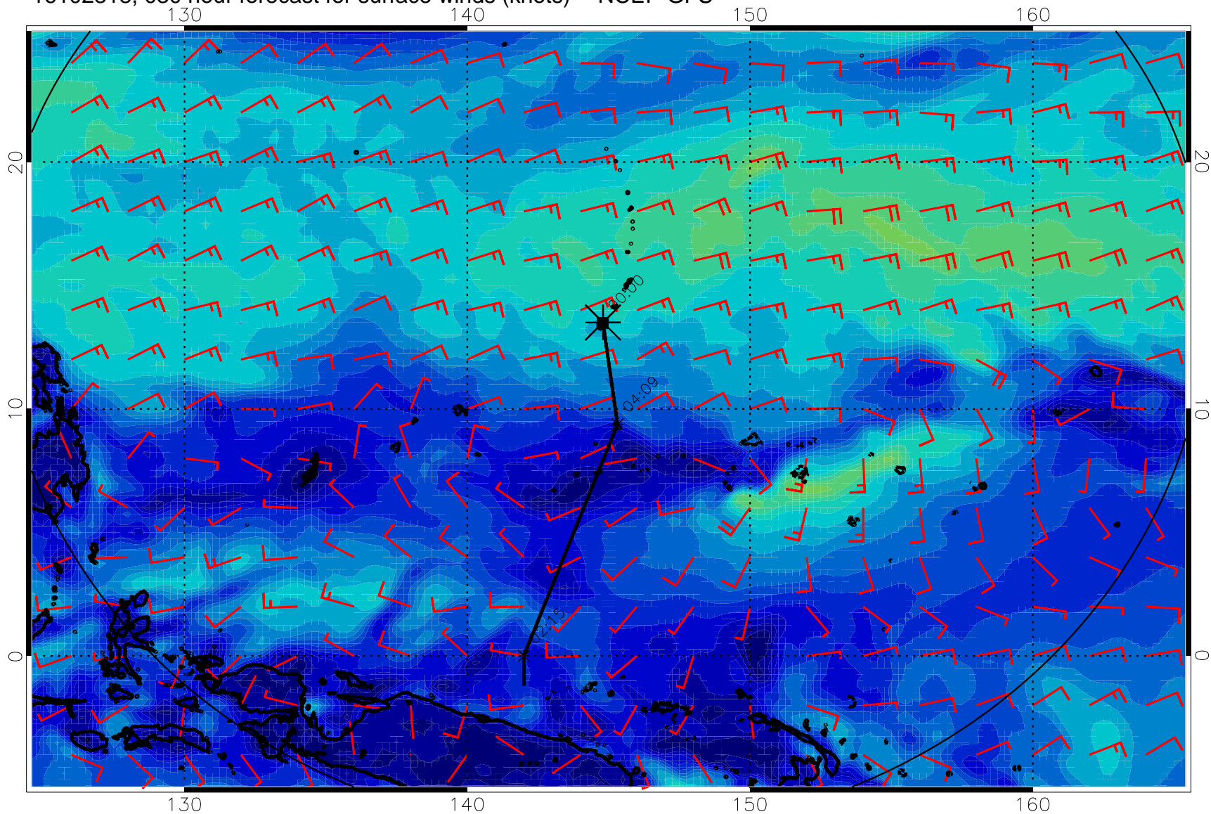
16102818, 030 hour forecast for surface winds (knots) -- NCEP GFS
