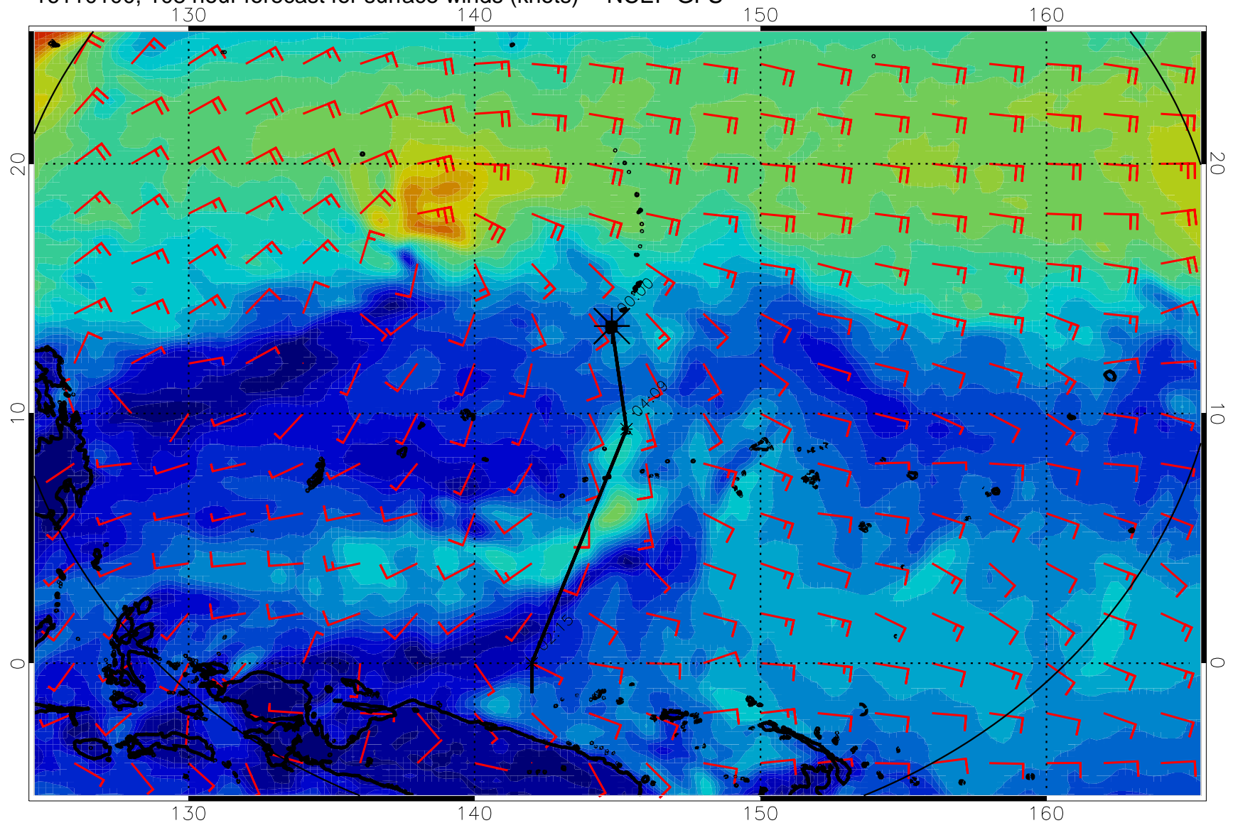
16110100, 108 hour forecast for surface winds (knots) -- NCEP GFS
