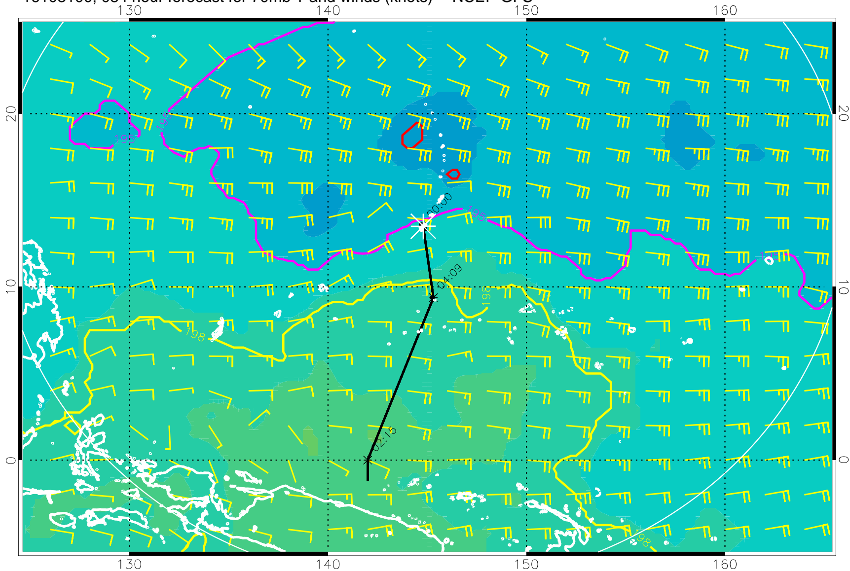
16103100, 084 hour forecast for 70mb T and winds (knots) -- NCEP GFS
