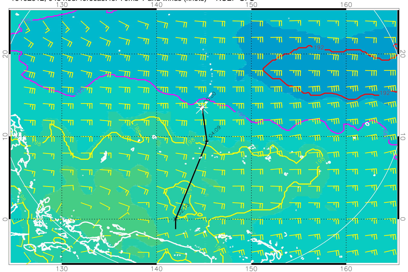
16102912, 048 hour forecast for 70mb T and winds (knots) -- NCEP GFS
