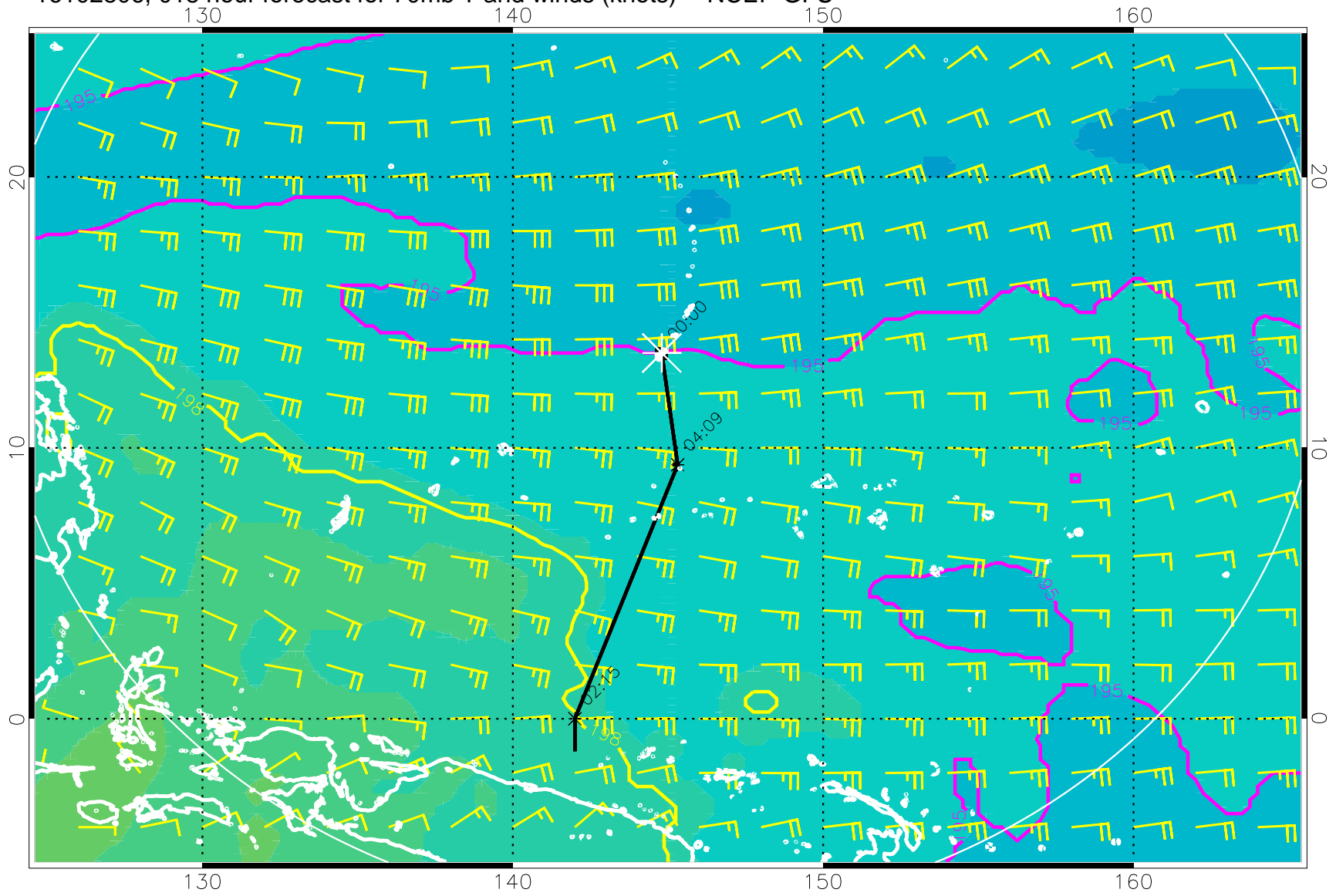
16102806, 018 hour forecast for 70mb T and winds (knots) -- NCEP GFS
