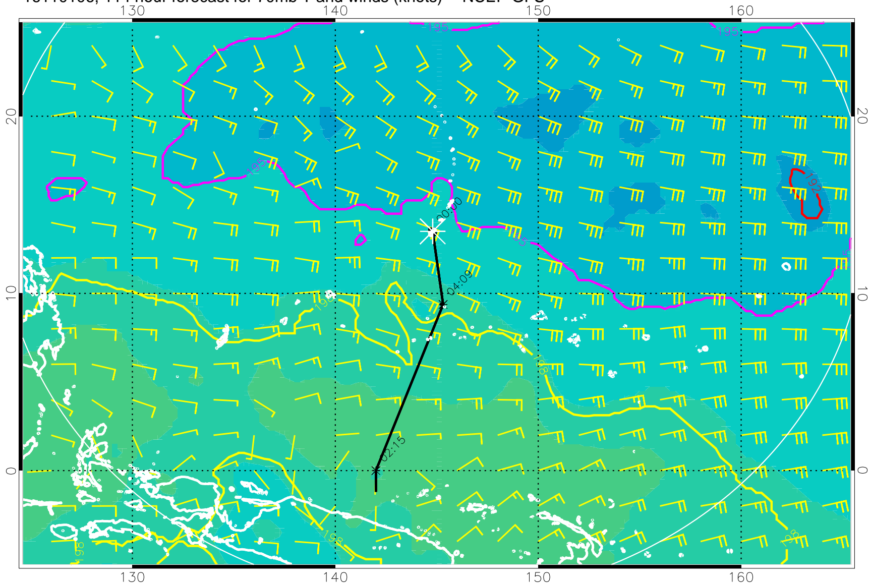
16110106, 114 hour forecast for 70mb T and winds (knots) -- NCEP GFS
