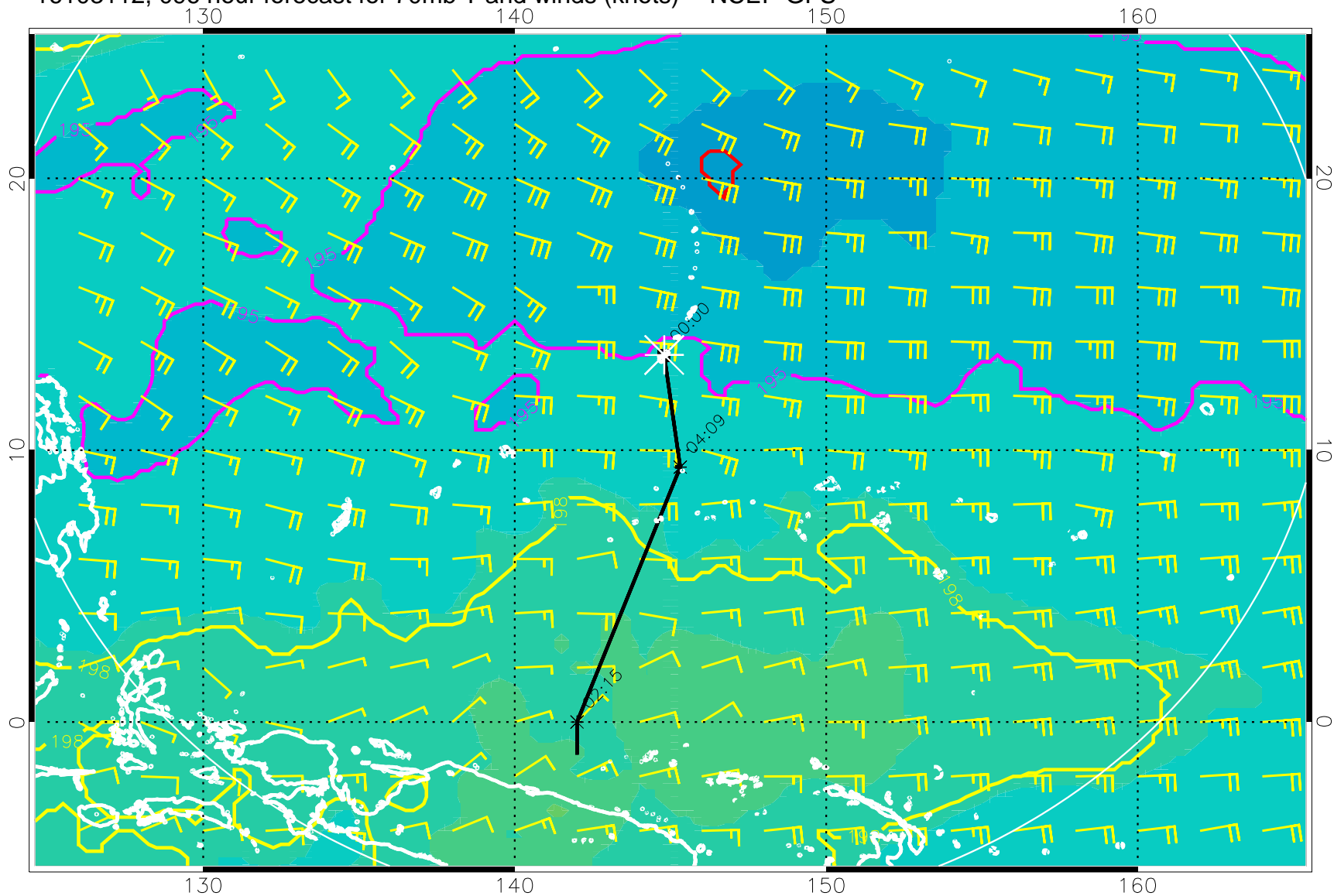
16103112, 096 hour forecast for 70mb T and winds (knots) -- NCEP GFS
