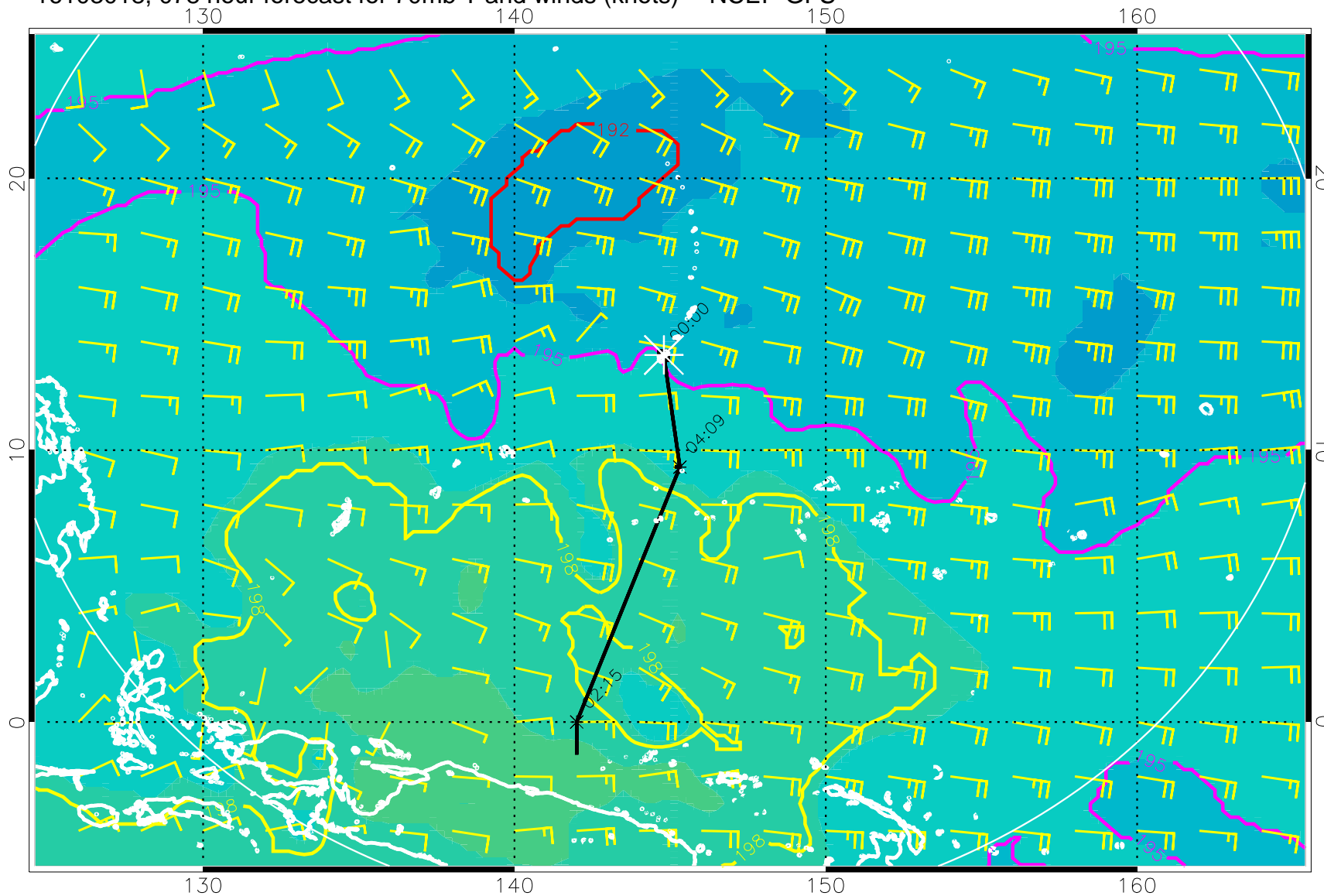
16103018, 078 hour forecast for 70mb T and winds (knots) -- NCEP GFS
