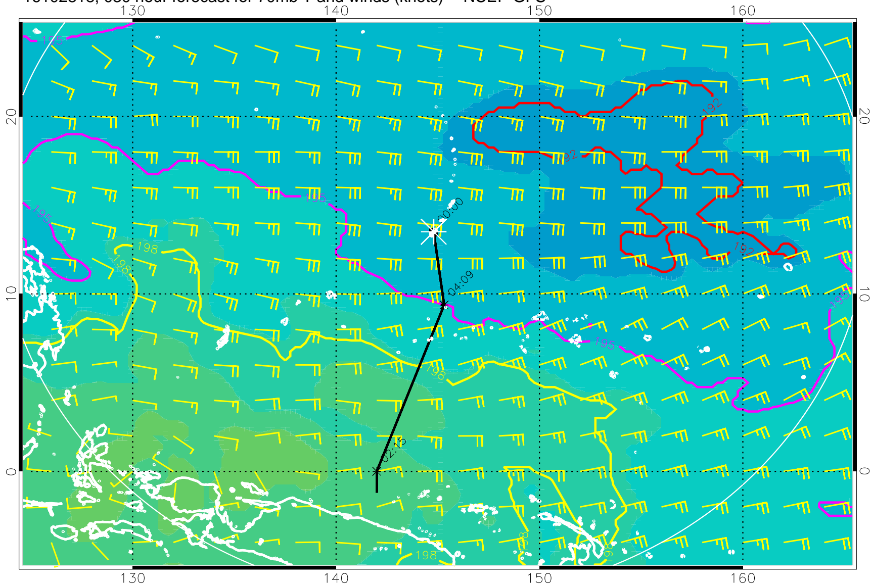
16102818, 030 hour forecast for 70mb T and winds (knots) -- NCEP GFS
