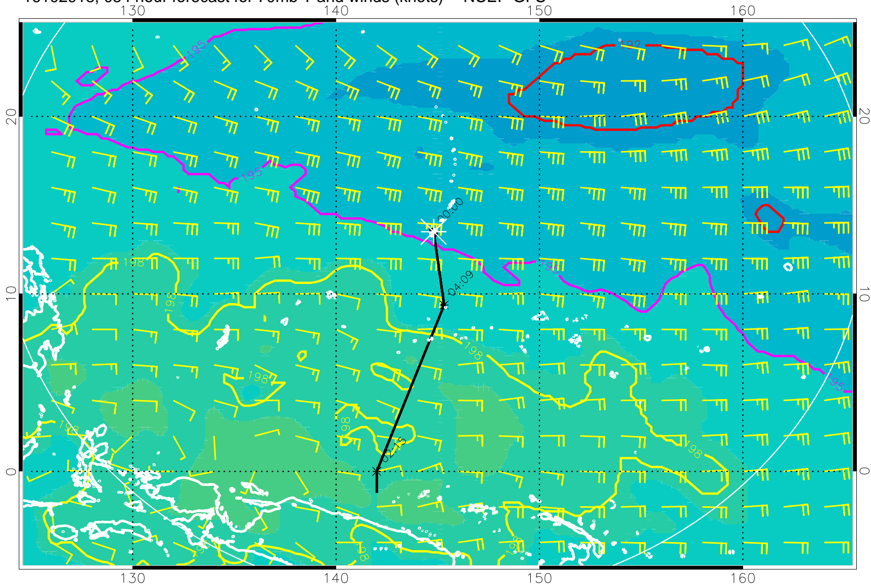
16102918, 054 hour forecast for 70mb T and winds (knots) -- NCEP GFS
