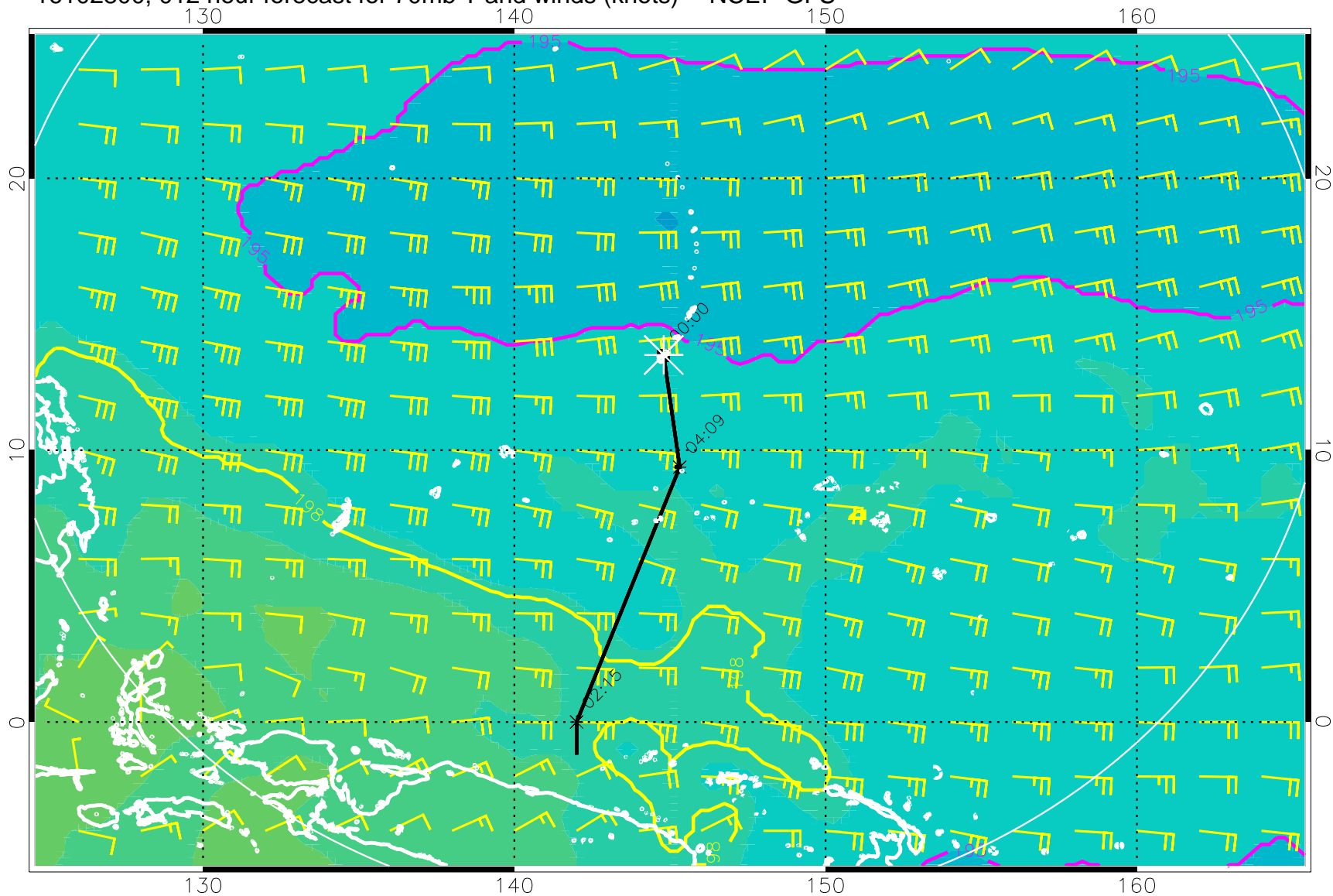
16102800, 012 hour forecast for 70mb T and winds (knots) -- NCEP GFS
