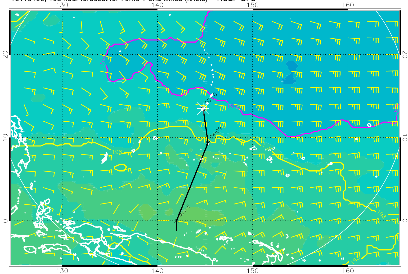
16110100, 108 hour forecast for 70mb T and winds (knots) -- NCEP GFS
