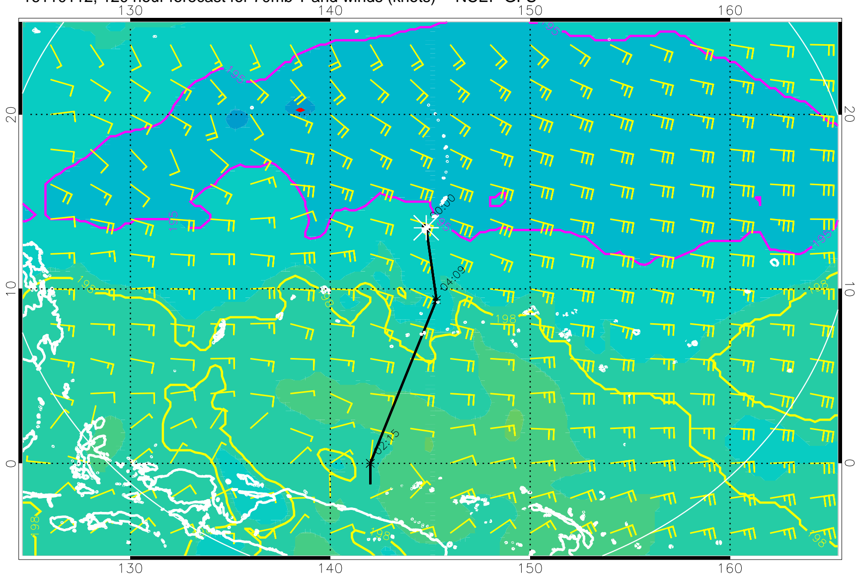
16110112, 120 hour forecast for 70mb T and winds (knots) -- NCEP GFS
