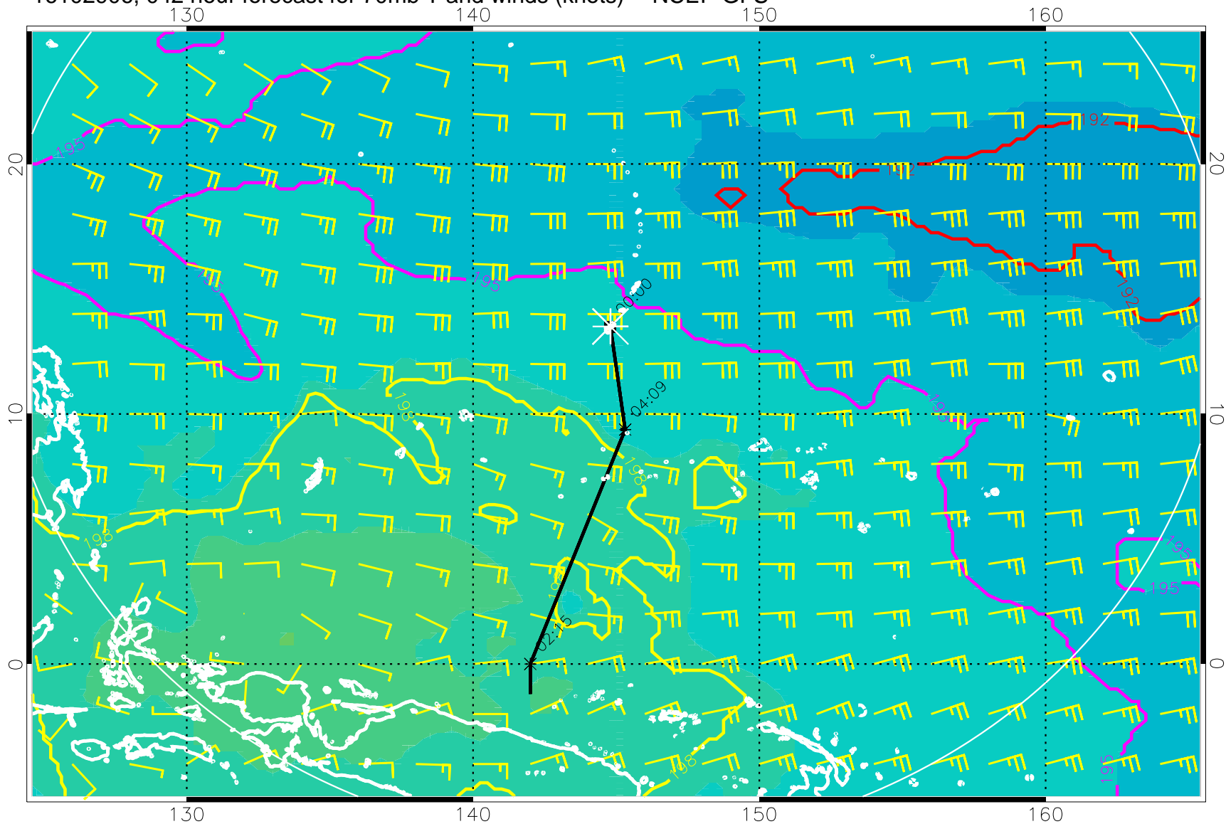
16102906, 042 hour forecast for 70mb T and winds (knots) -- NCEP GFS
