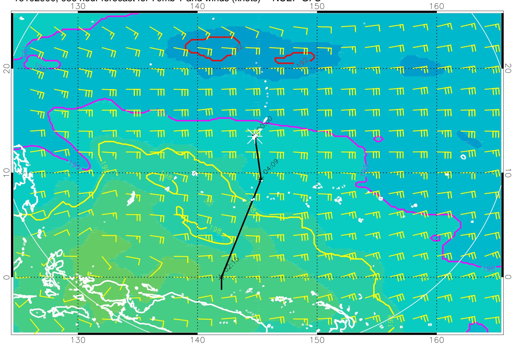
16102900, 036 hour forecast for 70mb T and winds (knots) -- NCEP GFS
