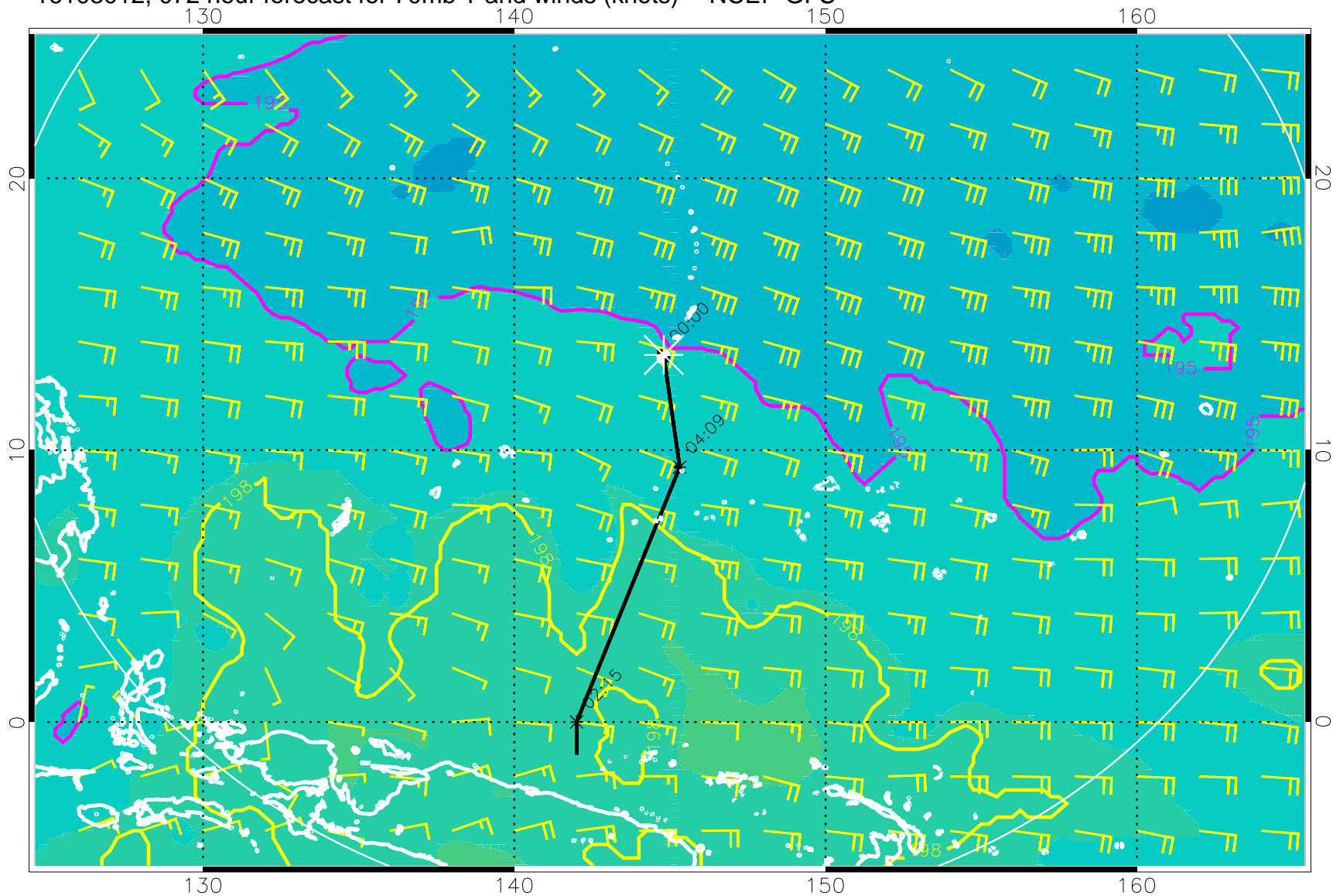
16103012, 072 hour forecast for 70mb T and winds (knots) -- NCEP GFS
