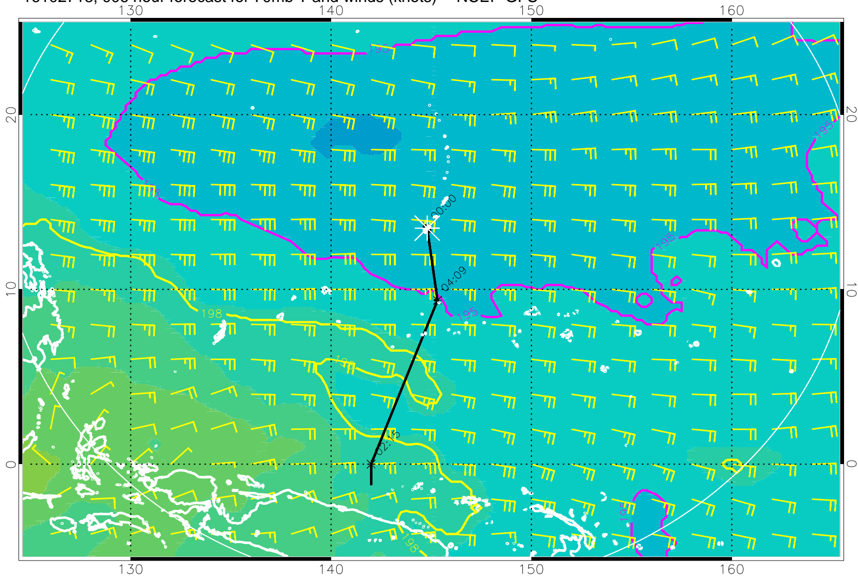
16102718, 006 hour forecast for 70mb T and winds (knots) -- NCEP GFS
