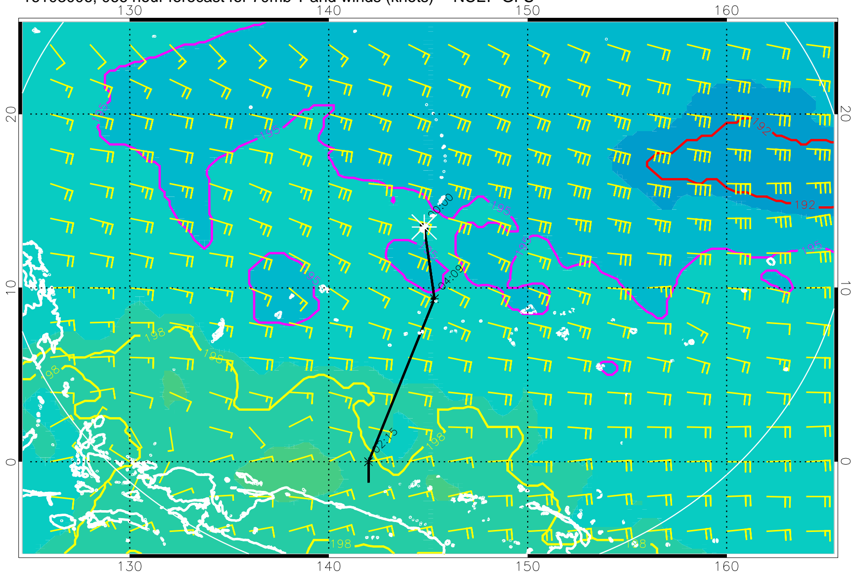
16103006, 066 hour forecast for 70mb T and winds (knots) -- NCEP GFS
