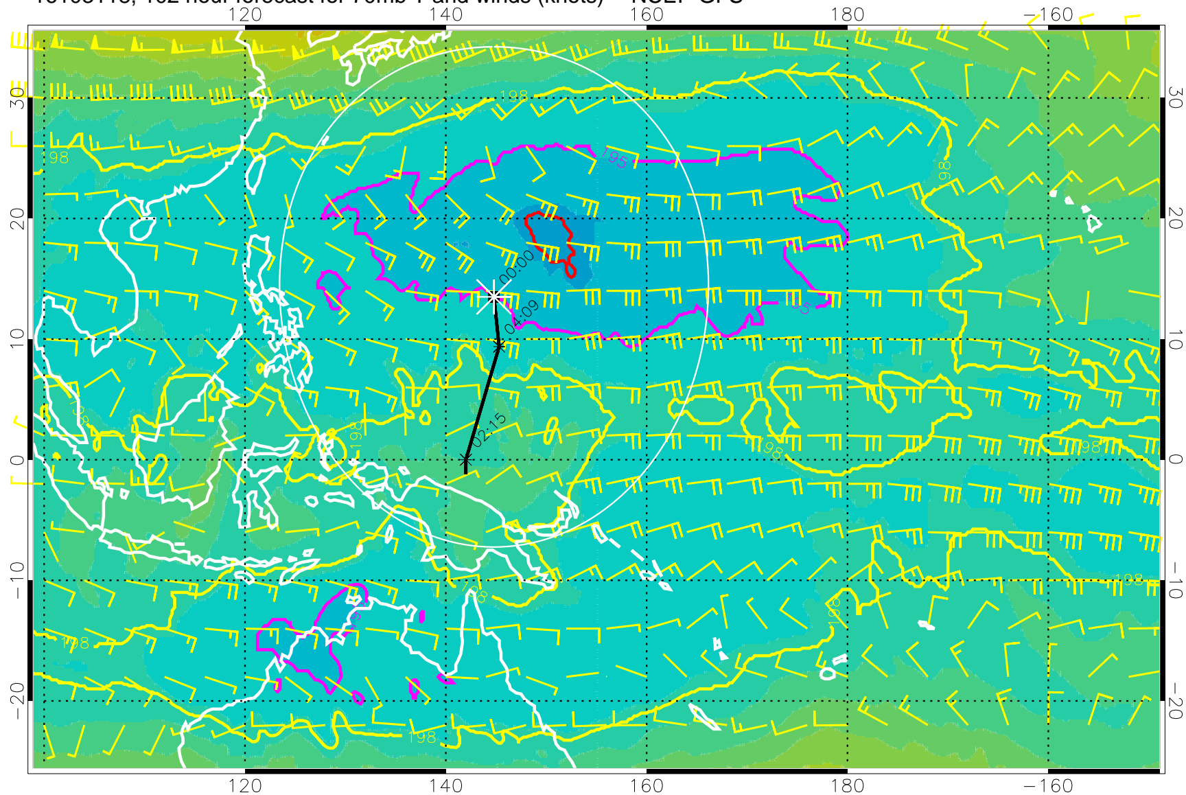
16103118, 102 hour forecast for 70mb T and winds (knots) -- NCEP GFS
