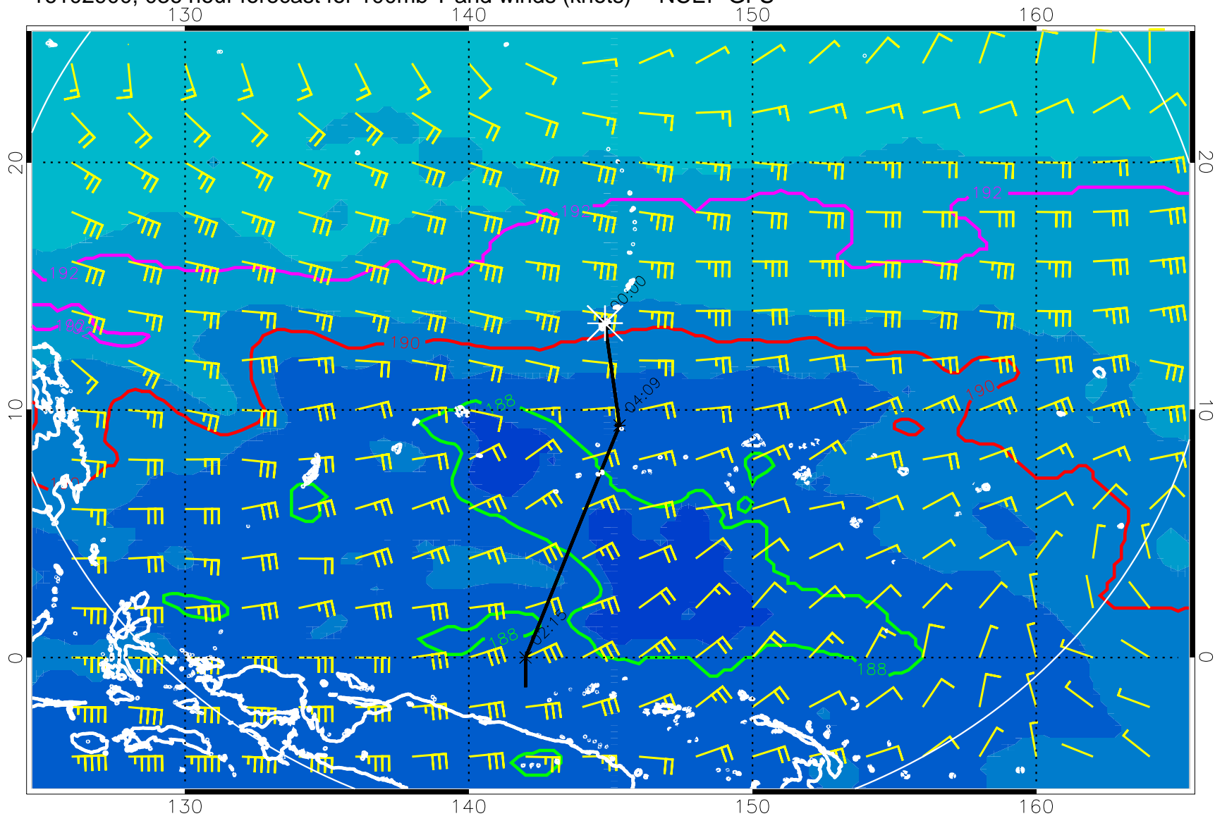
16102900, 036 hour forecast for 100mb T and winds (knots) -- NCEP GFS
