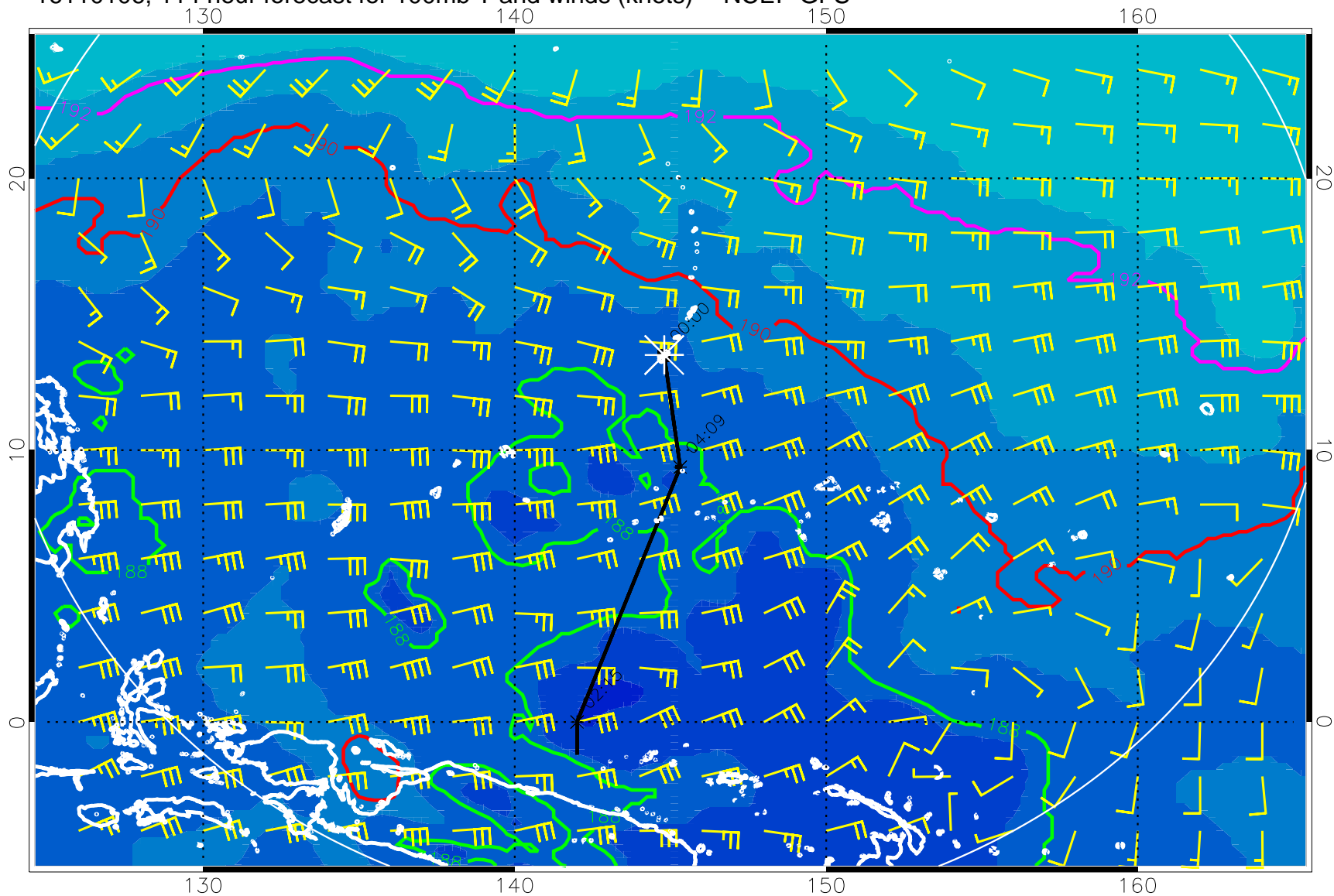
16110106, 114 hour forecast for 100mb T and winds (knots) -- NCEP GFS
