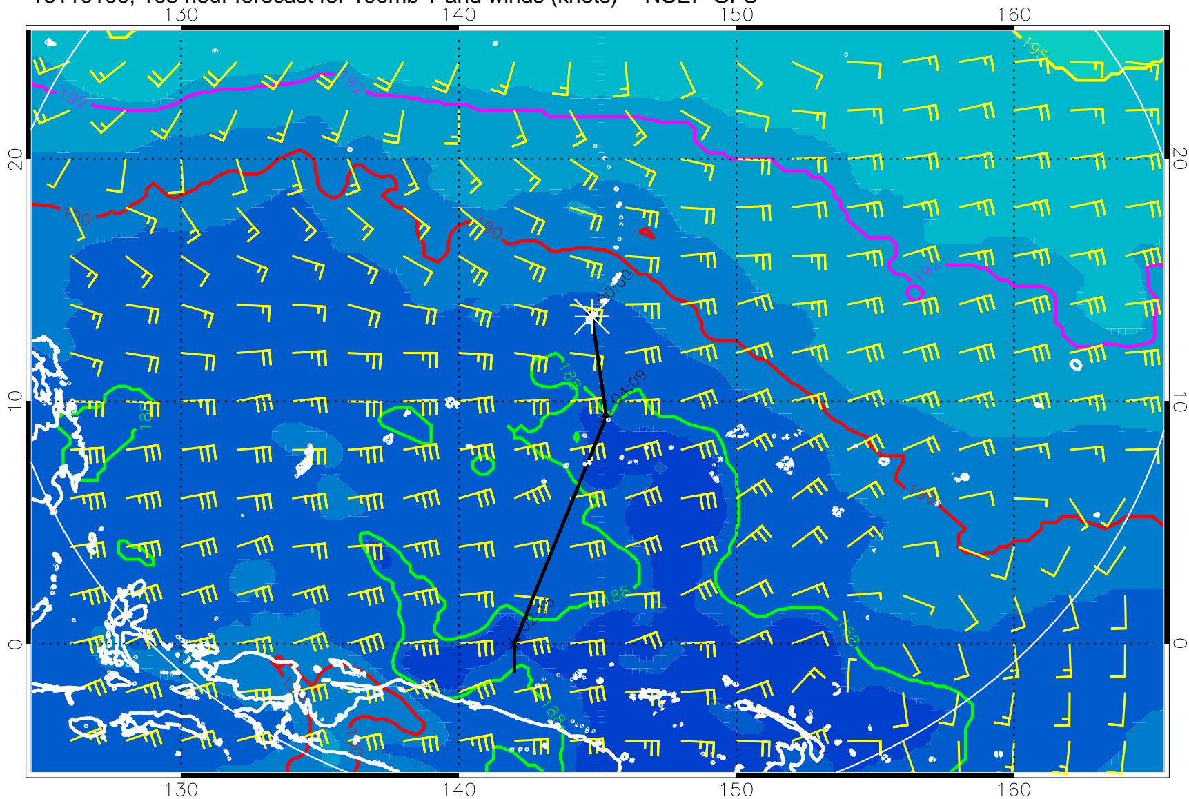
16110100, 108 hour forecast for 100mb T and winds (knots) -- NCEP GFS
