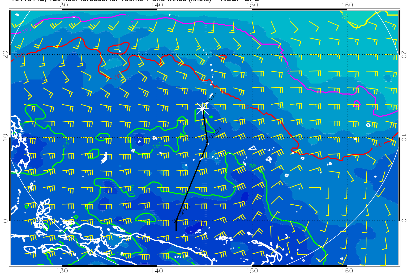
16110112, 120 hour forecast for 100mb T and winds (knots) -- NCEP GFS
