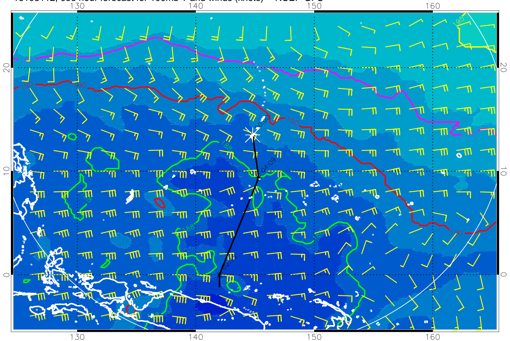
16103112, 096 hour forecast for 100mb T and winds (knots) -- NCEP GFS
