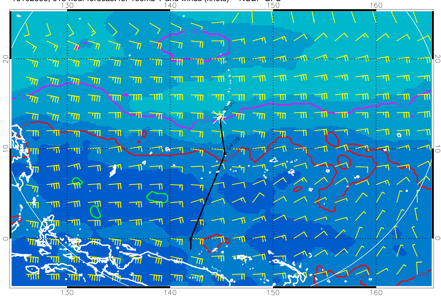
16102806, 018 hour forecast for 100mb T and winds (knots) -- NCEP GFS
