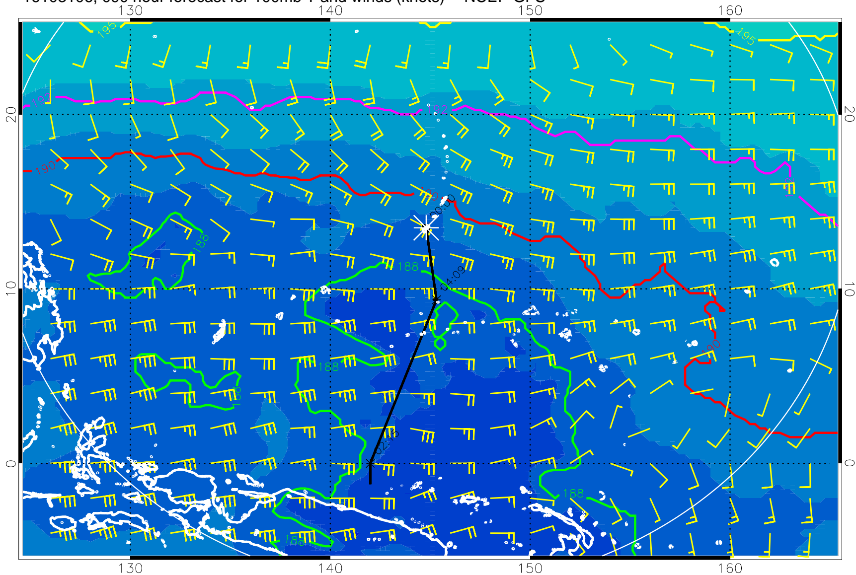
16103106, 090 hour forecast for 100mb T and winds (knots) -- NCEP GFS
