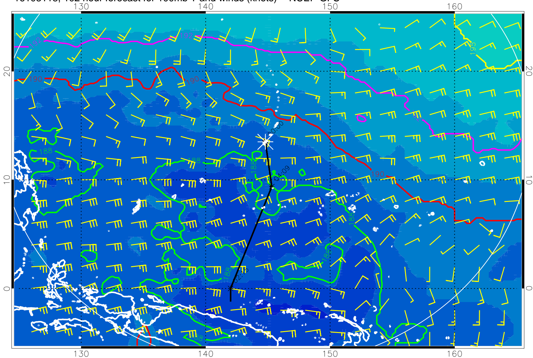
16103118, 102 hour forecast for 100mb T and winds (knots) -- NCEP GFS
