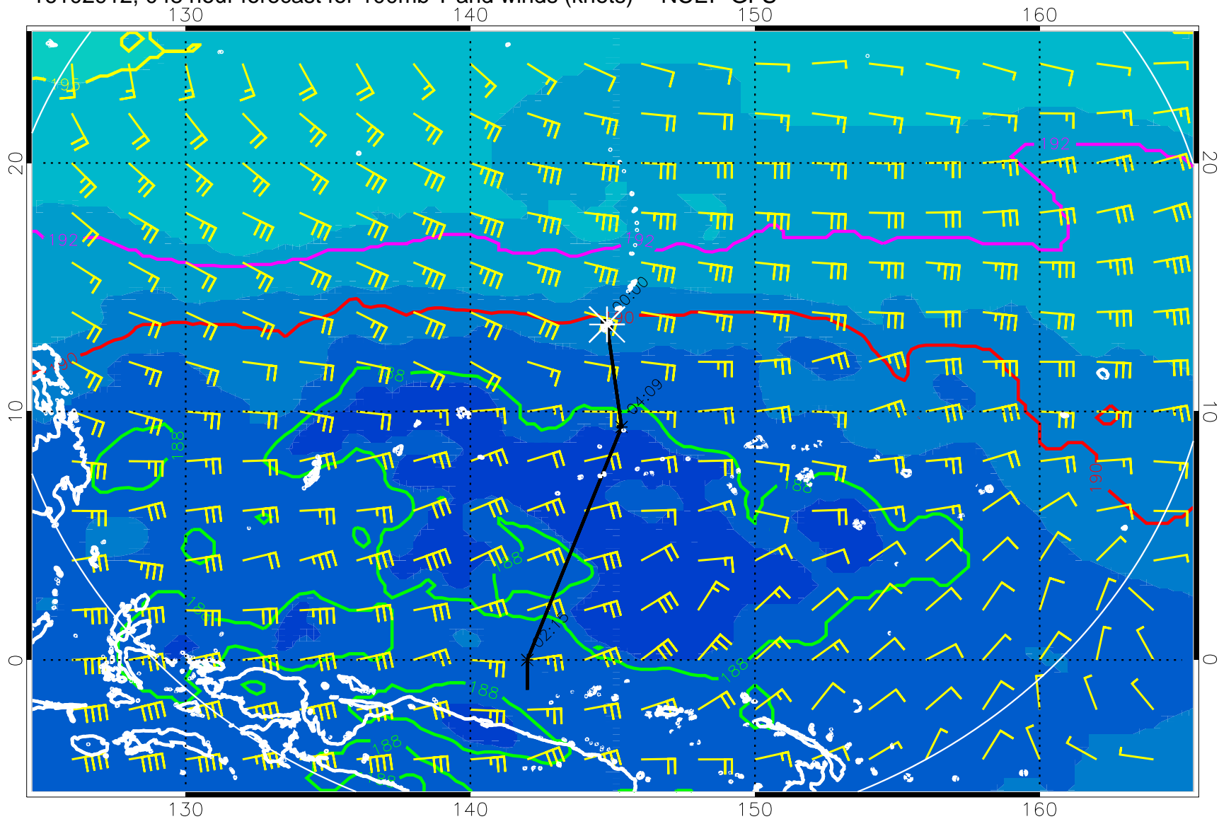
16102912, 048 hour forecast for 100mb T and winds (knots) -- NCEP GFS
