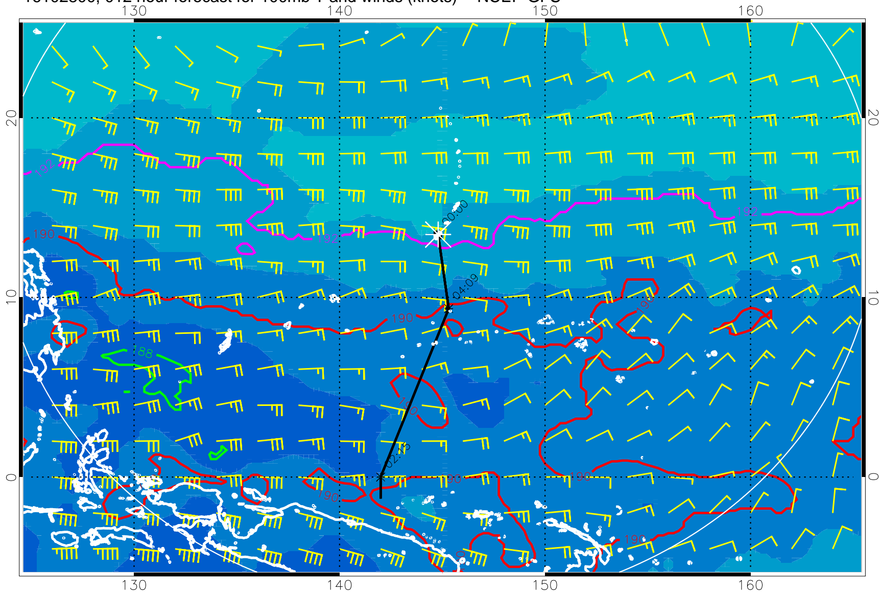
16102800, 012 hour forecast for 100mb T and winds (knots) -- NCEP GFS
