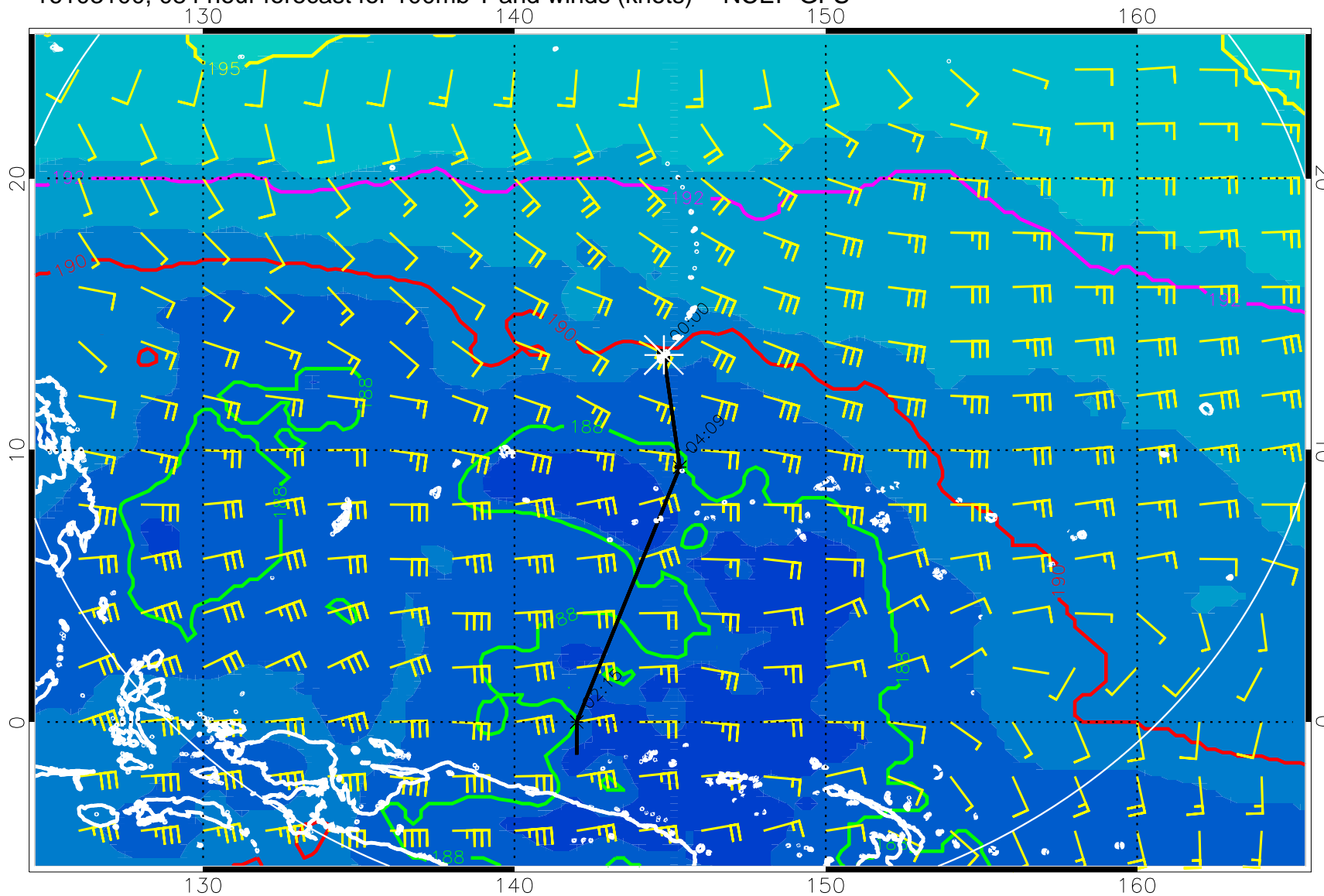
16103100, 084 hour forecast for 100mb T and winds (knots) -- NCEP GFS
