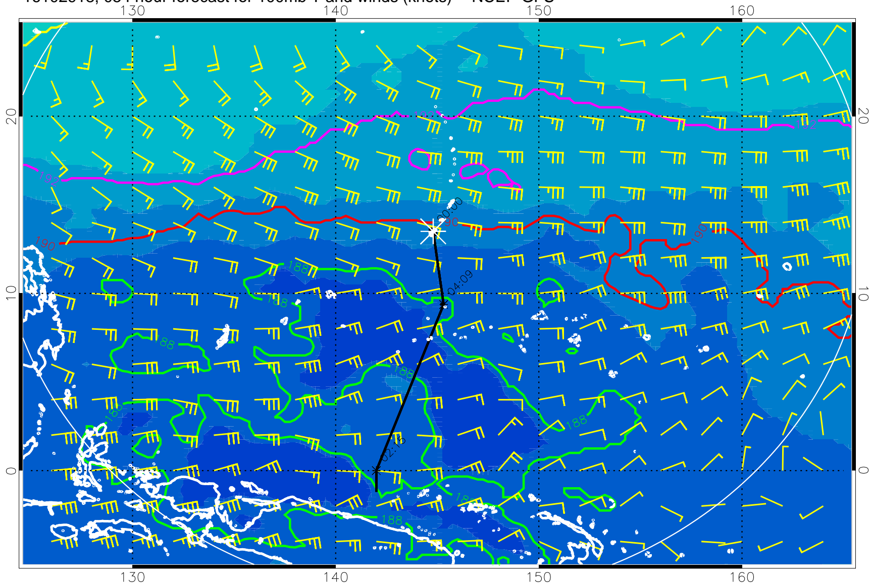
16102918, 054 hour forecast for 100mb T and winds (knots) -- NCEP GFS
