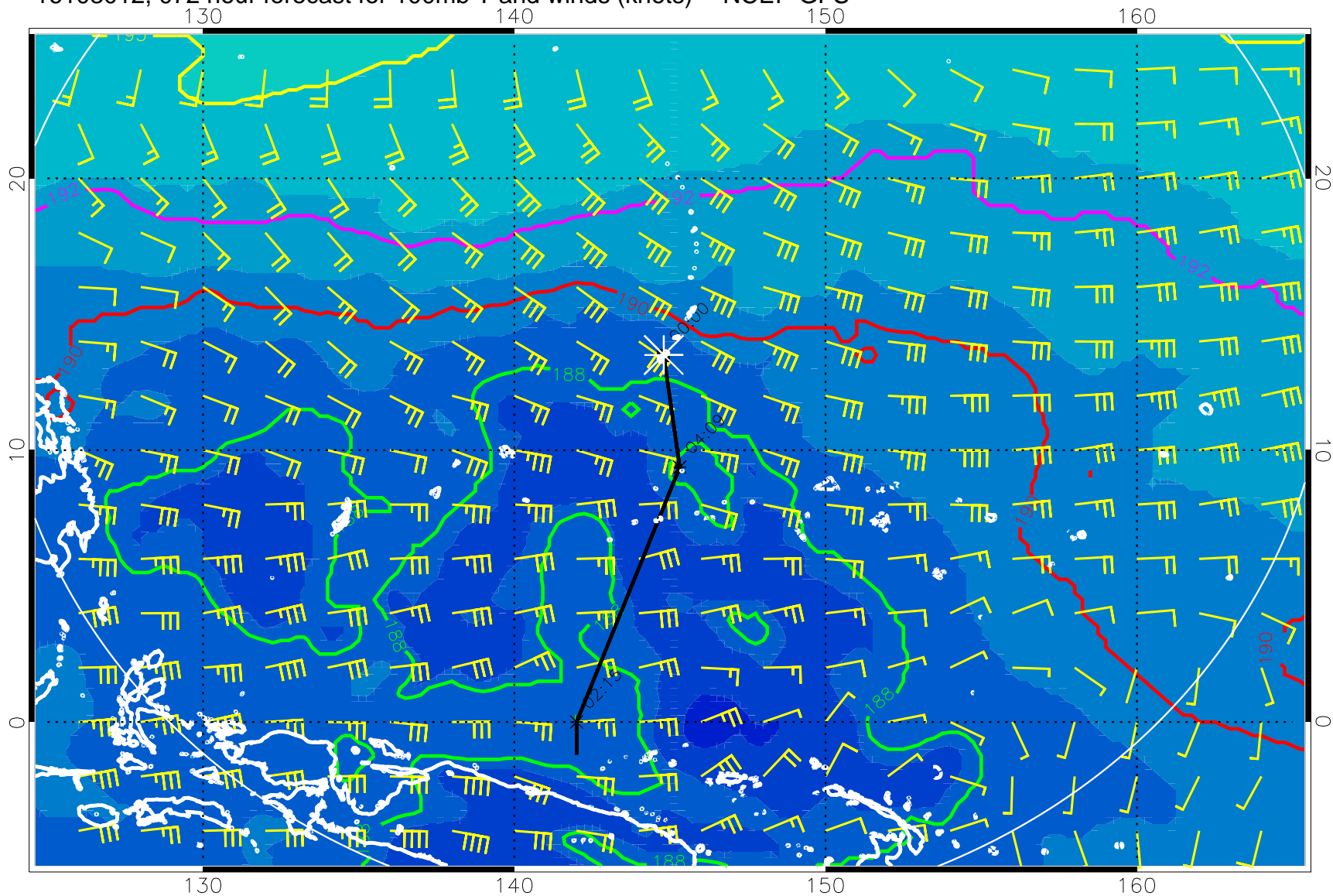
16103012, 072 hour forecast for 100mb T and winds (knots) -- NCEP GFS
