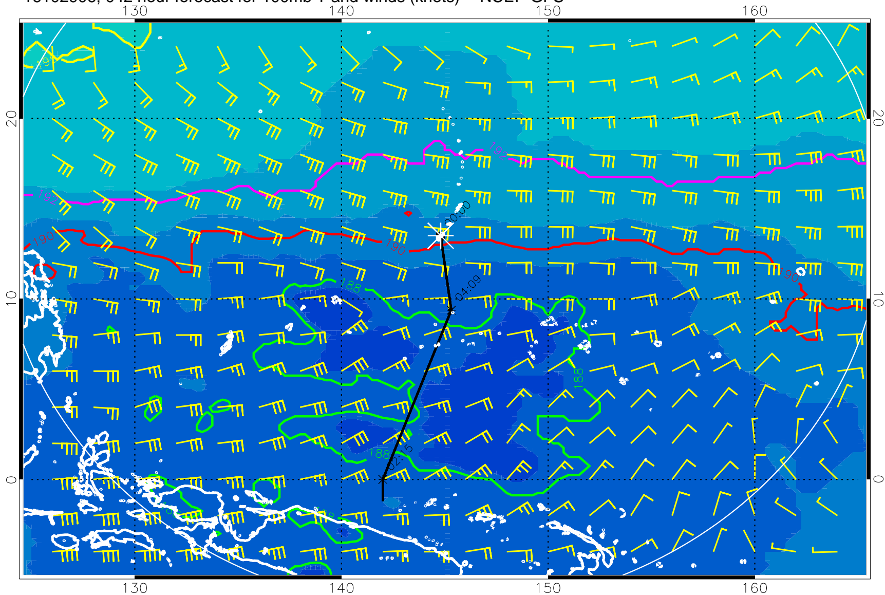
16102906, 042 hour forecast for 100mb T and winds (knots) -- NCEP GFS
