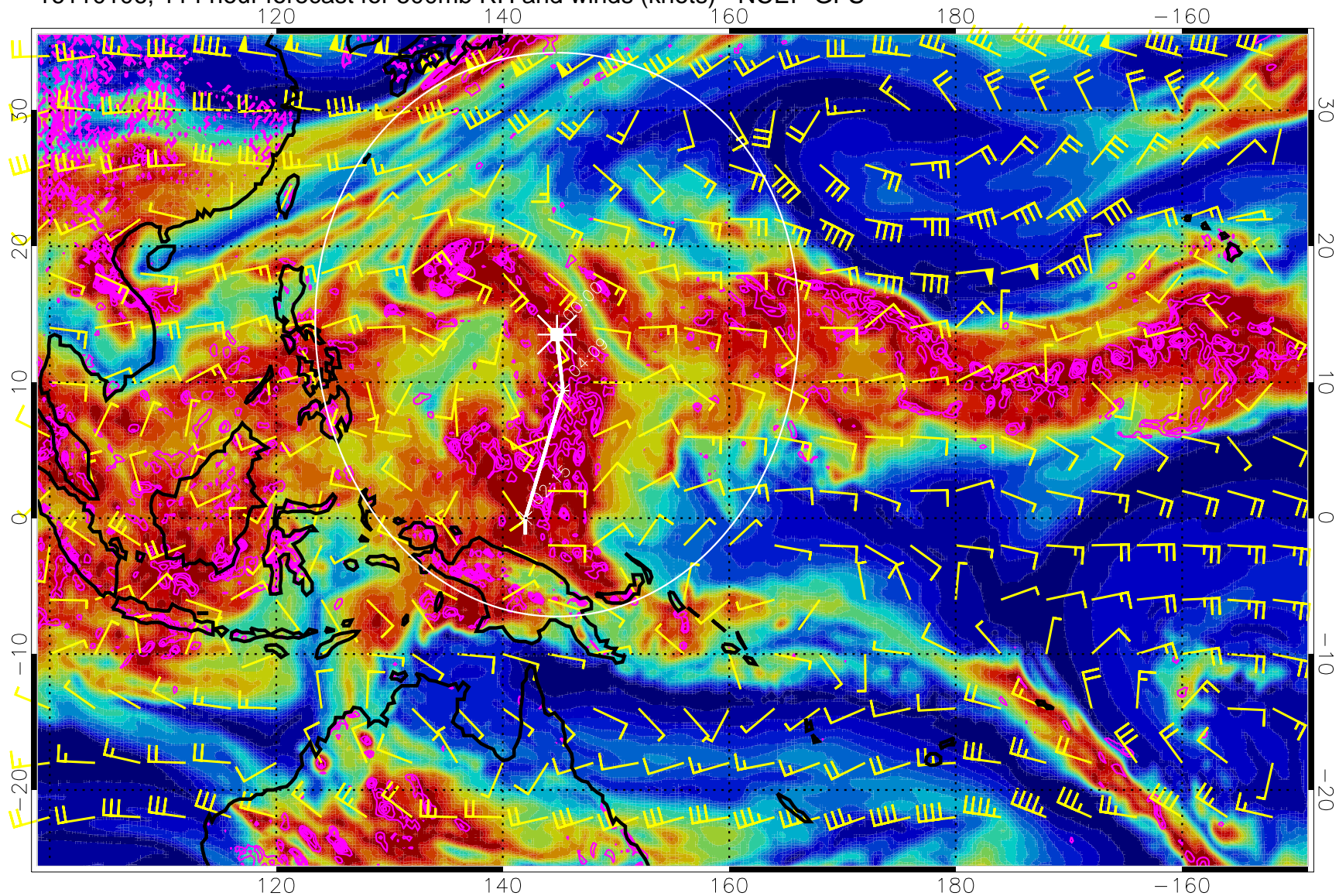
16110106, 114 hour forecast for 500mb RH and winds (knots) - NCEP GFS
