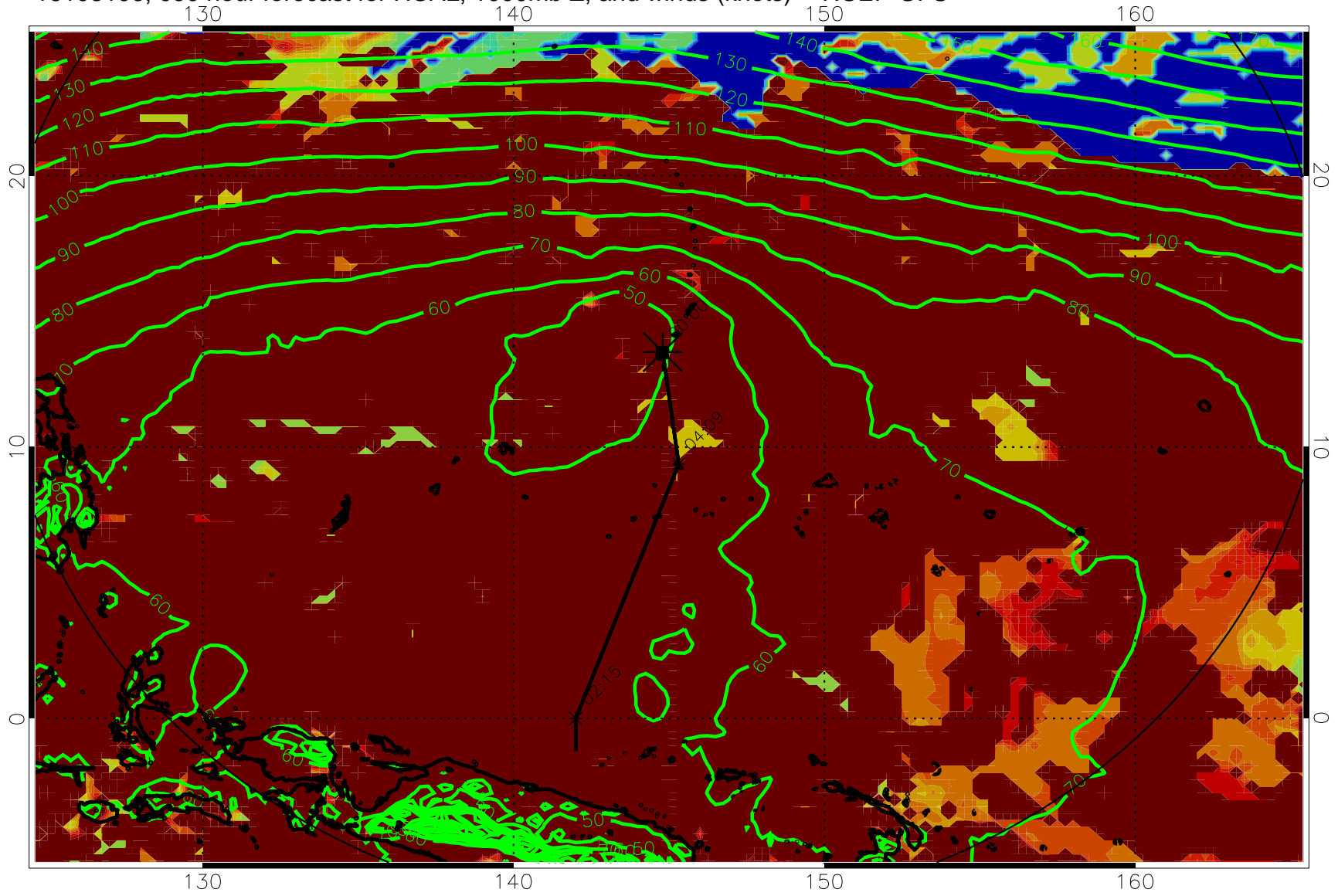
16103106, 090 hour forecast for HCAL, 1000mb Z, and winds (knots) -- NCEP GFS
