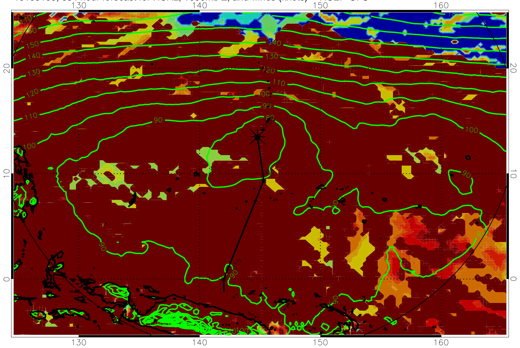
16103100, 084 hour forecast for HCAL, 1000mb Z, and winds (knots) -- NCEP GFS
