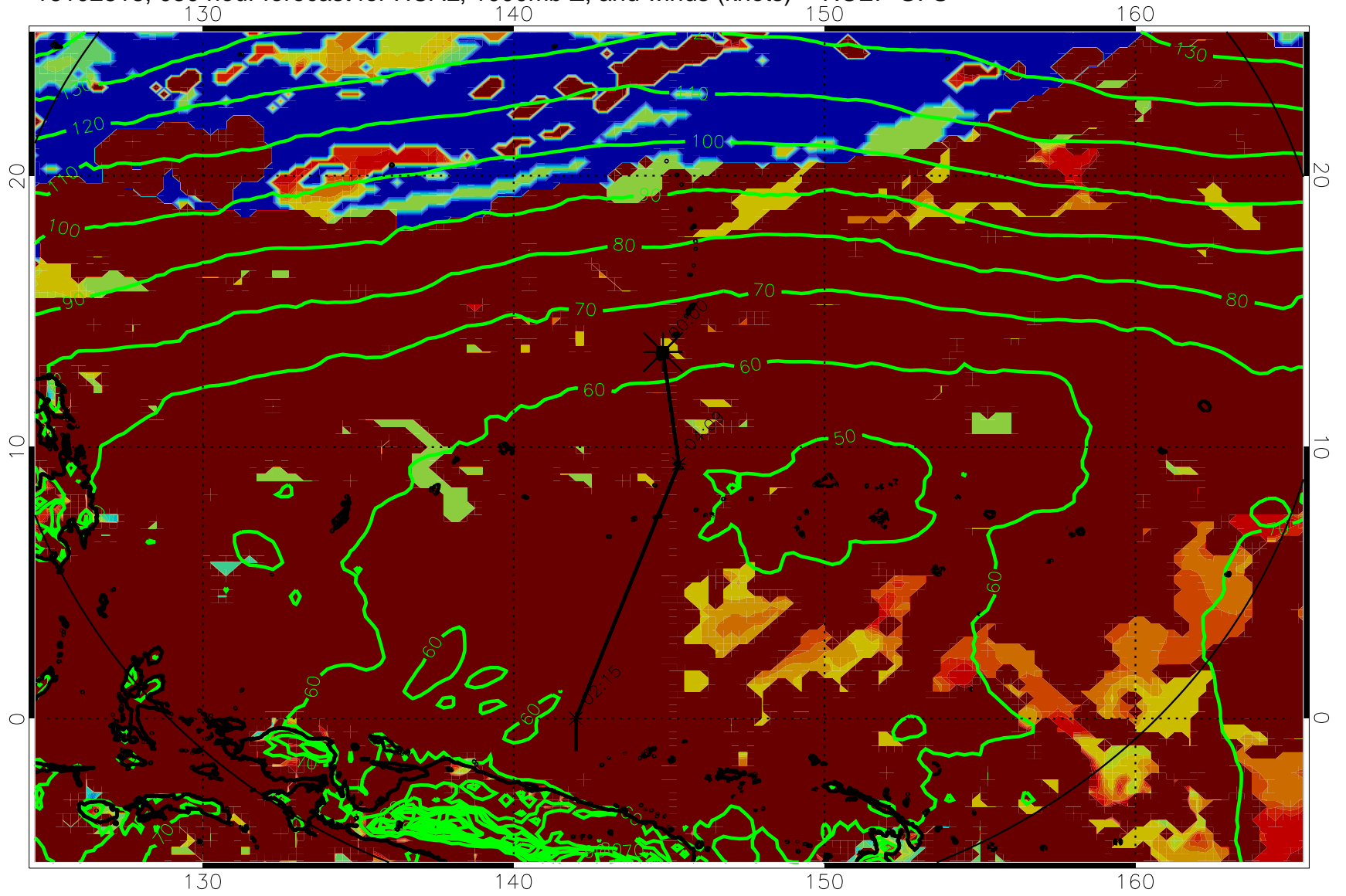
16102818, 030 hour forecast for HCAL, 1000mb Z, and winds (knots) -- NCEP GFS
