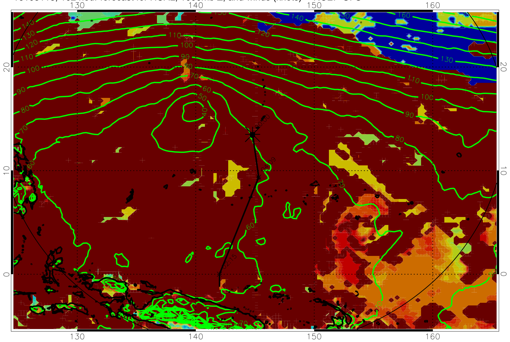
16103118, 102 hour forecast for HCAL, 1000mb Z, and winds (knots) -- NCEP GFS
