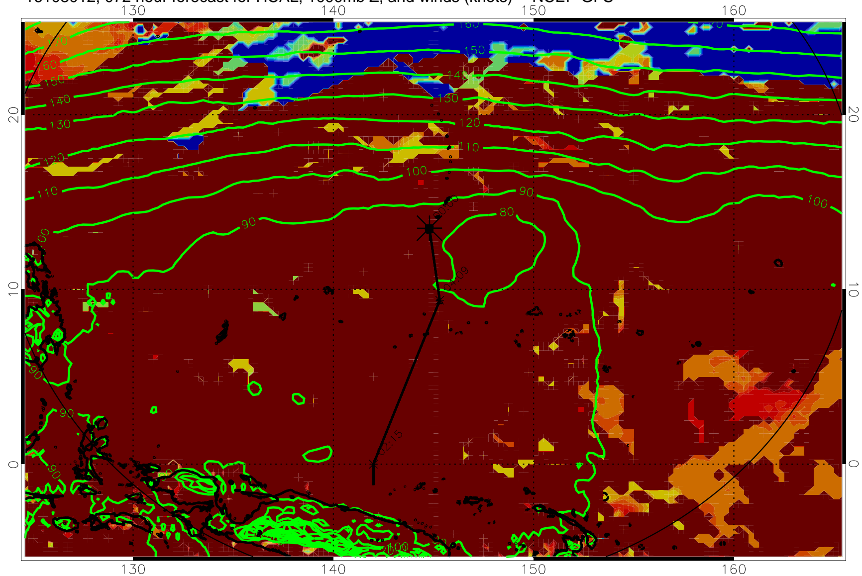
16103012, 072 hour forecast for HCAL, 1000mb Z, and winds (knots) -- NCEP GFS
