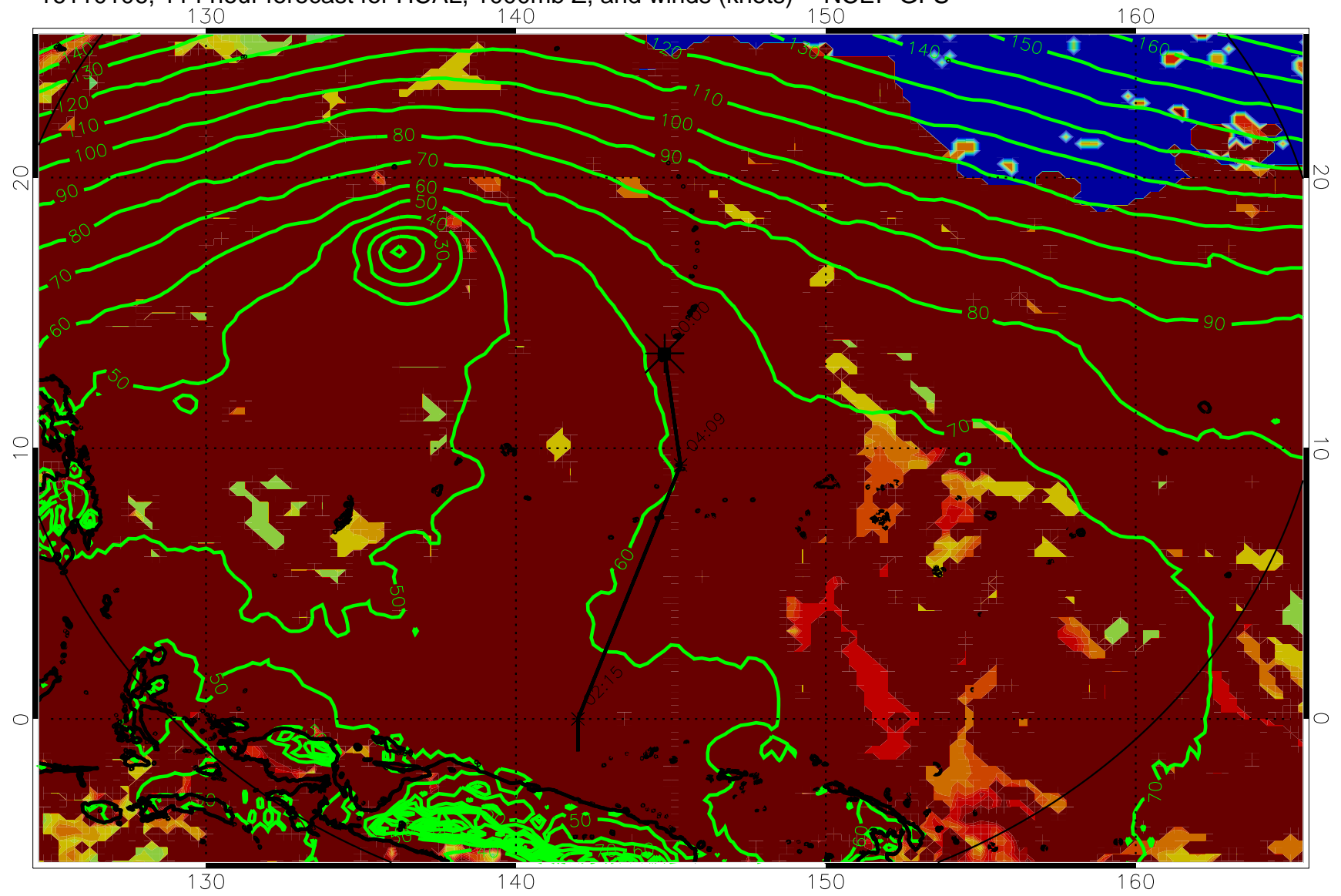
16110106, 114 hour forecast for HCAL, 1000mb Z, and winds (knots) -- NCEP GFS
