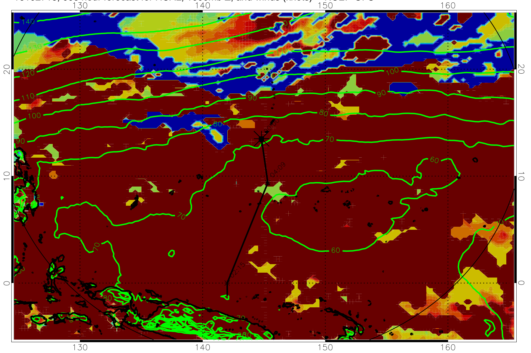
16102718, 006 hour forecast for HCAL, 1000mb Z, and winds (knots) -- NCEP GFS
