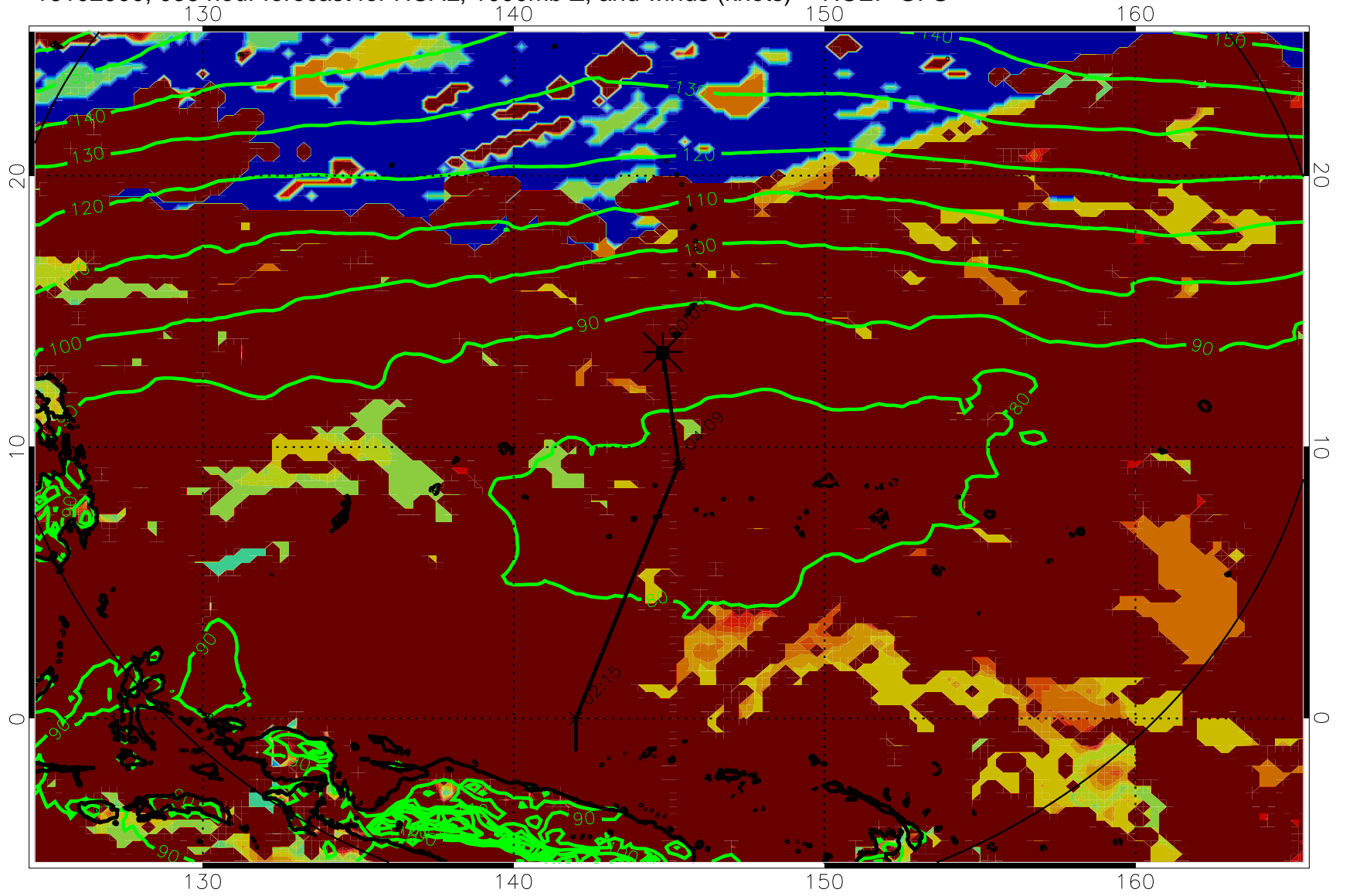
16102900, 036 hour forecast for HCAL, 1000mb Z, and winds (knots) -- NCEP GFS
