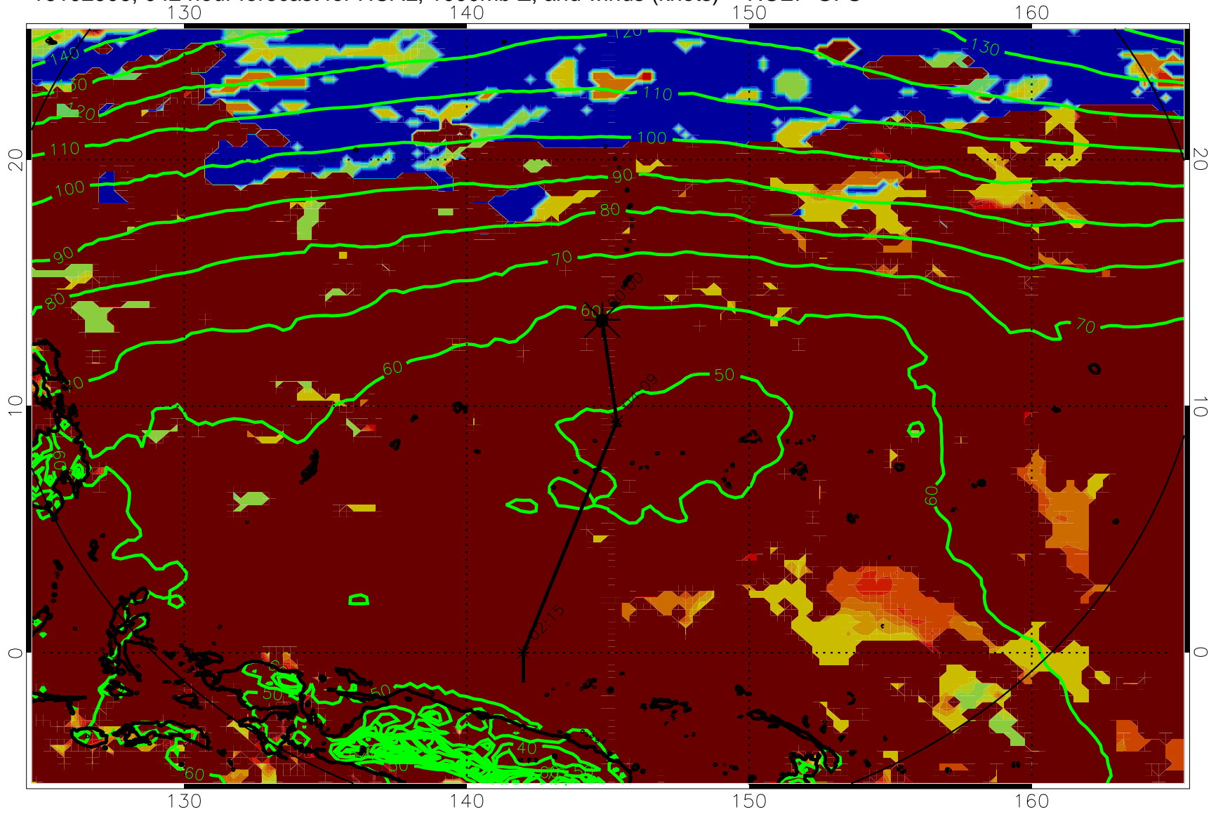
16102906, 042 hour forecast for HCAL, 1000mb Z, and winds (knots) -- NCEP GFS
