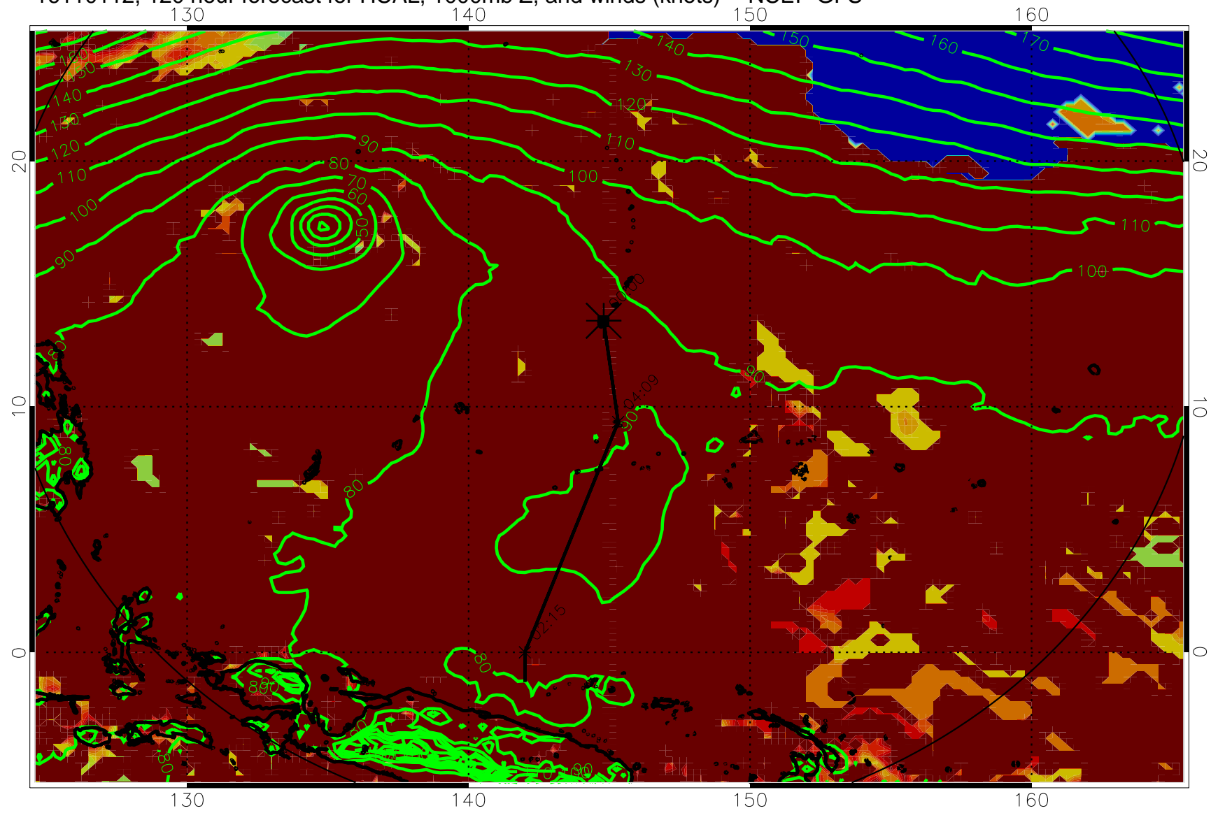
16110112, 120 hour forecast for HCAL, 1000mb Z, and winds (knots) -- NCEP GFS
