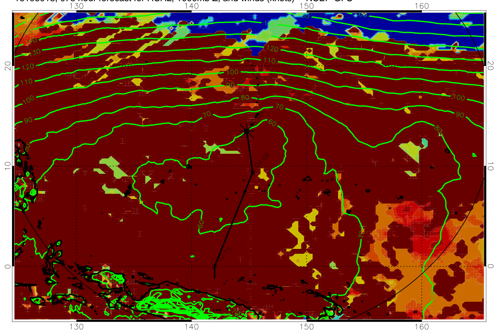
16103018, 078 hour forecast for HCAL, 1000mb Z, and winds (knots) -- NCEP GFS
