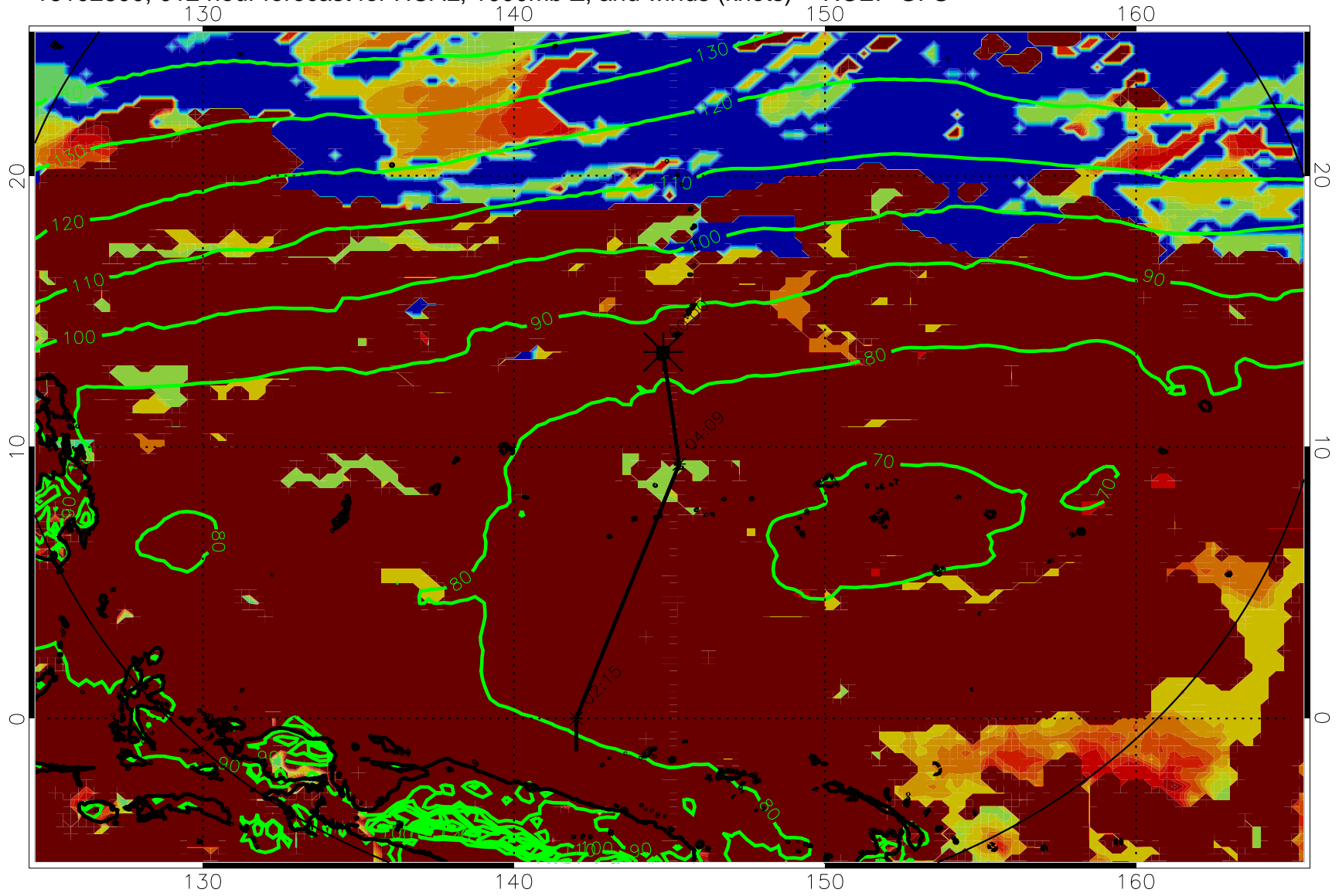
16102800, 012 hour forecast for HCAL, 1000mb Z, and winds (knots) -- NCEP GFS
