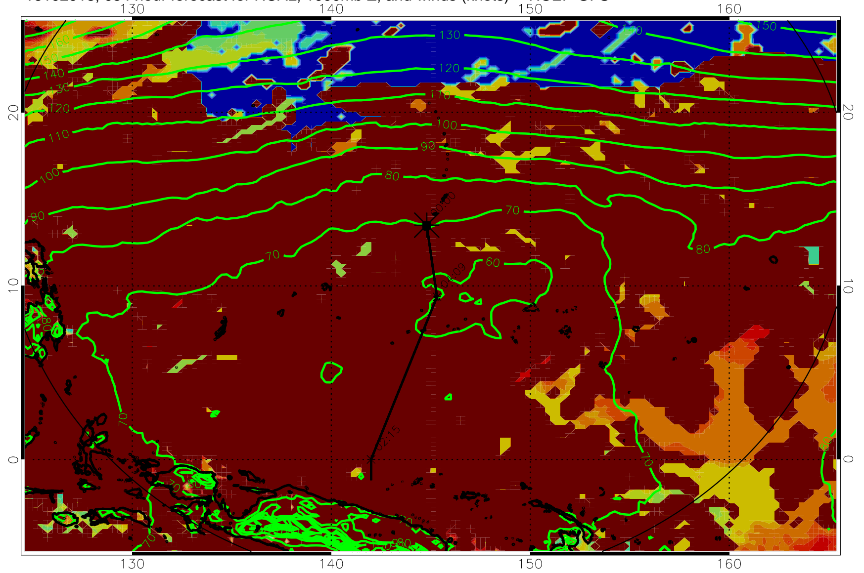
16102918, 054 hour forecast for HCAL, 1000mb Z, and winds (knots) -- NCEP GFS
