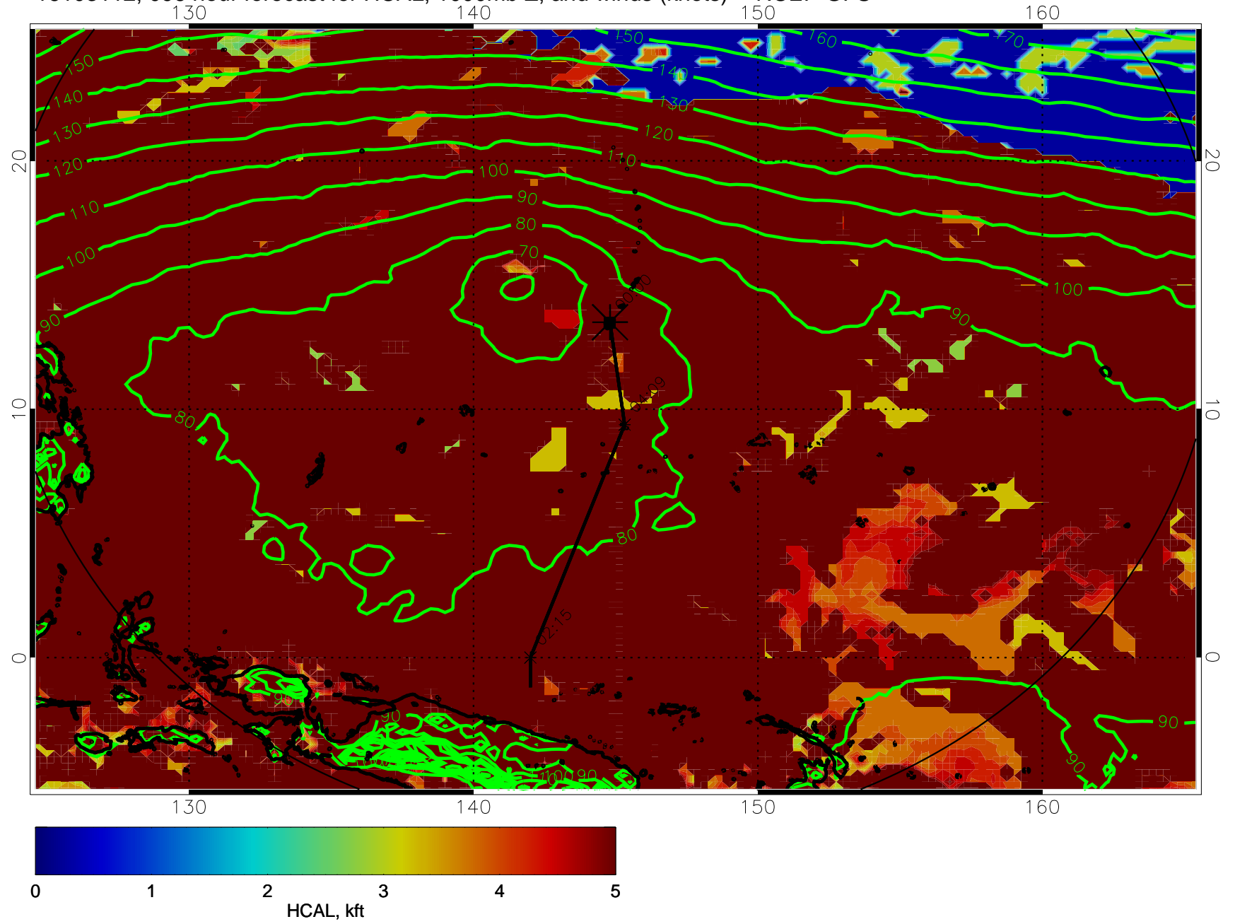
16103112, 096 hour forecast for HCAL, 1000mb Z, and winds (knots) -- NCEP GFS
