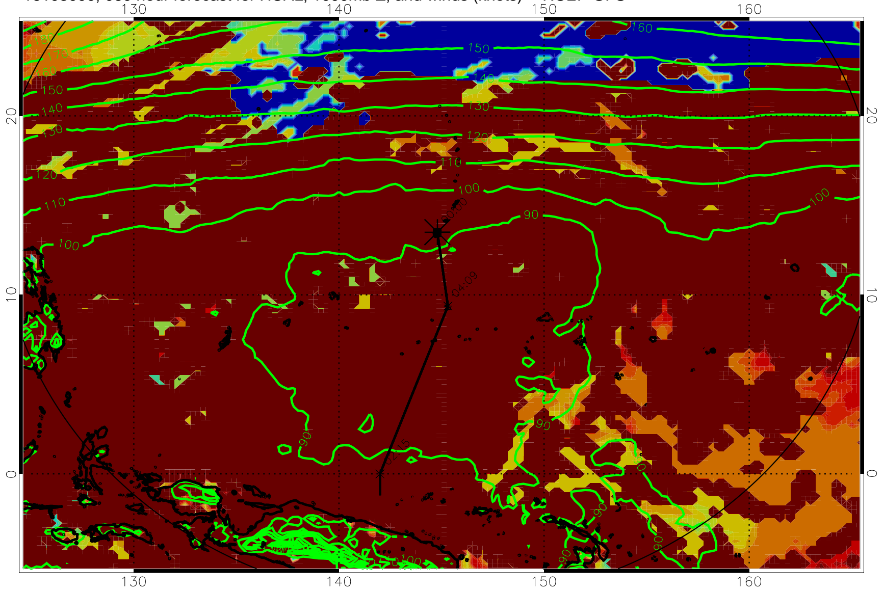
16103000, 060 hour forecast for HCAL, 1000mb Z, and winds (knots) -- NCEP GFS
