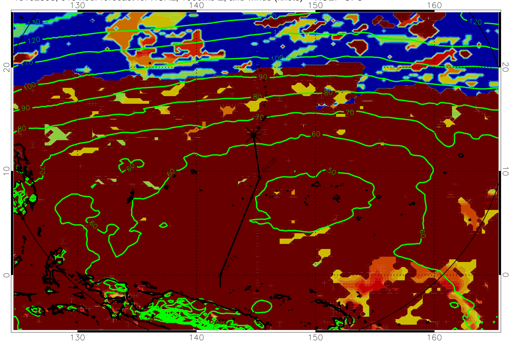
16102806, 018 hour forecast for HCAL, 1000mb Z, and winds (knots) -- NCEP GFS
