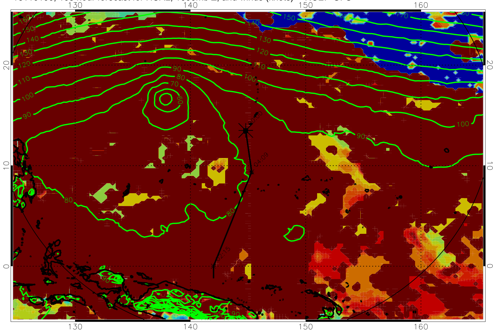
16110100, 108 hour forecast for HCAL, 1000mb Z, and winds (knots) -- NCEP GFS
