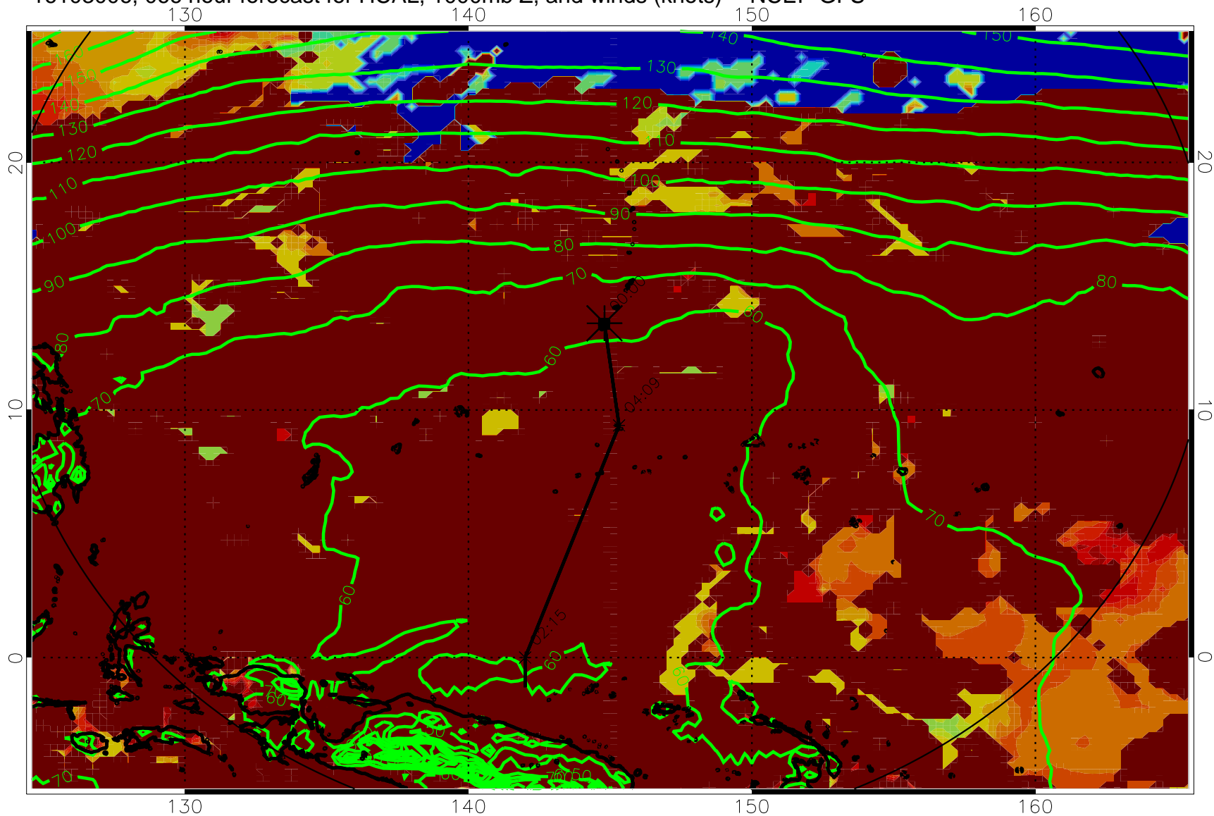
16103006, 066 hour forecast for HCAL, 1000mb Z, and winds (knots) -- NCEP GFS
