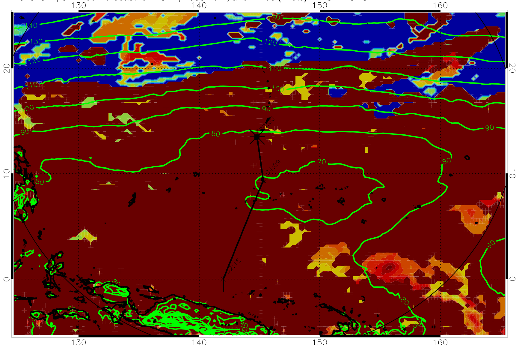
16102812, 024 hour forecast for HCAL, 1000mb Z, and winds (knots) -- NCEP GFS
