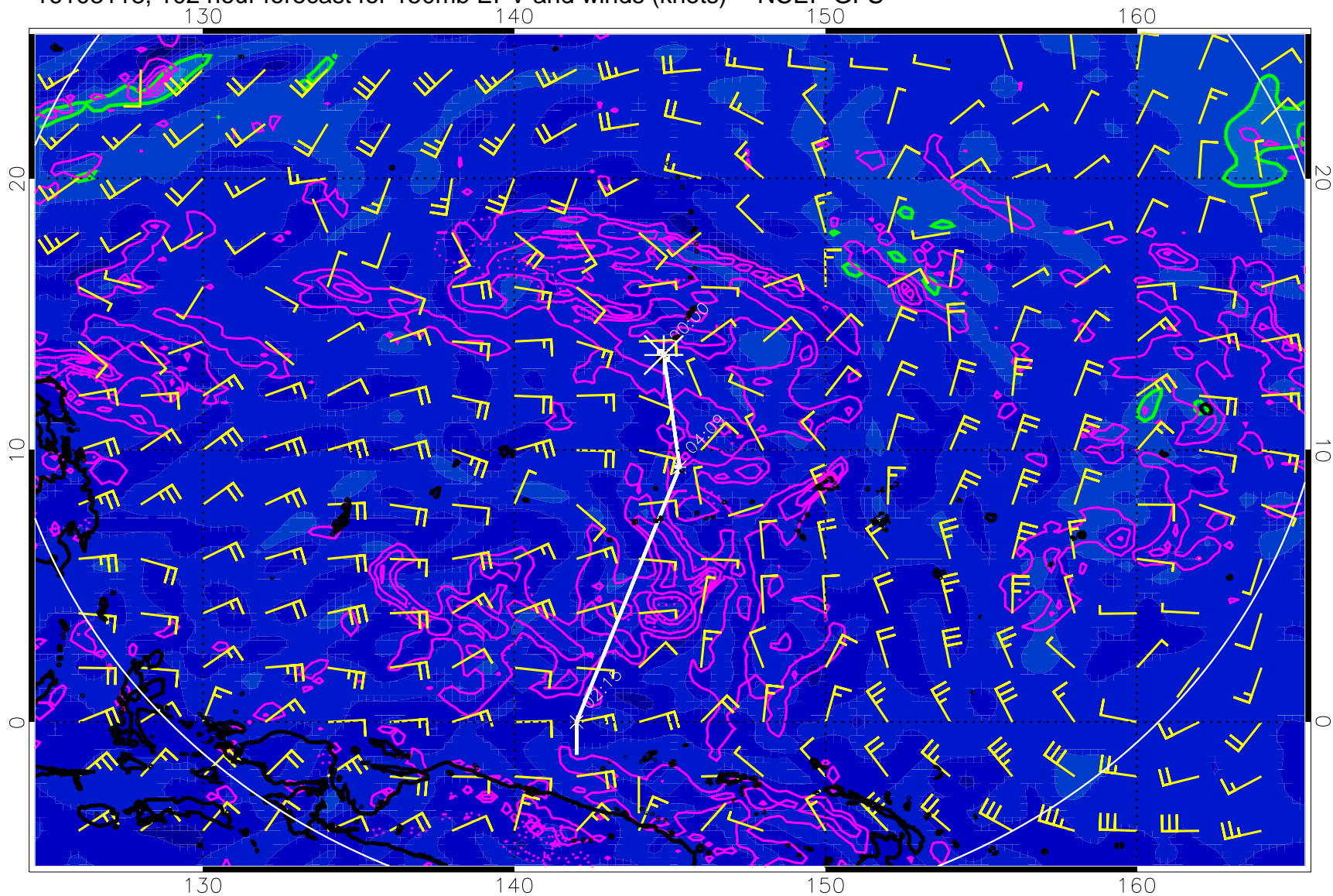
16103118, 102 hour forecast for 150mb EPV and winds (knots) -- NCEP GFS
