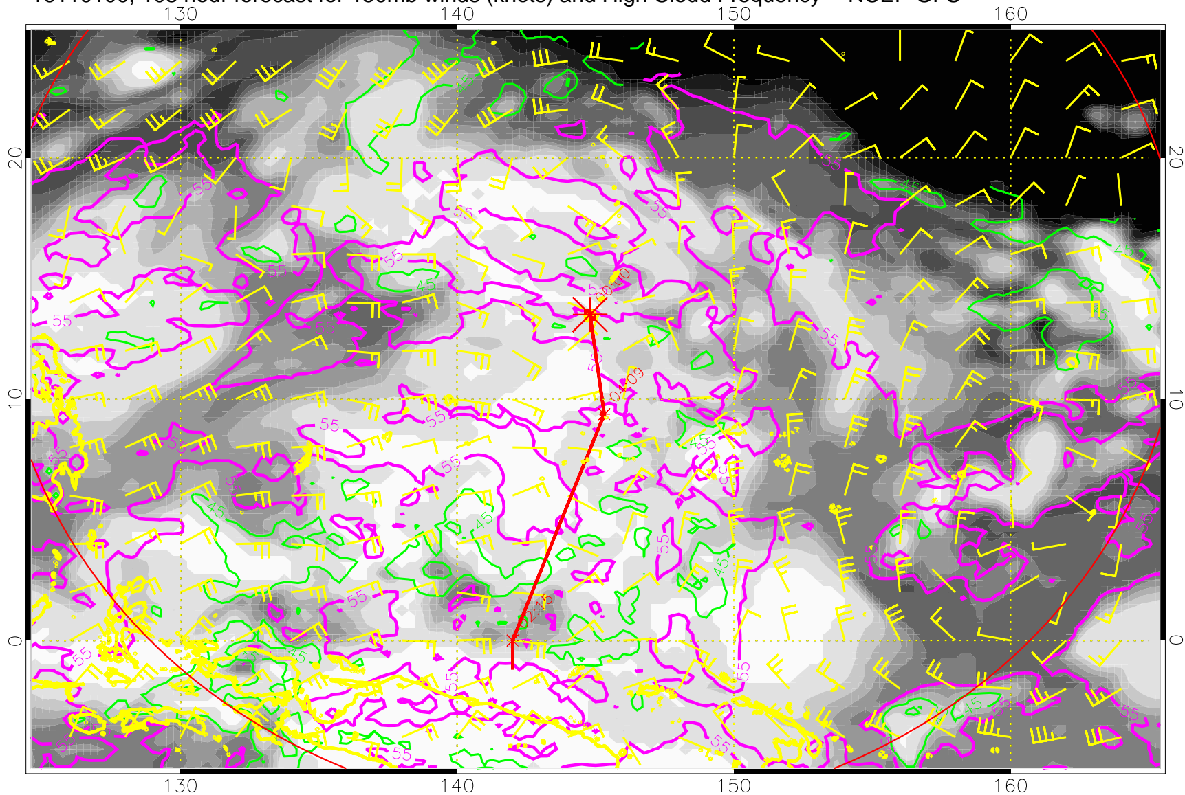
16110100, 108 hour forecast for 150mb winds (knots) and High Cloud Frequency -- NCEP GFS
