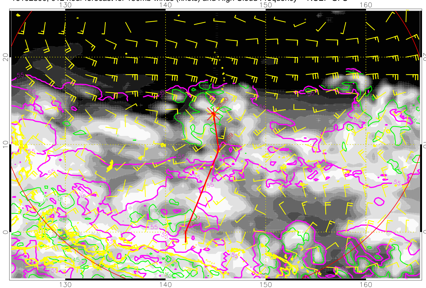
16102800, 012 hour forecast for 150mb winds (knots) and High Cloud Frequency -- NCEP GFS
