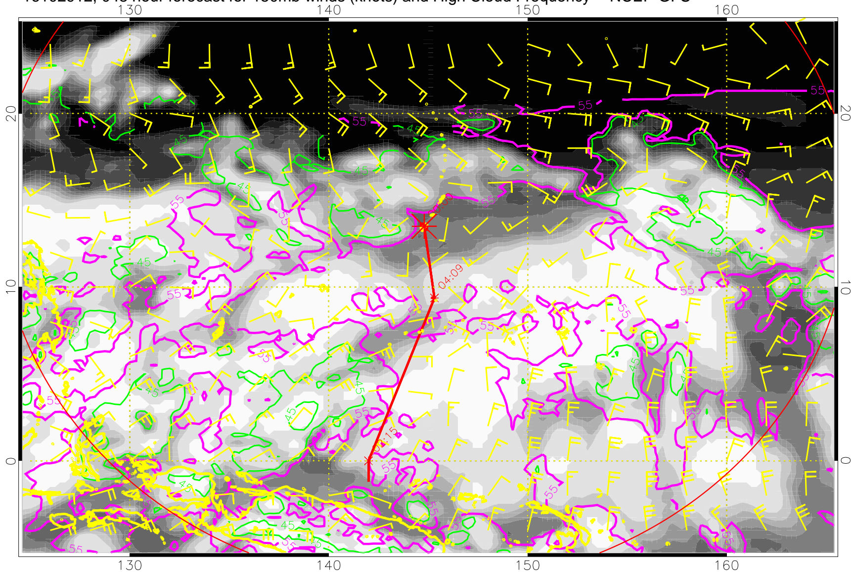
16102912, 048 hour forecast for 150mb winds (knots) and High Cloud Frequency -- NCEP GFS
