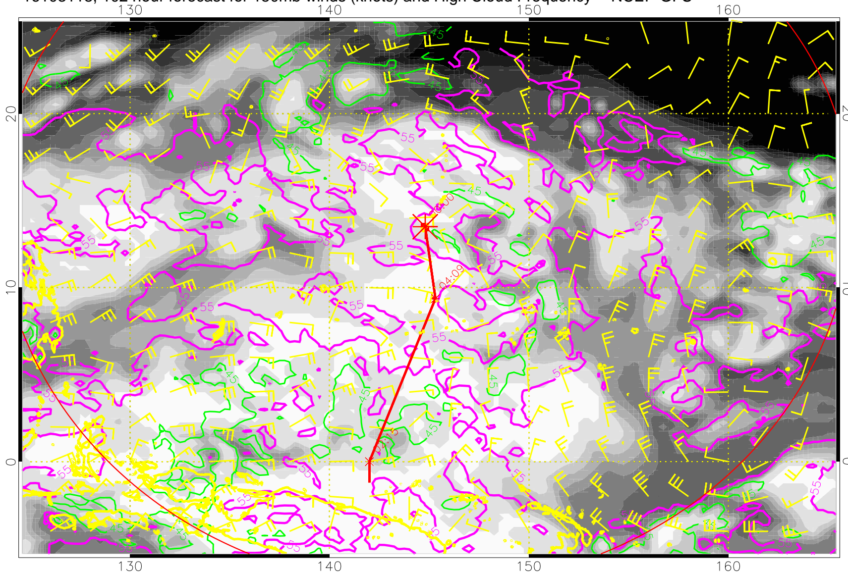
16103118, 102 hour forecast for 150mb winds (knots) and High Cloud Frequency -- NCEP GFS
