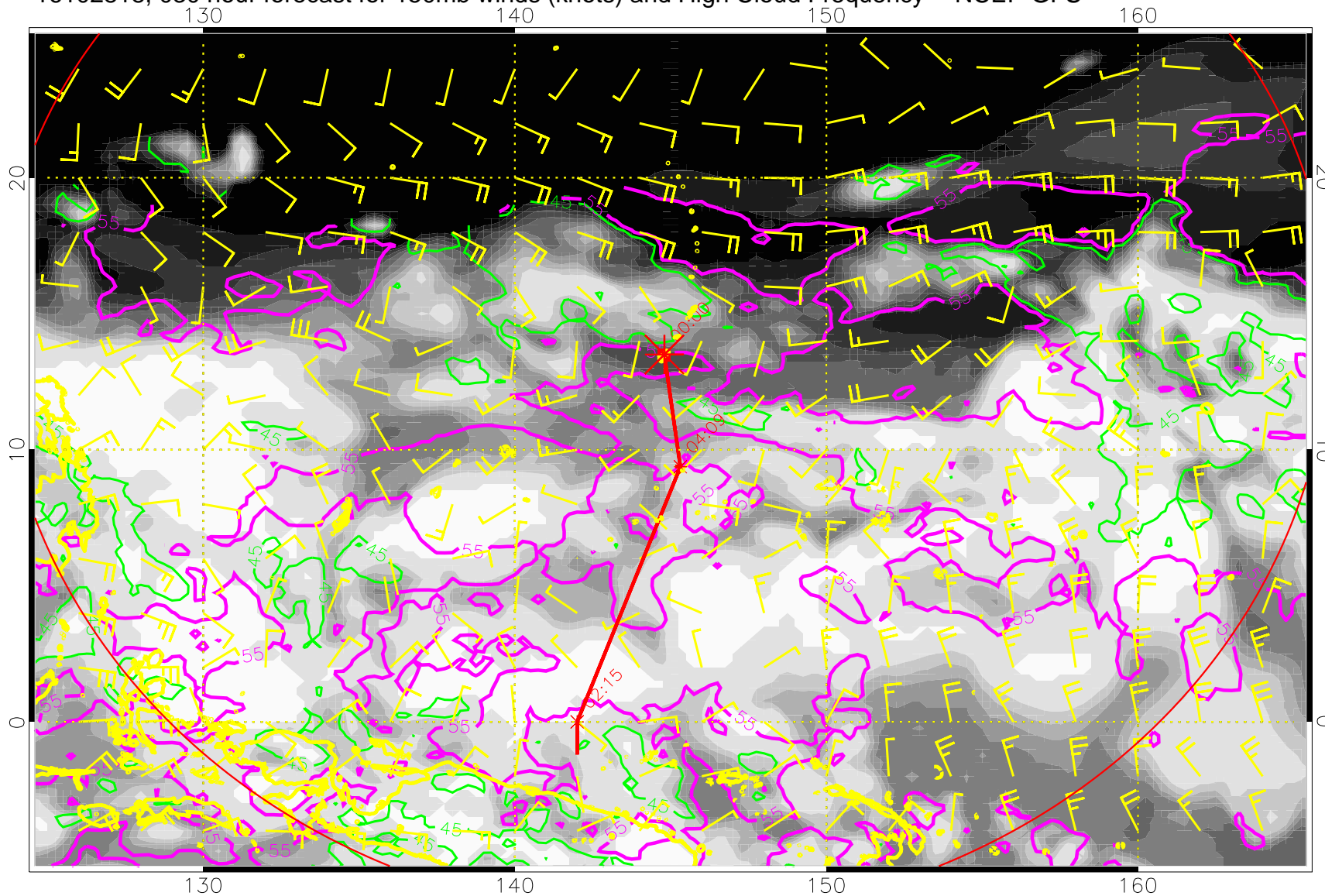
16102818, 030 hour forecast for 150mb winds (knots) and High Cloud Frequency -- NCEP GFS
