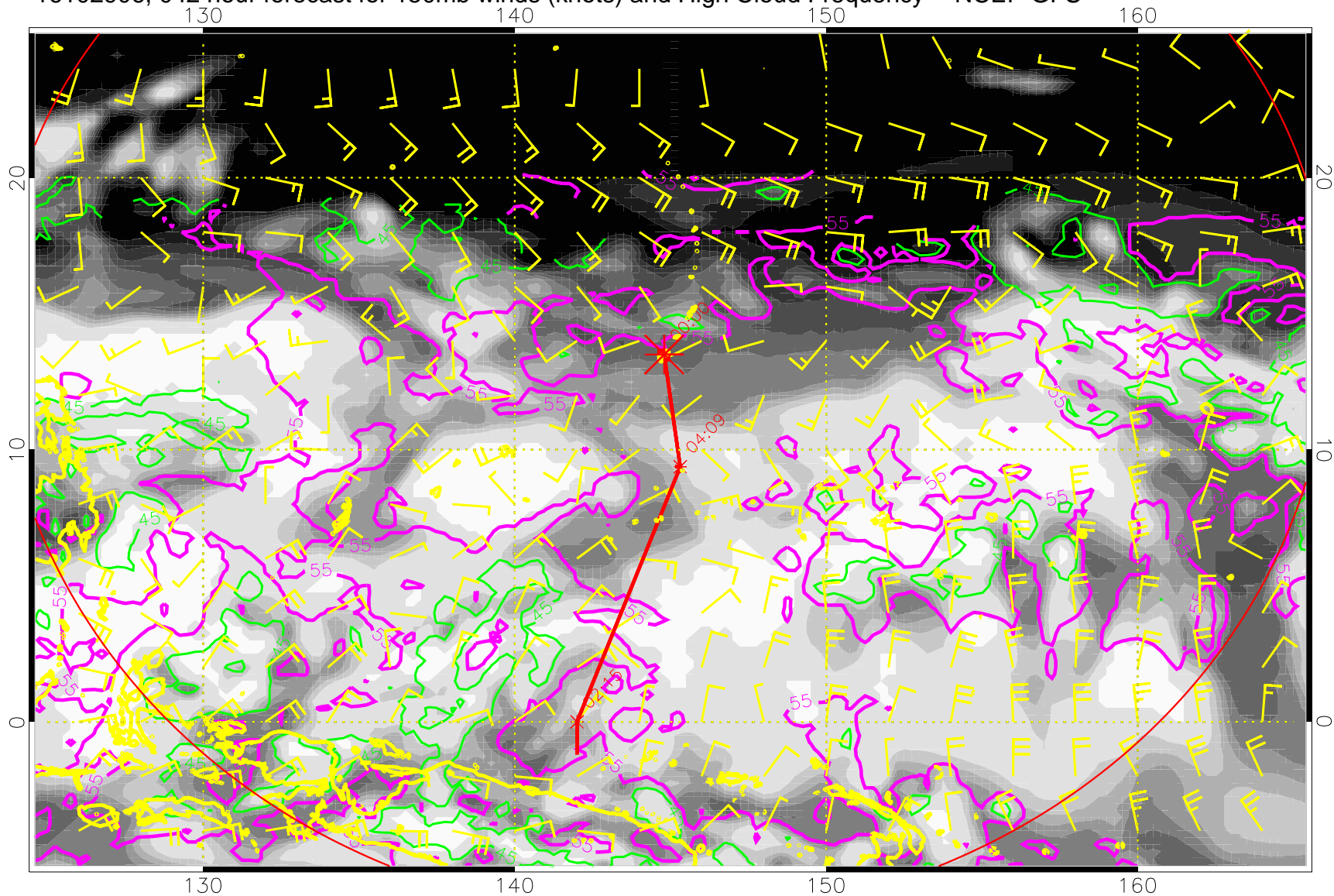
16102906, 042 hour forecast for 150mb winds (knots) and High Cloud Frequency -- NCEP GFS
