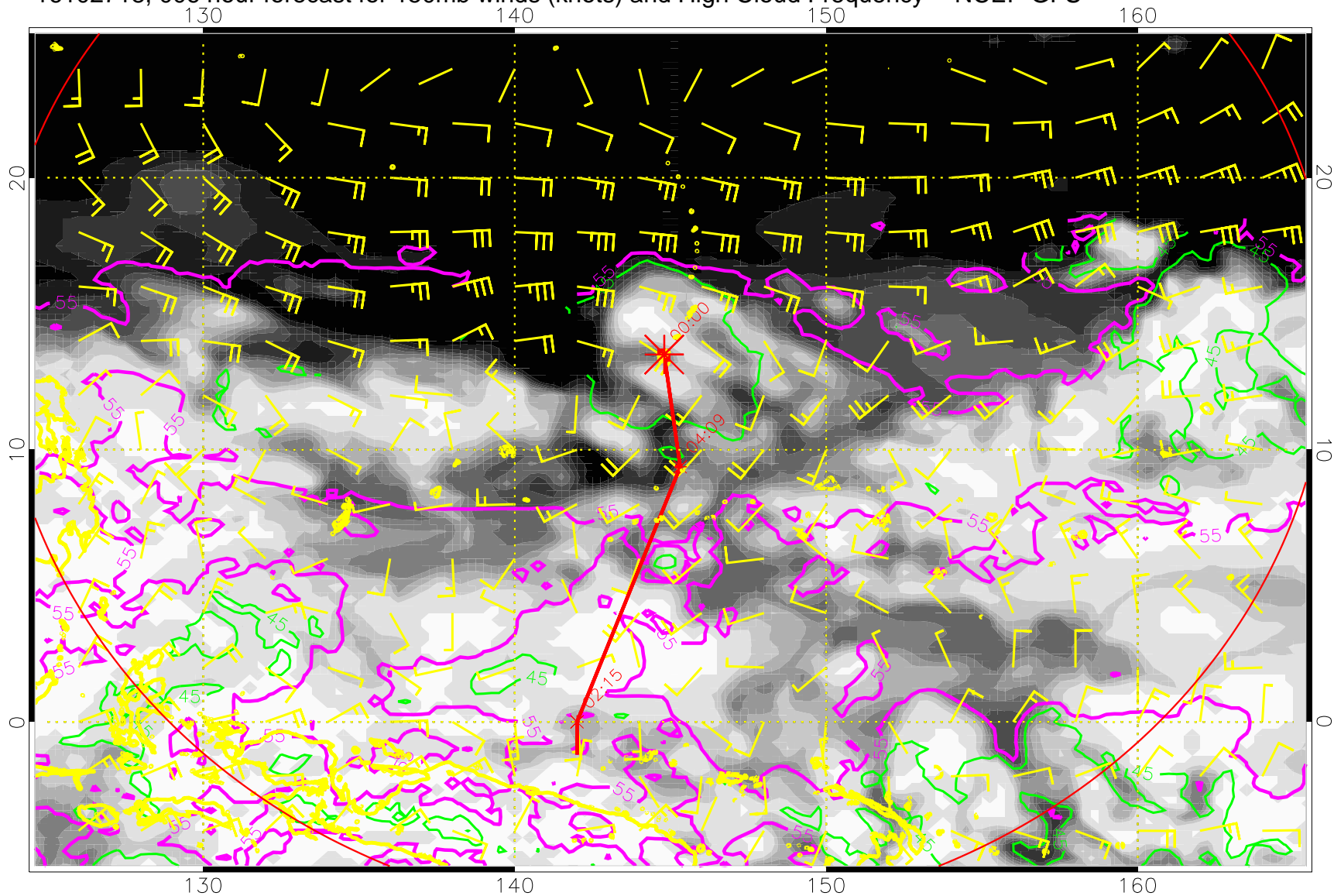
16102718, 006 hour forecast for 150mb winds (knots) and High Cloud Frequency -- NCEP GFS
