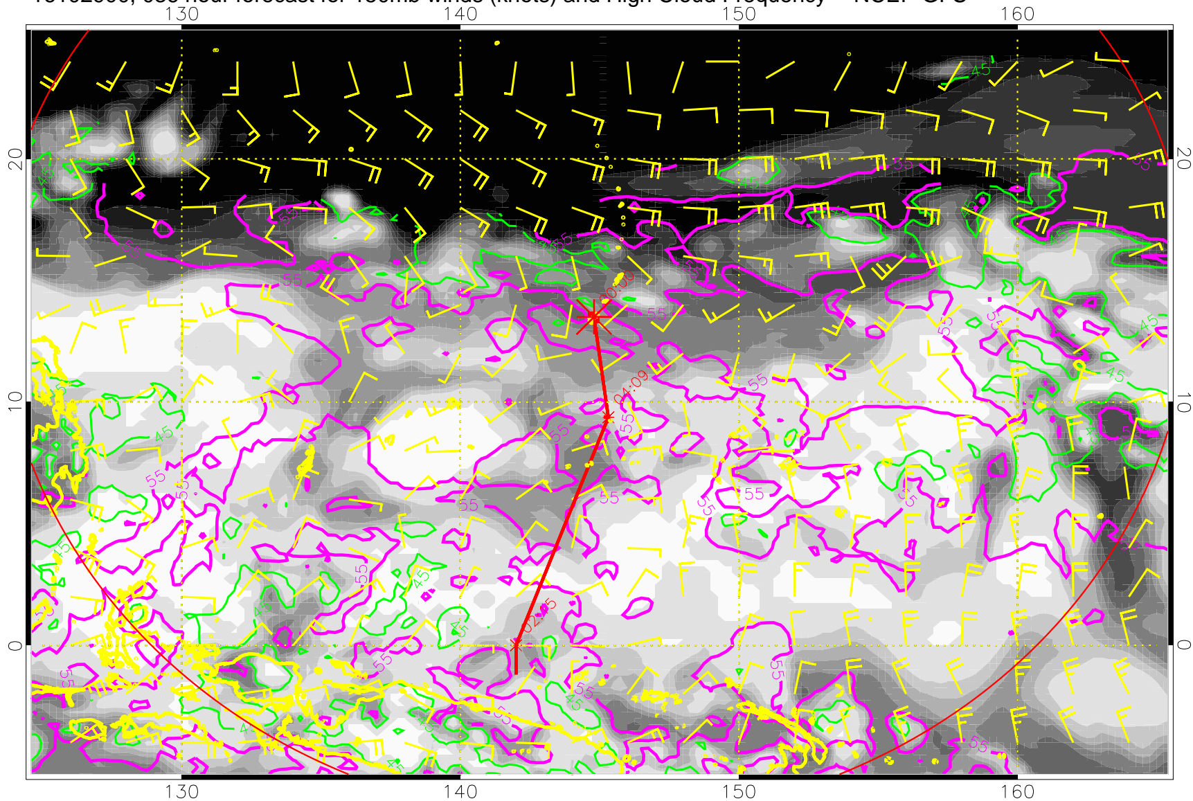
16102900, 036 hour forecast for 150mb winds (knots) and High Cloud Frequency -- NCEP GFS
