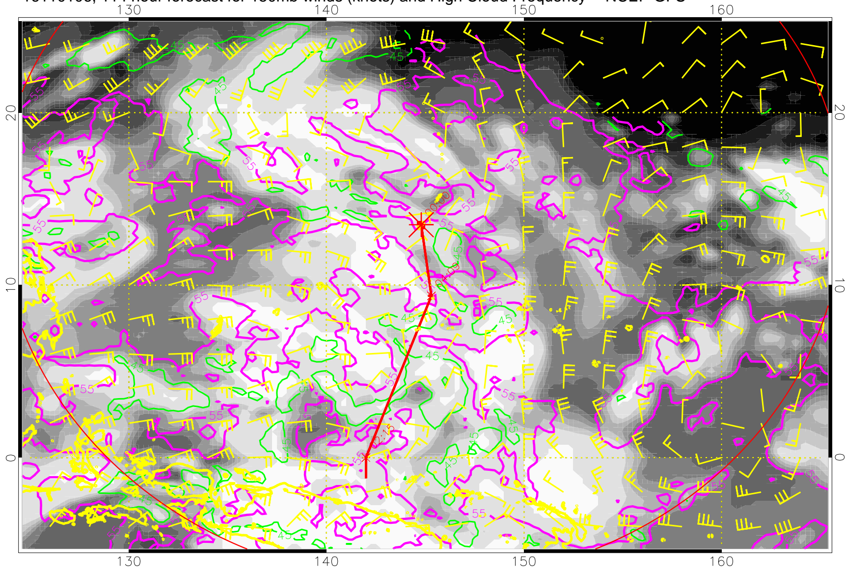
16110106, 114 hour forecast for 150mb winds (knots) and High Cloud Frequency -- NCEP GFS
