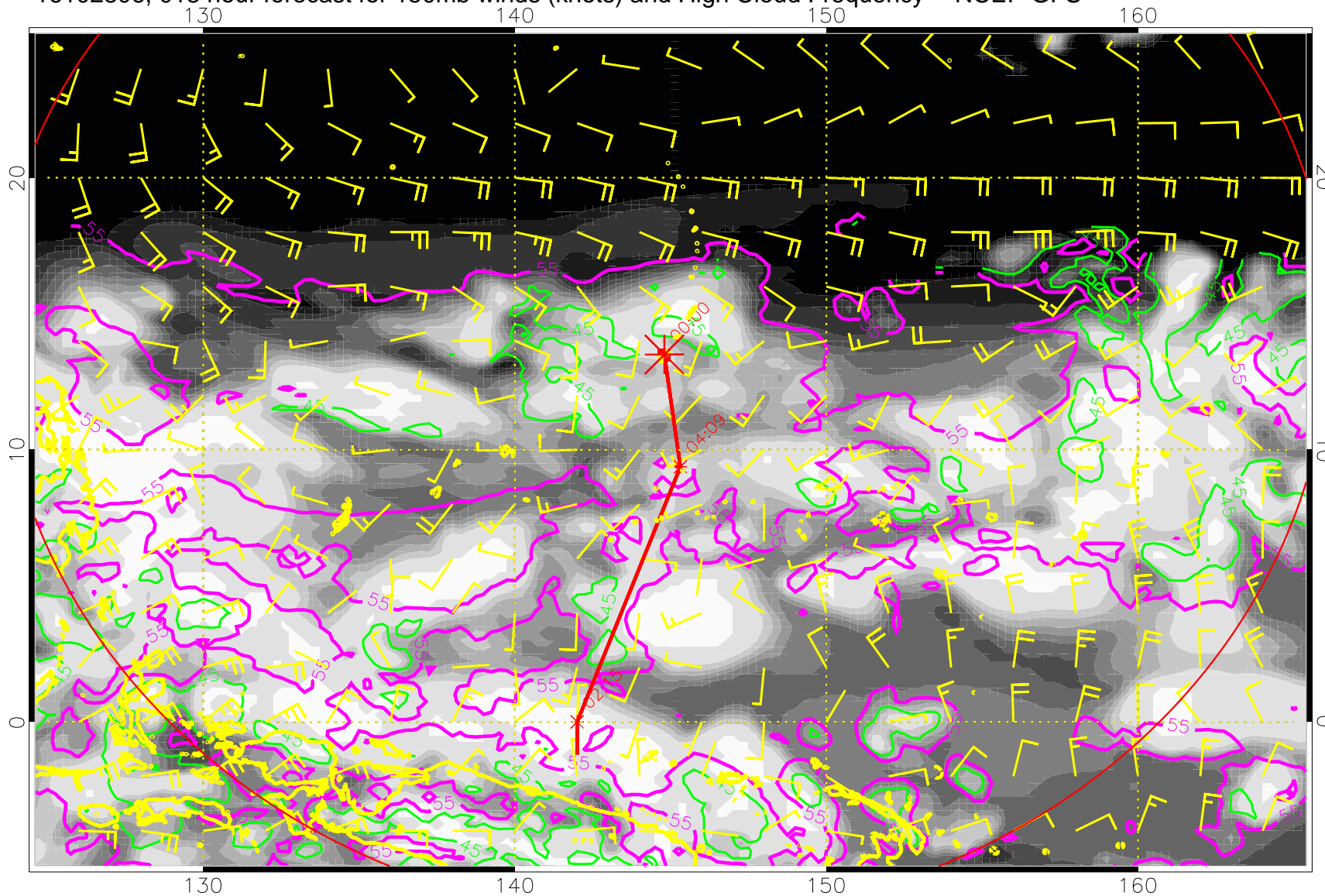
16102806, 018 hour forecast for 150mb winds (knots) and High Cloud Frequency -- NCEP GFS
