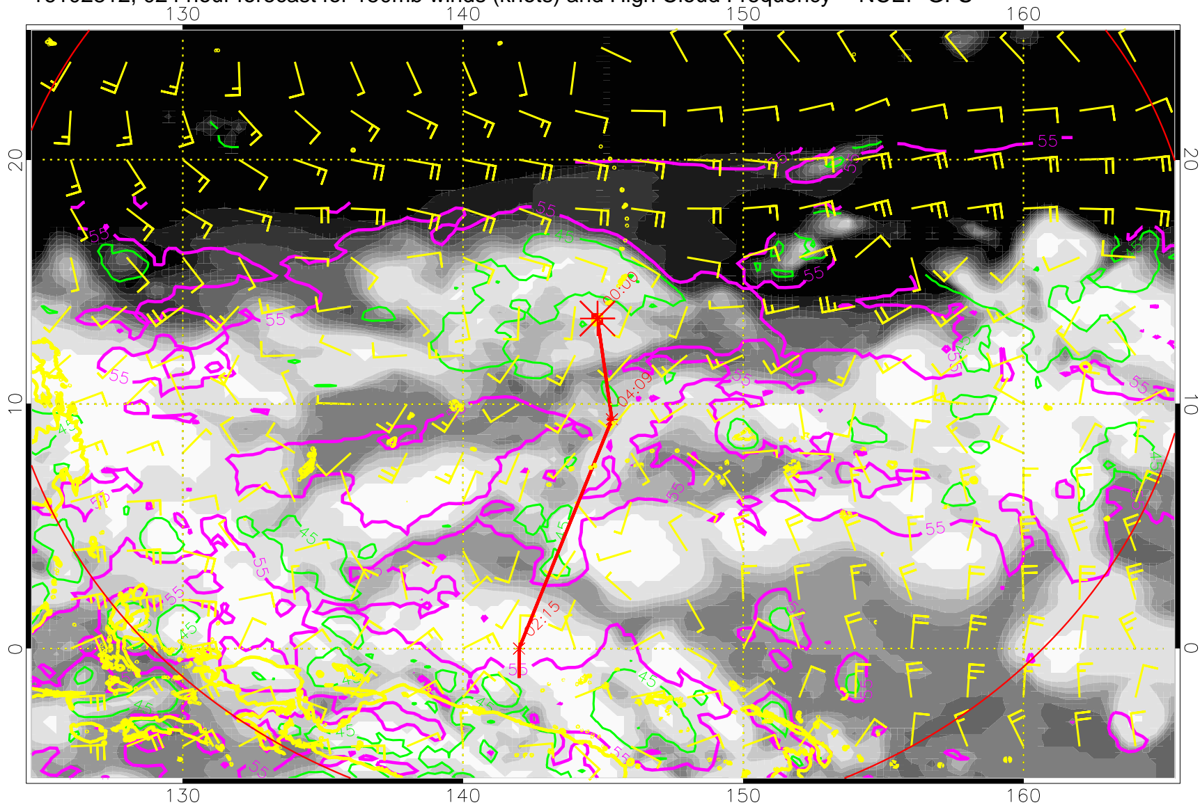
16102812, 024 hour forecast for 150mb winds (knots) and High Cloud Frequency -- NCEP GFS
