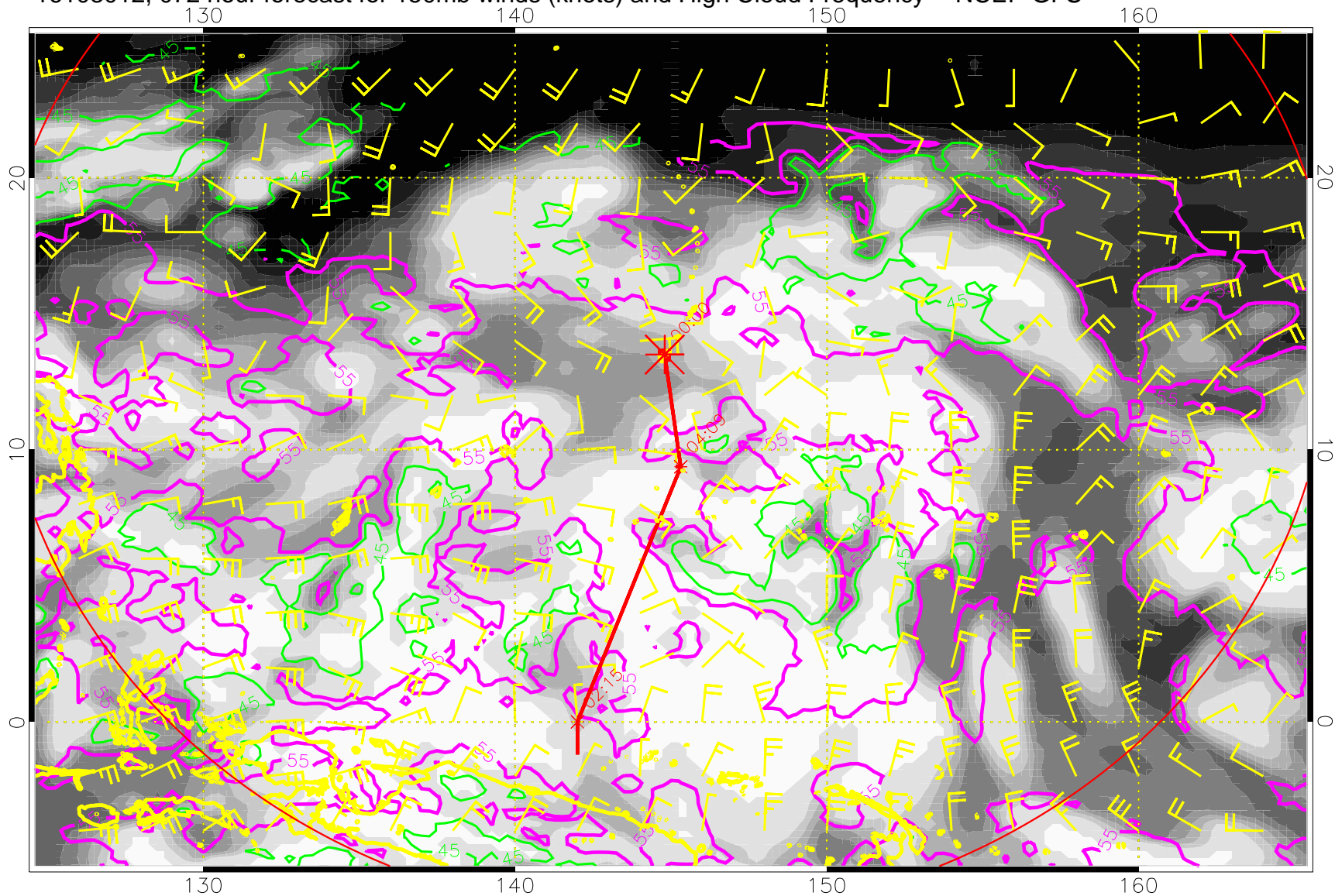
16103012, 072 hour forecast for 150mb winds (knots) and High Cloud Frequency -- NCEP GFS
