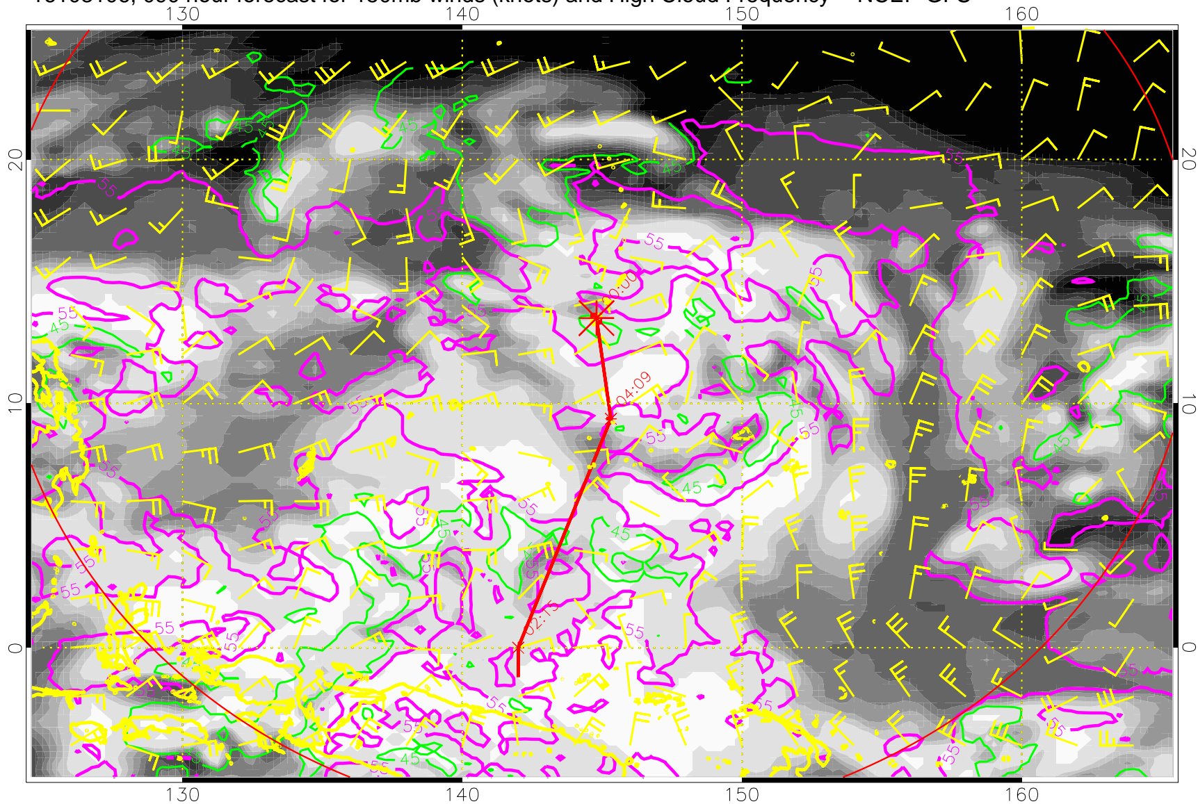
16103106, 090 hour forecast for 150mb winds (knots) and High Cloud Frequency -- NCEP GFS
