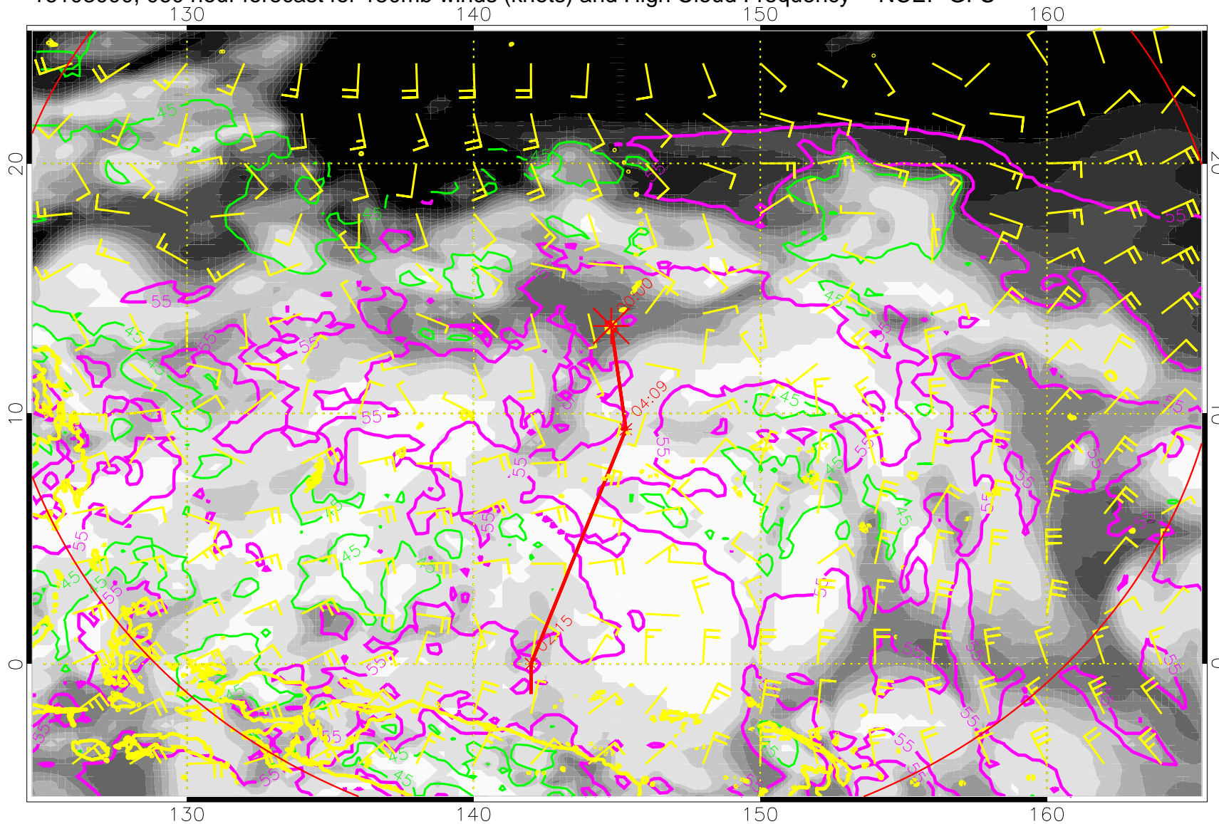
16103000, 060 hour forecast for 150mb winds (knots) and High Cloud Frequency -- NCEP GFS
