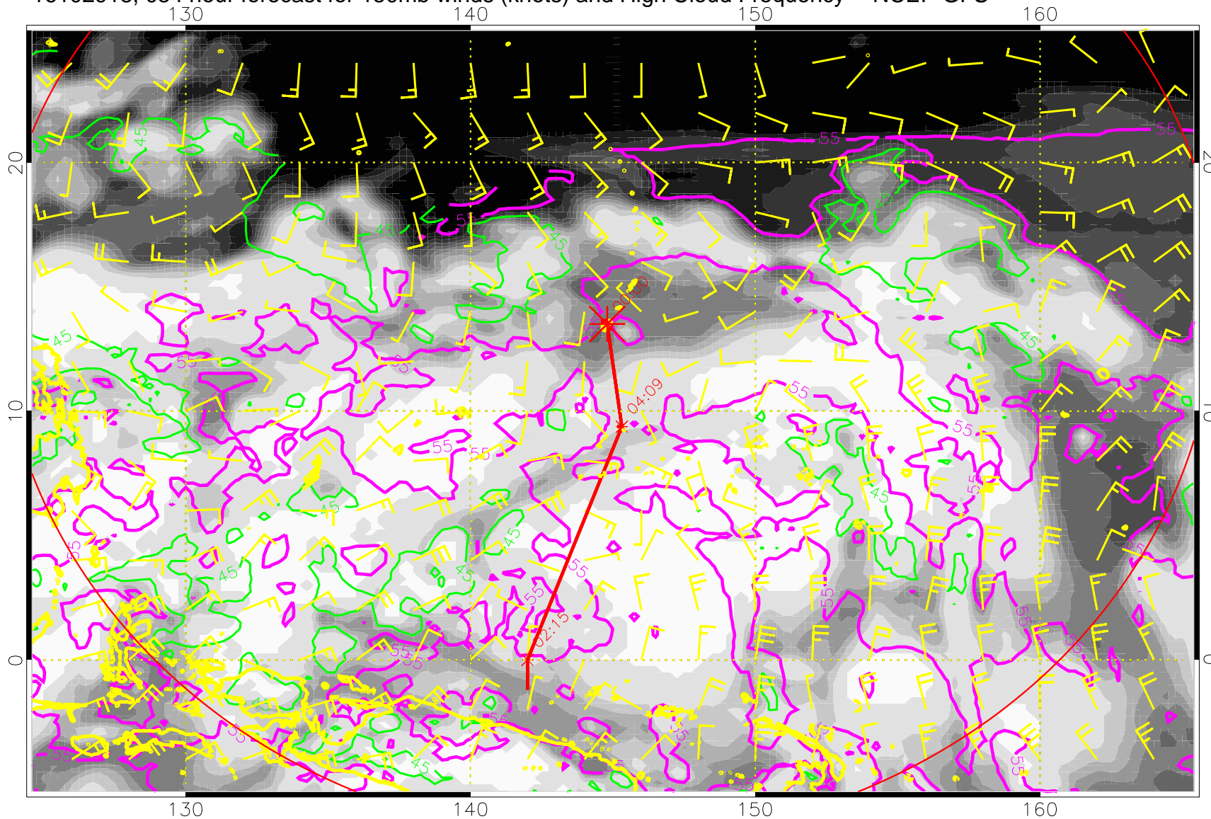
16102918, 054 hour forecast for 150mb winds (knots) and High Cloud Frequency -- NCEP GFS
