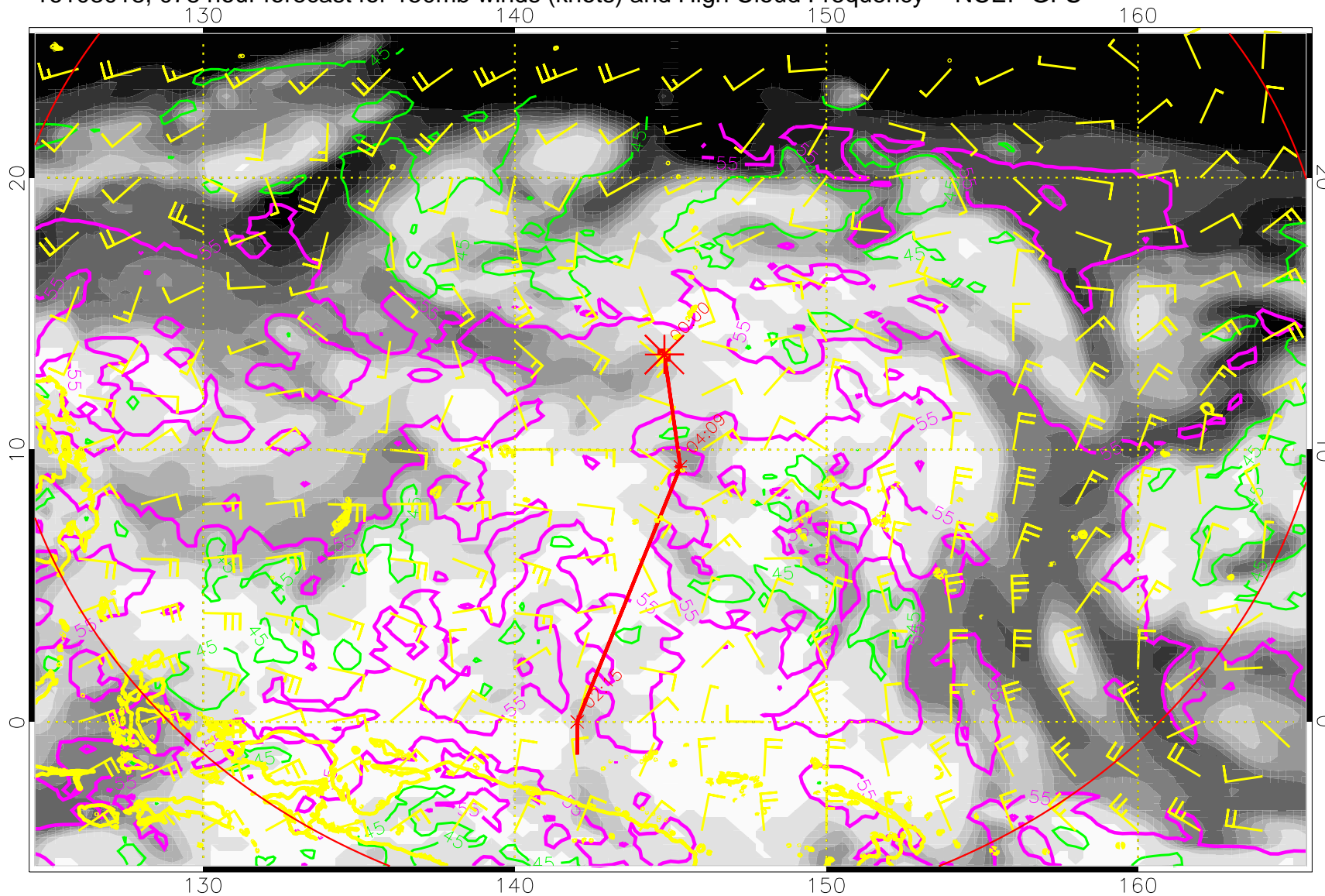
16103018, 078 hour forecast for 150mb winds (knots) and High Cloud Frequency -- NCEP GFS
