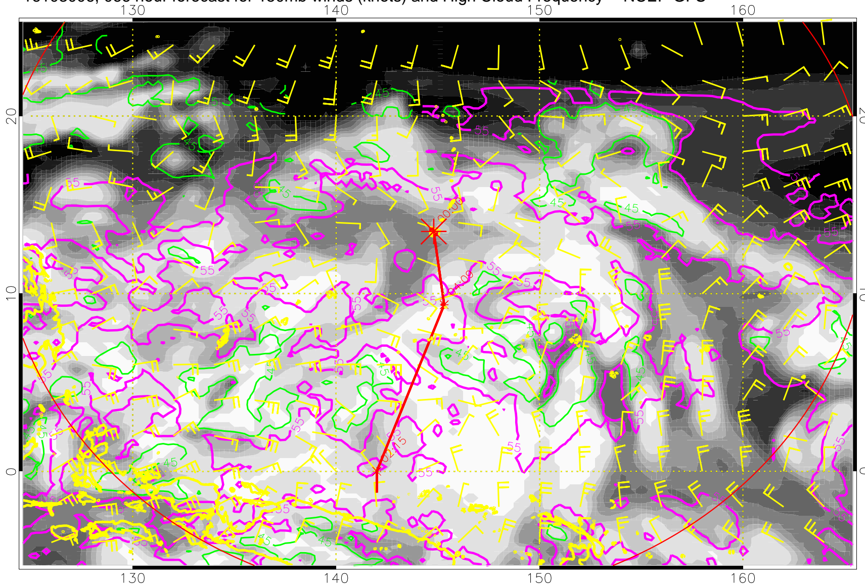
16103006, 066 hour forecast for 150mb winds (knots) and High Cloud Frequency -- NCEP GFS
