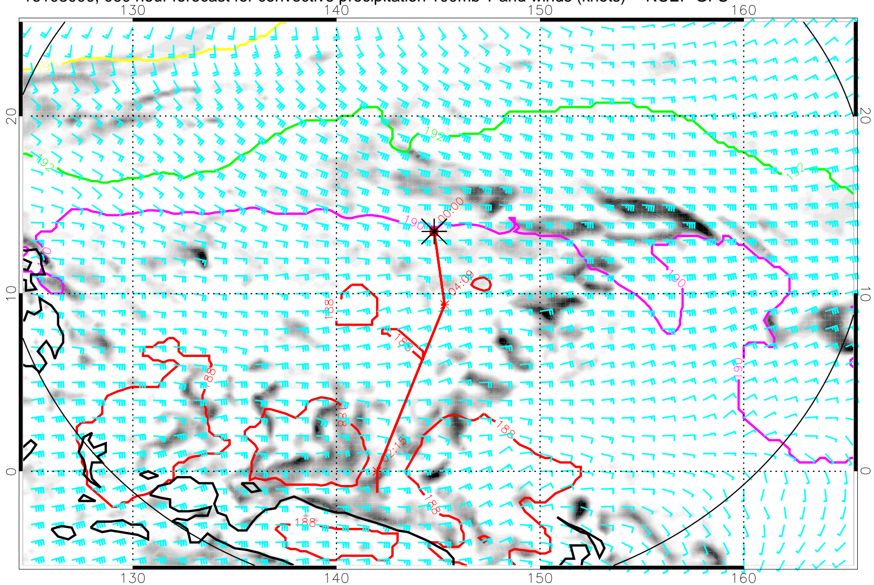
16103000, 060 hour forecast for convective precipitation 100mb T and winds (knots) -- NCEP GFS
