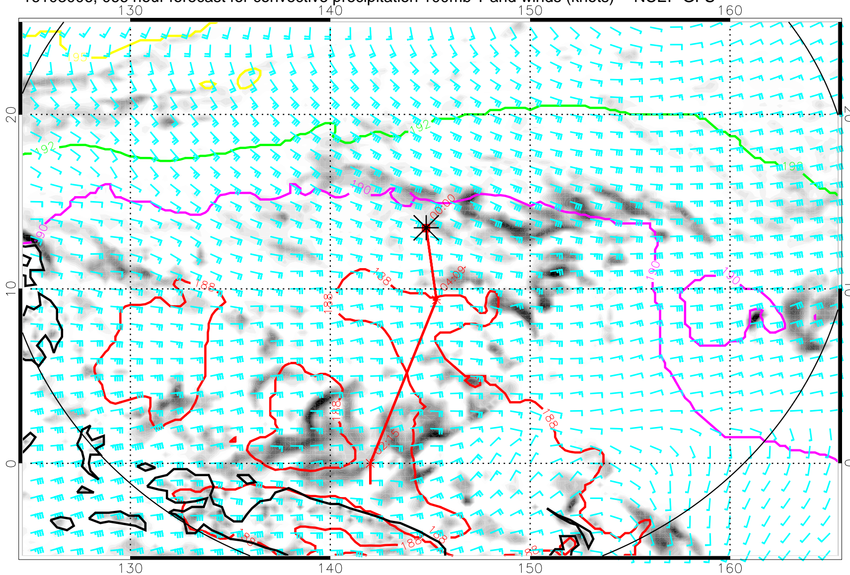
16103006, 066 hour forecast for convective precipitation 100mb T and winds (knots) -- NCEP GFS
