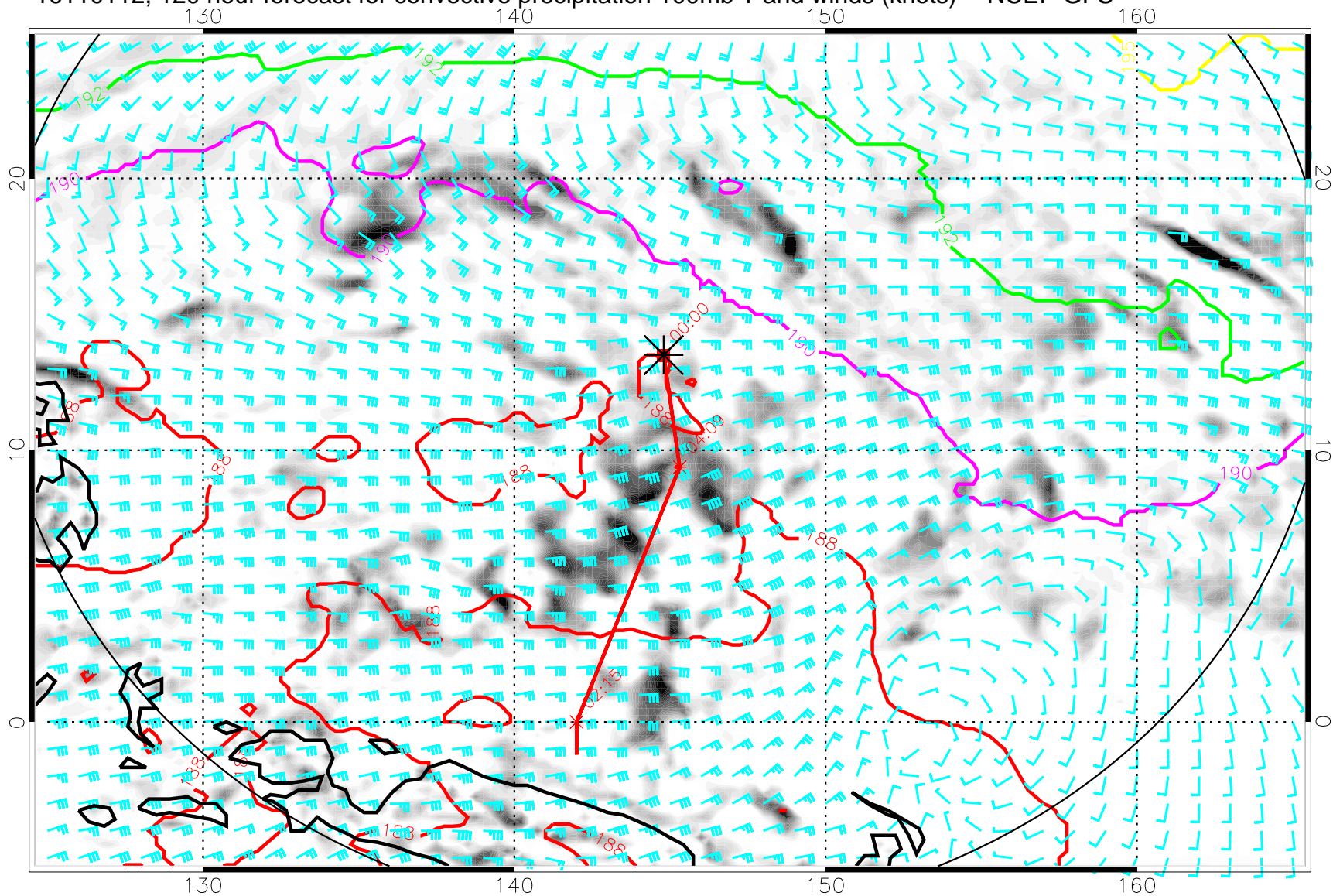
16110112, 120 hour forecast for convective precipitation 100mb T and winds (knots) -- NCEP GFS
