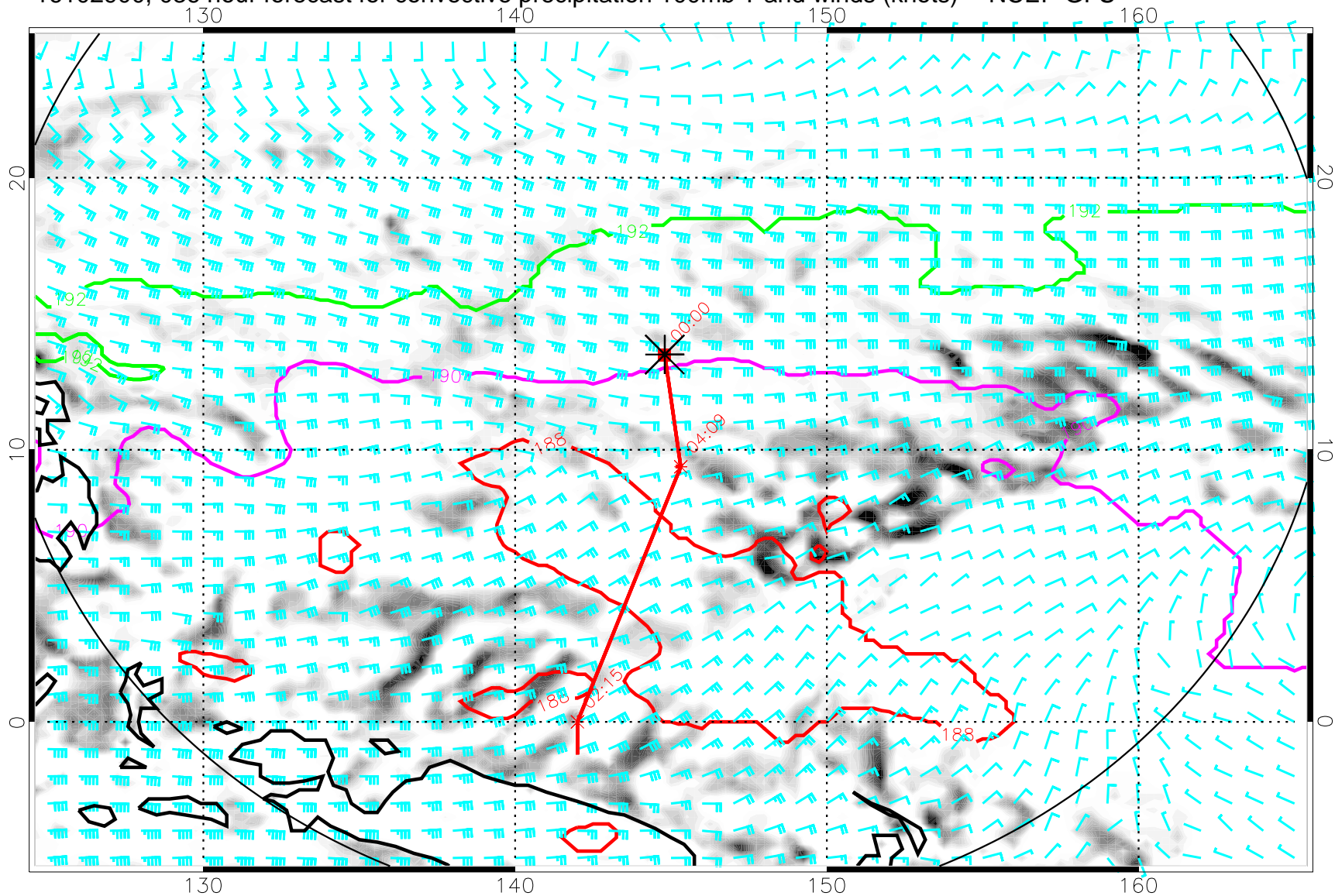
16102900, 036 hour forecast for convective precipitation 100mb T and winds (knots) -- NCEP GFS
