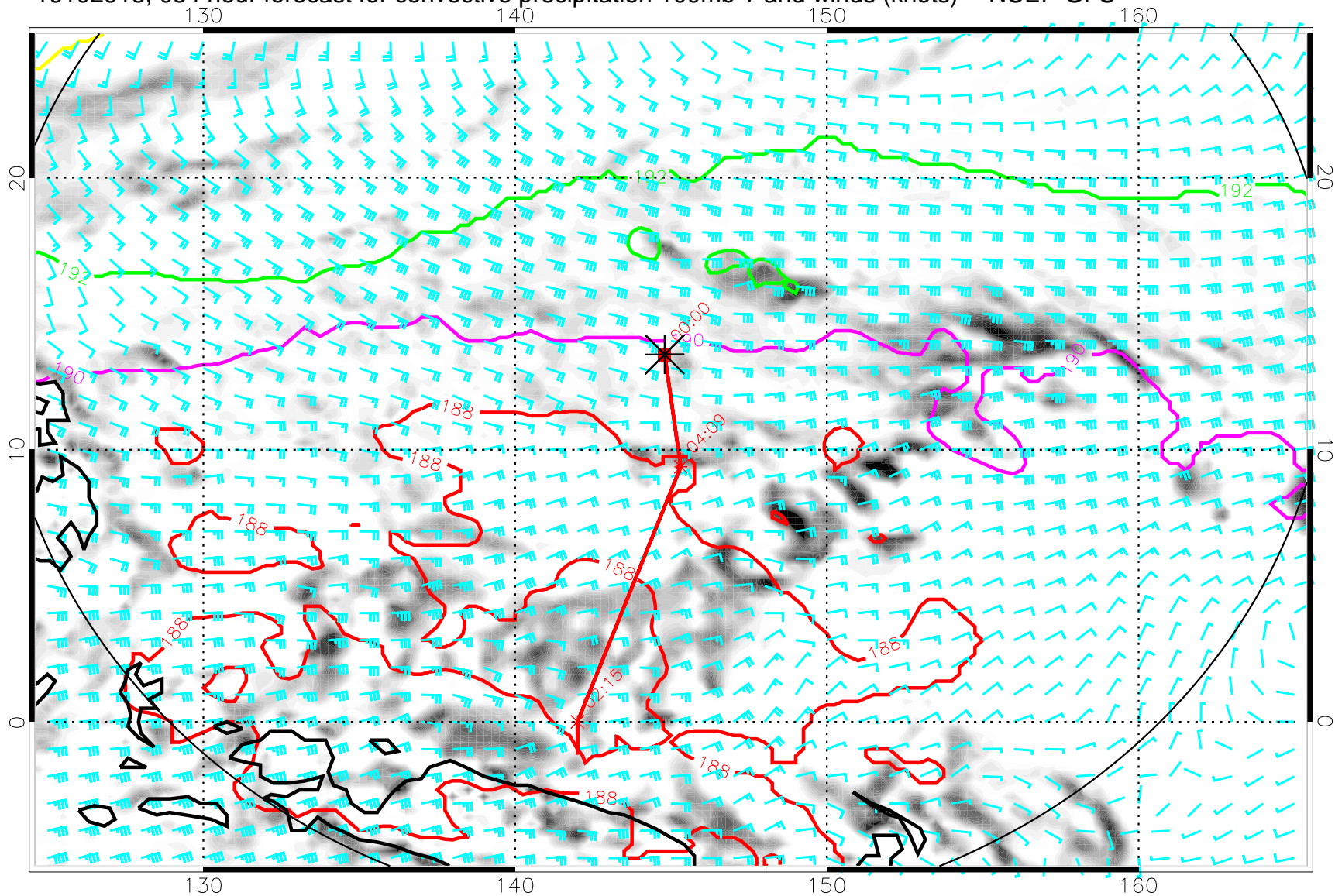
16102918, 054 hour forecast for convective precipitation 100mb T and winds (knots) -- NCEP GFS
