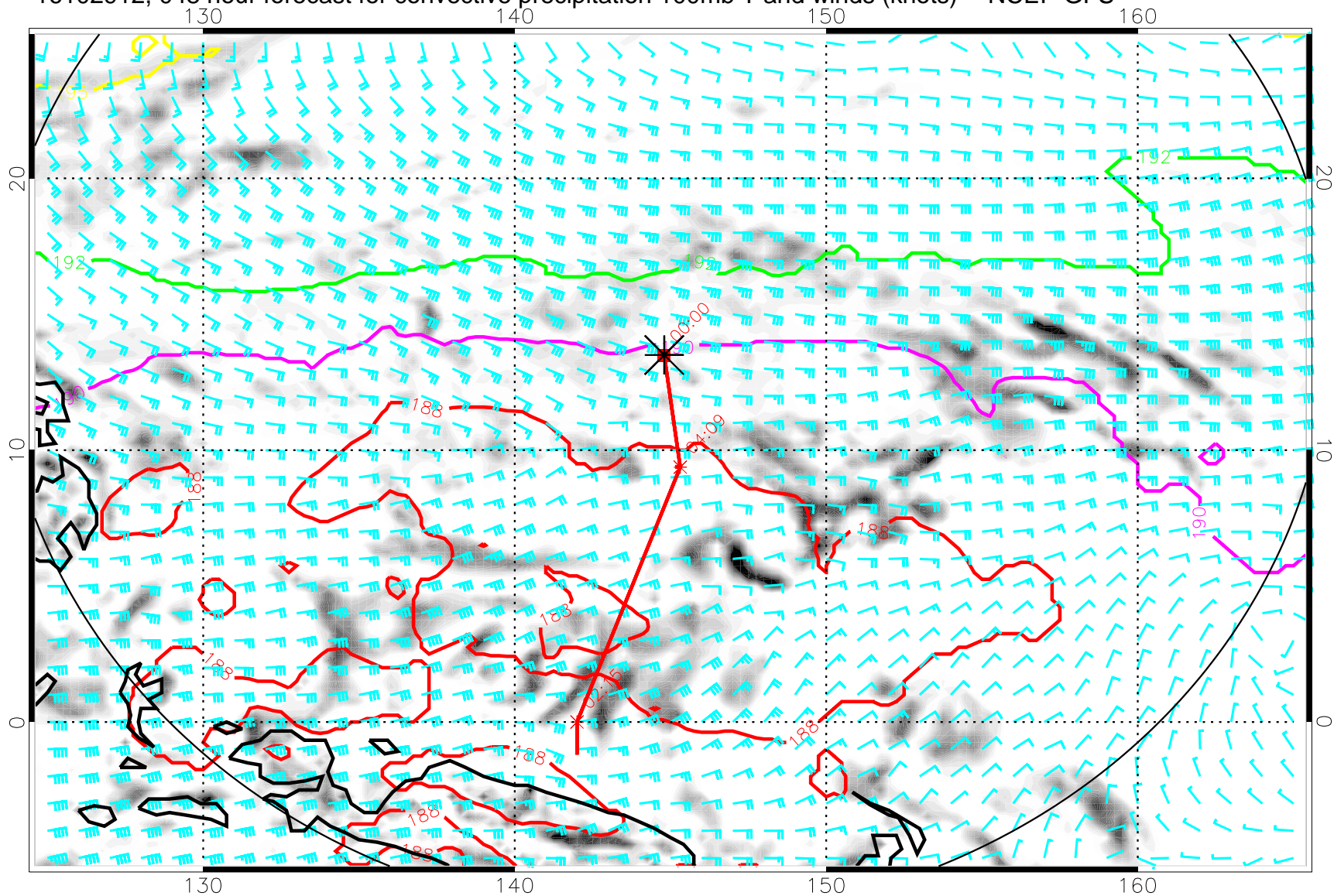
16102912, 048 hour forecast for convective precipitation 100mb T and winds (knots) -- NCEP GFS
