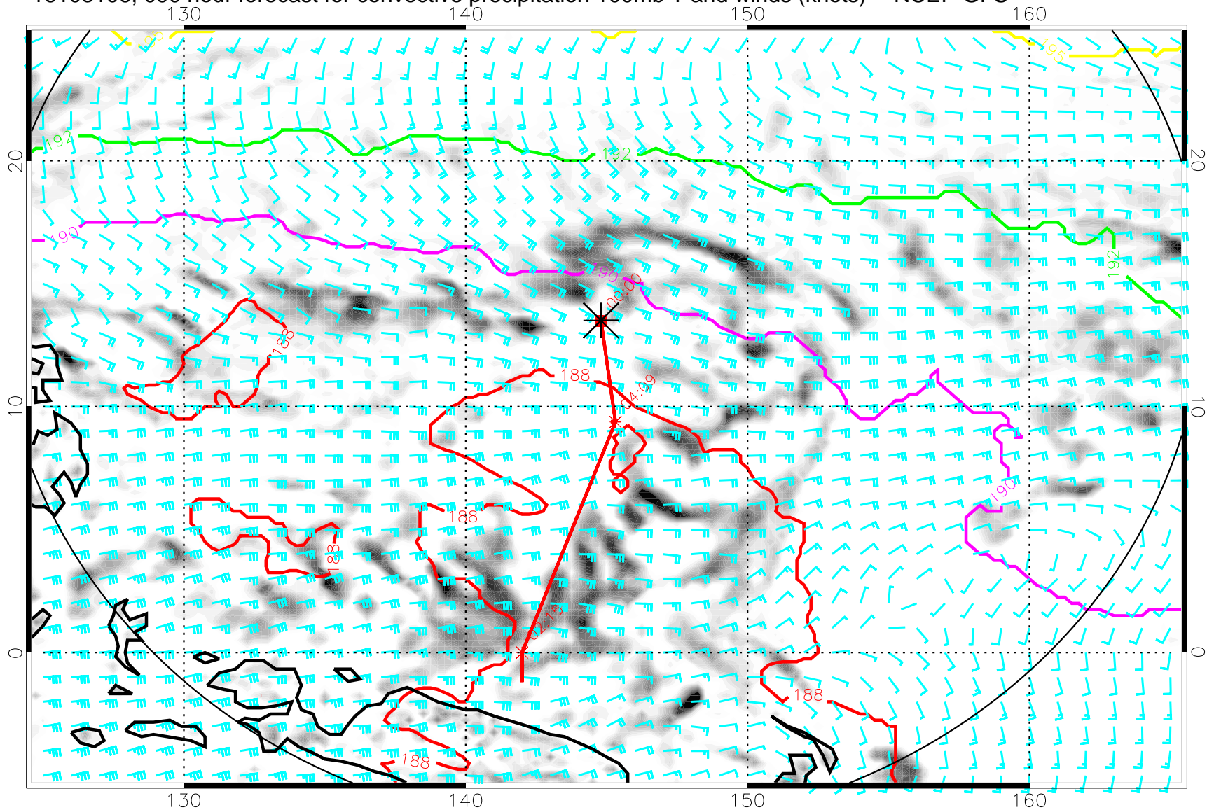
16103106, 090 hour forecast for convective precipitation 100mb T and winds (knots) -- NCEP GFS
