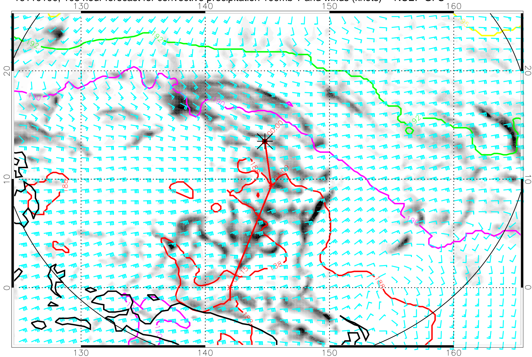
16110100, 108 hour forecast for convective precipitation 100mb T and winds (knots) -- NCEP GFS
