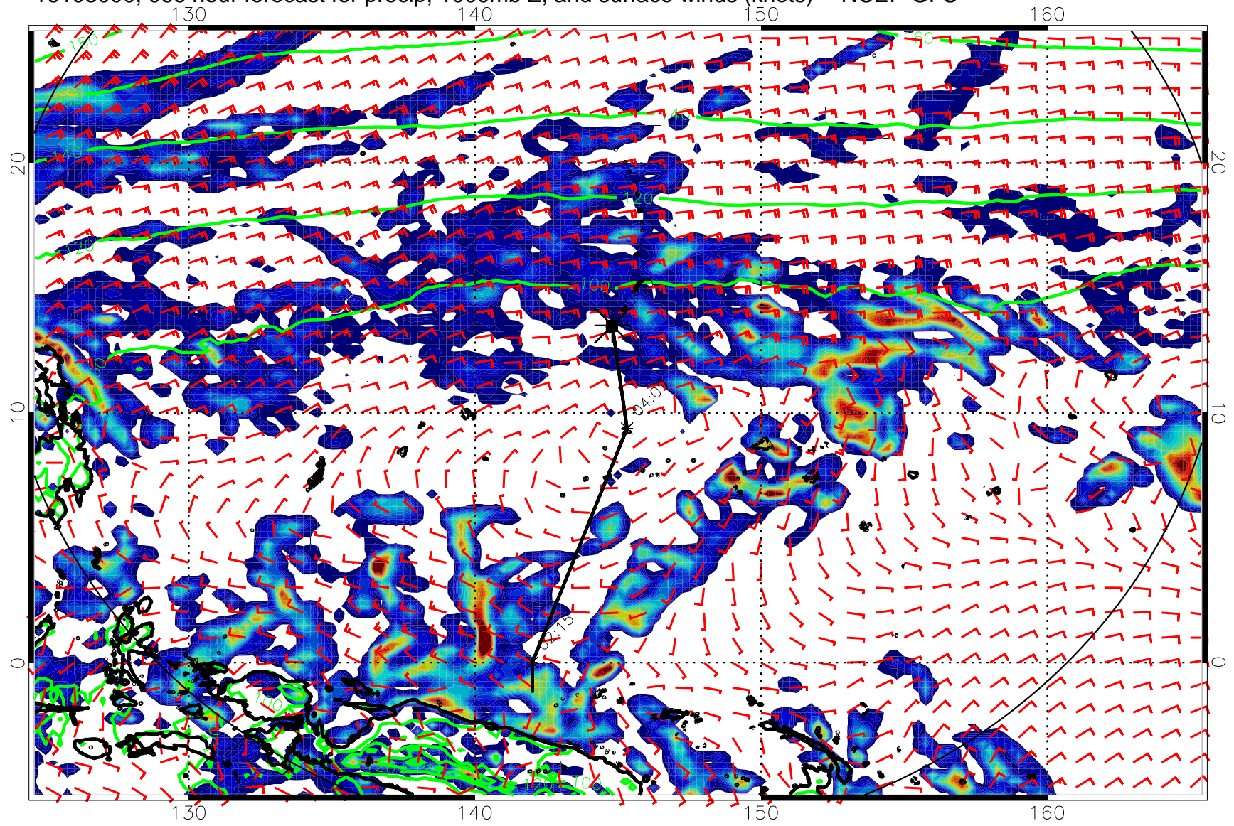
16103000, 066 hour forecast for precip, 1000mb Z, and surface winds (knots) -- NCEP GFS
