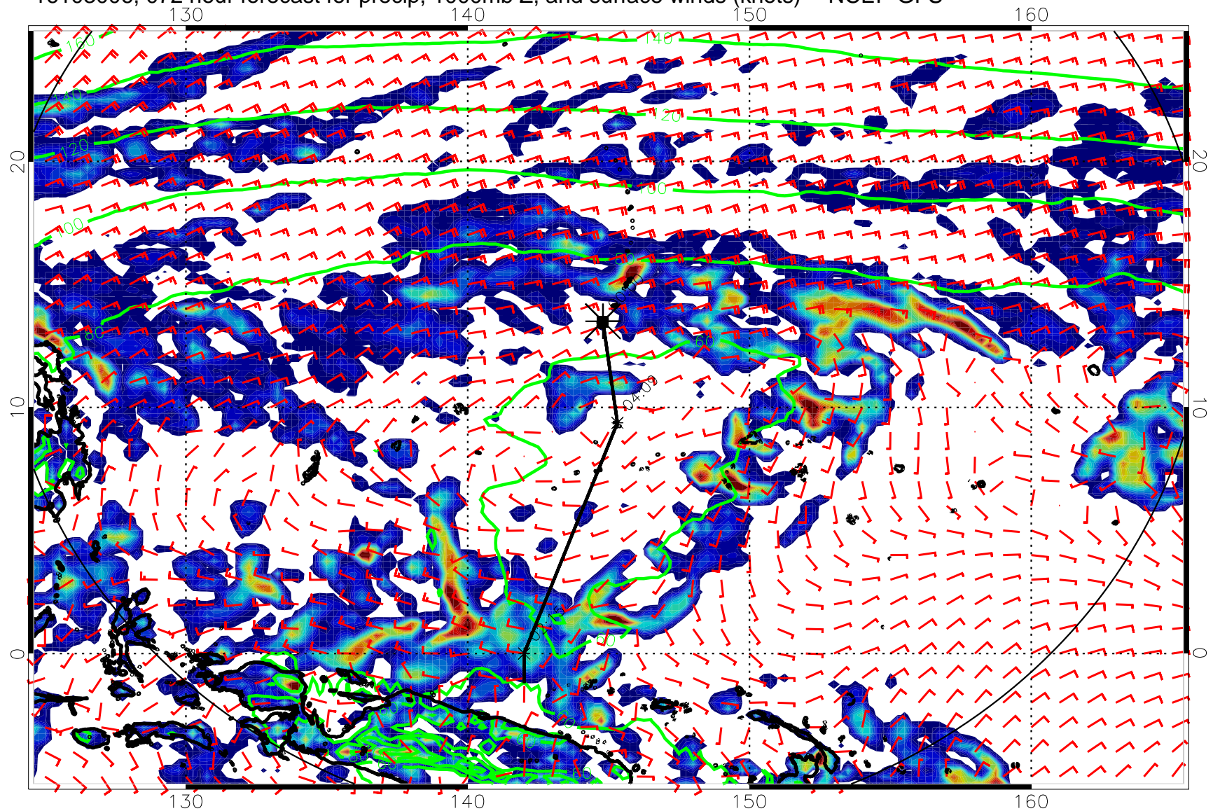
16103006, 072 hour forecast for precip, 1000mb Z, and surface winds (knots) -- NCEP GFS
