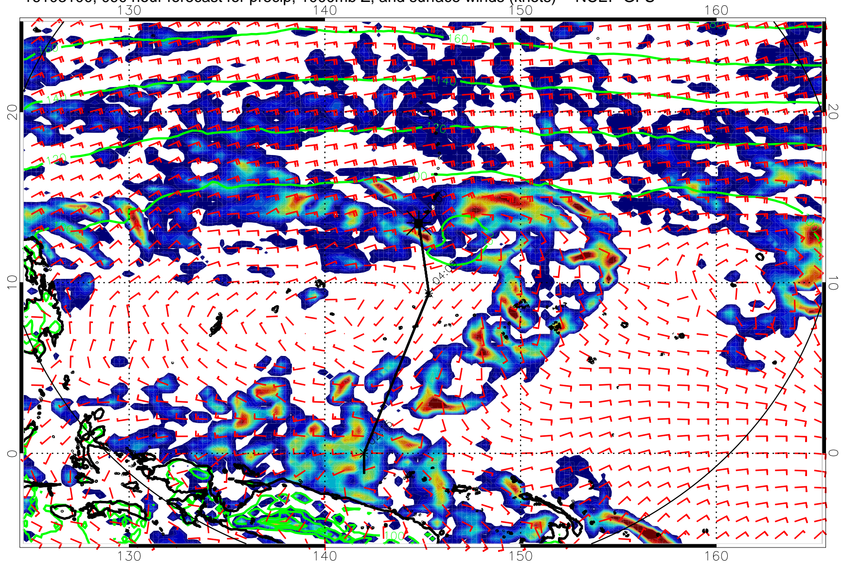
16103100, 090 hour forecast for precip, 1000mb Z, and surface winds (knots) -- NCEP GFS
