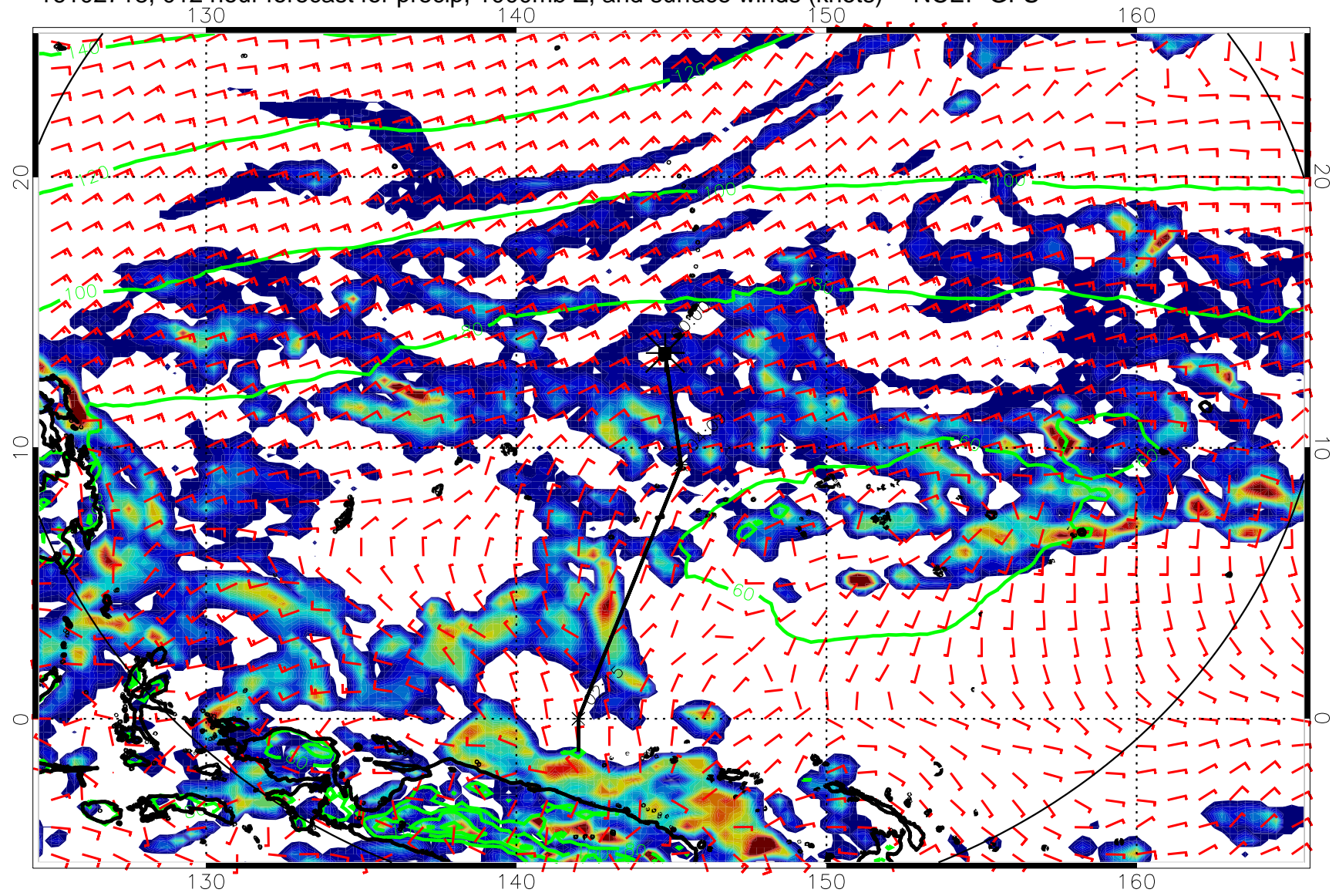
16102718, 012 hour forecast for precip, 1000mb Z, and surface winds (knots) -- NCEP GFS
