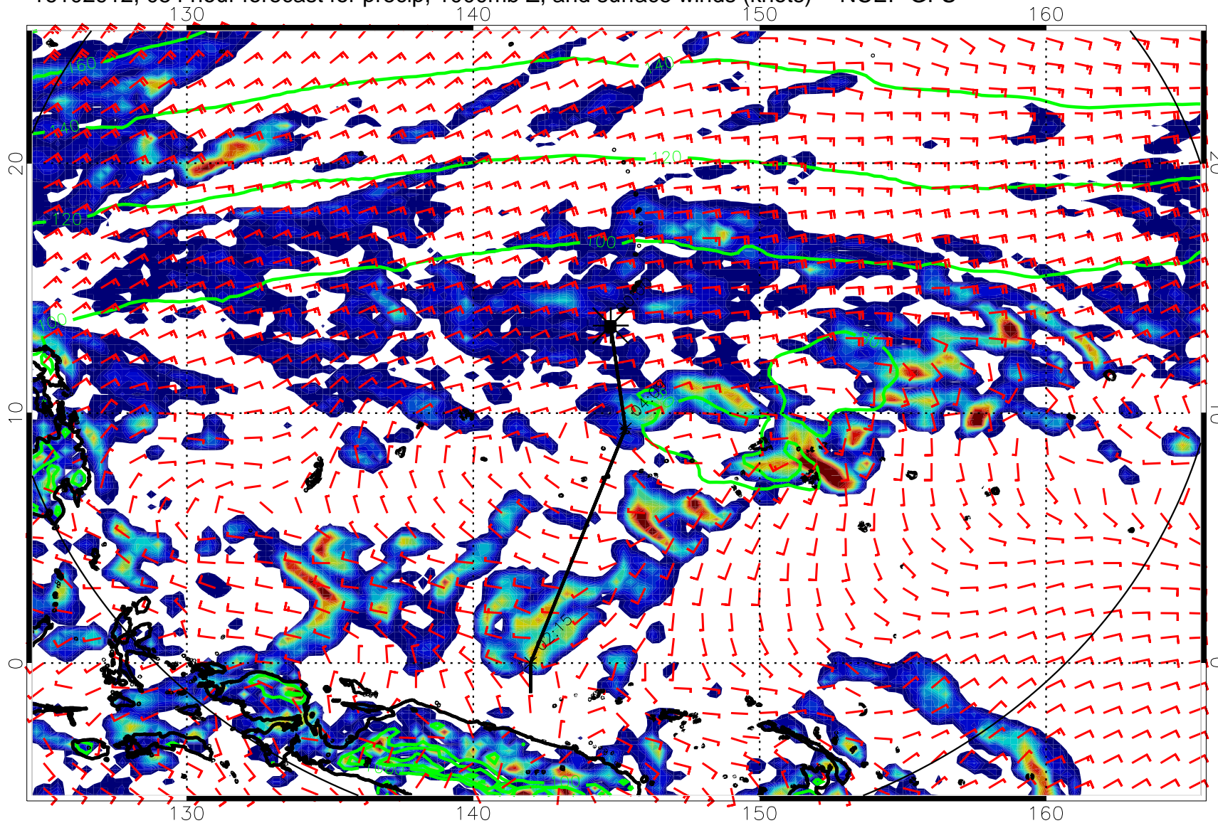
16102912, 054 hour forecast for precip, 1000mb Z, and surface winds (knots) -- NCEP GFS
