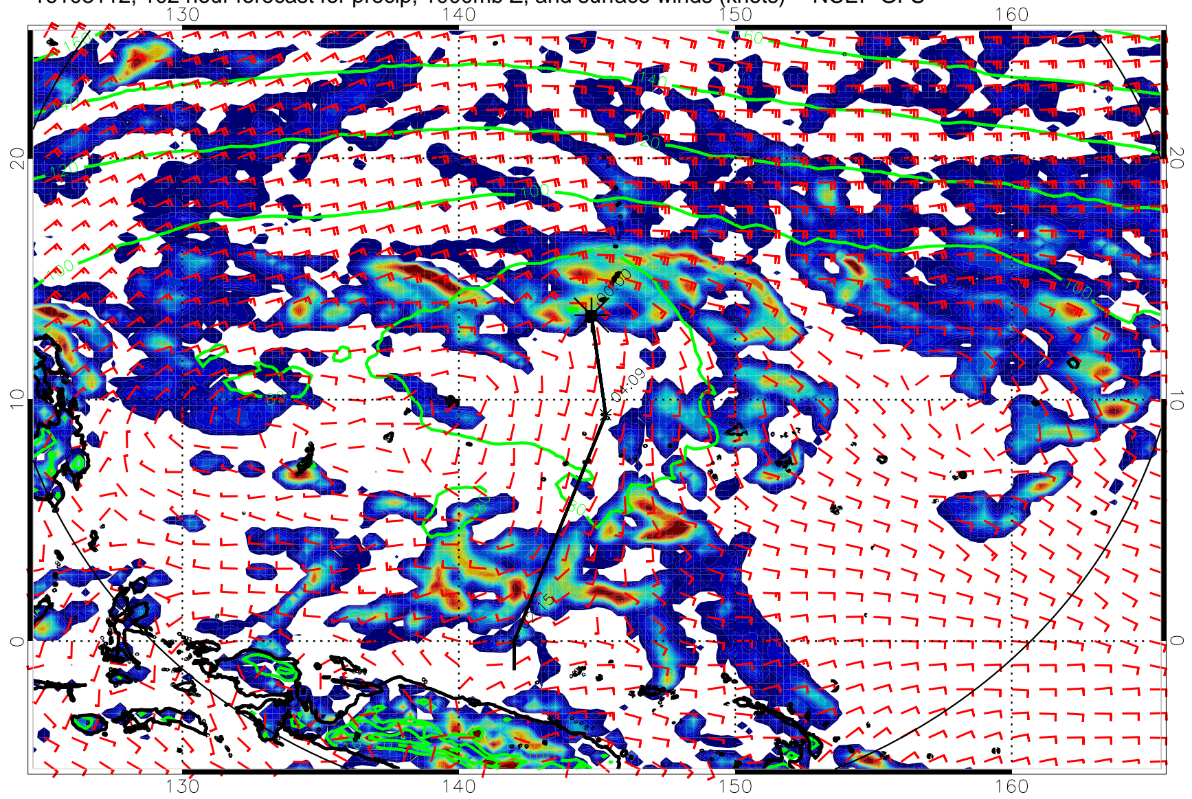
16103112, 102 hour forecast for precip, 1000mb Z, and surface winds (knots) -- NCEP GFS
