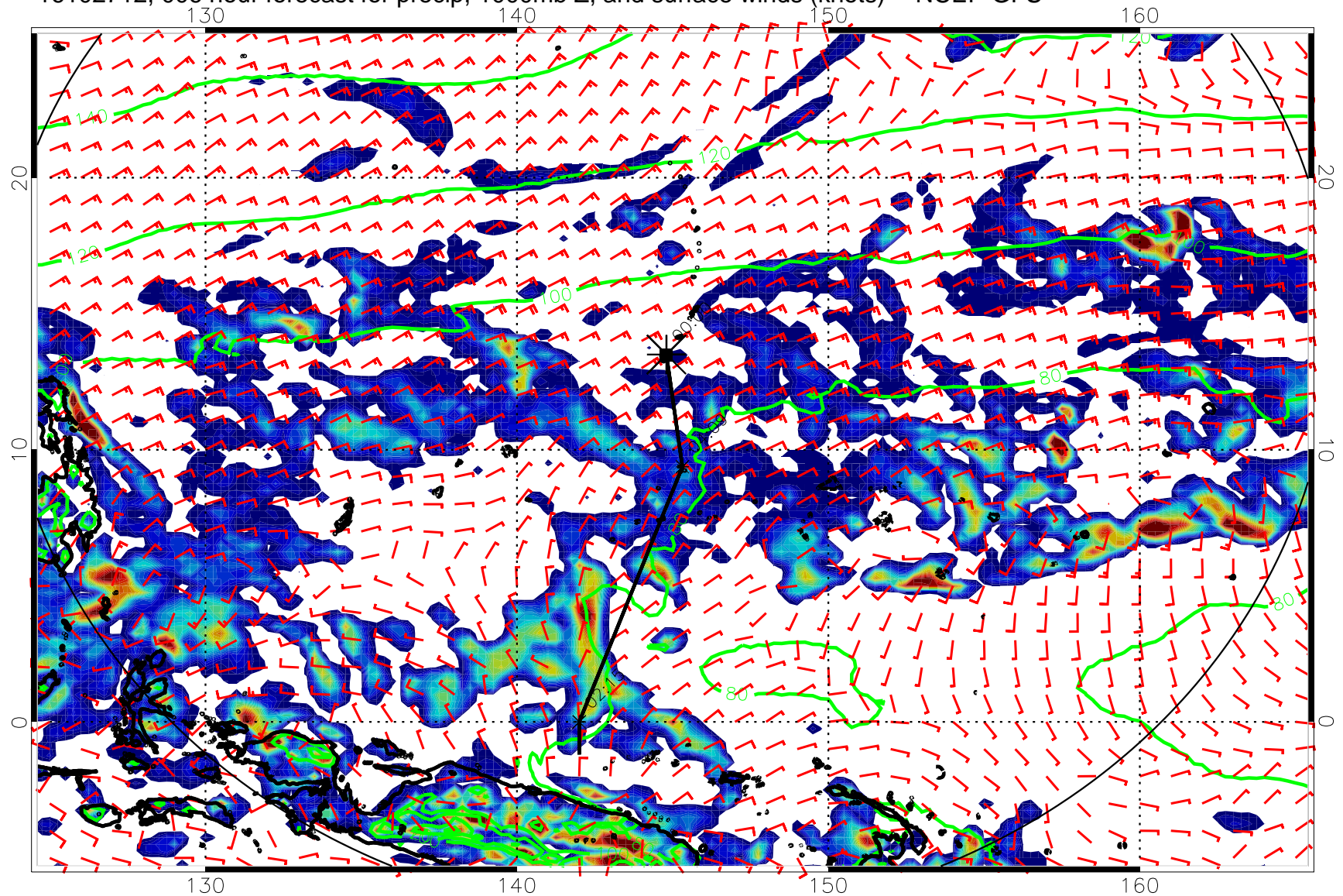
16102712, 006 hour forecast for precip, 1000mb Z, and surface winds (knots) -- NCEP GFS
