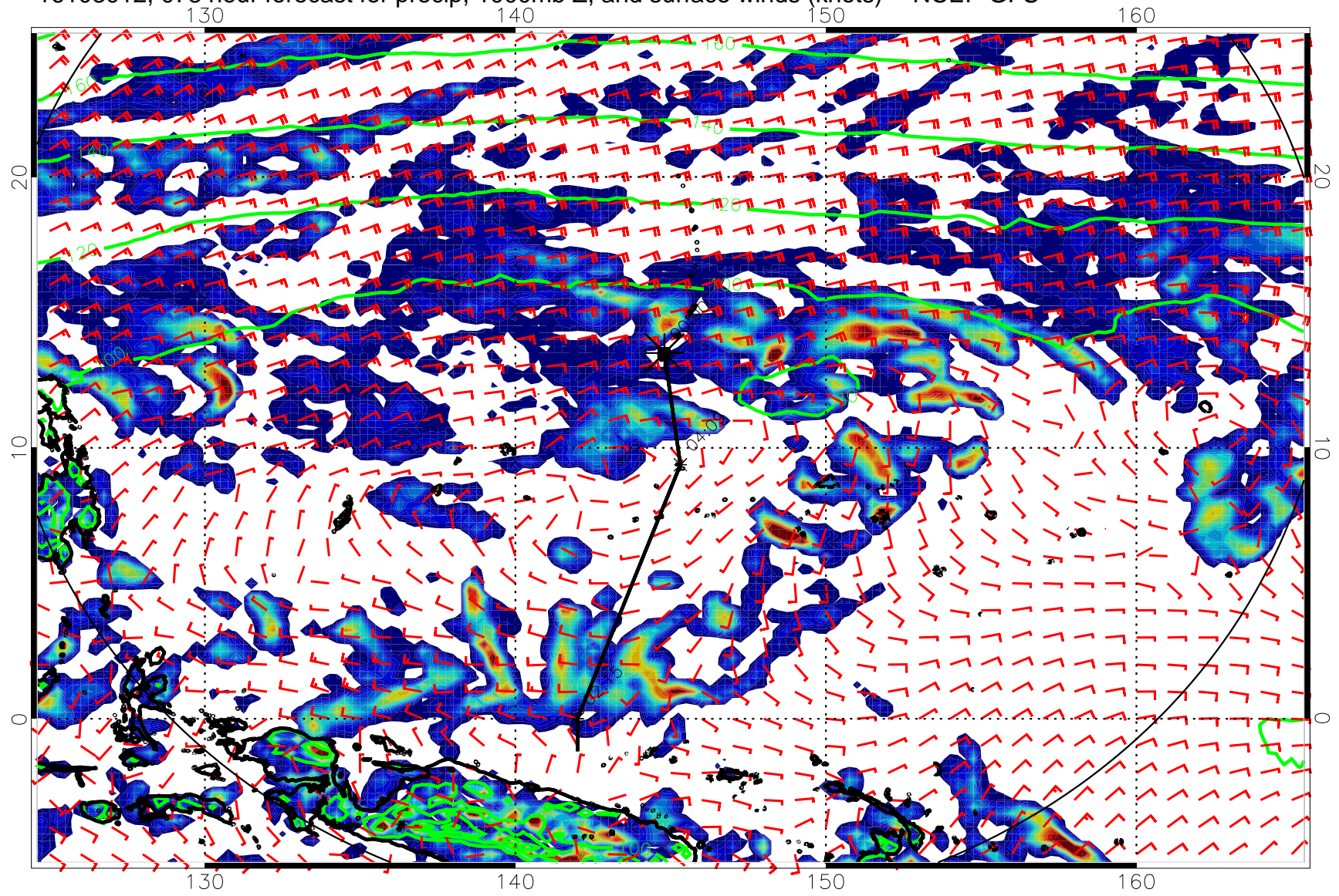
16103012, 078 hour forecast for precip, 1000mb Z, and surface winds (knots) -- NCEP GFS
