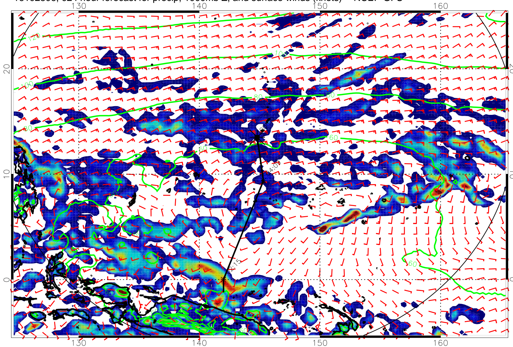
16102806, 024 hour forecast for precip, 1000mb Z, and surface winds (knots) -- NCEP GFS
