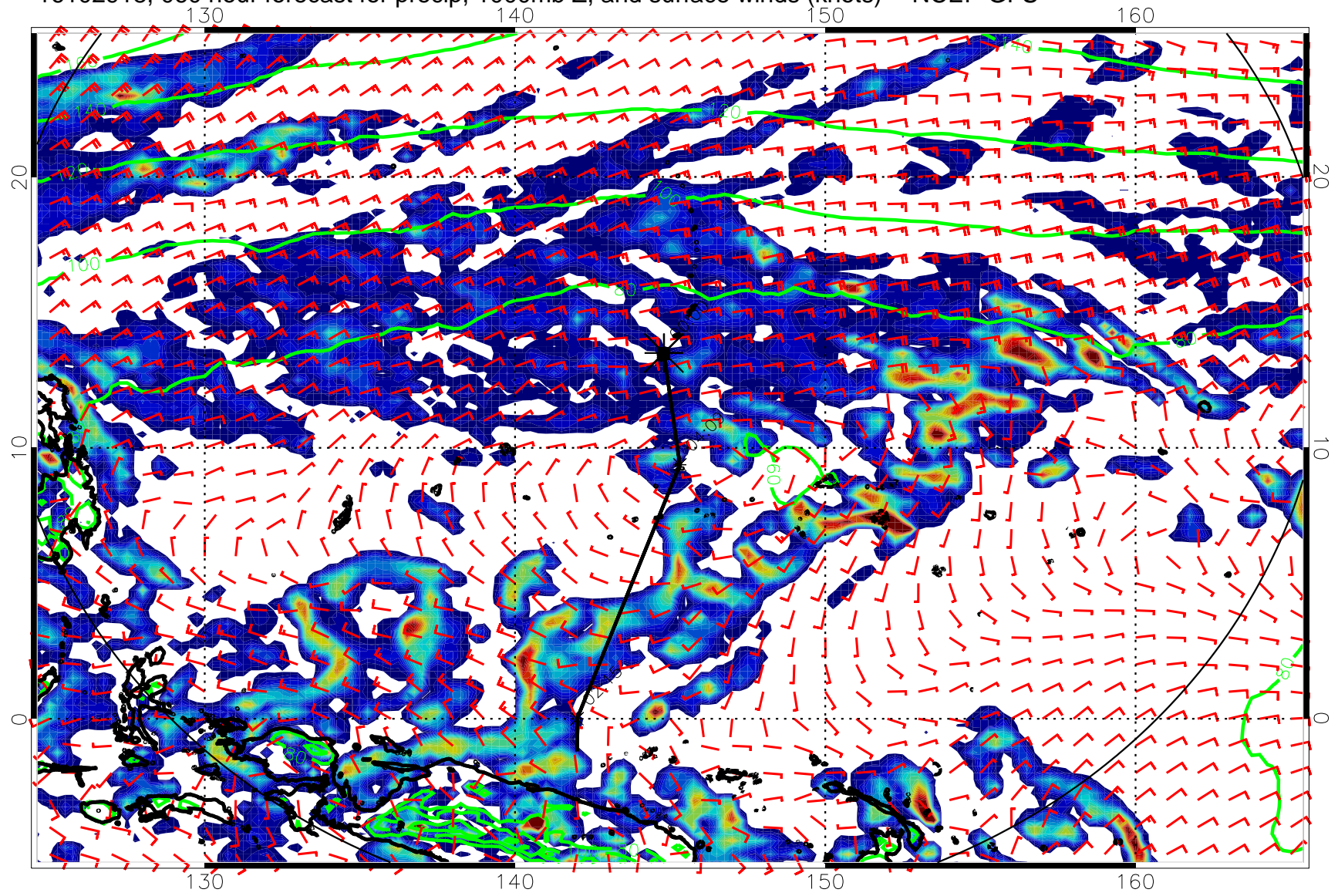
16102918, 060 hour forecast for precip, 1000mb Z, and surface winds (knots) -- NCEP GFS
