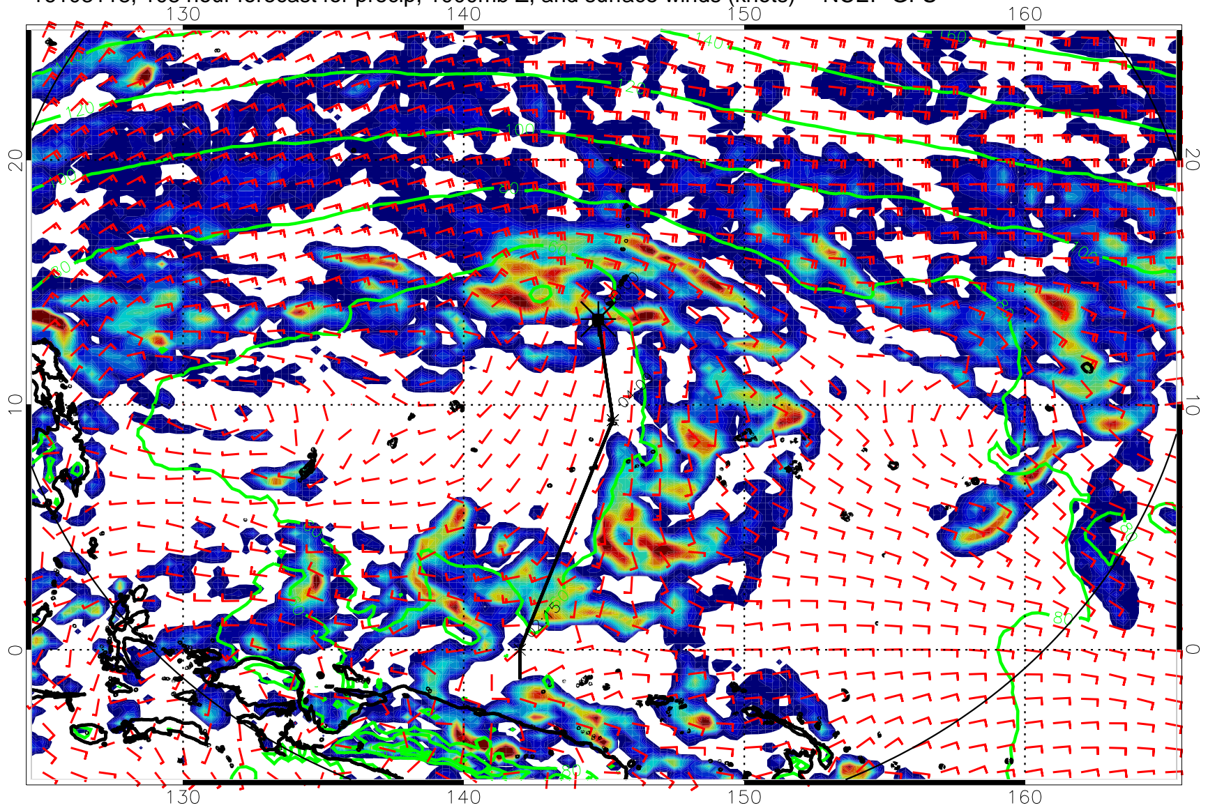
16103118, 108 hour forecast for precip, 1000mb Z, and surface winds (knots) -- NCEP GFS
