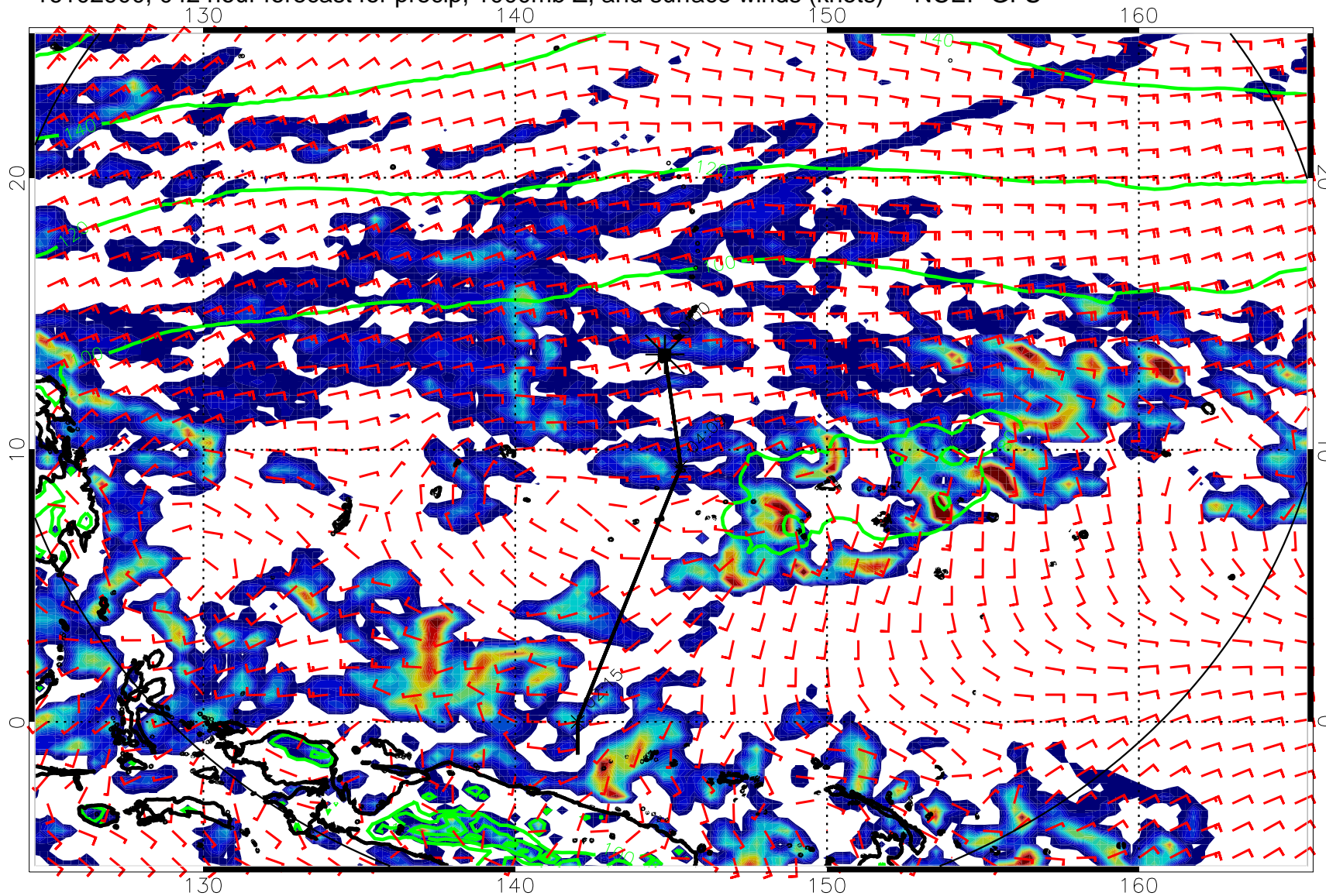
16102900, 042 hour forecast for precip, 1000mb Z, and surface winds (knots) -- NCEP GFS
