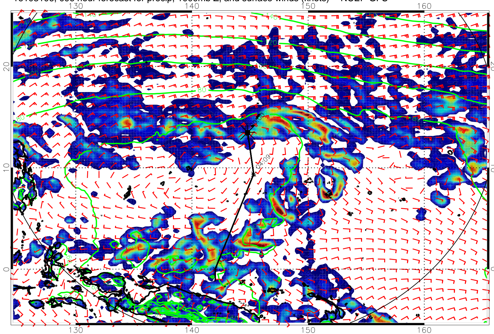
16103106, 096 hour forecast for precip, 1000mb Z, and surface winds (knots) -- NCEP GFS
