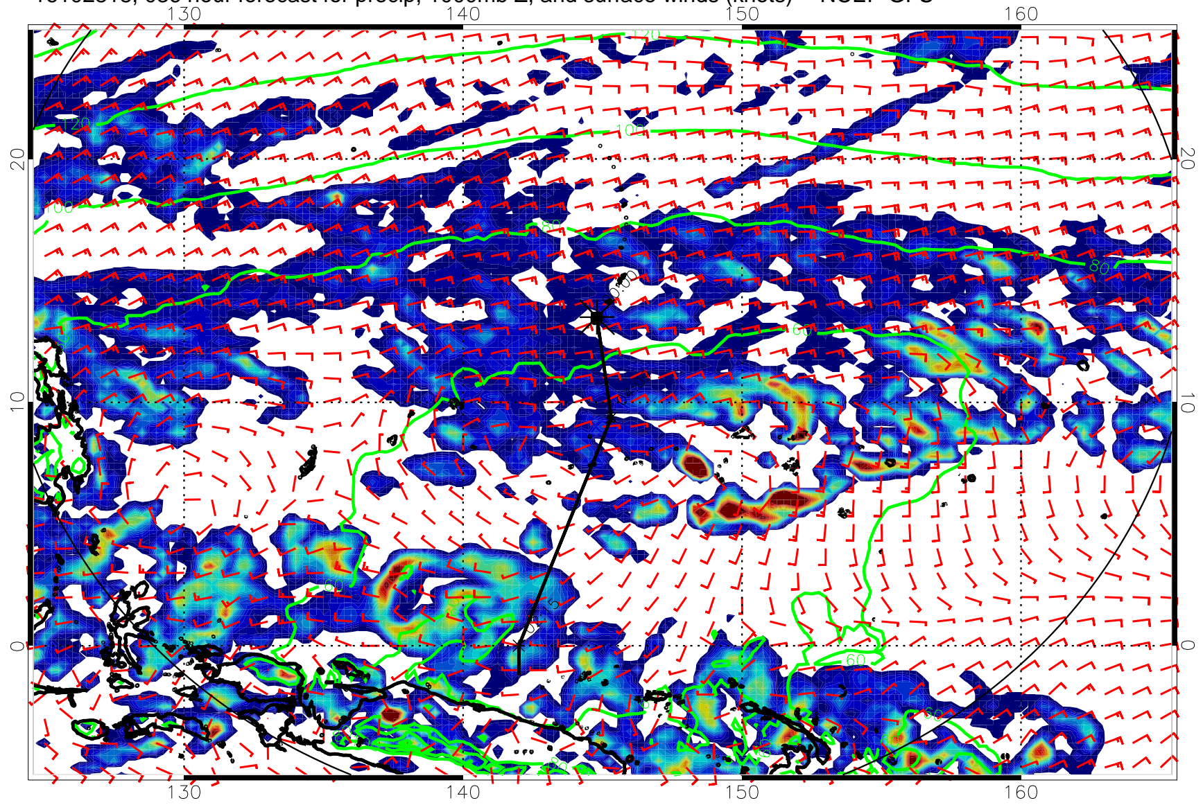
16102818, 036 hour forecast for precip, 1000mb Z, and surface winds (knots) -- NCEP GFS
