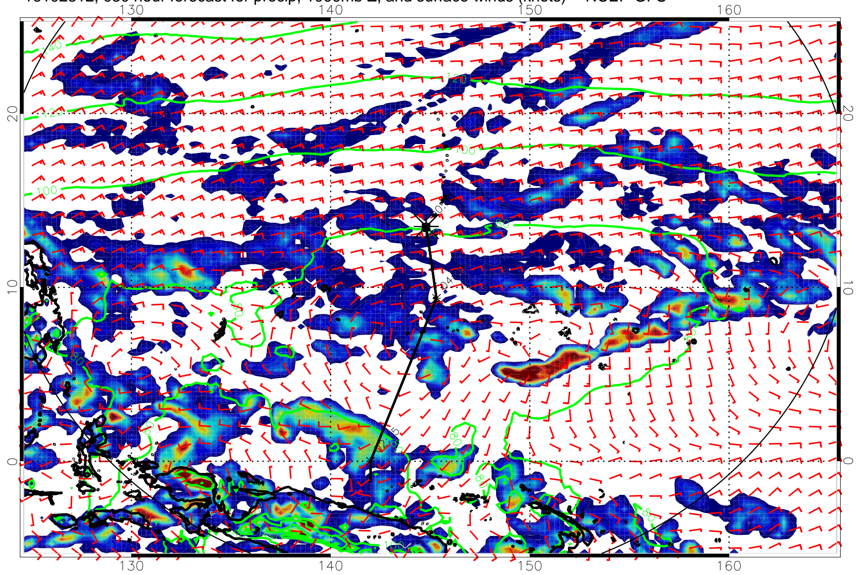
16102812, 030 hour forecast for precip, 1000mb Z, and surface winds (knots) -- NCEP GFS
