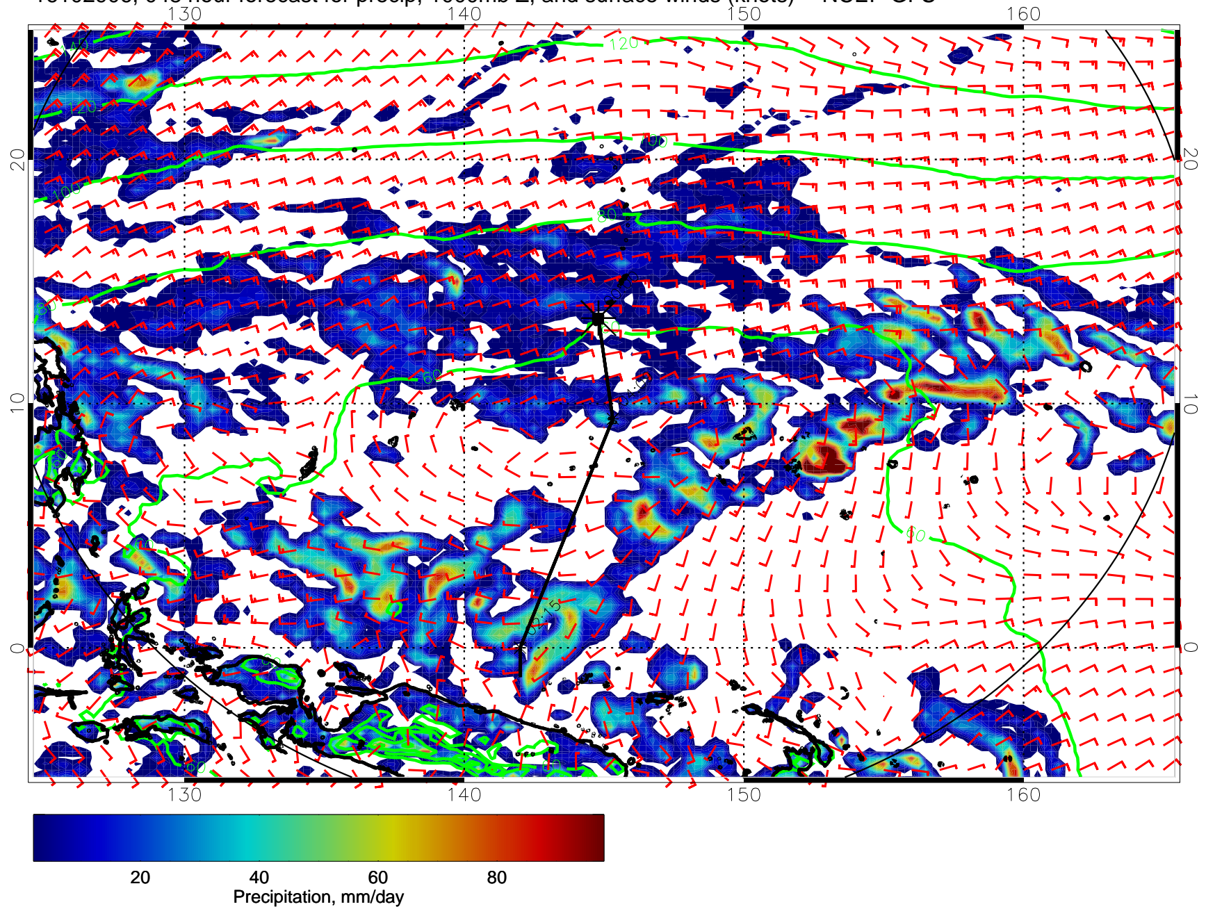
16102906, 048 hour forecast for precip, 1000mb Z, and surface winds (knots) -- NCEP GFS
