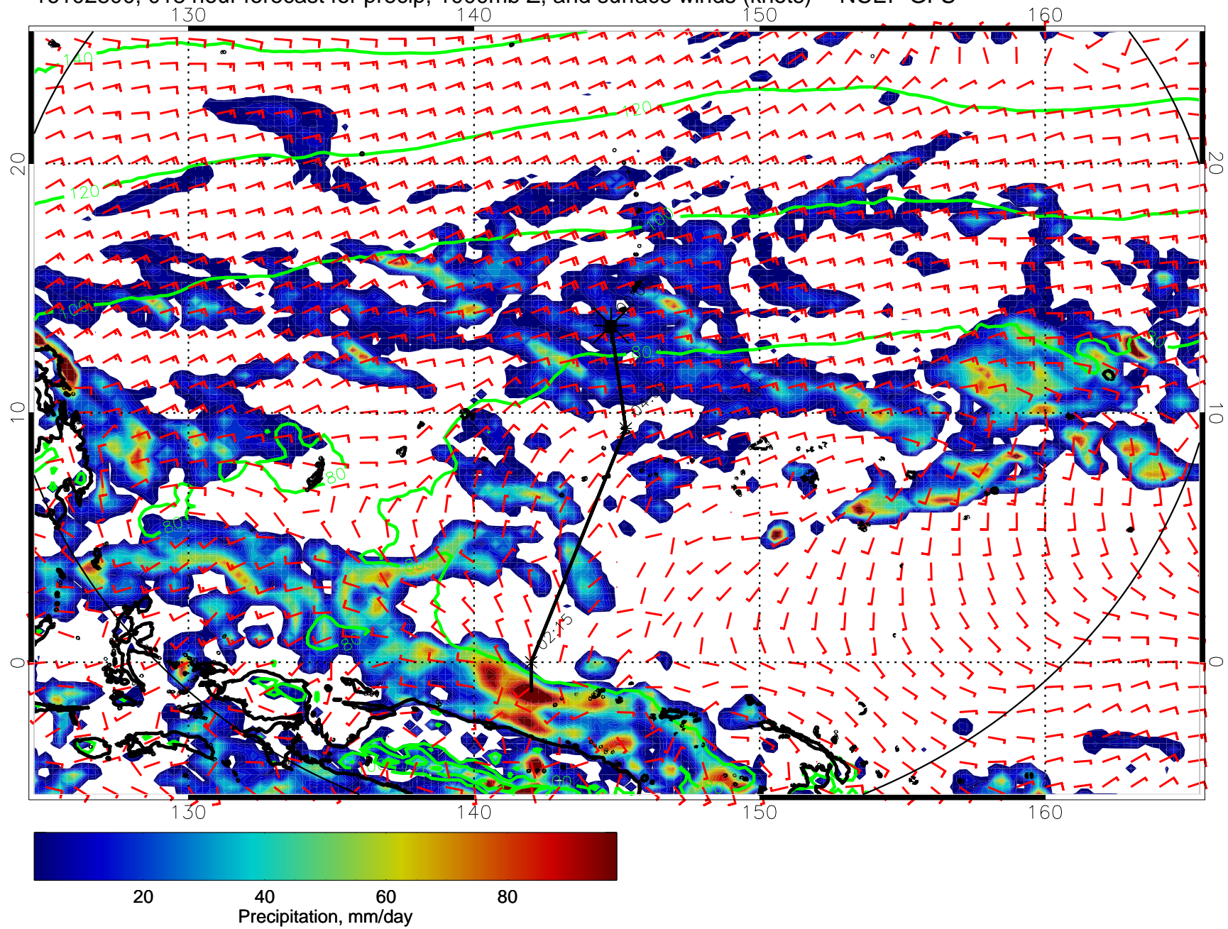
16102800, 018 hour forecast for precip, 1000mb Z, and surface winds (knots) -- NCEP GFS
