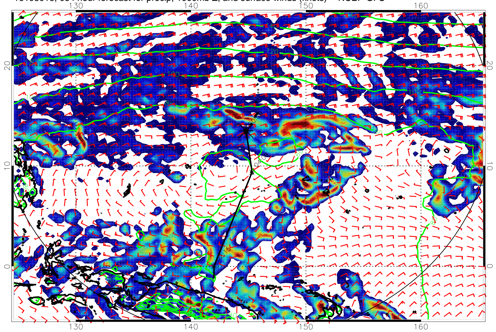
16103018, 084 hour forecast for precip, 1000mb Z, and surface winds (knots) -- NCEP GFS
