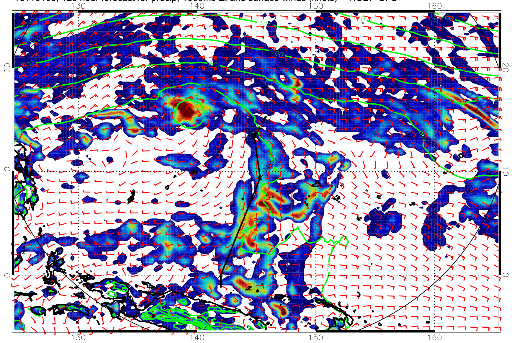
16110106, 120 hour forecast for precip, 1000mb Z, and surface winds (knots) -- NCEP GFS
