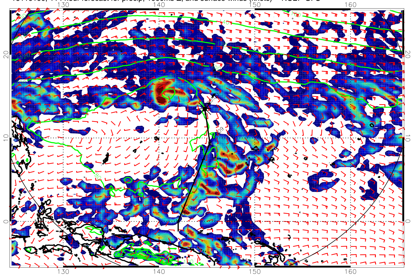
16110100, 114 hour forecast for precip, 1000mb Z, and surface winds (knots) -- NCEP GFS
