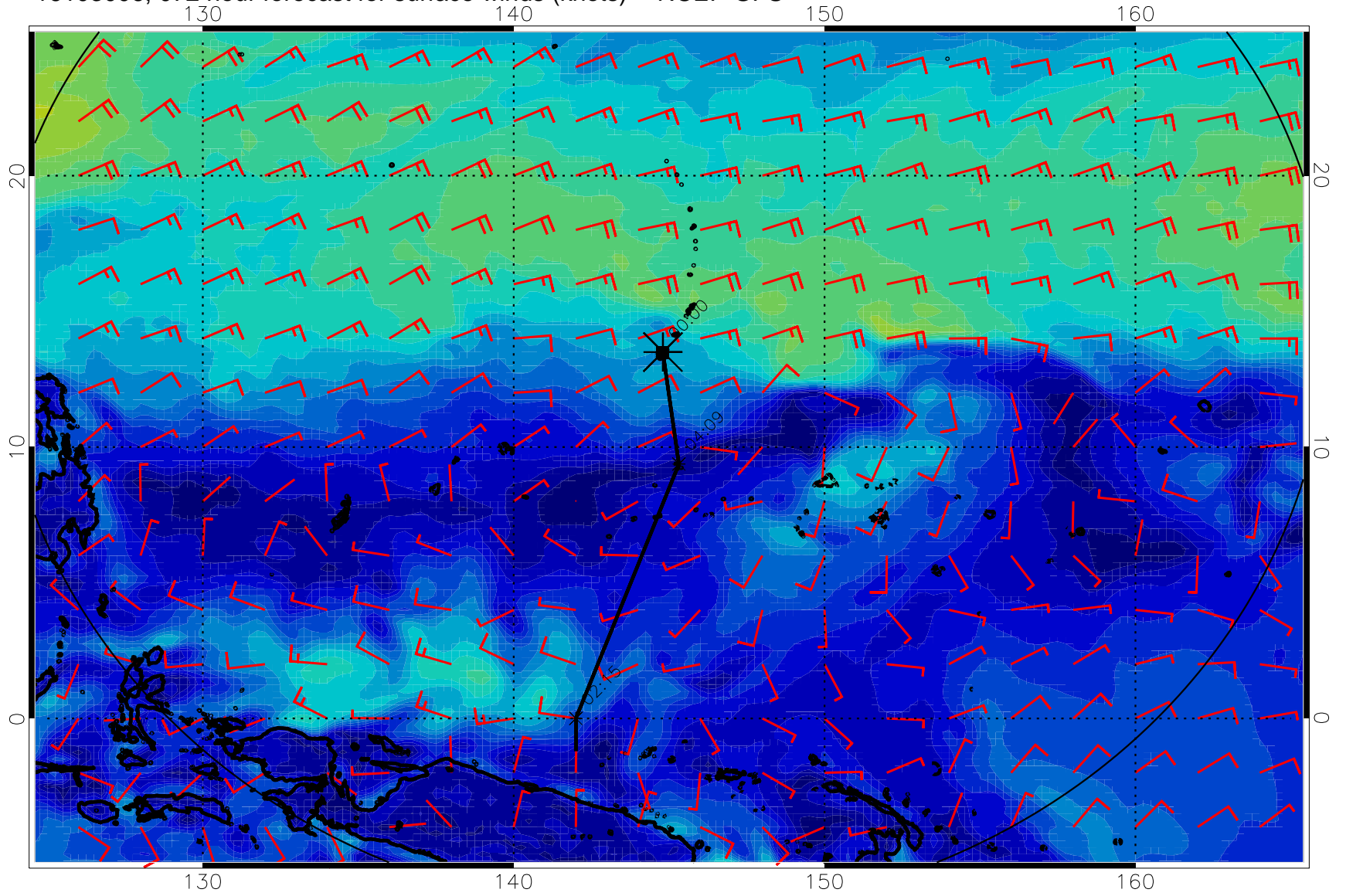
16103006, 072 hour forecast for surface winds (knots) -- NCEP GFS
