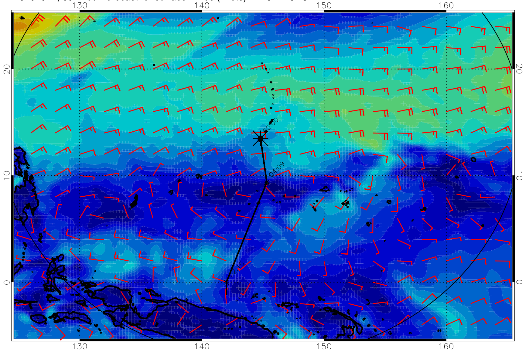
16102912, 054 hour forecast for surface winds (knots) -- NCEP GFS
