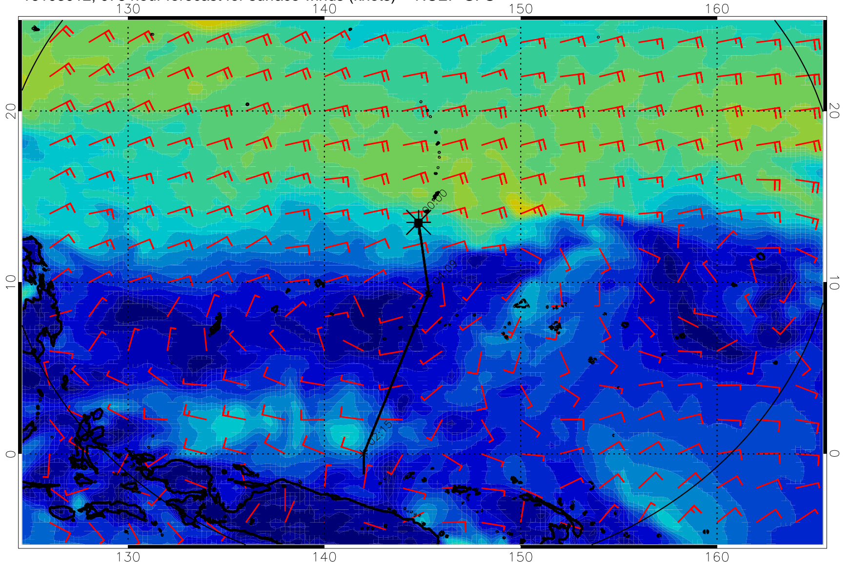
16103012, 078 hour forecast for surface winds (knots) -- NCEP GFS
