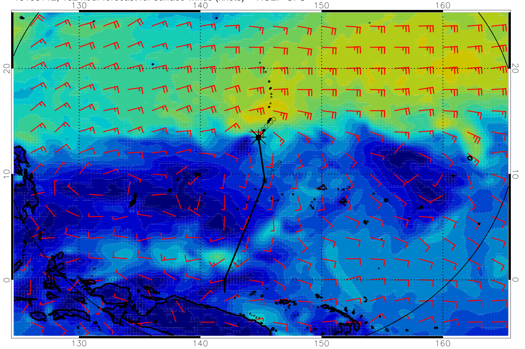
16103112, 102 hour forecast for surface winds (knots) -- NCEP GFS
