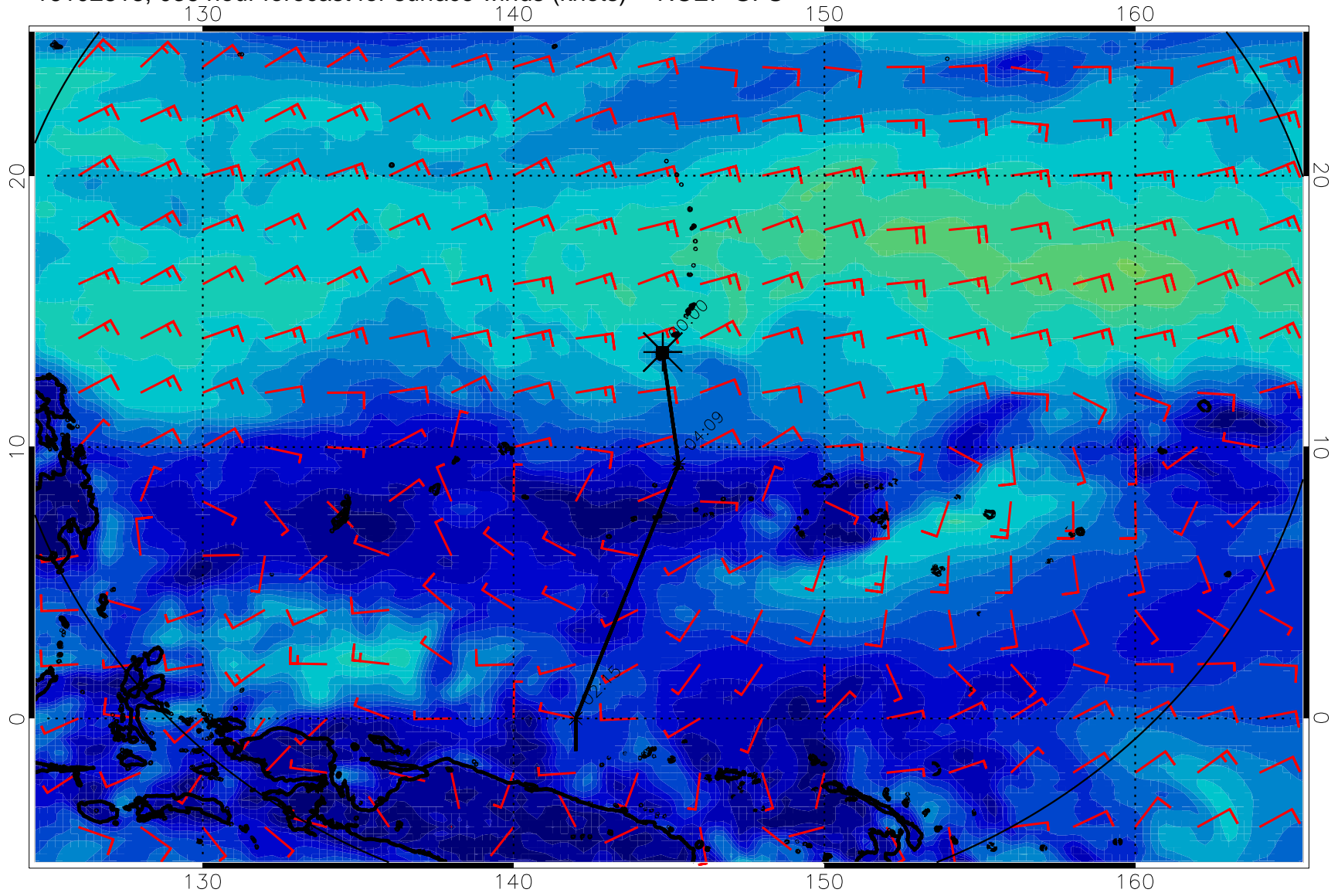
16102818, 036 hour forecast for surface winds (knots) -- NCEP GFS
