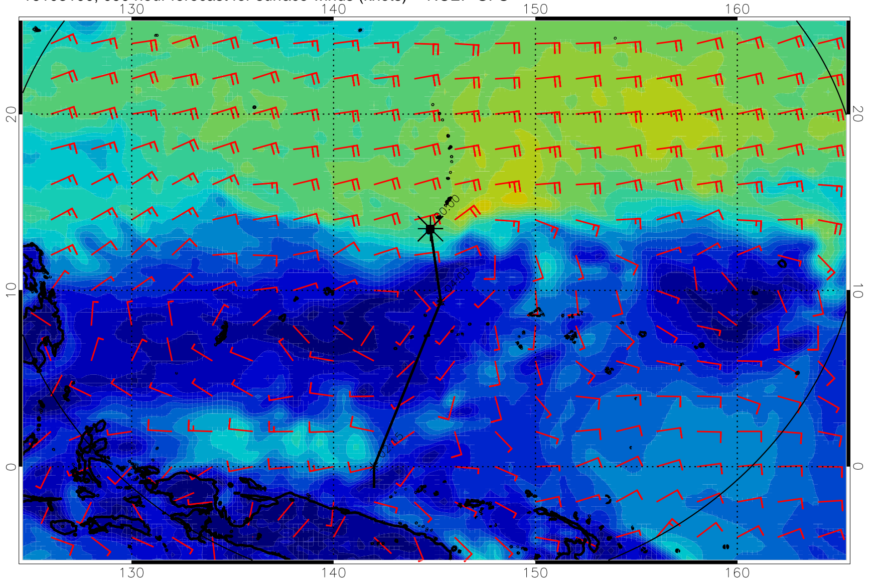
16103100, 090 hour forecast for surface winds (knots) -- NCEP GFS
