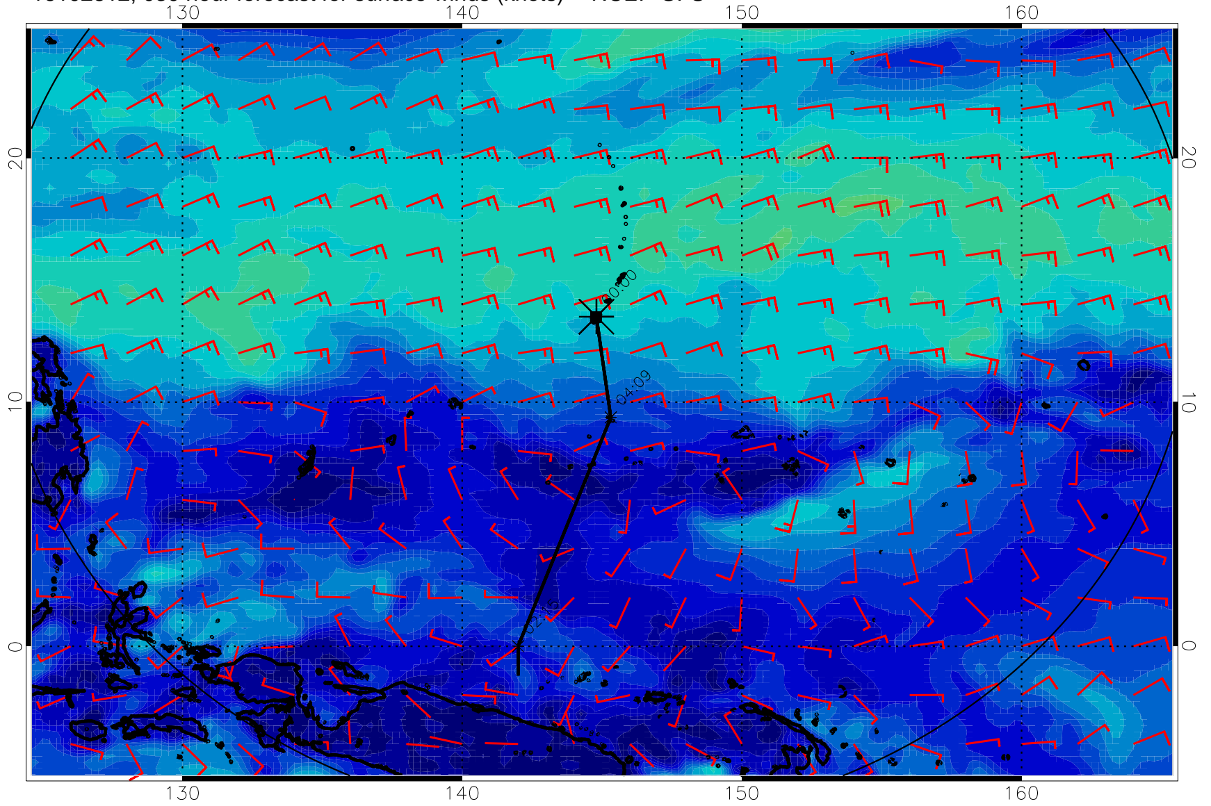
16102812, 030 hour forecast for surface winds (knots) -- NCEP GFS
