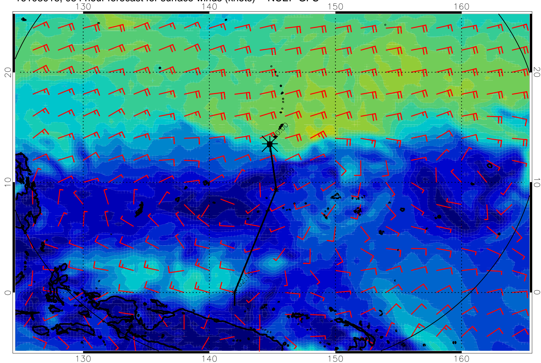
16103018, 084 hour forecast for surface winds (knots) -- NCEP GFS
