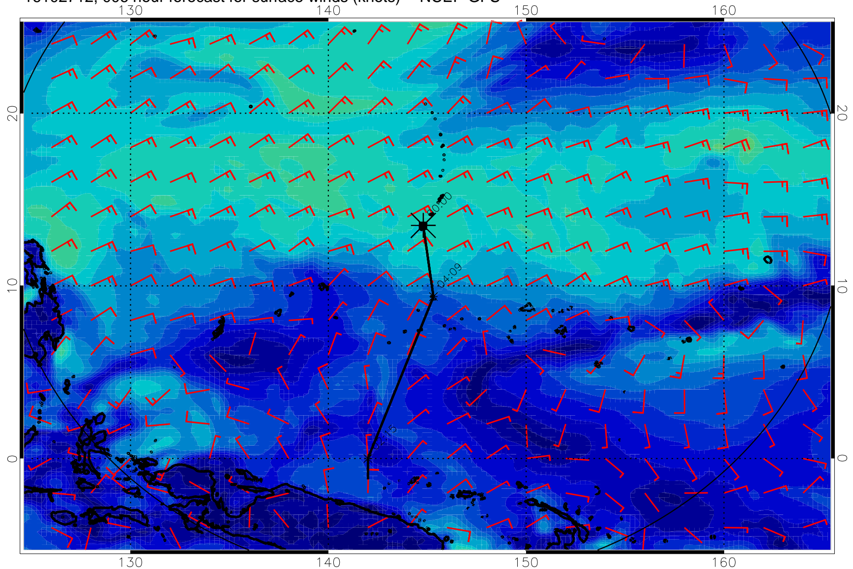
16102712, 006 hour forecast for surface winds (knots) -- NCEP GFS
