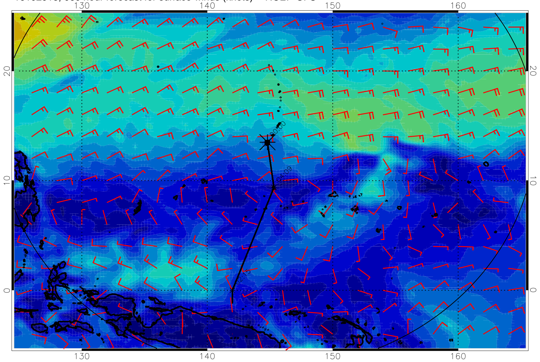
16102918, 060 hour forecast for surface winds (knots) -- NCEP GFS
