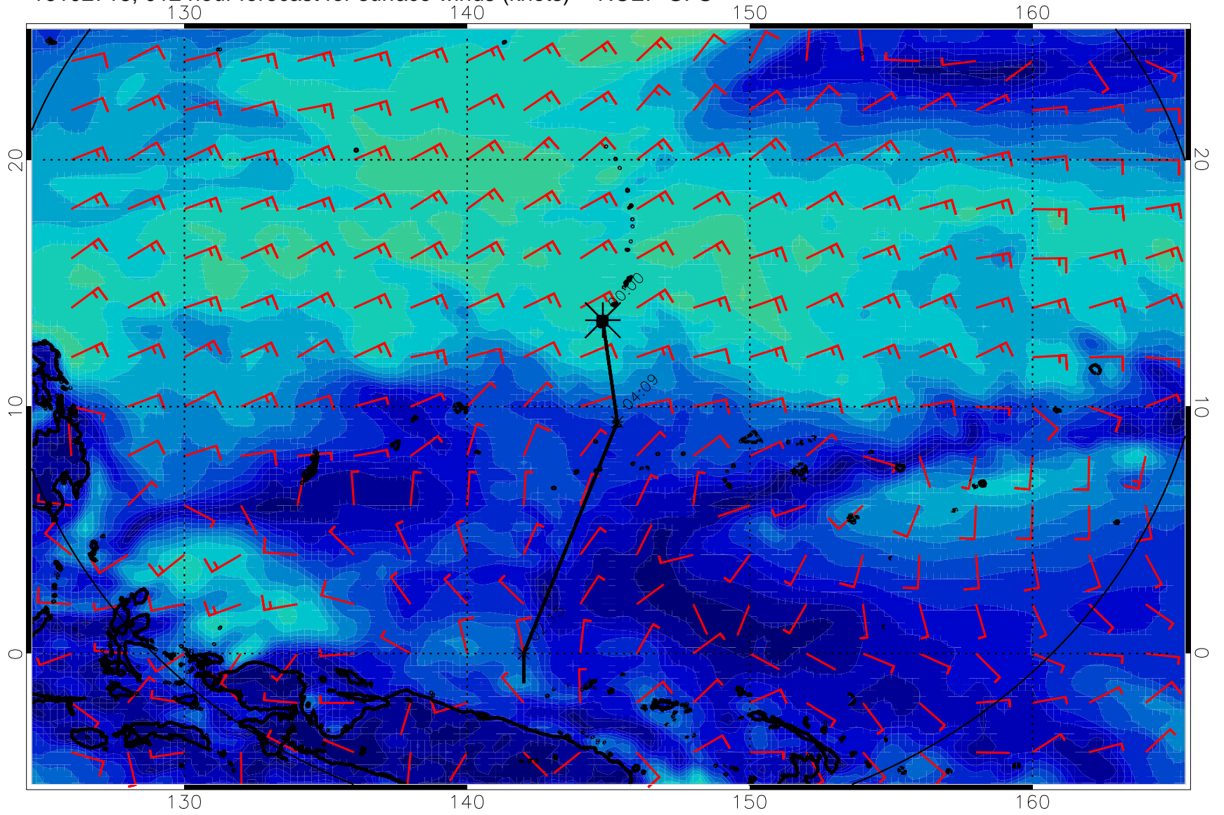
16102718, 012 hour forecast for surface winds (knots) -- NCEP GFS
