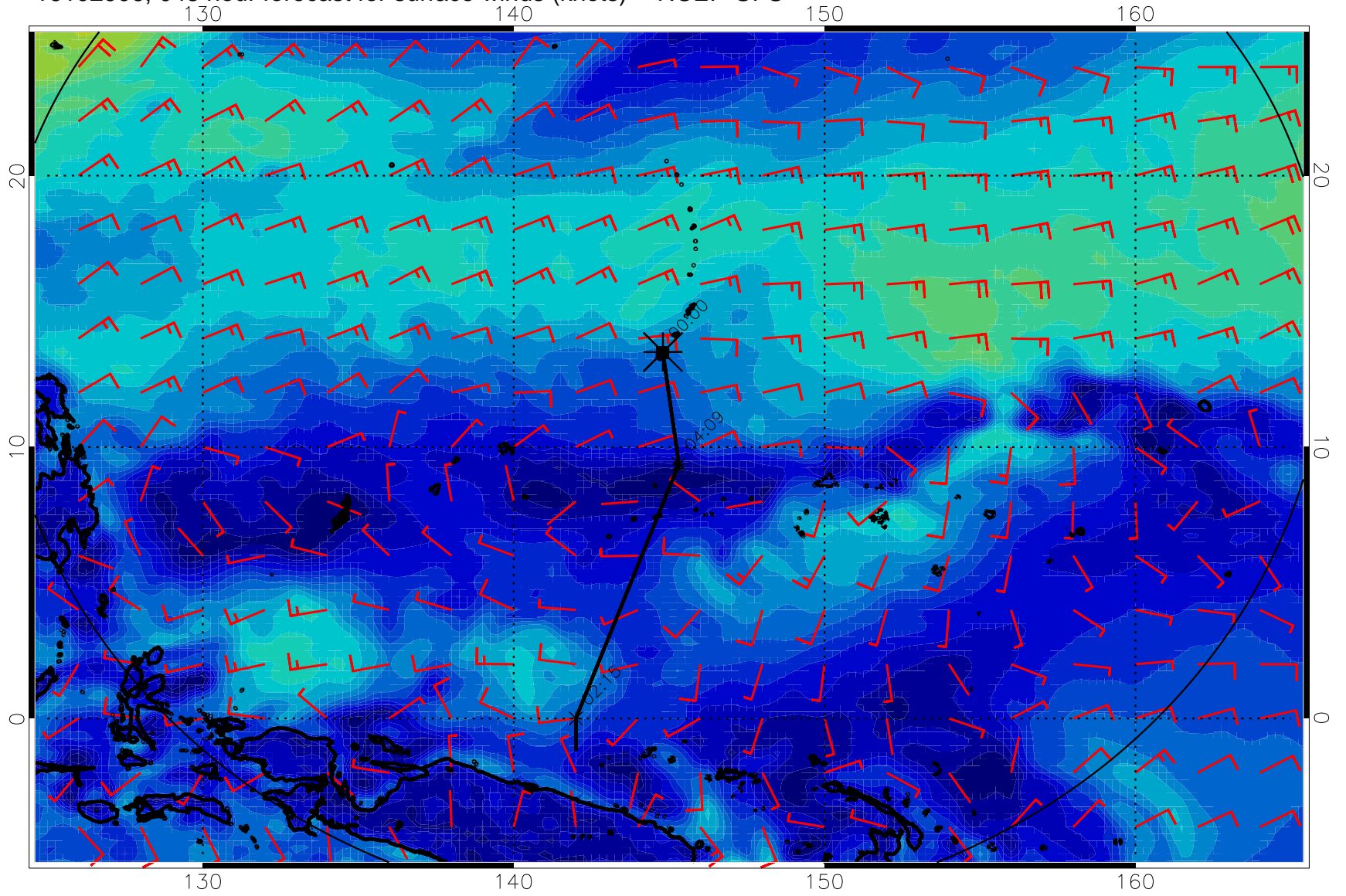
16102906, 048 hour forecast for surface winds (knots) -- NCEP GFS
