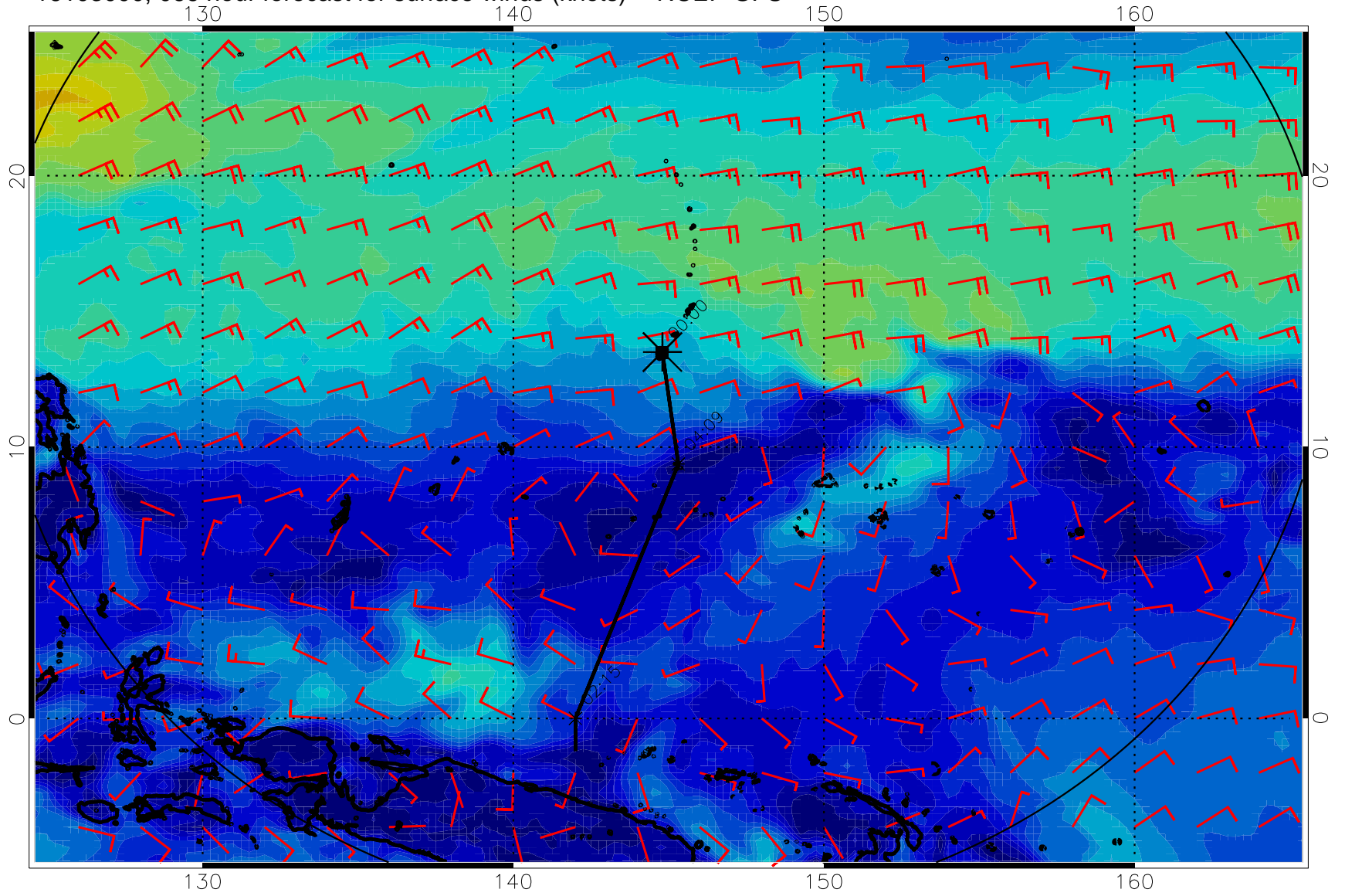
16103000, 066 hour forecast for surface winds (knots) -- NCEP GFS
