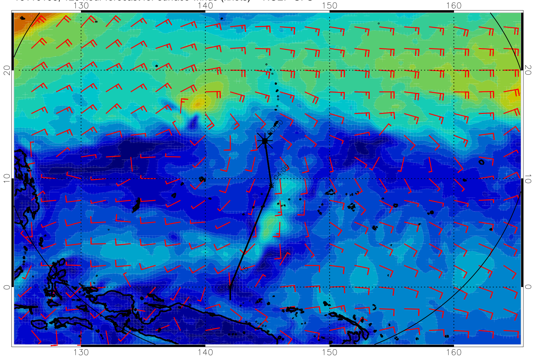
16110106, 120 hour forecast for surface winds (knots) -- NCEP GFS
