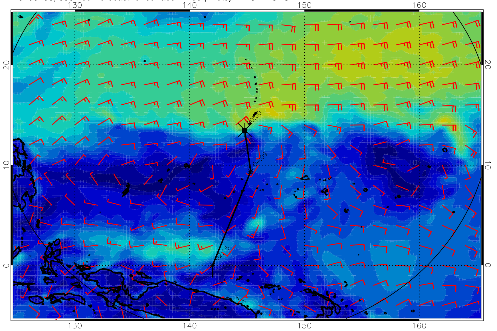
16103106, 096 hour forecast for surface winds (knots) -- NCEP GFS
