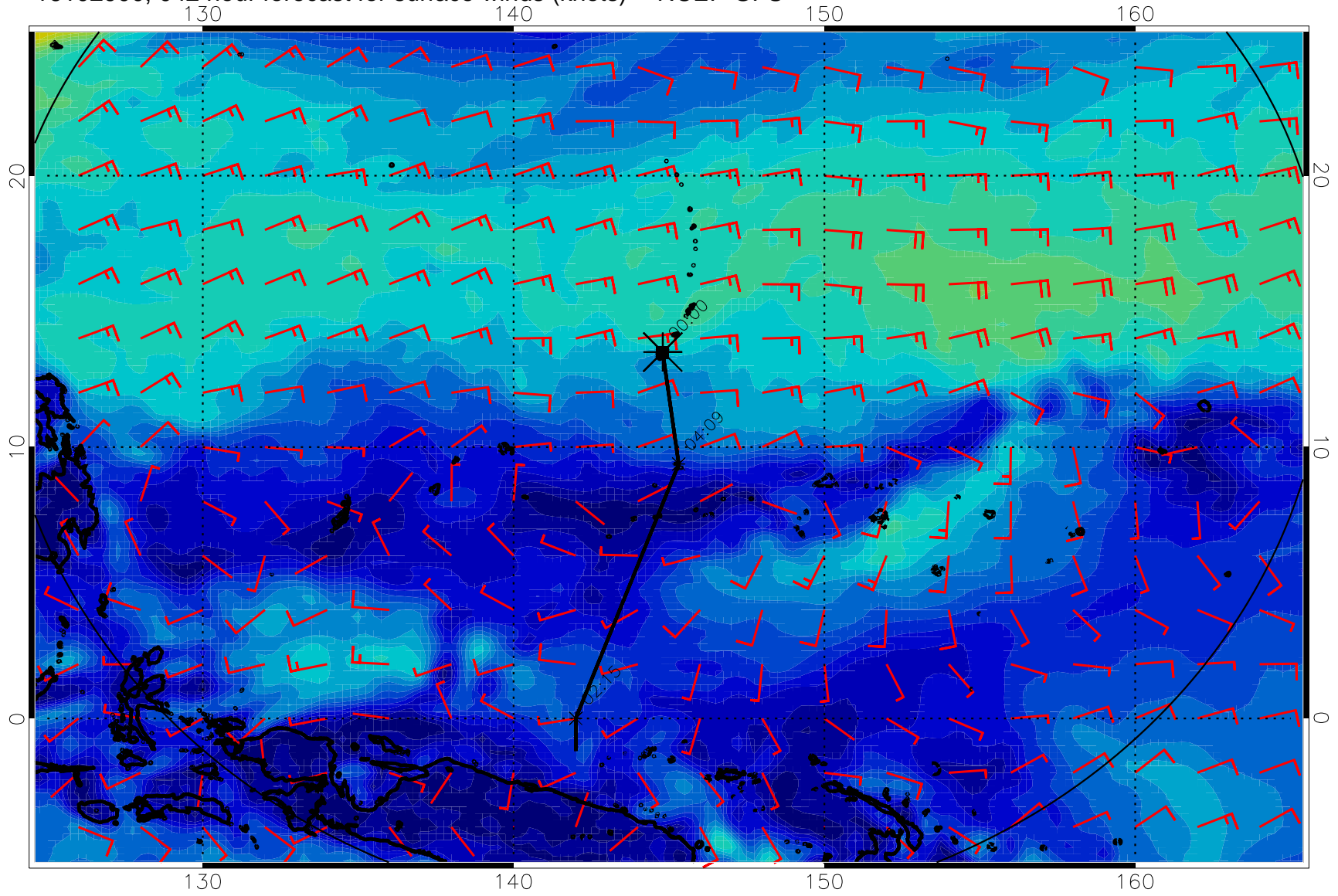
16102900, 042 hour forecast for surface winds (knots) -- NCEP GFS
