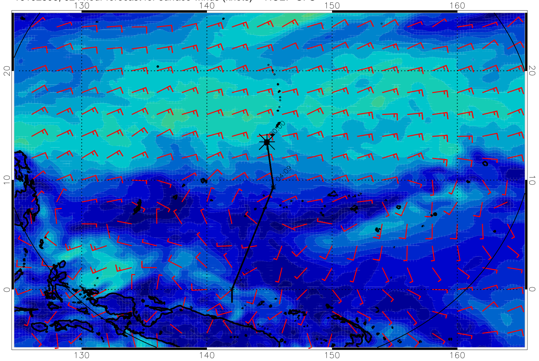
16102806, 024 hour forecast for surface winds (knots) -- NCEP GFS
