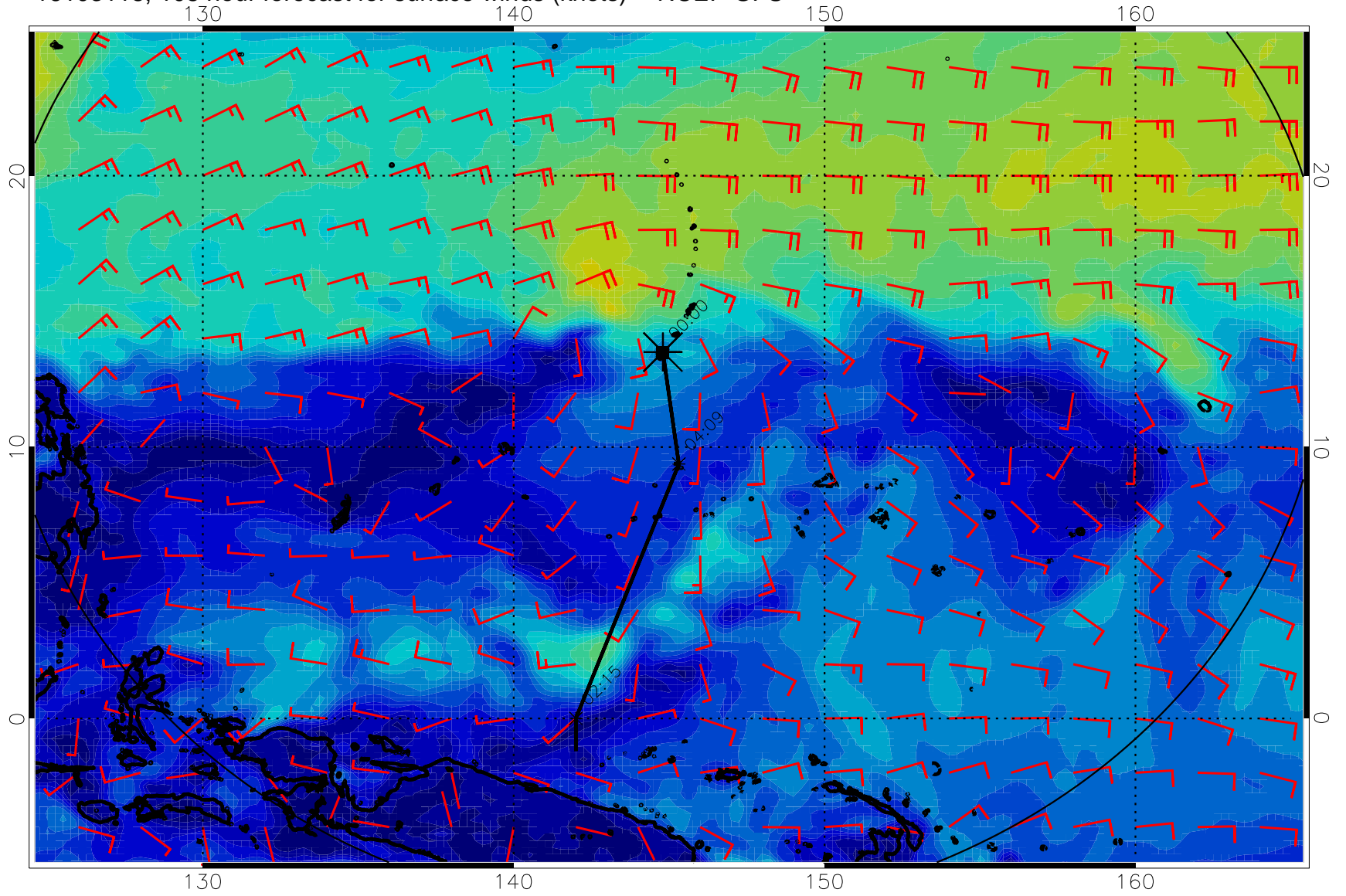
16103118, 108 hour forecast for surface winds (knots) -- NCEP GFS
