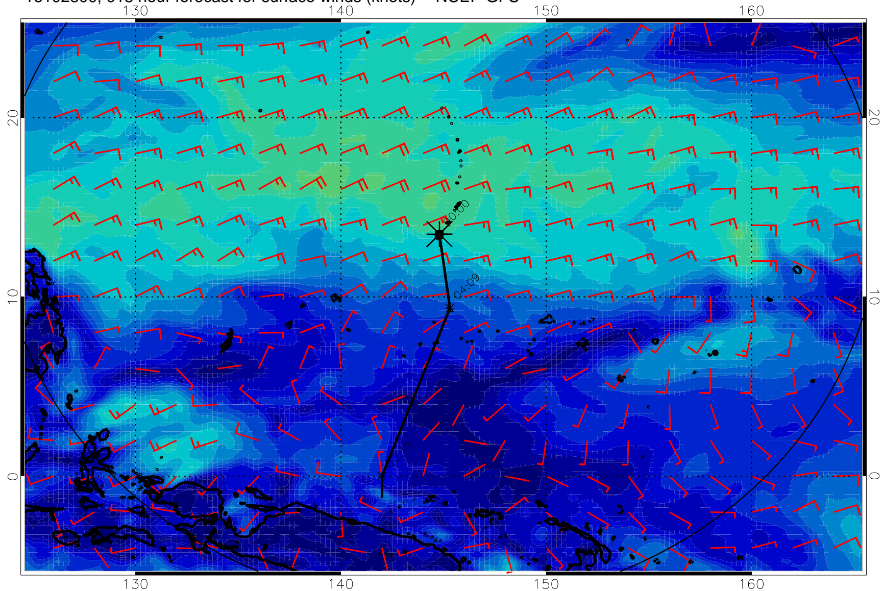
16102800, 018 hour forecast for surface winds (knots) -- NCEP GFS
