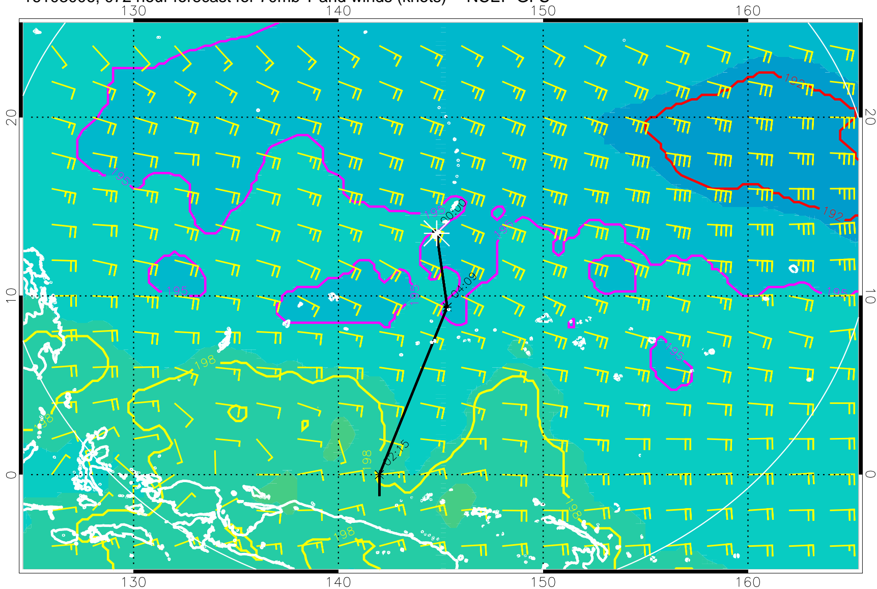
16103006, 072 hour forecast for 70mb T and winds (knots) -- NCEP GFS
