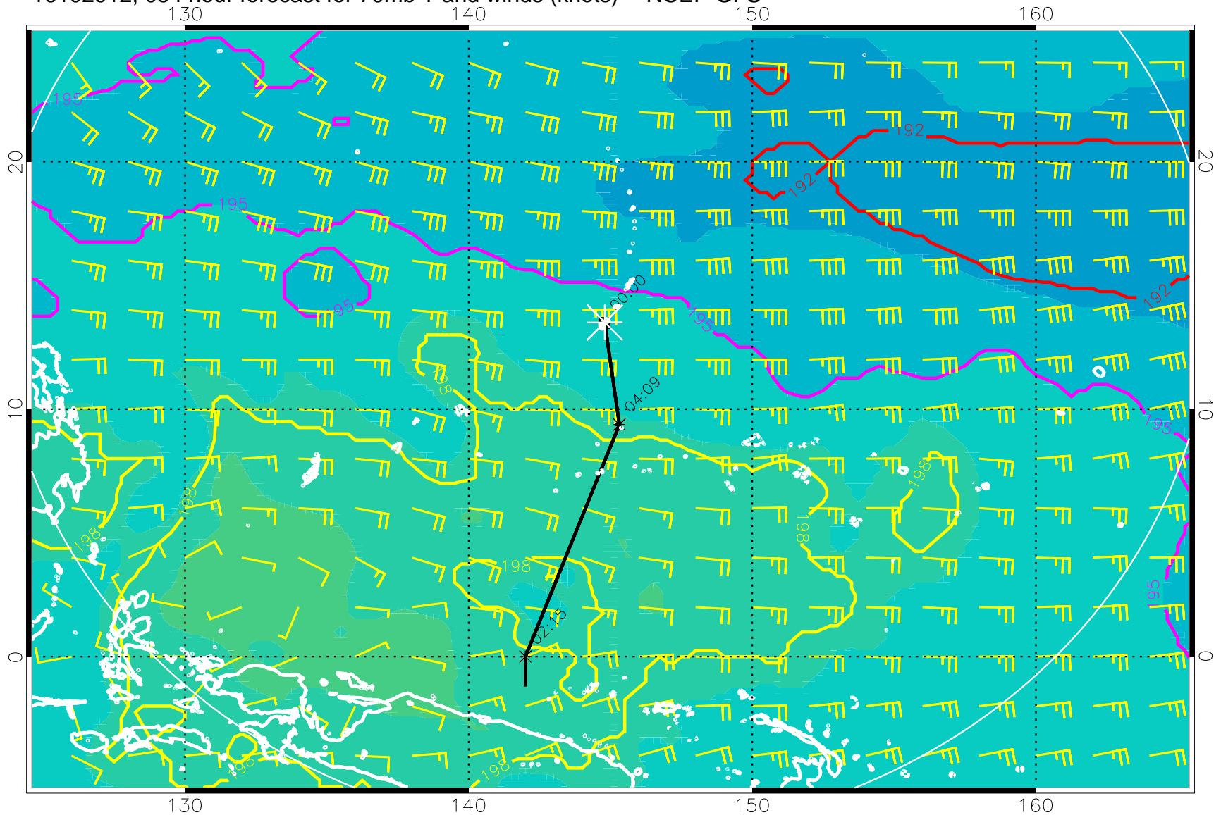
16102912, 054 hour forecast for 70mb T and winds (knots) -- NCEP GFS
