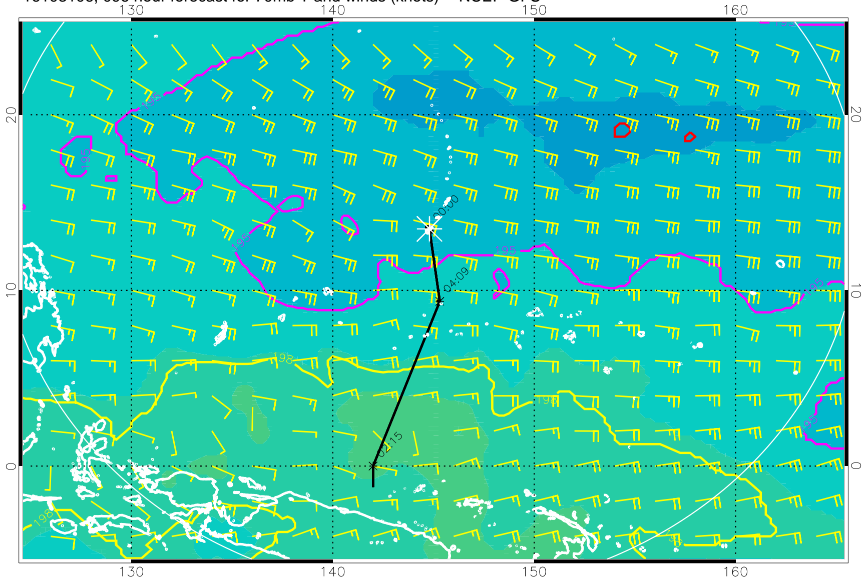
16103106, 096 hour forecast for 70mb T and winds (knots) -- NCEP GFS
