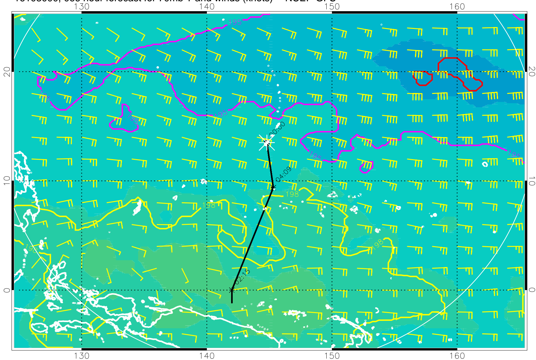
16103000, 066 hour forecast for 70mb T and winds (knots) -- NCEP GFS
