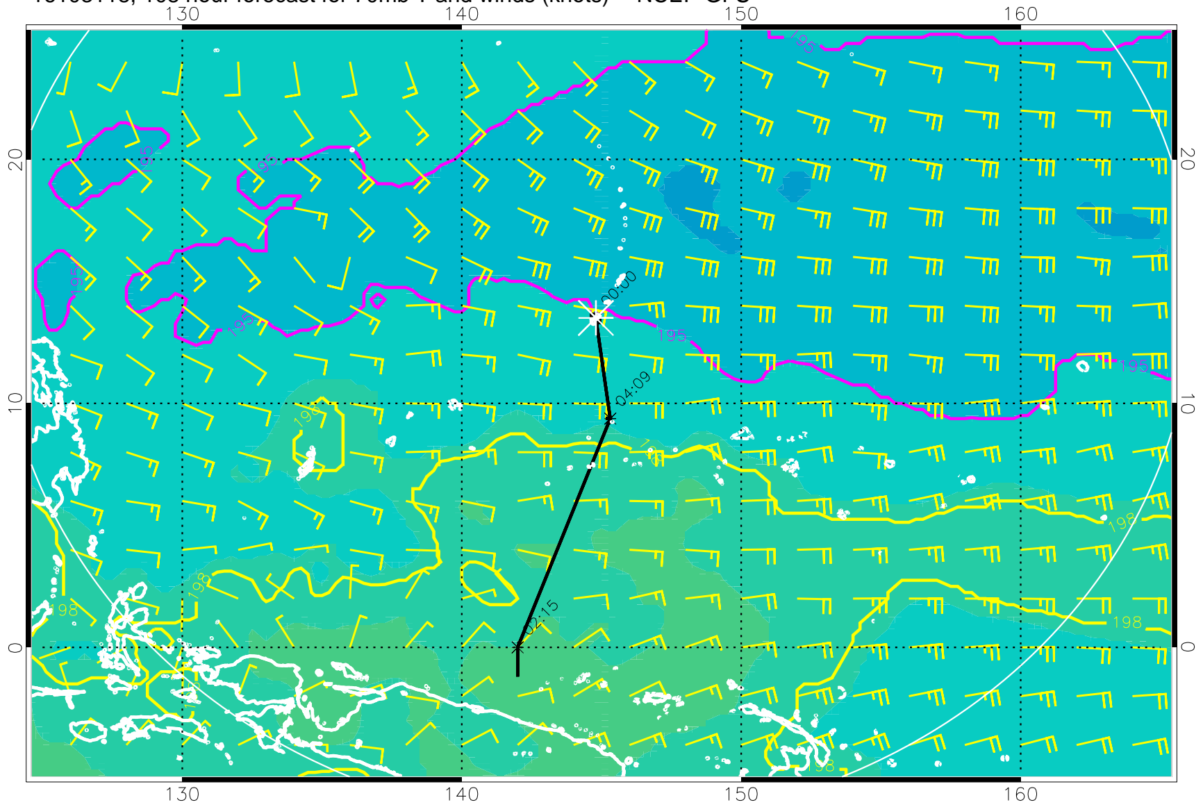
16103118, 108 hour forecast for 70mb T and winds (knots) -- NCEP GFS
