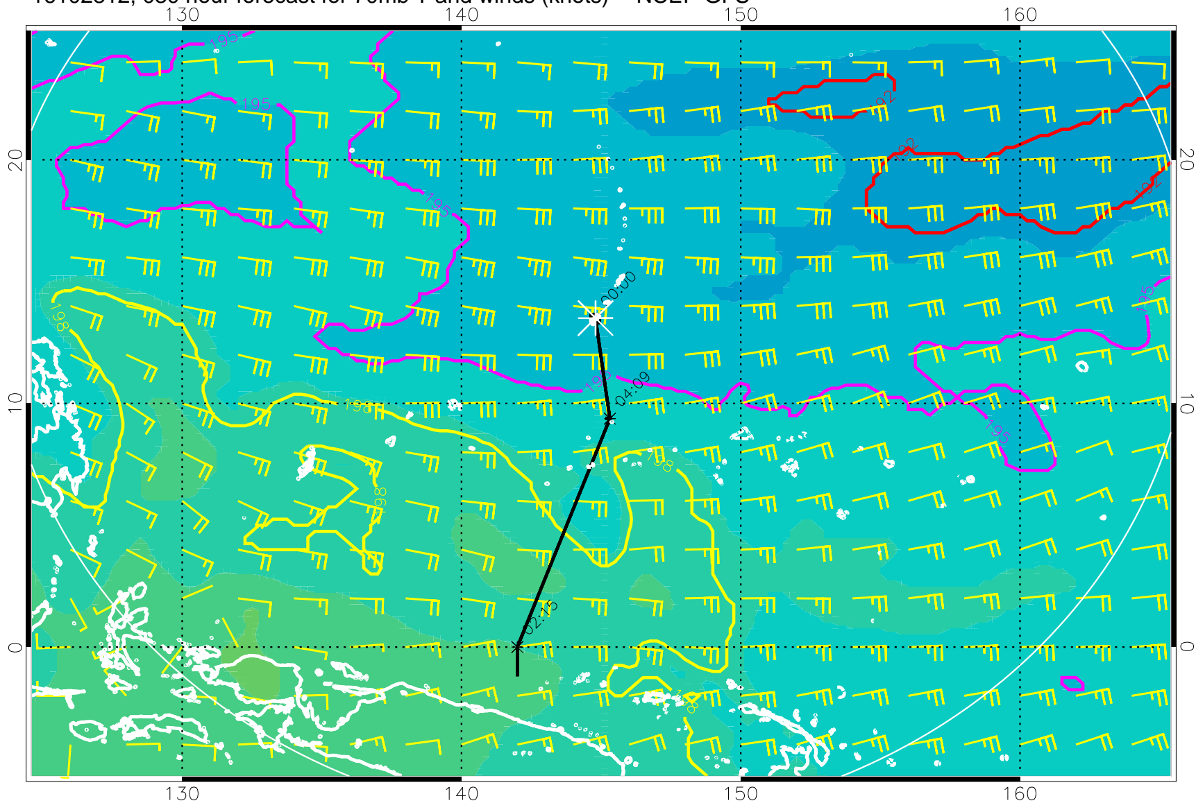
16102812, 030 hour forecast for 70mb T and winds (knots) -- NCEP GFS
