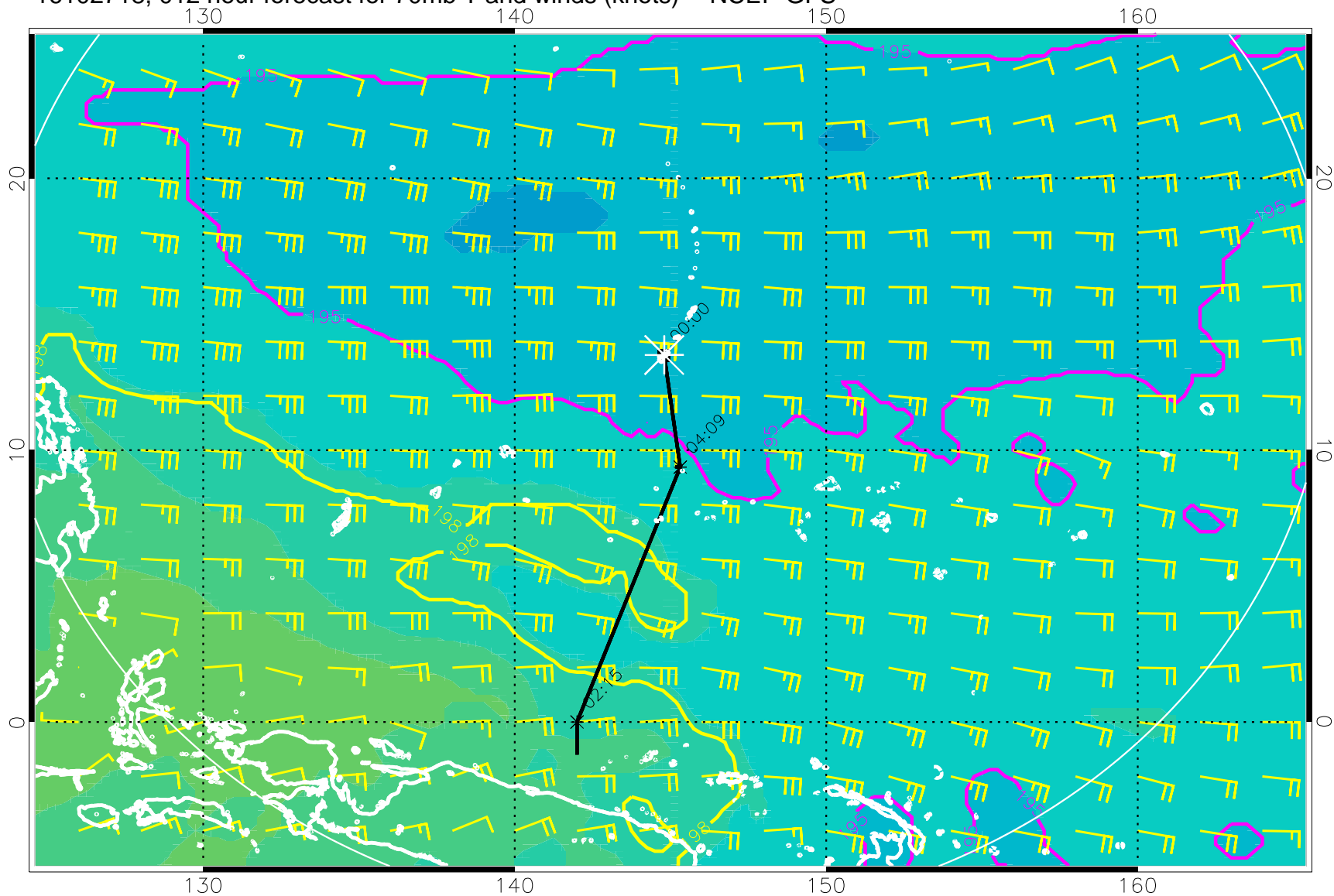
16102718, 012 hour forecast for 70mb T and winds (knots) -- NCEP GFS
