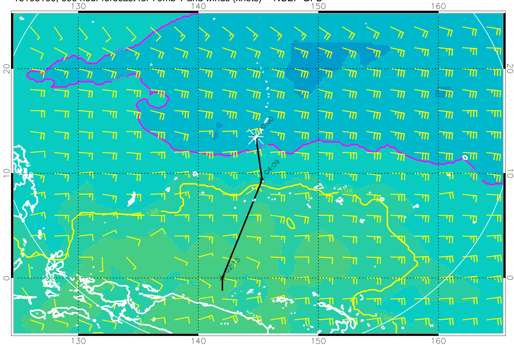
16103100, 090 hour forecast for 70mb T and winds (knots) -- NCEP GFS
