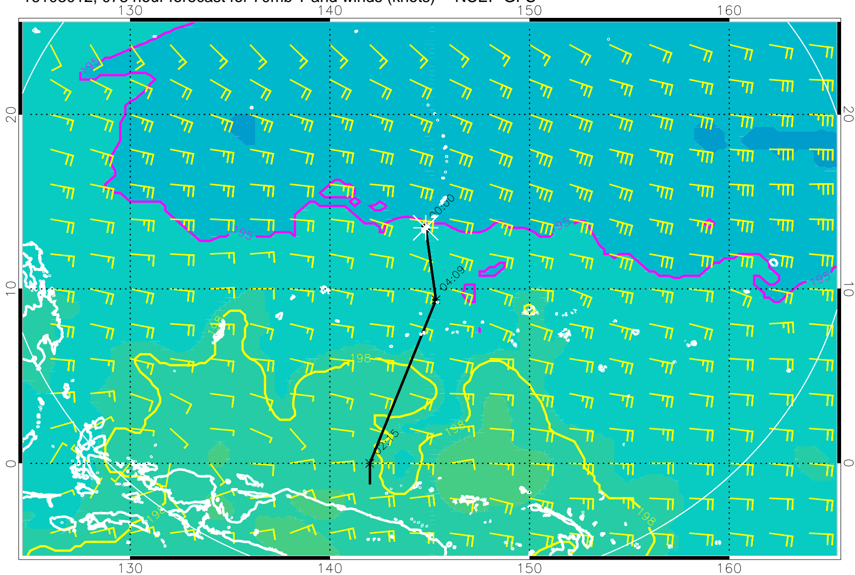
16103012, 078 hour forecast for 70mb T and winds (knots) -- NCEP GFS
