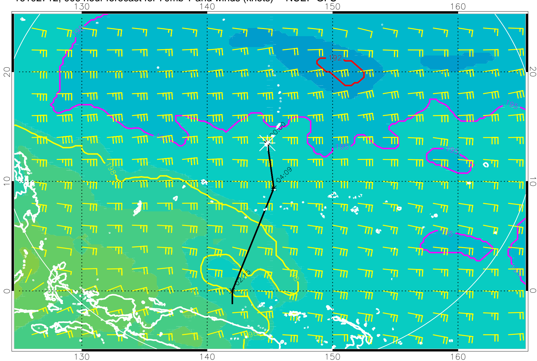
16102712, 006 hour forecast for 70mb T and winds (knots) -- NCEP GFS
