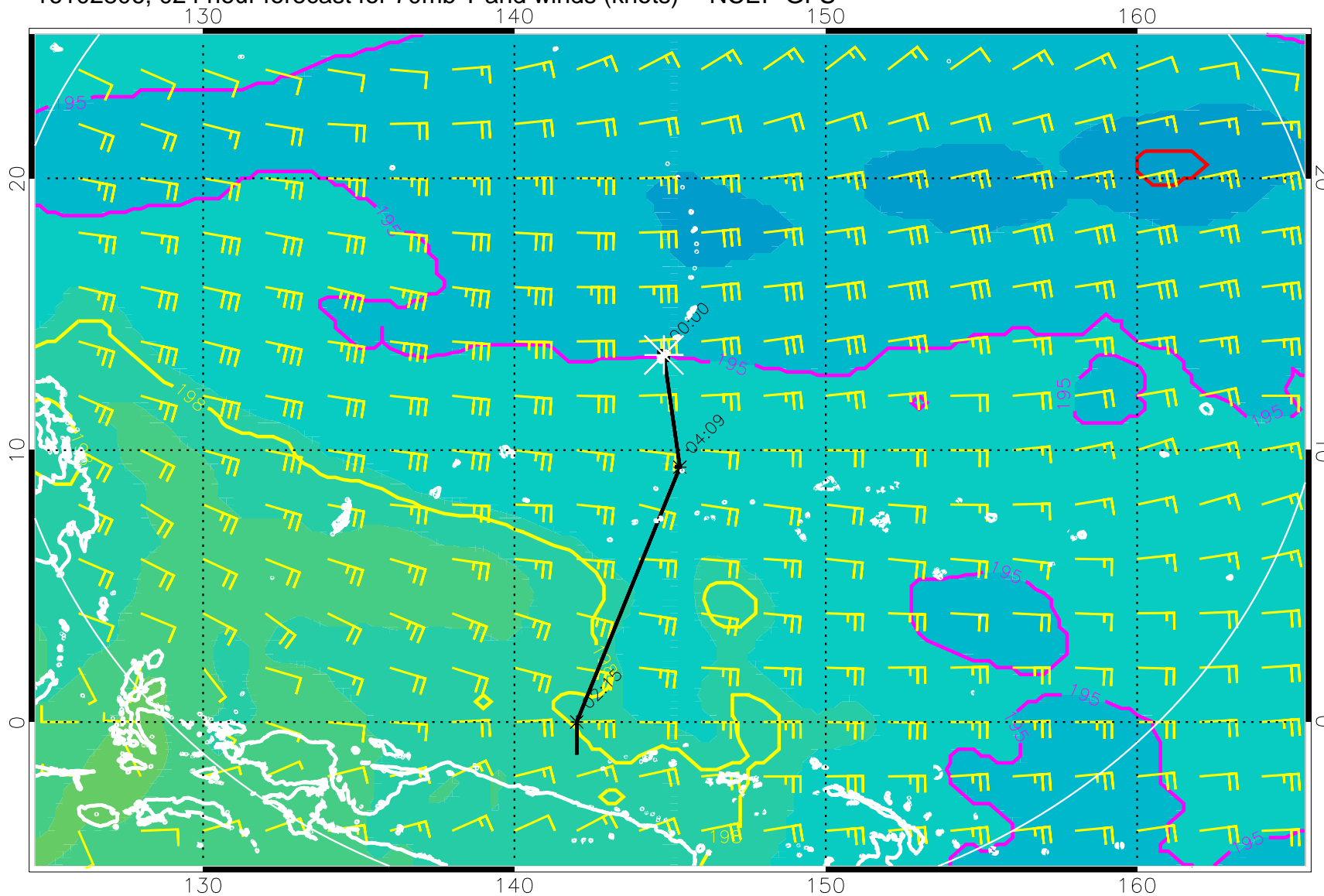
16102806, 024 hour forecast for 70mb T and winds (knots) -- NCEP GFS
