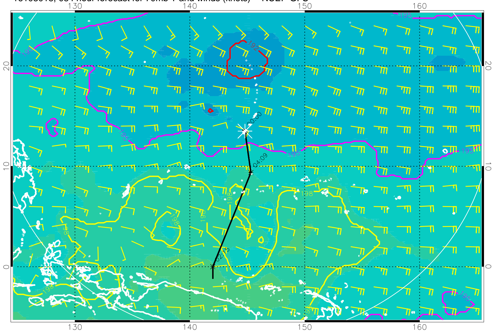
16103018, 084 hour forecast for 70mb T and winds (knots) -- NCEP GFS
