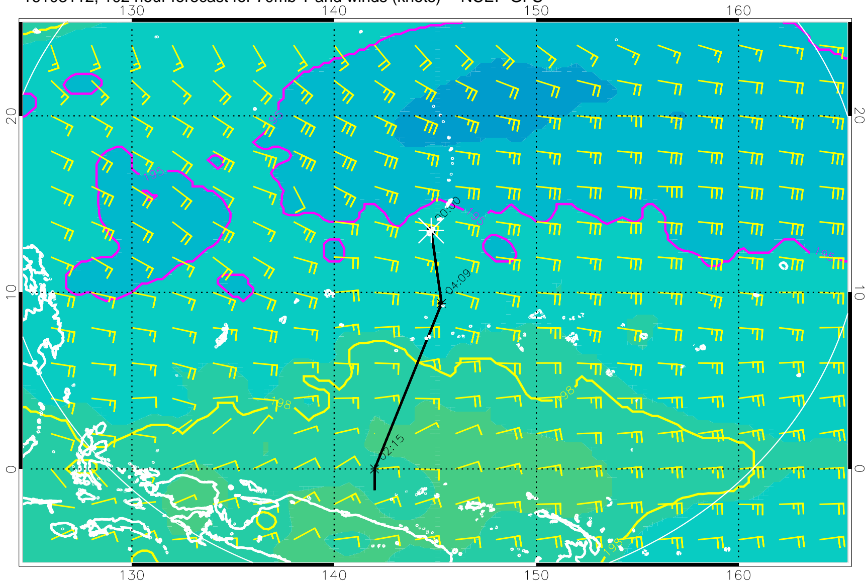
16103112, 102 hour forecast for 70mb T and winds (knots) -- NCEP GFS
