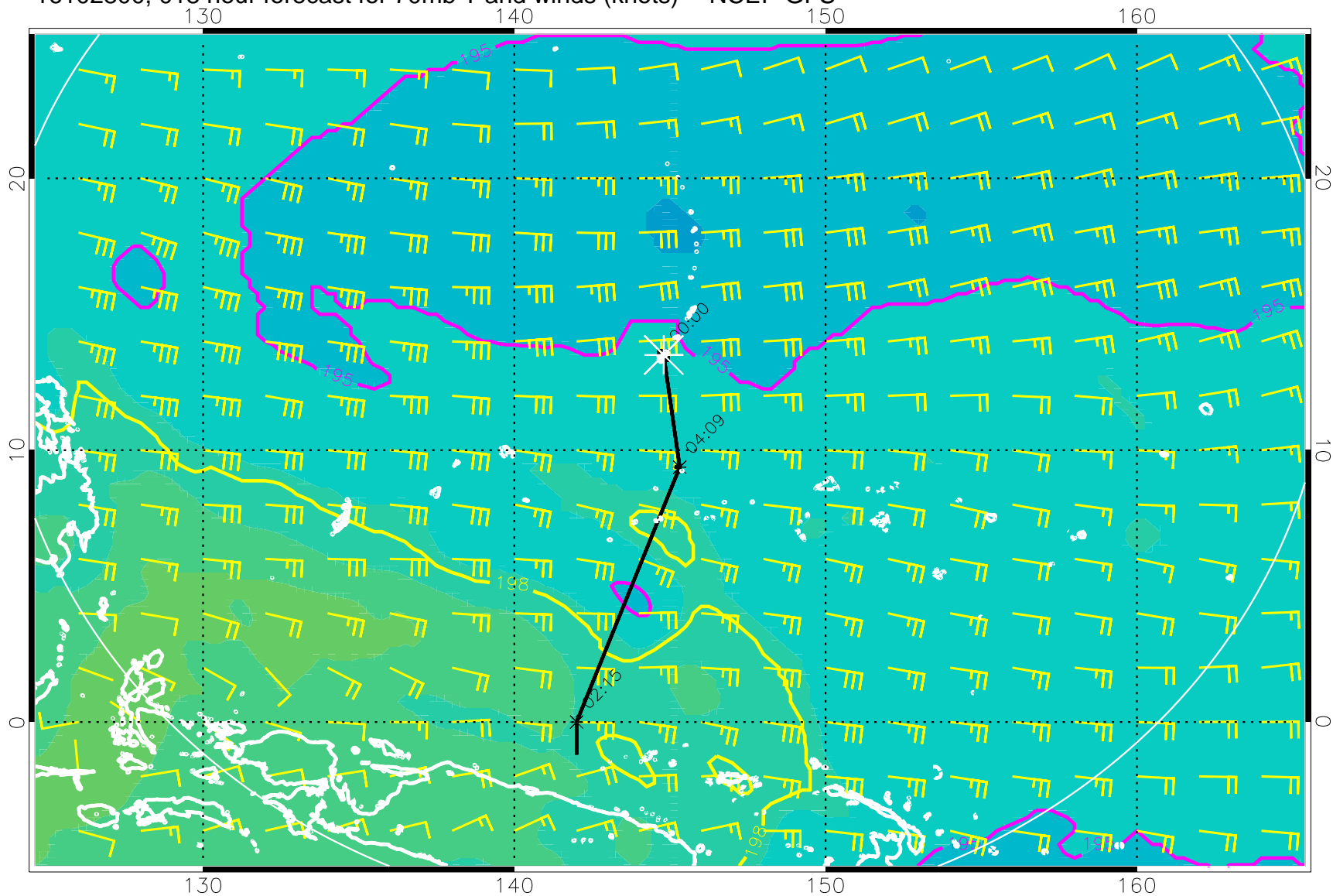
16102800, 018 hour forecast for 70mb T and winds (knots) -- NCEP GFS
