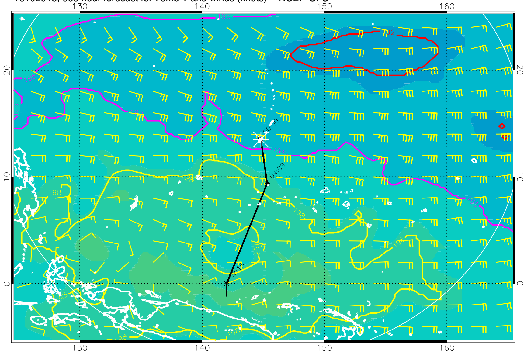
16102918, 060 hour forecast for 70mb T and winds (knots) -- NCEP GFS
