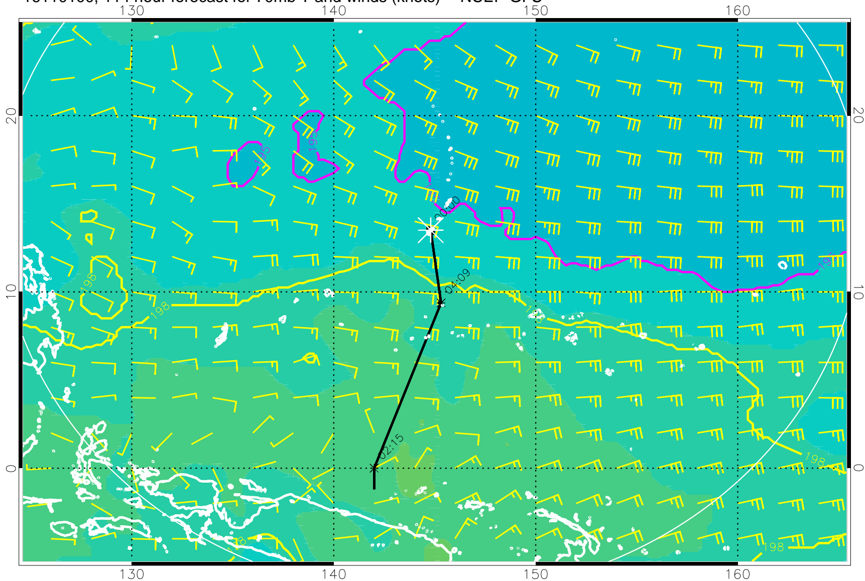
16110100, 114 hour forecast for 70mb T and winds (knots) -- NCEP GFS
