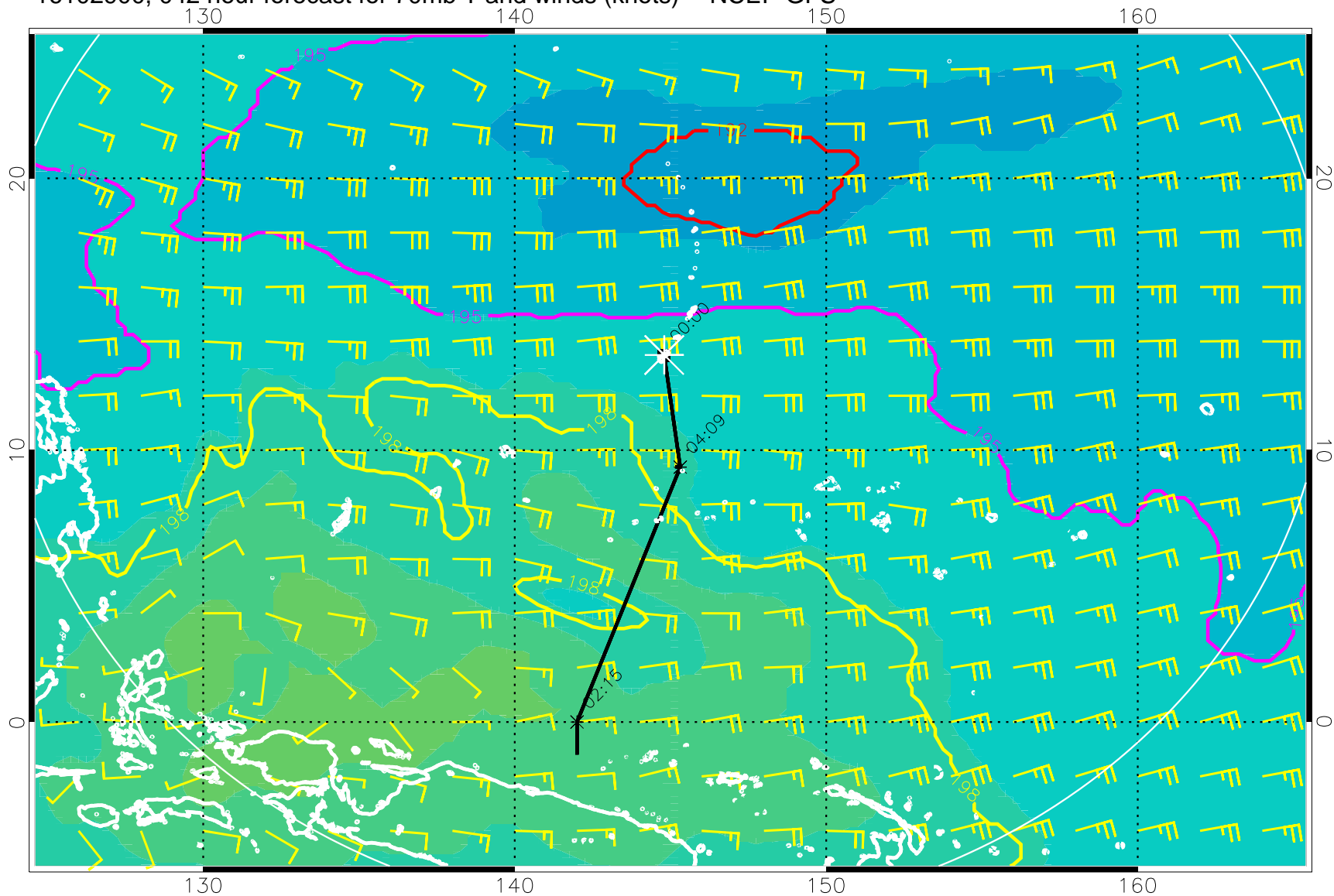
16102900, 042 hour forecast for 70mb T and winds (knots) -- NCEP GFS
