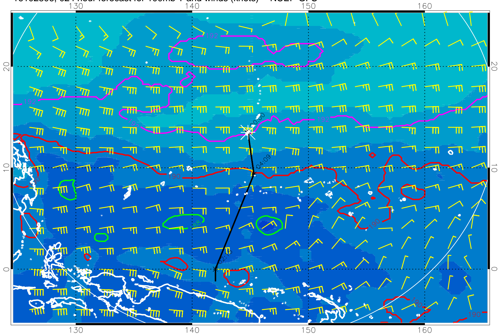
16102806, 024 hour forecast for 100mb T and winds (knots) -- NCEP GFS
