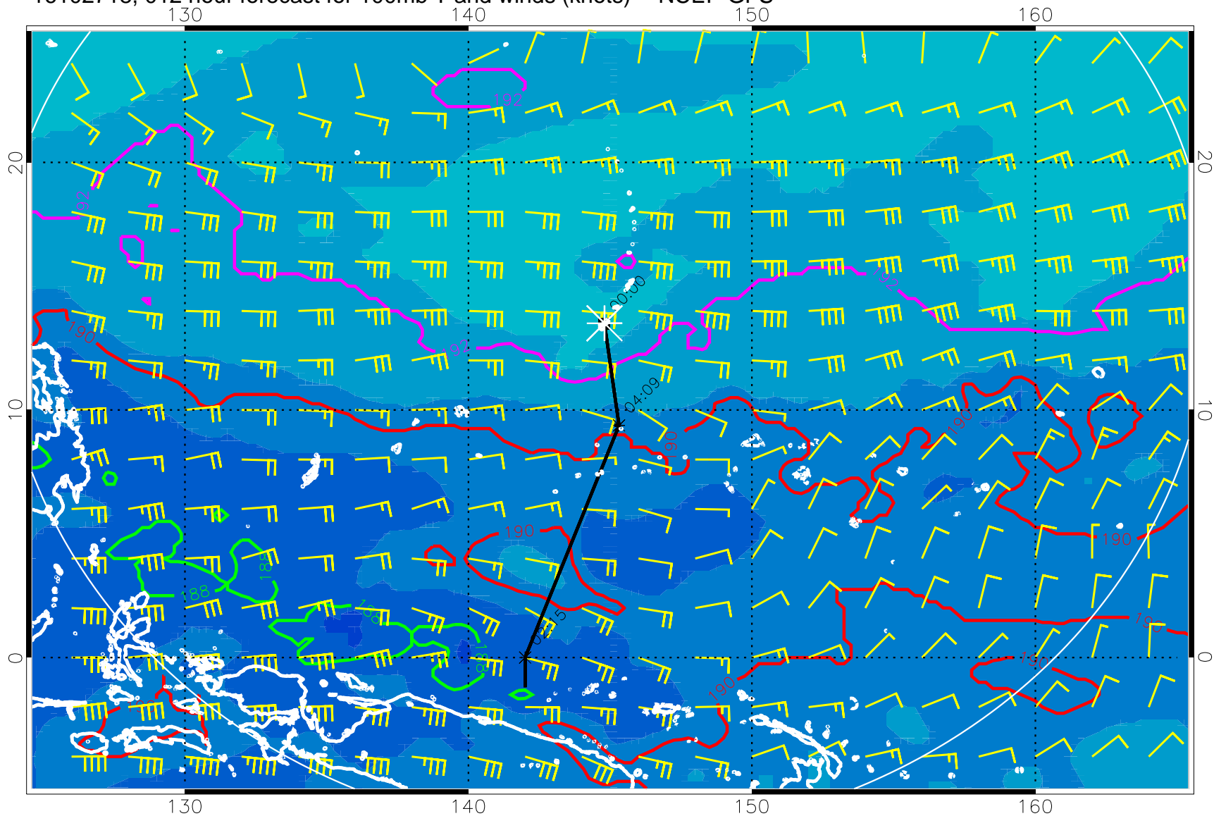
16102718, 012 hour forecast for 100mb T and winds (knots) -- NCEP GFS
