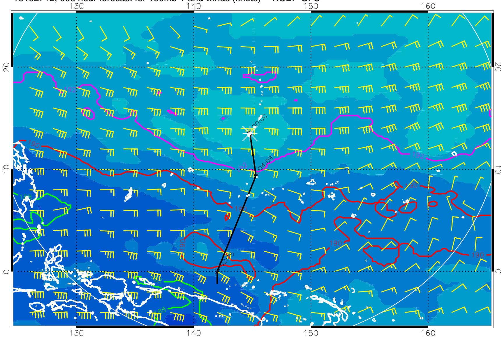
16102712, 006 hour forecast for 100mb T and winds (knots) -- NCEP GFS
