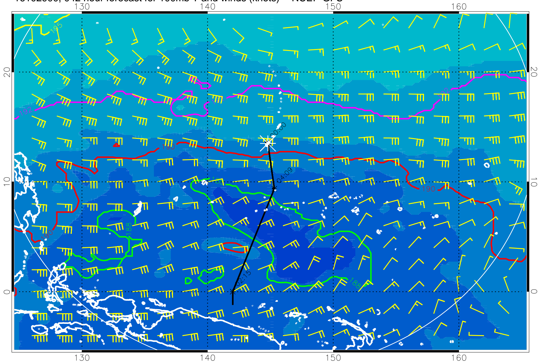
16102900, 042 hour forecast for 100mb T and winds (knots) -- NCEP GFS
