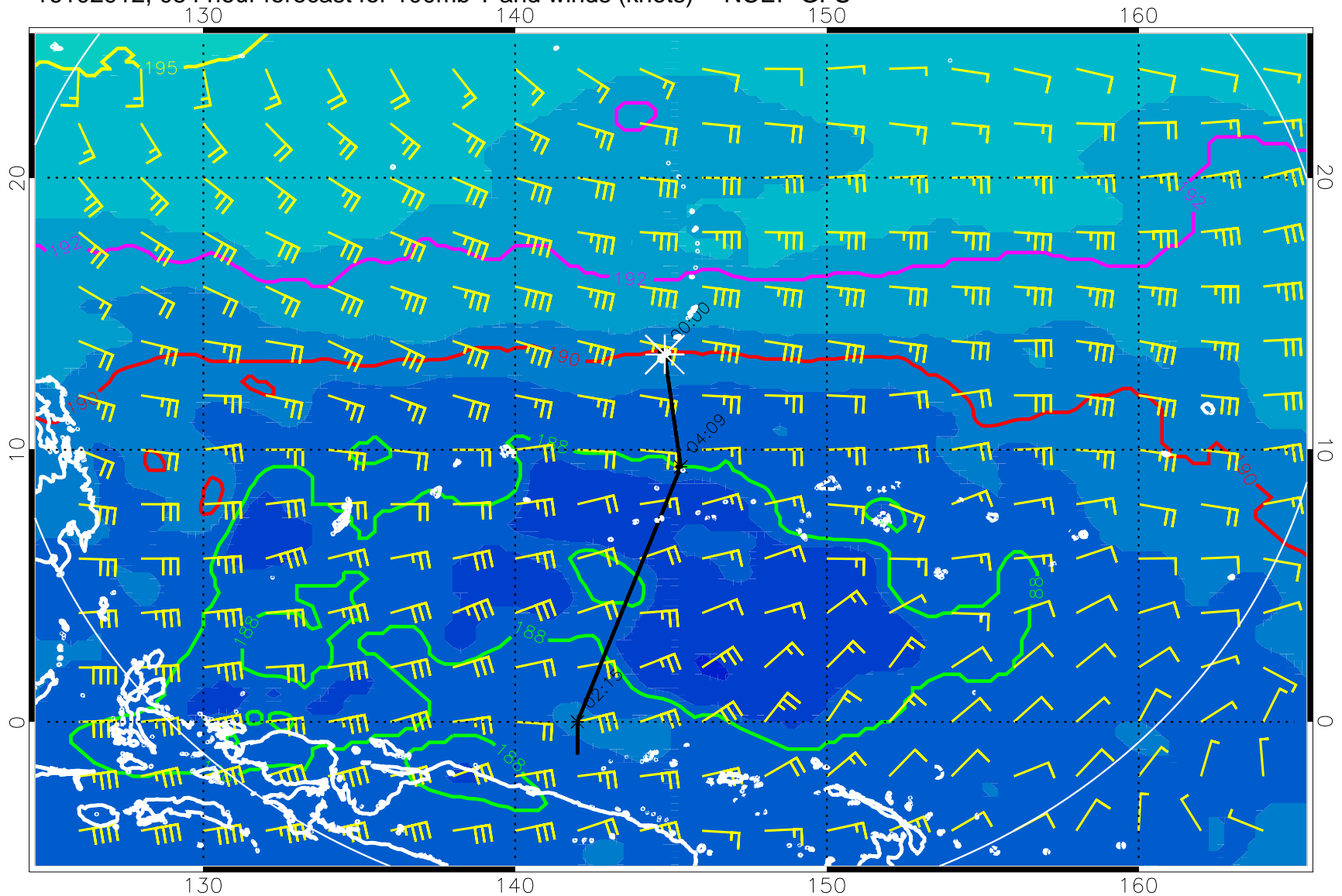
16102912, 054 hour forecast for 100mb T and winds (knots) -- NCEP GFS
