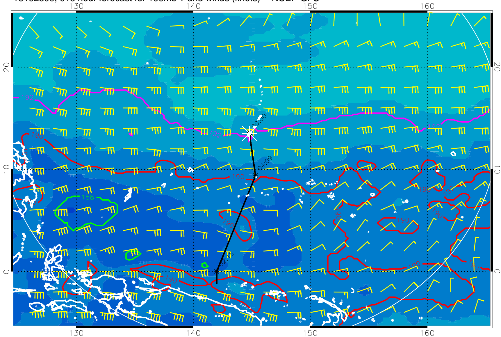
16102800, 018 hour forecast for 100mb T and winds (knots) -- NCEP GFS
