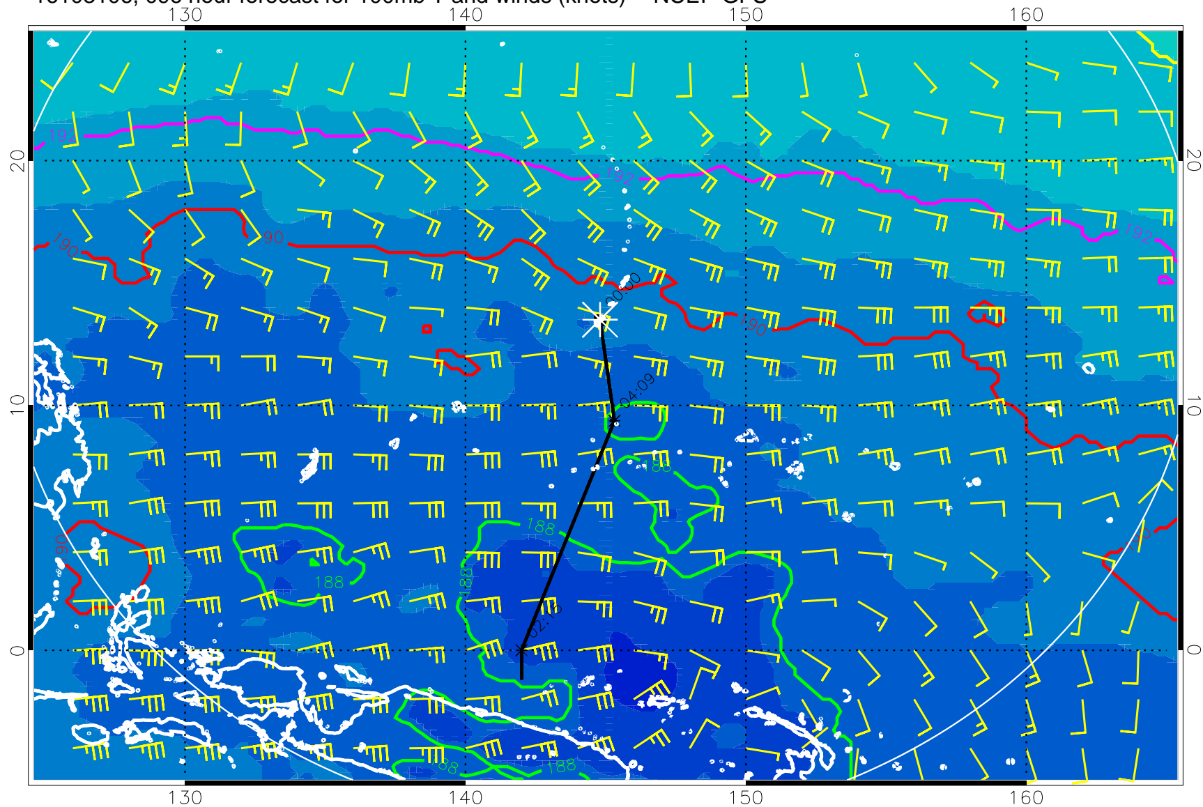
16103106, 096 hour forecast for 100mb T and winds (knots) -- NCEP GFS
