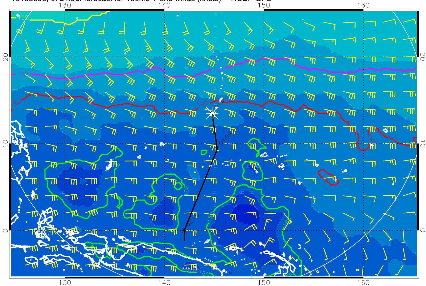
16103006, 072 hour forecast for 100mb T and winds (knots) -- NCEP GFS
