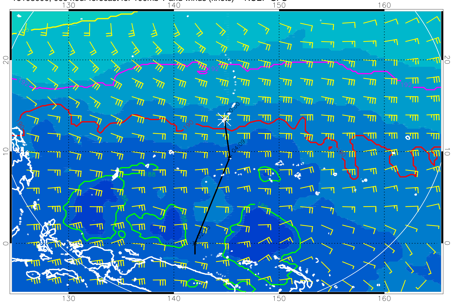
16103000, 066 hour forecast for 100mb T and winds (knots) -- NCEP GFS
