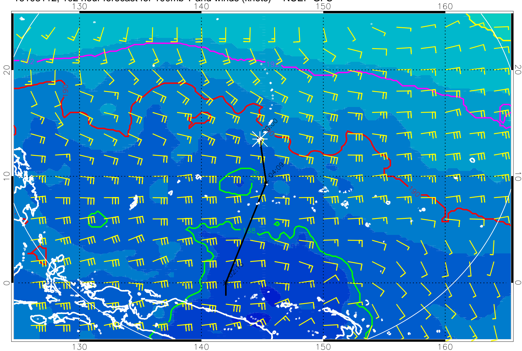
16103112, 102 hour forecast for 100mb T and winds (knots) -- NCEP GFS
