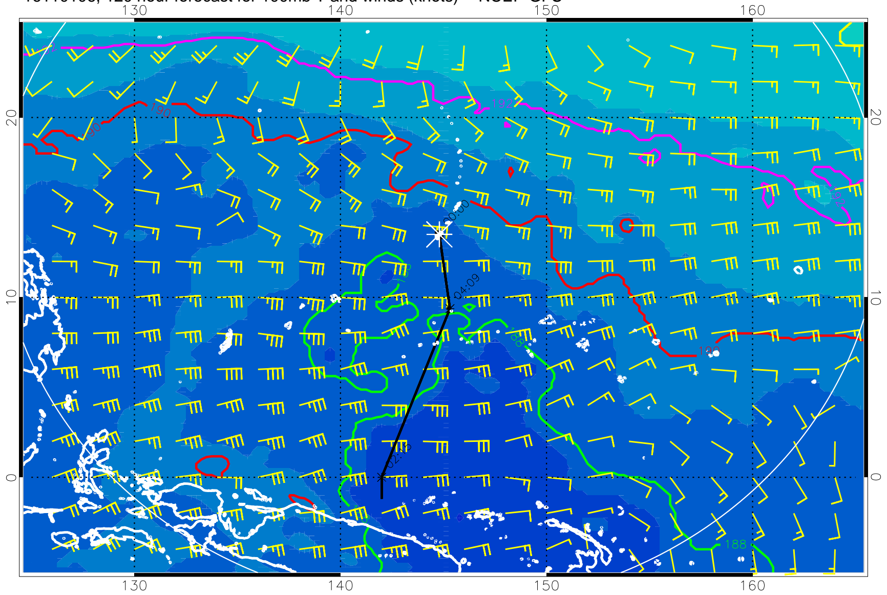
16110106, 120 hour forecast for 100mb T and winds (knots) -- NCEP GFS
