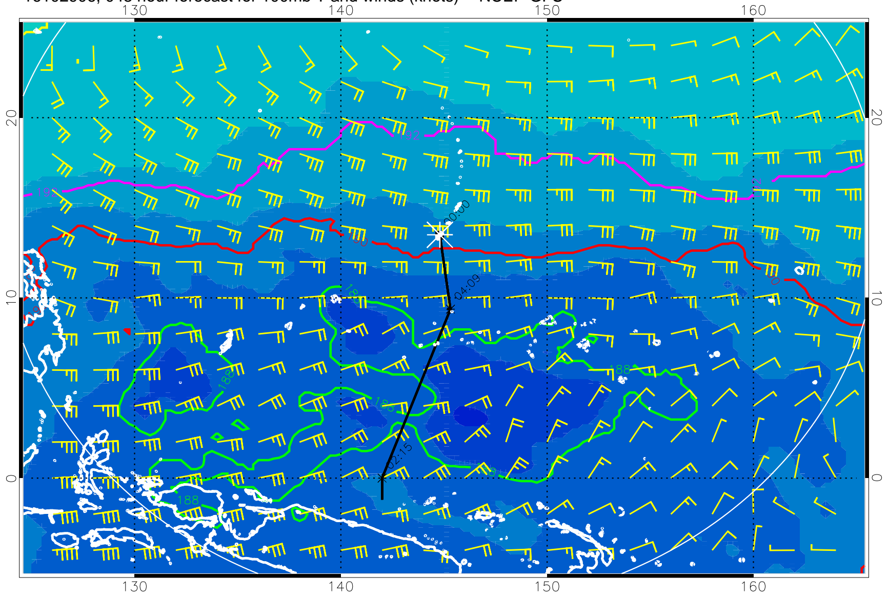
16102906, 048 hour forecast for 100mb T and winds (knots) -- NCEP GFS
