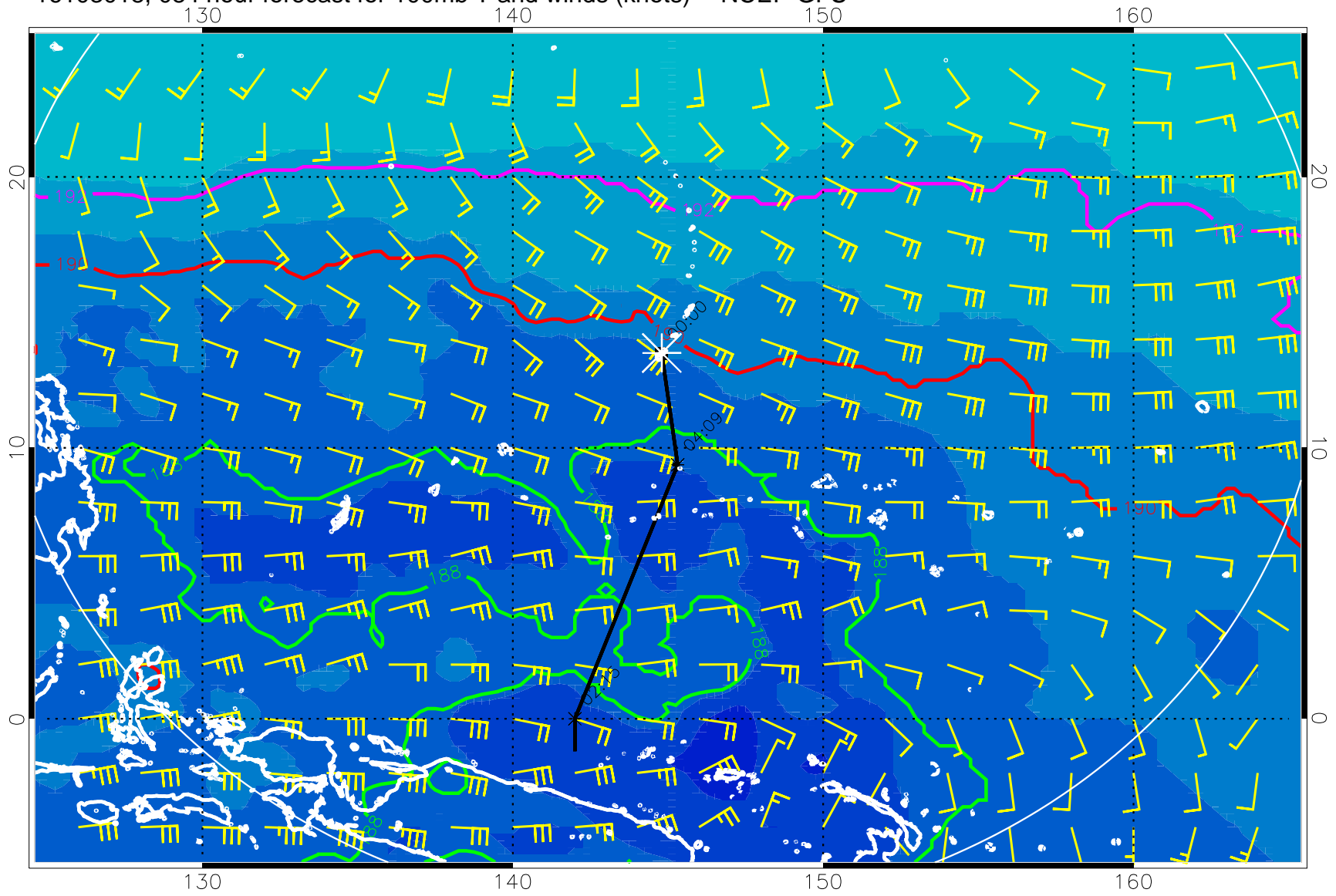
16103018, 084 hour forecast for 100mb T and winds (knots) -- NCEP GFS
