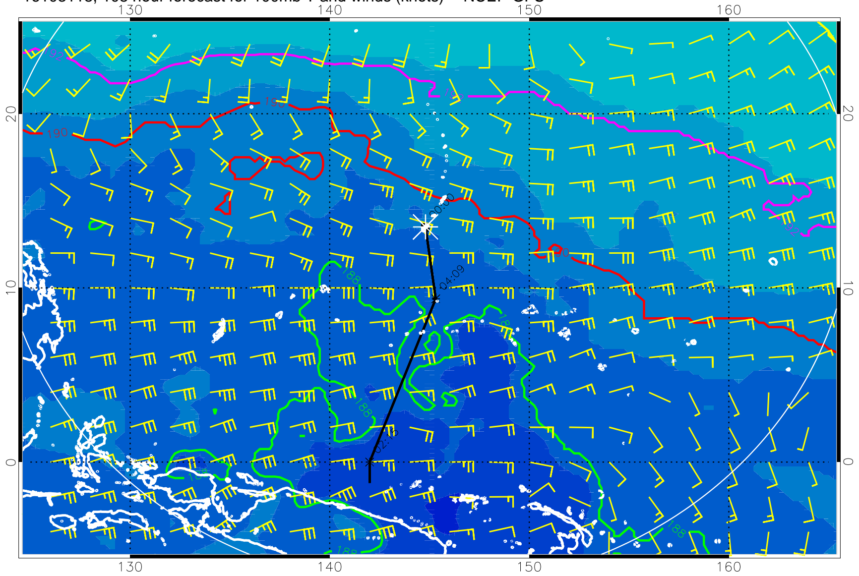
16103118, 108 hour forecast for 100mb T and winds (knots) -- NCEP GFS
