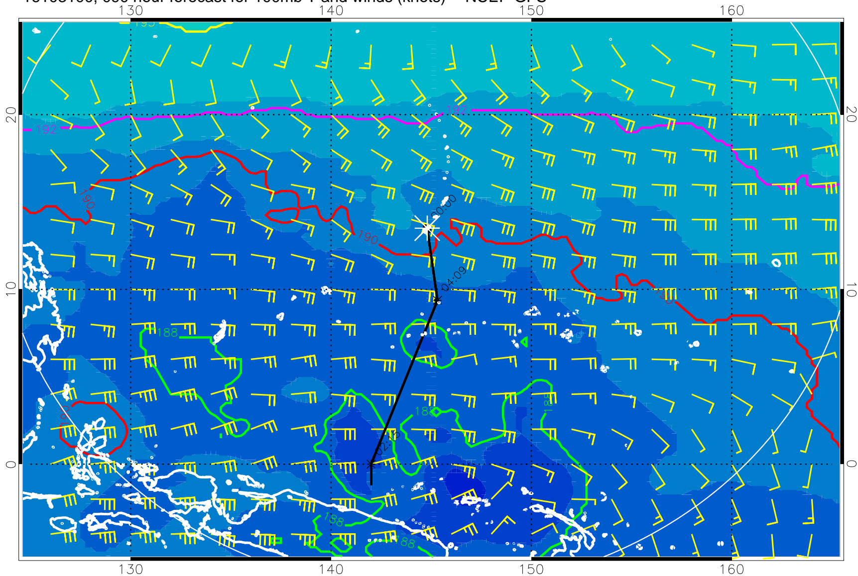
16103100, 090 hour forecast for 100mb T and winds (knots) -- NCEP GFS
