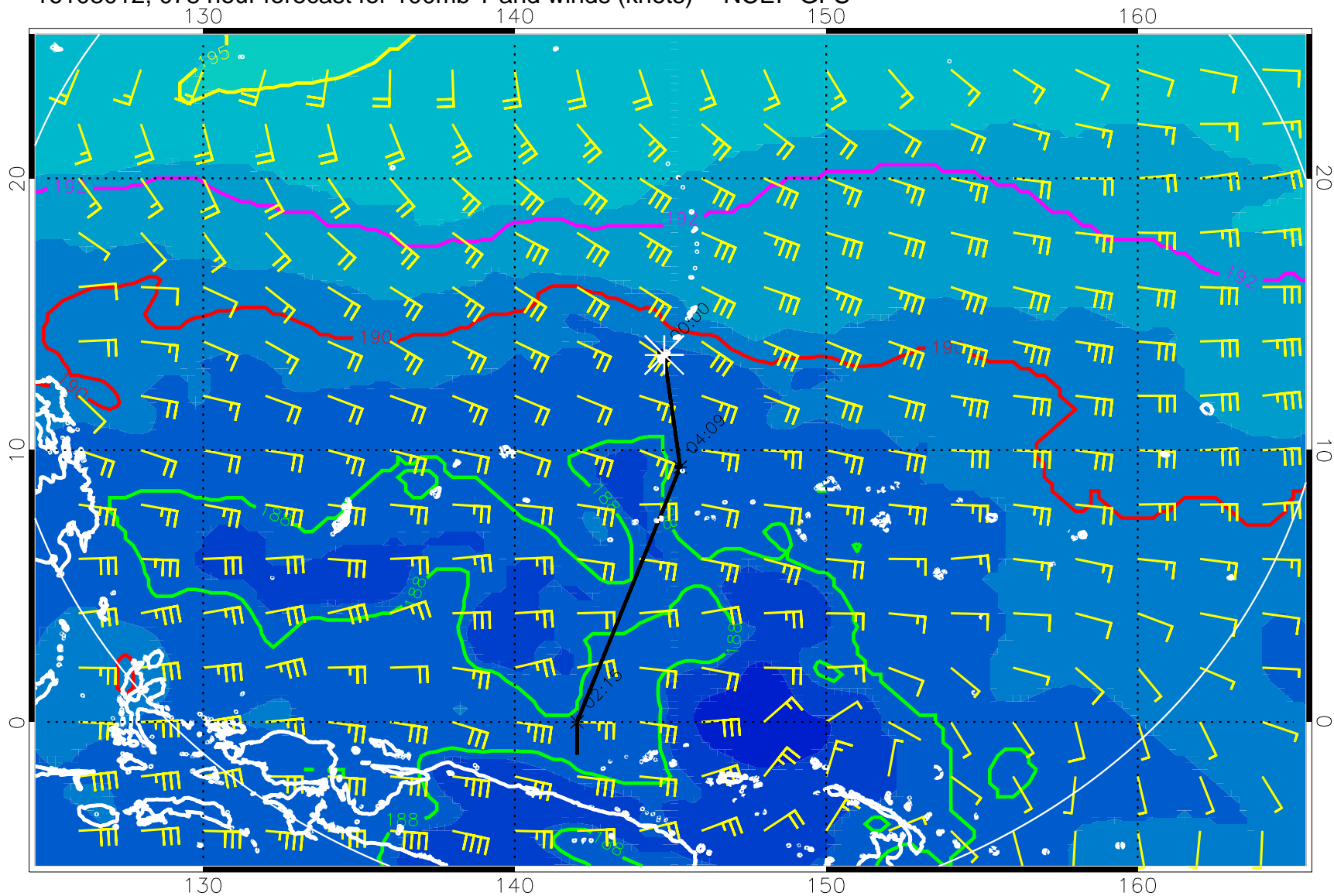
16103012, 078 hour forecast for 100mb T and winds (knots) -- NCEP GFS
