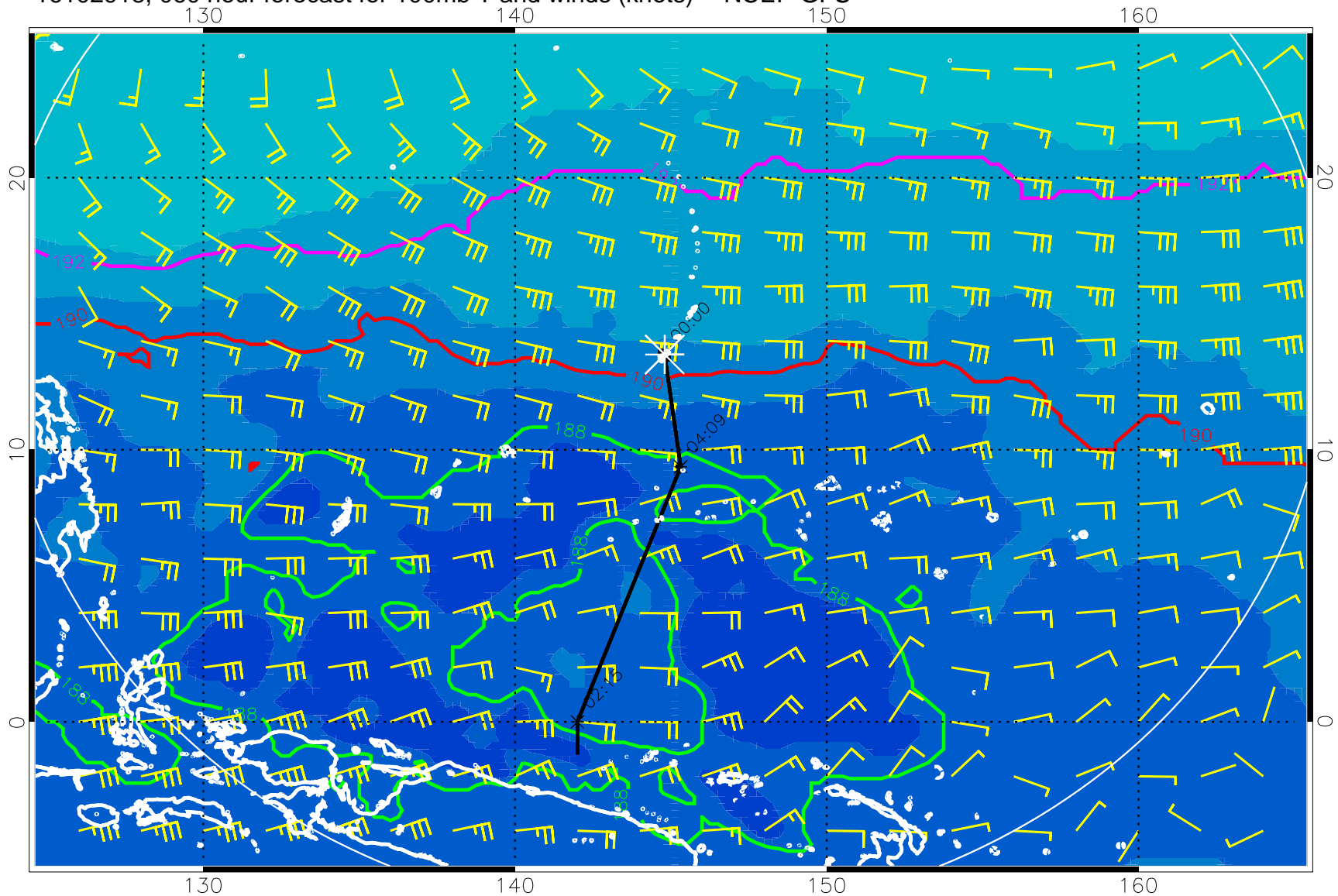
16102918, 060 hour forecast for 100mb T and winds (knots) -- NCEP GFS
