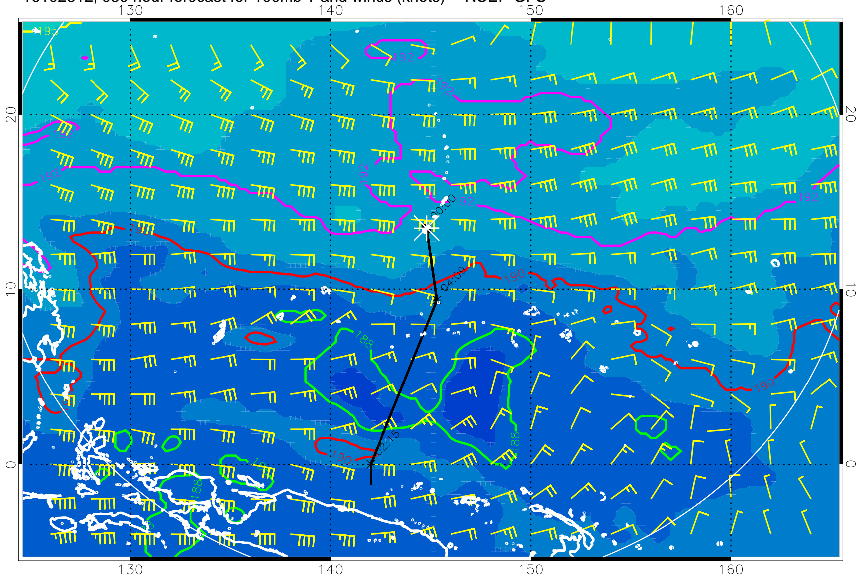
16102812, 030 hour forecast for 100mb T and winds (knots) -- NCEP GFS
