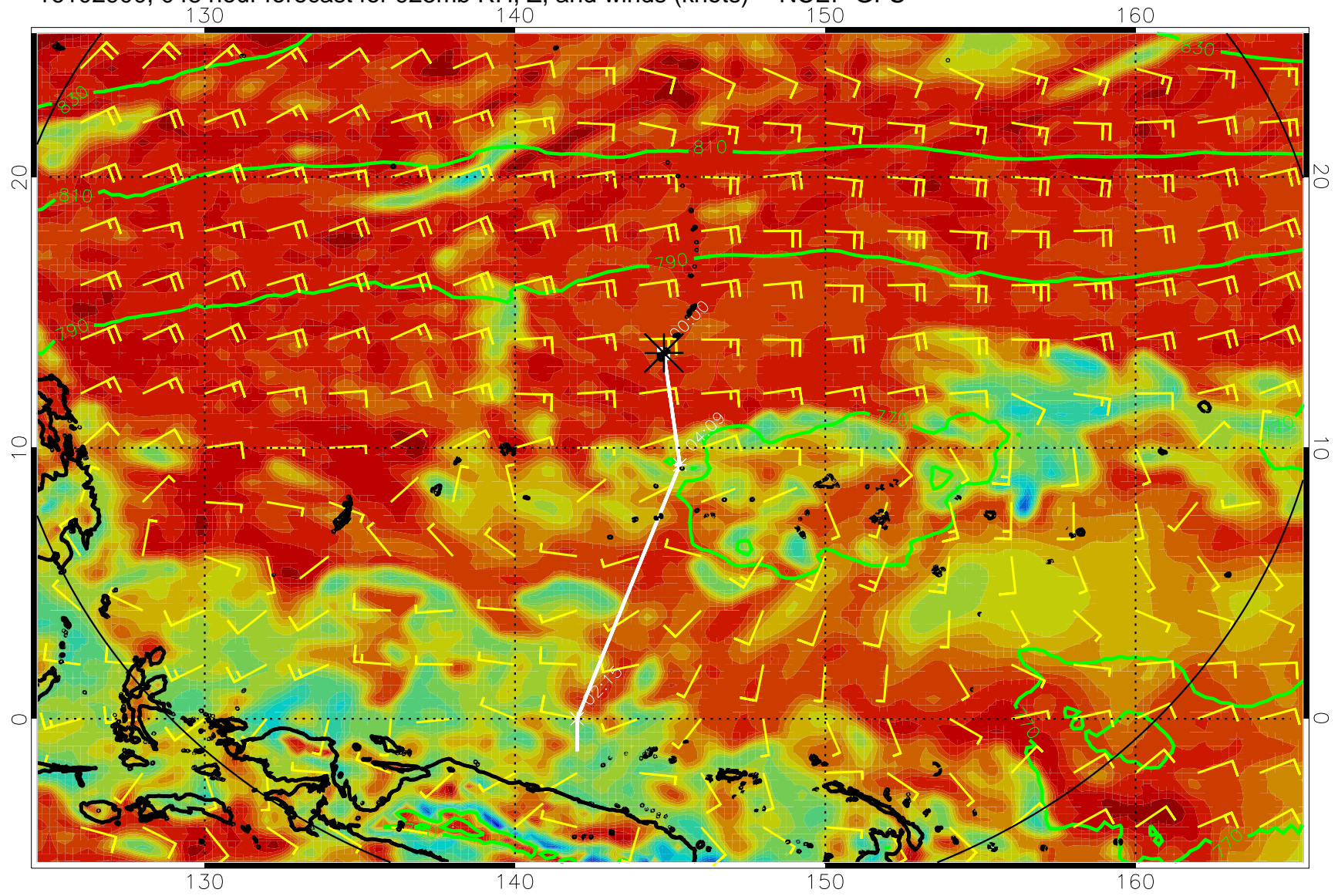
16102900, 048 hour forecast for 925mb RH, Z, and winds (knots) -- NCEP GFS
