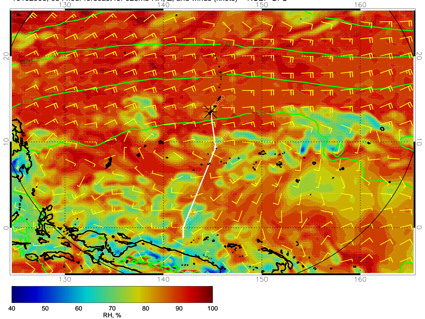
16102906, 054 hour forecast for 925mb RH, Z, and winds (knots) -- NCEP GFS
