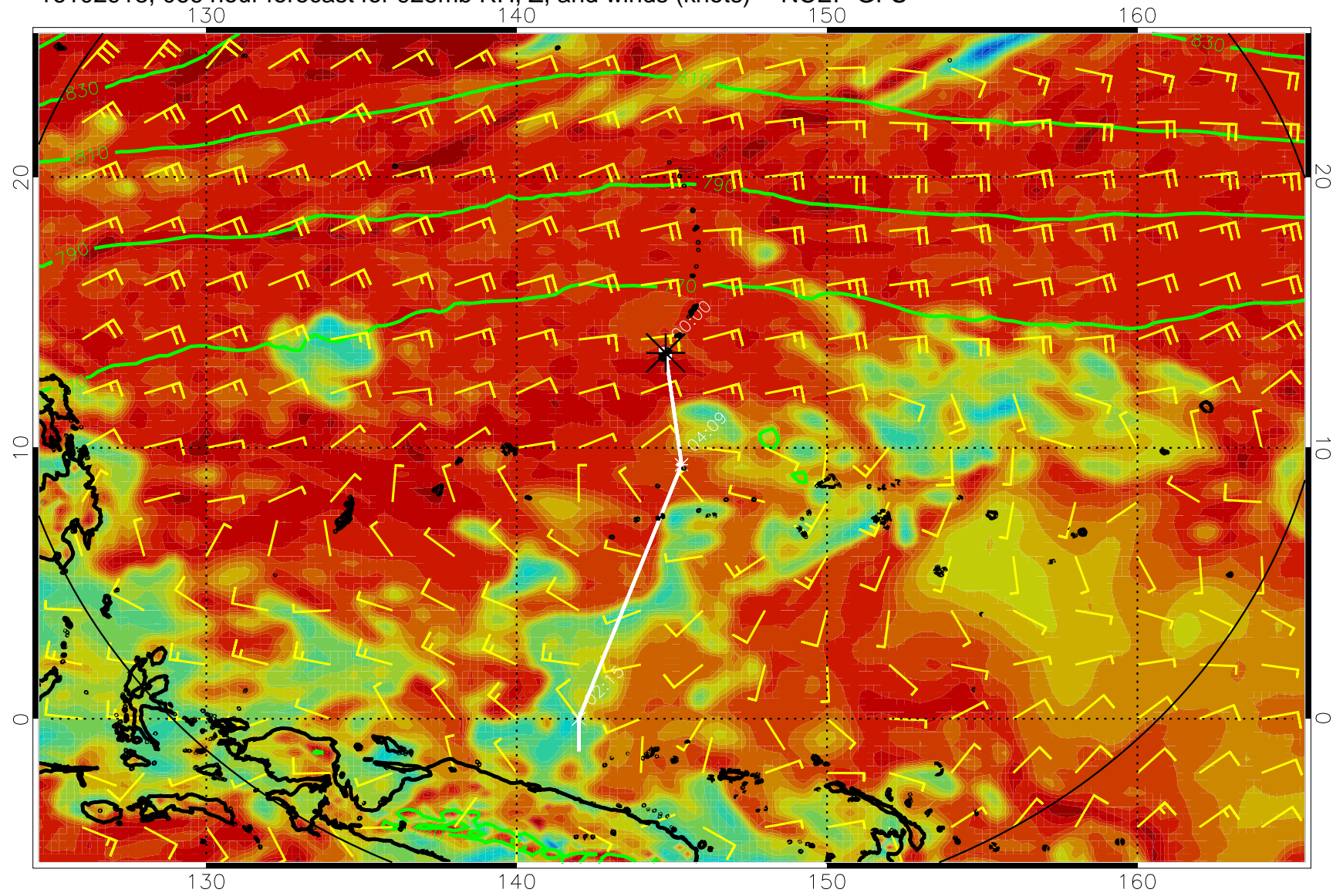
16102918, 066 hour forecast for 925mb RH, Z, and winds (knots) -- NCEP GFS
