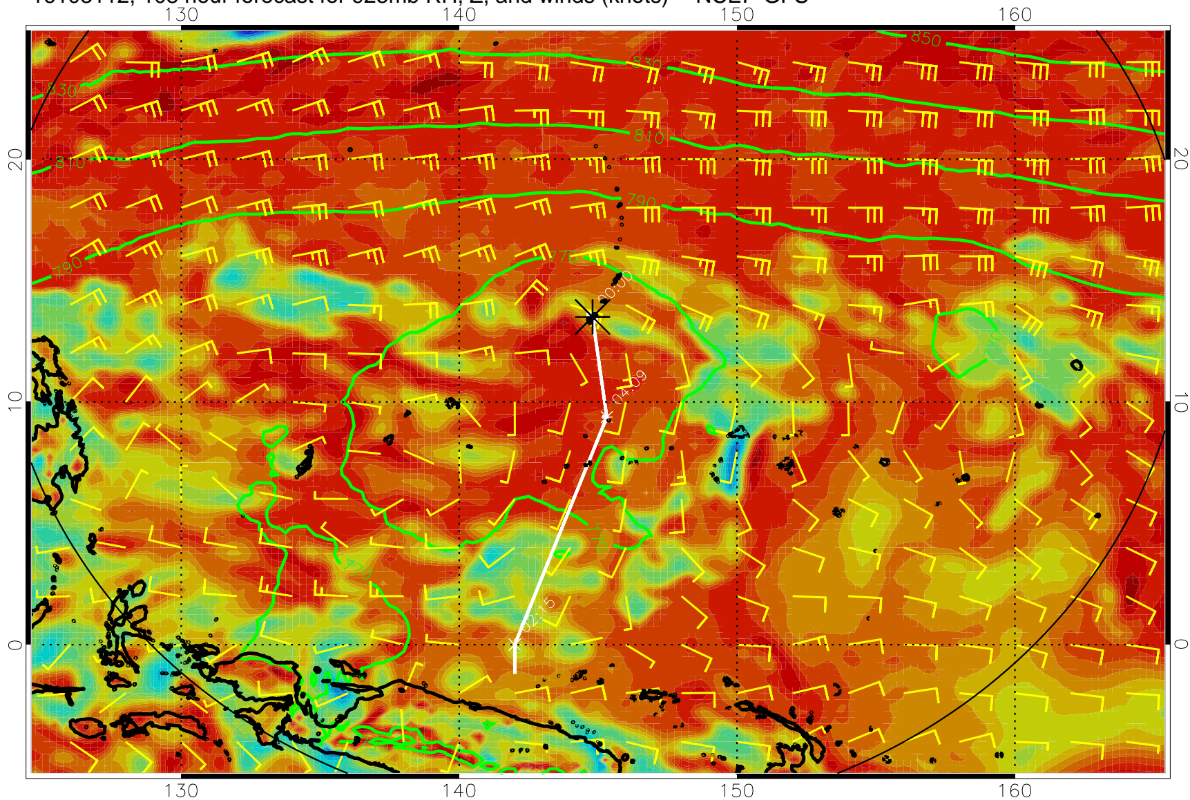
16103112, 108 hour forecast for 925mb RH, Z, and winds (knots) -- NCEP GFS
