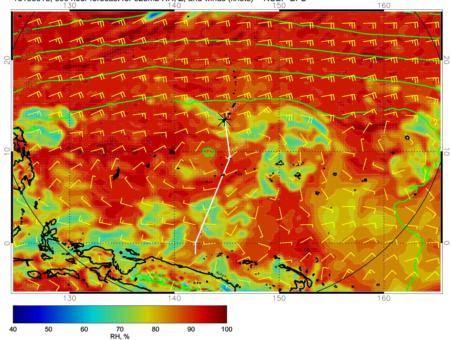
16103018, 090 hour forecast for 925mb RH, Z, and winds (knots) -- NCEP GFS
