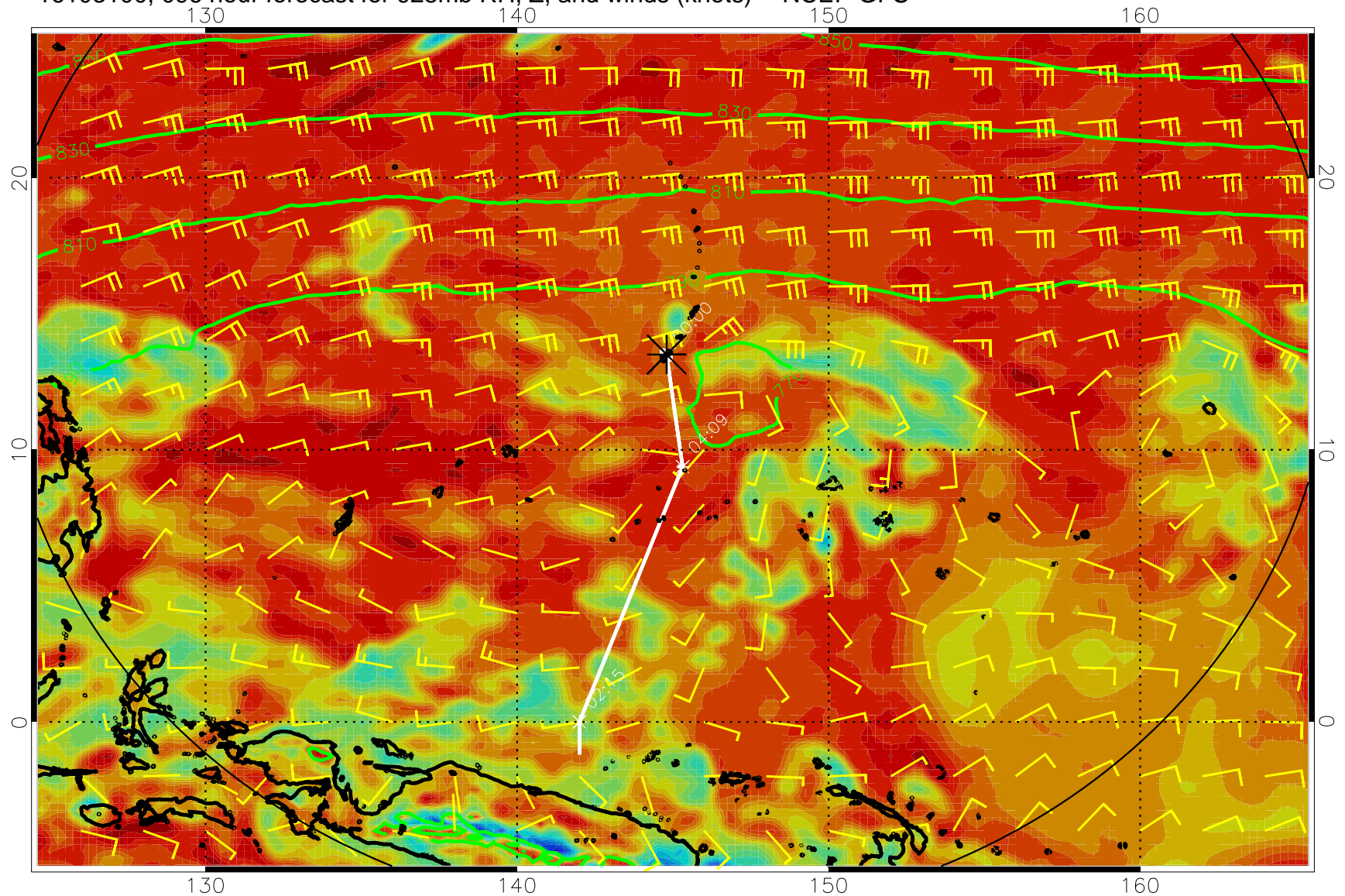
16103100, 096 hour forecast for 925mb RH, Z, and winds (knots) -- NCEP GFS
