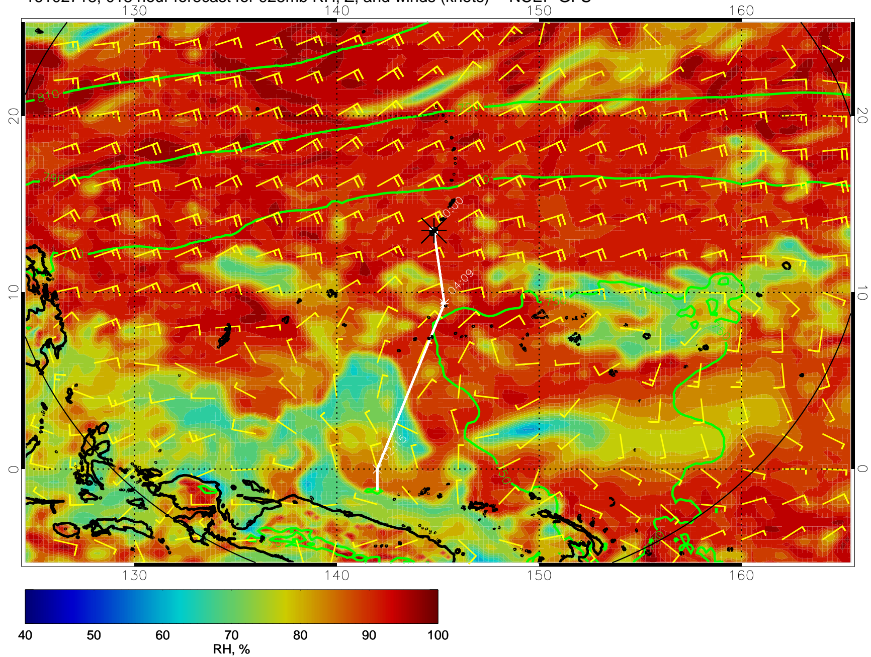
16102718, 018 hour forecast for 925mb RH, Z, and winds (knots) -- NCEP GFS
