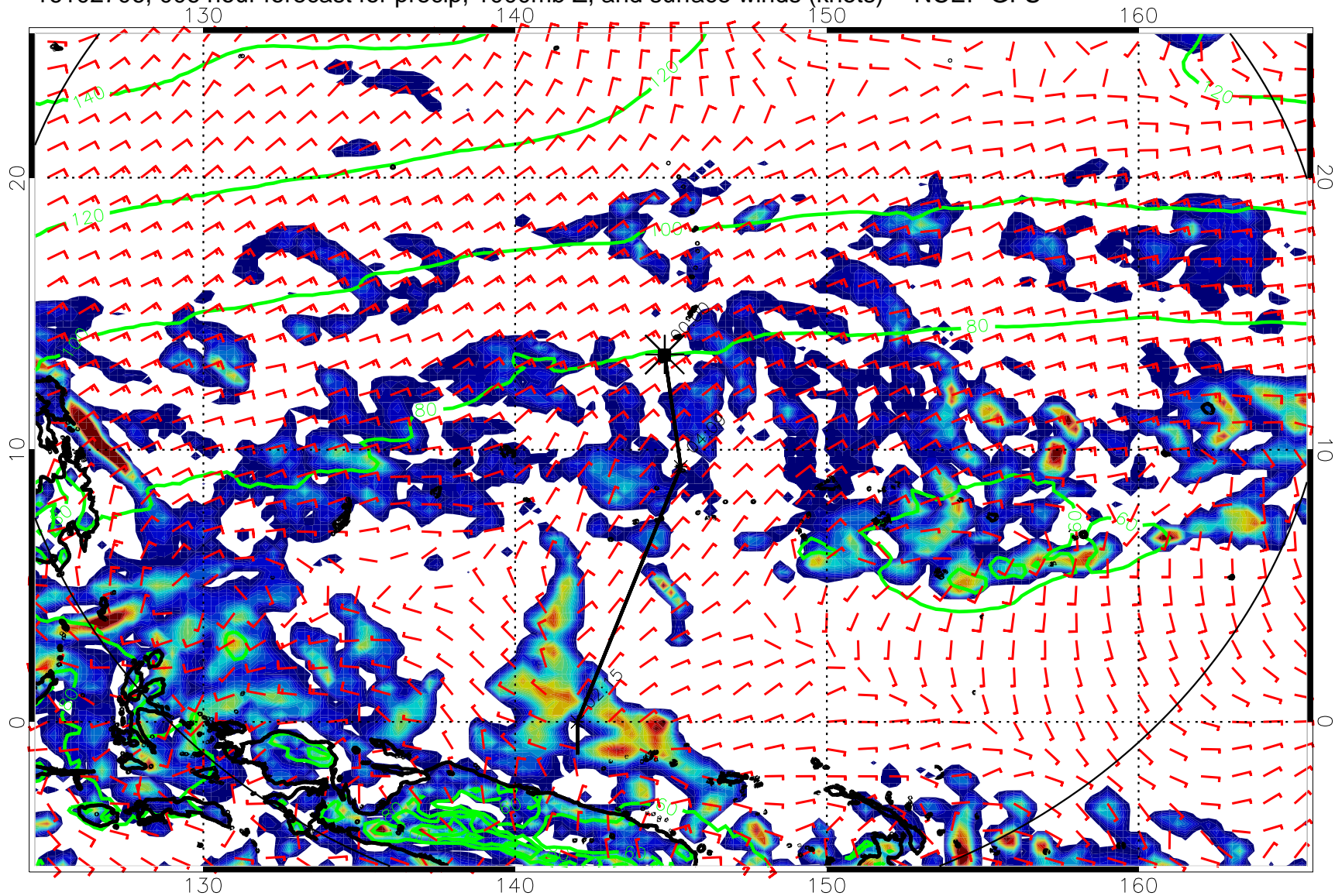
16102706, 006 hour forecast for precip, 1000mb Z, and surface winds (knots) -- NCEP GFS
