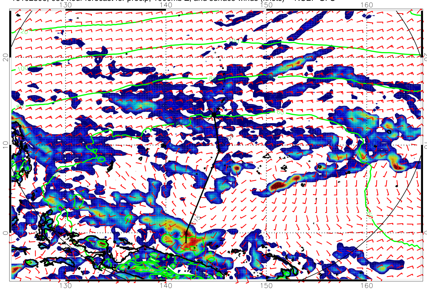
16102806, 030 hour forecast for precip, 1000mb Z, and surface winds (knots) -- NCEP GFS
