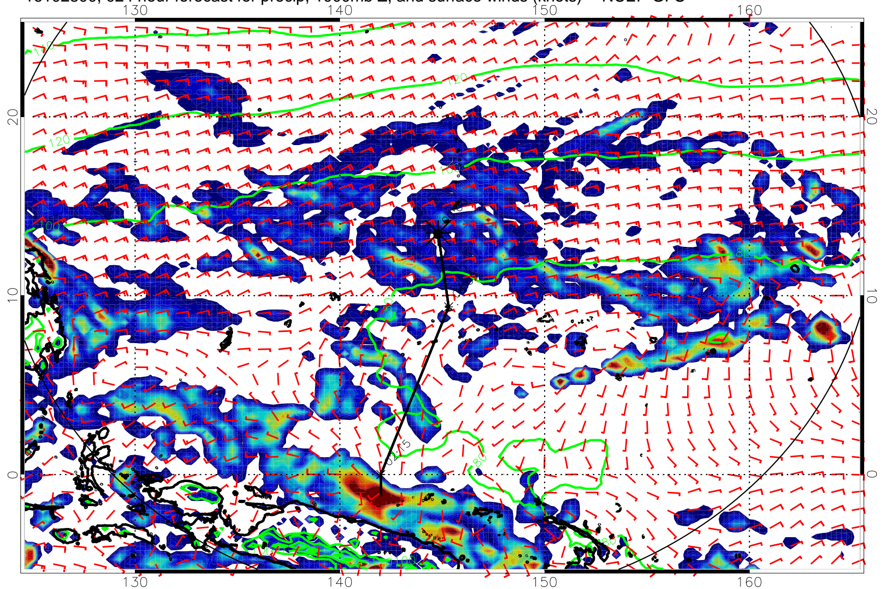
16102800, 024 hour forecast for precip, 1000mb Z, and surface winds (knots) -- NCEP GFS
