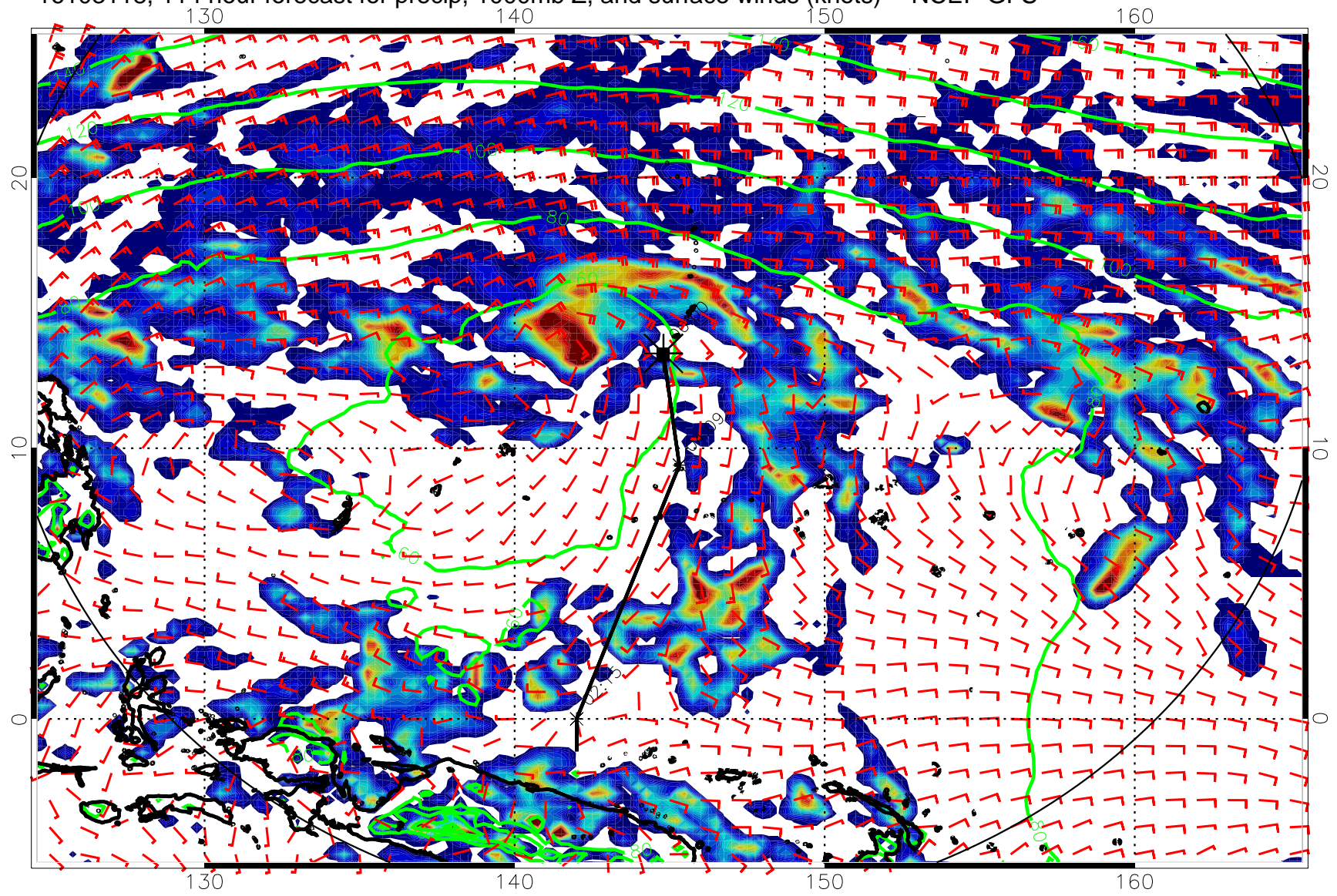
16103118, 114 hour forecast for precip, 1000mb Z, and surface winds (knots) -- NCEP GFS
