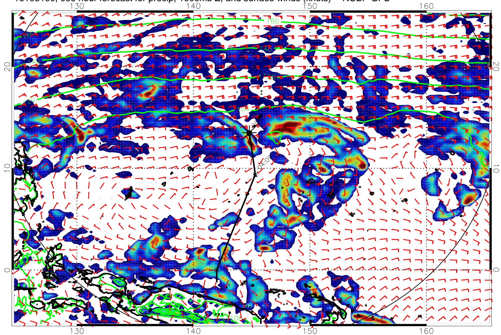
16103100, 096 hour forecast for precip, 1000mb Z, and surface winds (knots) -- NCEP GFS
