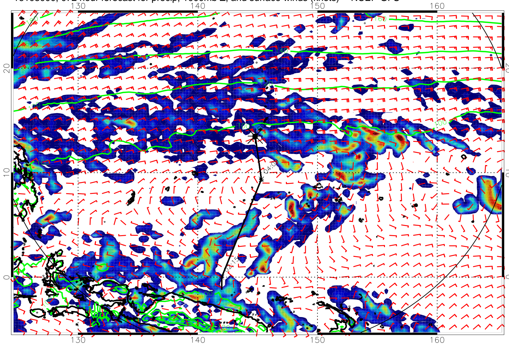
16103000, 072 hour forecast for precip, 1000mb Z, and surface winds (knots) -- NCEP GFS
