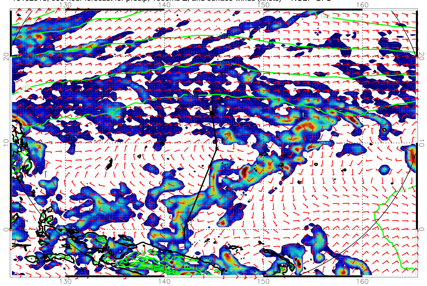
16102918, 066 hour forecast for precip, 1000mb Z, and surface winds (knots) -- NCEP GFS
