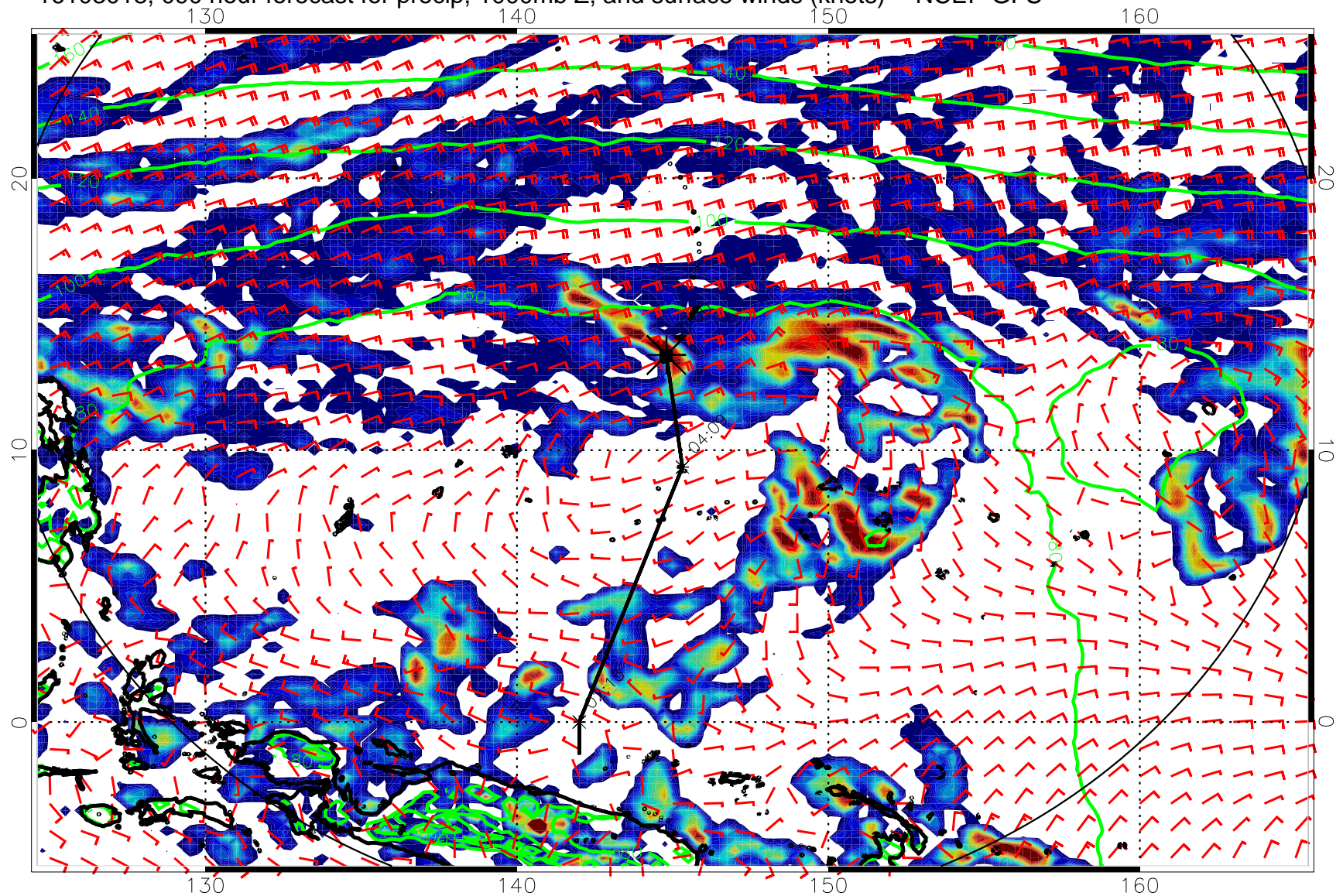
16103018, 090 hour forecast for precip, 1000mb Z, and surface winds (knots) -- NCEP GFS
