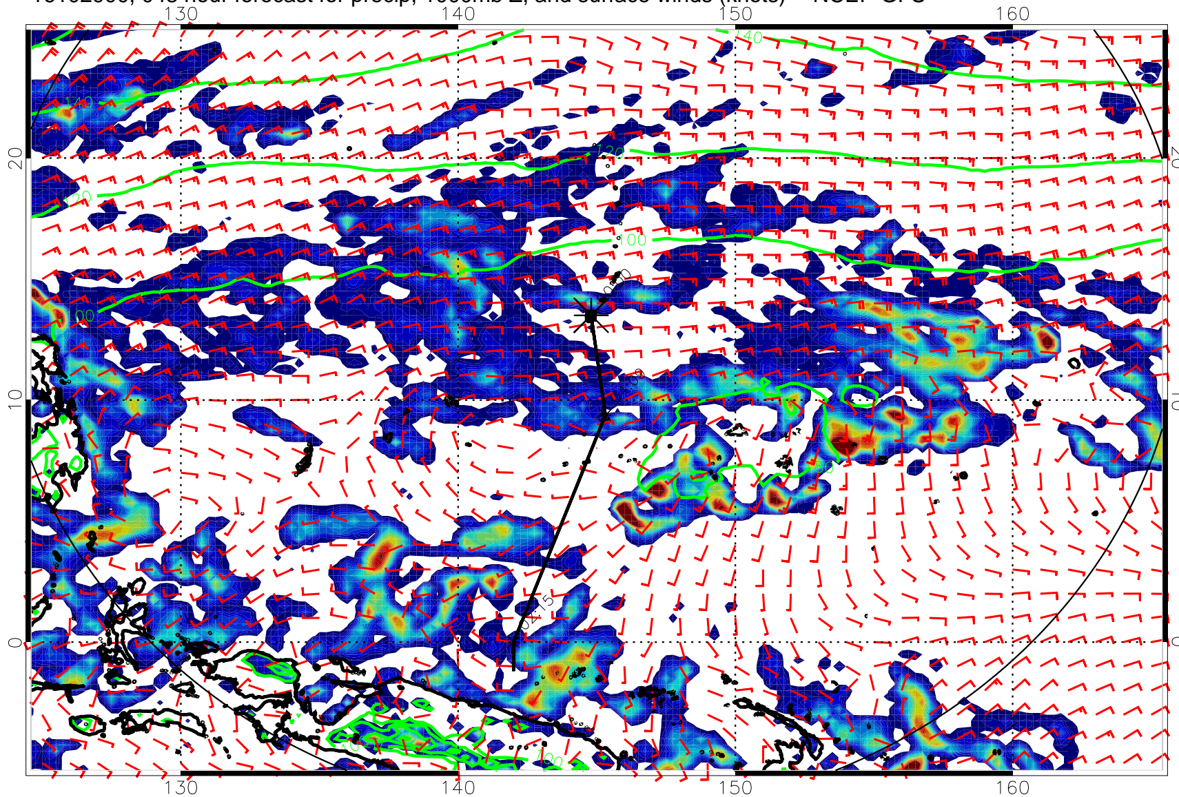
16102900, 048 hour forecast for precip, 1000mb Z, and surface winds (knots) -- NCEP GFS
