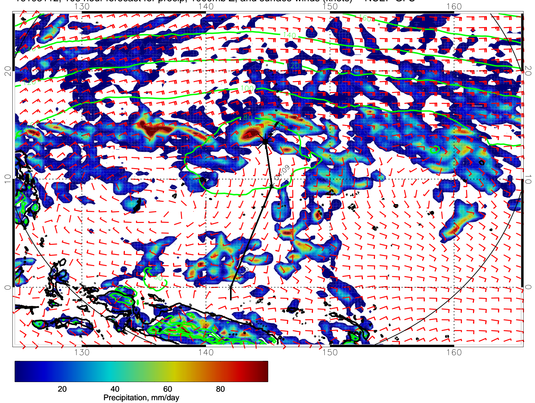
16103112, 108 hour forecast for precip, 1000mb Z, and surface winds (knots) -- NCEP GFS
