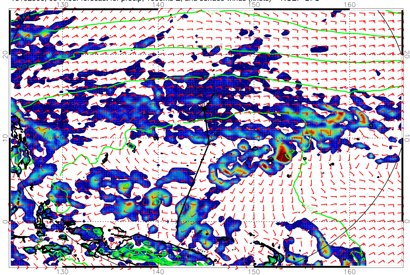
16102906, 054 hour forecast for precip, 1000mb Z, and surface winds (knots) -- NCEP GFS
