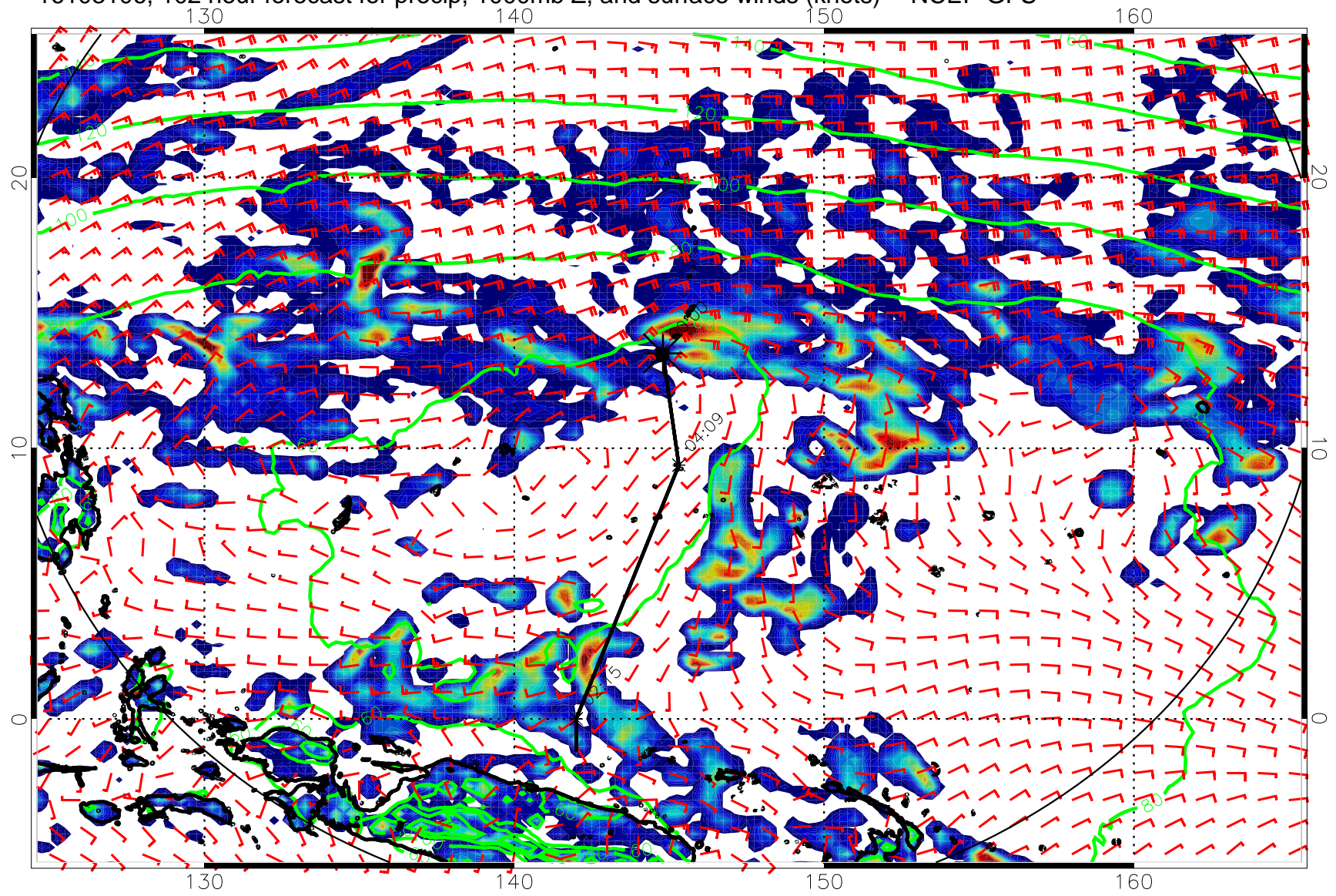
16103106, 102 hour forecast for precip, 1000mb Z, and surface winds (knots) -- NCEP GFS
