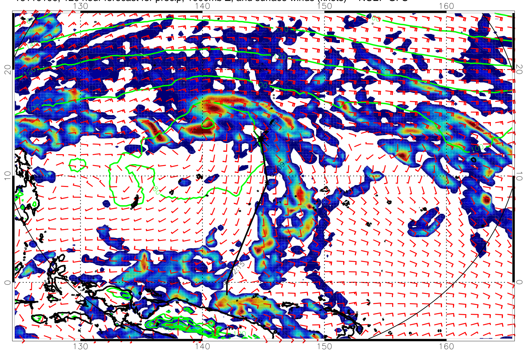
16110100, 120 hour forecast for precip, 1000mb Z, and surface winds (knots) -- NCEP GFS
