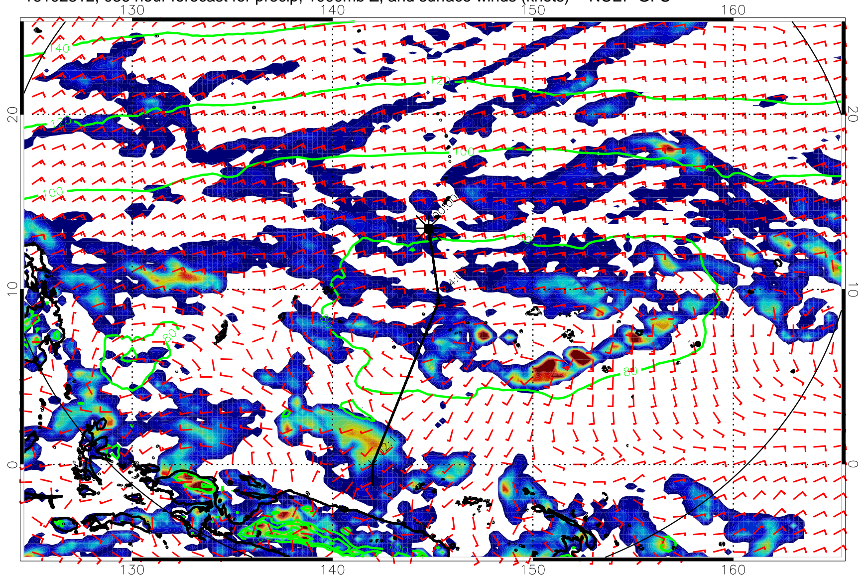
16102812, 036 hour forecast for precip, 1000mb Z, and surface winds (knots) -- NCEP GFS
