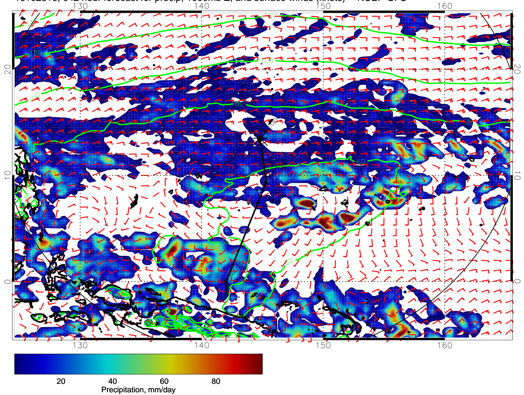
16102818, 042 hour forecast for precip, 1000mb Z, and surface winds (knots) -- NCEP GFS
