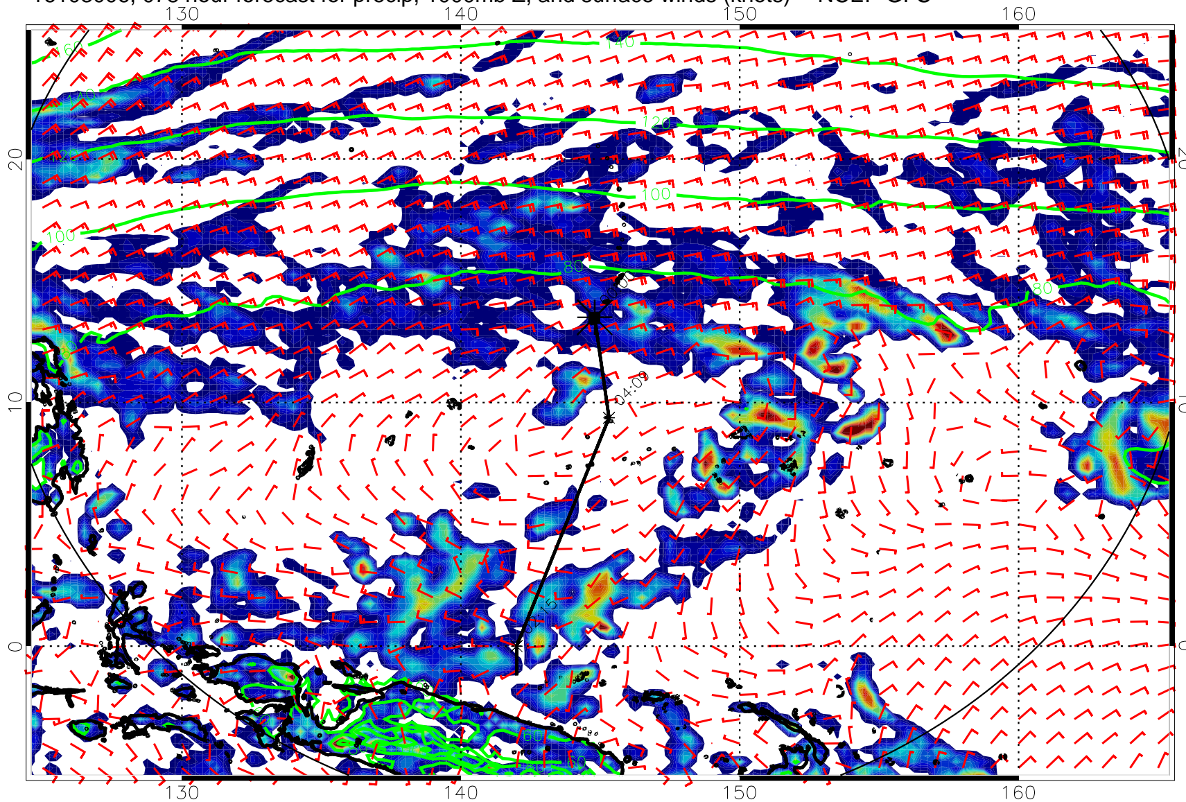
16103006, 078 hour forecast for precip, 1000mb Z, and surface winds (knots) -- NCEP GFS
