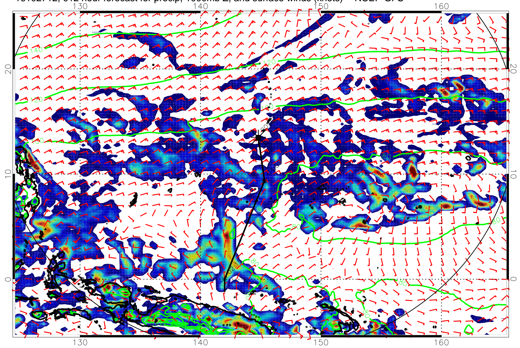
16102712, 012 hour forecast for precip, 1000mb Z, and surface winds (knots) -- NCEP GFS
