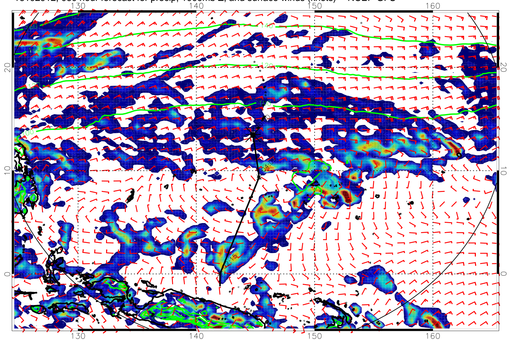
16102912, 060 hour forecast for precip, 1000mb Z, and surface winds (knots) -- NCEP GFS
