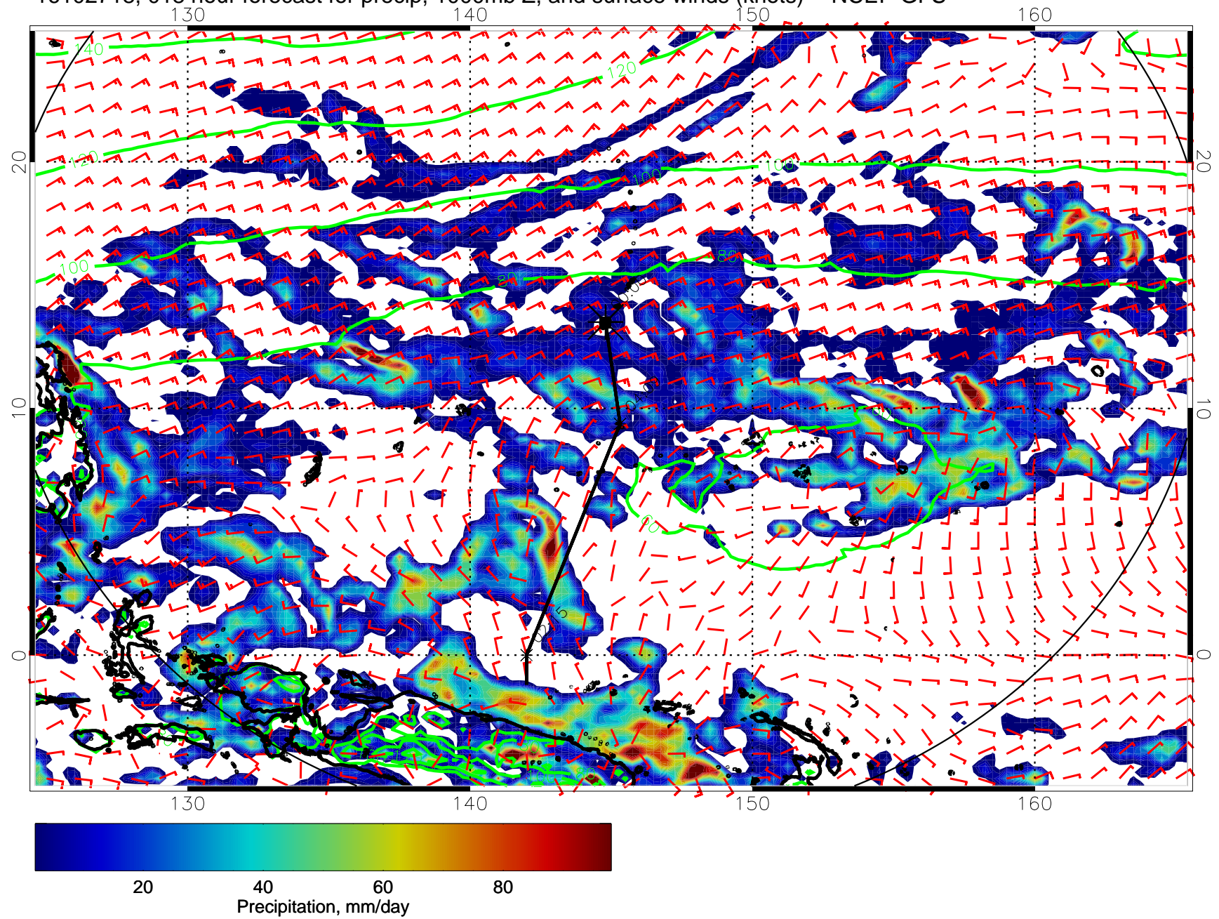
16102718, 018 hour forecast for precip, 1000mb Z, and surface winds (knots) -- NCEP GFS
