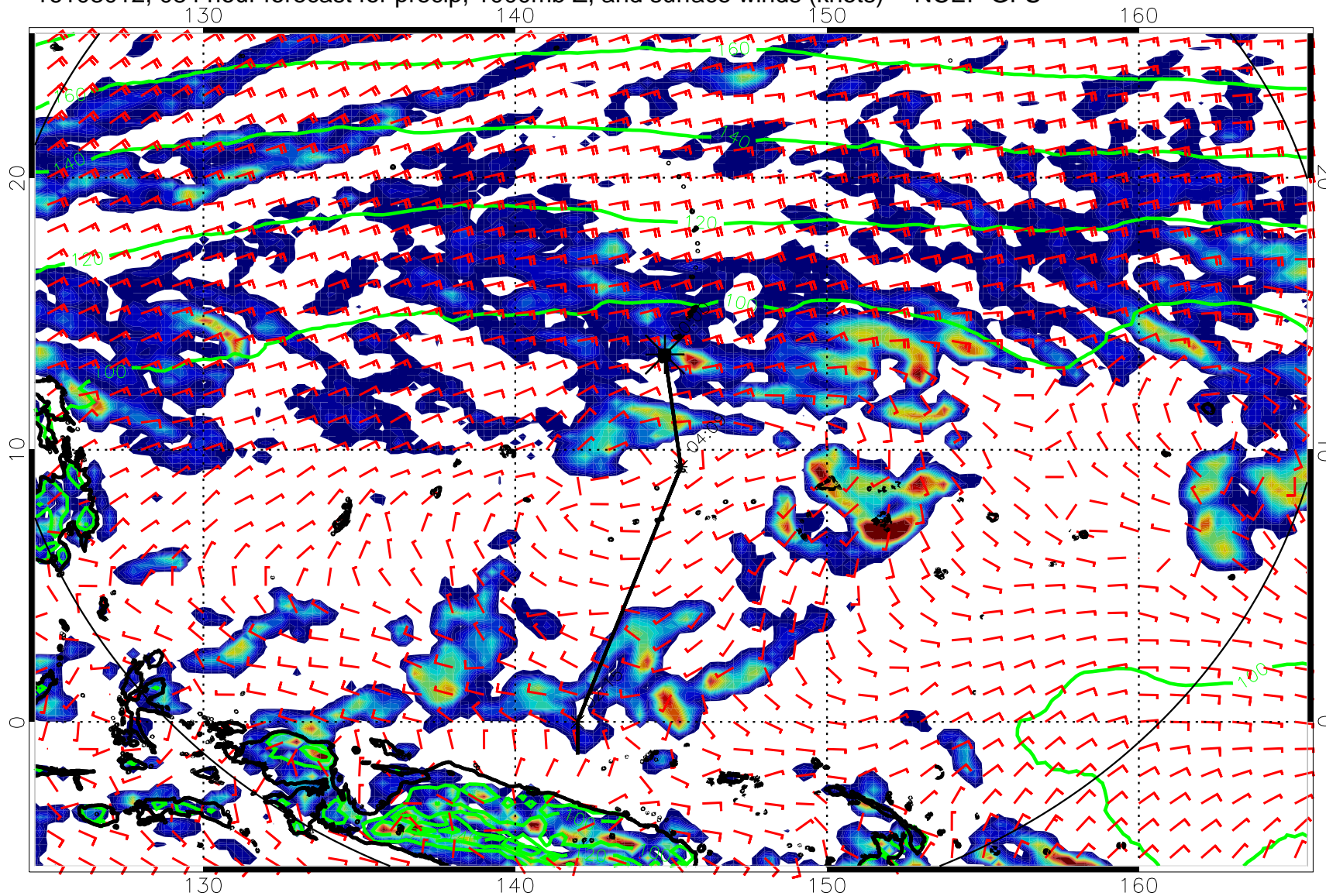
16103012, 084 hour forecast for precip, 1000mb Z, and surface winds (knots) -- NCEP GFS
