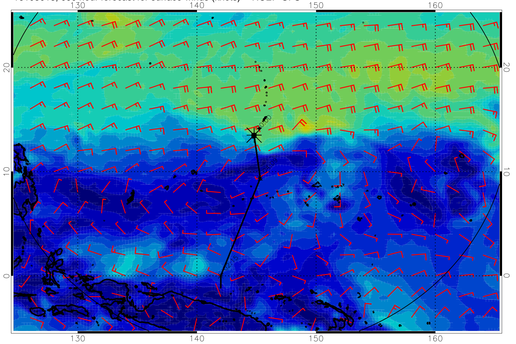
16103018, 090 hour forecast for surface winds (knots) -- NCEP GFS
