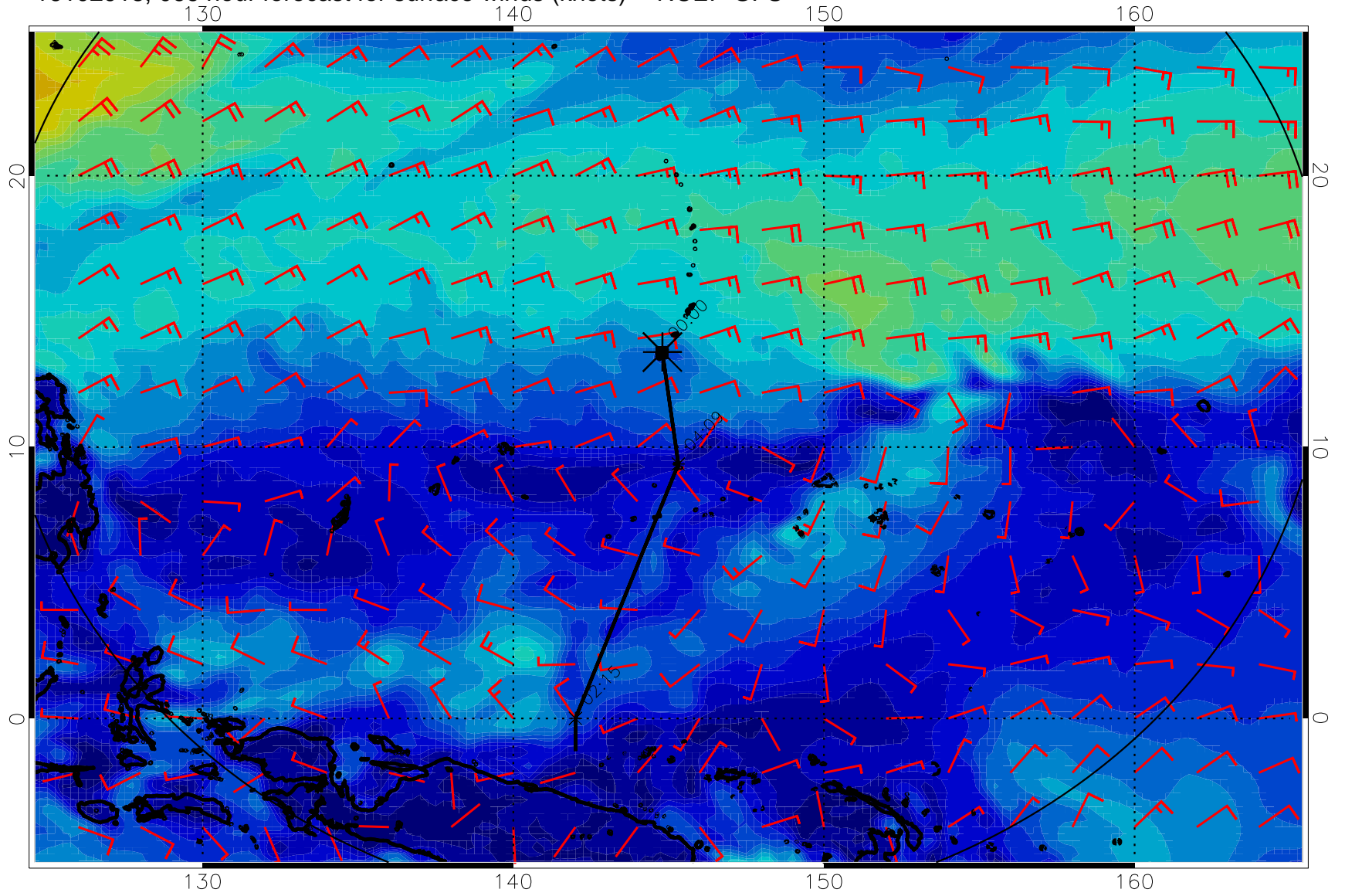
16102918, 066 hour forecast for surface winds (knots) -- NCEP GFS
