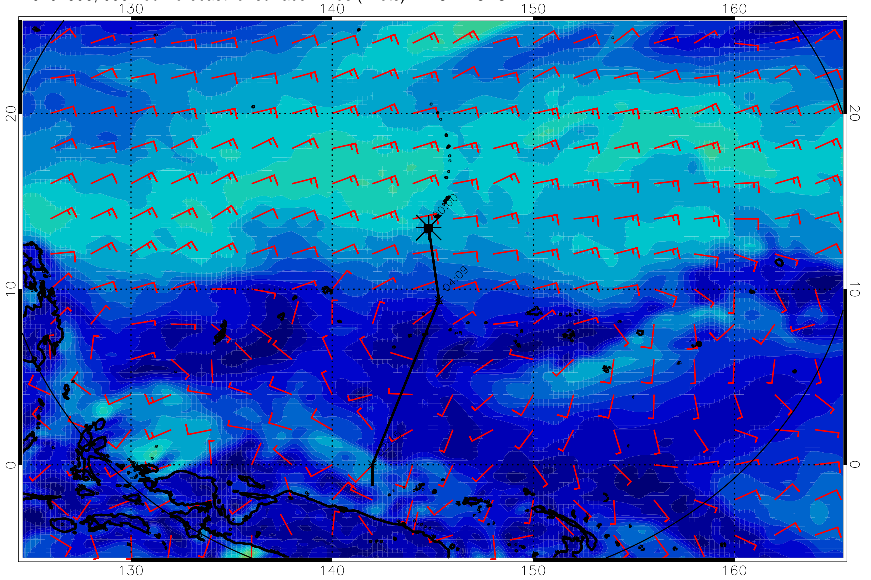
16102806, 030 hour forecast for surface winds (knots) -- NCEP GFS
