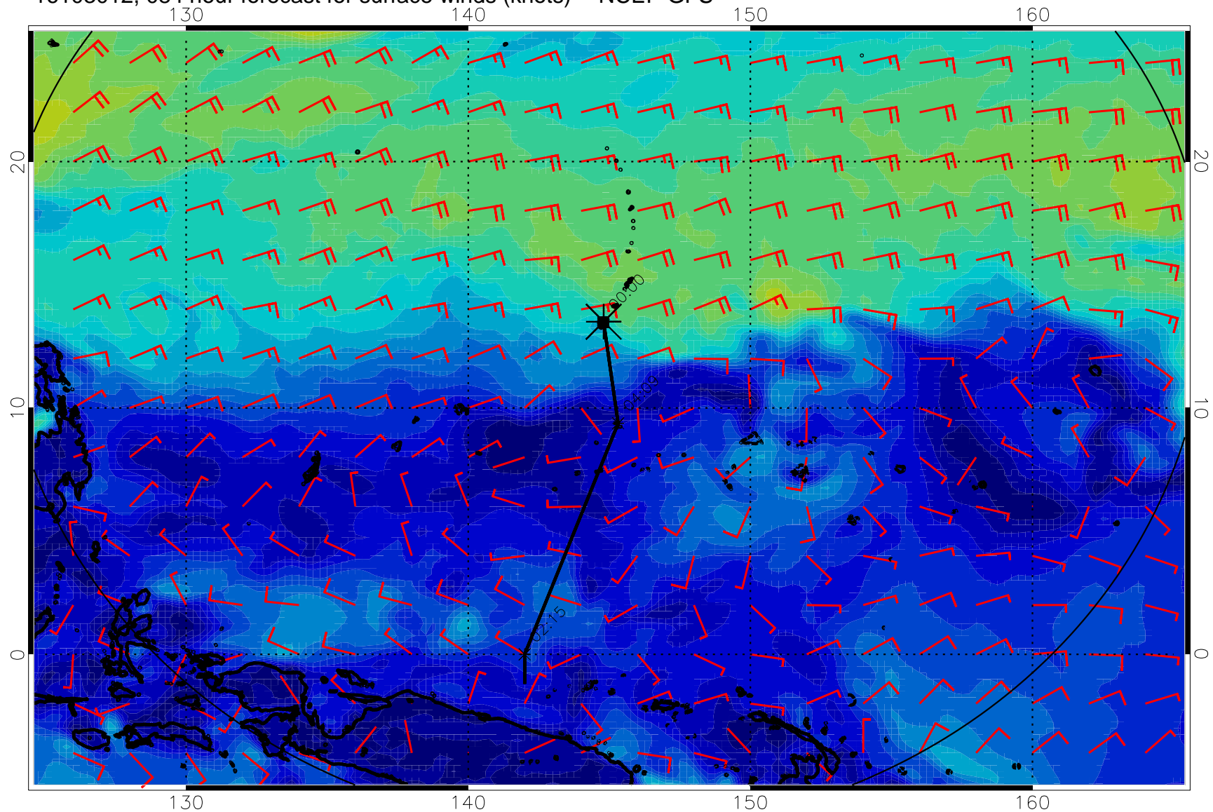
16103012, 084 hour forecast for surface winds (knots) -- NCEP GFS
