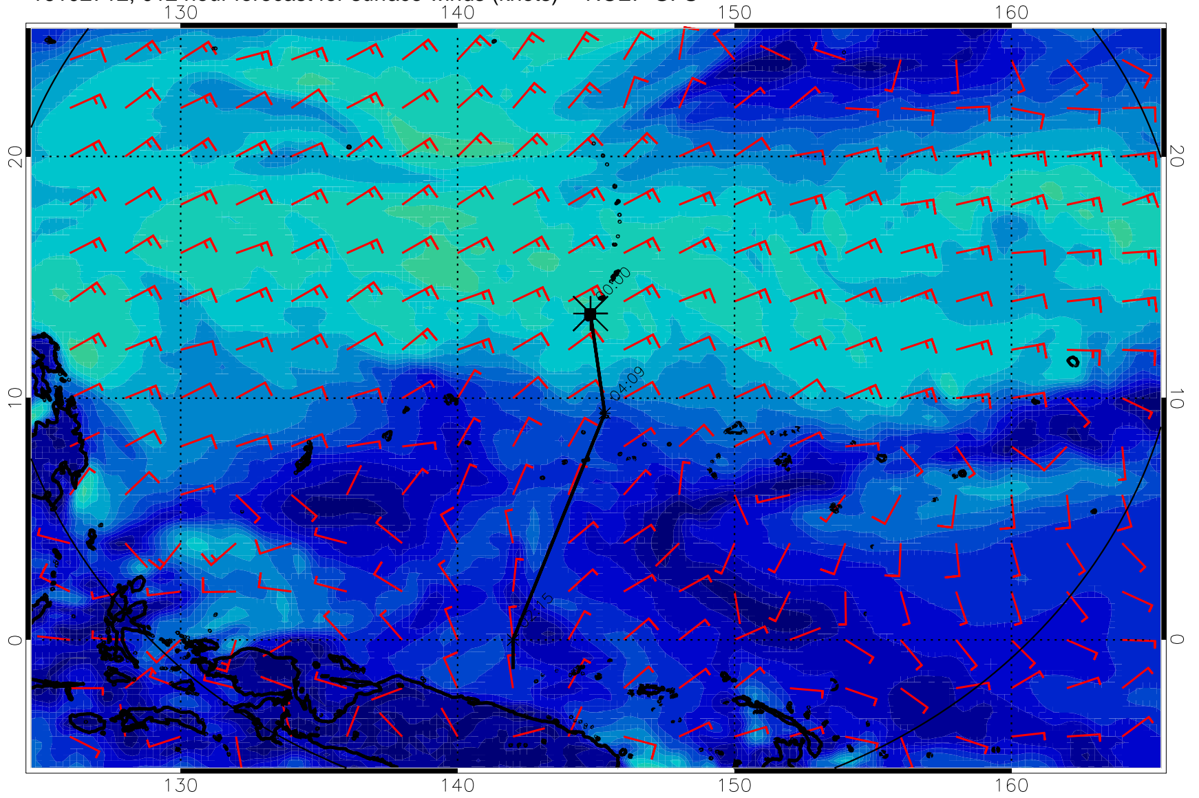
16102712, 012 hour forecast for surface winds (knots) -- NCEP GFS
