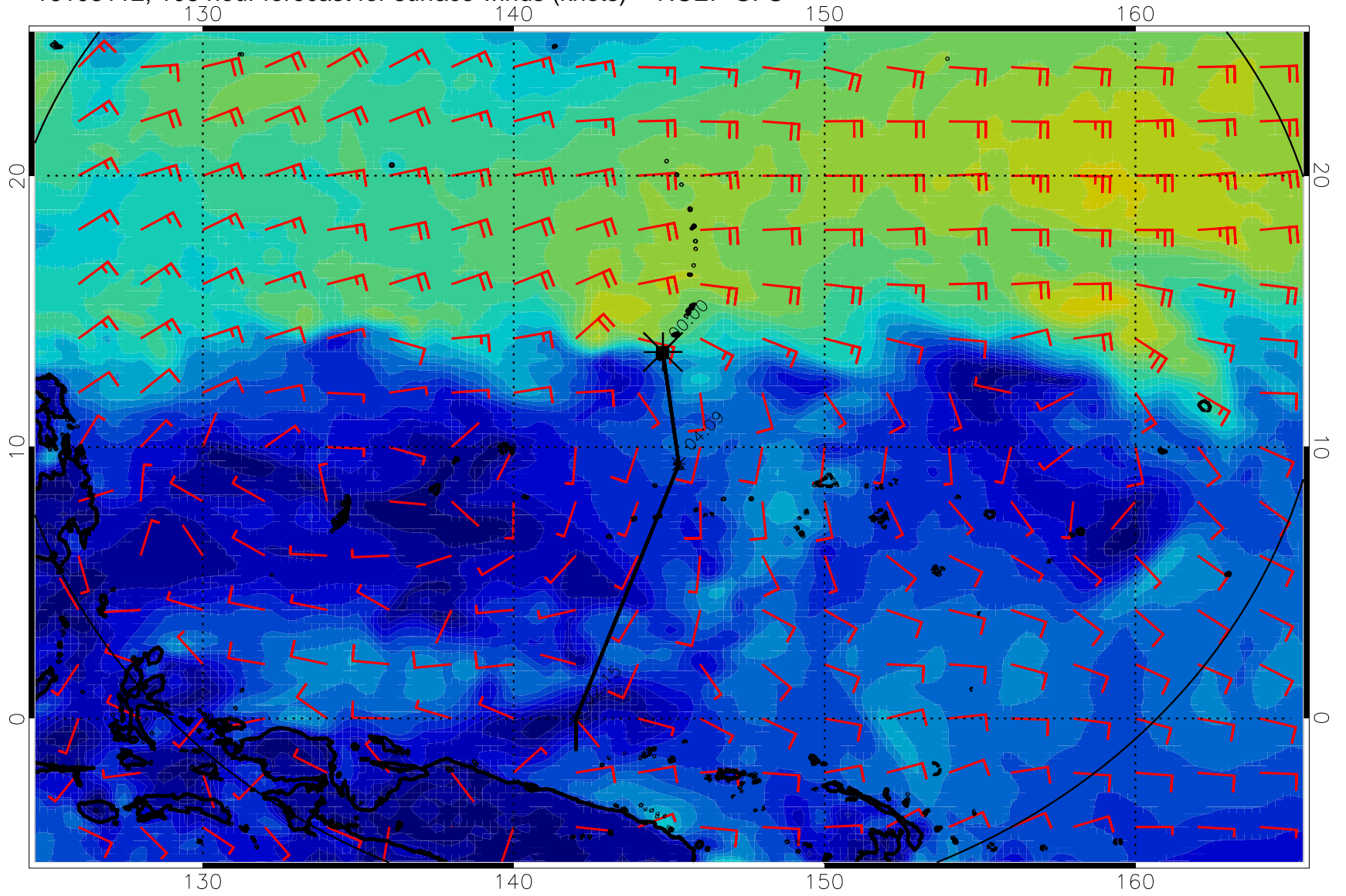
16103112, 108 hour forecast for surface winds (knots) -- NCEP GFS
