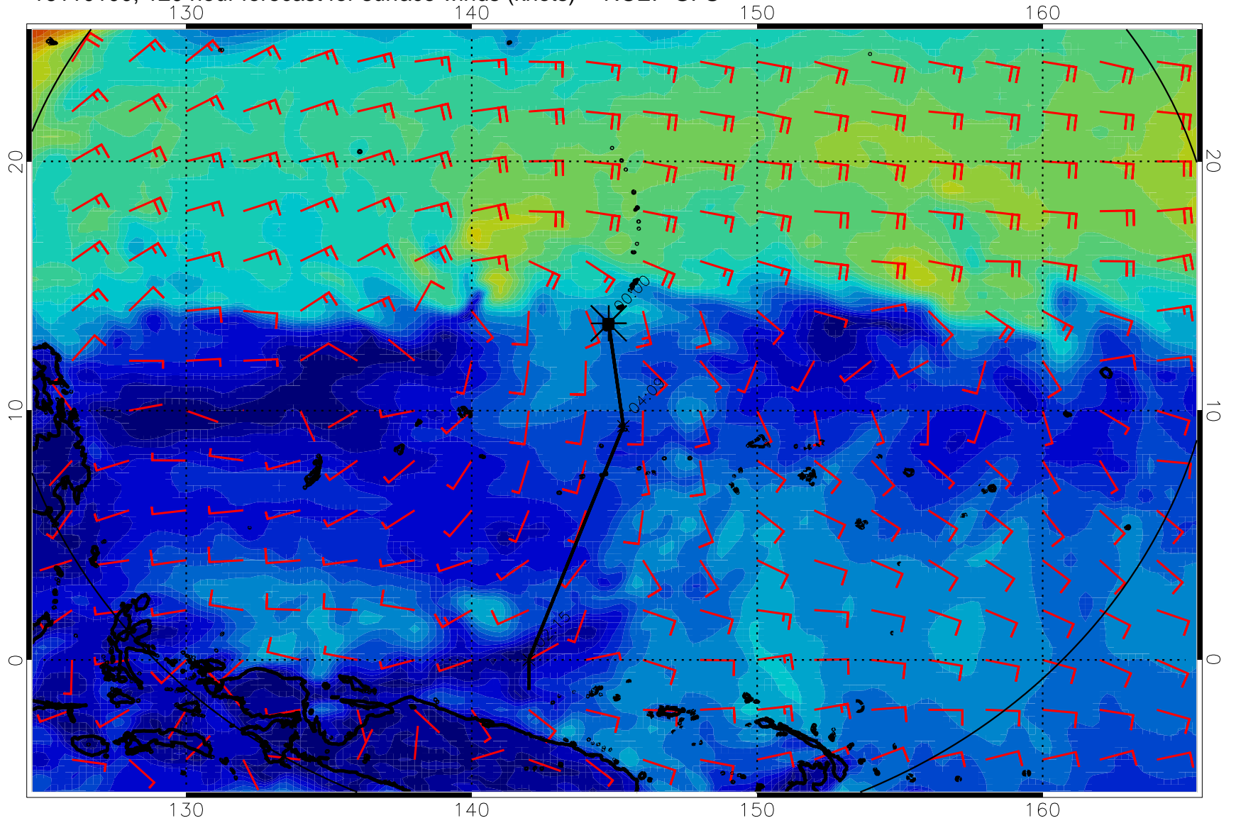
16110100, 120 hour forecast for surface winds (knots) -- NCEP GFS
