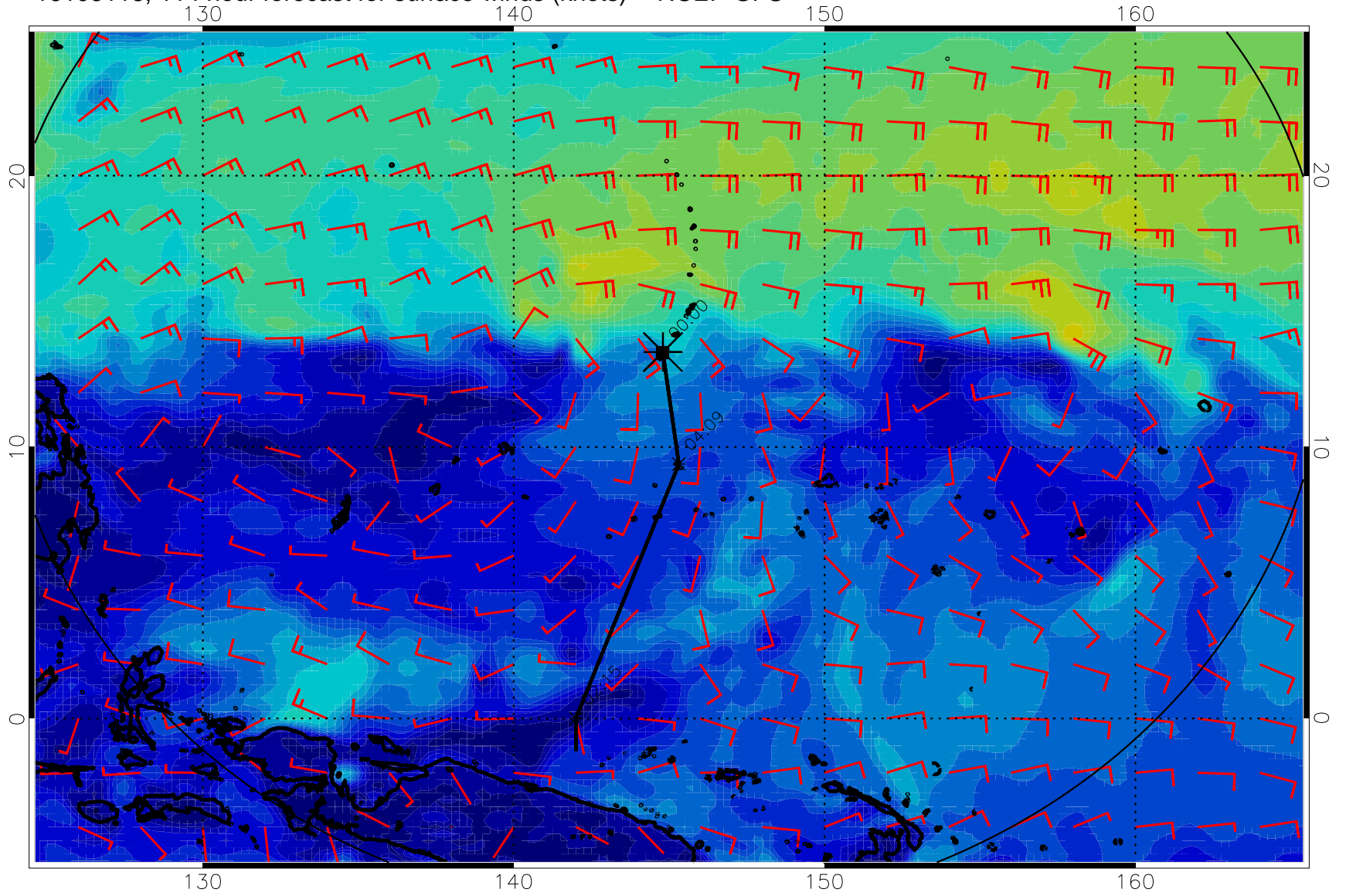
16103118, 114 hour forecast for surface winds (knots) -- NCEP GFS
