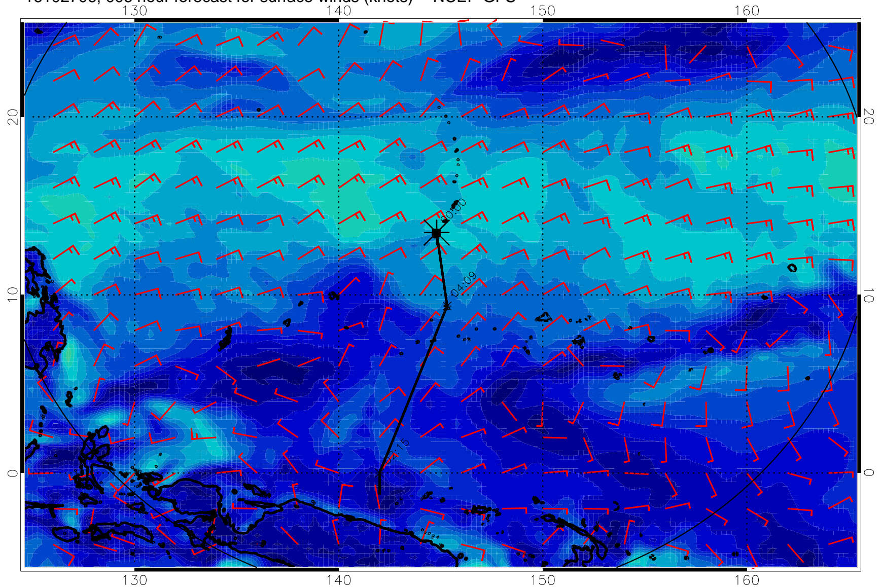
16102706, 006 hour forecast for surface winds (knots) -- NCEP GFS
