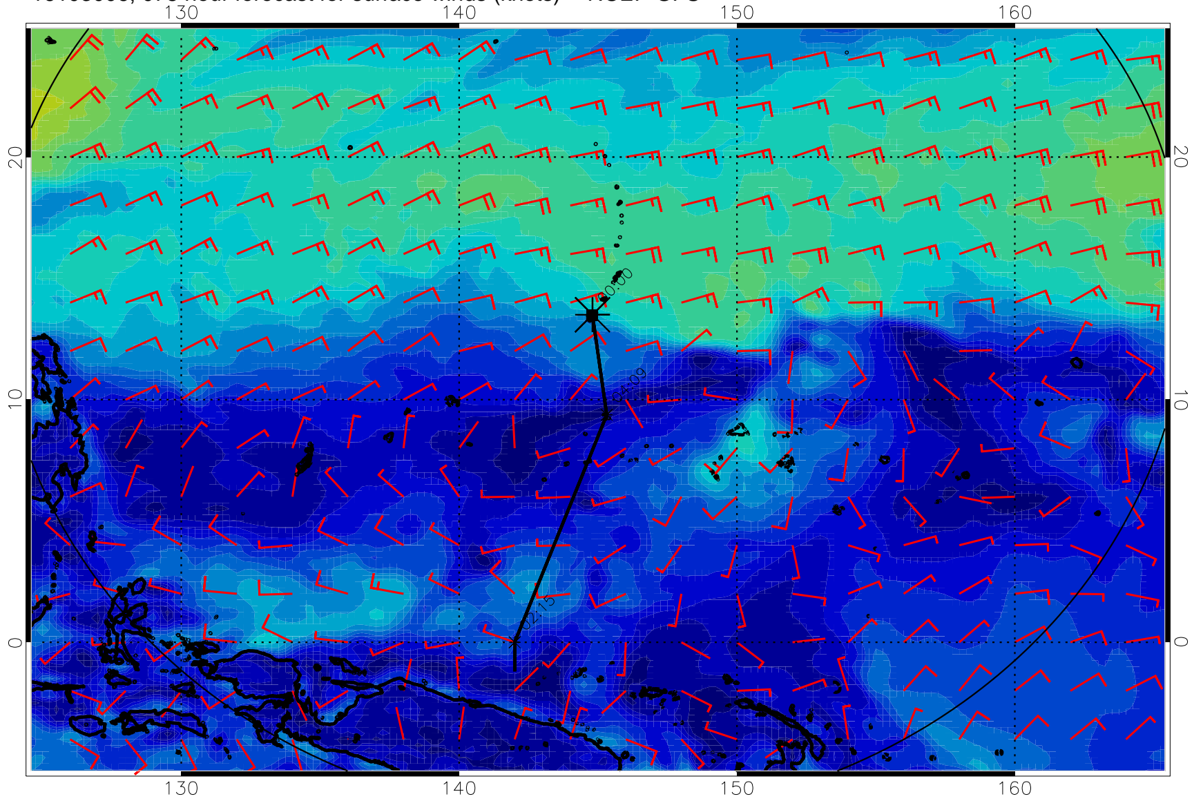
16103006, 078 hour forecast for surface winds (knots) -- NCEP GFS
