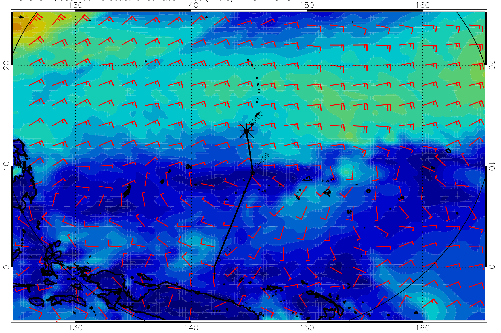
16102912, 060 hour forecast for surface winds (knots) -- NCEP GFS
