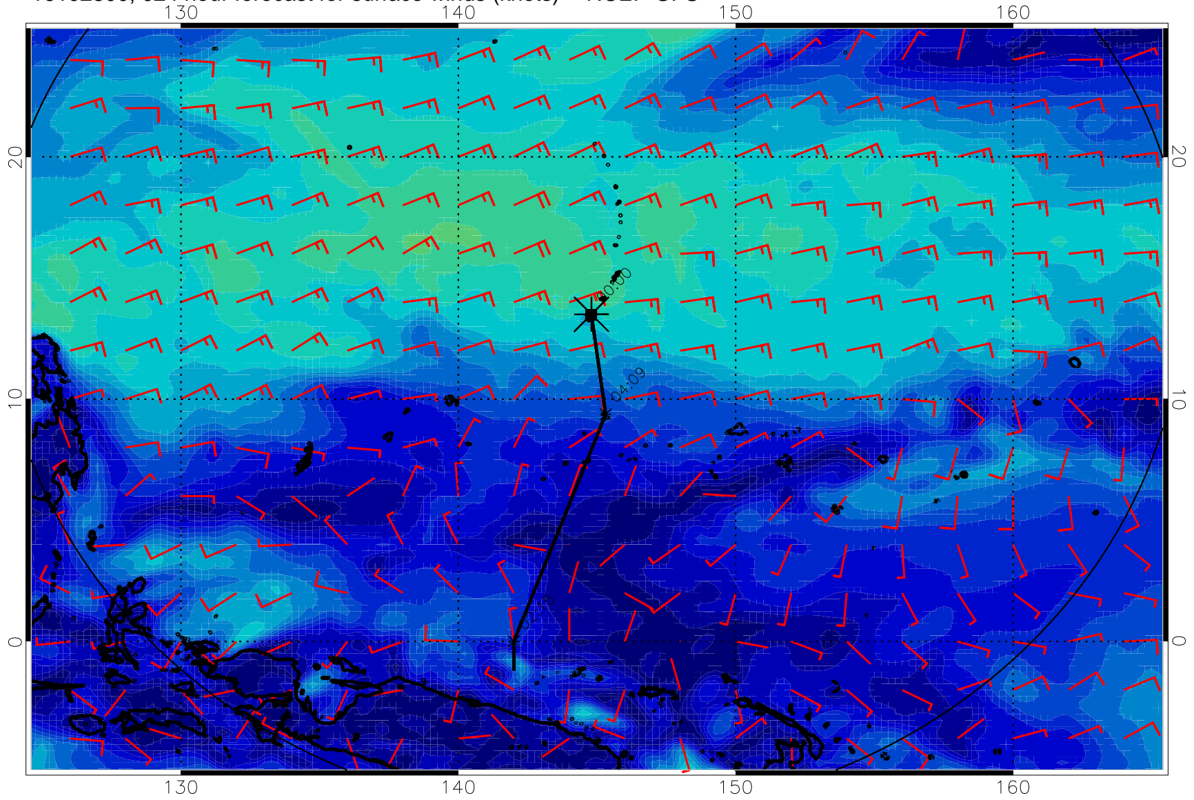
16102800, 024 hour forecast for surface winds (knots) -- NCEP GFS
