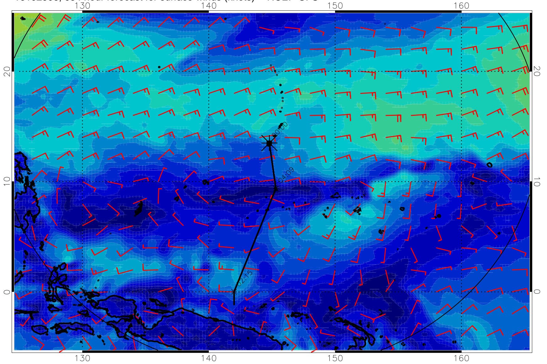
16102906, 054 hour forecast for surface winds (knots) -- NCEP GFS
