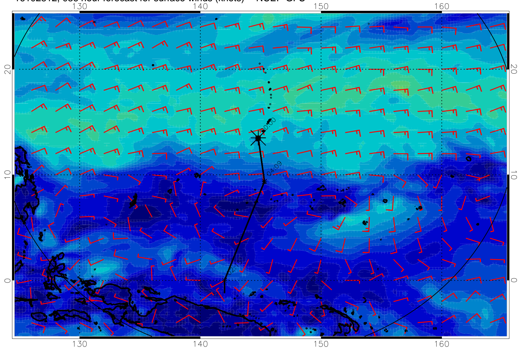
16102812, 036 hour forecast for surface winds (knots) -- NCEP GFS
