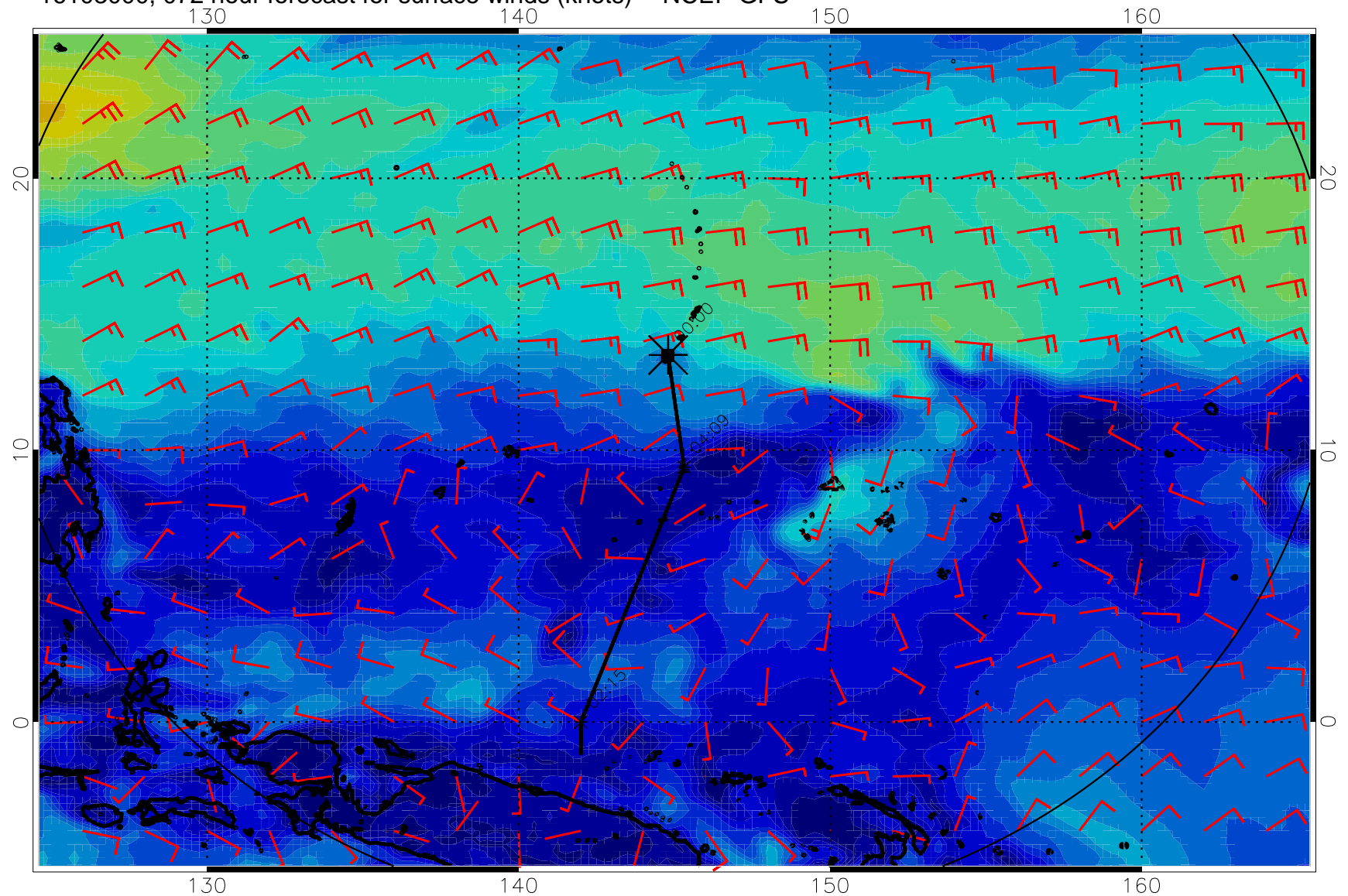
16103000, 072 hour forecast for surface winds (knots) -- NCEP GFS
