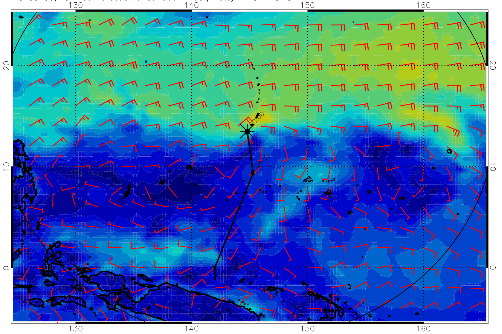
16103106, 102 hour forecast for surface winds (knots) -- NCEP GFS
