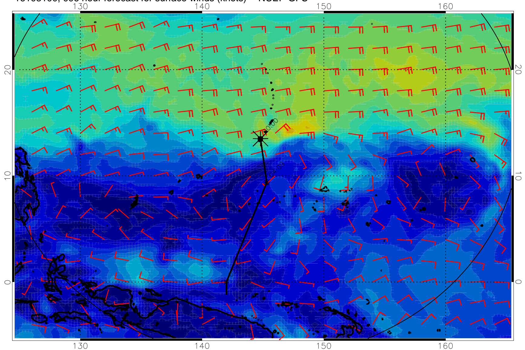
16103100, 096 hour forecast for surface winds (knots) -- NCEP GFS
