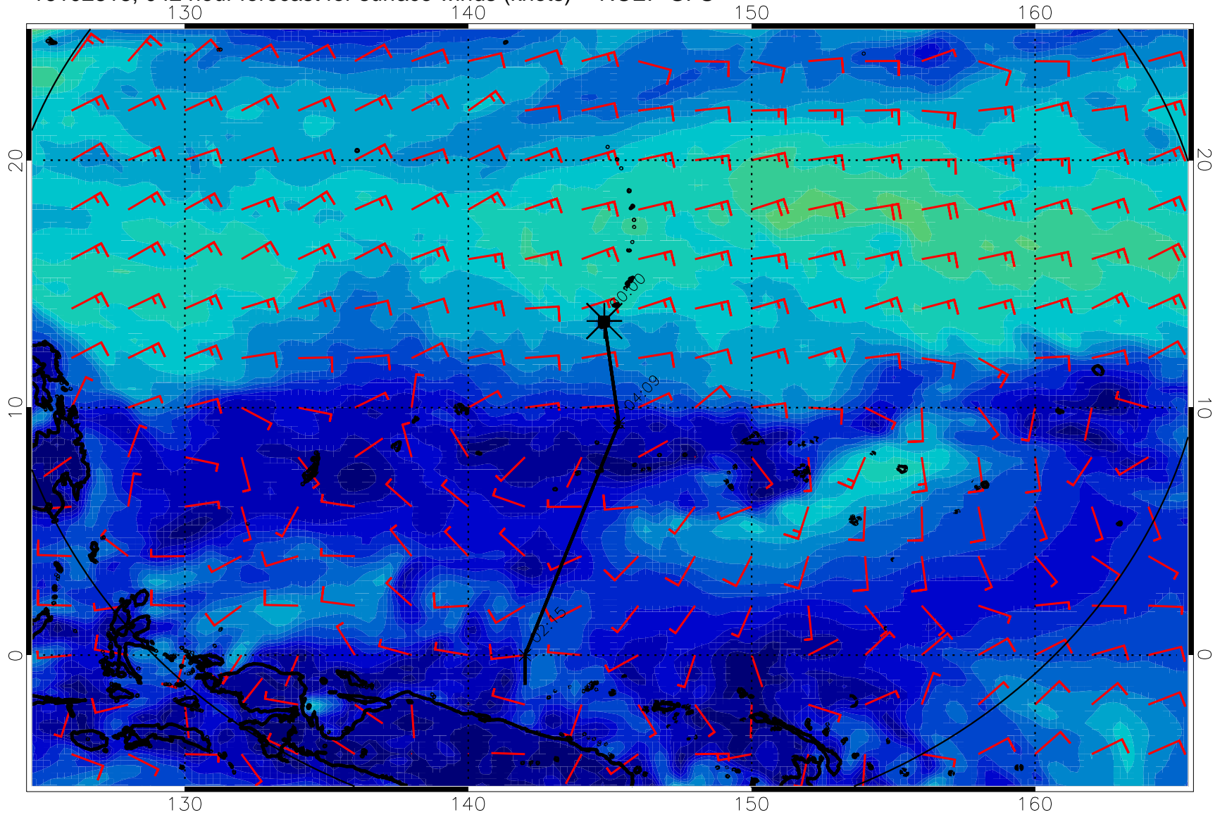
16102818, 042 hour forecast for surface winds (knots) -- NCEP GFS
