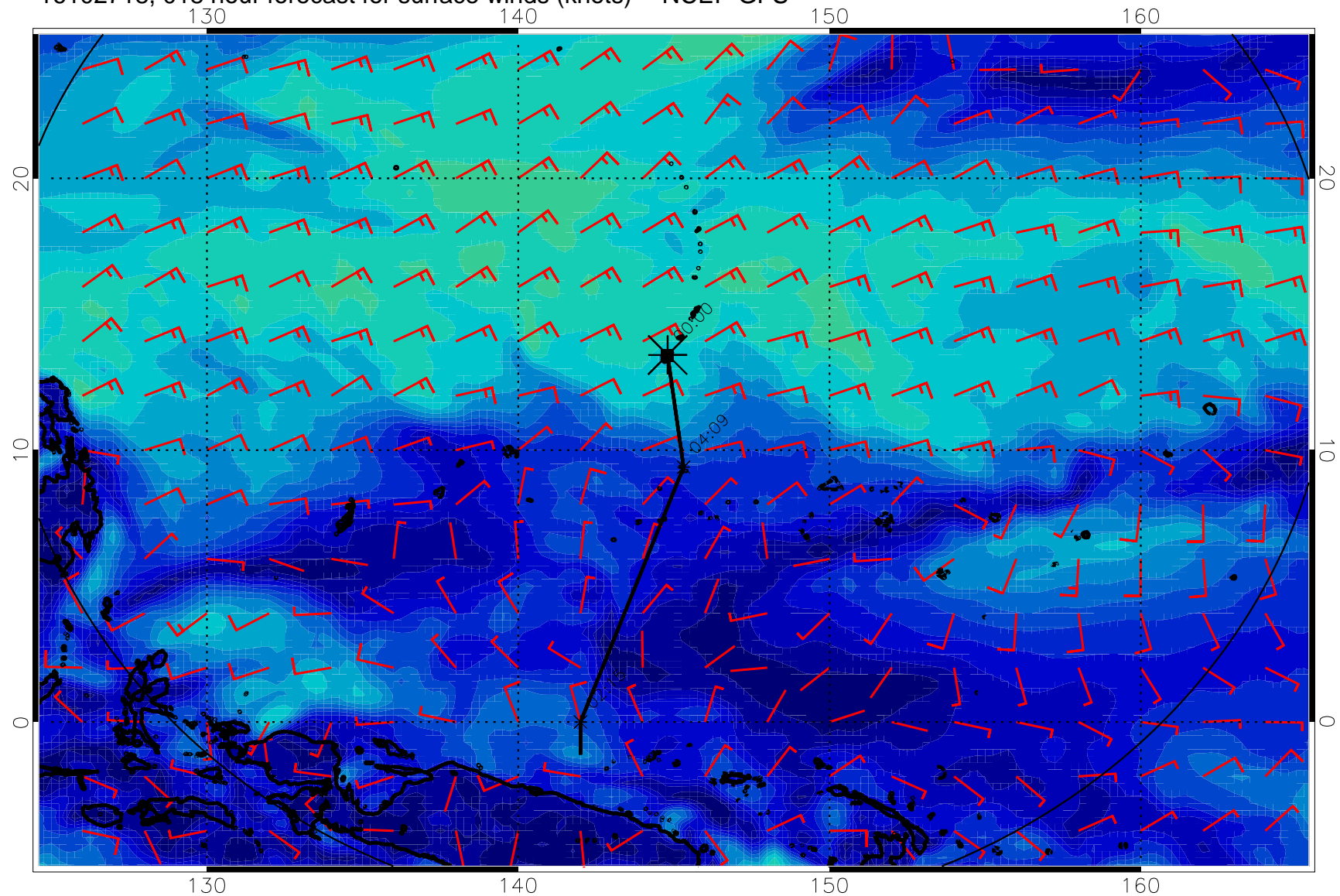
16102718, 018 hour forecast for surface winds (knots) -- NCEP GFS
