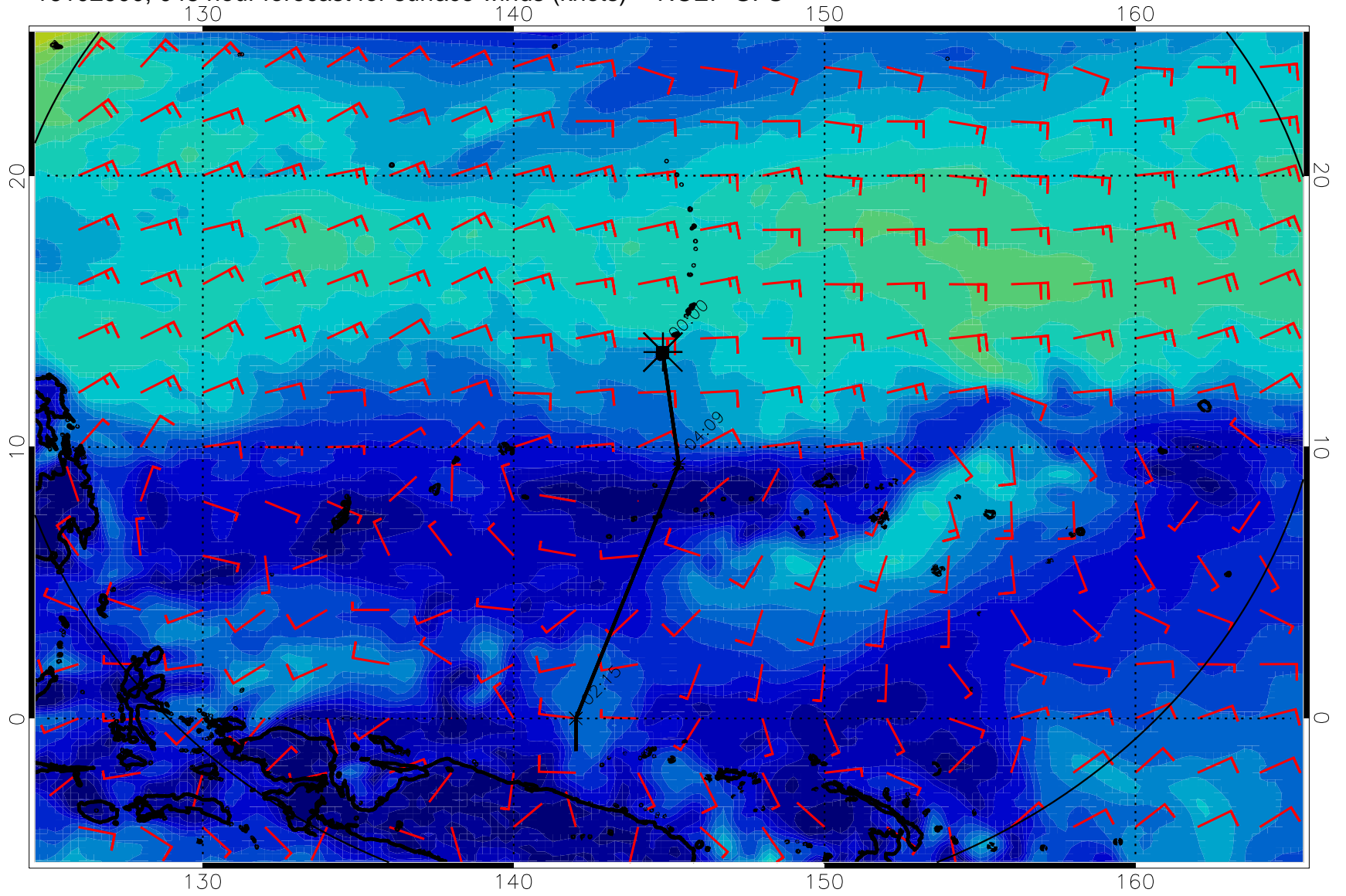
16102900, 048 hour forecast for surface winds (knots) -- NCEP GFS
