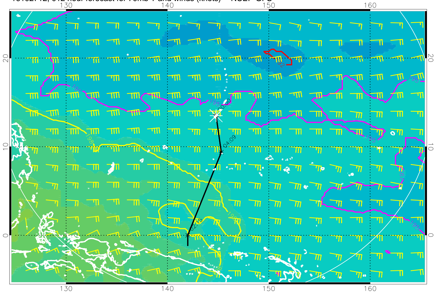
16102712, 012 hour forecast for 70mb T and winds (knots) -- NCEP GFS
