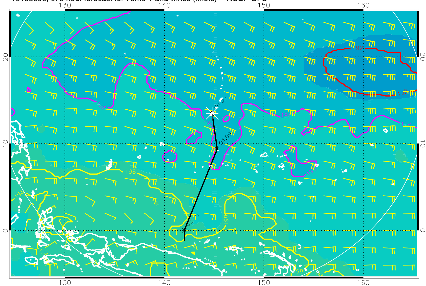
16103006, 078 hour forecast for 70mb T and winds (knots) -- NCEP GFS
