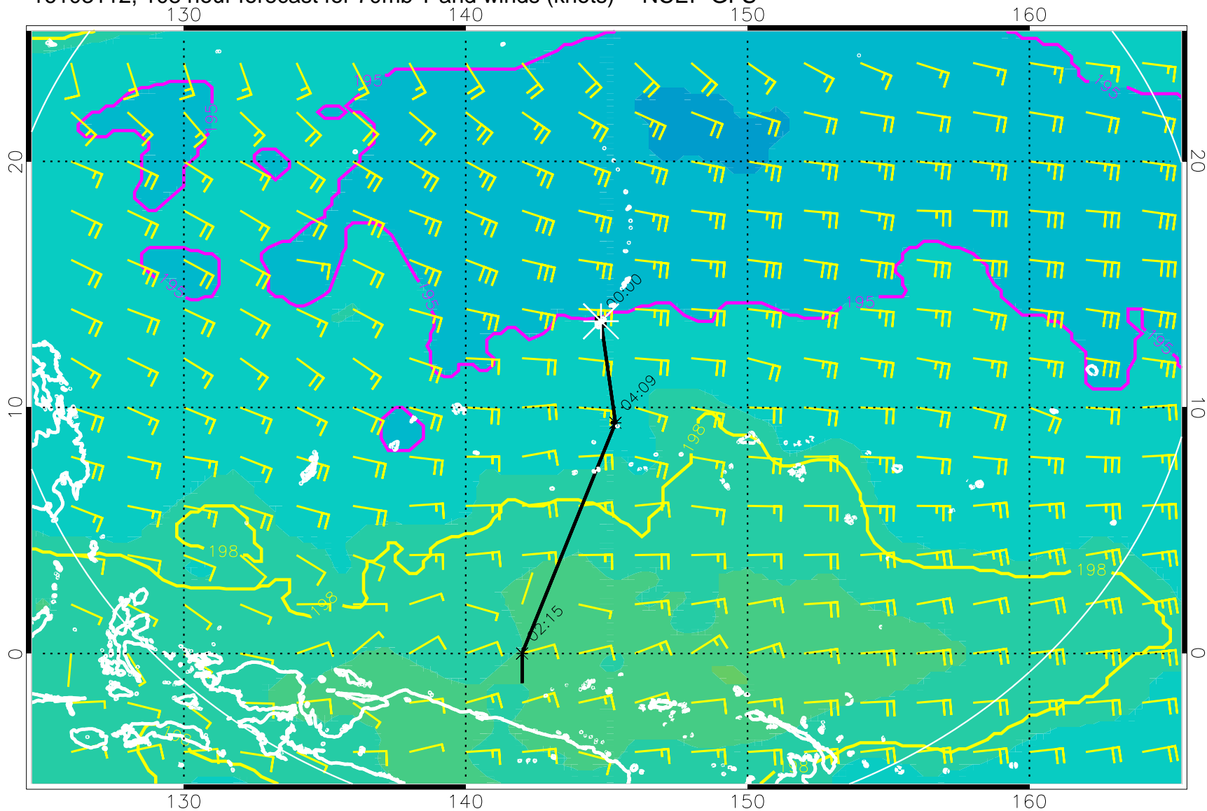
16103112, 108 hour forecast for 70mb T and winds (knots) -- NCEP GFS
