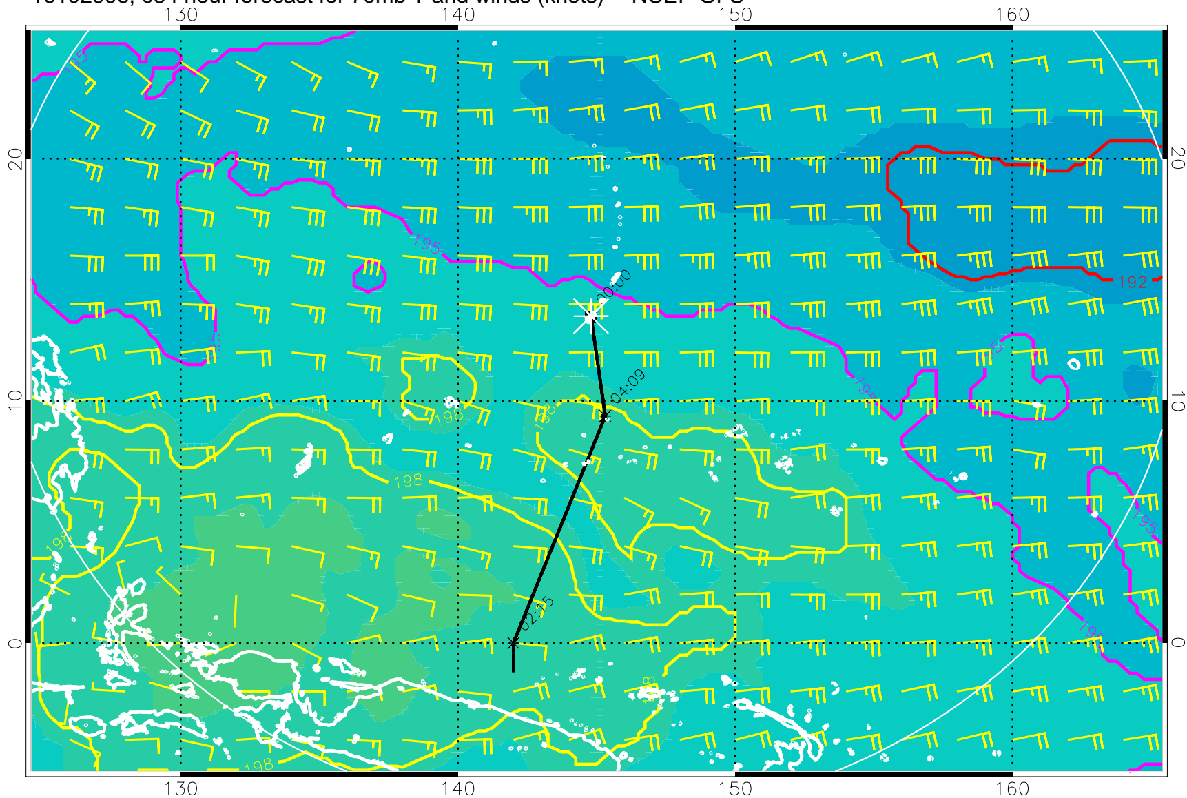
16102906, 054 hour forecast for 70mb T and winds (knots) -- NCEP GFS
