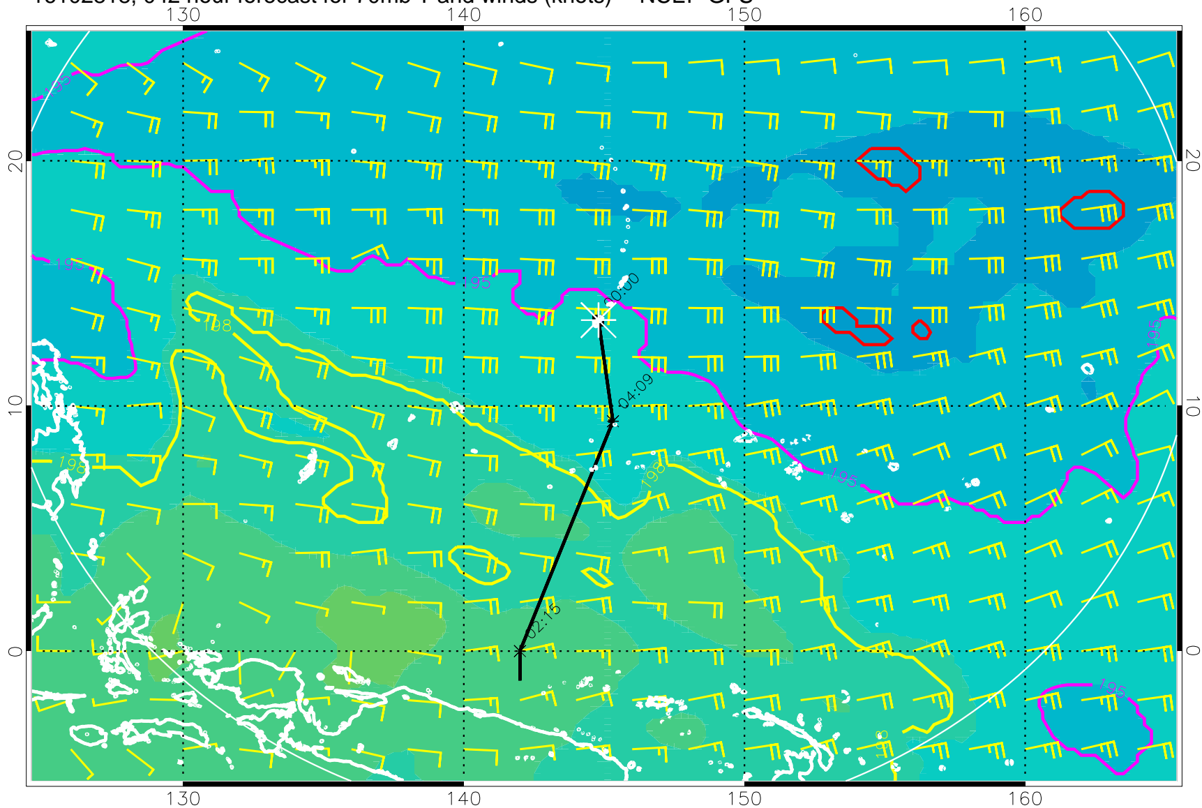
16102818, 042 hour forecast for 70mb T and winds (knots) -- NCEP GFS
