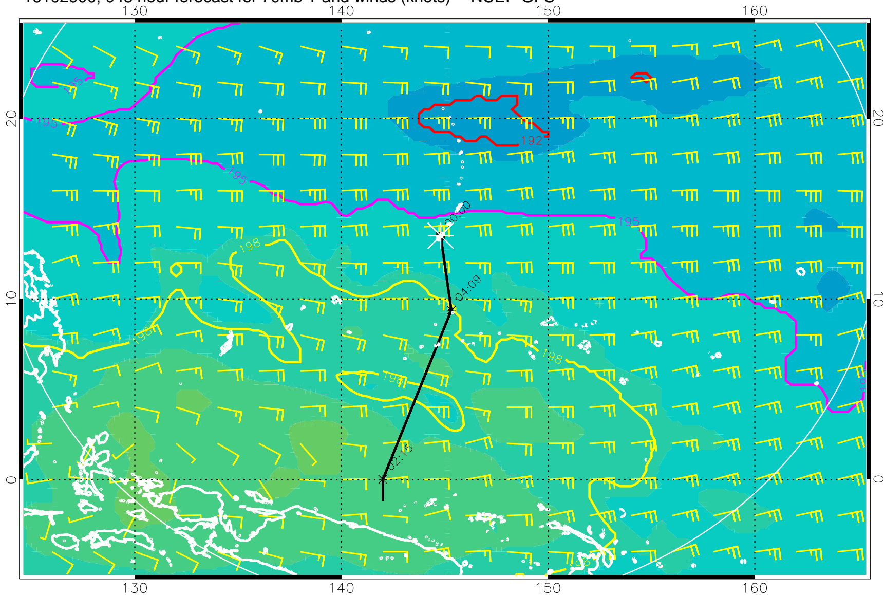
16102900, 048 hour forecast for 70mb T and winds (knots) -- NCEP GFS
