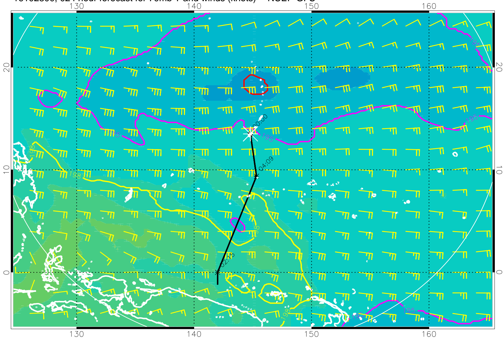
16102800, 024 hour forecast for 70mb T and winds (knots) -- NCEP GFS
