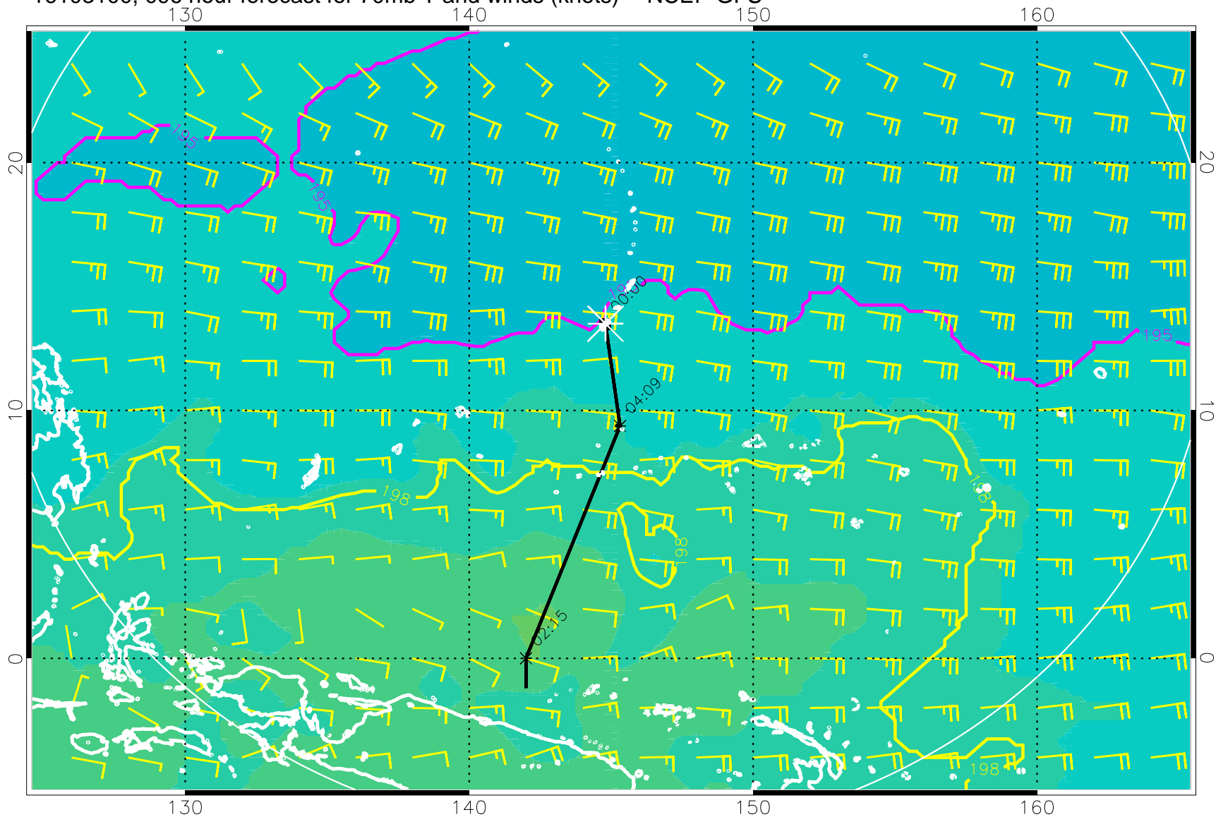
16103100, 096 hour forecast for 70mb T and winds (knots) -- NCEP GFS
