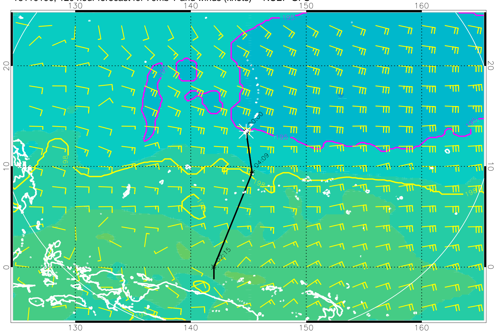
16110100, 120 hour forecast for 70mb T and winds (knots) -- NCEP GFS
