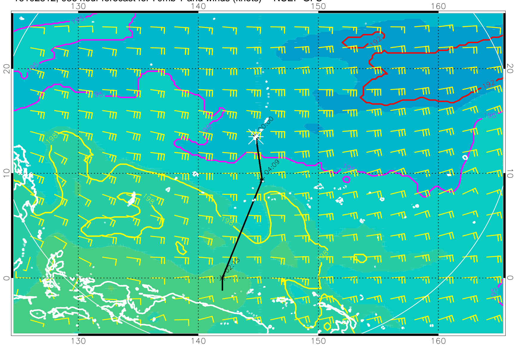
16102812, 036 hour forecast for 70mb T and winds (knots) -- NCEP GFS
