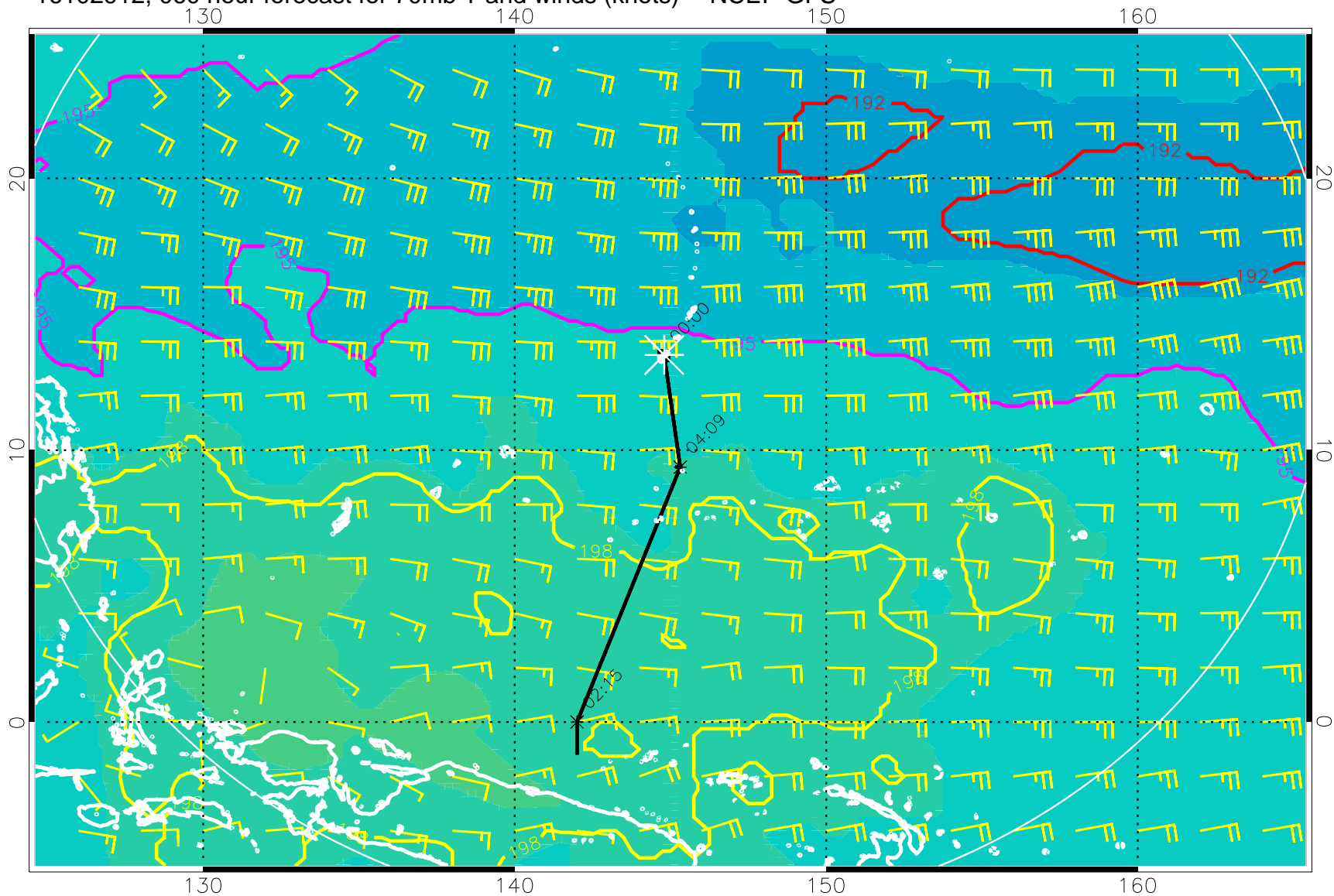
16102912, 060 hour forecast for 70mb T and winds (knots) -- NCEP GFS
