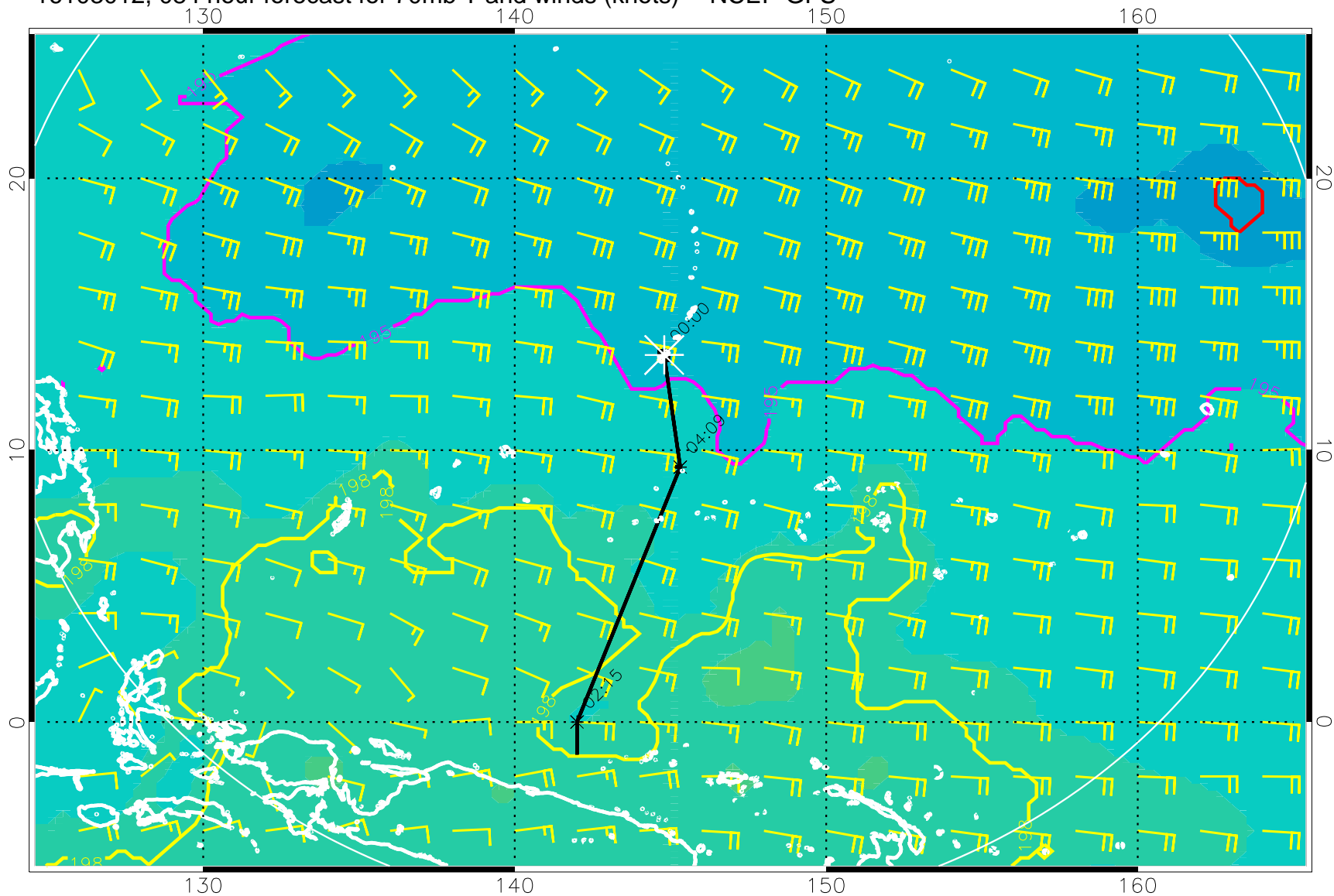
16103012, 084 hour forecast for 70mb T and winds (knots) -- NCEP GFS
