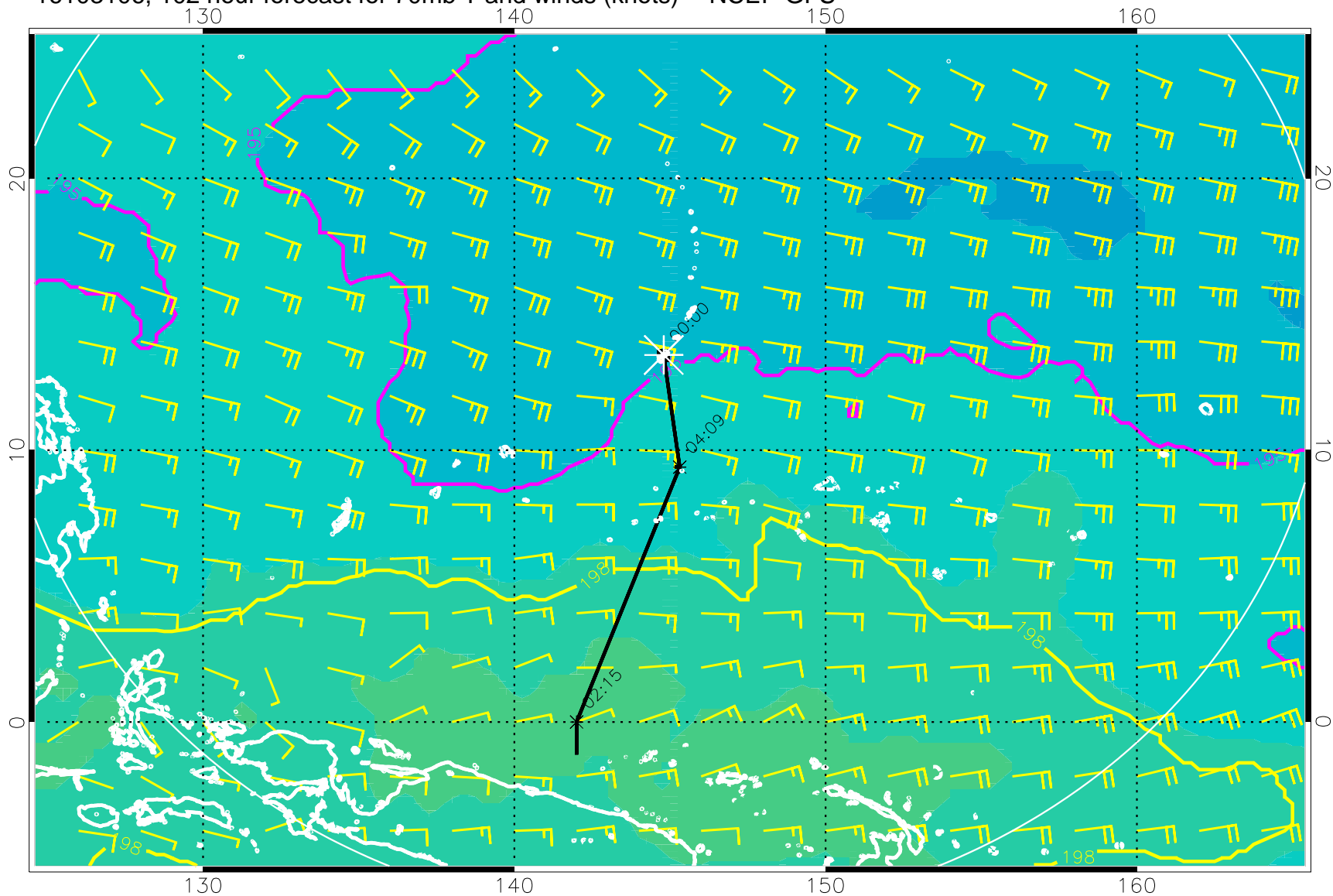
16103106, 102 hour forecast for 70mb T and winds (knots) -- NCEP GFS
