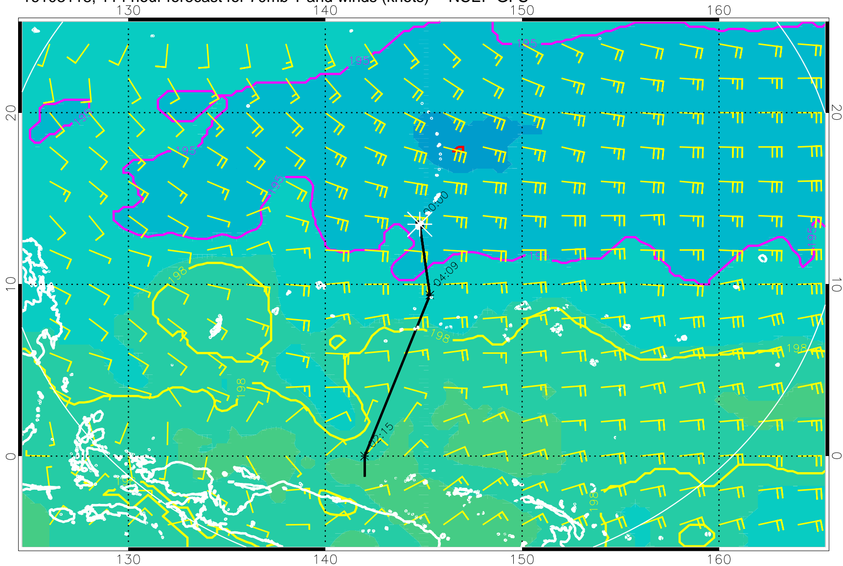
16103118, 114 hour forecast for 70mb T and winds (knots) -- NCEP GFS
