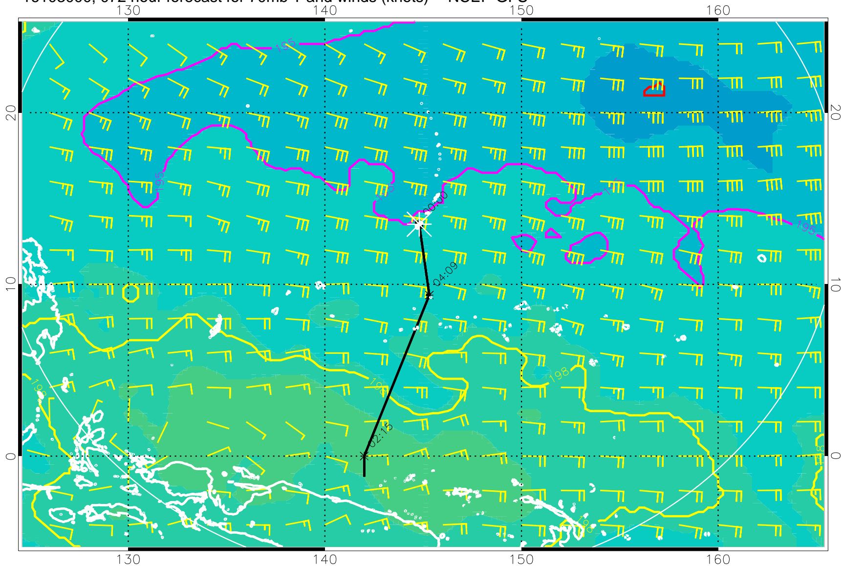
16103000, 072 hour forecast for 70mb T and winds (knots) -- NCEP GFS
