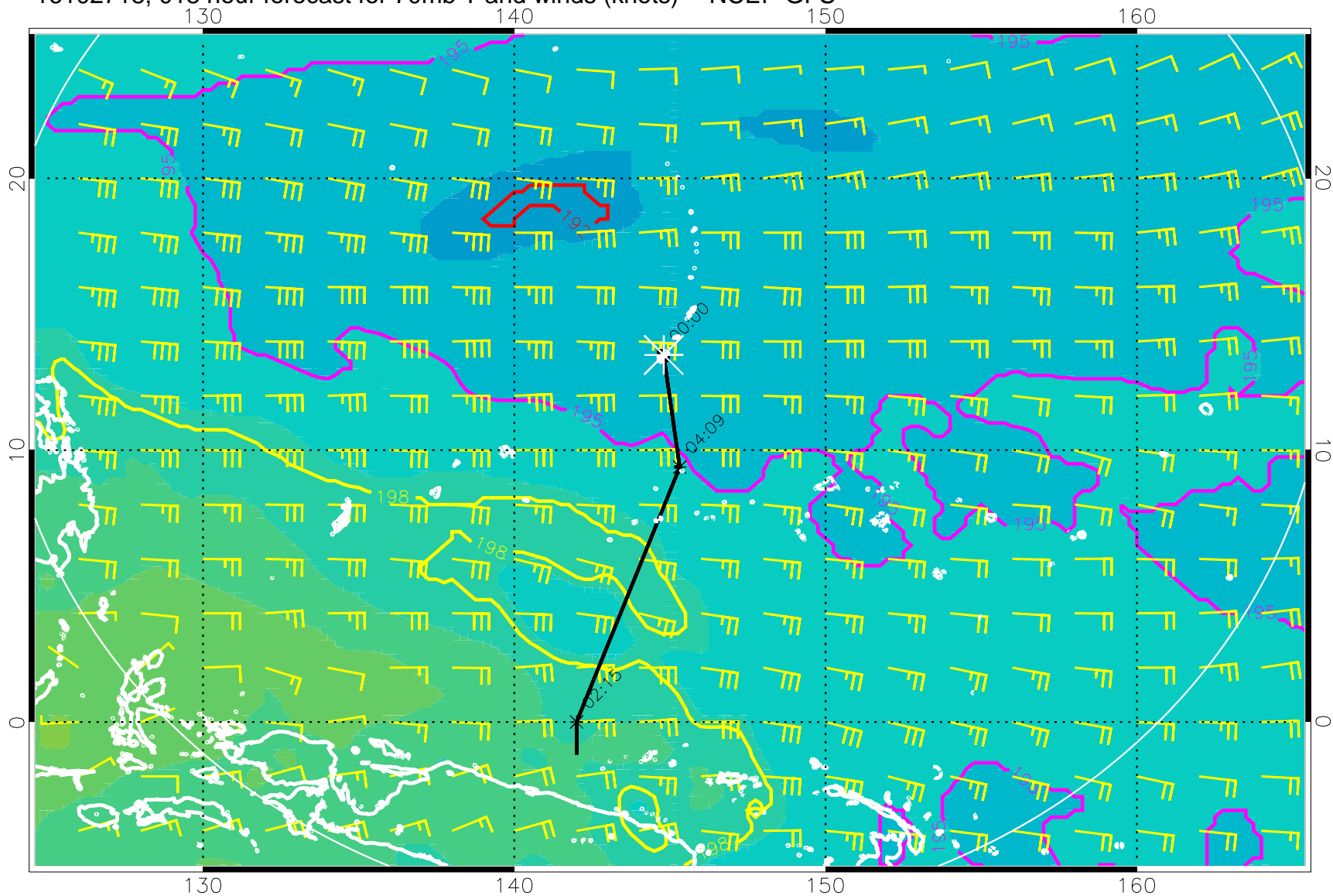
16102718, 018 hour forecast for 70mb T and winds (knots) -- NCEP GFS
