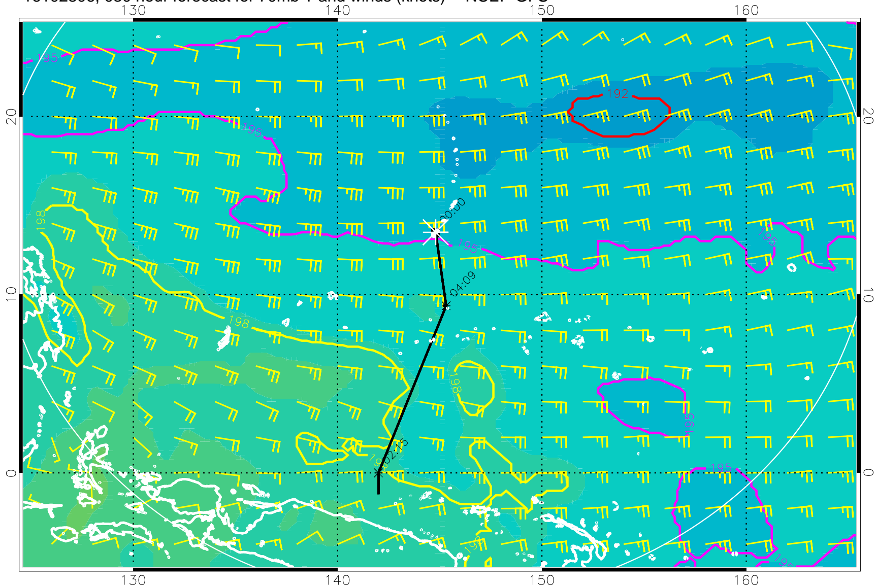
16102806, 030 hour forecast for 70mb T and winds (knots) -- NCEP GFS
