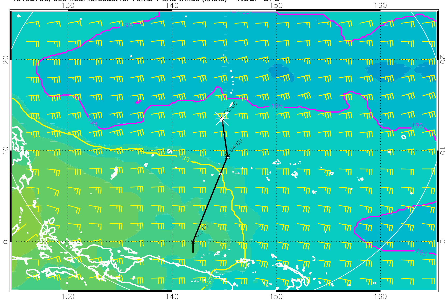
16102706, 006 hour forecast for 70mb T and winds (knots) -- NCEP GFS
