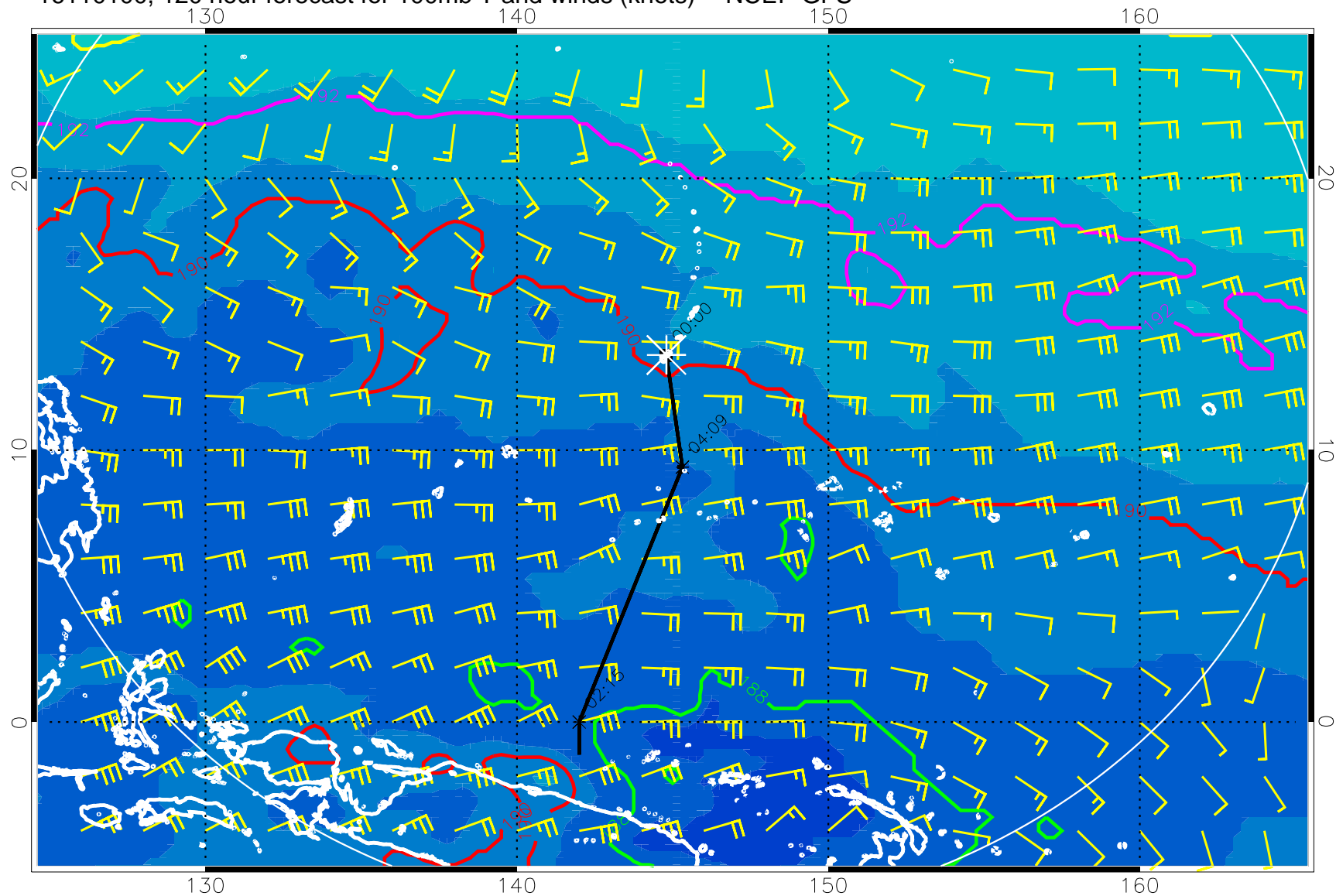
16110100, 120 hour forecast for 100mb T and winds (knots) -- NCEP GFS
