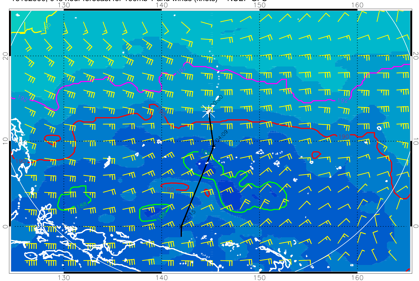
16102900, 048 hour forecast for 100mb T and winds (knots) -- NCEP GFS
