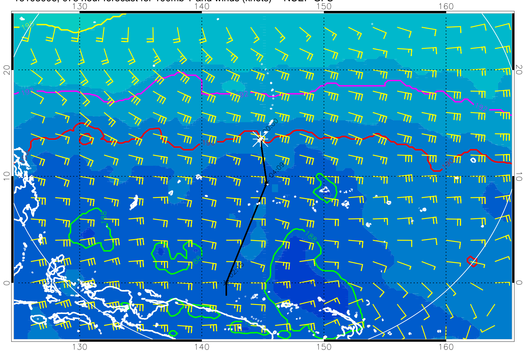
16103006, 078 hour forecast for 100mb T and winds (knots) -- NCEP GFS
