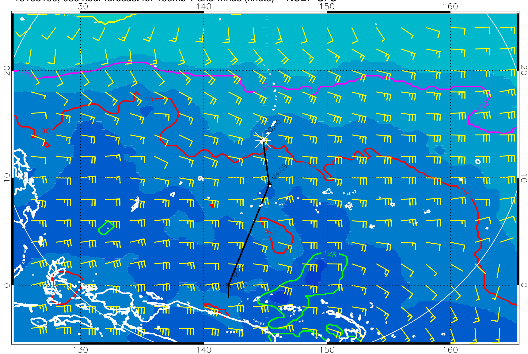
16103100, 096 hour forecast for 100mb T and winds (knots) -- NCEP GFS
