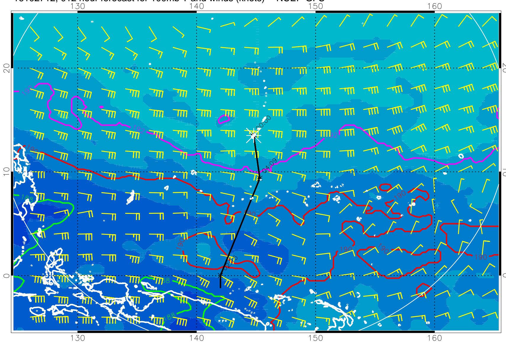
16102712, 012 hour forecast for 100mb T and winds (knots) -- NCEP GFS
