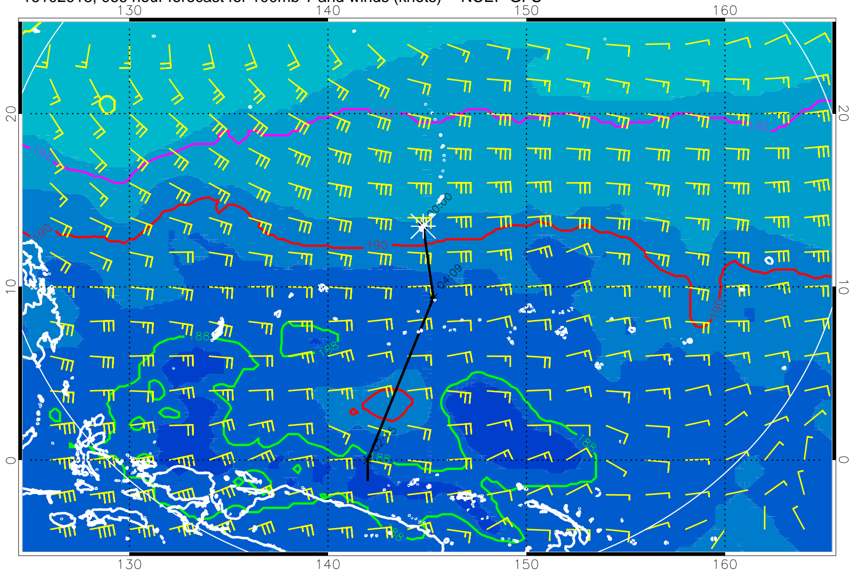
16102918, 066 hour forecast for 100mb T and winds (knots) -- NCEP GFS
