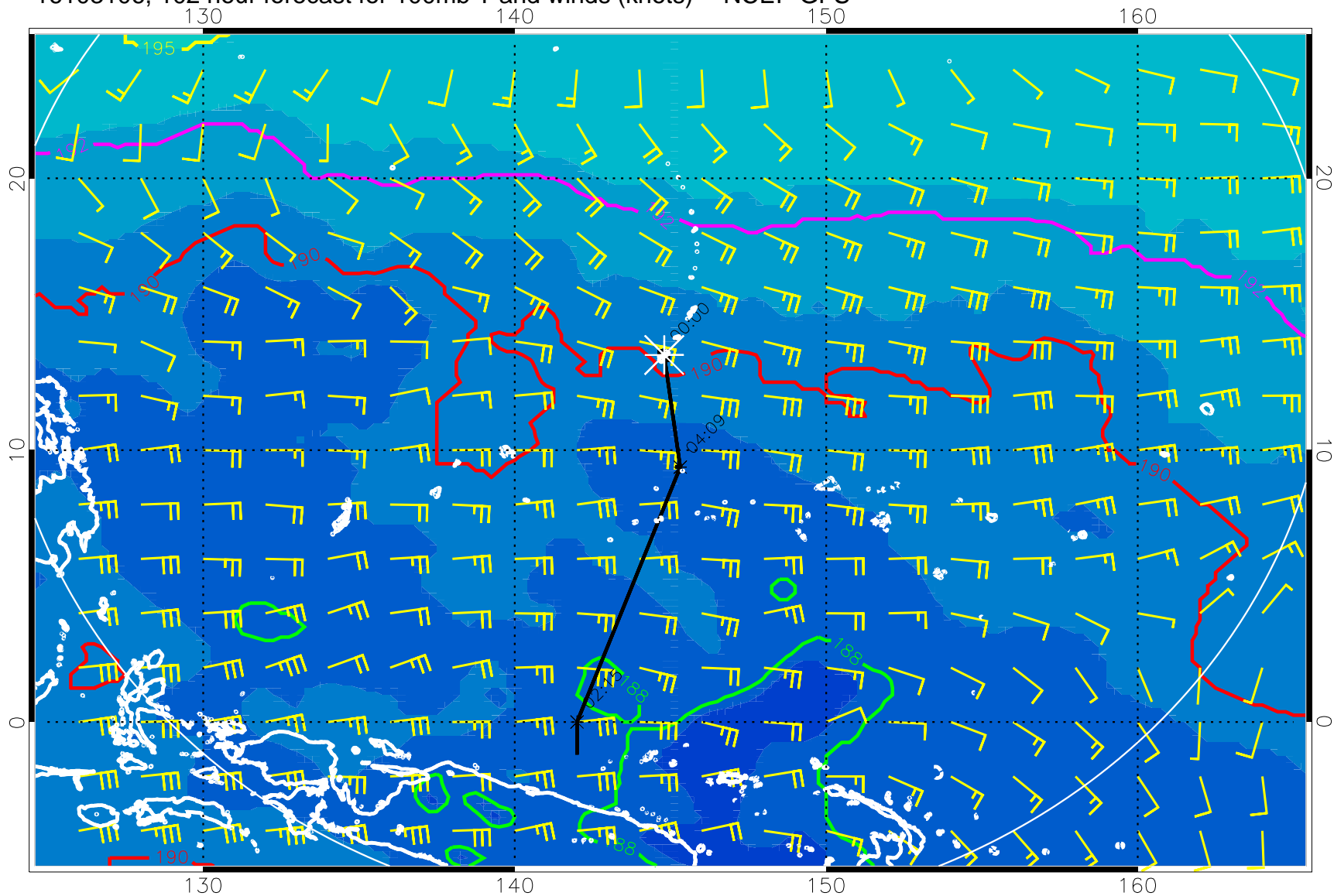
16103106, 102 hour forecast for 100mb T and winds (knots) -- NCEP GFS
