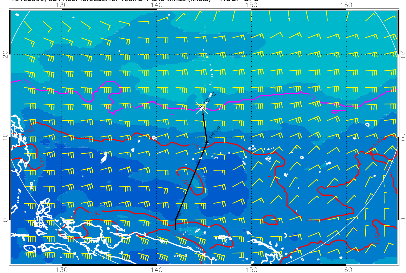
16102800, 024 hour forecast for 100mb T and winds (knots) -- NCEP GFS
