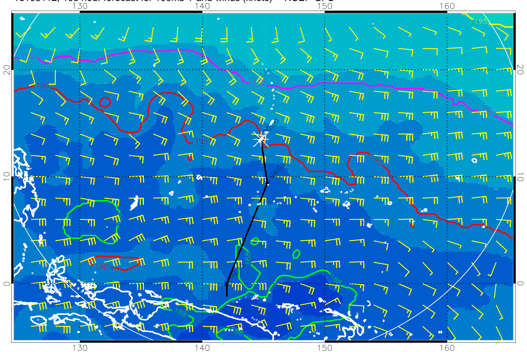
16103112, 108 hour forecast for 100mb T and winds (knots) -- NCEP GFS
