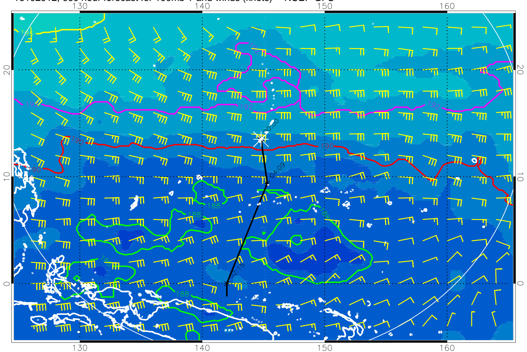
16102912, 060 hour forecast for 100mb T and winds (knots) -- NCEP GFS
