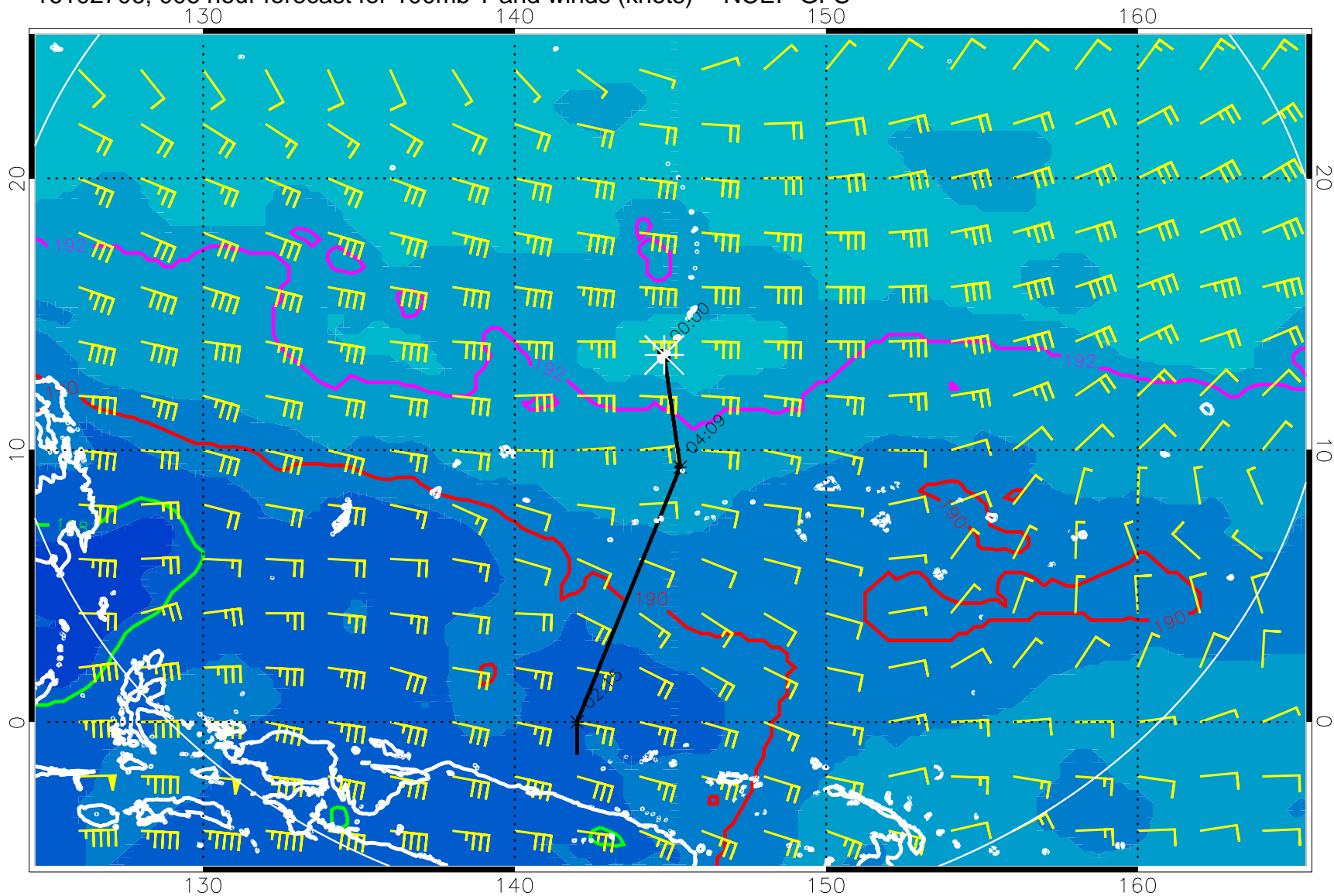
16102706, 006 hour forecast for 100mb T and winds (knots) -- NCEP GFS
