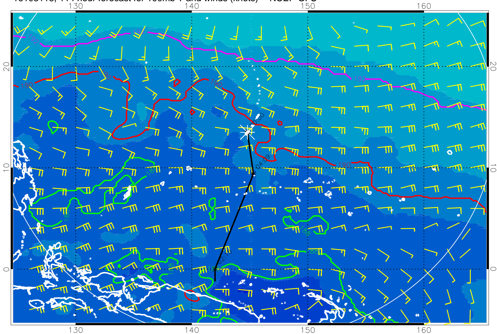
16103118, 114 hour forecast for 100mb T and winds (knots) -- NCEP GFS
