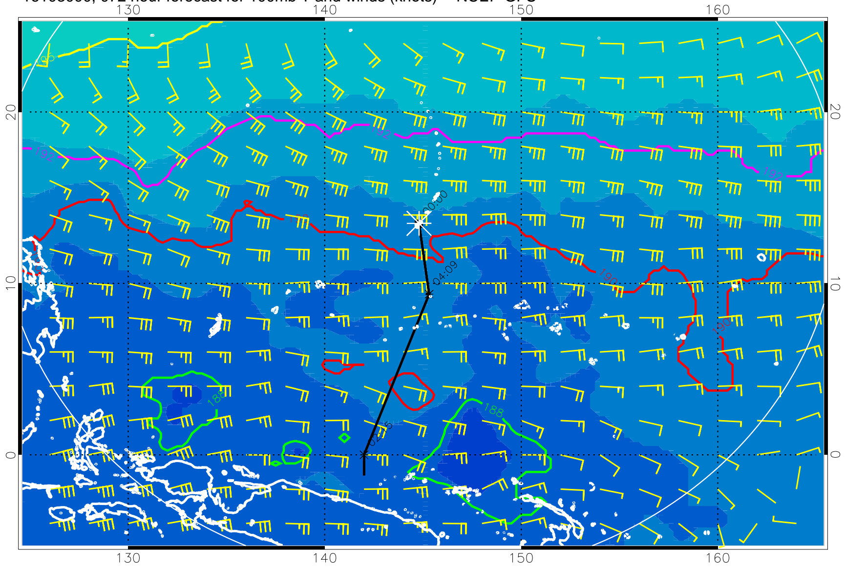
16103000, 072 hour forecast for 100mb T and winds (knots) -- NCEP GFS
