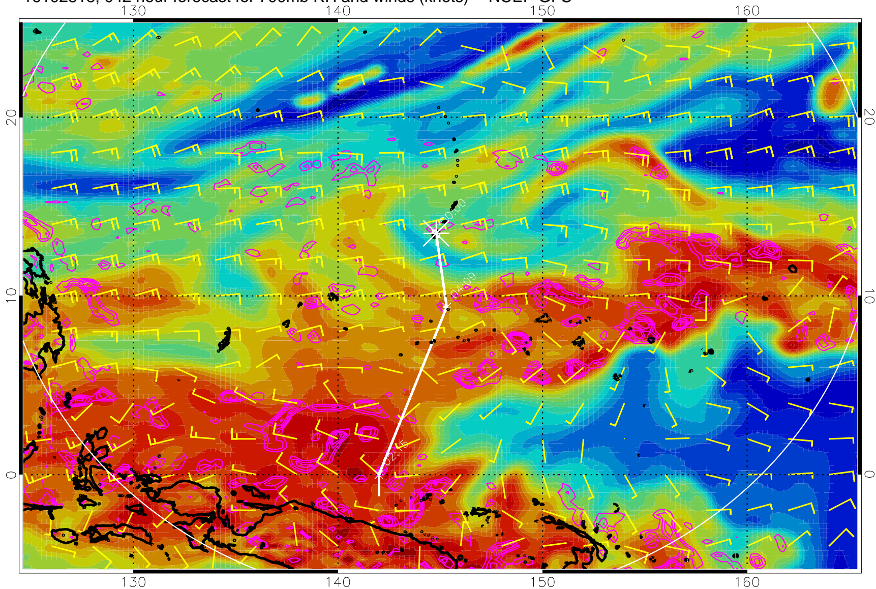
16102818, 042 hour forecast for 700mb RH and winds (knots) -- NCEP GFS
