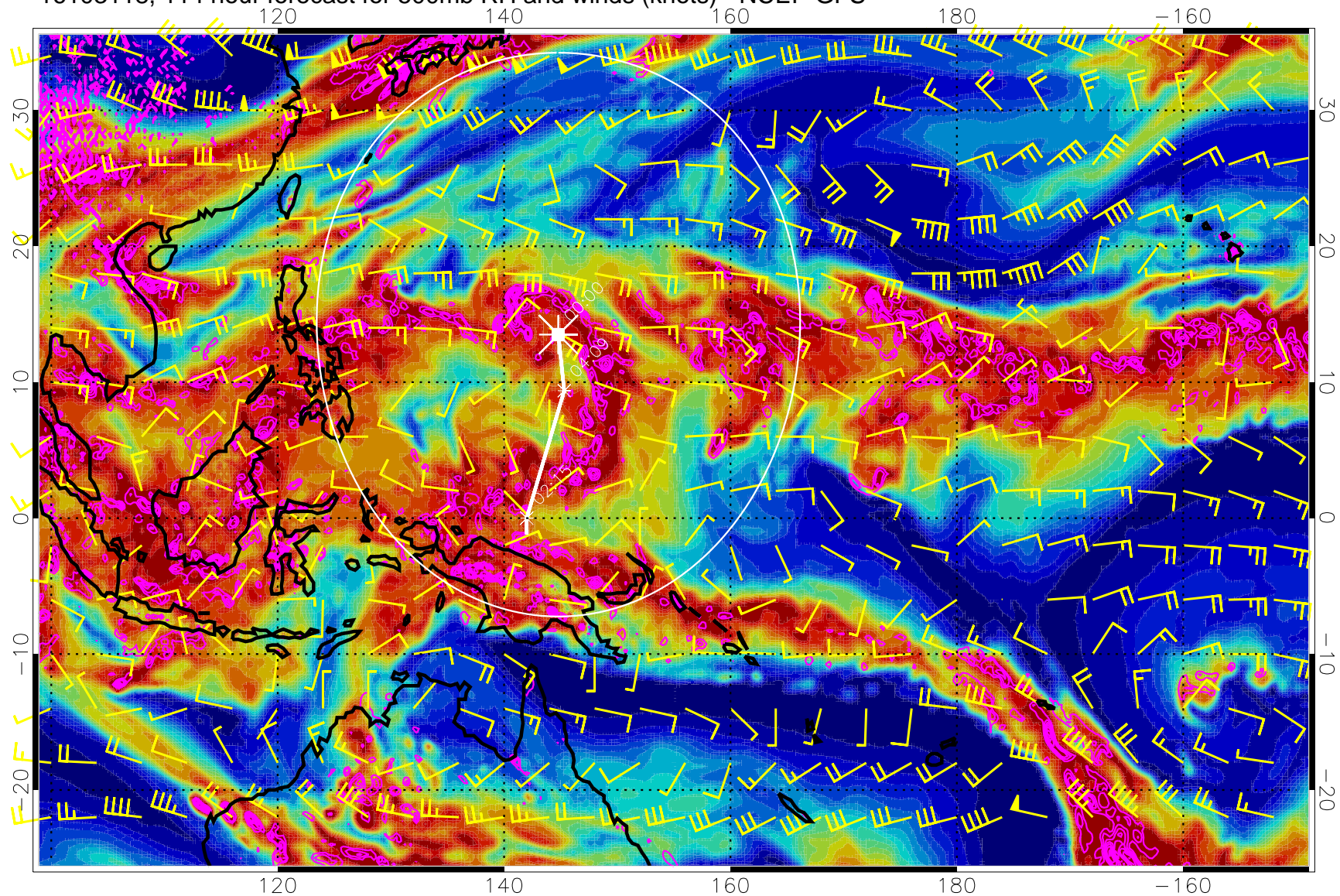
16103118, 114 hour forecast for 500mb RH and winds (knots) - NCEP GFS
