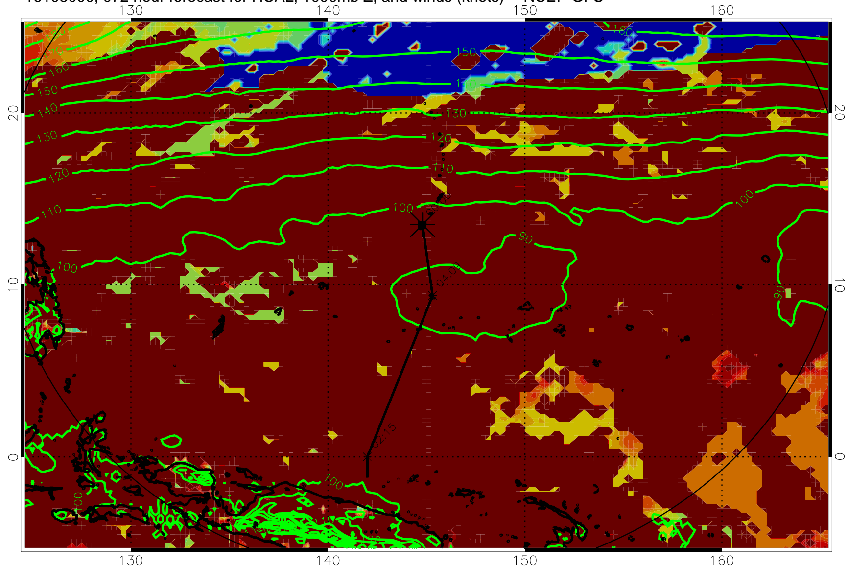
16103000, 072 hour forecast for HCAL, 1000mb Z, and winds (knots) -- NCEP GFS
