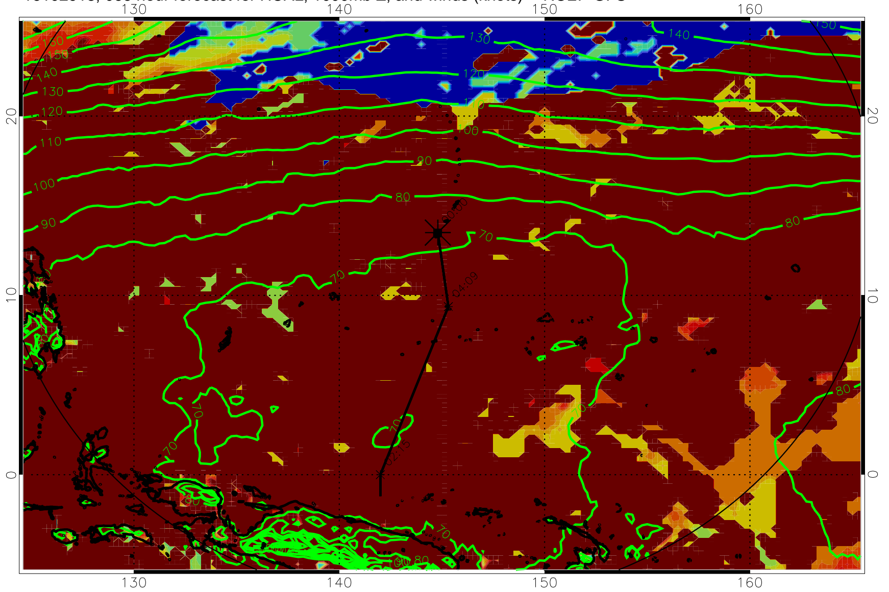
16102918, 066 hour forecast for HCAL, 1000mb Z, and winds (knots) -- NCEP GFS
