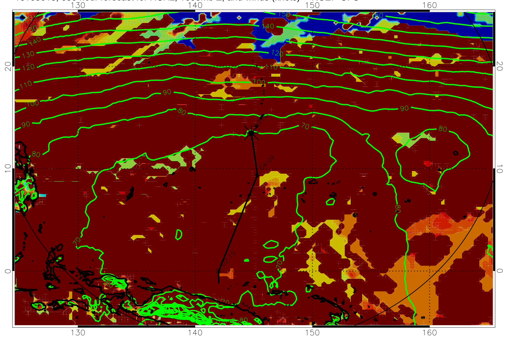
16103018, 090 hour forecast for HCAL, 1000mb Z, and winds (knots) -- NCEP GFS
