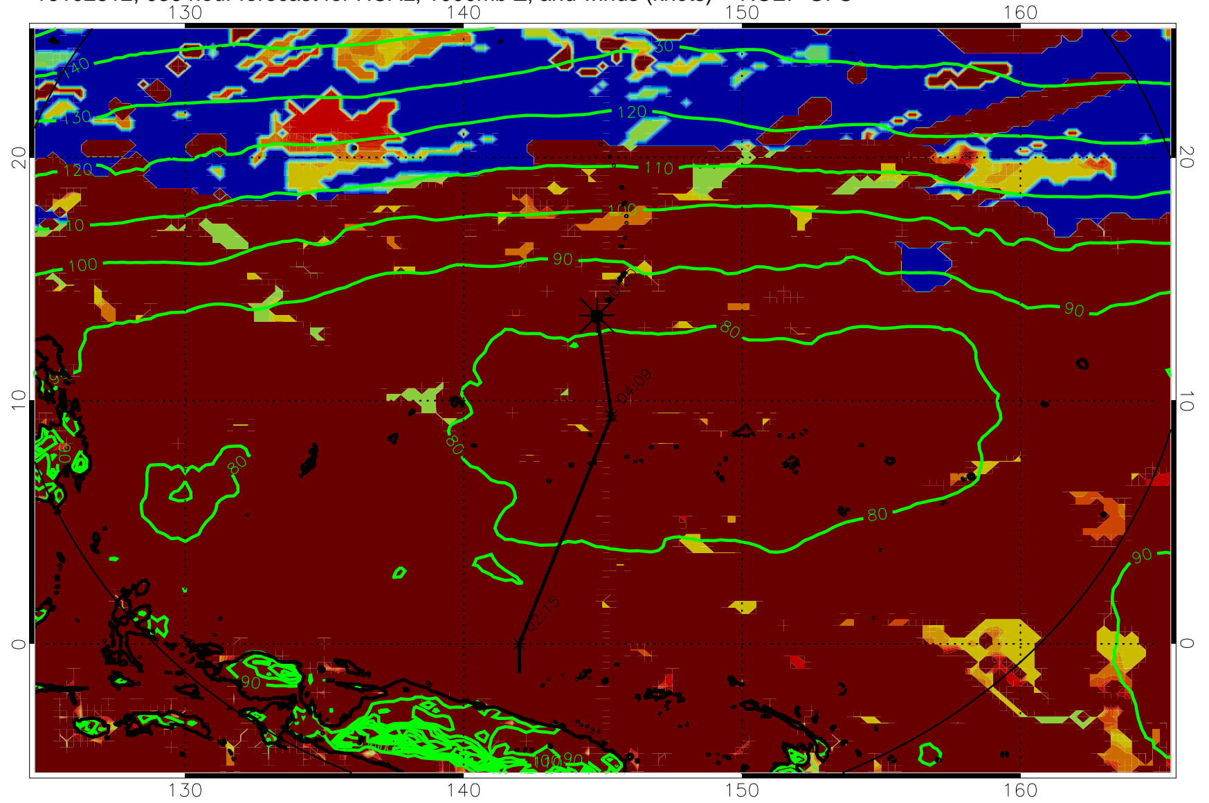
16102812, 036 hour forecast for HCAL, 1000mb Z, and winds (knots) -- NCEP GFS
