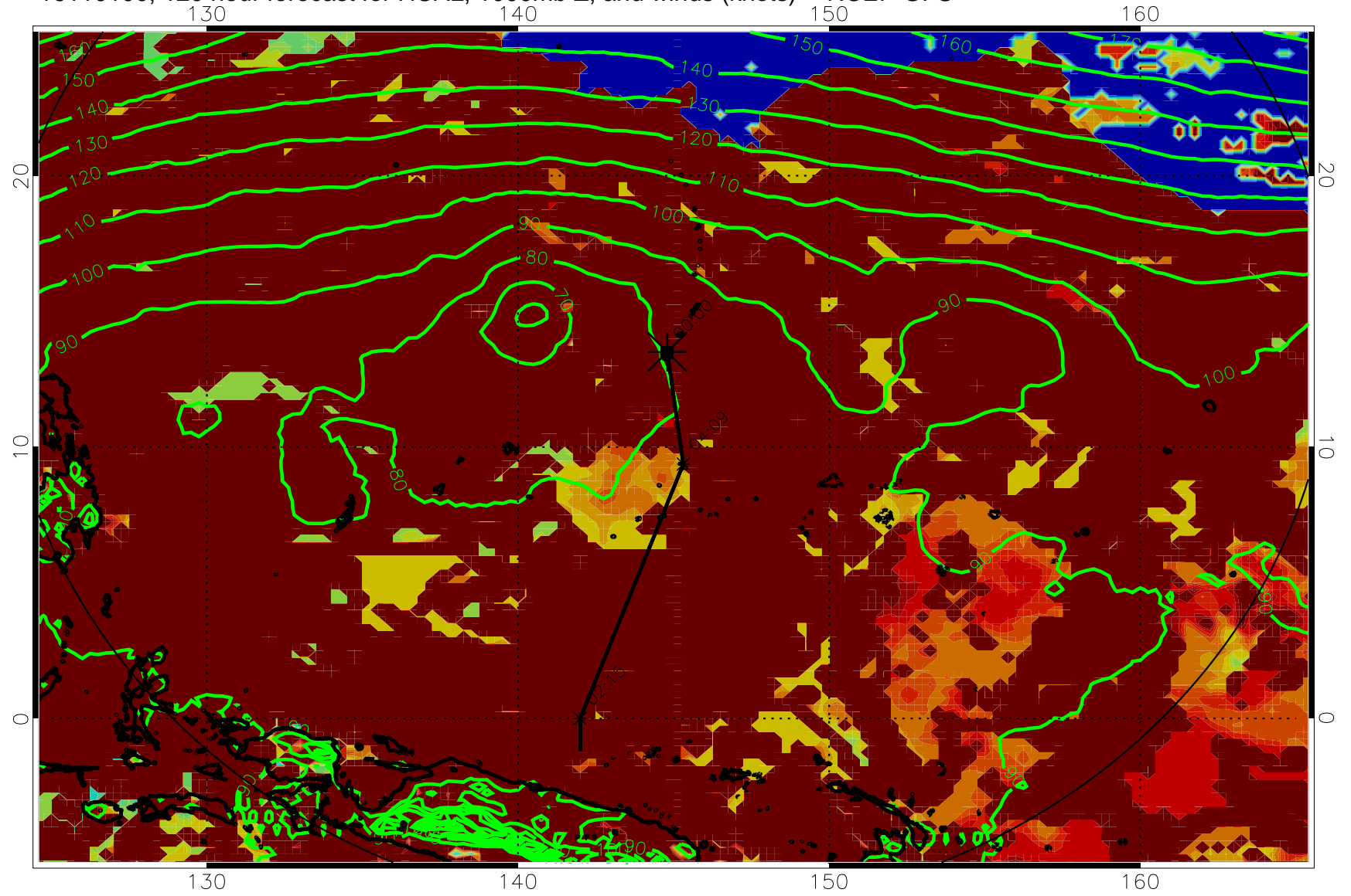
16110100, 120 hour forecast for HCAL, 1000mb Z, and winds (knots) -- NCEP GFS
