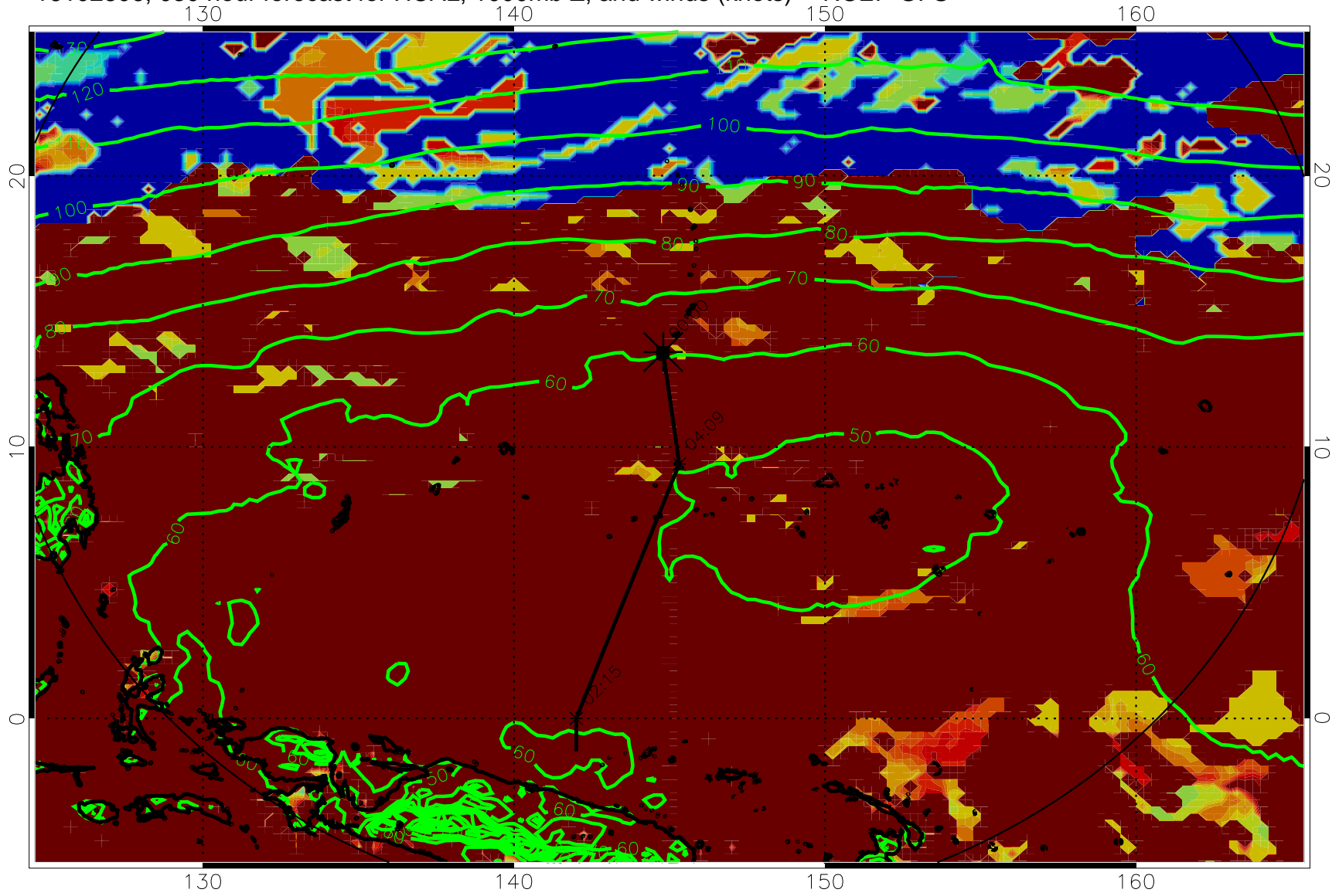
16102806, 030 hour forecast for HCAL, 1000mb Z, and winds (knots) -- NCEP GFS
