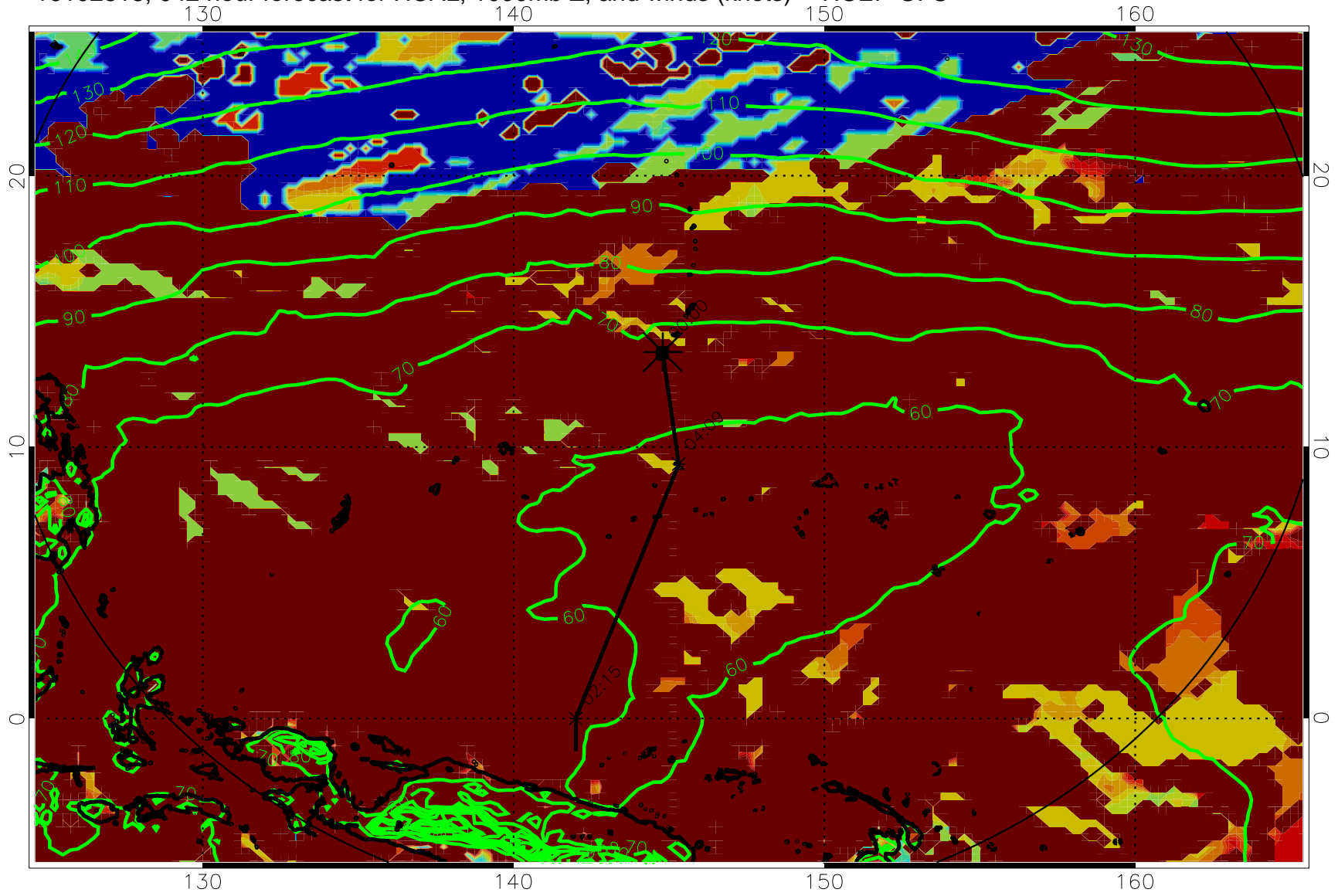
16102818, 042 hour forecast for HCAL, 1000mb Z, and winds (knots) -- NCEP GFS
