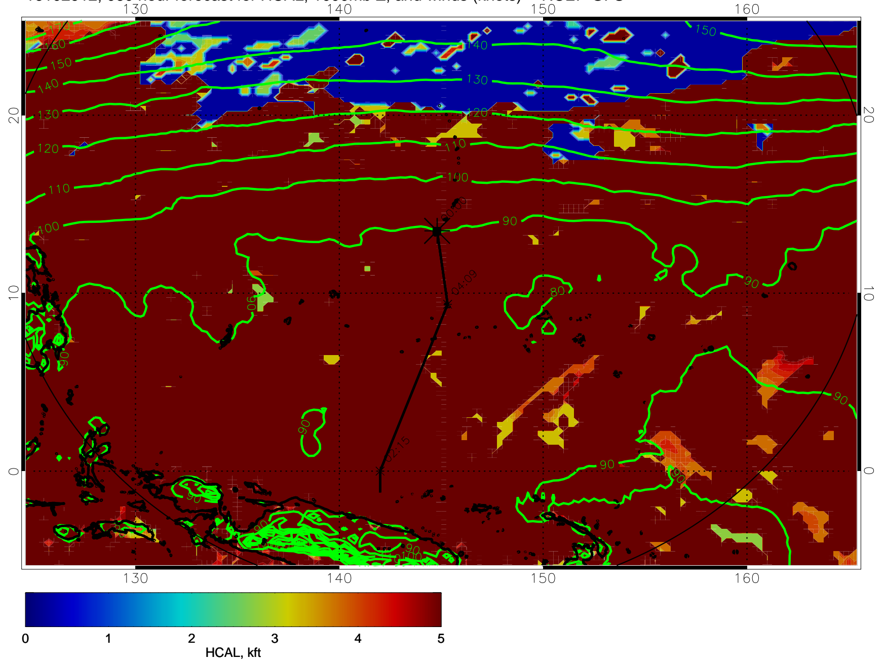
16102912, 060 hour forecast for HCAL, 1000mb Z, and winds (knots) -- NCEP GFS
