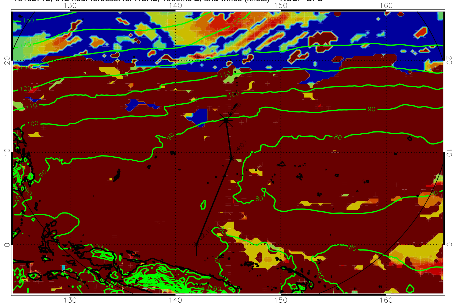
16102712, 012 hour forecast for HCAL, 1000mb Z, and winds (knots) -- NCEP GFS
