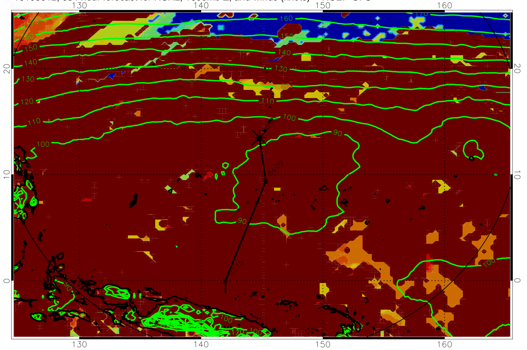
16103012, 084 hour forecast for HCAL, 1000mb Z, and winds (knots) -- NCEP GFS
