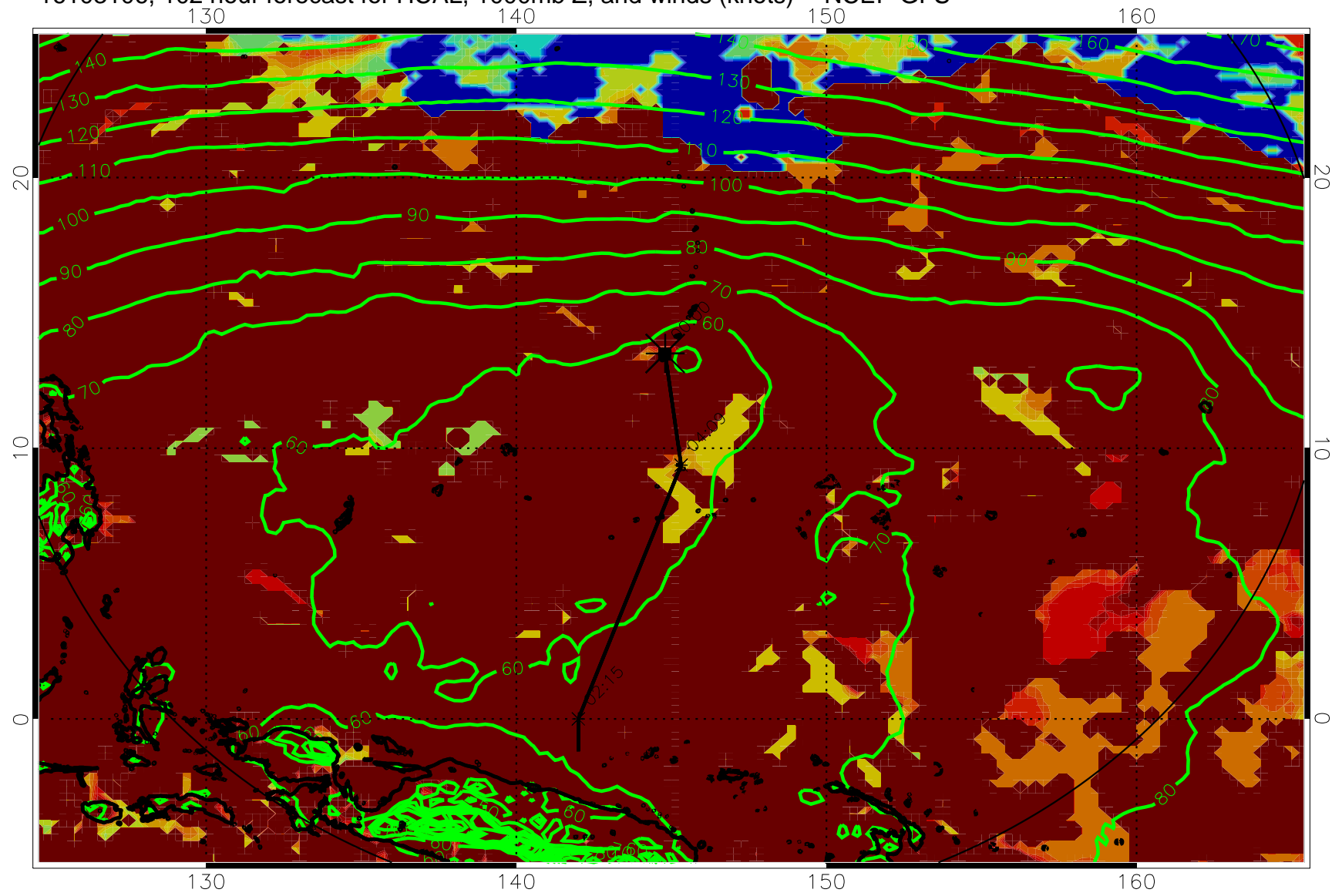
16103106, 102 hour forecast for HCAL, 1000mb Z, and winds (knots) -- NCEP GFS
