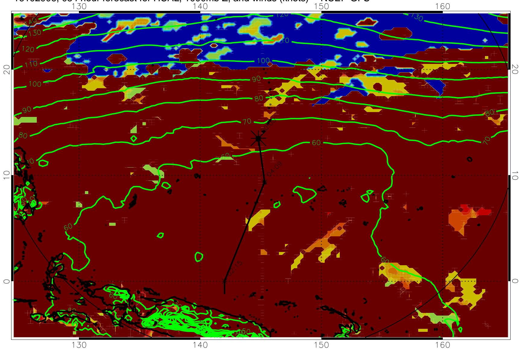
16102906, 054 hour forecast for HCAL, 1000mb Z, and winds (knots) -- NCEP GFS
