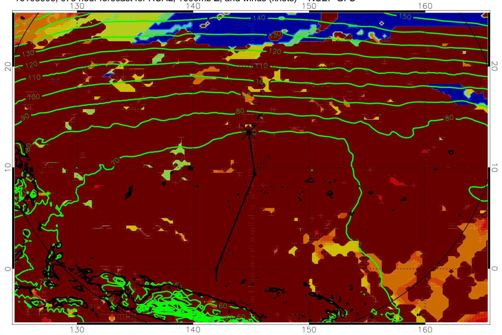
16103006, 078 hour forecast for HCAL, 1000mb Z, and winds (knots) -- NCEP GFS
