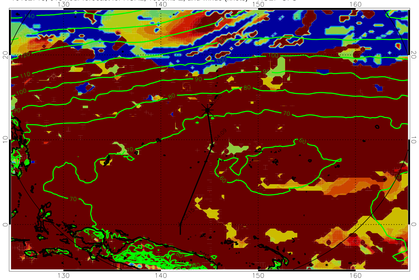
16102718, 018 hour forecast for HCAL, 1000mb Z, and winds (knots) -- NCEP GFS
