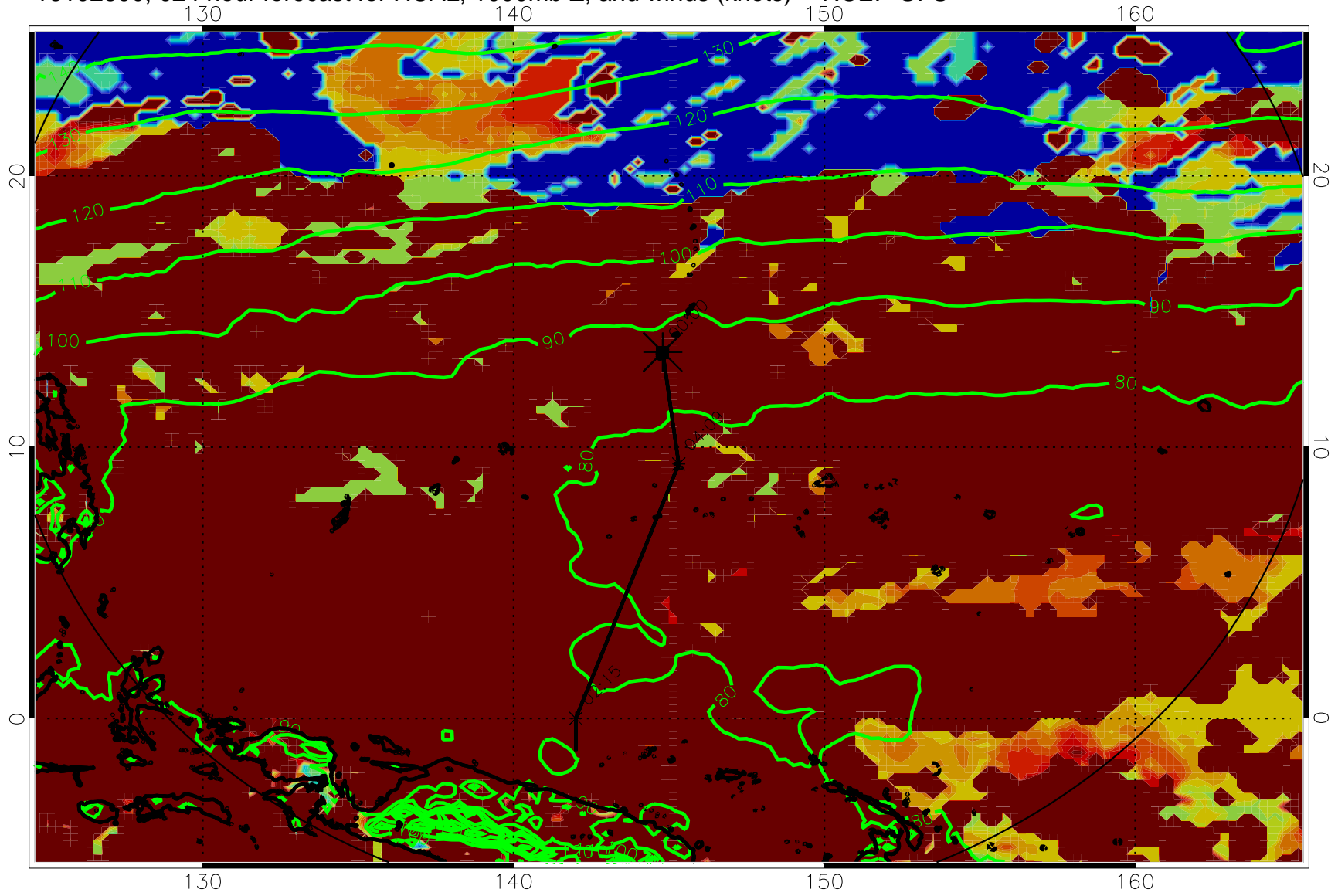
16102800, 024 hour forecast for HCAL, 1000mb Z, and winds (knots) -- NCEP GFS
