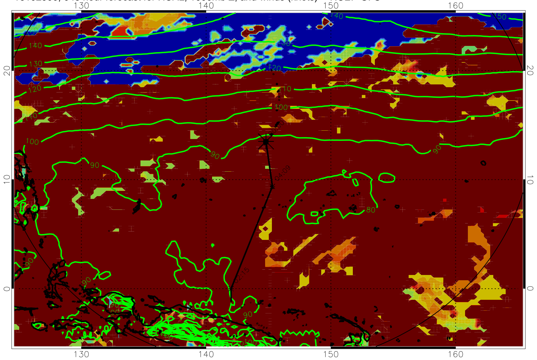
16102900, 048 hour forecast for HCAL, 1000mb Z, and winds (knots) -- NCEP GFS
