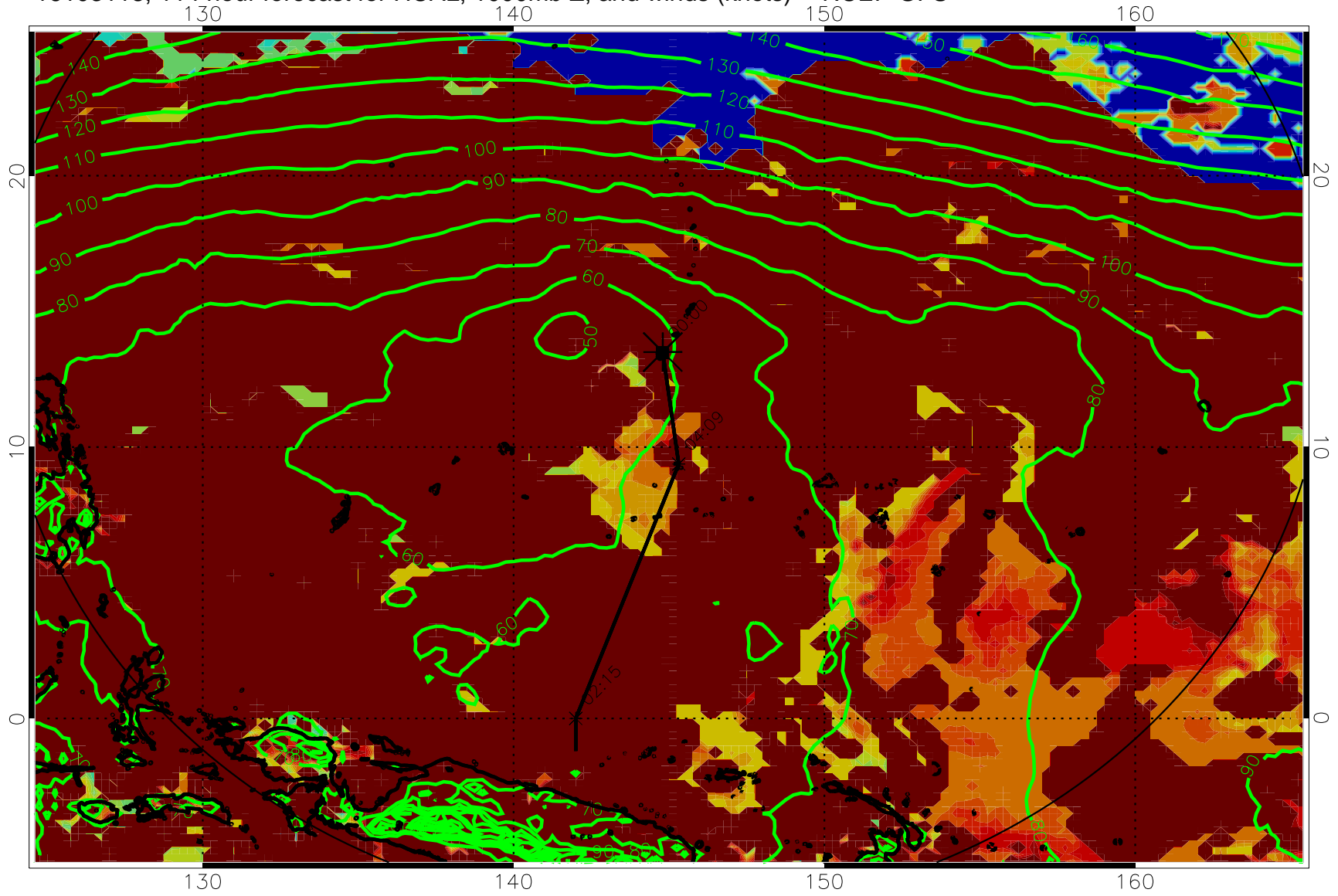
16103118, 114 hour forecast for HCAL, 1000mb Z, and winds (knots) -- NCEP GFS
