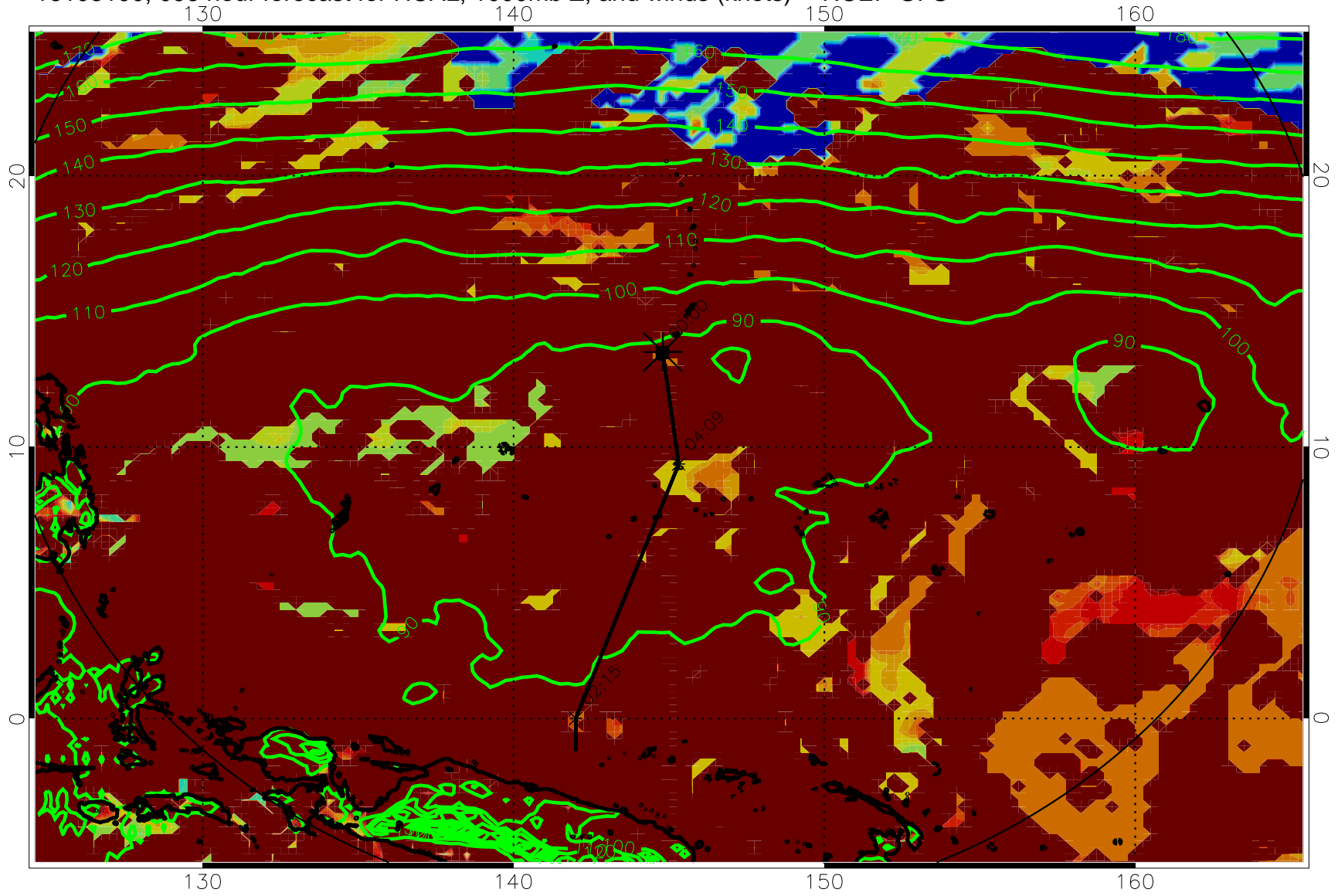
16103100, 096 hour forecast for HCAL, 1000mb Z, and winds (knots) -- NCEP GFS
