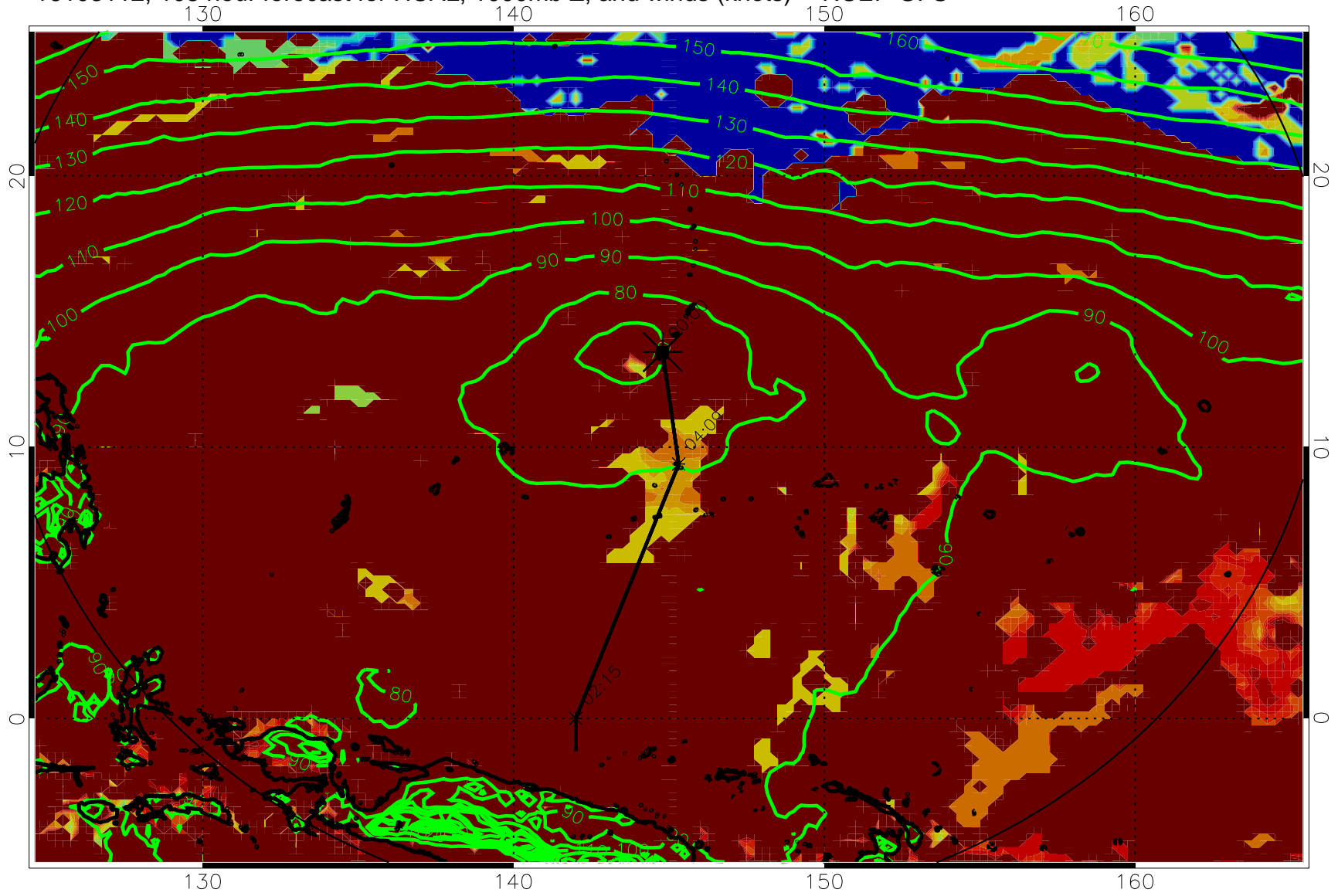
16103112, 108 hour forecast for HCAL, 1000mb Z, and winds (knots) -- NCEP GFS
