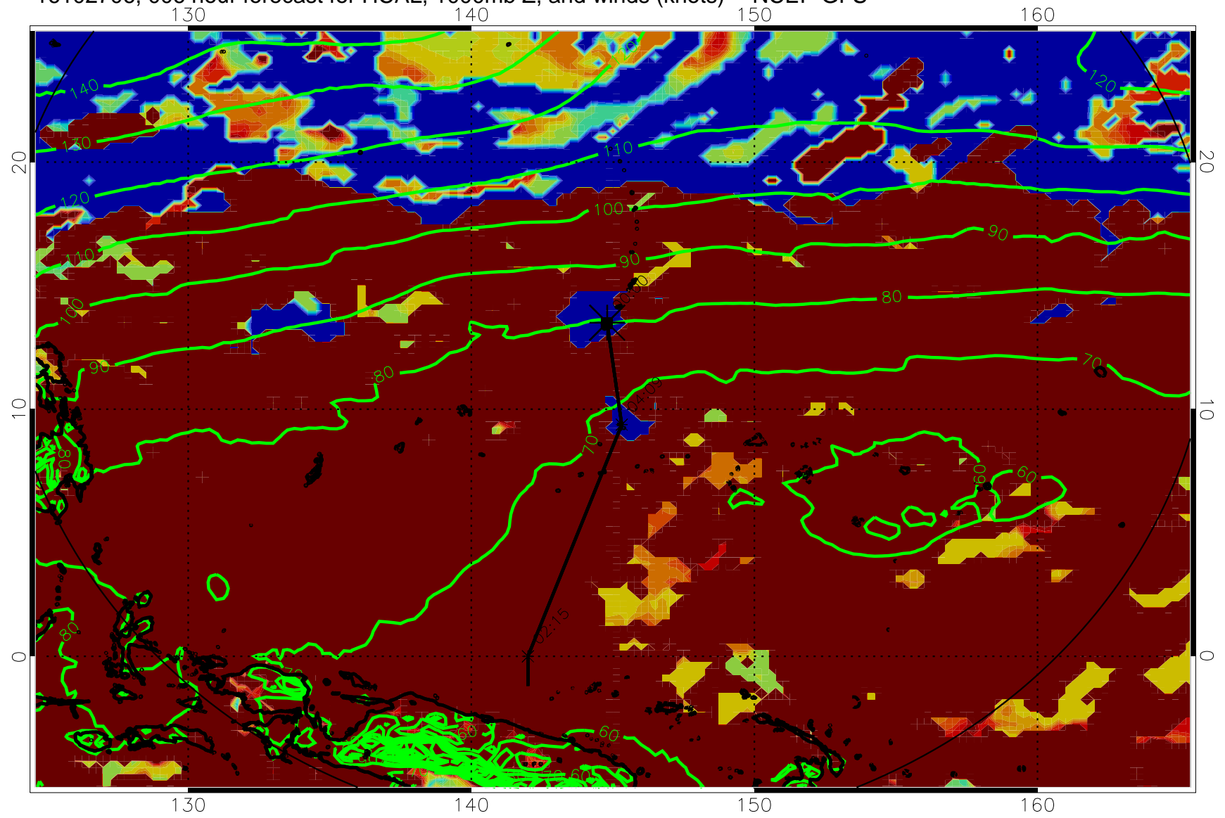
16102706, 006 hour forecast for HCAL, 1000mb Z, and winds (knots) -- NCEP GFS
