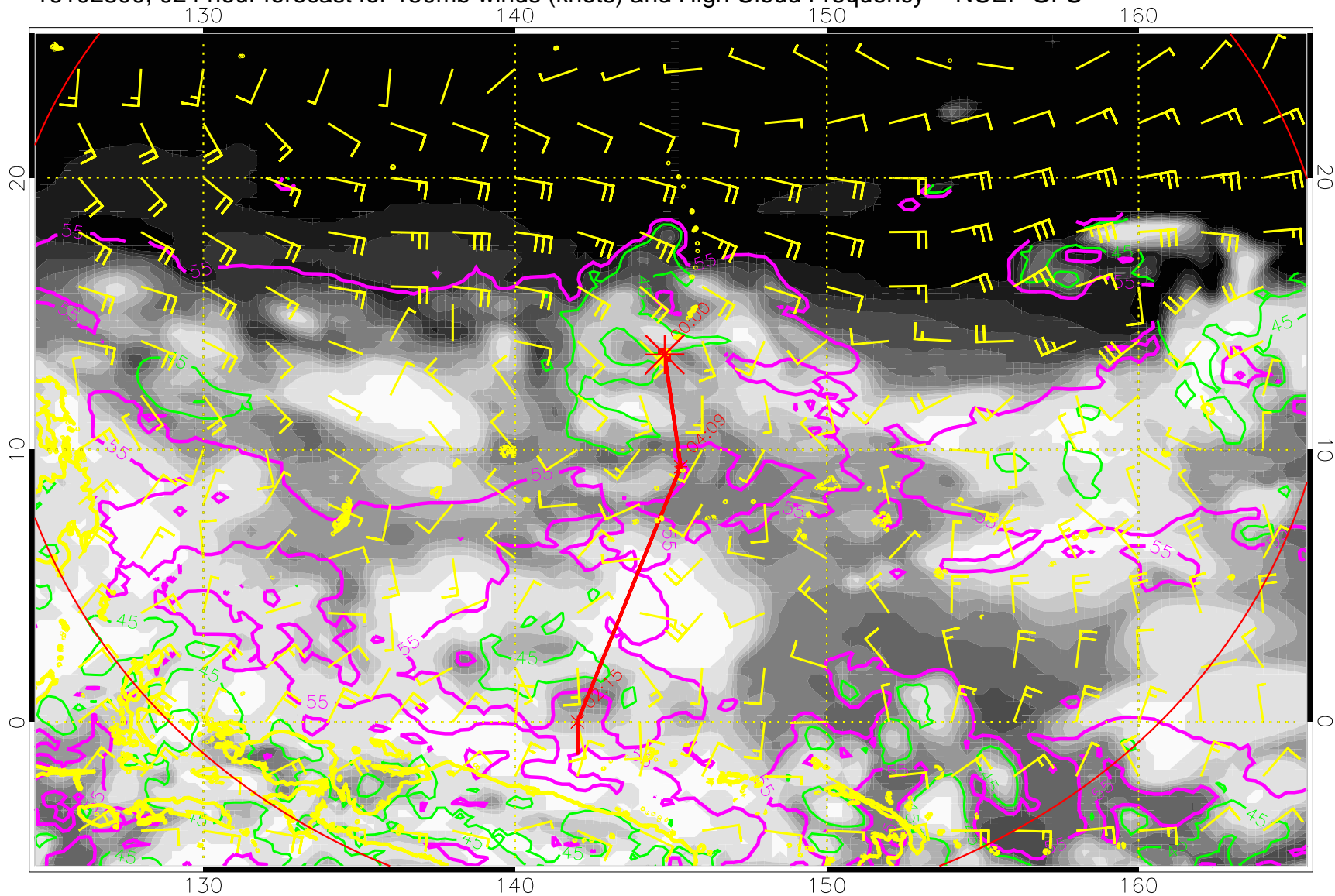
16102800, 024 hour forecast for 150mb winds (knots) and High Cloud Frequency -- NCEP GFS
