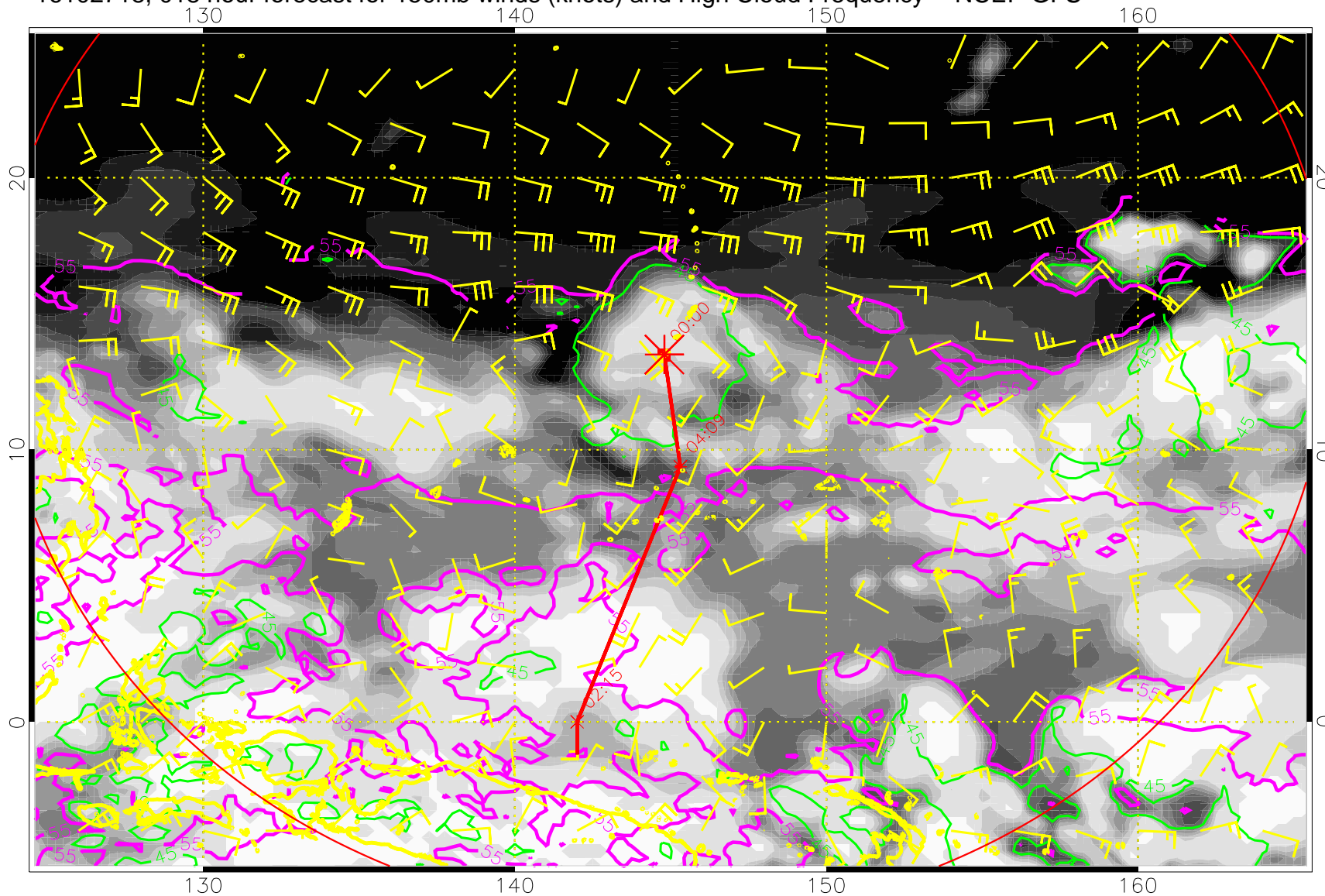
16102718, 018 hour forecast for 150mb winds (knots) and High Cloud Frequency -- NCEP GFS
