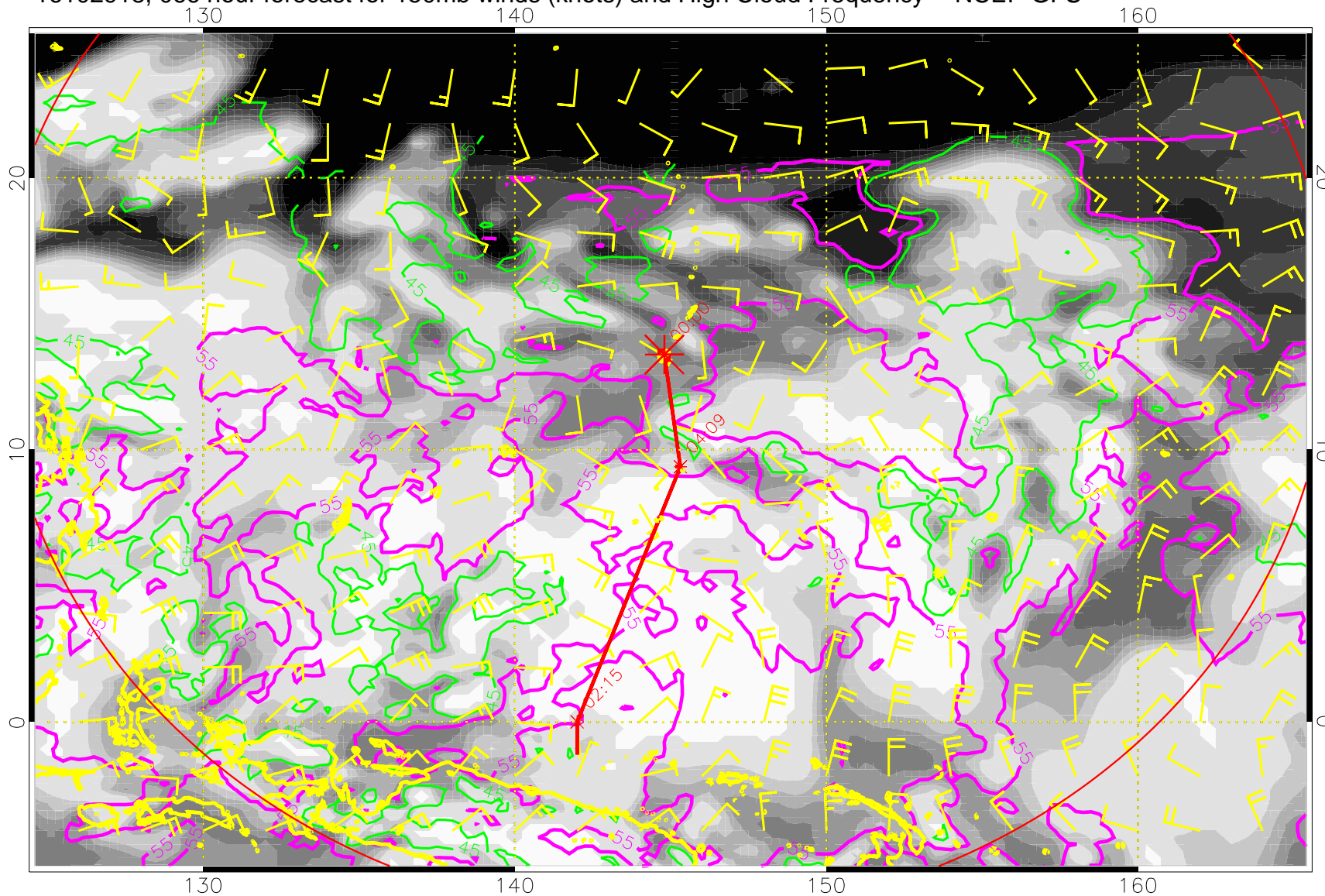
16102918, 066 hour forecast for 150mb winds (knots) and High Cloud Frequency -- NCEP GFS
