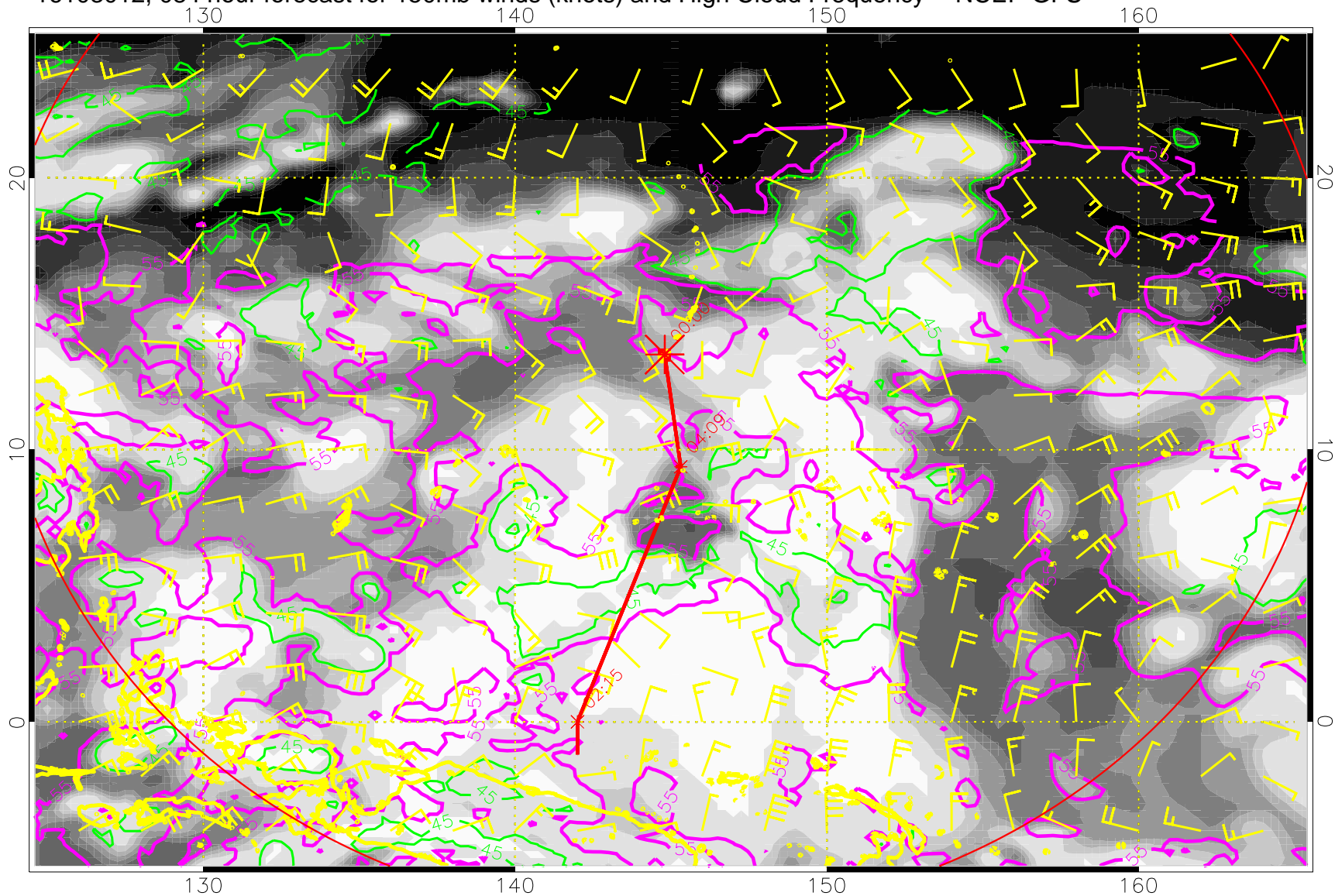
16103012, 084 hour forecast for 150mb winds (knots) and High Cloud Frequency -- NCEP GFS
