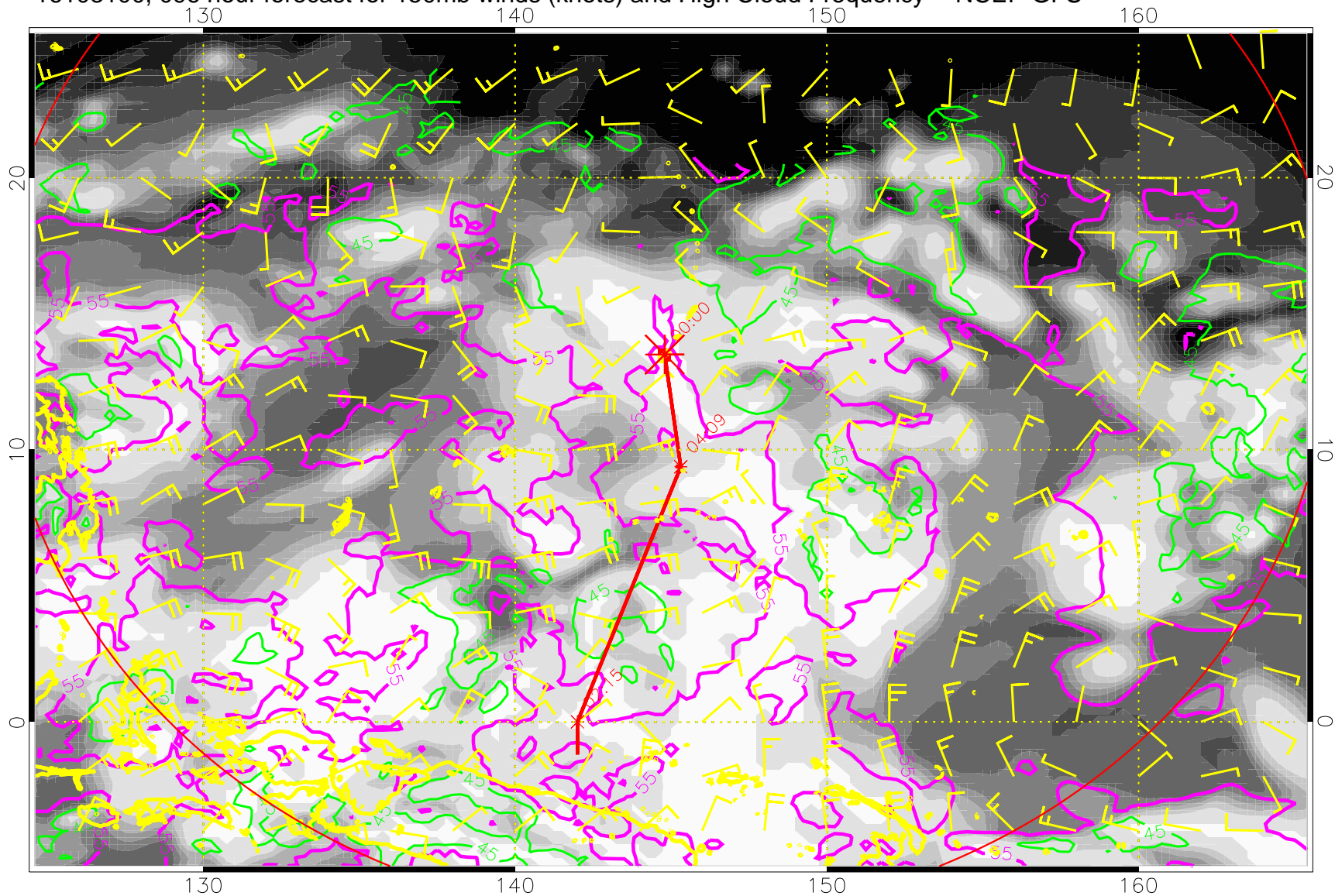
16103100, 096 hour forecast for 150mb winds (knots) and High Cloud Frequency -- NCEP GFS
