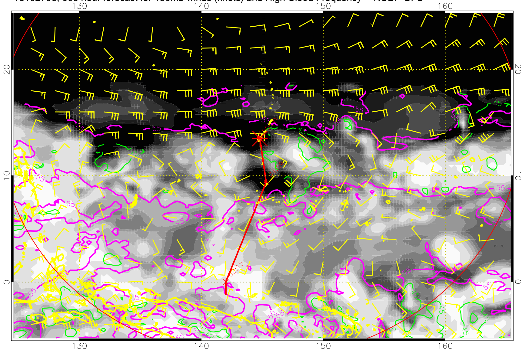
16102706, 006 hour forecast for 150mb winds (knots) and High Cloud Frequency -- NCEP GFS
