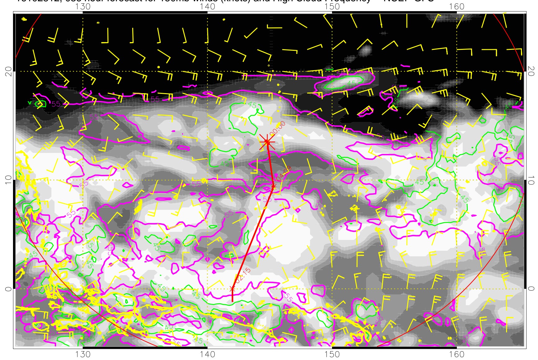
16102812, 036 hour forecast for 150mb winds (knots) and High Cloud Frequency -- NCEP GFS
