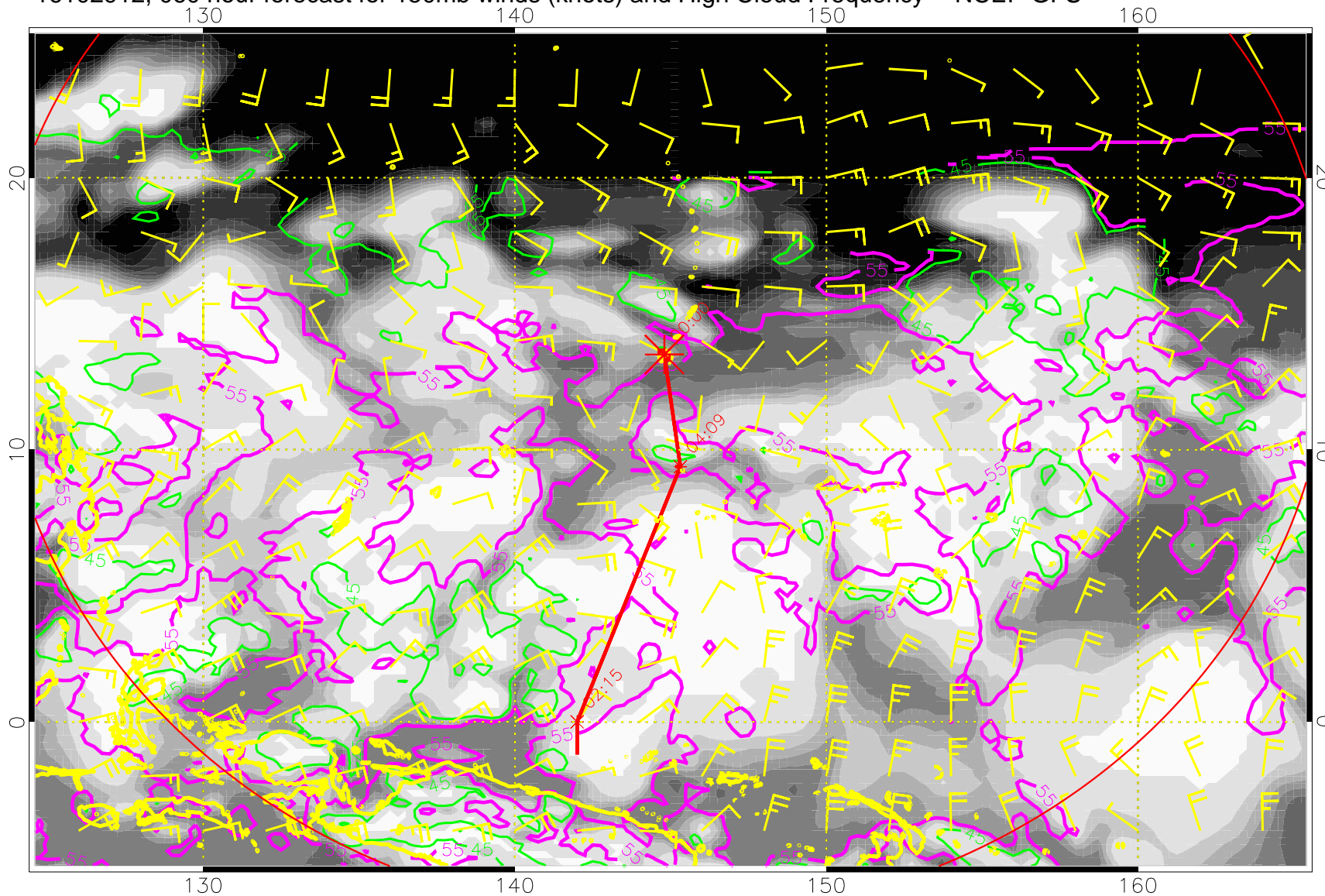
16102912, 060 hour forecast for 150mb winds (knots) and High Cloud Frequency -- NCEP GFS
