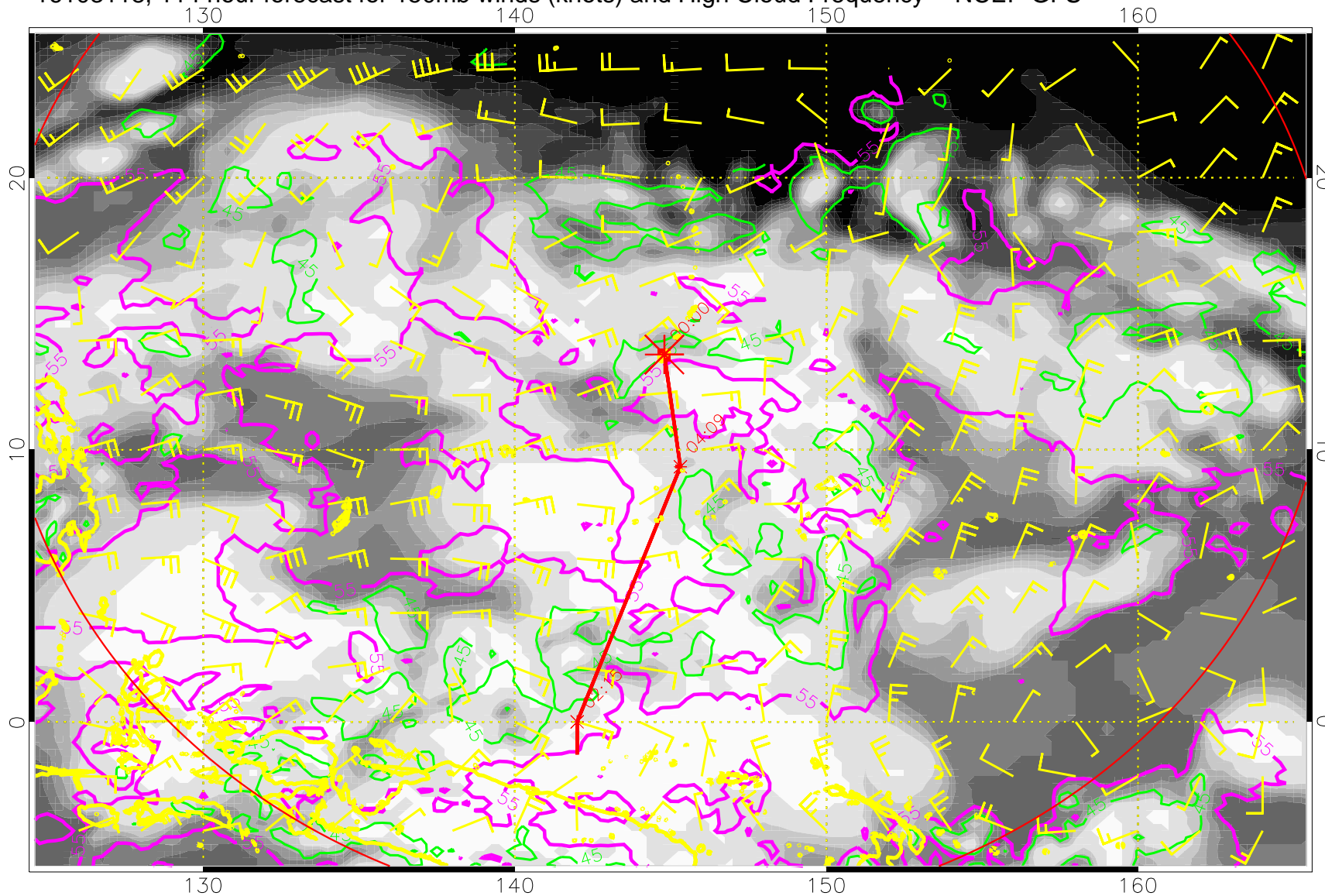
16103118, 114 hour forecast for 150mb winds (knots) and High Cloud Frequency -- NCEP GFS
