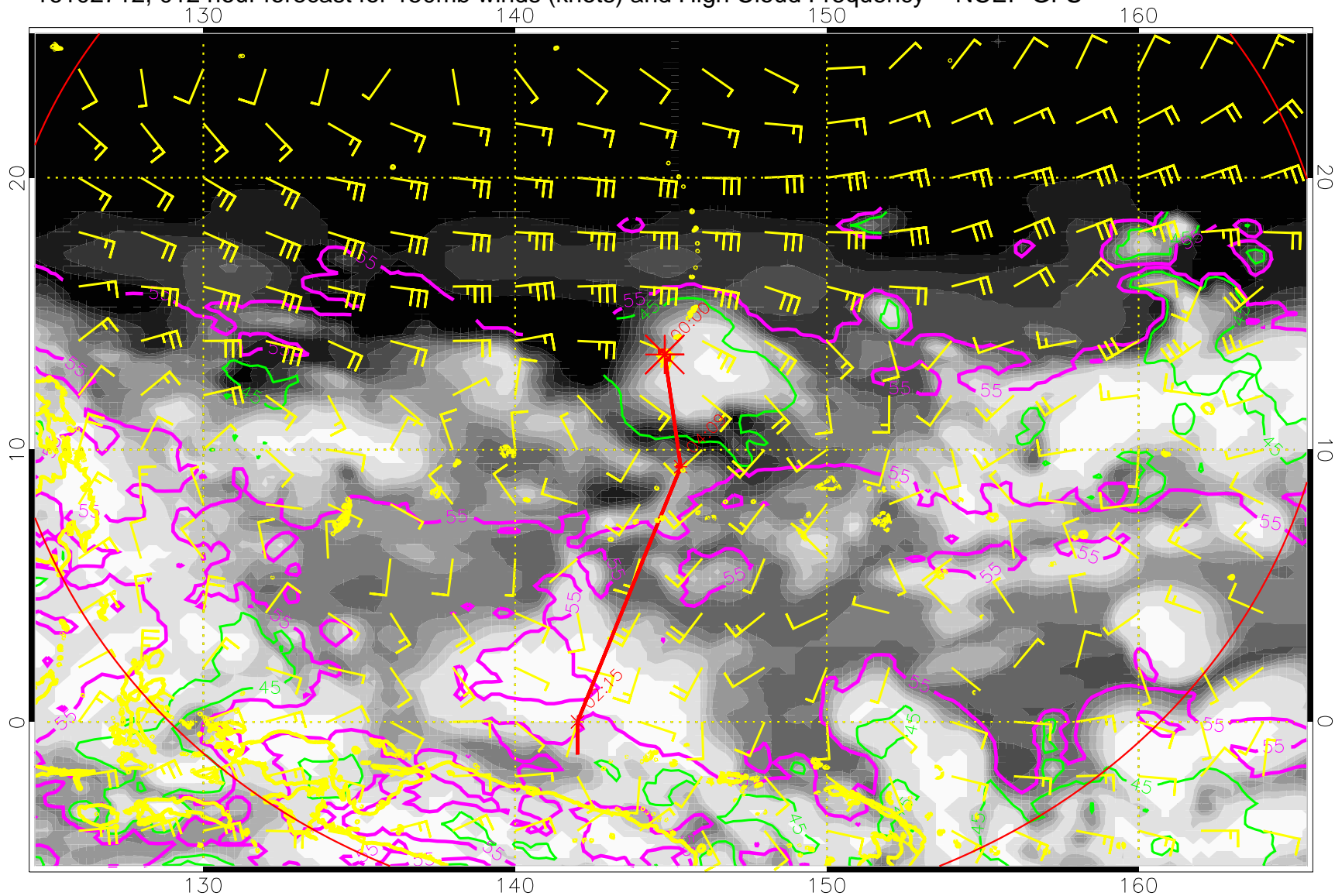
16102712, 012 hour forecast for 150mb winds (knots) and High Cloud Frequency -- NCEP GFS
