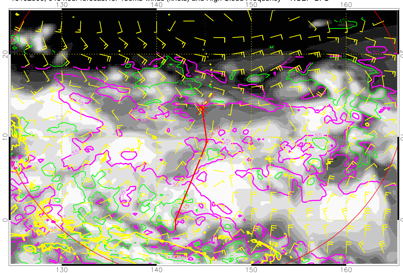
16102900, 048 hour forecast for 150mb winds (knots) and High Cloud Frequency -- NCEP GFS
