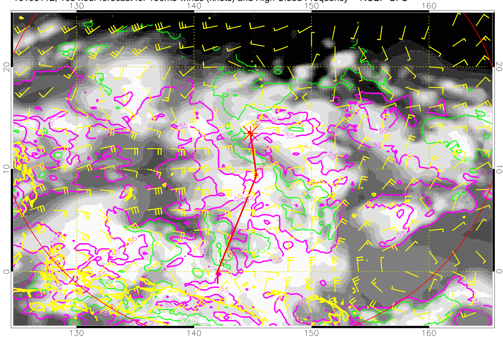
16103112, 108 hour forecast for 150mb winds (knots) and High Cloud Frequency -- NCEP GFS
