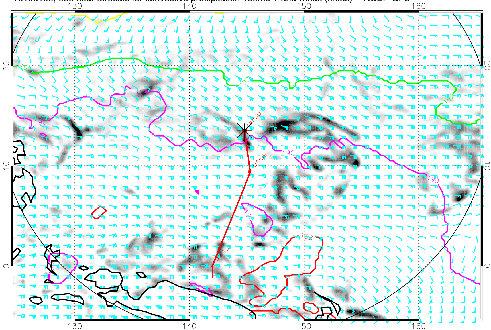
16103100, 096 hour forecast for convective precipitation 100mb T and winds (knots) -- NCEP GFS
