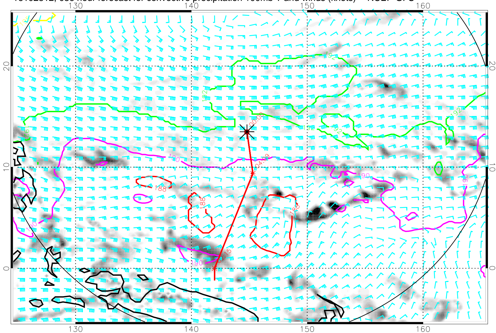
16102812, 036 hour forecast for convective precipitation 100mb T and winds (knots) -- NCEP GFS
