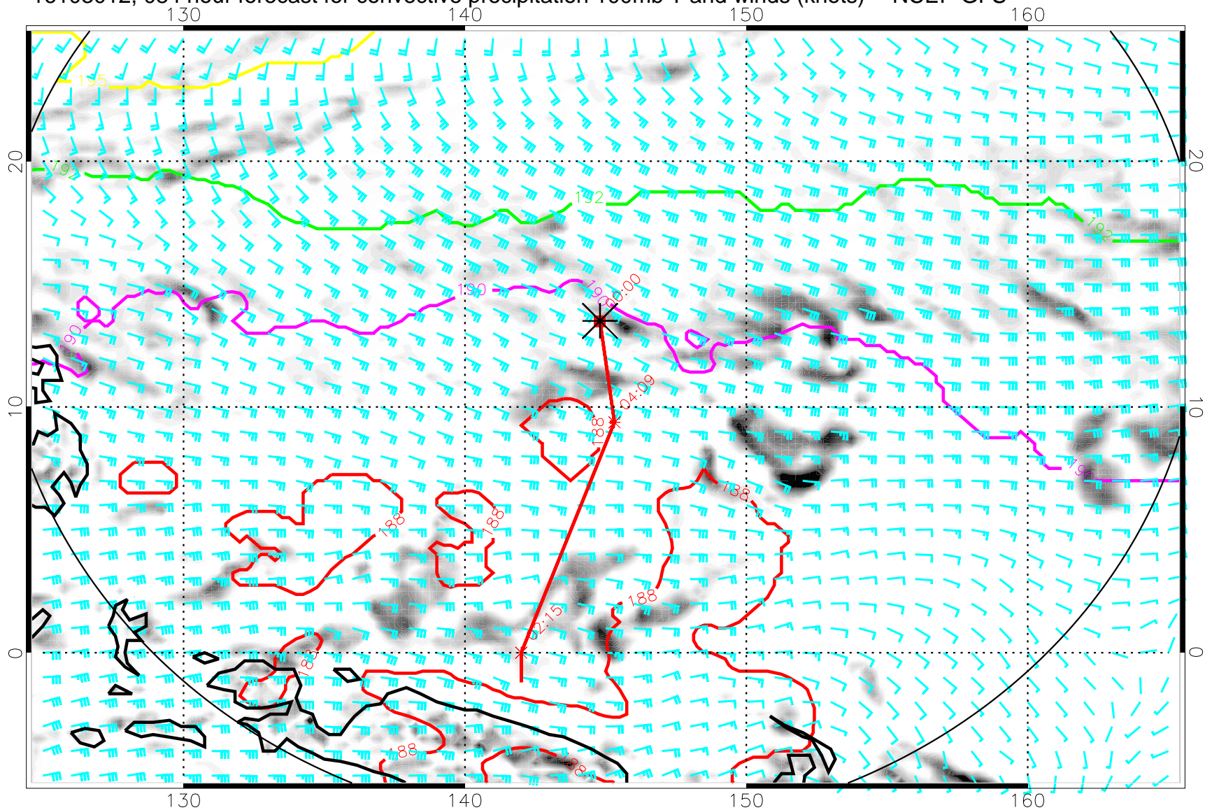
16103012, 084 hour forecast for convective precipitation 100mb T and winds (knots) -- NCEP GFS
