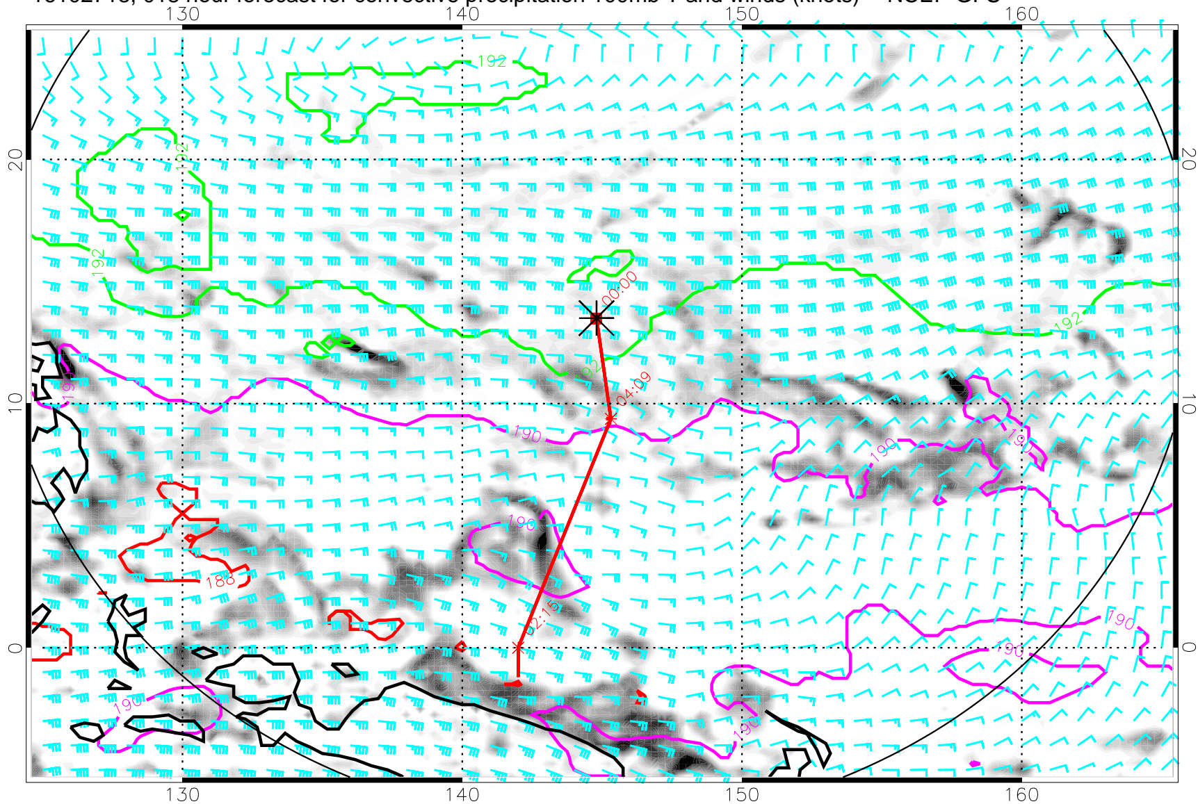
16102718, 018 hour forecast for convective precipitation 100mb T and winds (knots) -- NCEP GFS
