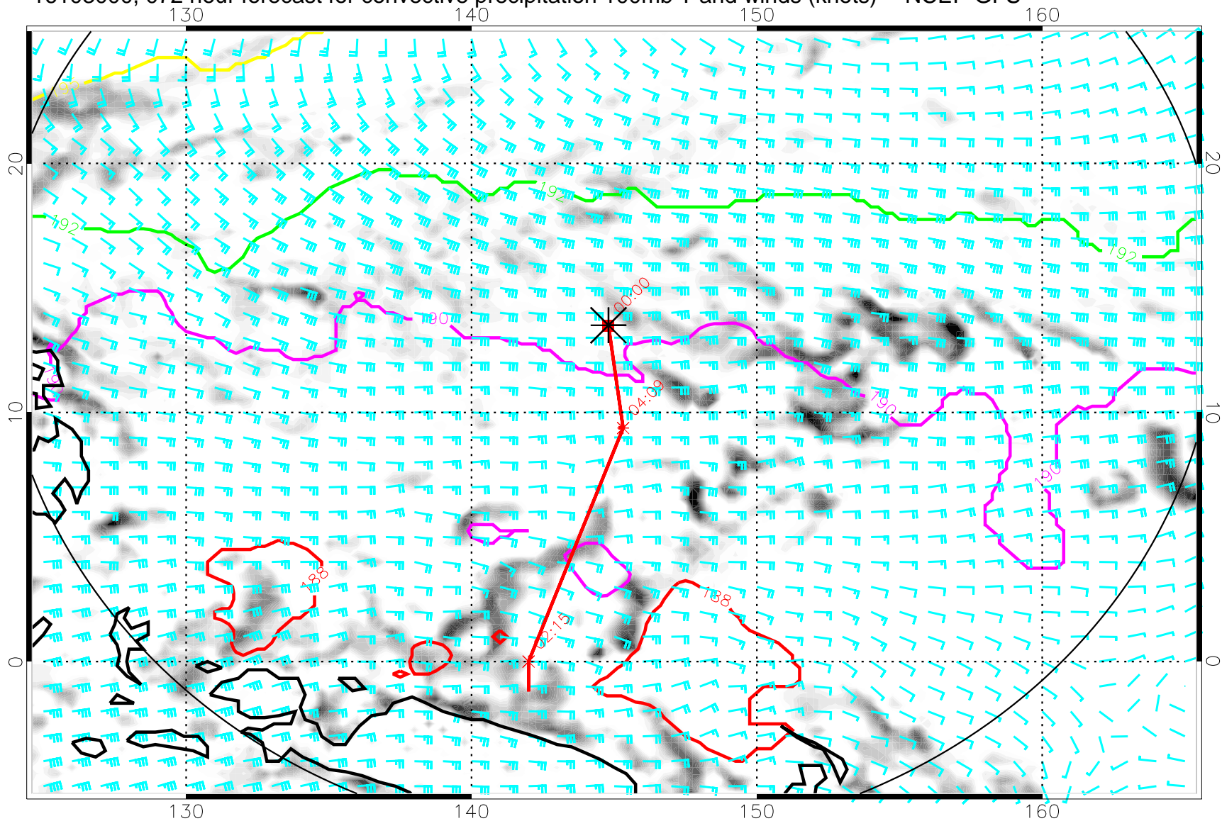
16103000, 072 hour forecast for convective precipitation 100mb T and winds (knots) -- NCEP GFS
