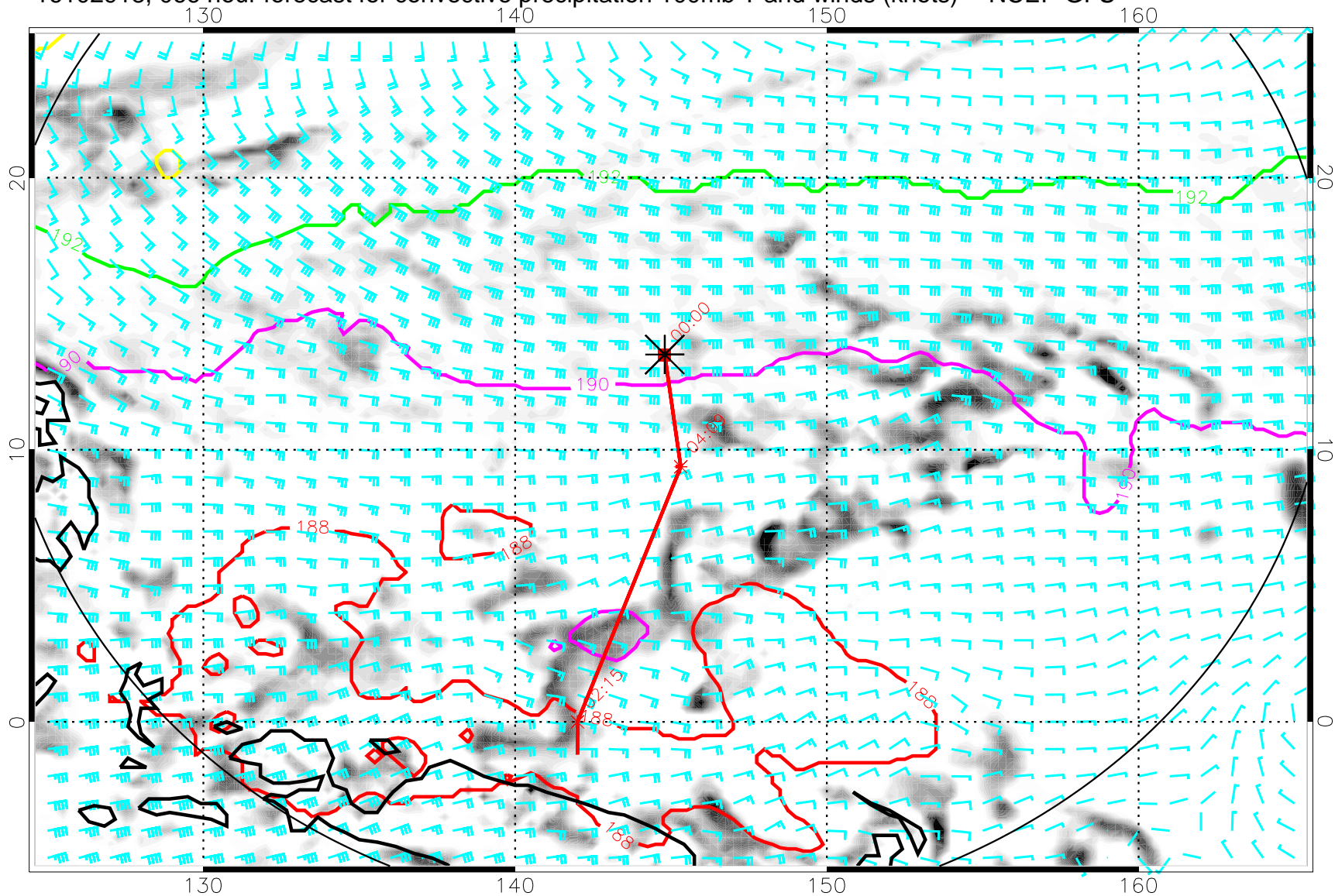
16102918, 066 hour forecast for convective precipitation 100mb T and winds (knots) -- NCEP GFS
