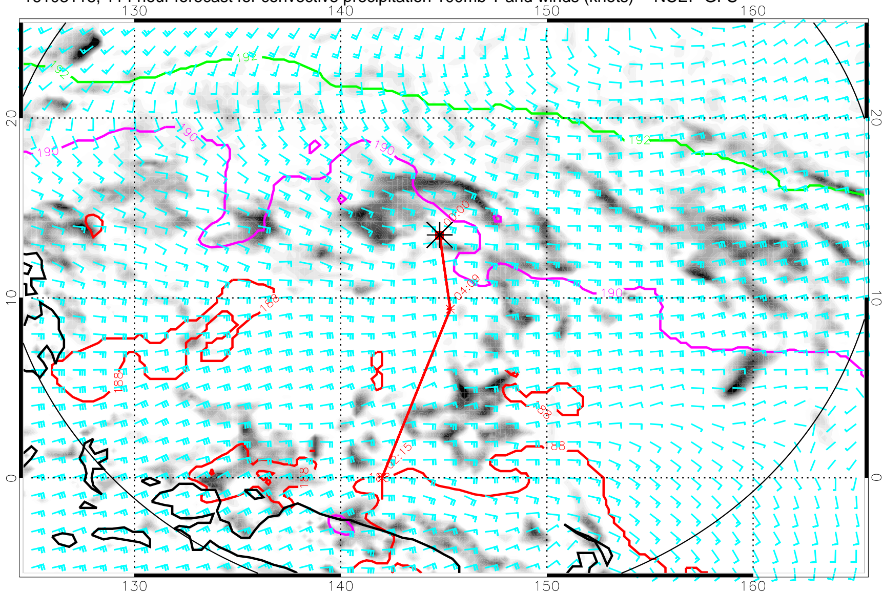
16103118, 114 hour forecast for convective precipitation 100mb T and winds (knots) -- NCEP GFS
