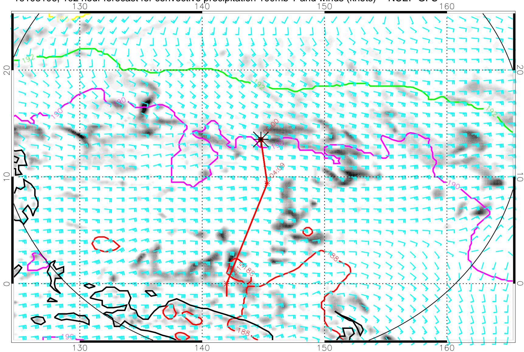
16103106, 102 hour forecast for convective precipitation 100mb T and winds (knots) -- NCEP GFS
