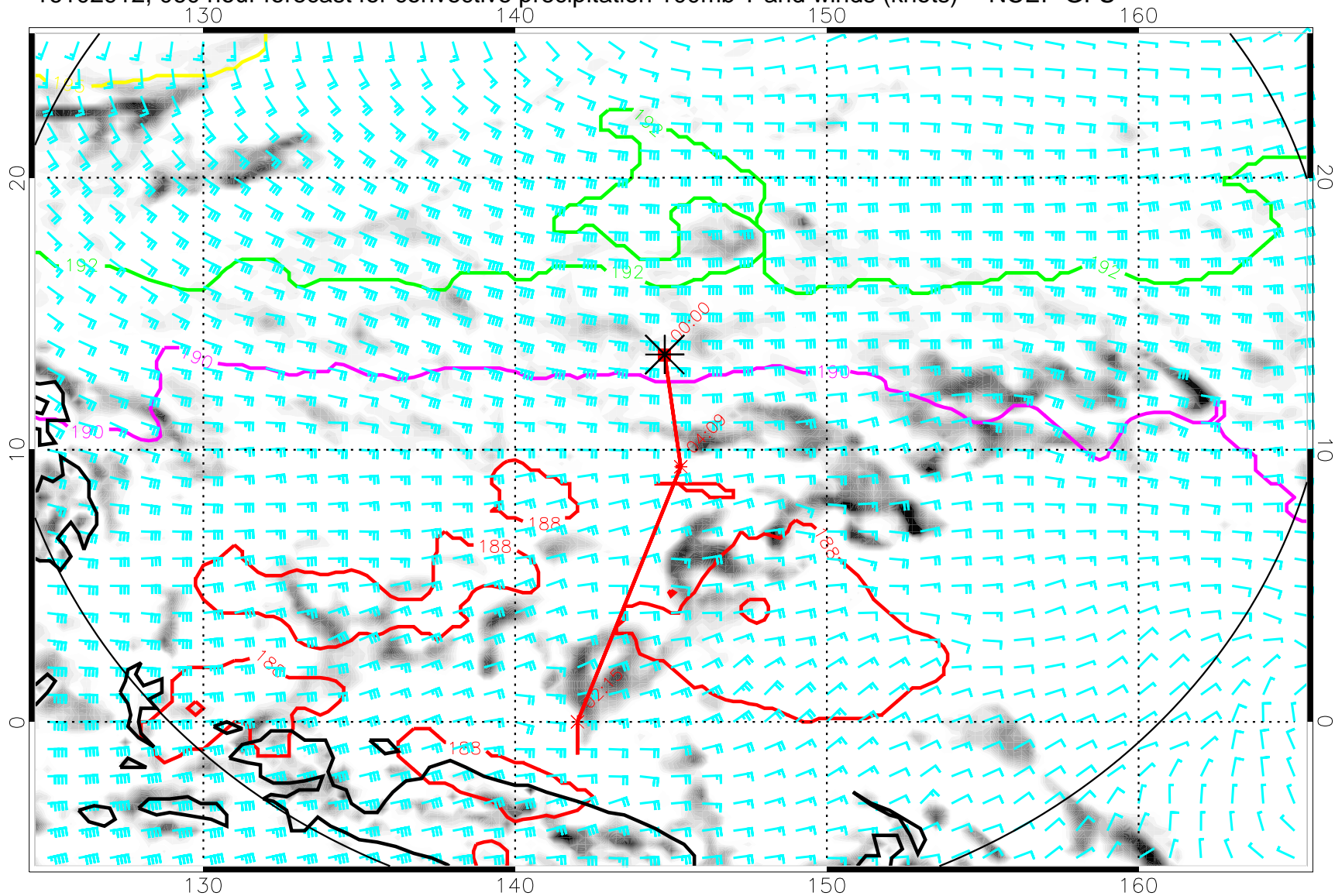
16102912, 060 hour forecast for convective precipitation 100mb T and winds (knots) -- NCEP GFS
