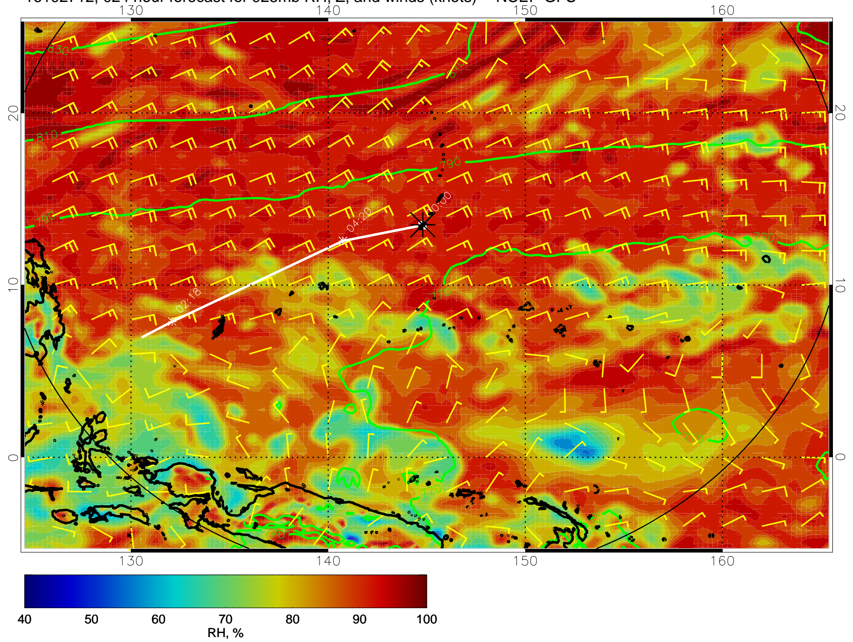
16102712, 024 hour forecast for 925mb RH, Z, and winds (knots) -- NCEP GFS
