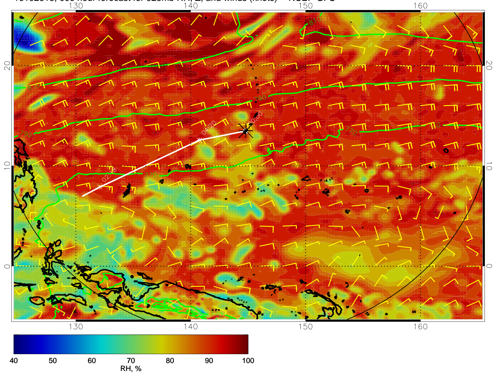
16102618, 006 hour forecast for 925mb RH, Z, and winds (knots) -- NCEP GFS
