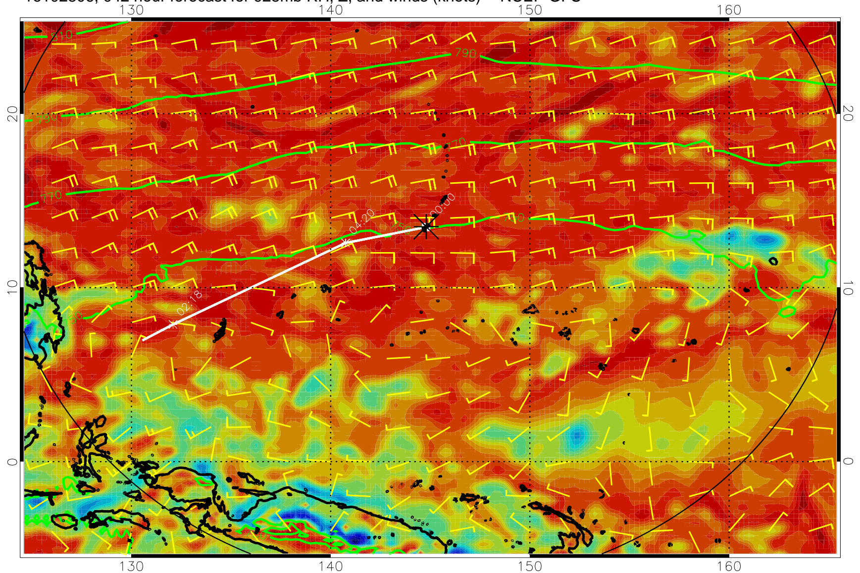
16102806, 042 hour forecast for 925mb RH, Z, and winds (knots) -- NCEP GFS
