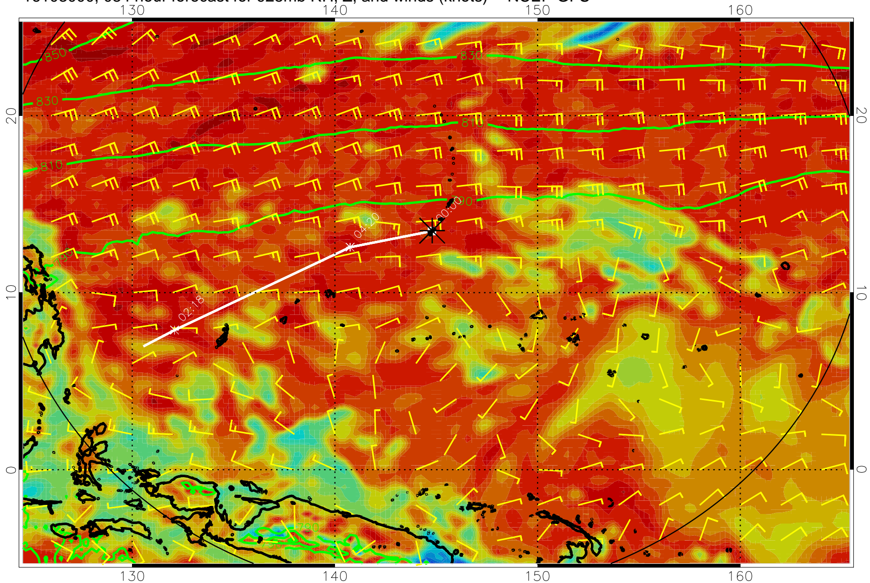
16103000, 084 hour forecast for 925mb RH, Z, and winds (knots) -- NCEP GFS
