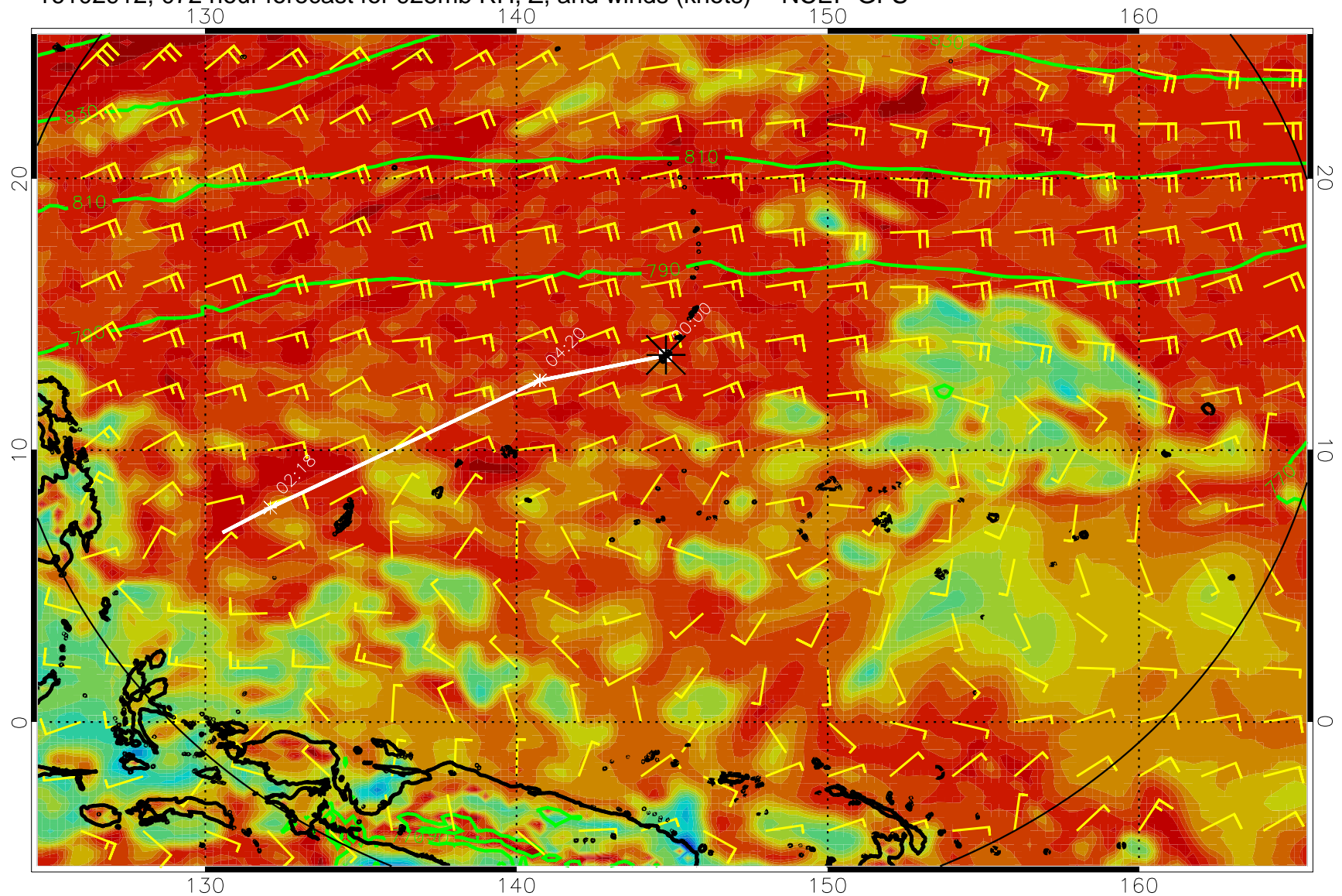
16102912, 072 hour forecast for 925mb RH, Z, and winds (knots) -- NCEP GFS
