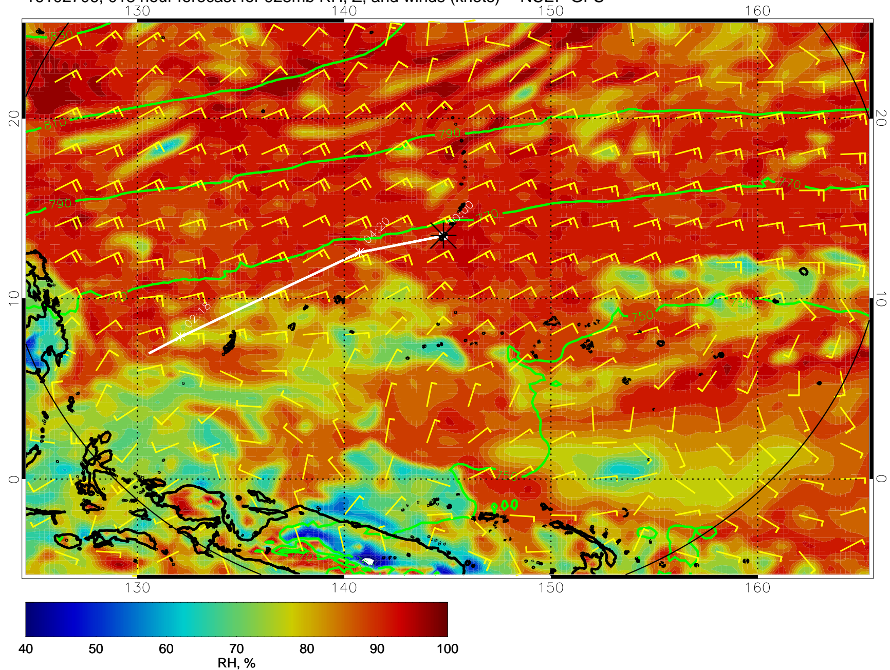
16102706, 018 hour forecast for 925mb RH, Z, and winds (knots) -- NCEP GFS
