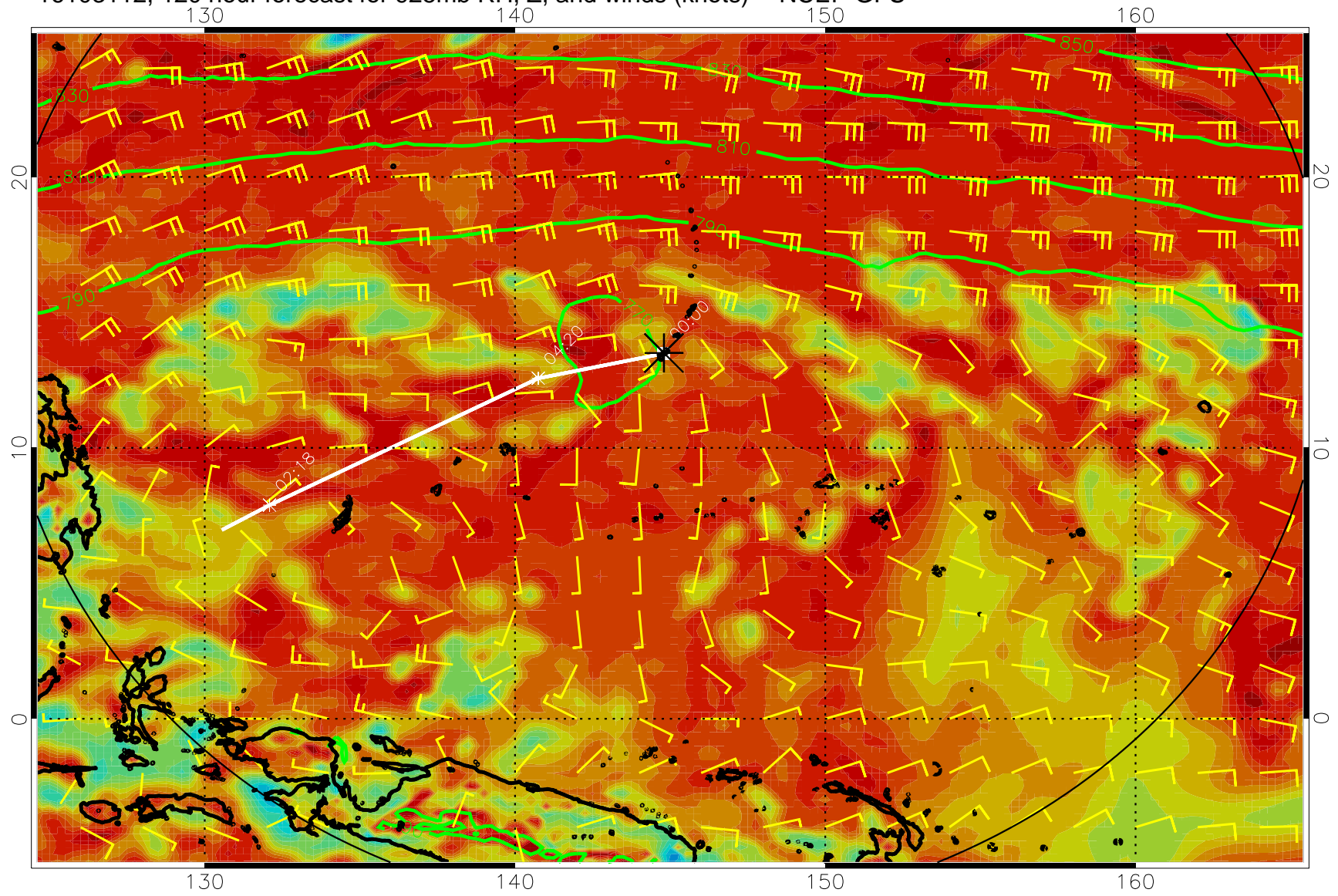
16103112, 120 hour forecast for 925mb RH, Z, and winds (knots) -- NCEP GFS
