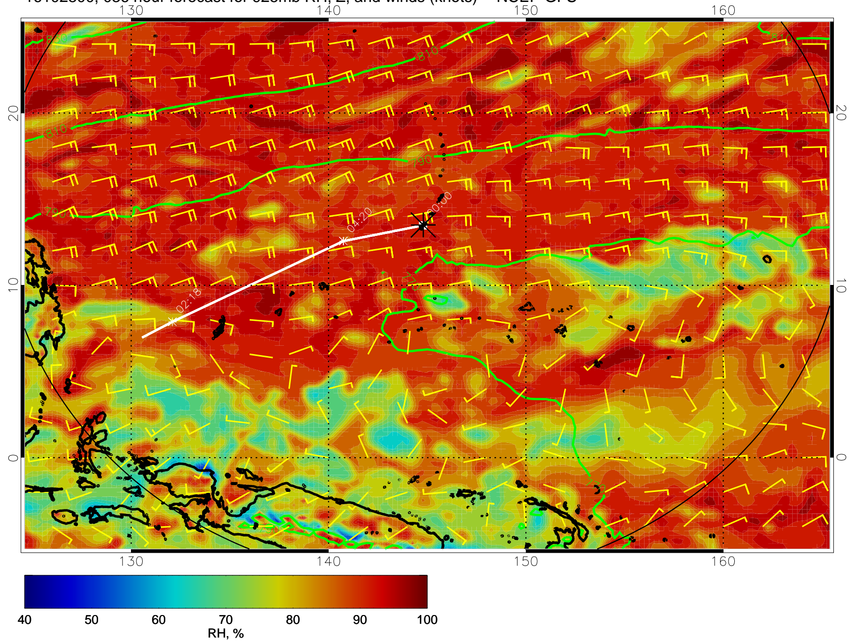
16102800, 036 hour forecast for 925mb RH, Z, and winds (knots) -- NCEP GFS
