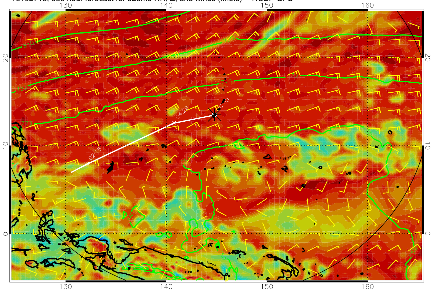
16102718, 030 hour forecast for 925mb RH, Z, and winds (knots) -- NCEP GFS
