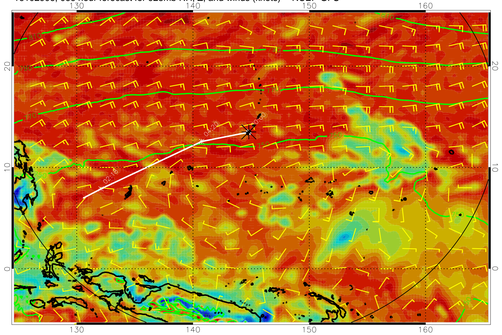
16102906, 066 hour forecast for 925mb RH, Z, and winds (knots) -- NCEP GFS
