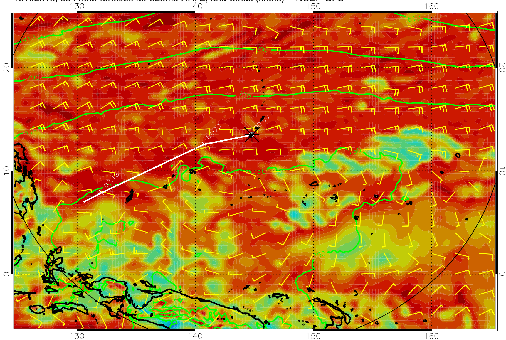
16102818, 054 hour forecast for 925mb RH, Z, and winds (knots) -- NCEP GFS
