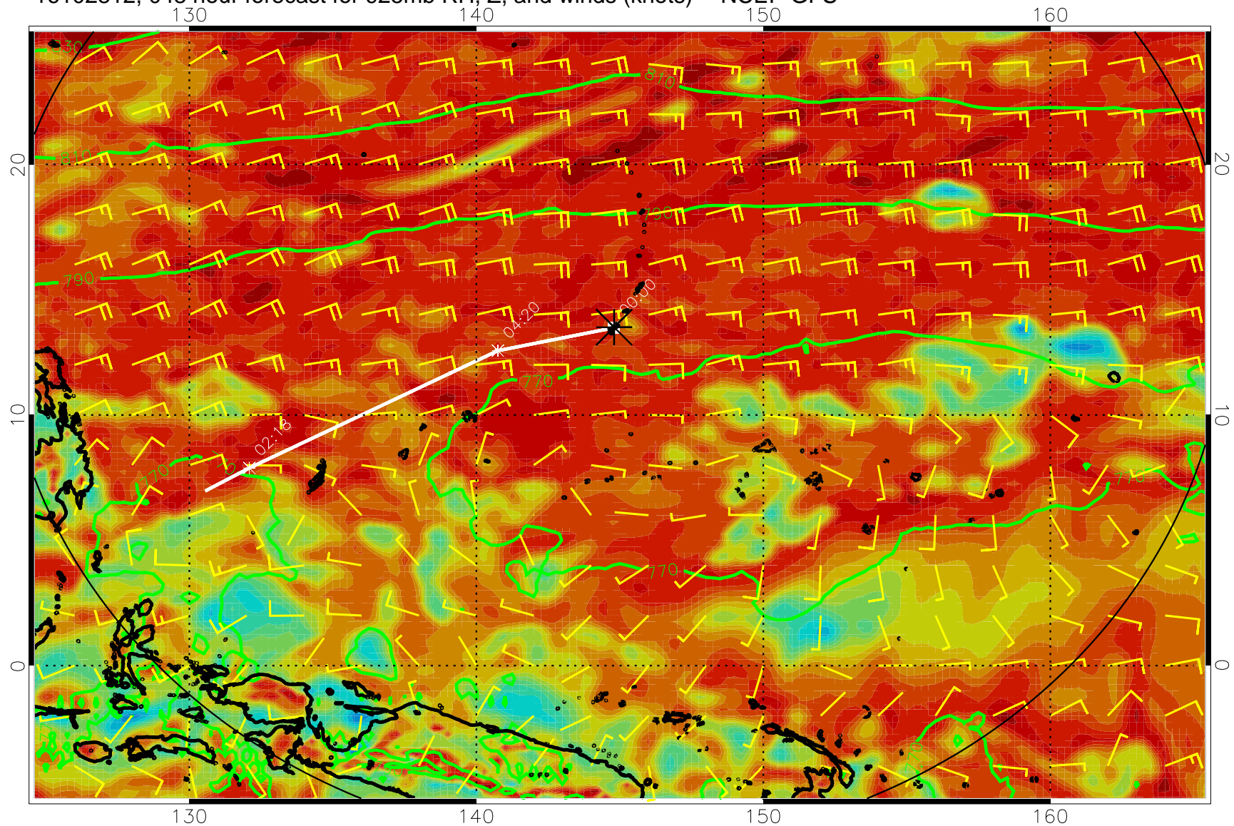
16102812, 048 hour forecast for 925mb RH, Z, and winds (knots) -- NCEP GFS
