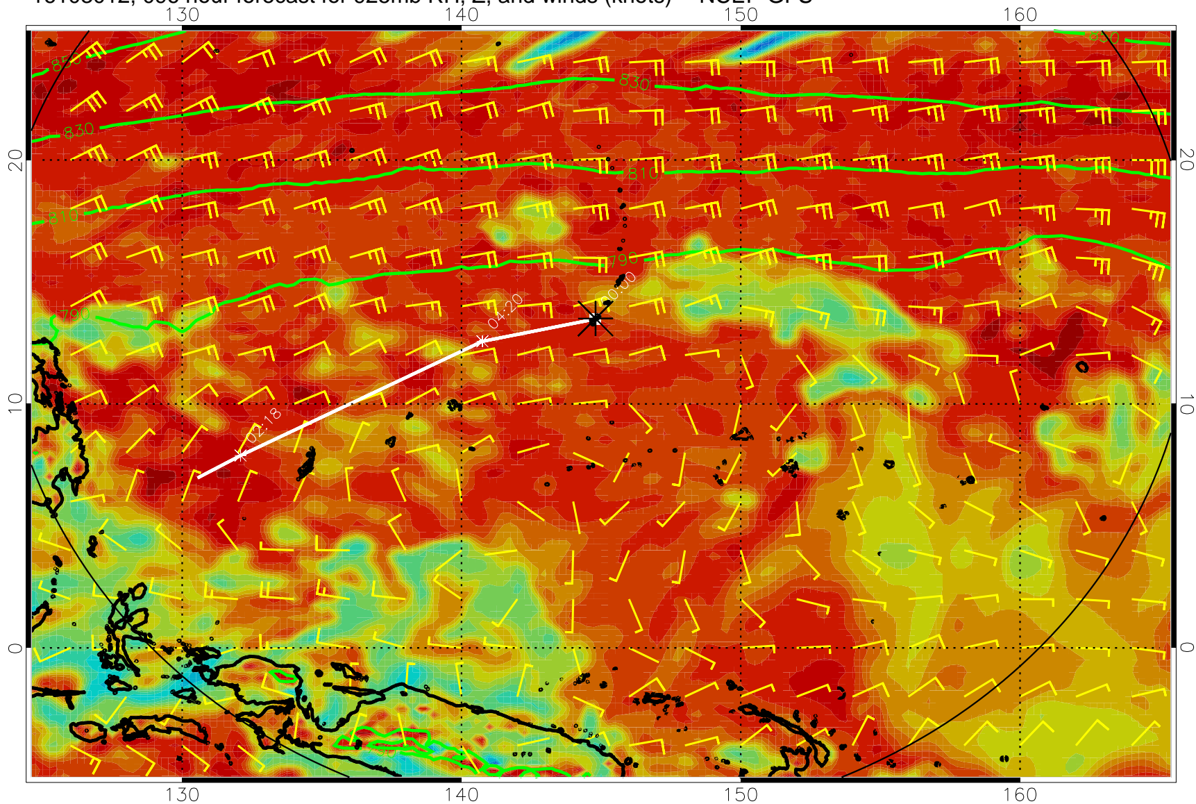
16103012, 096 hour forecast for 925mb RH, Z, and winds (knots) -- NCEP GFS
