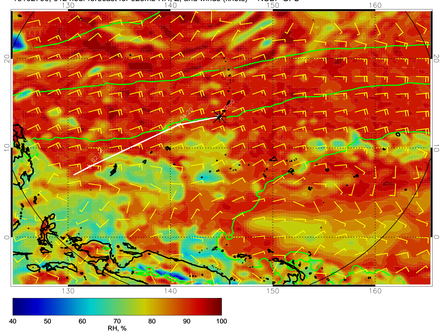
16102700, 012 hour forecast for 925mb RH, Z, and winds (knots) -- NCEP GFS
