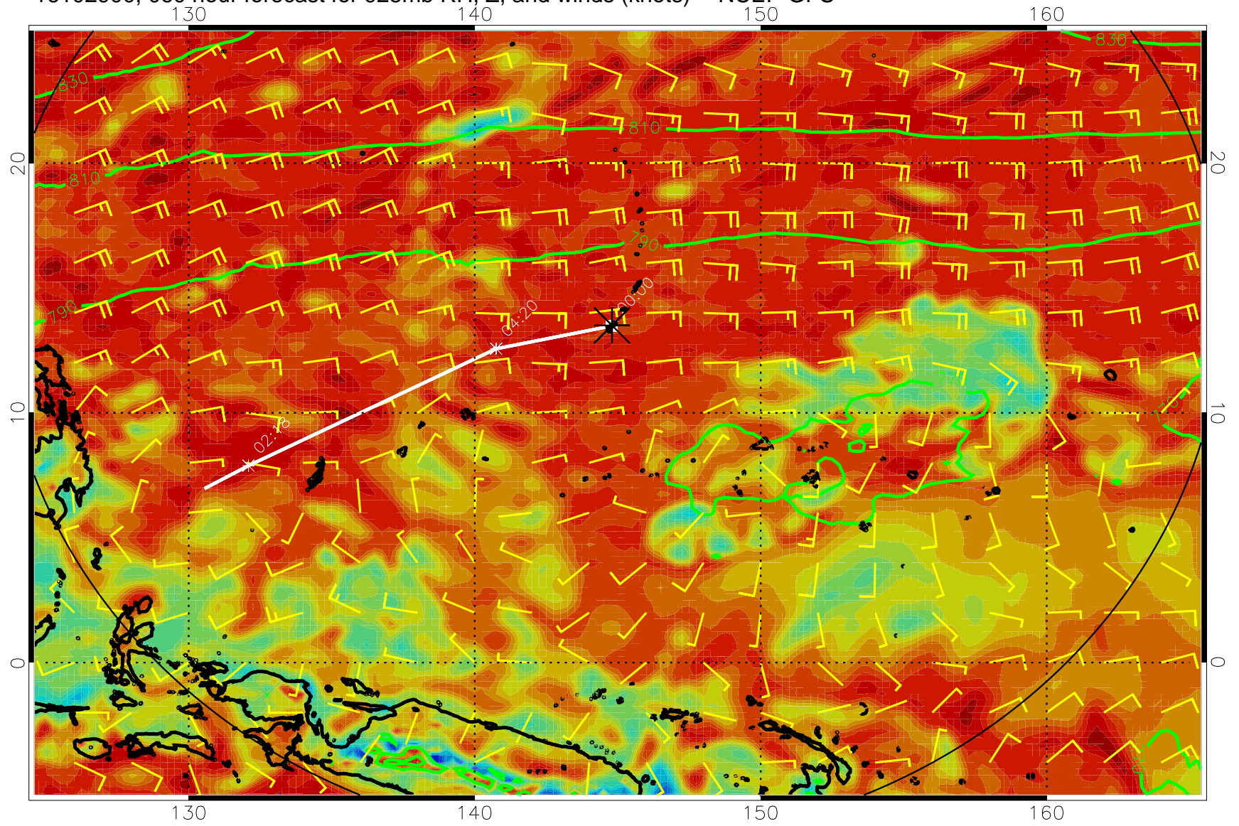
16102900, 060 hour forecast for 925mb RH, Z, and winds (knots) -- NCEP GFS
