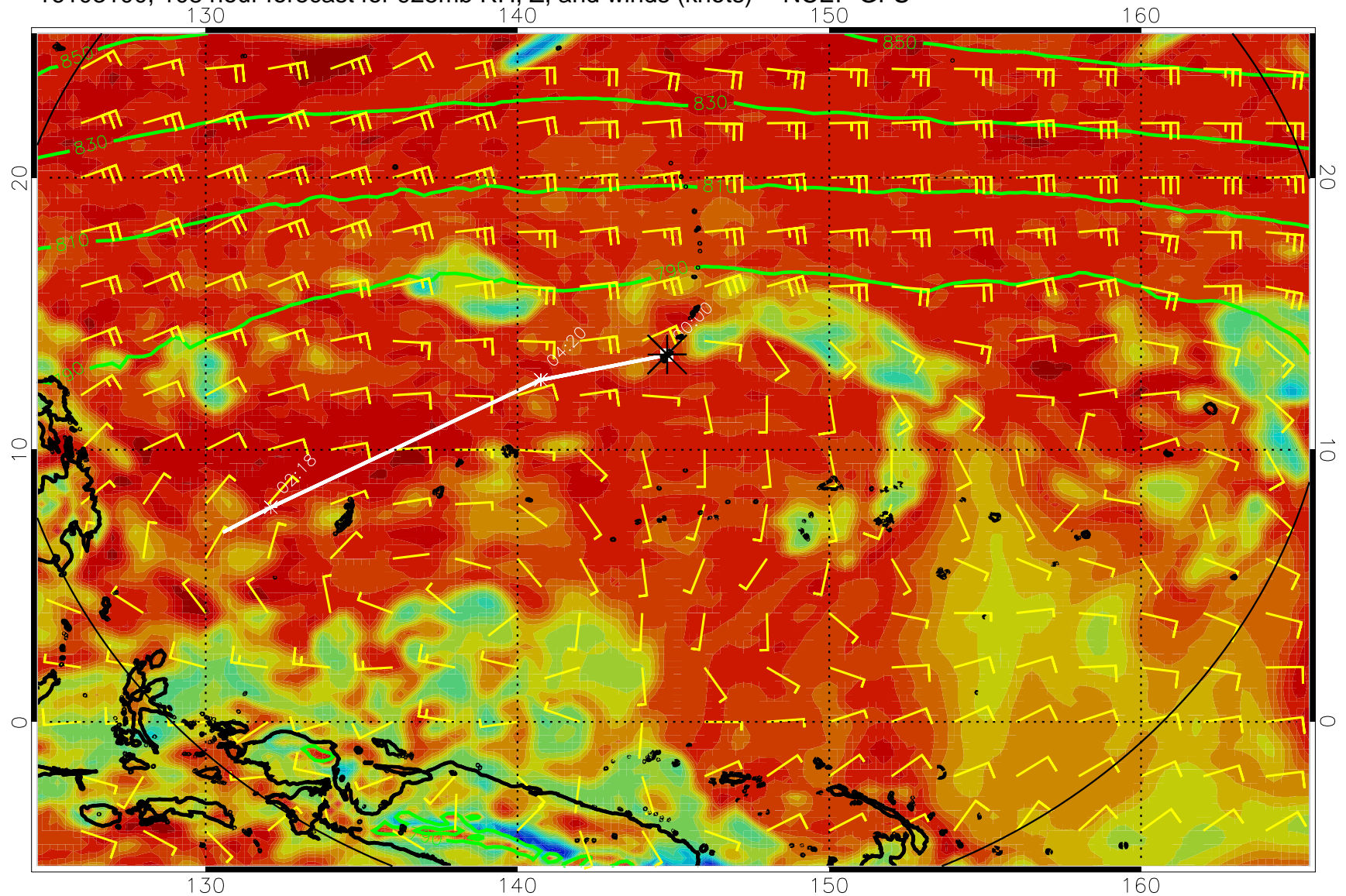
16103100, 108 hour forecast for 925mb RH, Z, and winds (knots) -- NCEP GFS
