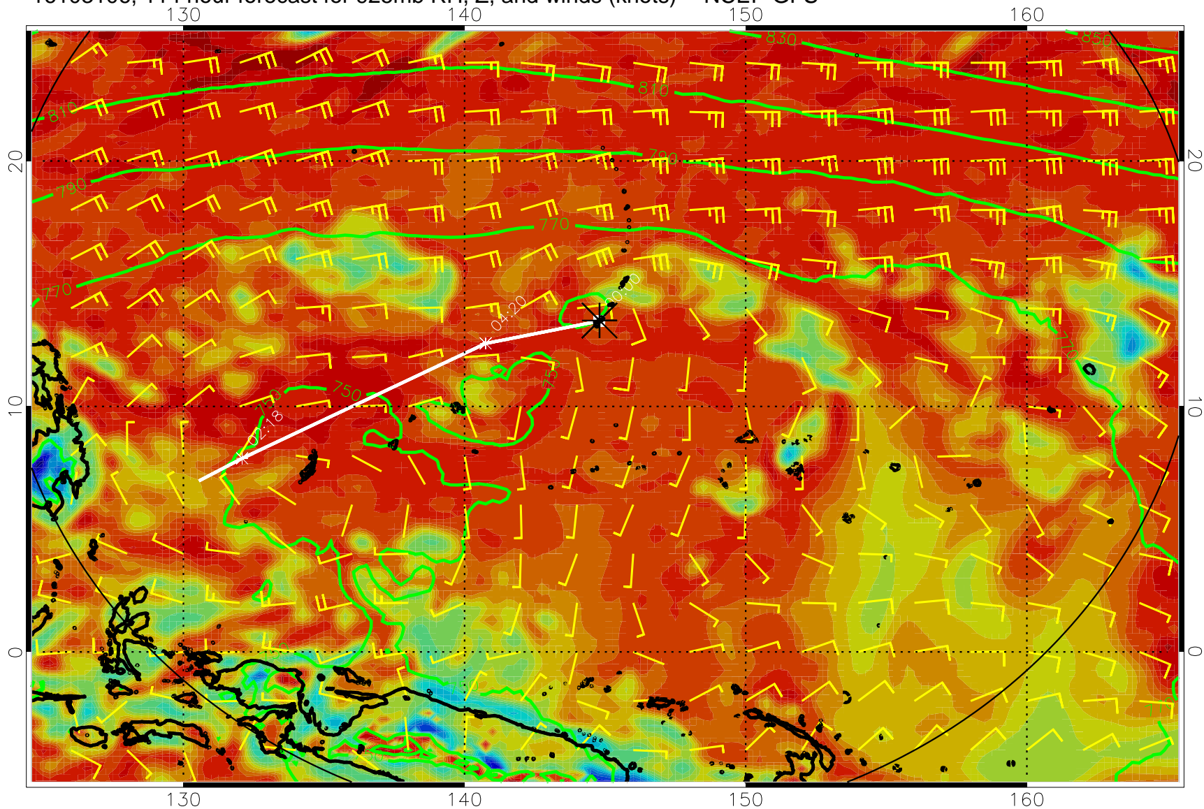
16103106, 114 hour forecast for 925mb RH, Z, and winds (knots) -- NCEP GFS
