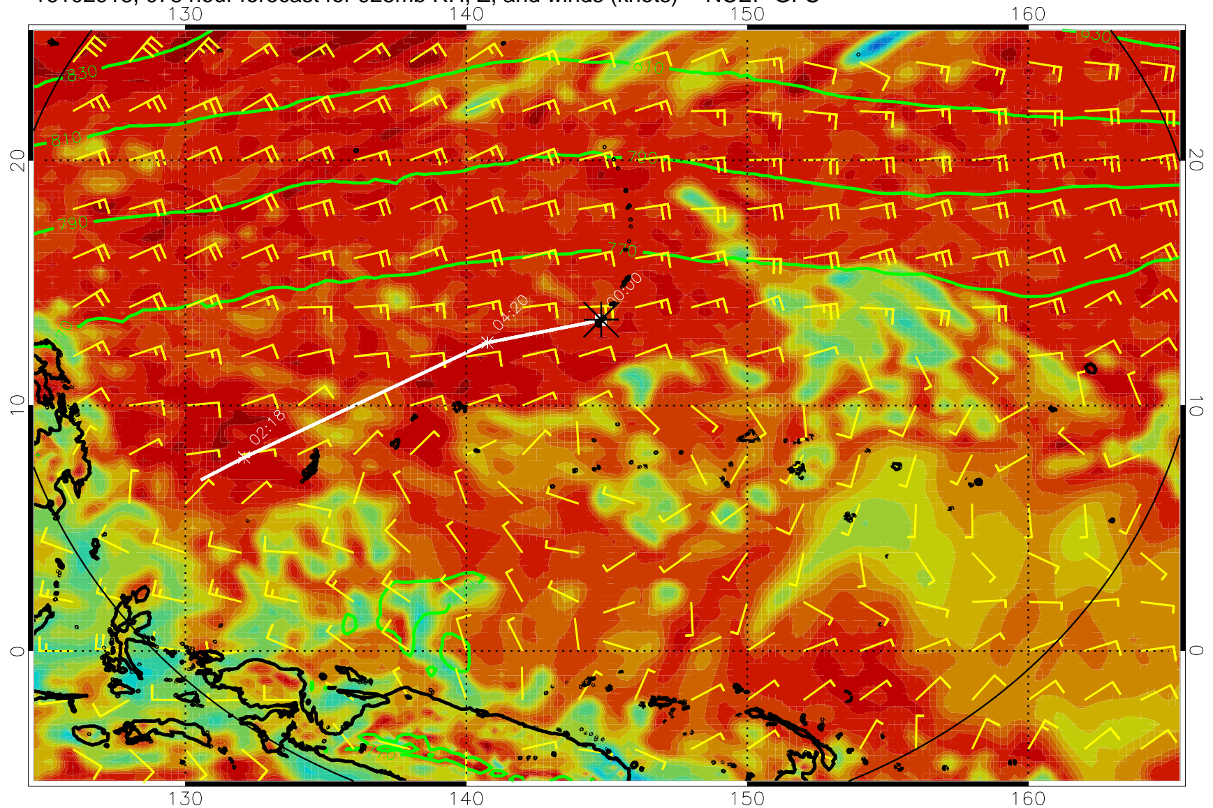
16102918, 078 hour forecast for 925mb RH, Z, and winds (knots) -- NCEP GFS
