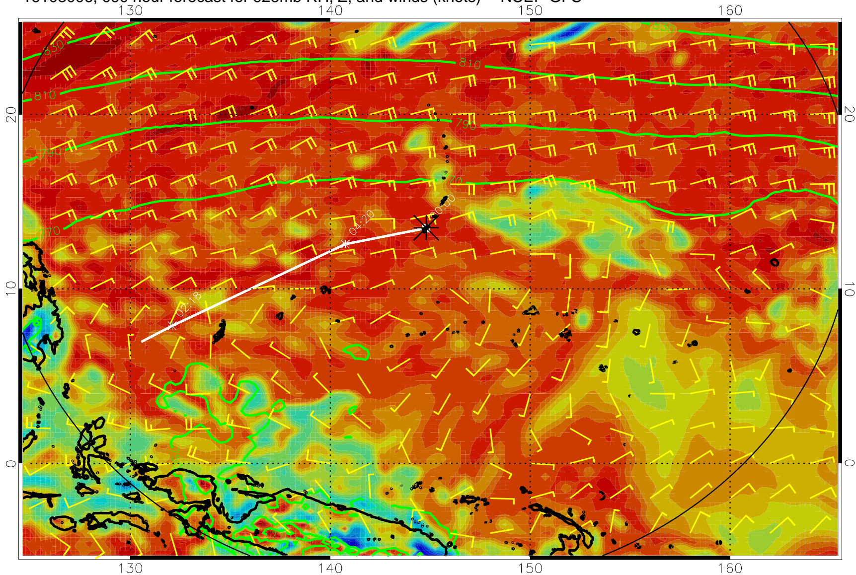
16103006, 090 hour forecast for 925mb RH, Z, and winds (knots) -- NCEP GFS
