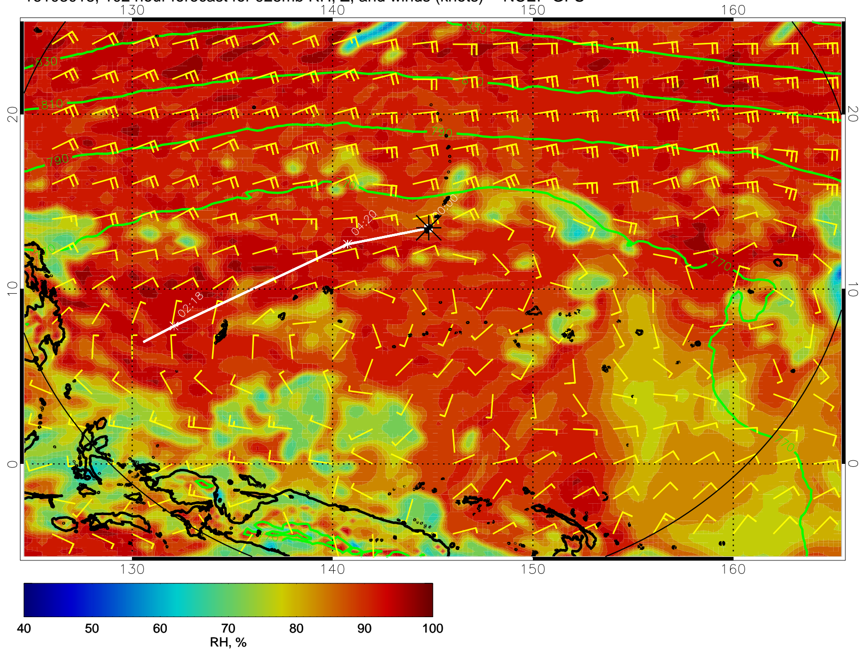
16103018, 102 hour forecast for 925mb RH, Z, and winds (knots) -- NCEP GFS
