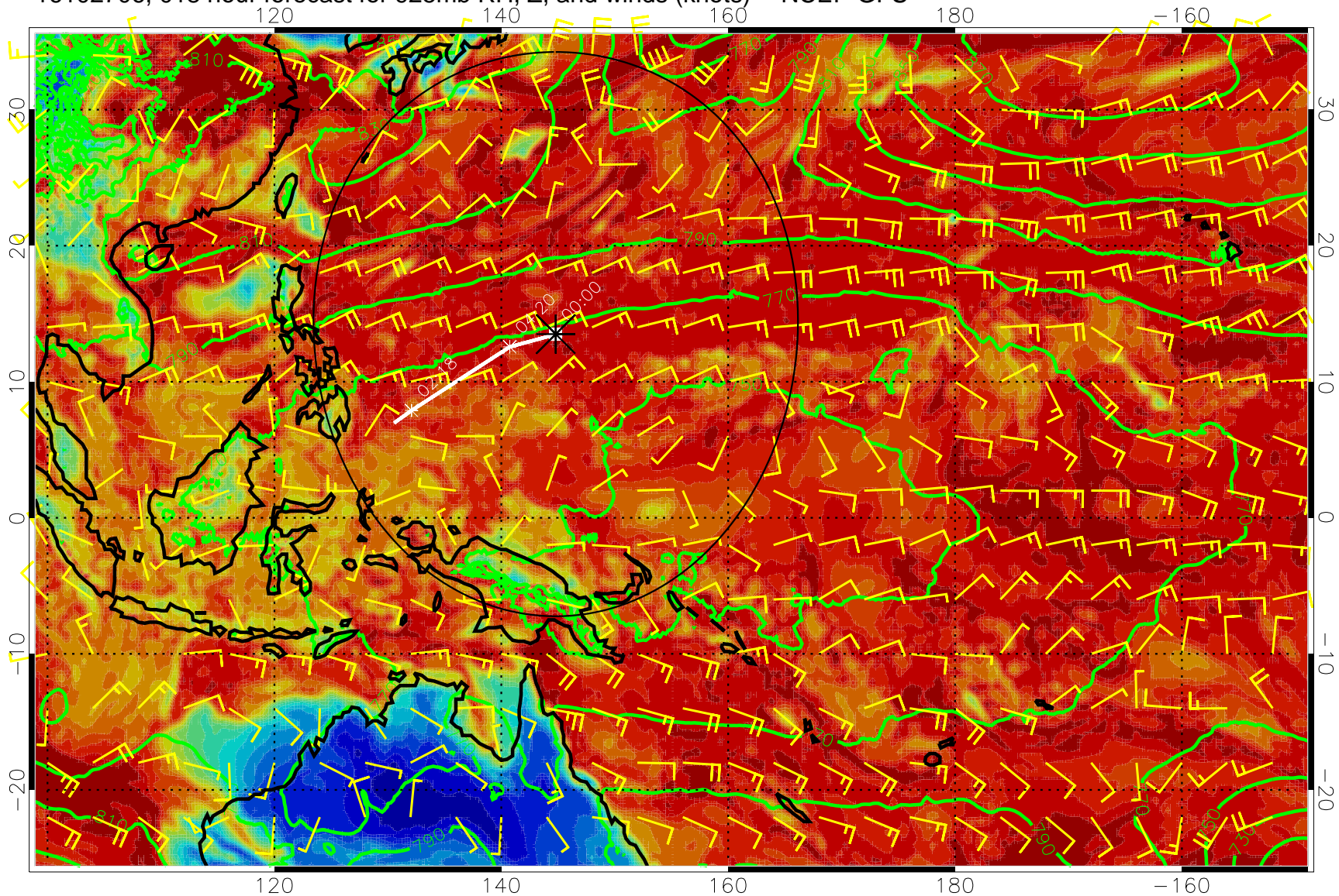
16102706, 018 hour forecast for 925mb RH, Z, and winds (knots) -- NCEP GFS
