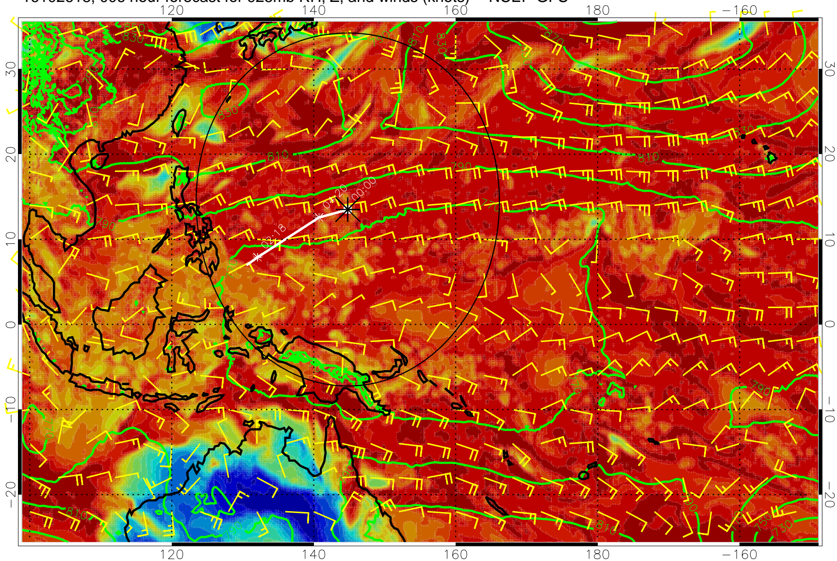
16102618, 006 hour forecast for 925mb RH, Z, and winds (knots) -- NCEP GFS
