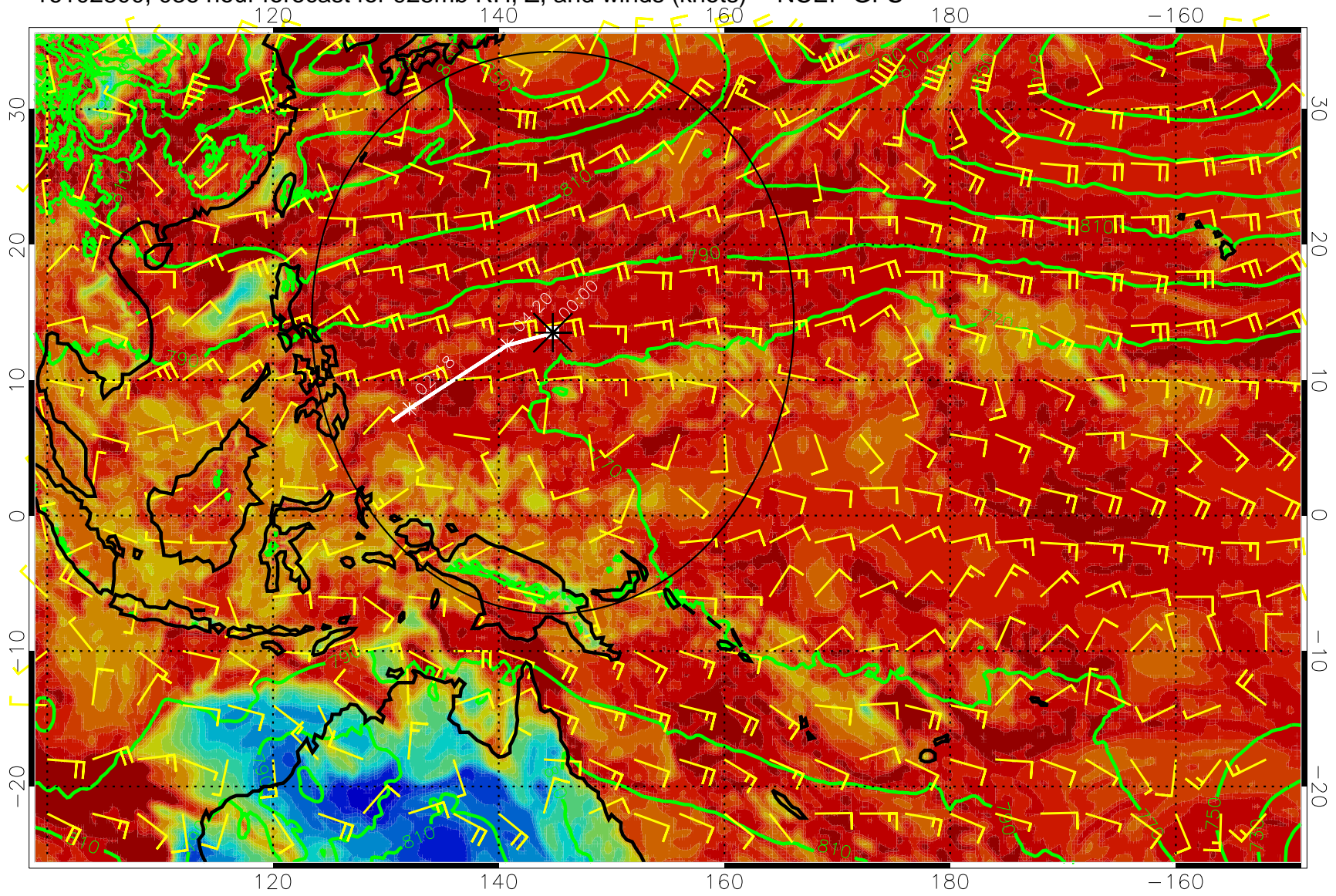
16102800, 036 hour forecast for 925mb RH, Z, and winds (knots) -- NCEP GFS
