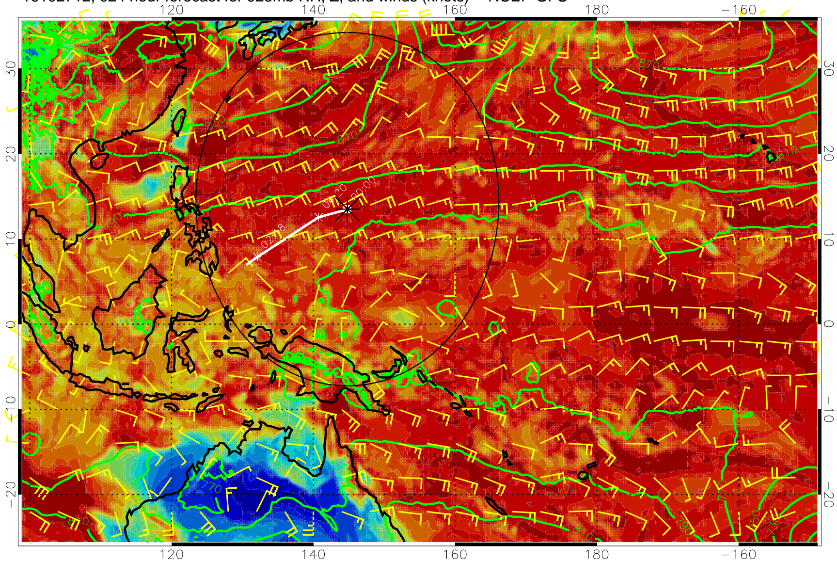
16102712, 024 hour forecast for 925mb RH, Z, and winds (knots) -- NCEP GFS
