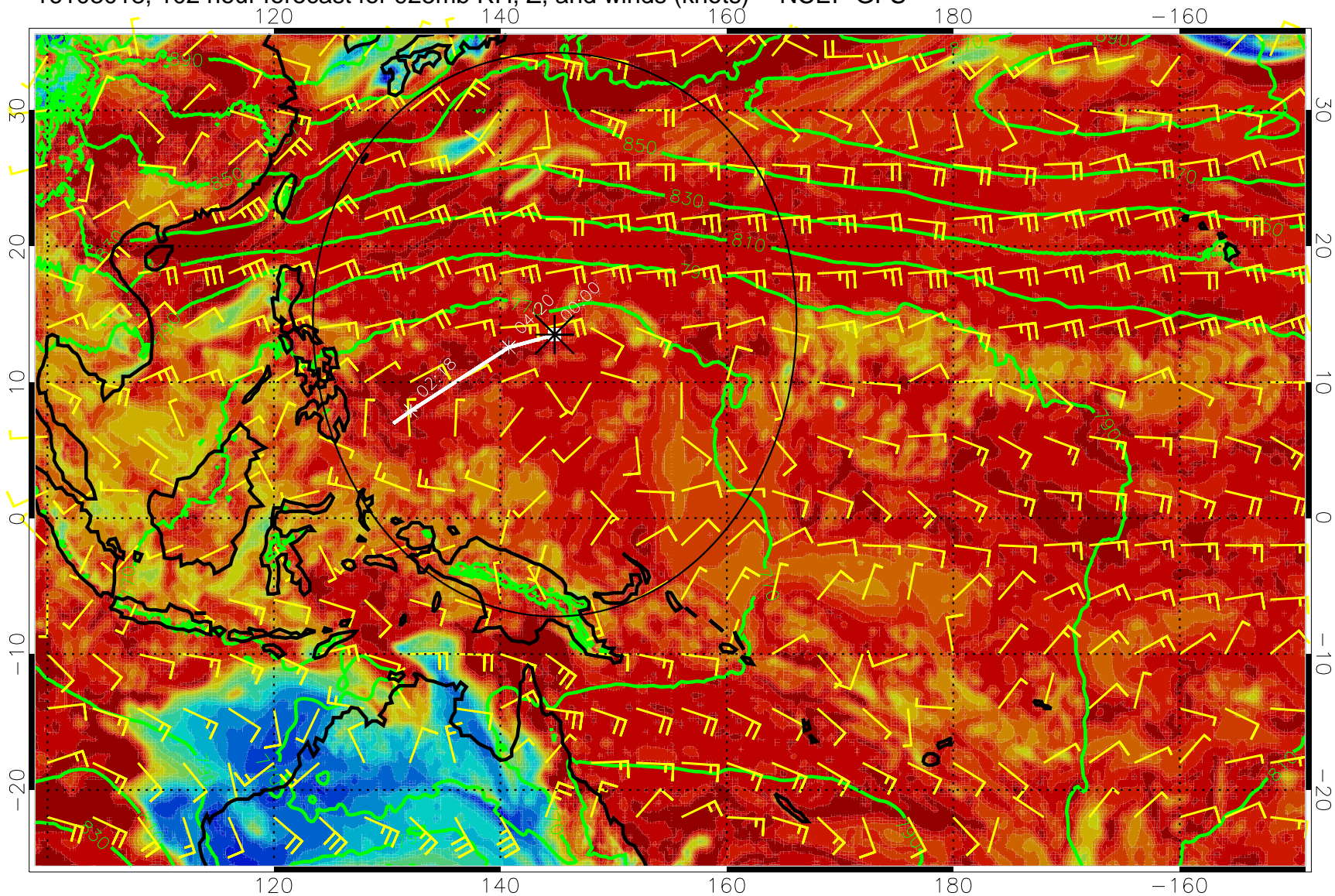
16103018, 102 hour forecast for 925mb RH, Z, and winds (knots) -- NCEP GFS
