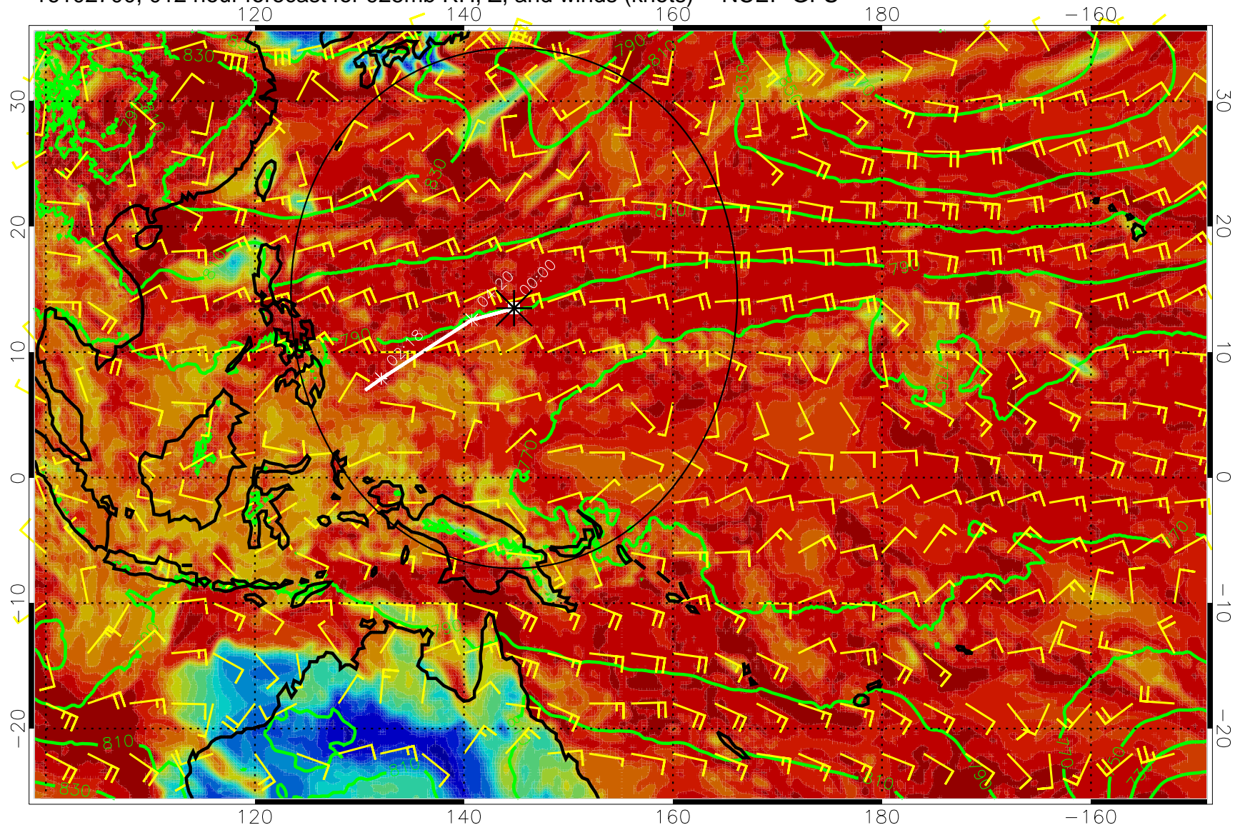
16102700, 012 hour forecast for 925mb RH, Z, and winds (knots) -- NCEP GFS
