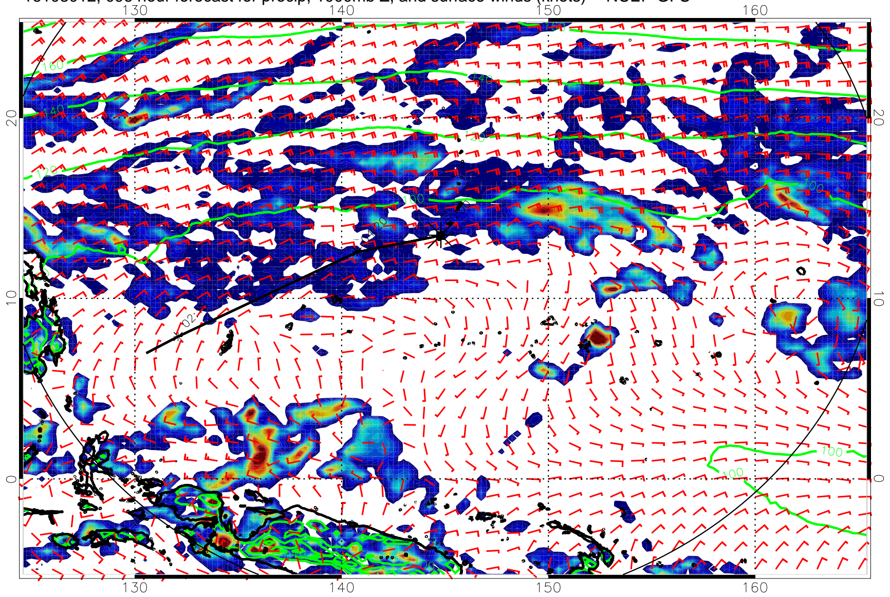
16103012, 096 hour forecast for precip, 1000mb Z, and surface winds (knots) -- NCEP GFS
