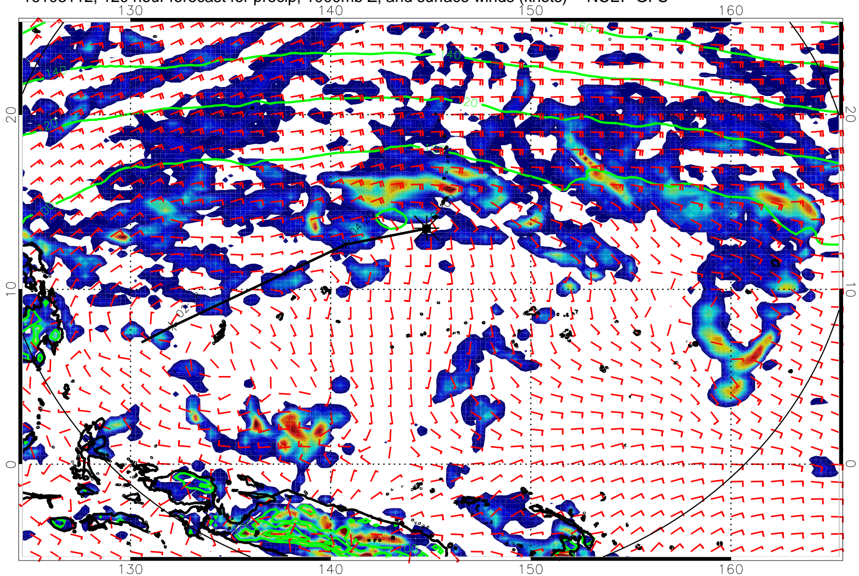
16103112, 120 hour forecast for precip, 1000mb Z, and surface winds (knots) -- NCEP GFS
