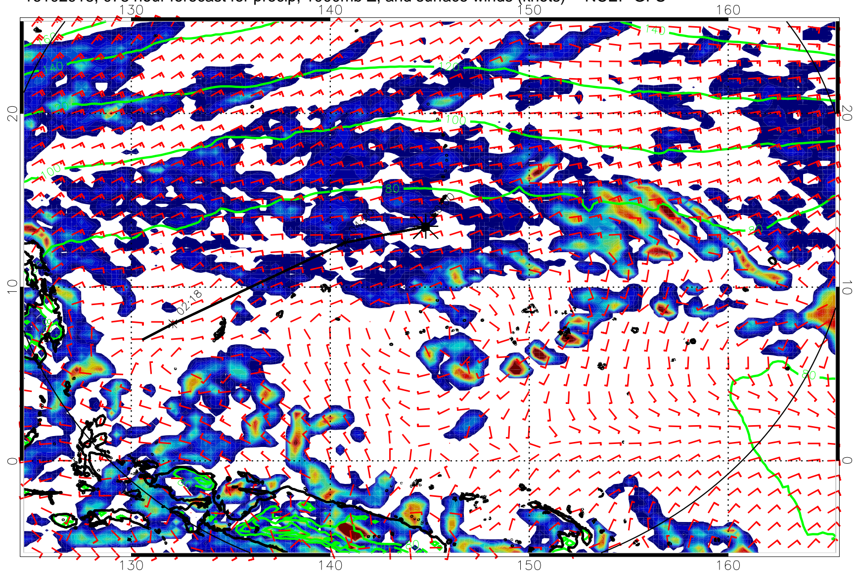
16102918, 078 hour forecast for precip, 1000mb Z, and surface winds (knots) -- NCEP GFS
