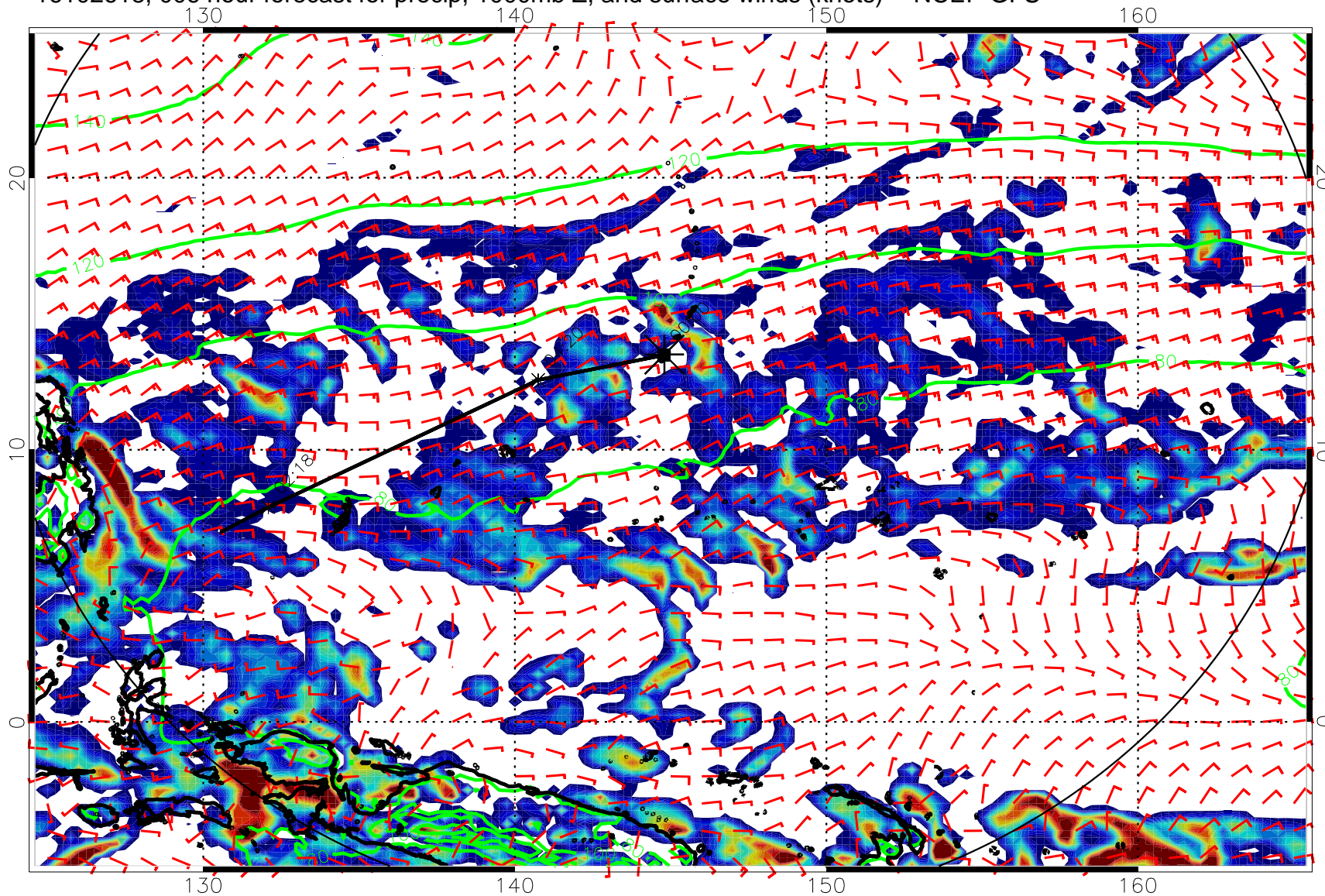
16102618, 006 hour forecast for precip, 1000mb Z, and surface winds (knots) -- NCEP GFS
