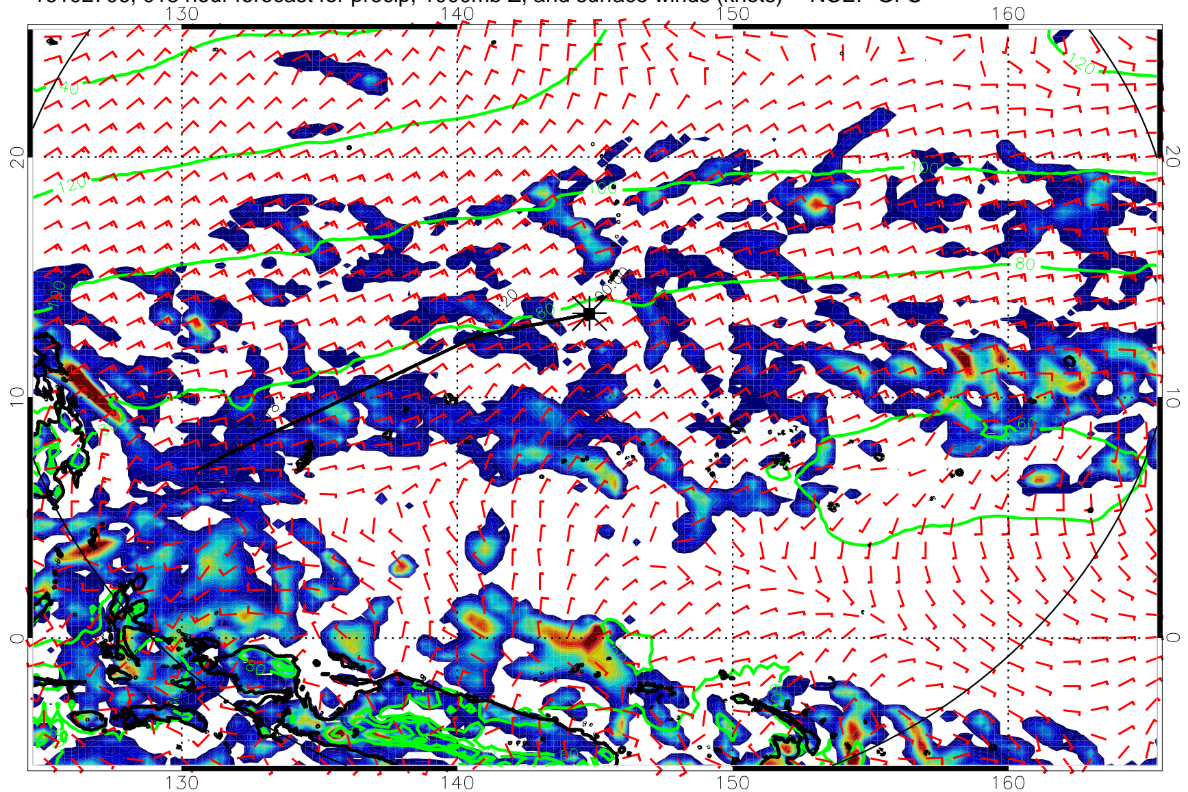
16102706, 018 hour forecast for precip, 1000mb Z, and surface winds (knots) -- NCEP GFS
