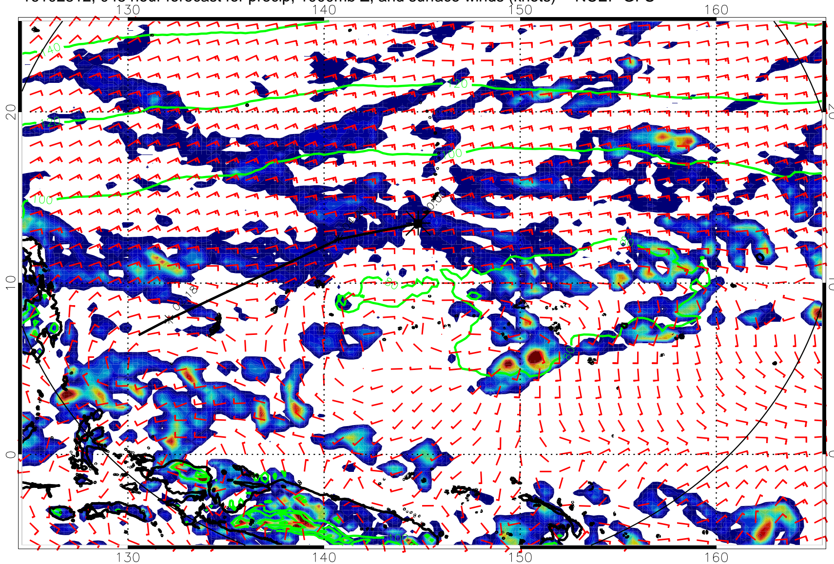
16102812, 048 hour forecast for precip, 1000mb Z, and surface winds (knots) -- NCEP GFS
