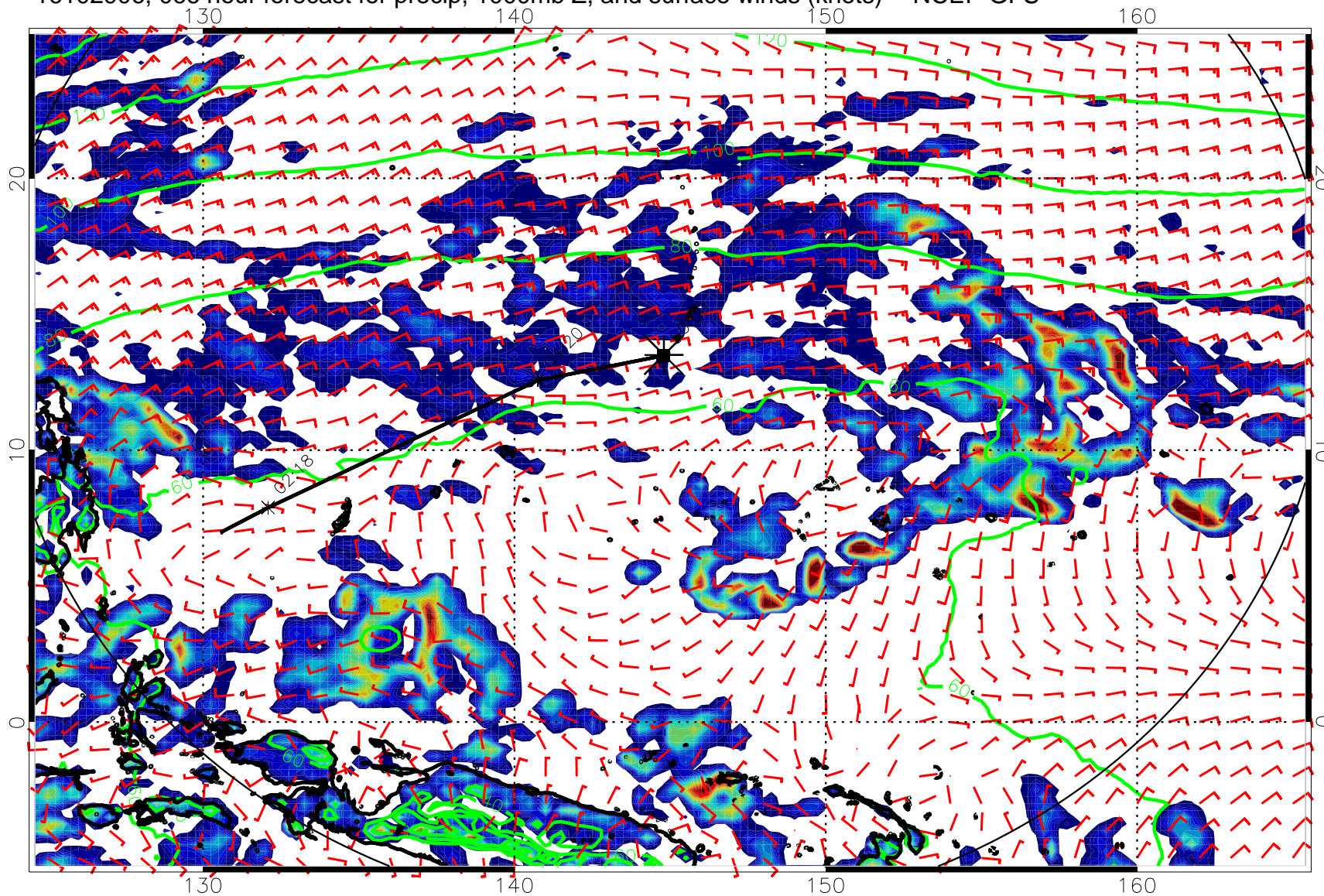
16102906, 066 hour forecast for precip, 1000mb Z, and surface winds (knots) -- NCEP GFS
