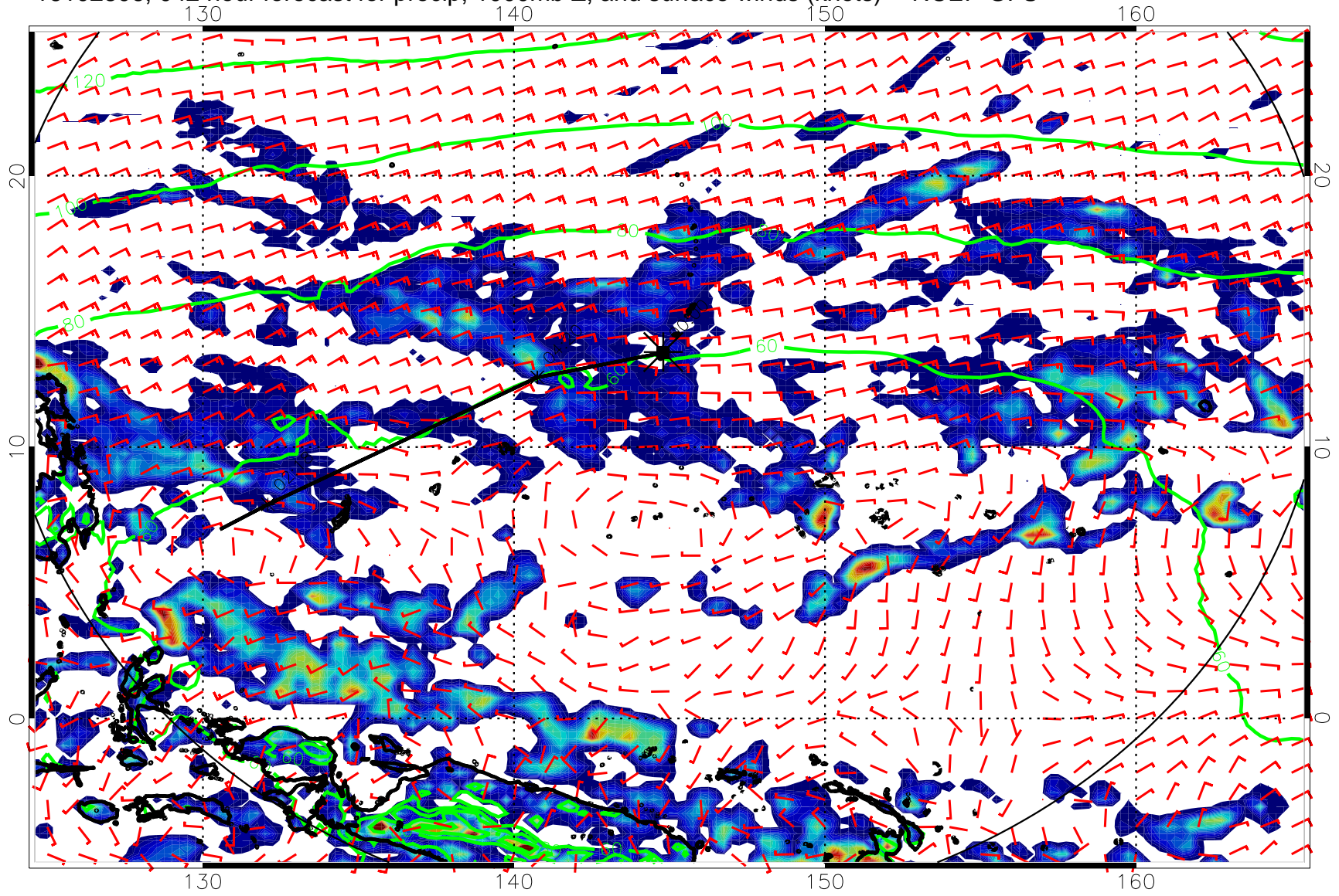
16102806, 042 hour forecast for precip, 1000mb Z, and surface winds (knots) -- NCEP GFS
