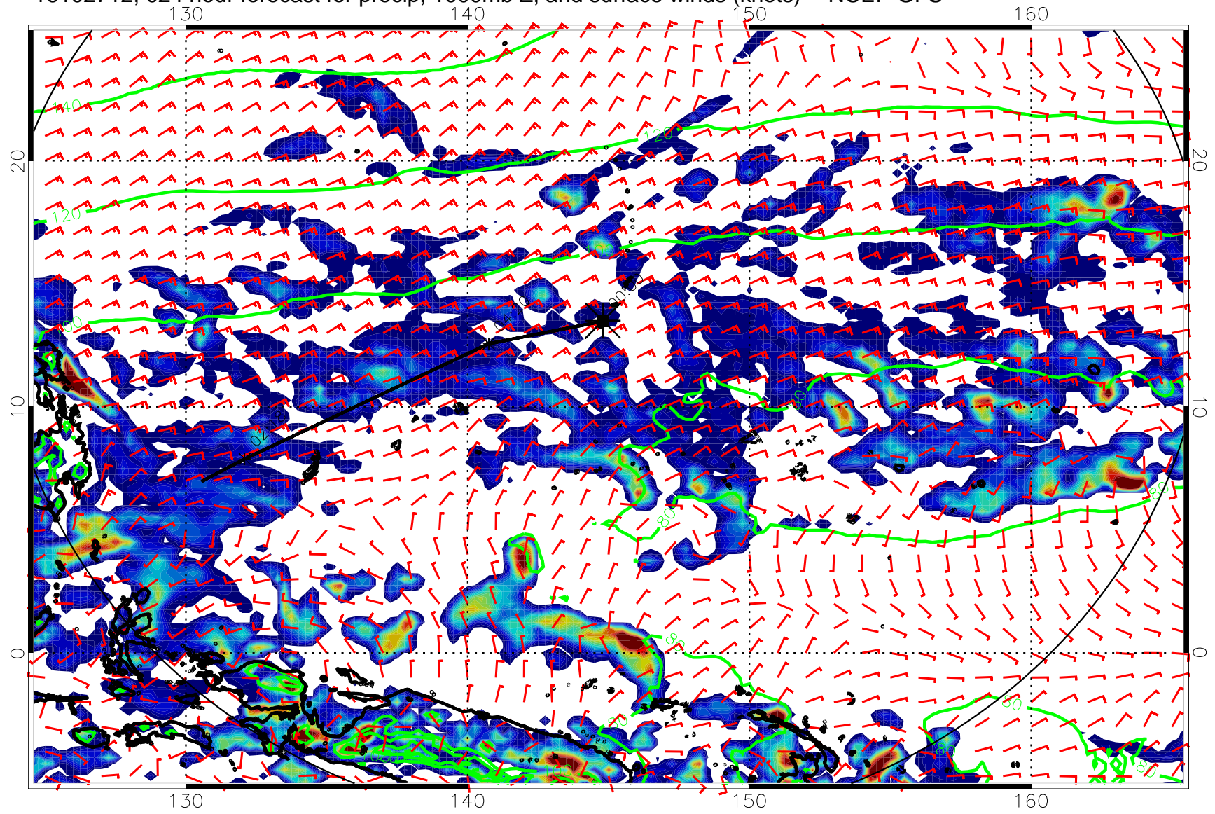
16102712, 024 hour forecast for precip, 1000mb Z, and surface winds (knots) -- NCEP GFS
