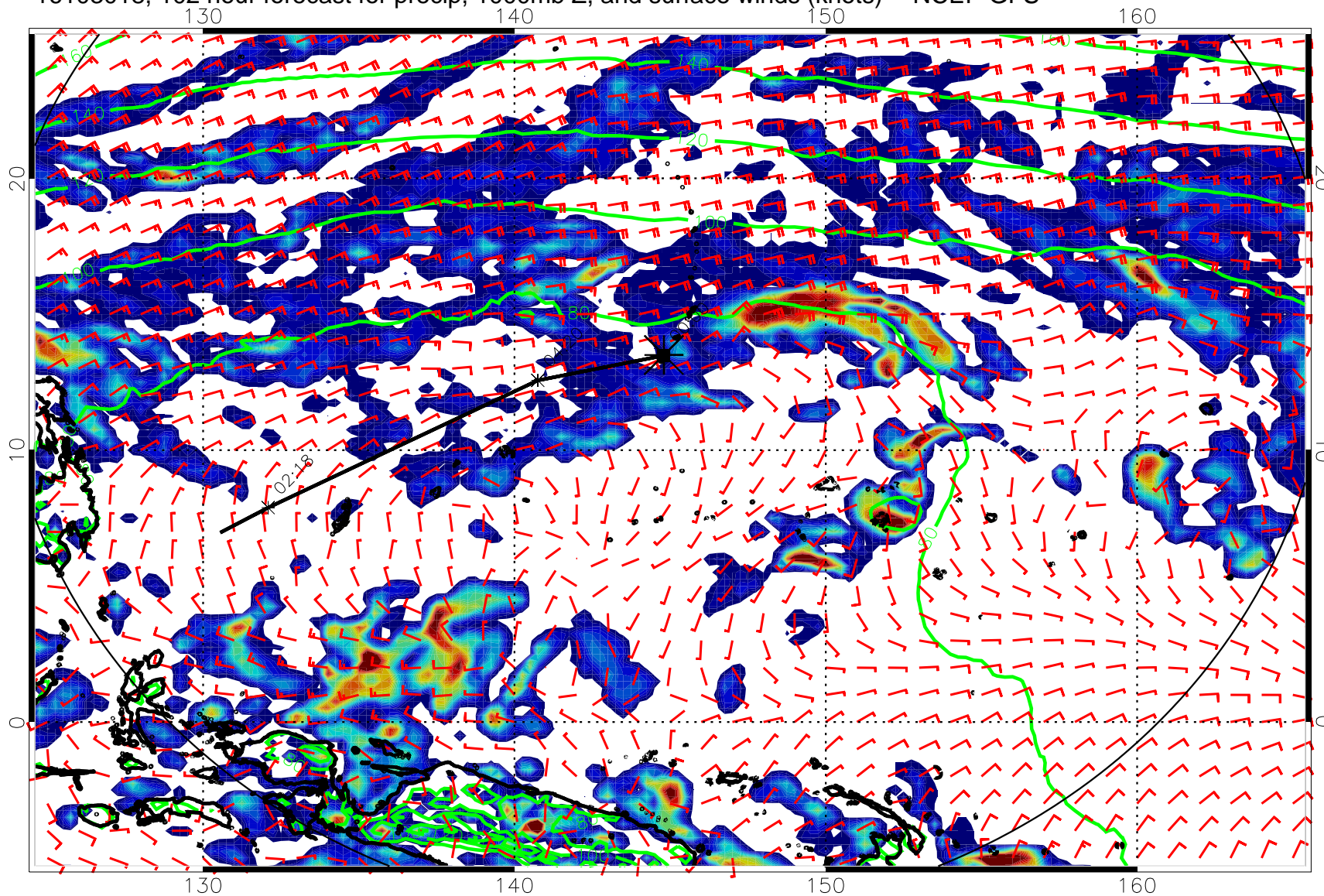
16103018, 102 hour forecast for precip, 1000mb Z, and surface winds (knots) -- NCEP GFS
