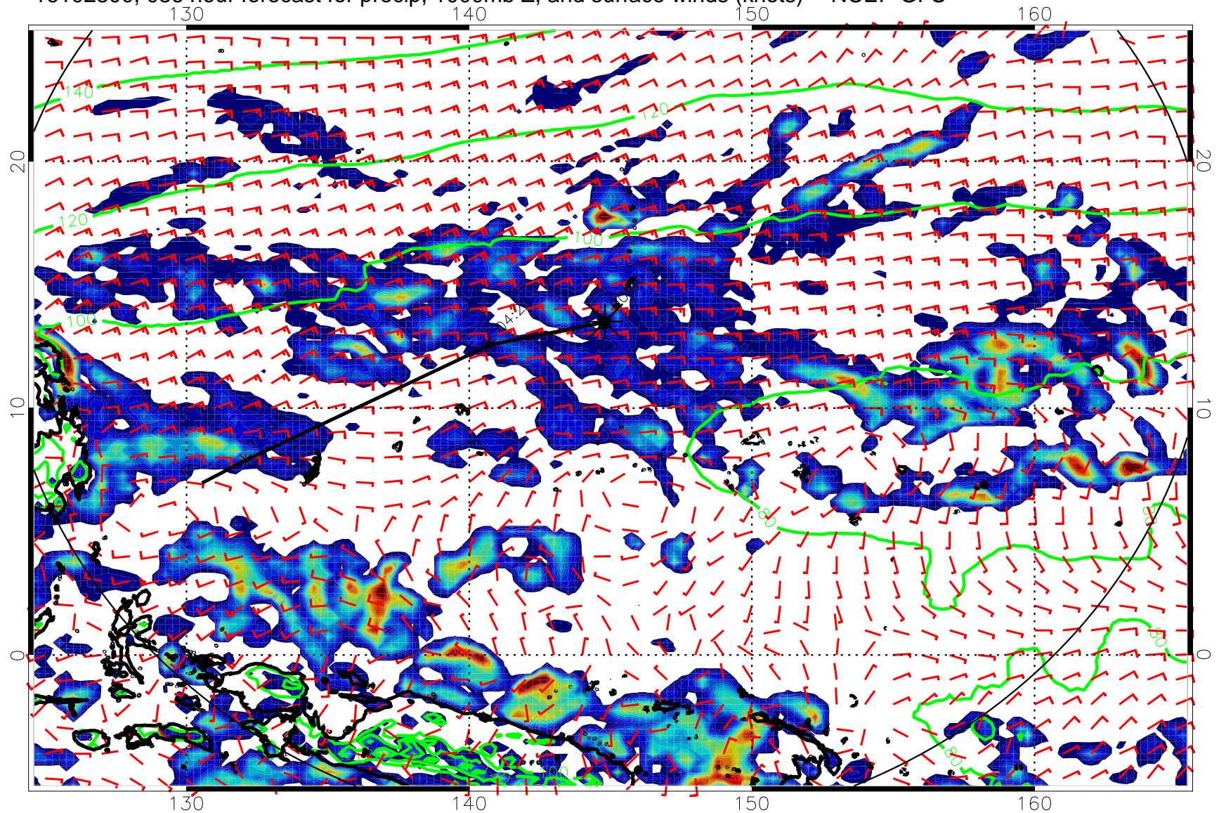
16102800, 036 hour forecast for precip, 1000mb Z, and surface winds (knots) -- NCEP GFS
