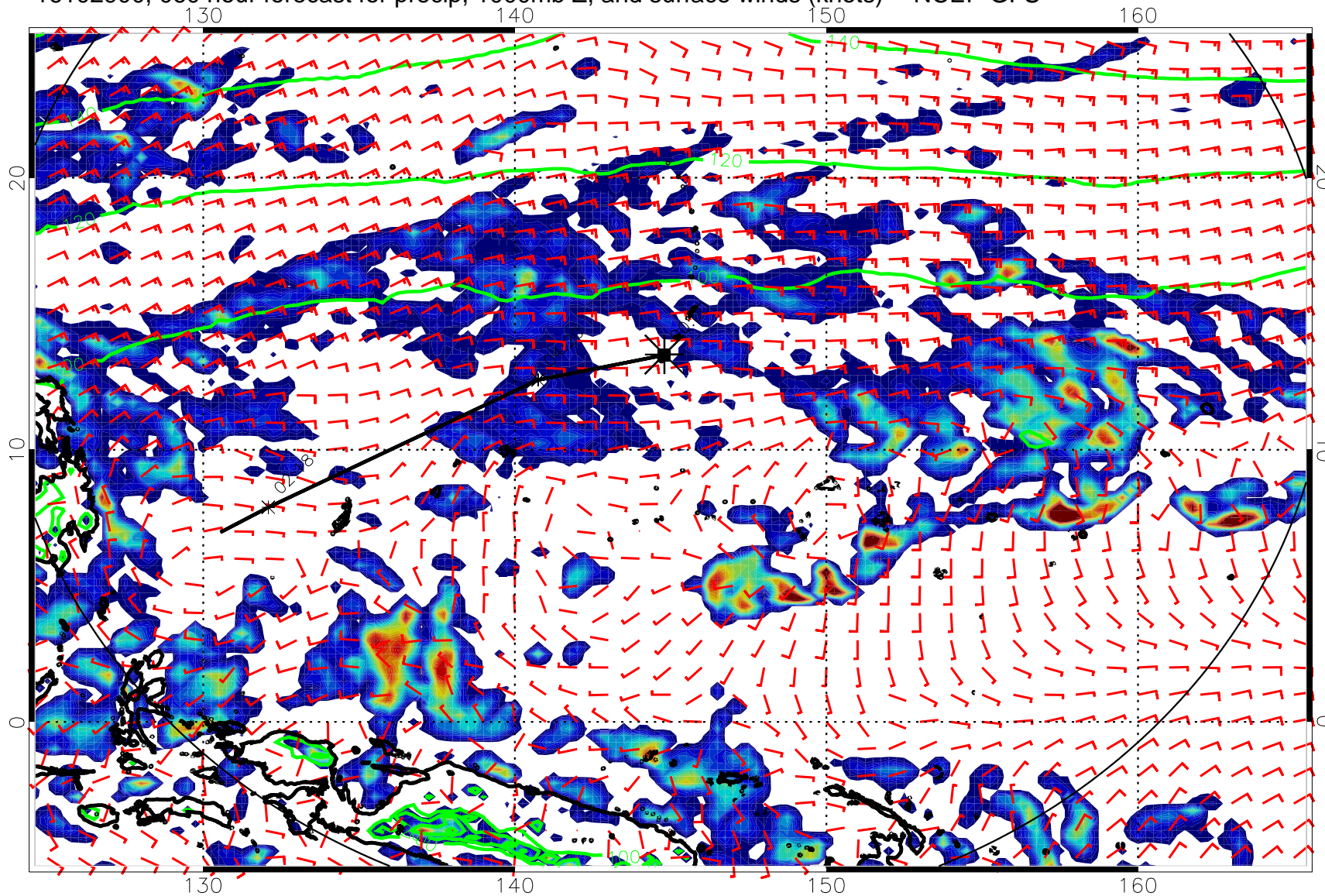
16102900, 060 hour forecast for precip, 1000mb Z, and surface winds (knots) -- NCEP GFS
