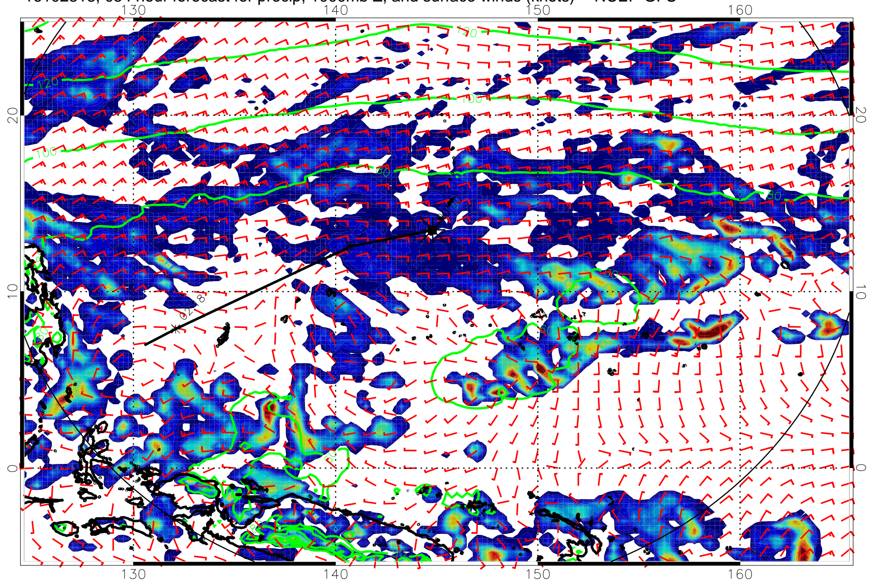
16102818, 054 hour forecast for precip, 1000mb Z, and surface winds (knots) -- NCEP GFS
