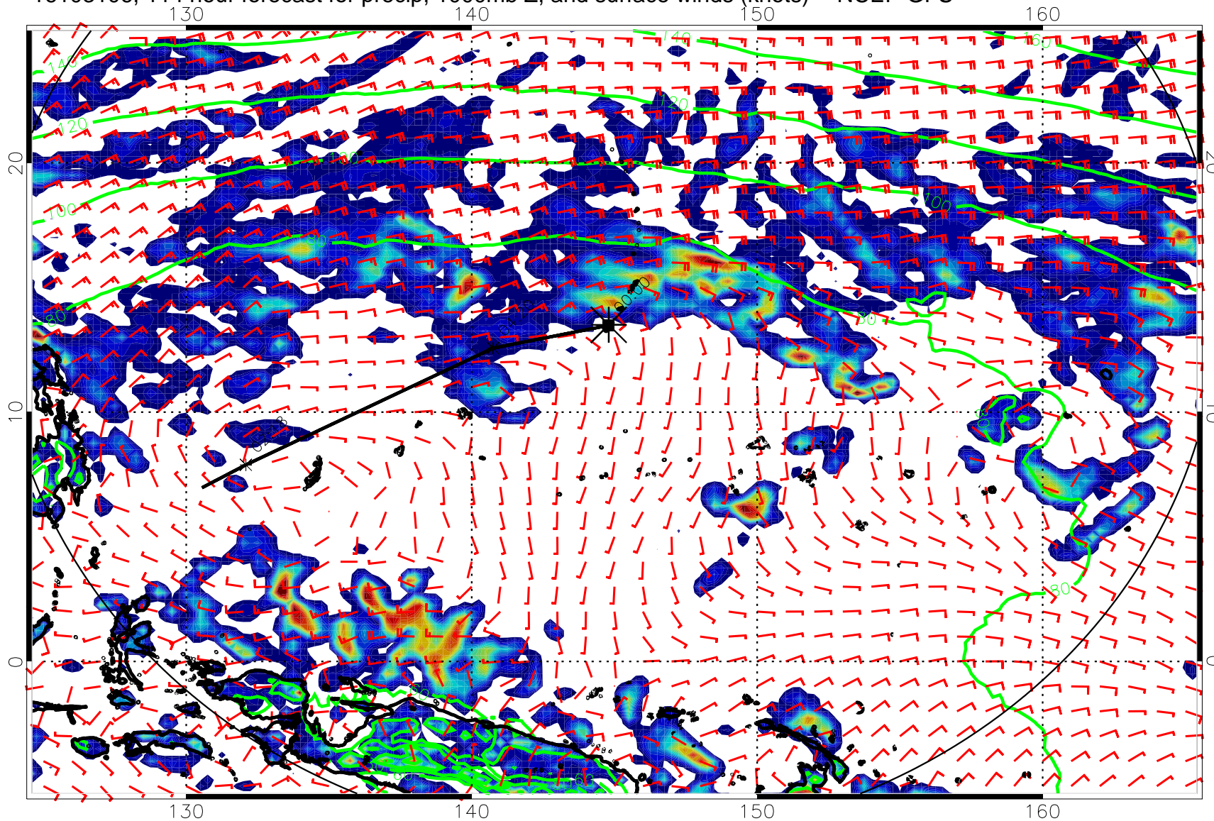
16103106, 114 hour forecast for precip, 1000mb Z, and surface winds (knots) -- NCEP GFS
