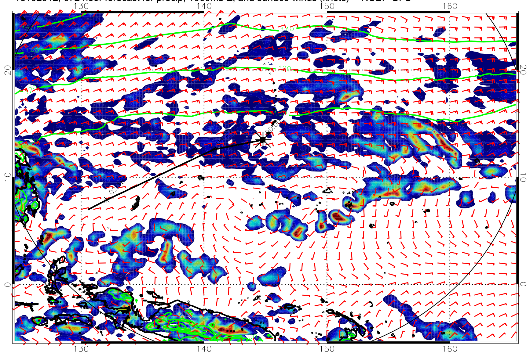
16102912, 072 hour forecast for precip, 1000mb Z, and surface winds (knots) -- NCEP GFS
