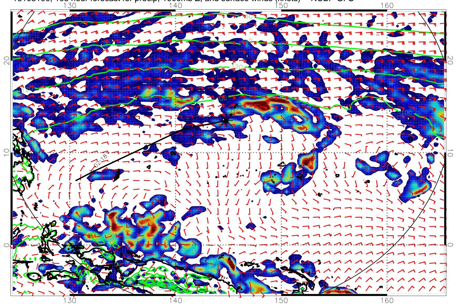
16103100, 108 hour forecast for precip, 1000mb Z, and surface winds (knots) -- NCEP GFS
