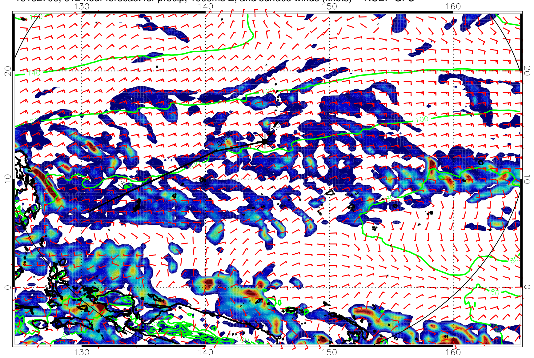
16102700, 012 hour forecast for precip, 1000mb Z, and surface winds (knots) -- NCEP GFS
