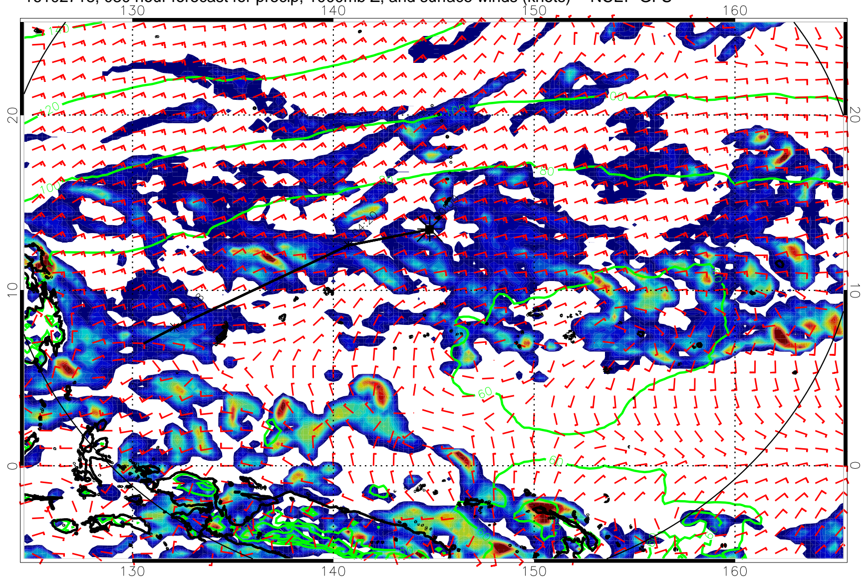
16102718, 030 hour forecast for precip, 1000mb Z, and surface winds (knots) -- NCEP GFS
