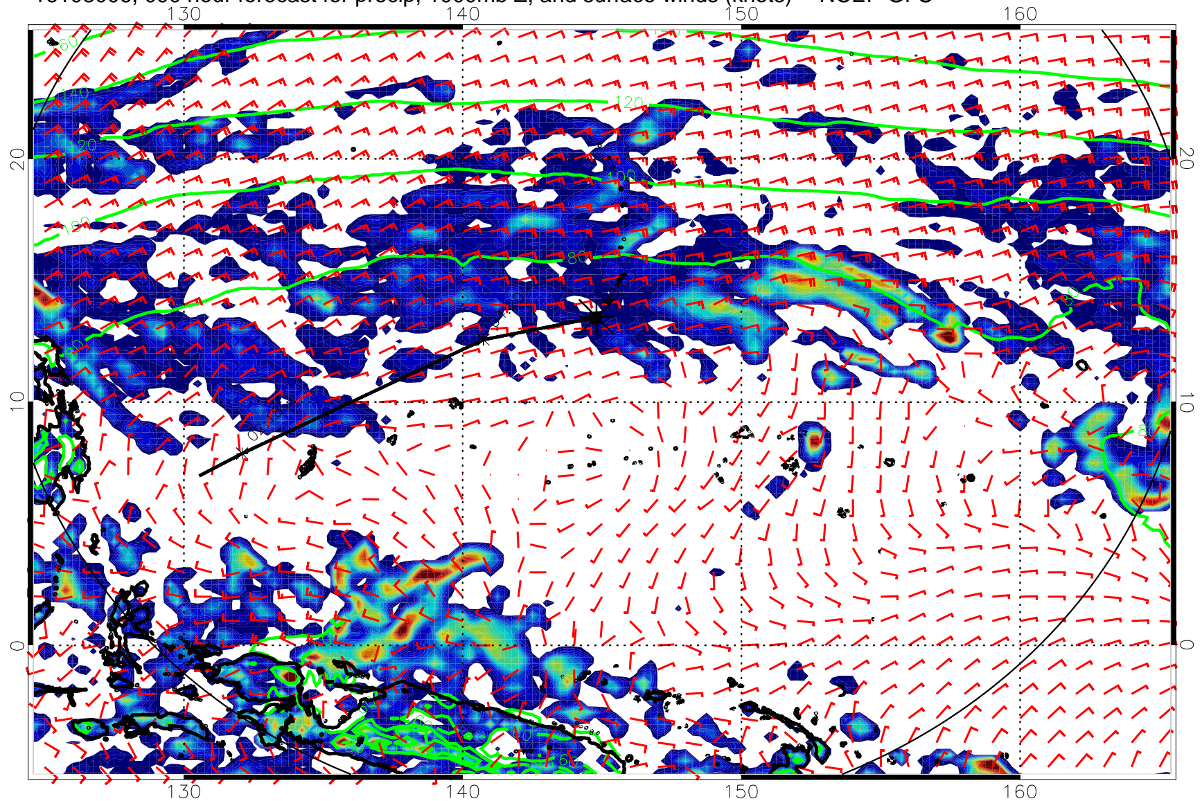
16103006, 090 hour forecast for precip, 1000mb Z, and surface winds (knots) -- NCEP GFS
