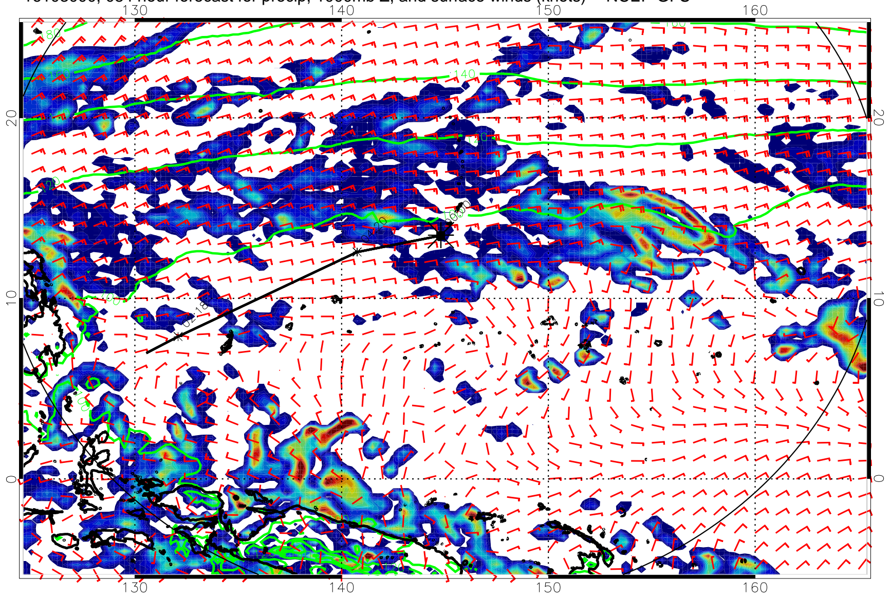
16103000, 084 hour forecast for precip, 1000mb Z, and surface winds (knots) -- NCEP GFS
