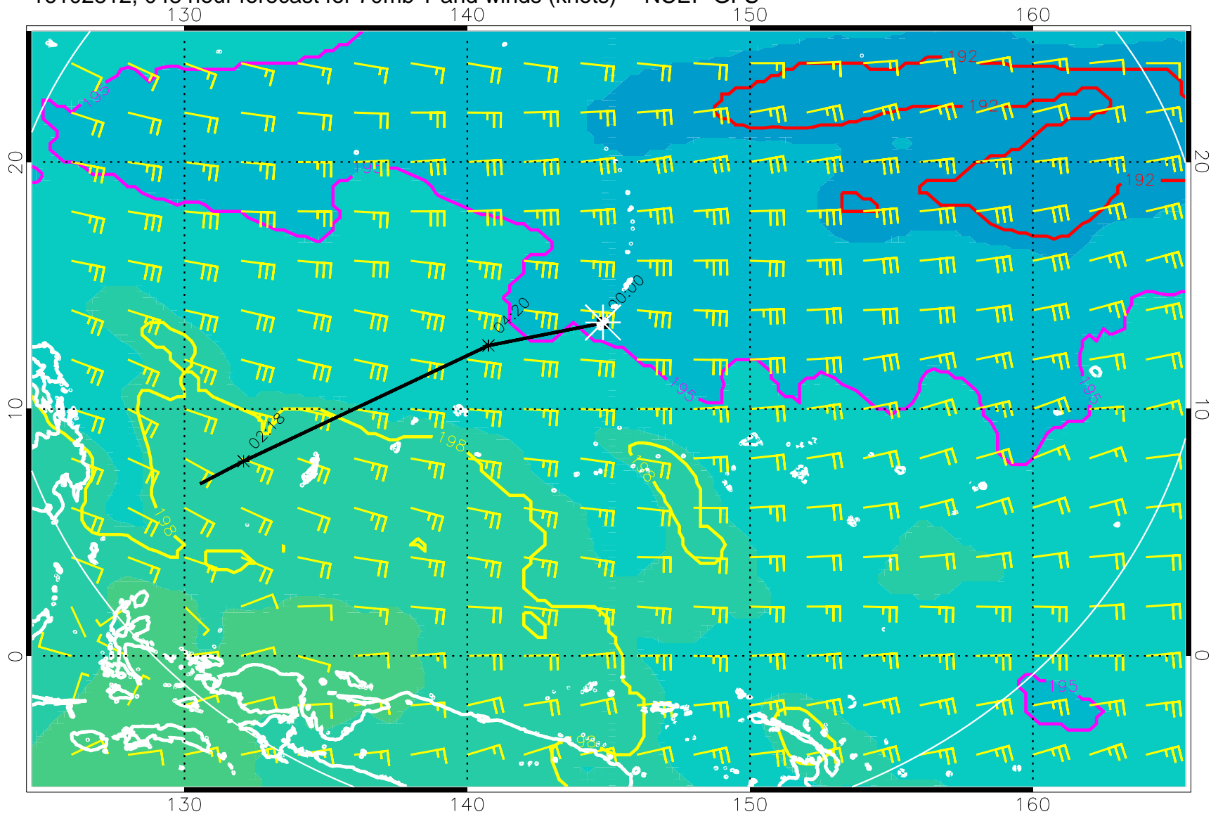
16102812, 048 hour forecast for 70mb T and winds (knots) -- NCEP GFS
