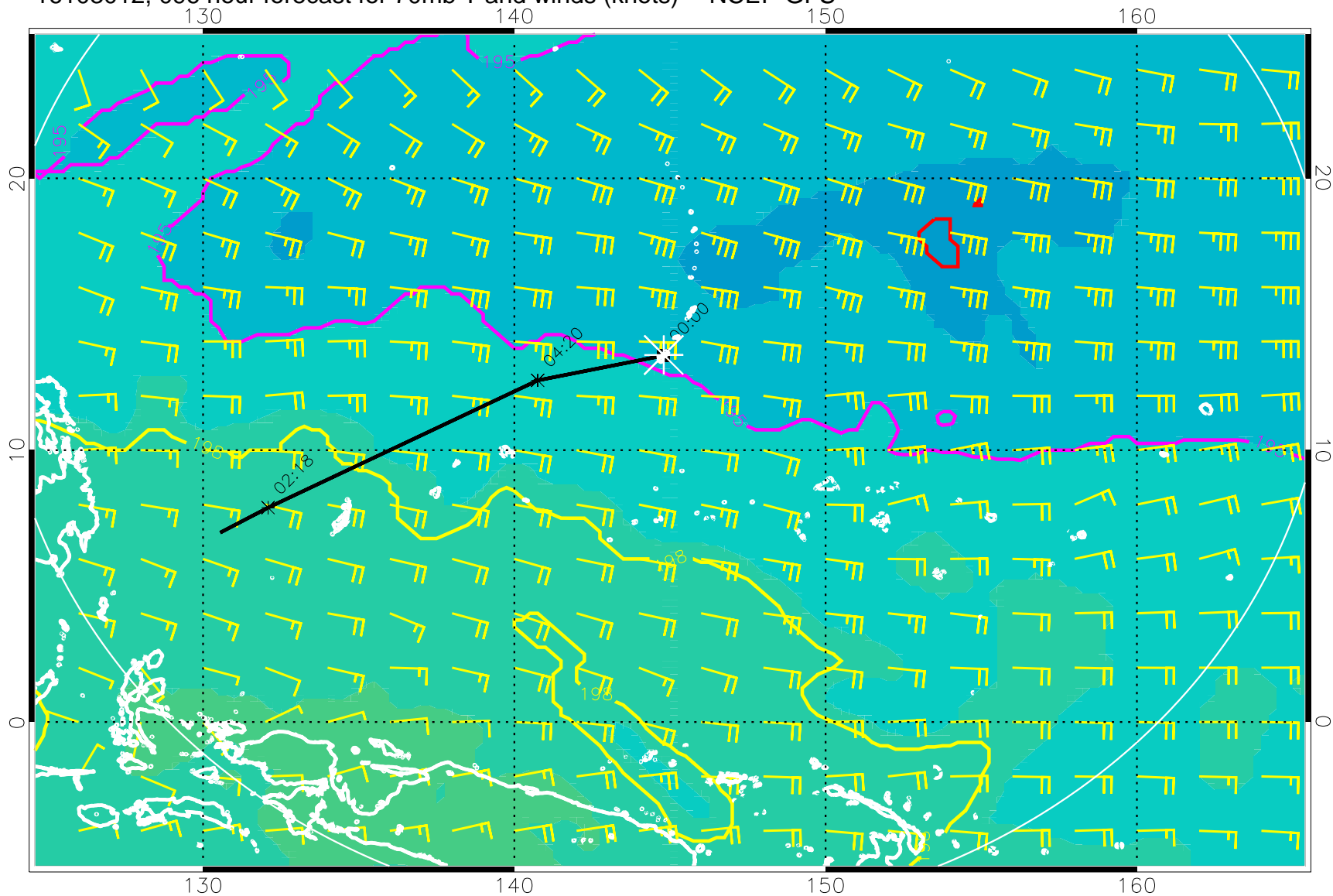
16103012, 096 hour forecast for 70mb T and winds (knots) -- NCEP GFS
