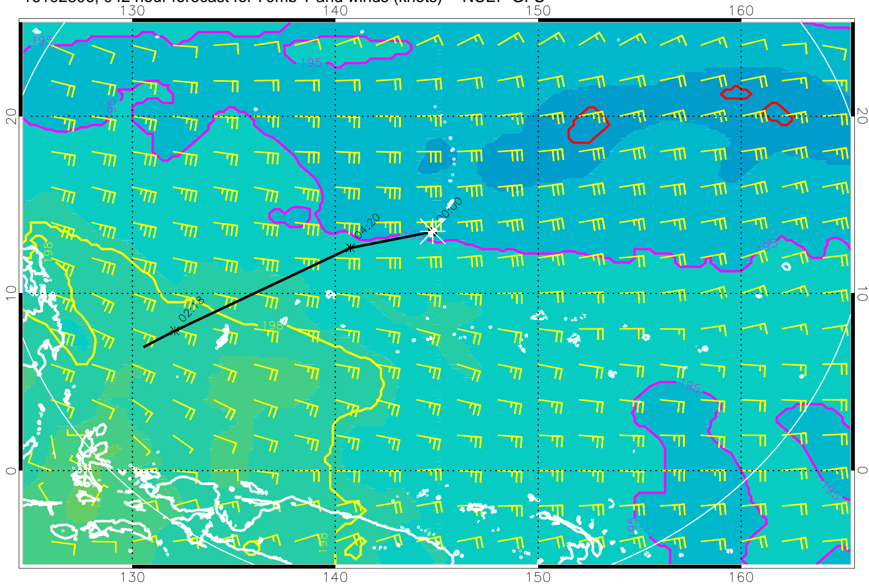
16102806, 042 hour forecast for 70mb T and winds (knots) -- NCEP GFS
