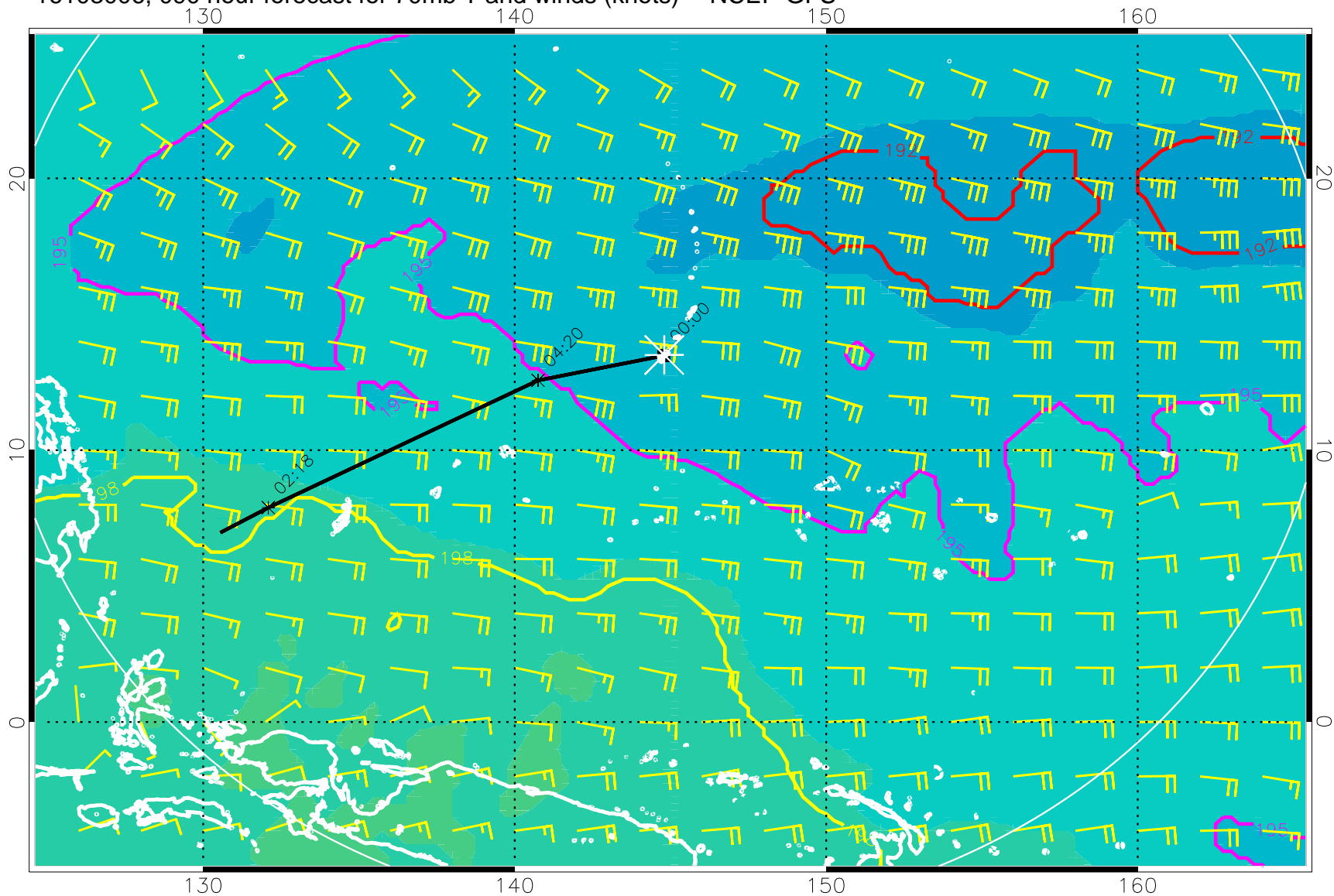
16103006, 090 hour forecast for 70mb T and winds (knots) -- NCEP GFS
