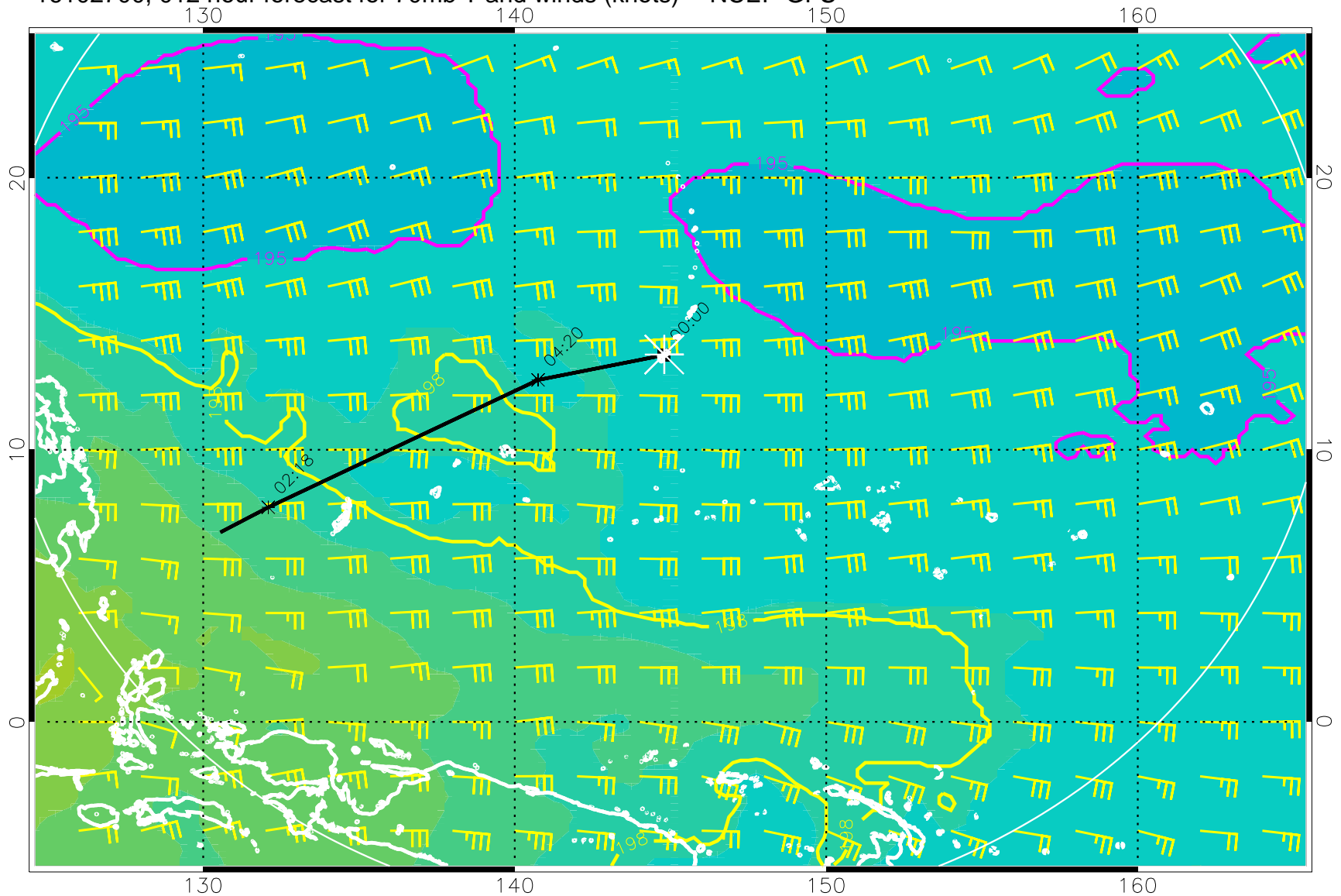
16102700, 012 hour forecast for 70mb T and winds (knots) -- NCEP GFS
