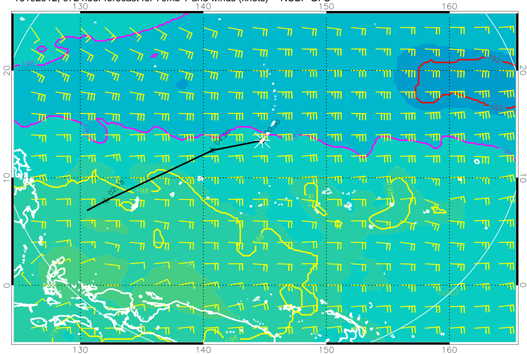
16102912, 072 hour forecast for 70mb T and winds (knots) -- NCEP GFS
