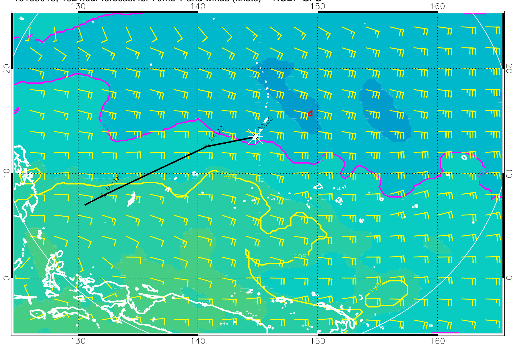
16103018, 102 hour forecast for 70mb T and winds (knots) -- NCEP GFS
