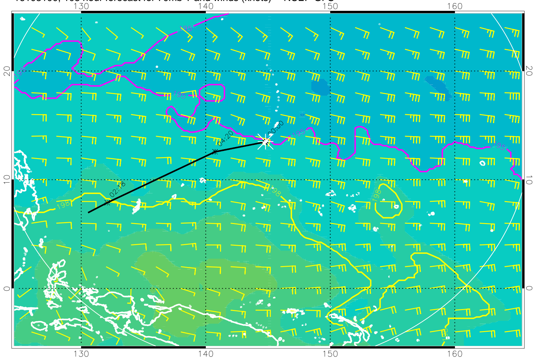
16103100, 108 hour forecast for 70mb T and winds (knots) -- NCEP GFS
