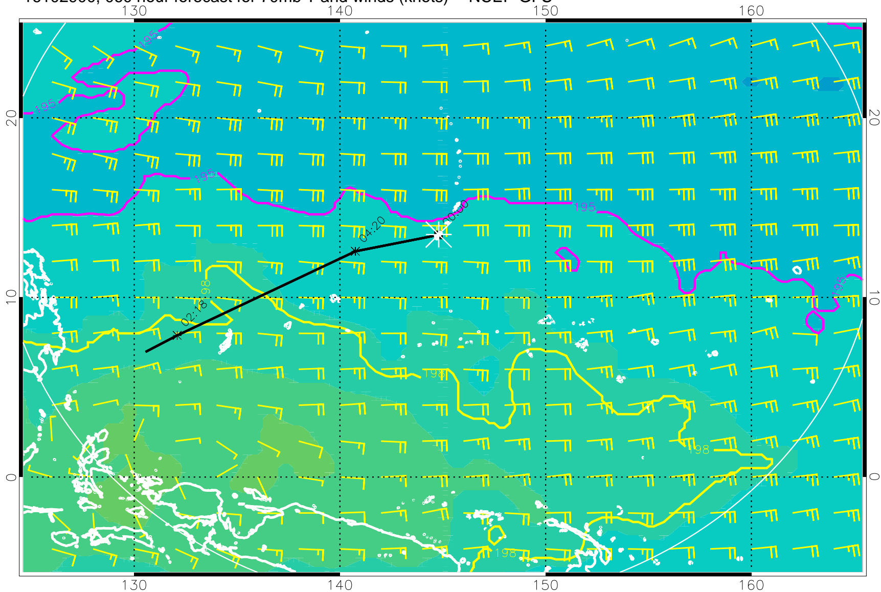
16102900, 060 hour forecast for 70mb T and winds (knots) -- NCEP GFS
