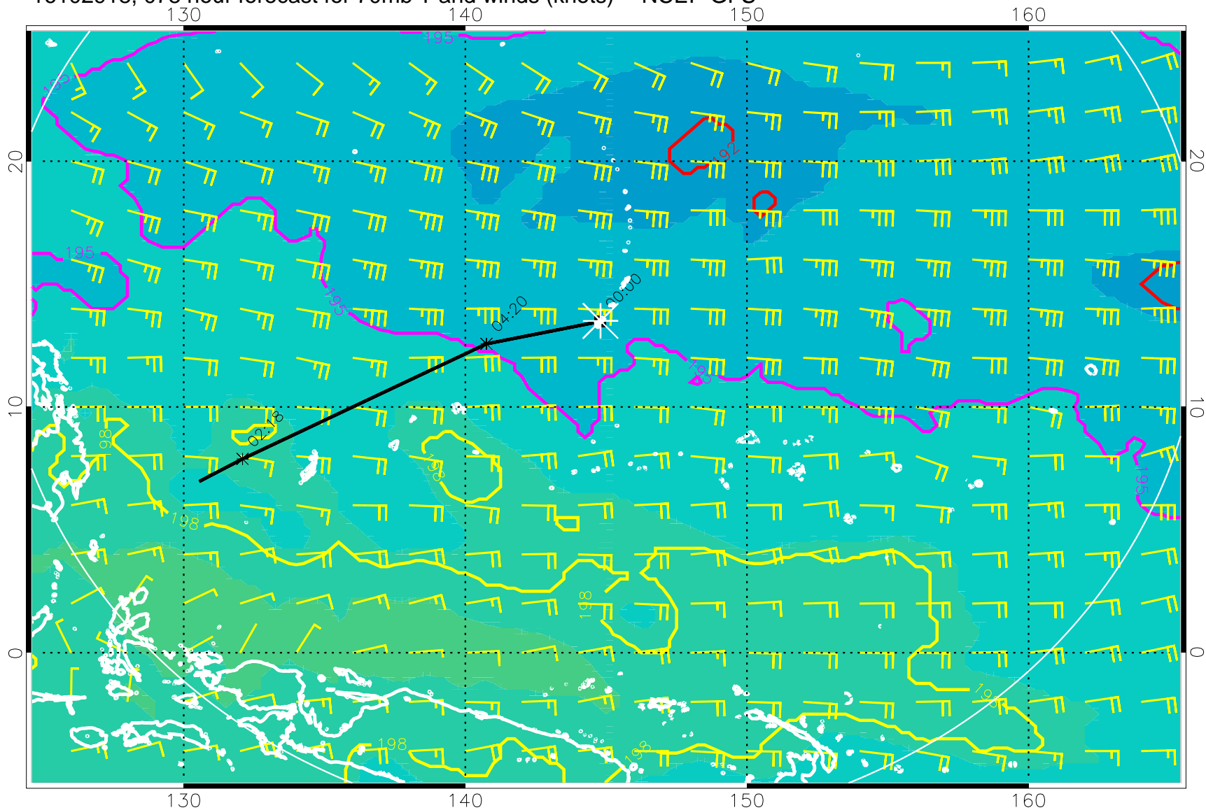
16102918, 078 hour forecast for 70mb T and winds (knots) -- NCEP GFS
