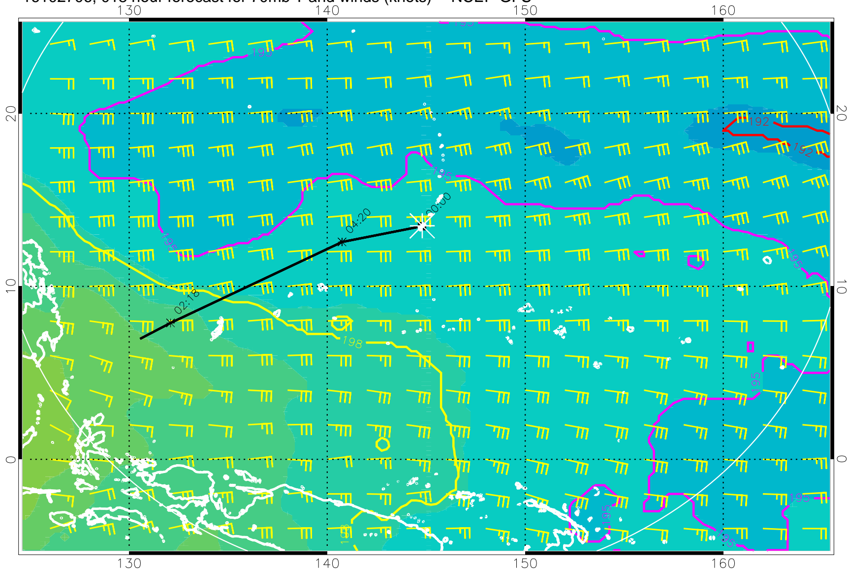
16102706, 018 hour forecast for 70mb T and winds (knots) -- NCEP GFS
