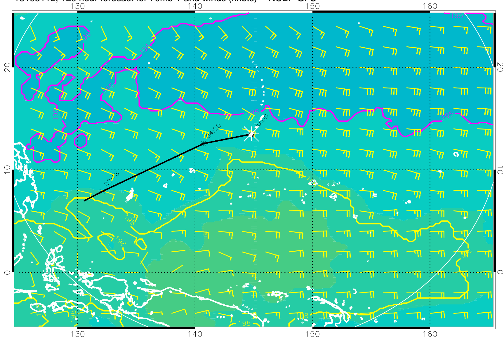
16103112, 120 hour forecast for 70mb T and winds (knots) -- NCEP GFS
