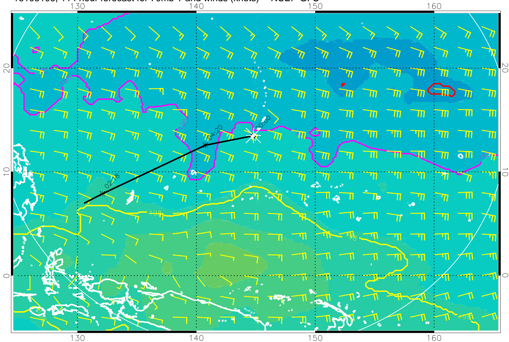
16103106, 114 hour forecast for 70mb T and winds (knots) -- NCEP GFS
