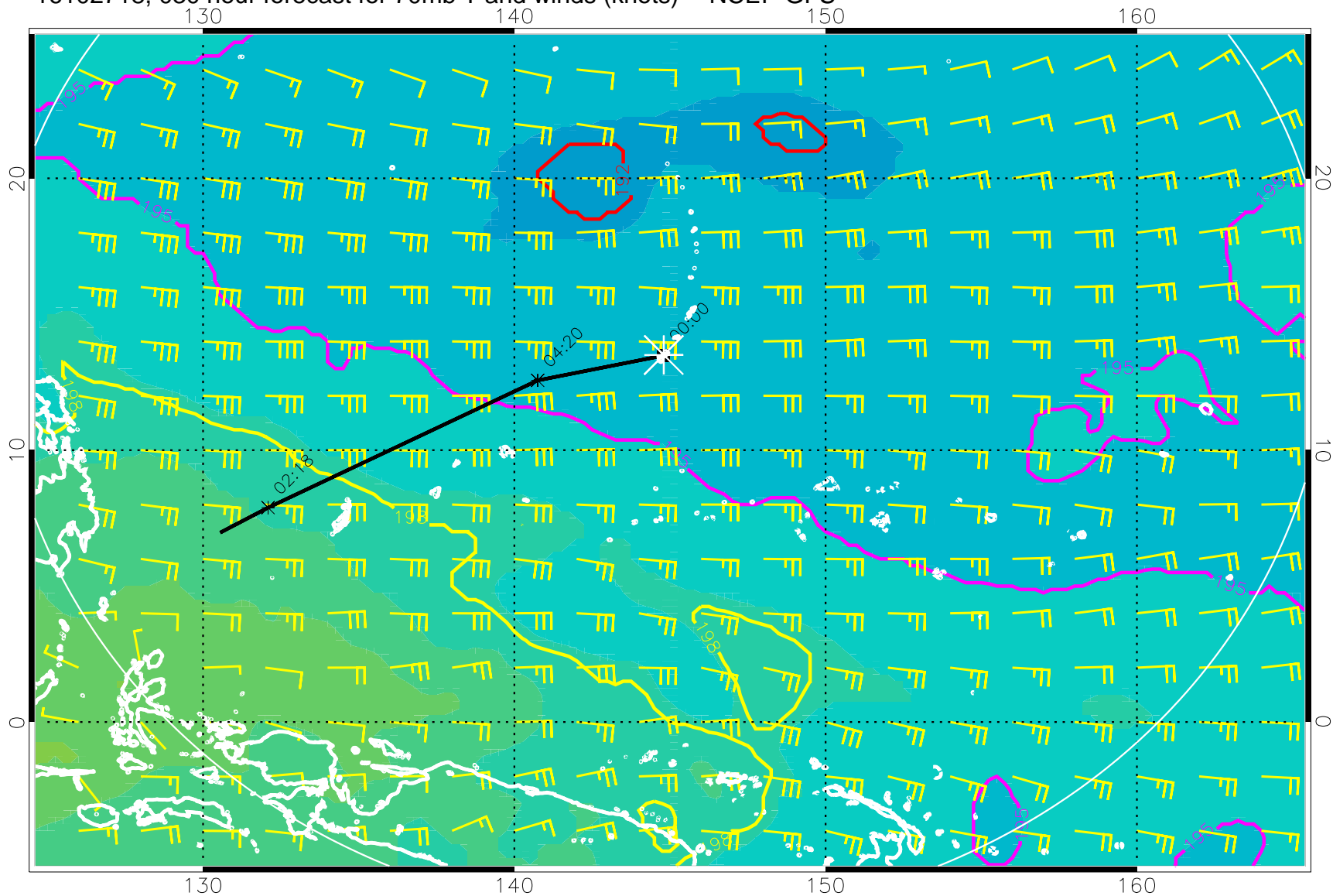
16102718, 030 hour forecast for 70mb T and winds (knots) -- NCEP GFS
