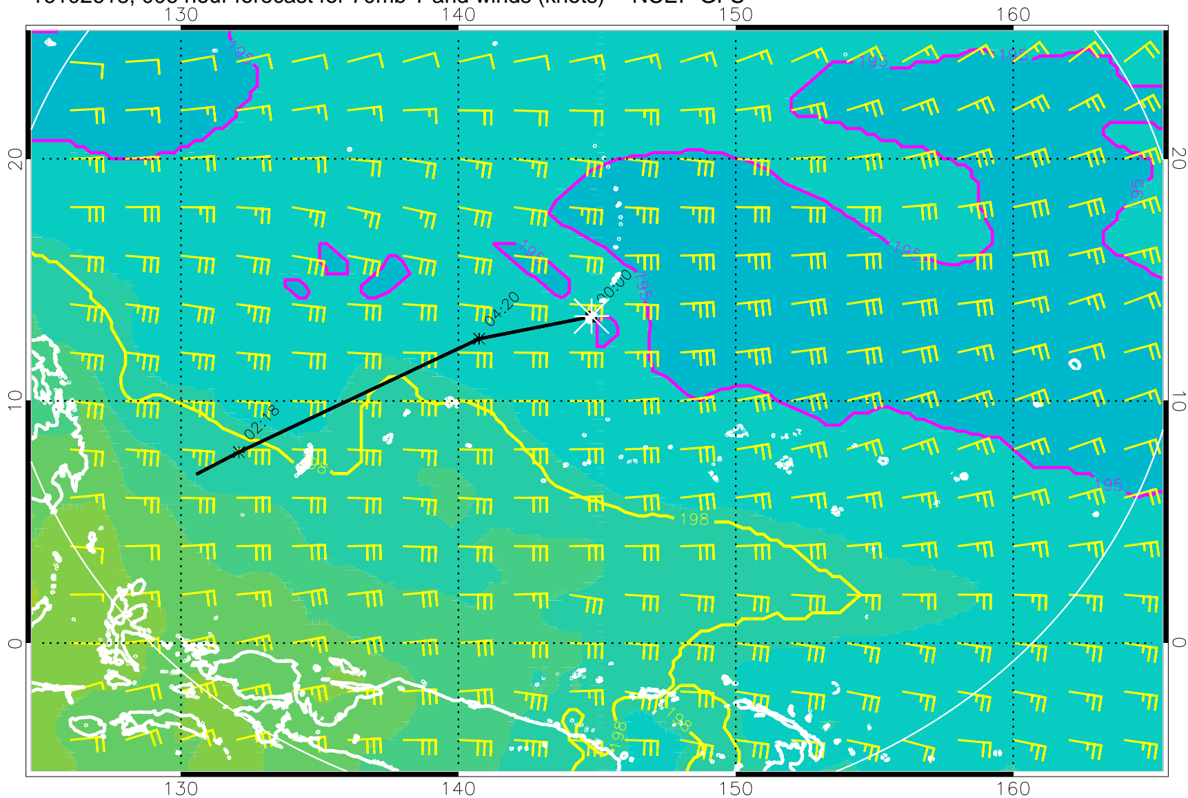
16102618, 006 hour forecast for 70mb T and winds (knots) -- NCEP GFS
