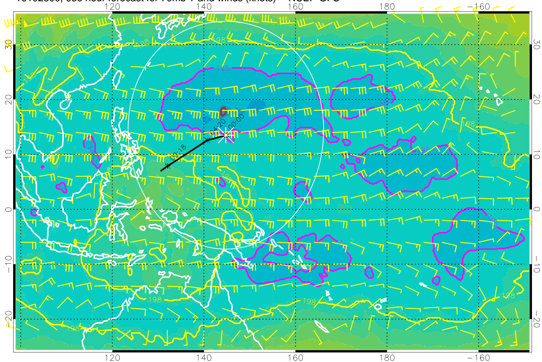
16102800, 036 hour forecast for 70mb T and winds (knots) -- NCEP GFS
