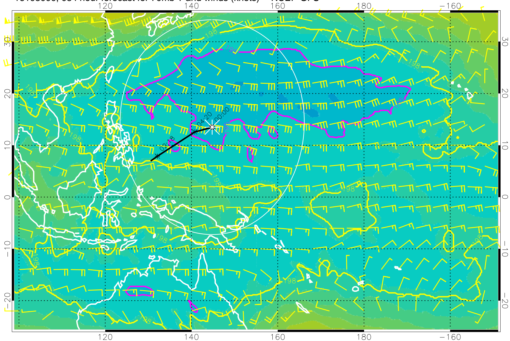
16103000, 084 hour forecast for 70mb T and winds (knots) -- NCEP GFS
