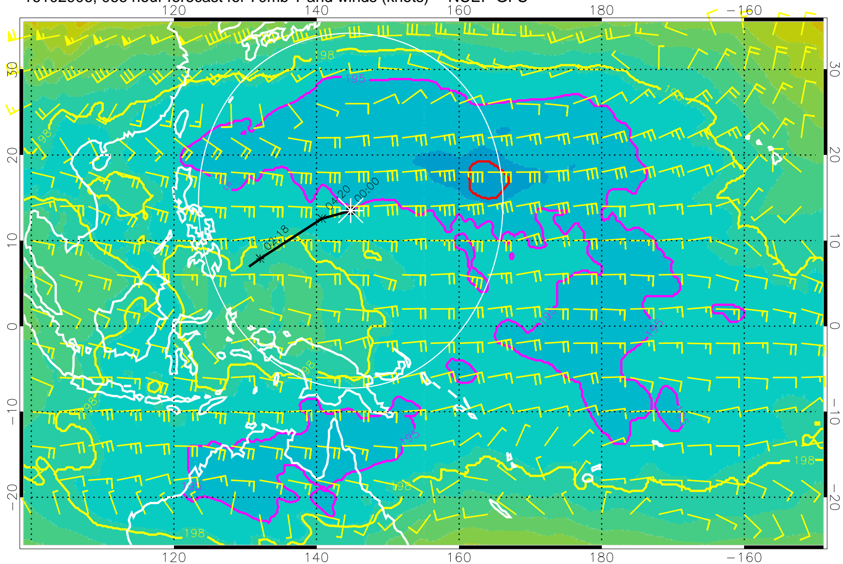
16102906, 066 hour forecast for 70mb T and winds (knots) -- NCEP GFS
