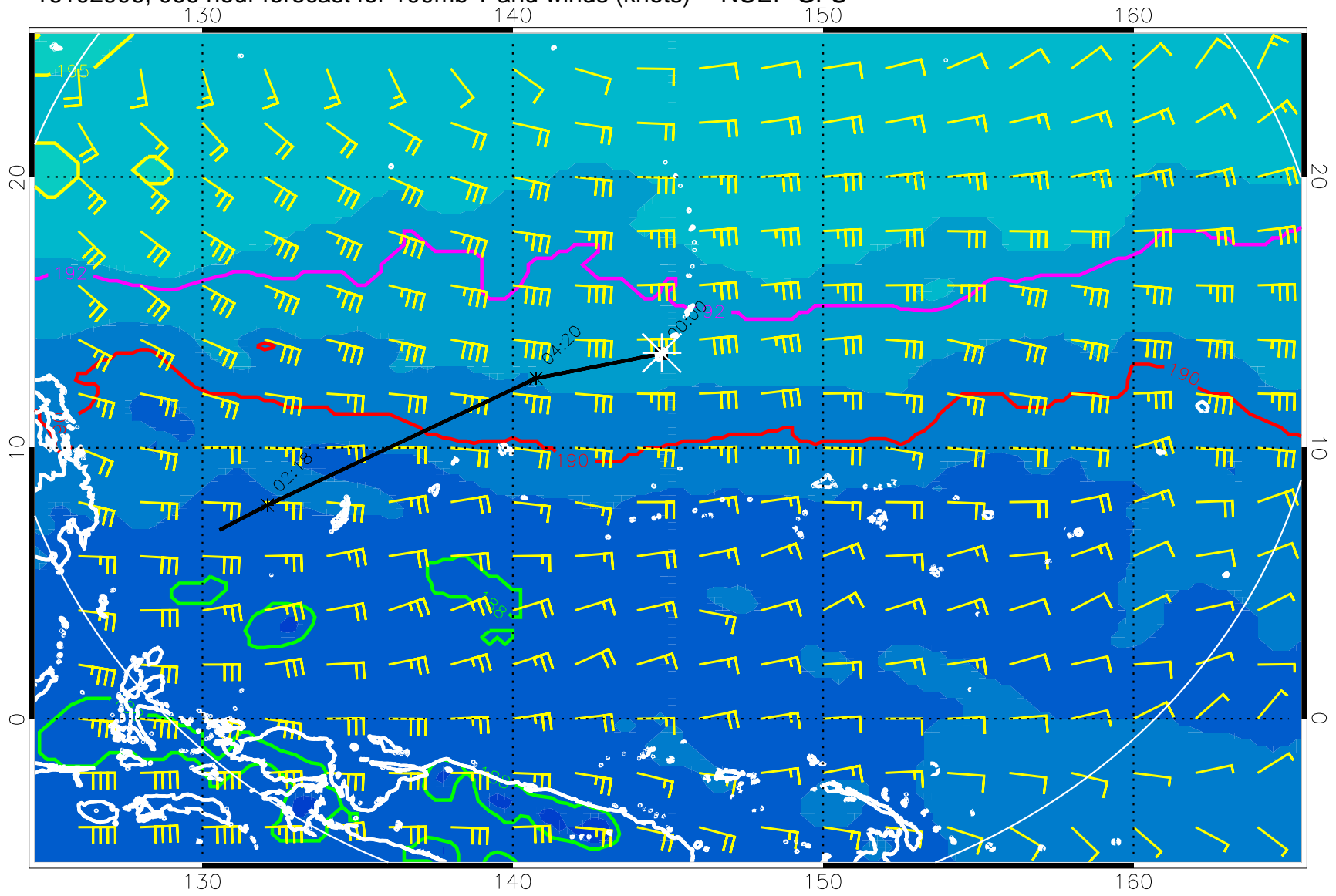
16102906, 066 hour forecast for 100mb T and winds (knots) -- NCEP GFS
