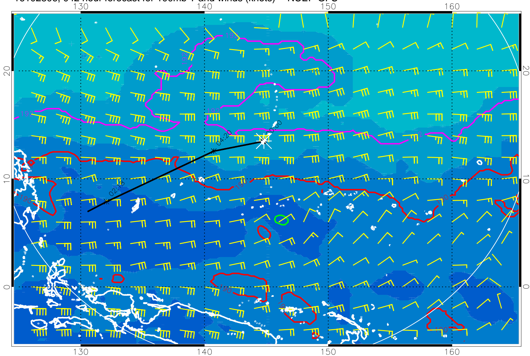
16102806, 042 hour forecast for 100mb T and winds (knots) -- NCEP GFS
