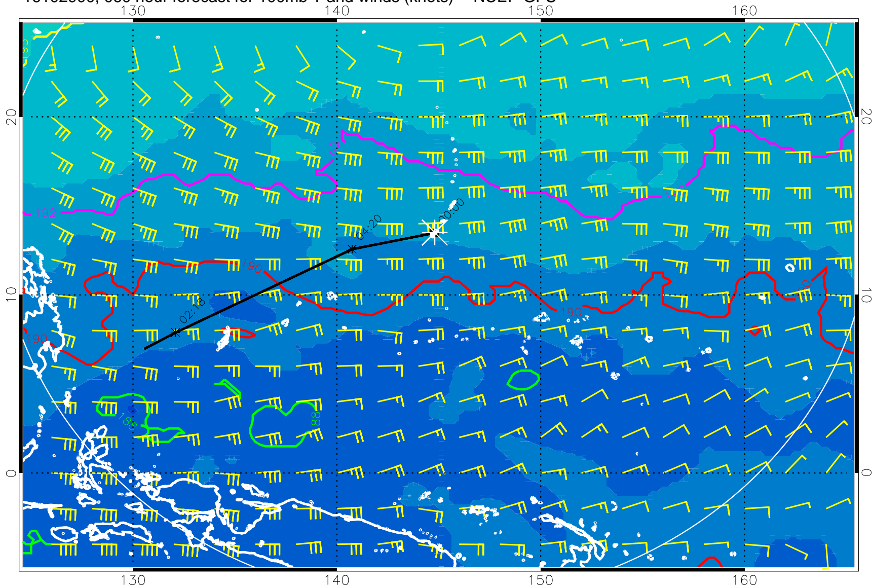
16102900, 060 hour forecast for 100mb T and winds (knots) -- NCEP GFS
