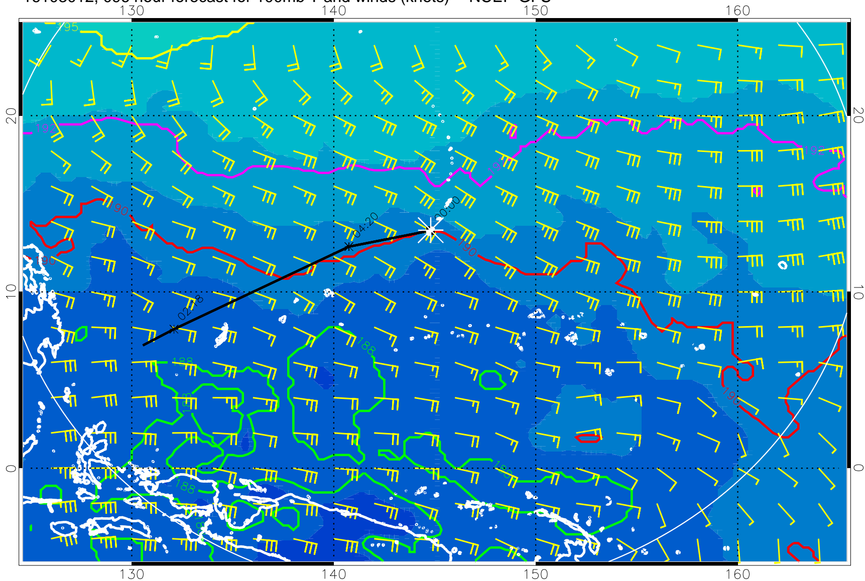
16103012, 096 hour forecast for 100mb T and winds (knots) -- NCEP GFS
