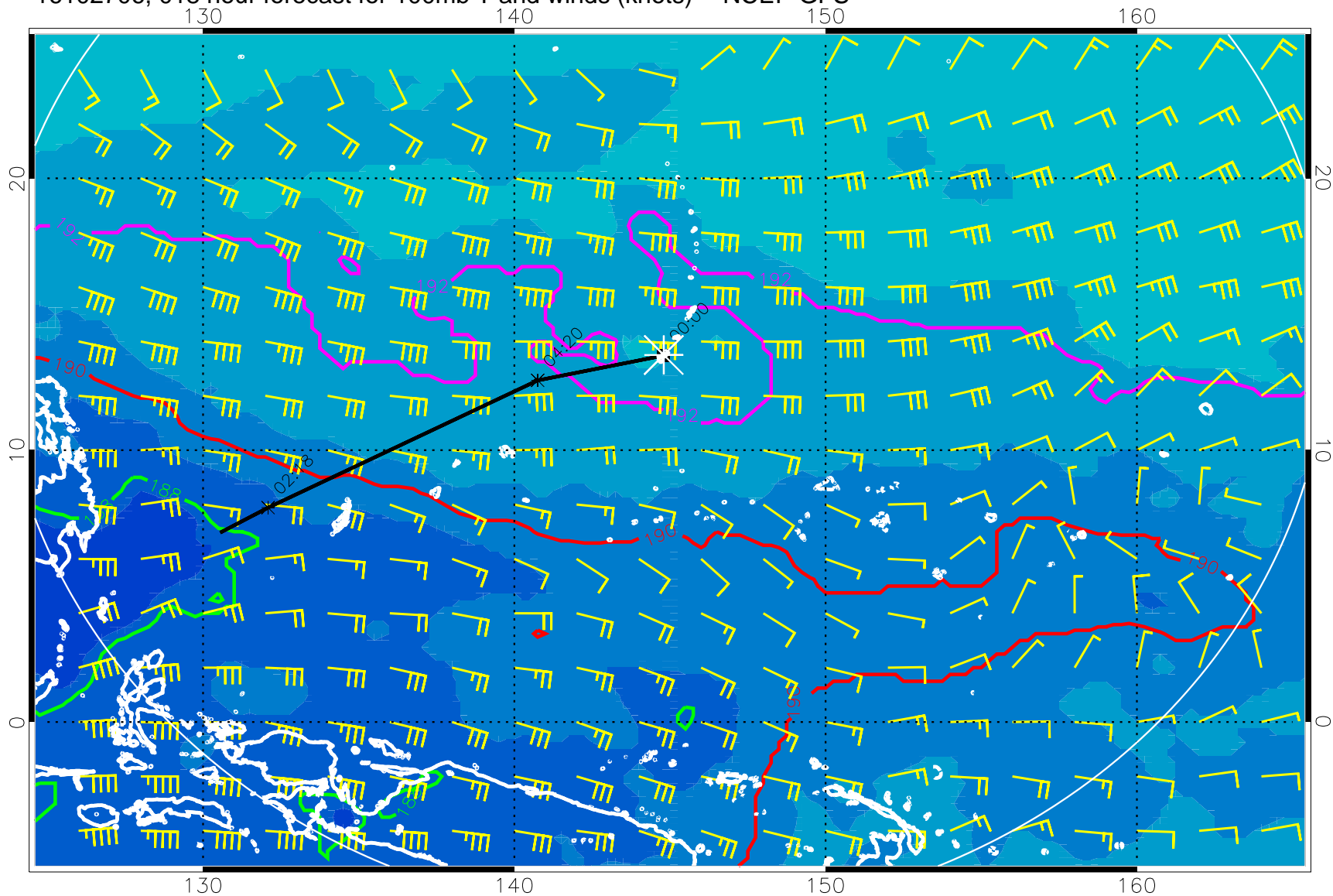
16102706, 018 hour forecast for 100mb T and winds (knots) -- NCEP GFS
