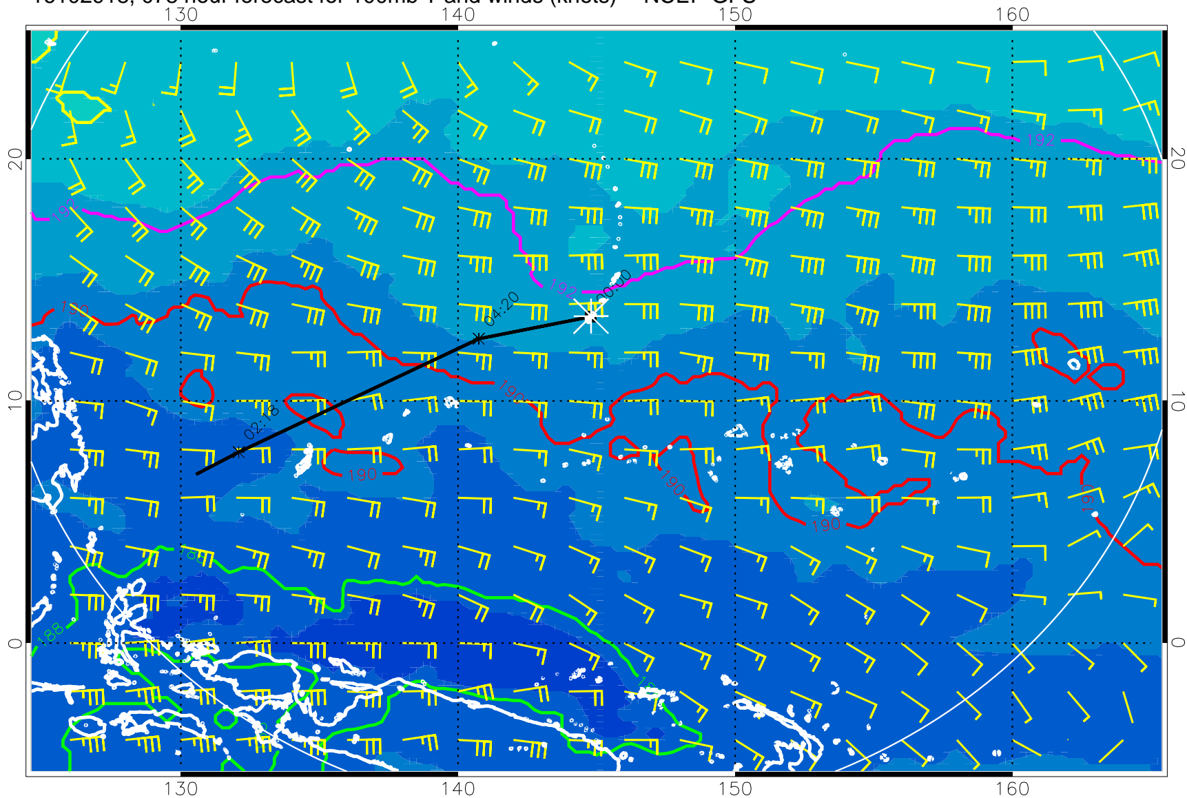
16102918, 078 hour forecast for 100mb T and winds (knots) -- NCEP GFS
