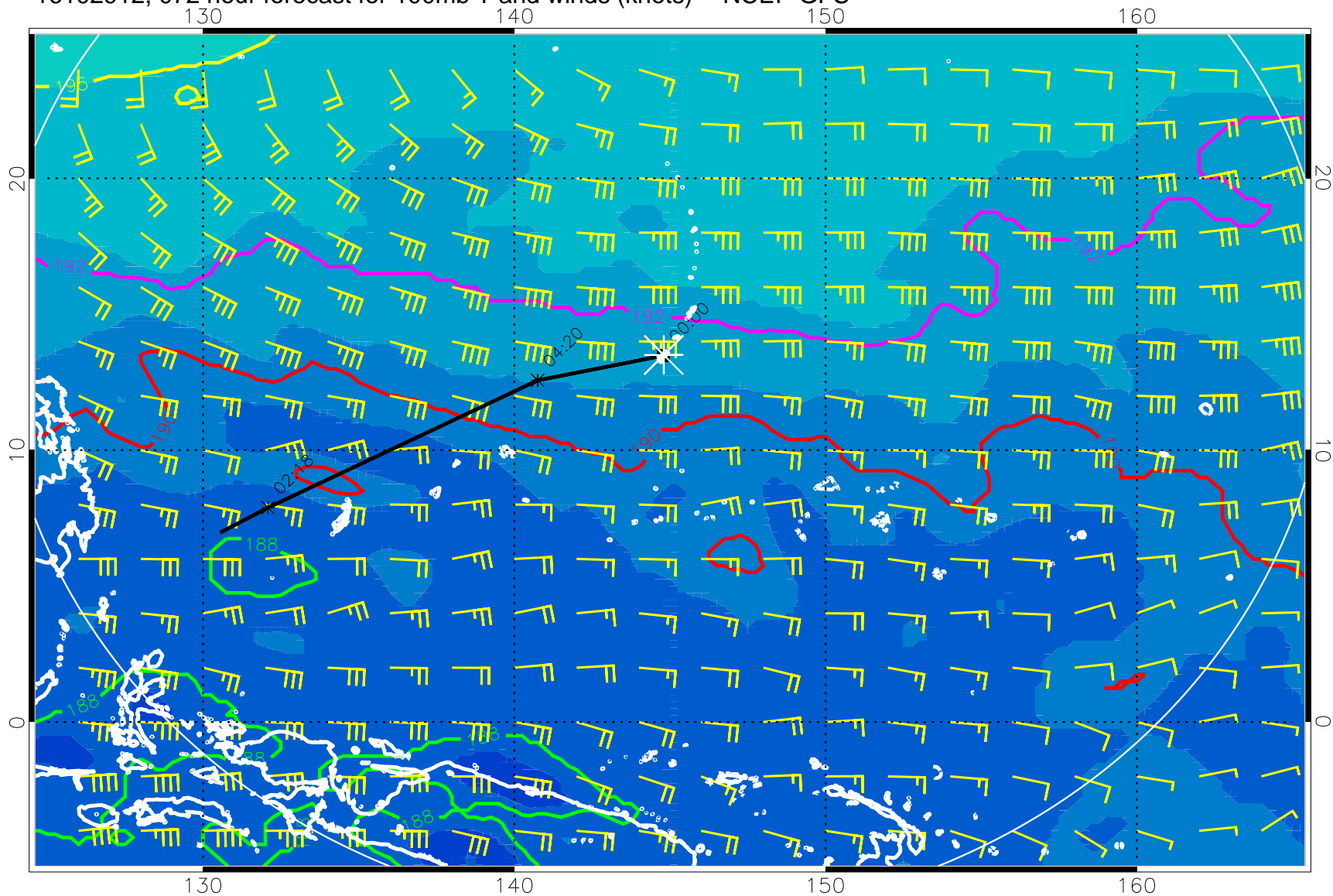
16102912, 072 hour forecast for 100mb T and winds (knots) -- NCEP GFS
