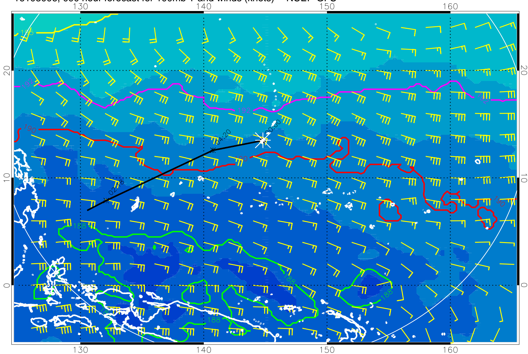
16103006, 090 hour forecast for 100mb T and winds (knots) -- NCEP GFS
