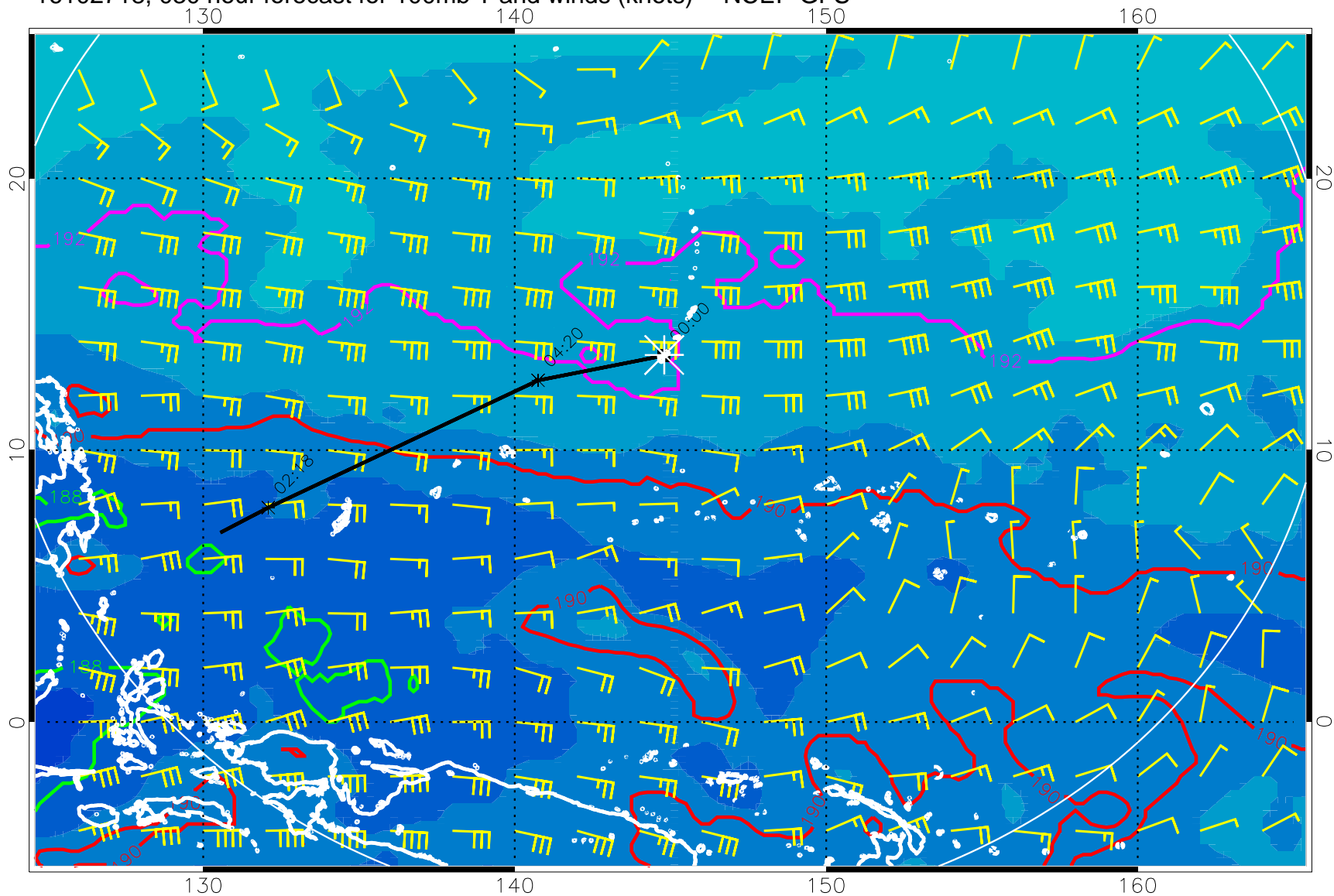
16102718, 030 hour forecast for 100mb T and winds (knots) -- NCEP GFS
