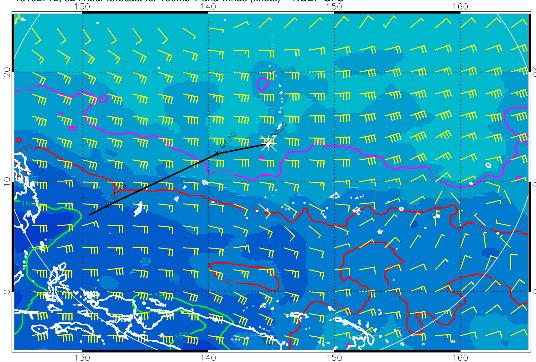
16102712, 024 hour forecast for 100mb T and winds (knots) -- NCEP GFS
