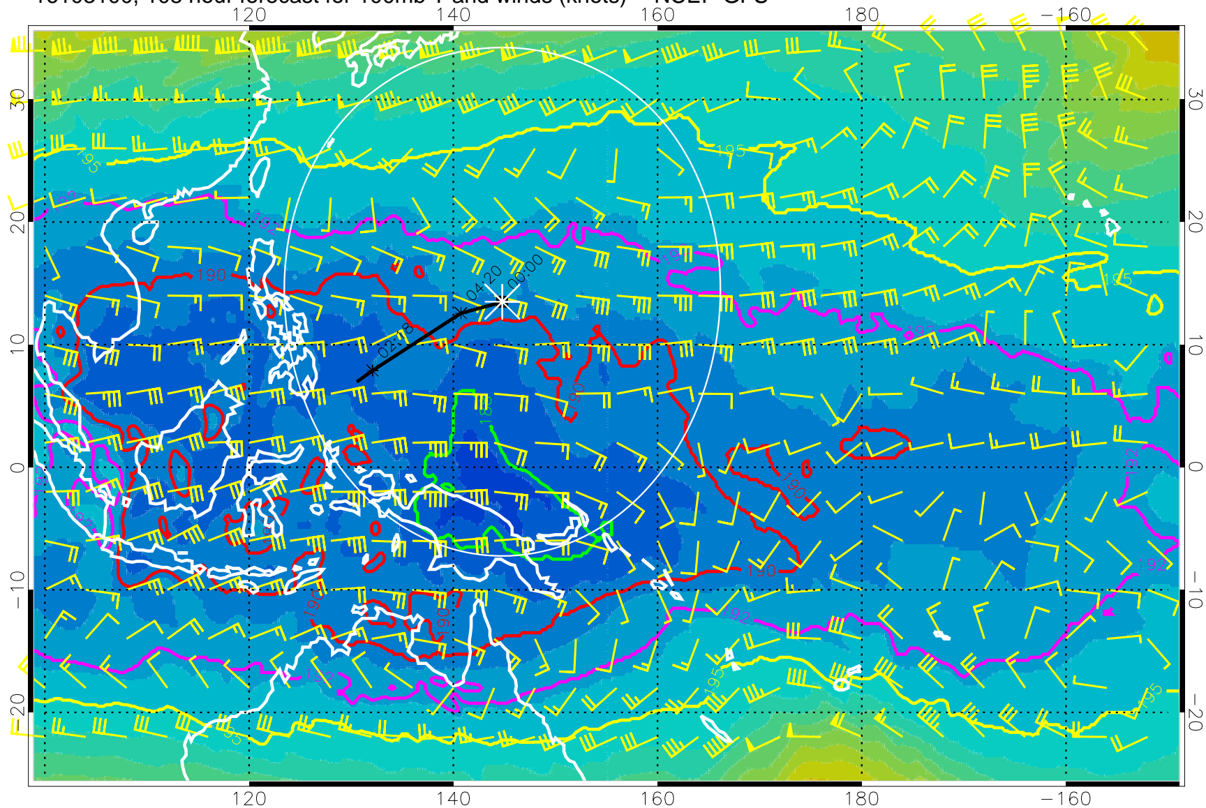
16103100, 108 hour forecast for 100mb T and winds (knots) -- NCEP GFS
