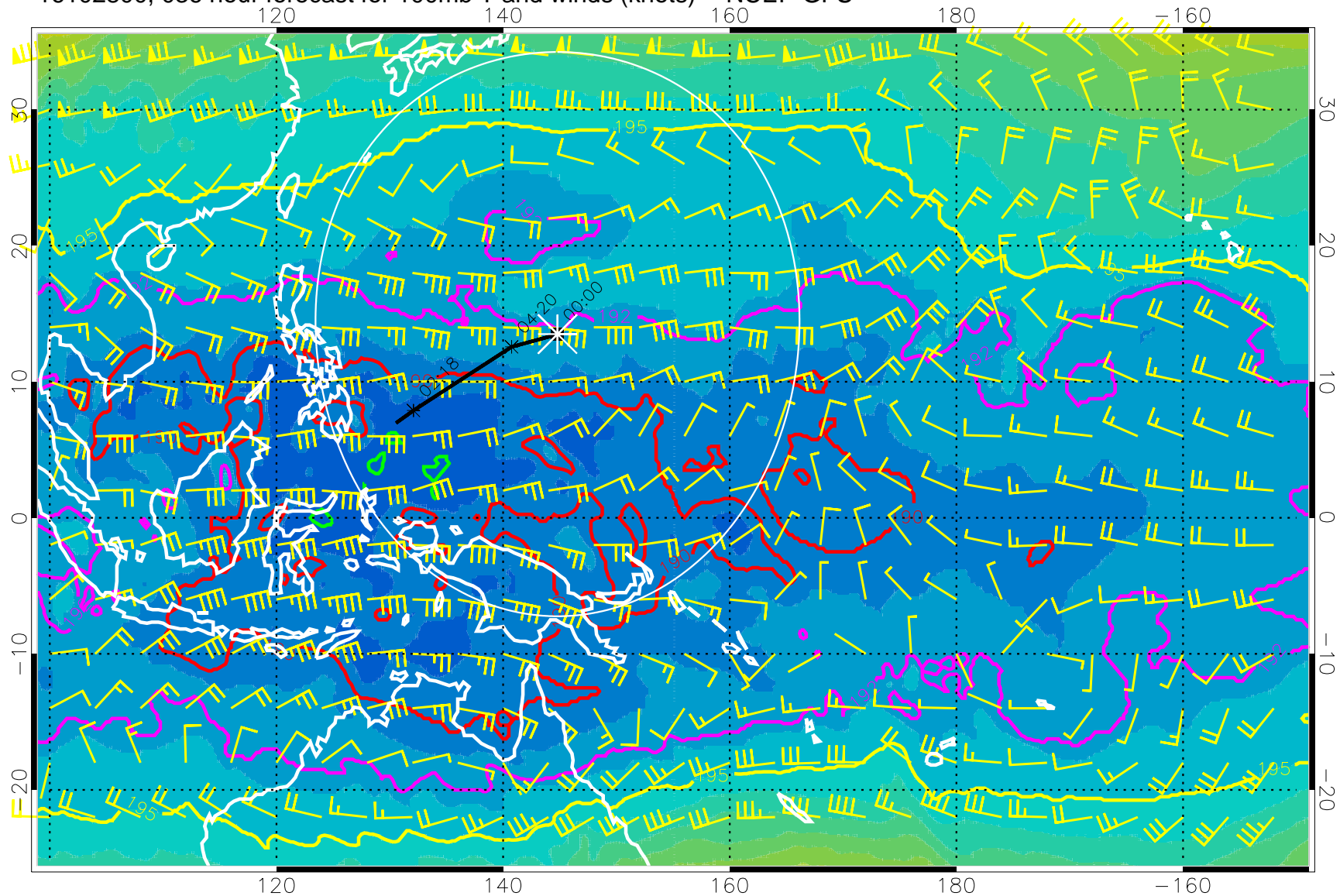
16102800, 036 hour forecast for 100mb T and winds (knots) -- NCEP GFS
