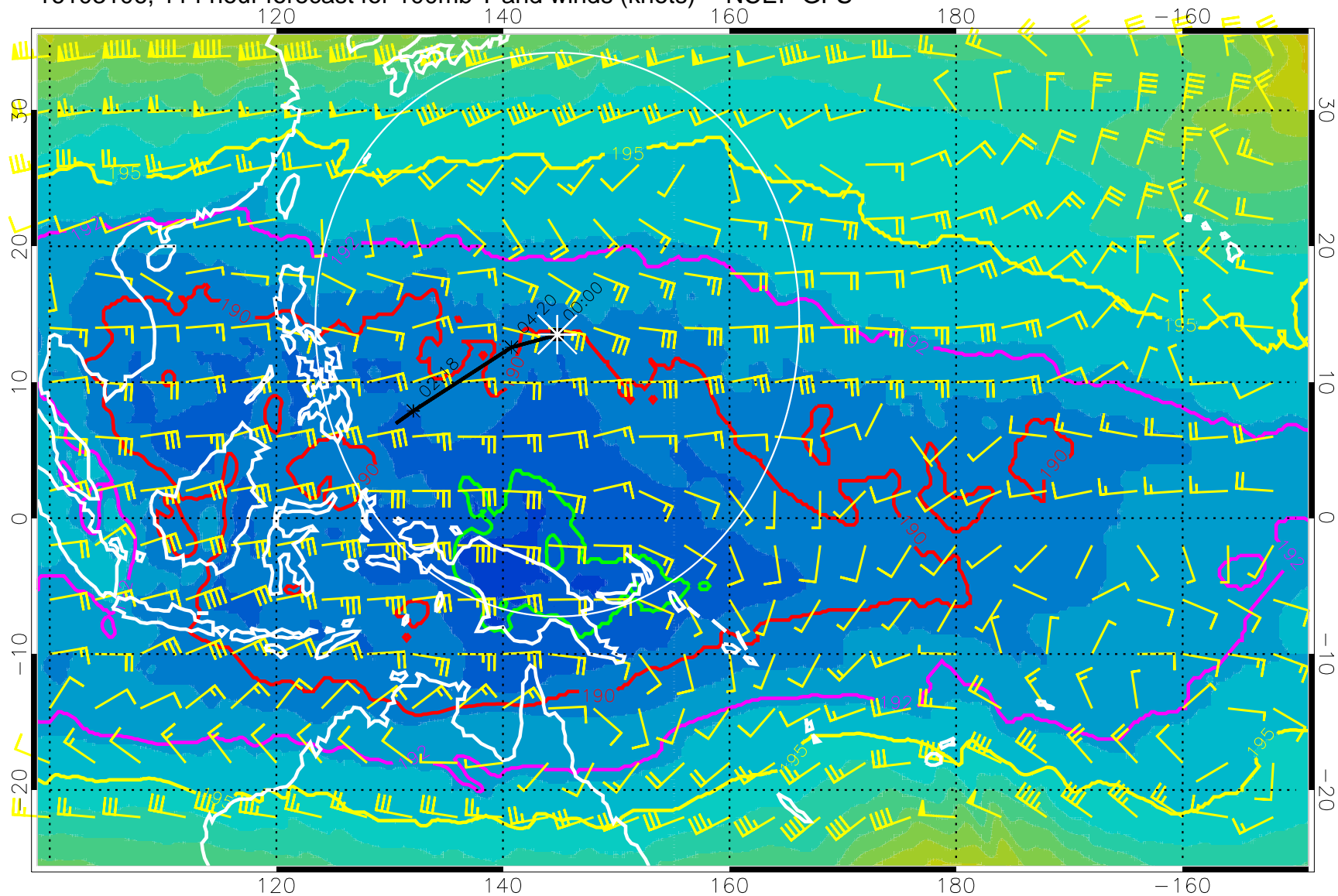
16103106, 114 hour forecast for 100mb T and winds (knots) -- NCEP GFS
