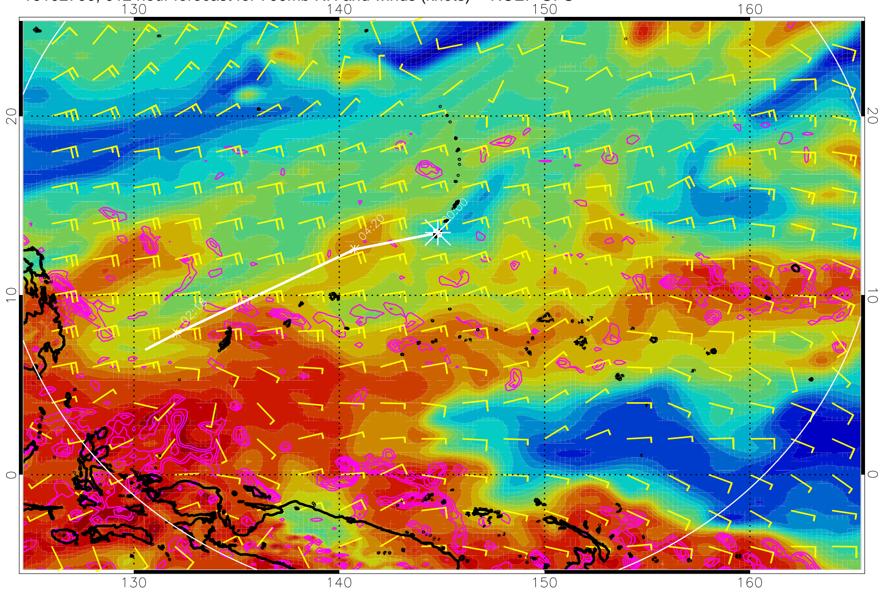
16102700, 012 hour forecast for 700mb RH and winds (knots) -- NCEP GFS
