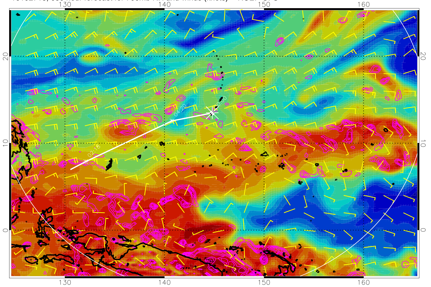
16102718, 030 hour forecast for 700mb RH and winds (knots) -- NCEP GFS
