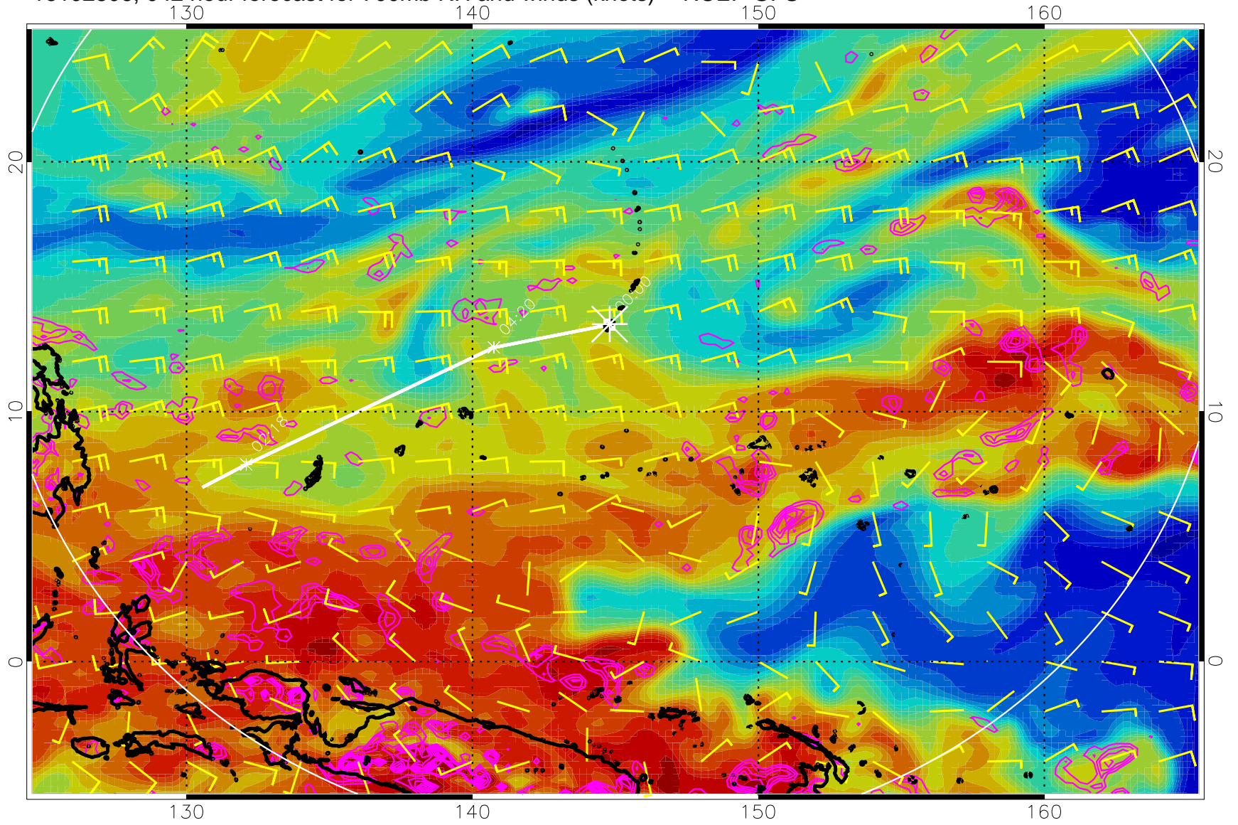
16102806, 042 hour forecast for 700mb RH and winds (knots) -- NCEP GFS
