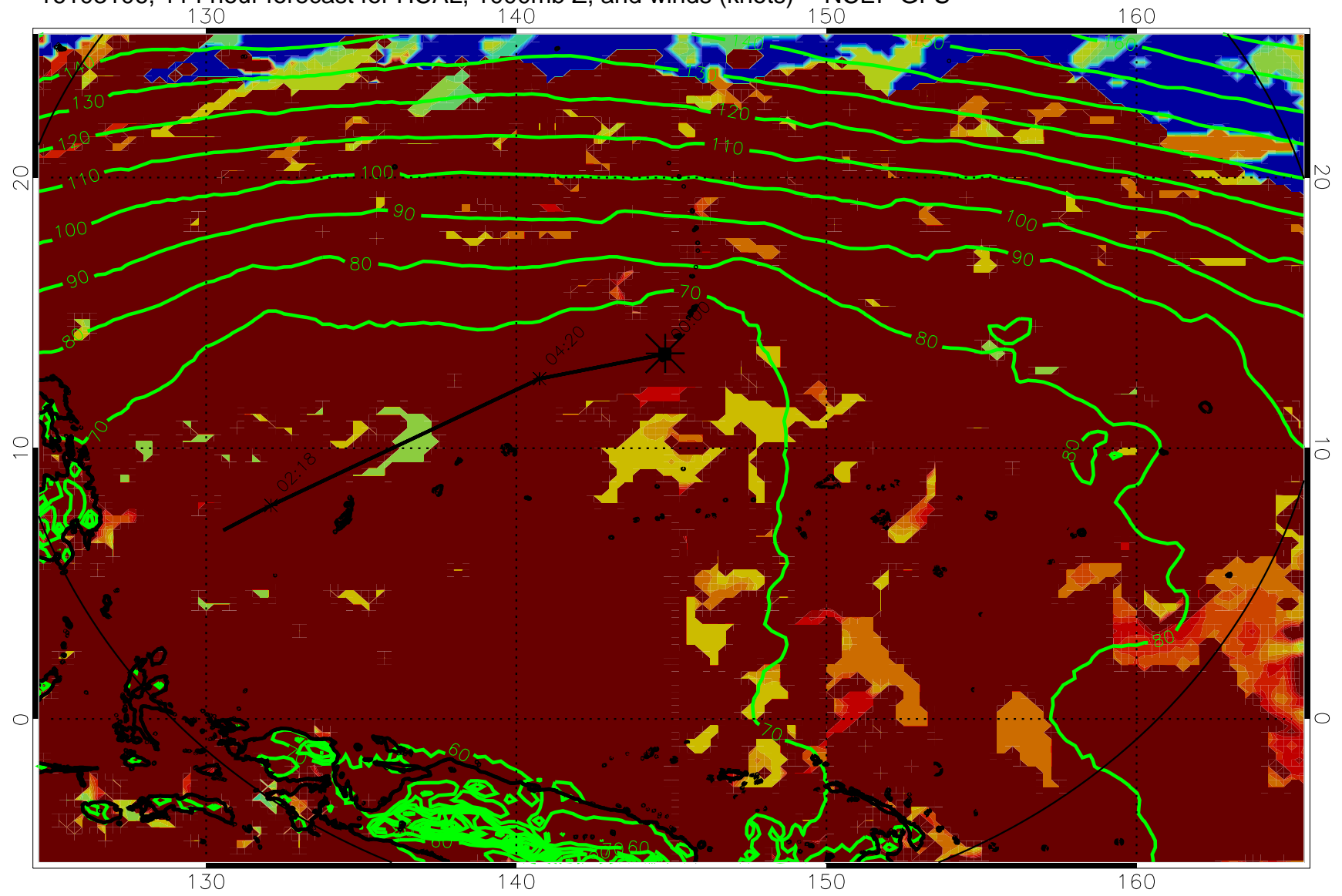
16103106, 114 hour forecast for HCAL, 1000mb Z, and winds (knots) -- NCEP GFS
