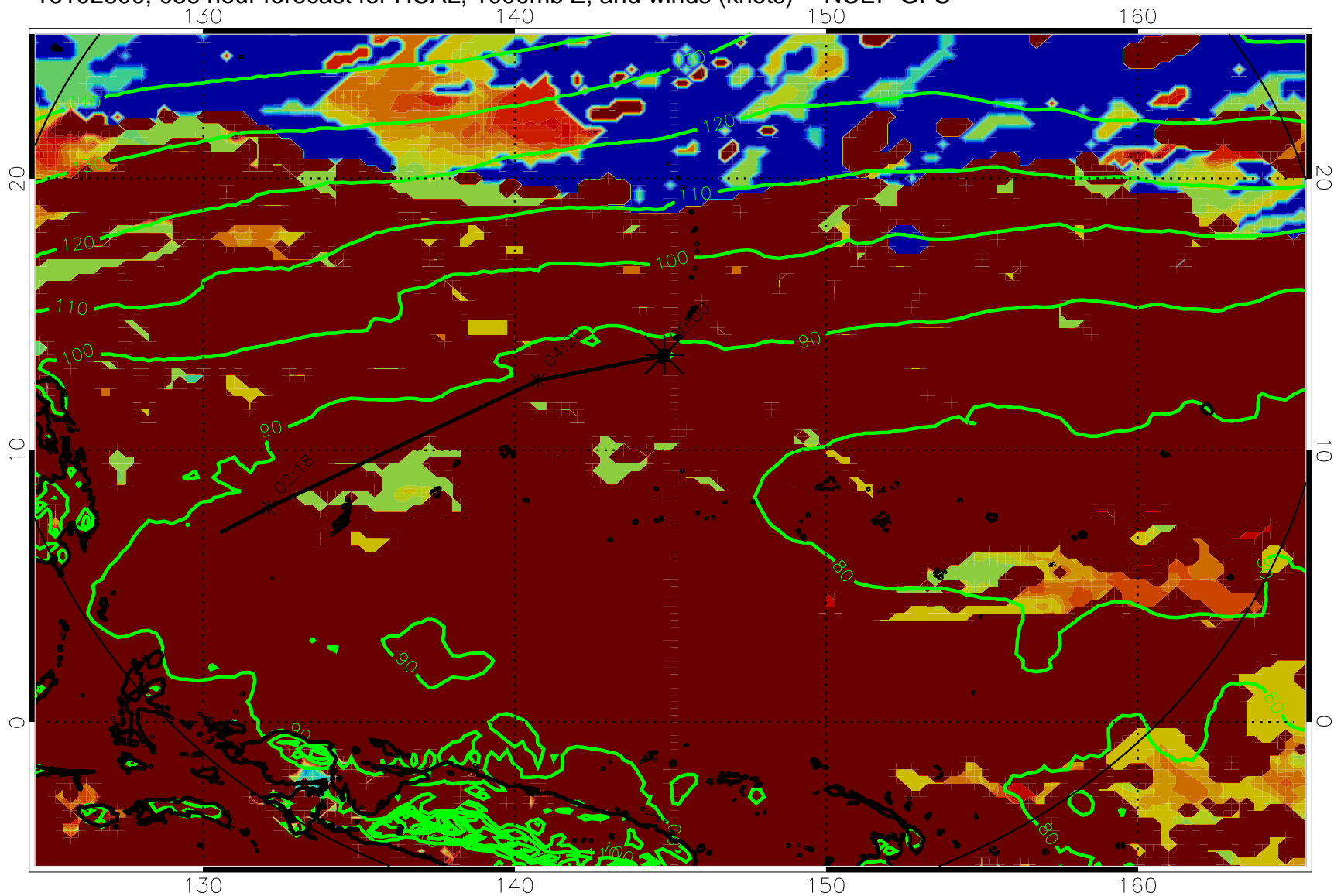
16102800, 036 hour forecast for HCAL, 1000mb Z, and winds (knots) -- NCEP GFS
