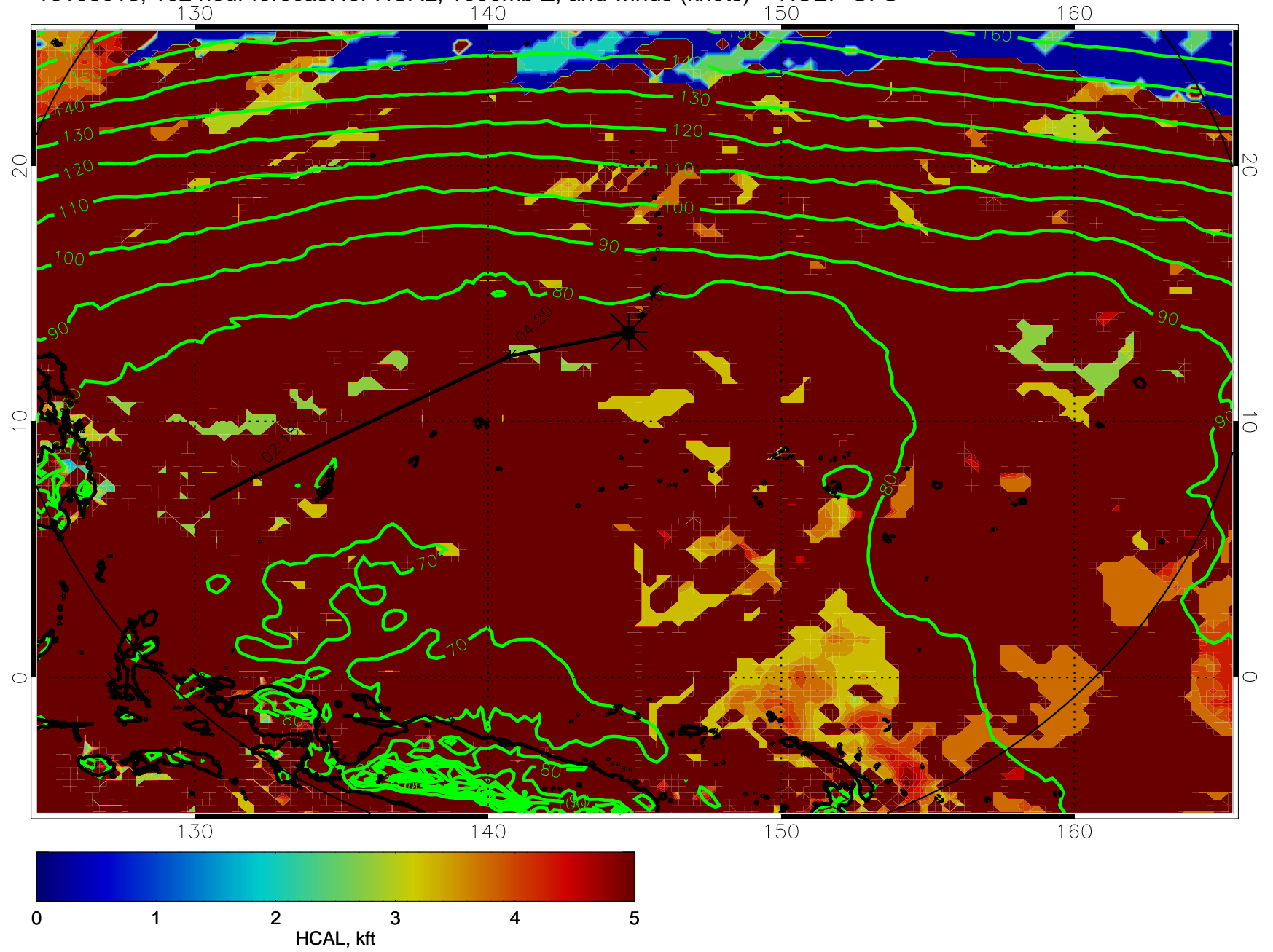
16103018, 102 hour forecast for HCAL, 1000mb Z, and winds (knots) -- NCEP GFS
