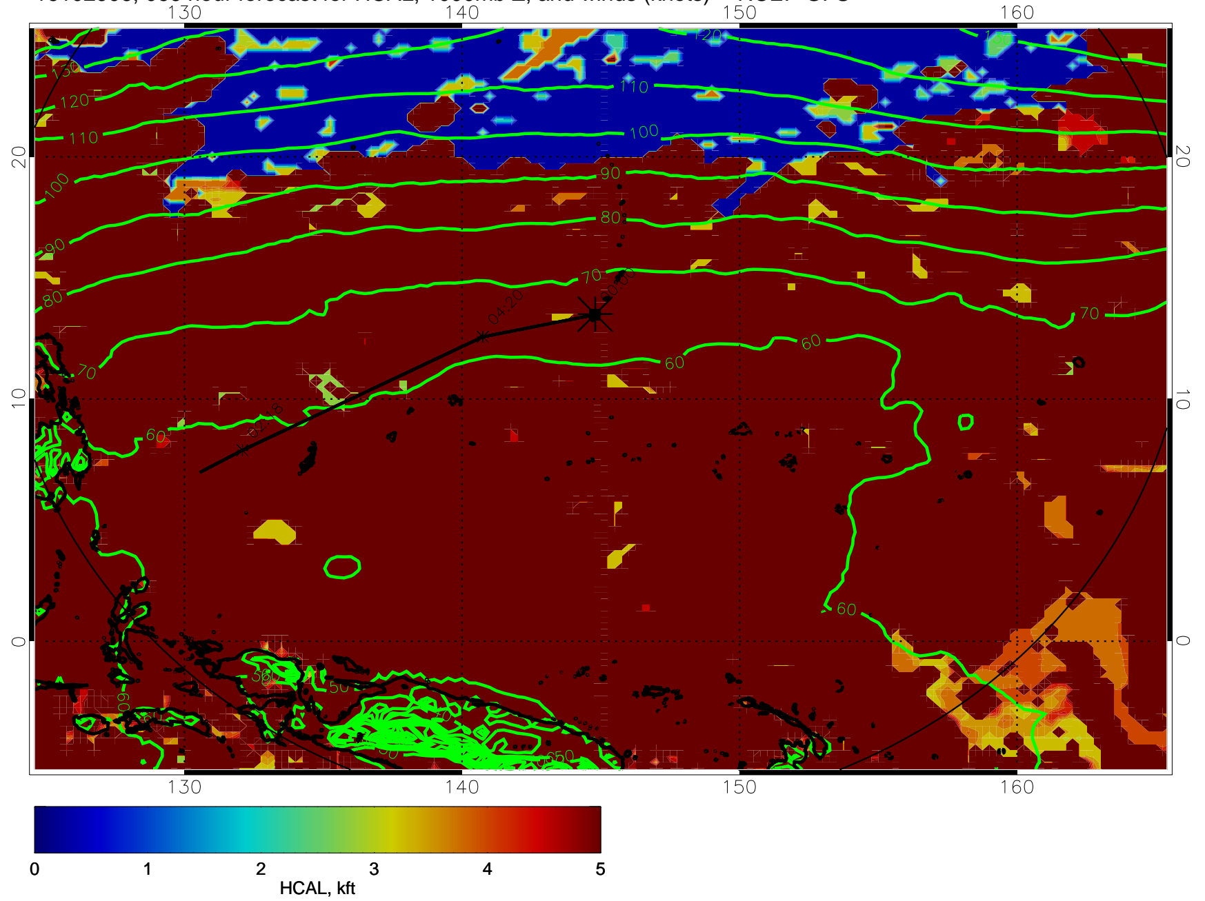
16102906, 066 hour forecast for HCAL, 1000mb Z, and winds (knots) -- NCEP GFS
