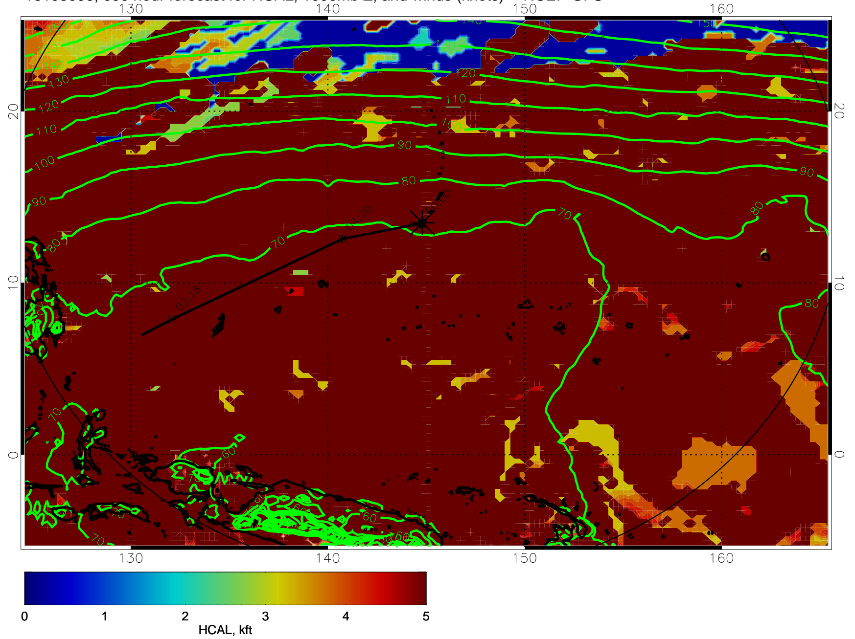
16103006, 090 hour forecast for HCAL, 1000mb Z, and winds (knots) -- NCEP GFS
