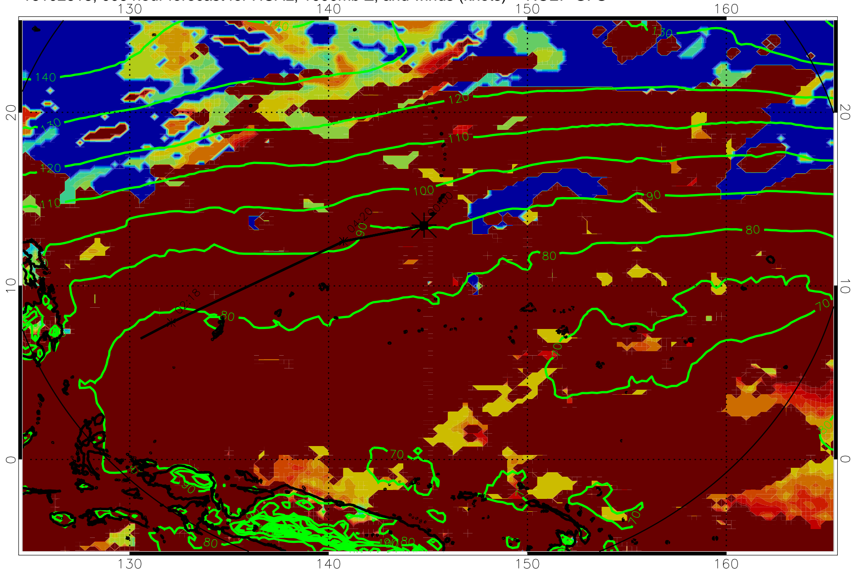
16102618, 006 hour forecast for HCAL, 1000mb Z, and winds (knots) -- NCEP GFS
