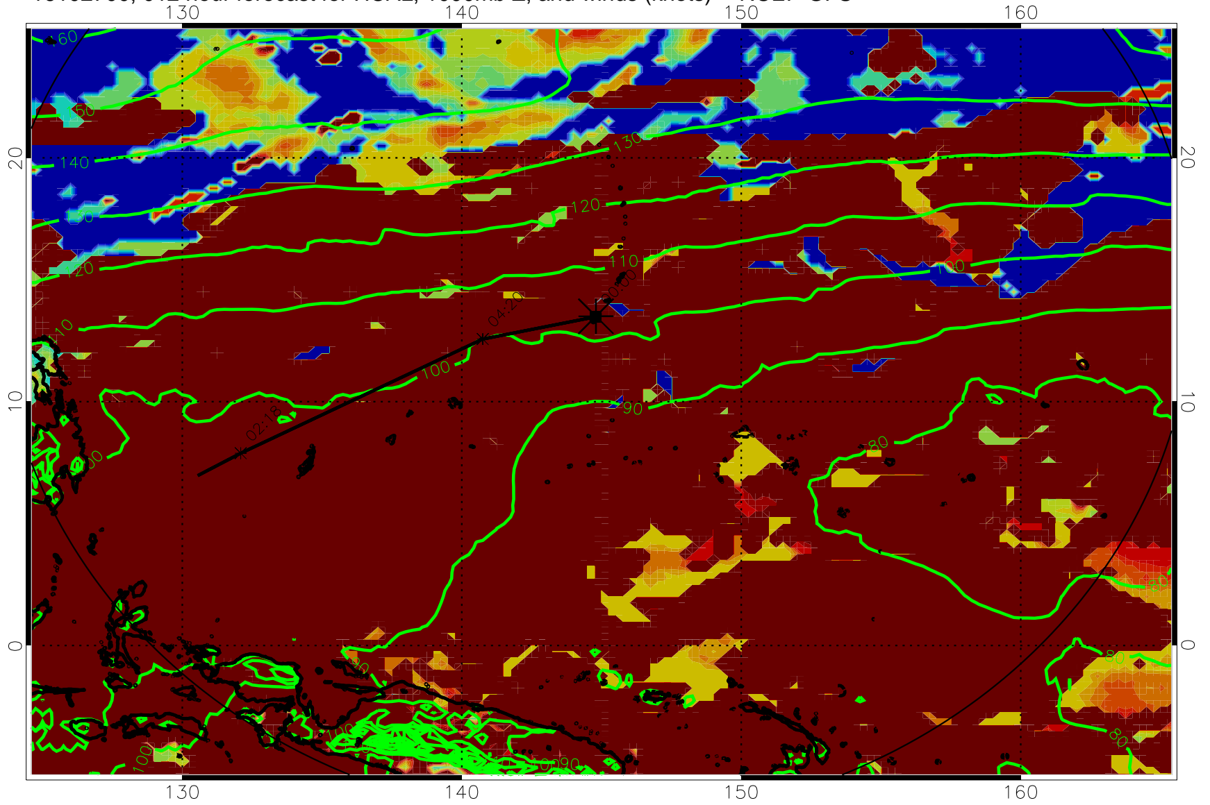
16102700, 012 hour forecast for HCAL, 1000mb Z, and winds (knots) -- NCEP GFS
