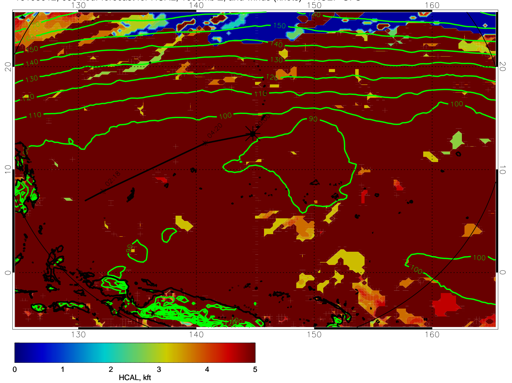
16103012, 096 hour forecast for HCAL, 1000mb Z, and winds (knots) -- NCEP GFS
