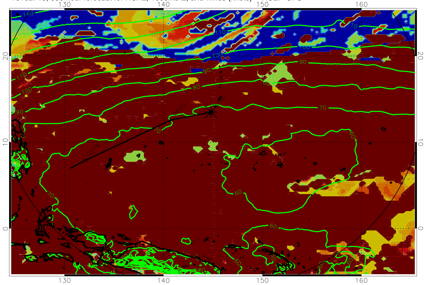
16102718, 030 hour forecast for HCAL, 1000mb Z, and winds (knots) -- NCEP GFS
