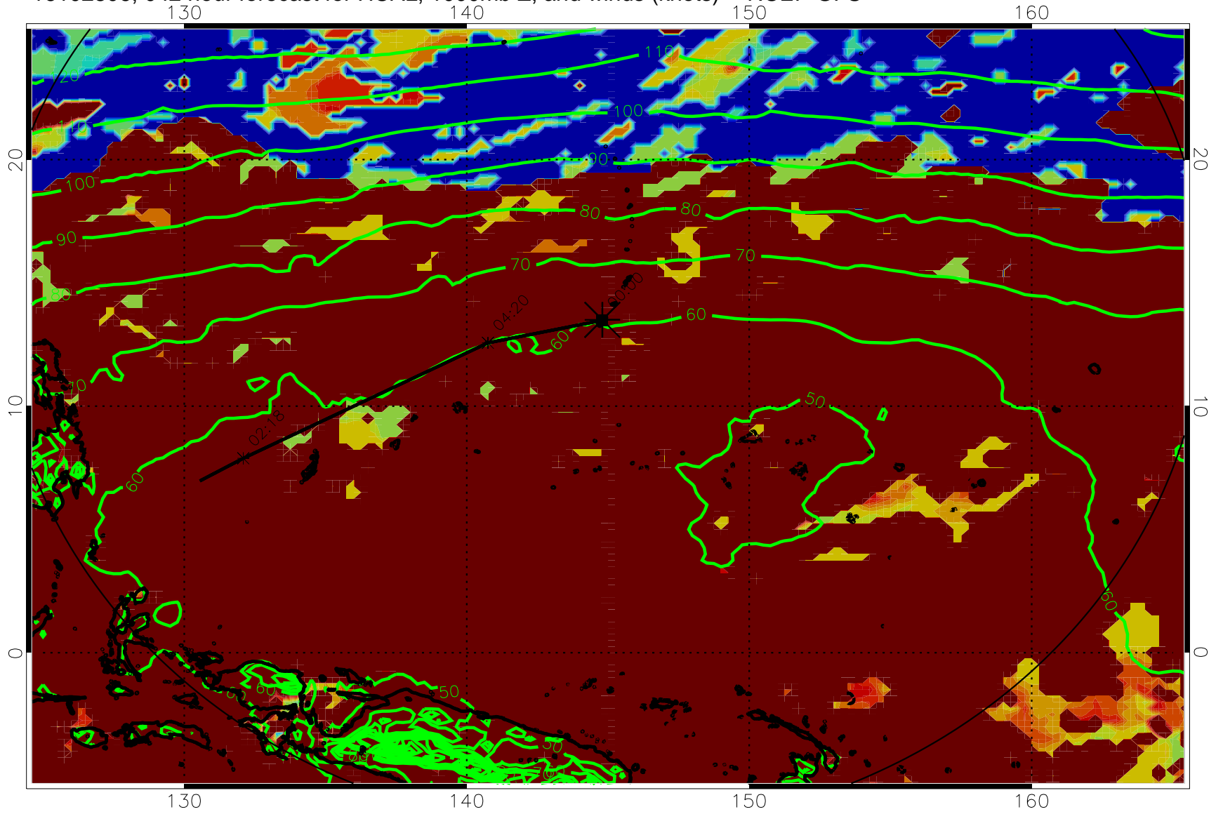
16102806, 042 hour forecast for HCAL, 1000mb Z, and winds (knots) -- NCEP GFS
