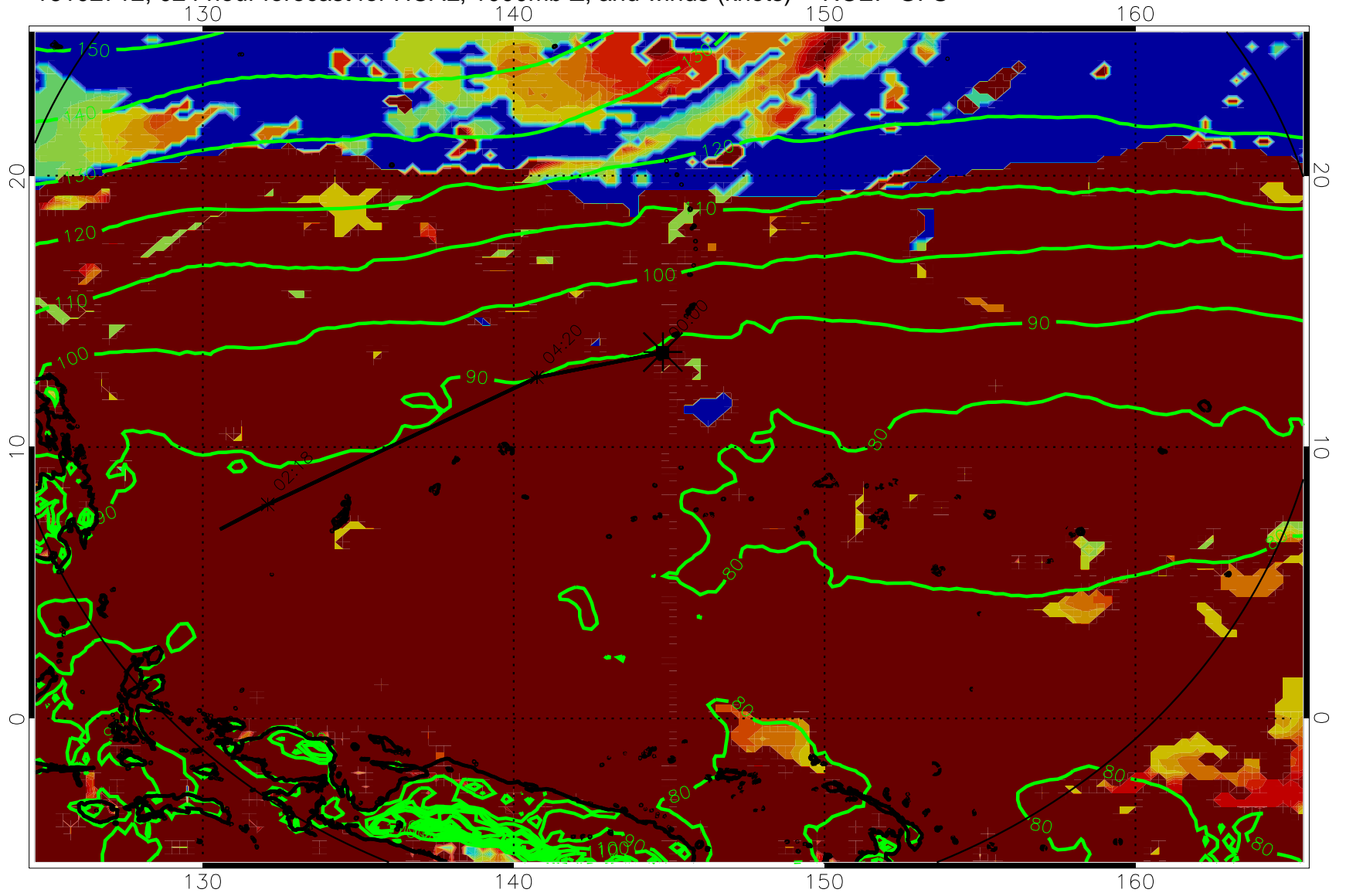
16102712, 024 hour forecast for HCAL, 1000mb Z, and winds (knots) -- NCEP GFS
