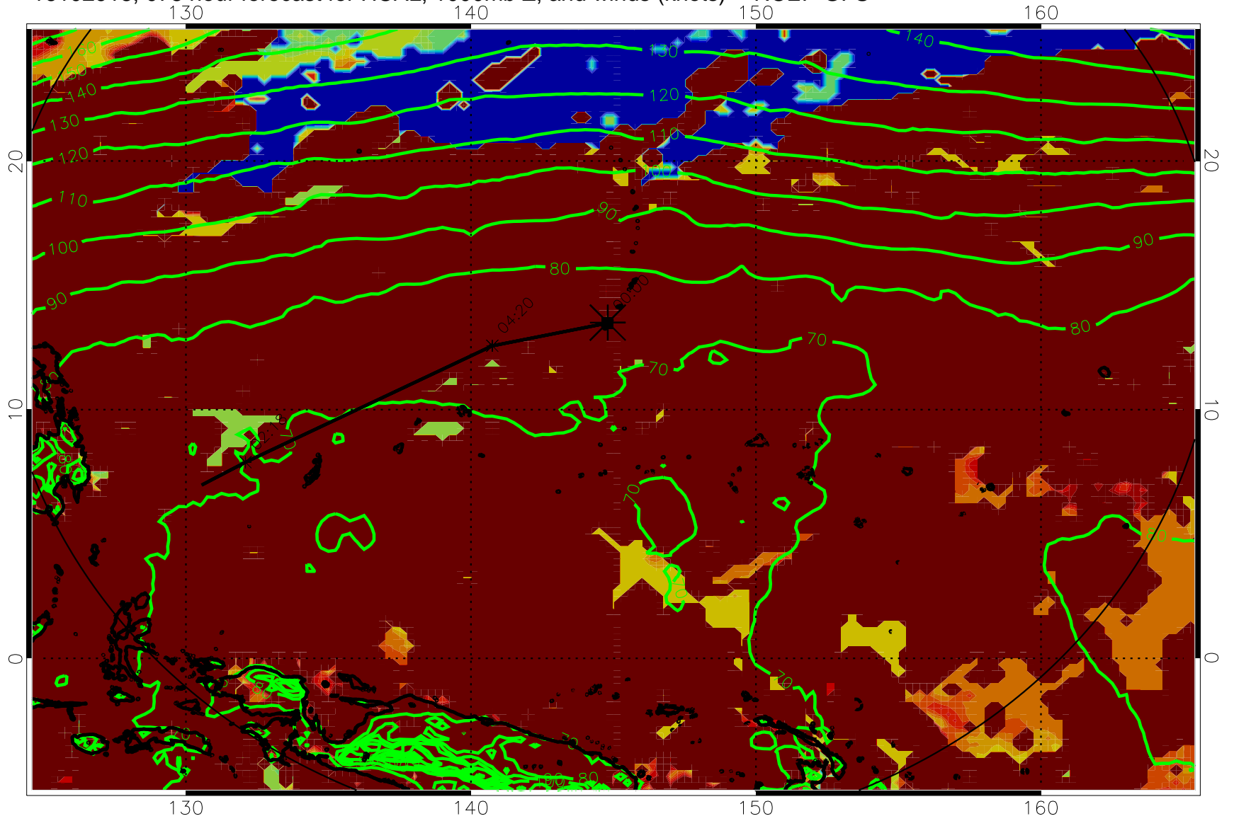
16102918, 078 hour forecast for HCAL, 1000mb Z, and winds (knots) -- NCEP GFS
