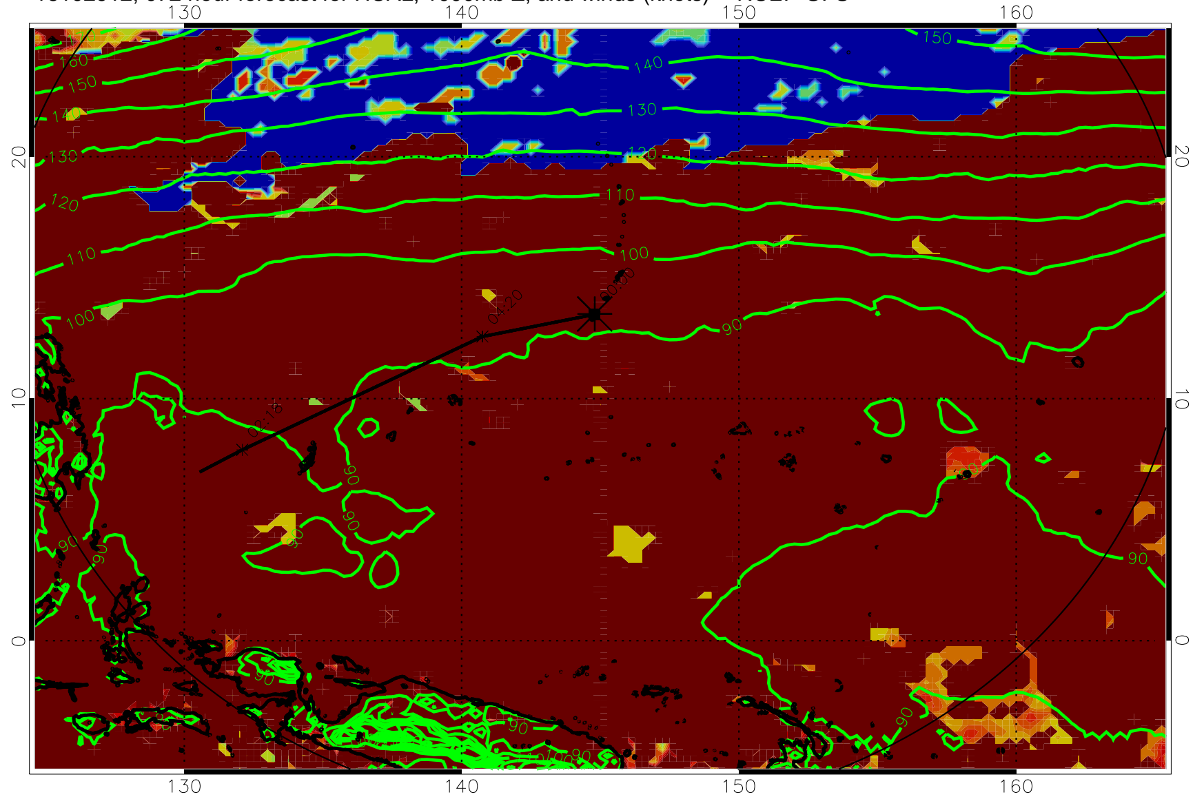
16102912, 072 hour forecast for HCAL, 1000mb Z, and winds (knots) -- NCEP GFS
