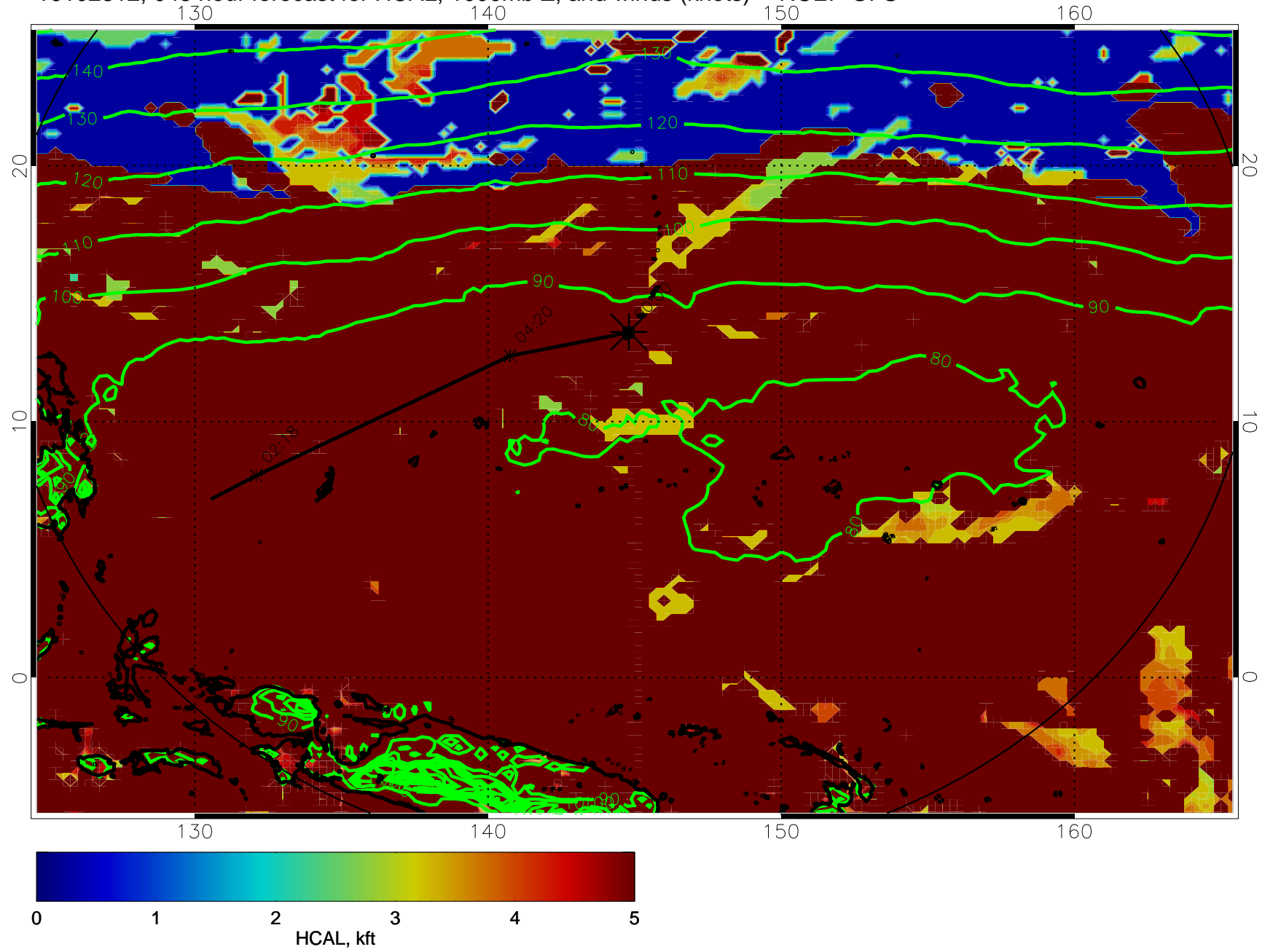
16102812, 048 hour forecast for HCAL, 1000mb Z, and winds (knots) -- NCEP GFS
