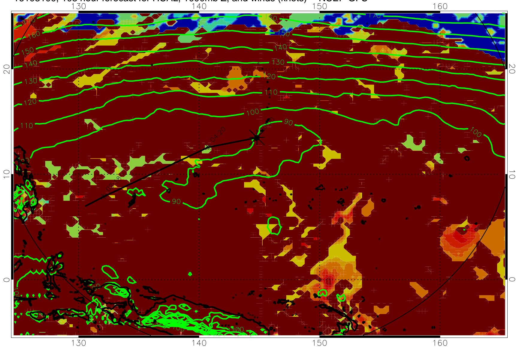
16103100, 108 hour forecast for HCAL, 1000mb Z, and winds (knots) -- NCEP GFS
