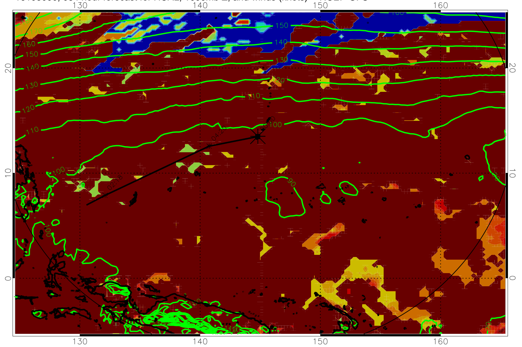
16103000, 084 hour forecast for HCAL, 1000mb Z, and winds (knots) -- NCEP GFS
