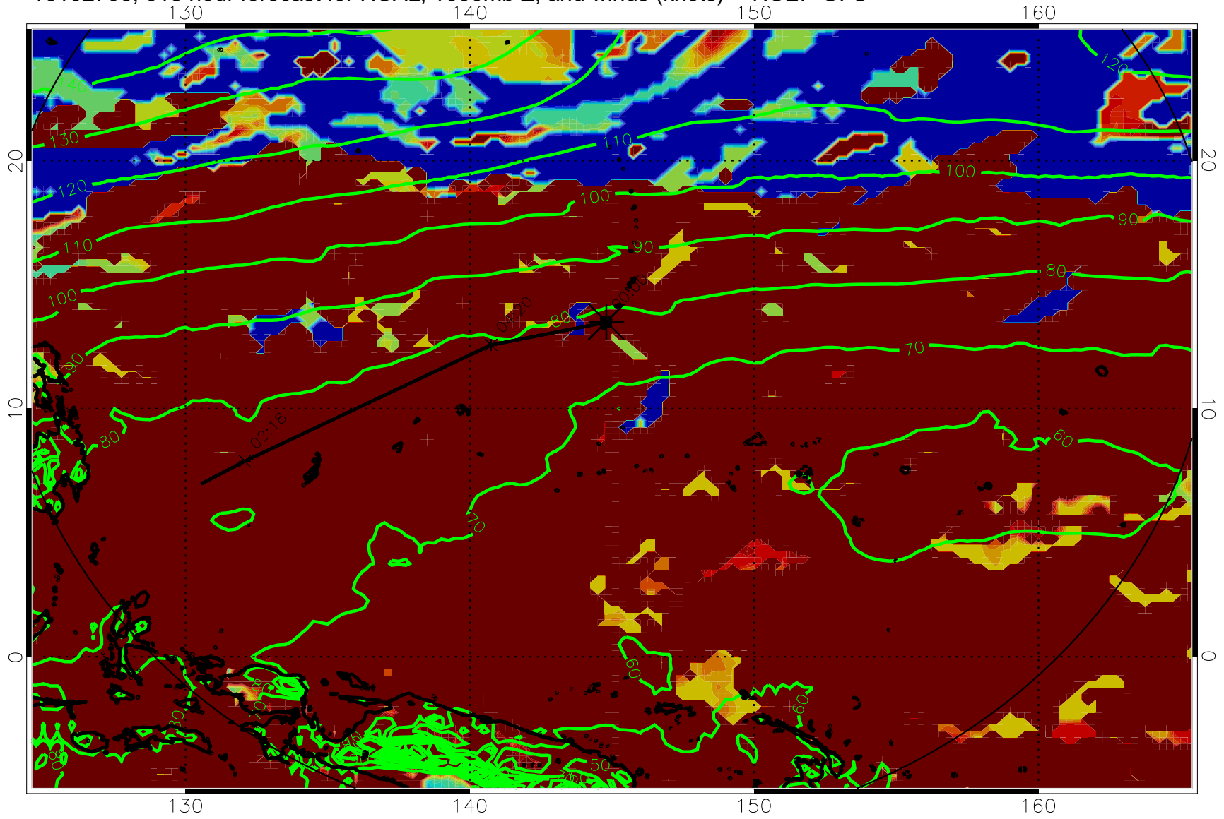
16102706, 018 hour forecast for HCAL, 1000mb Z, and winds (knots) -- NCEP GFS
