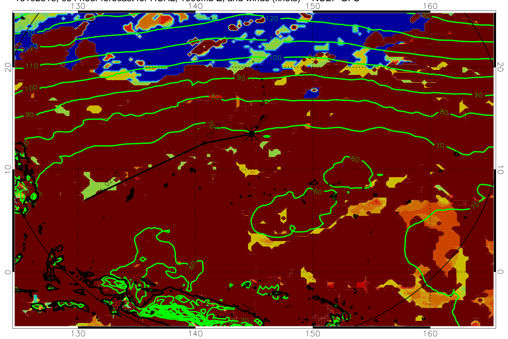
16102818, 054 hour forecast for HCAL, 1000mb Z, and winds (knots) -- NCEP GFS
