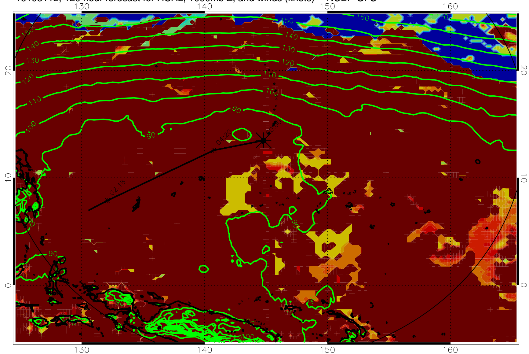
16103112, 120 hour forecast for HCAL, 1000mb Z, and winds (knots) -- NCEP GFS
