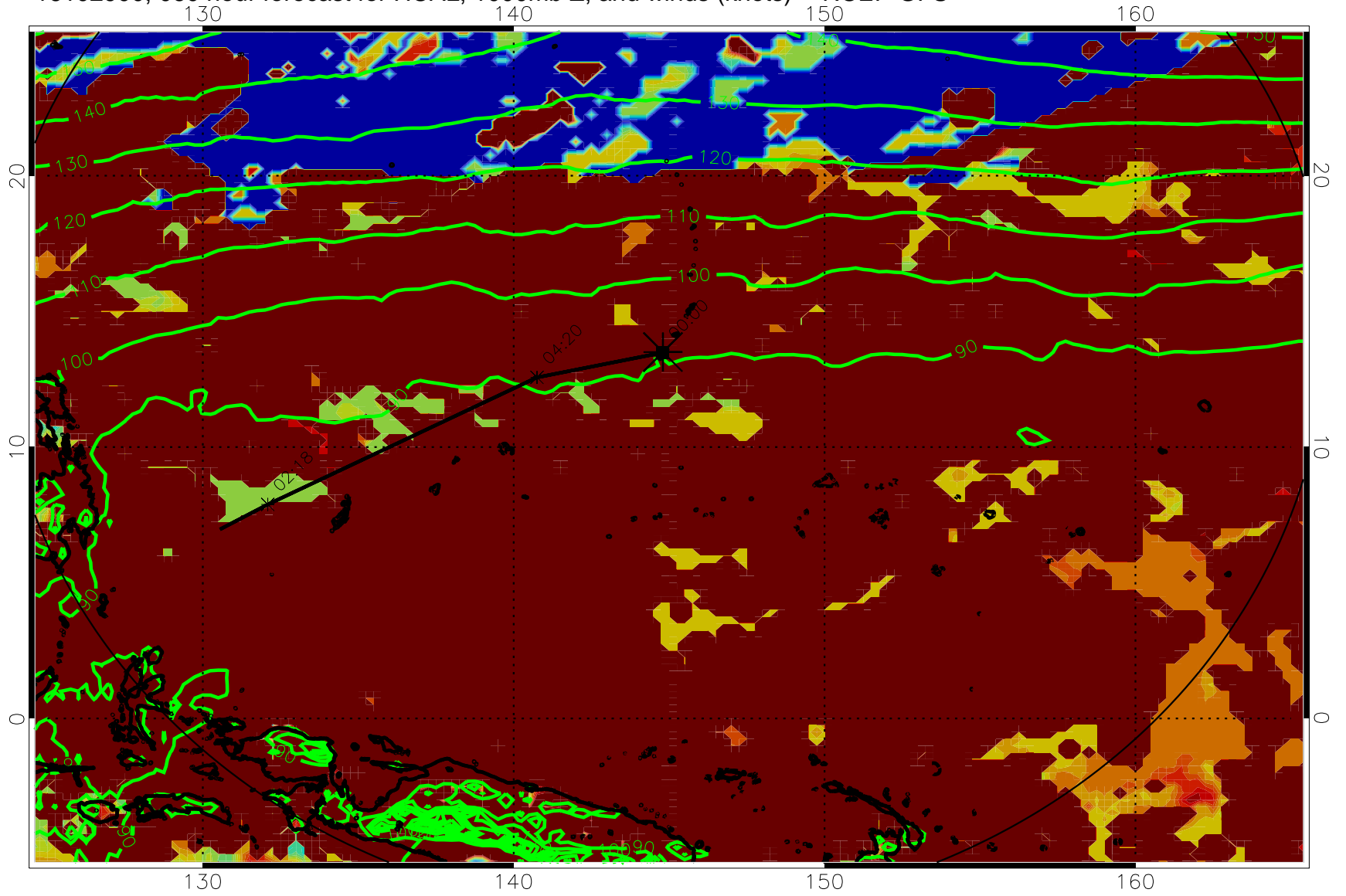
16102900, 060 hour forecast for HCAL, 1000mb Z, and winds (knots) -- NCEP GFS
