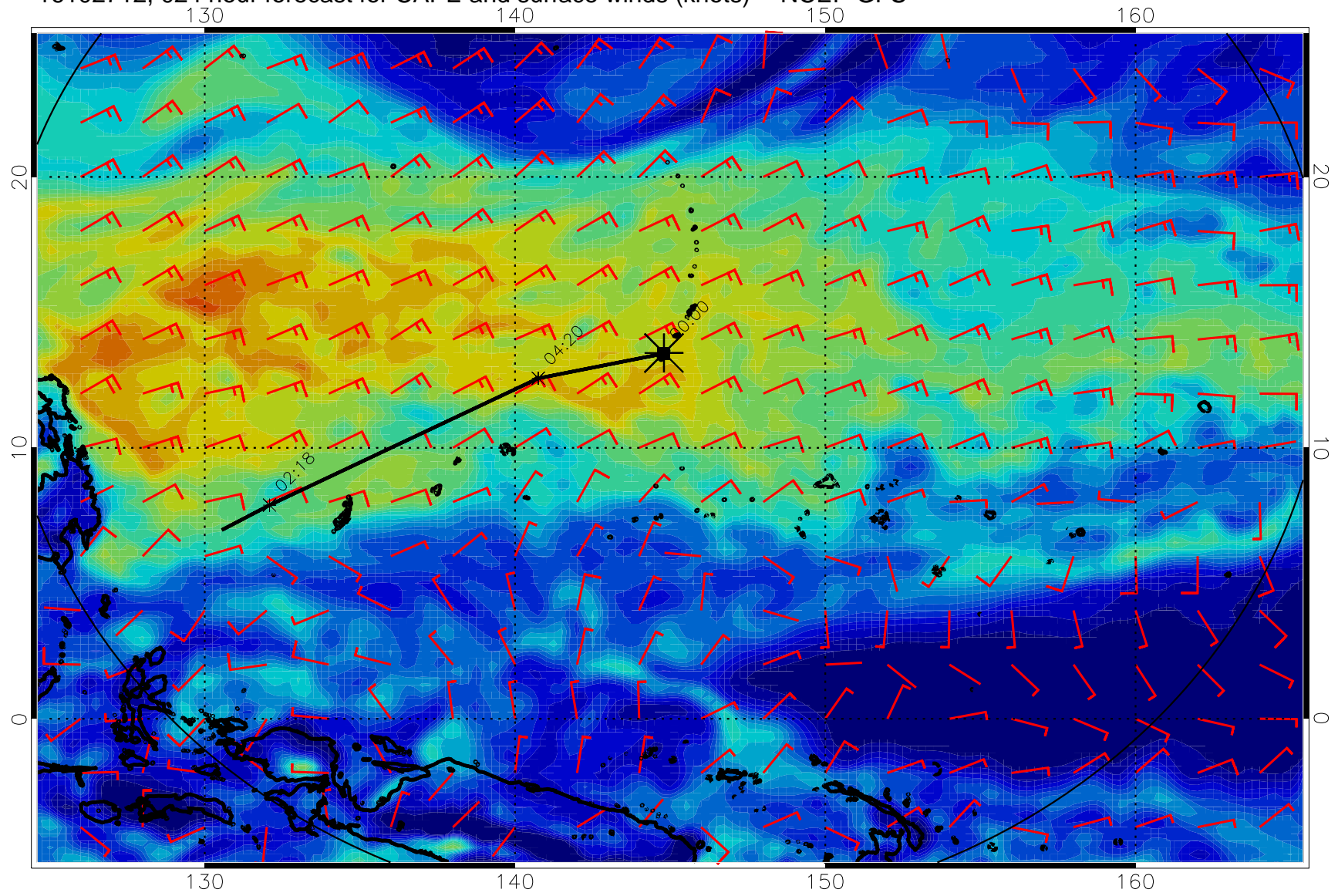
16102712, 024 hour forecast for CAPE and surface winds (knots) -- NCEP GFS
