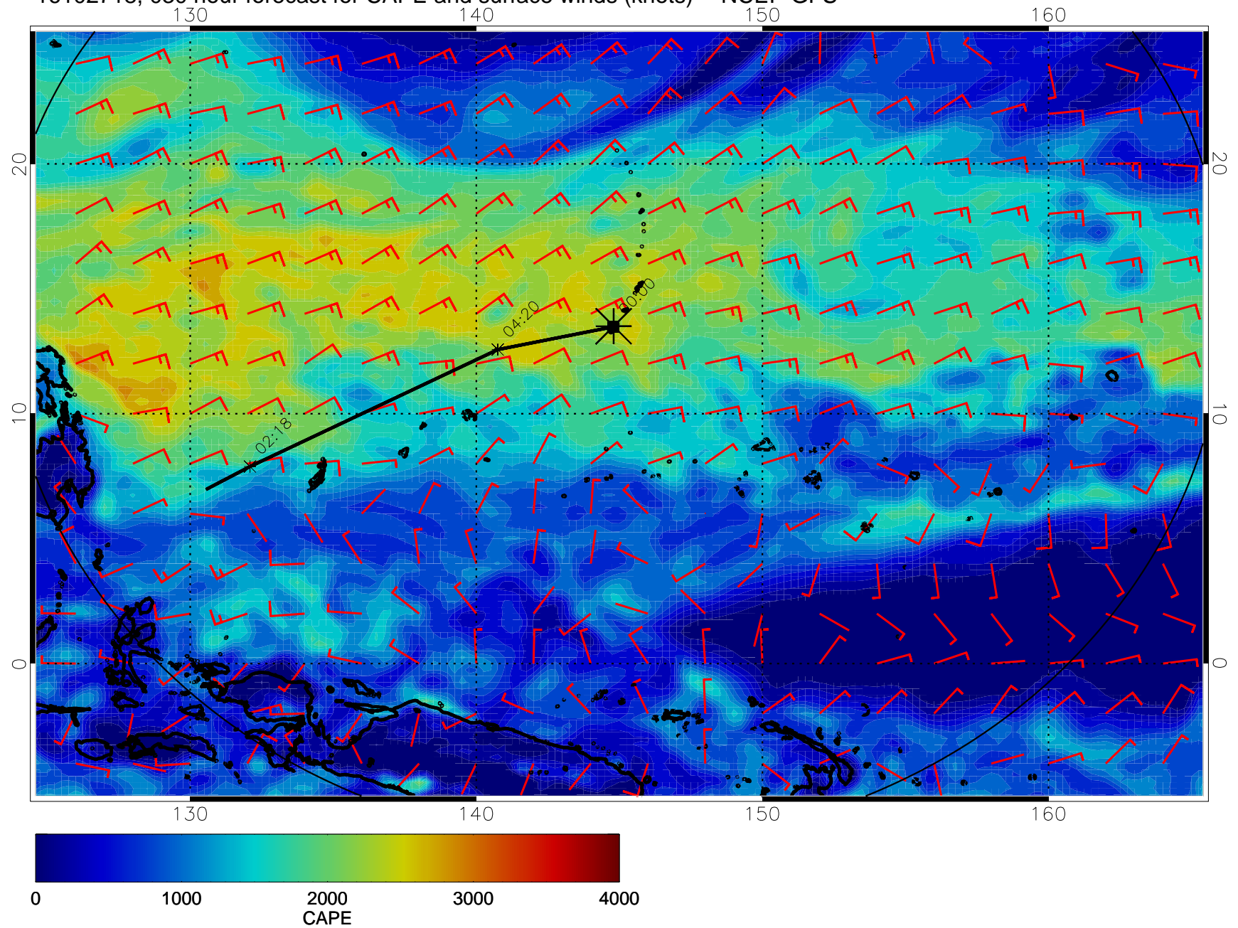
16102718, 030 hour forecast for CAPE and surface winds (knots) -- NCEP GFS
