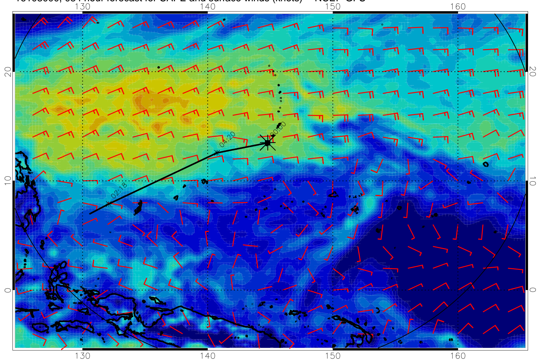
16103000, 084 hour forecast for CAPE and surface winds (knots) -- NCEP GFS
