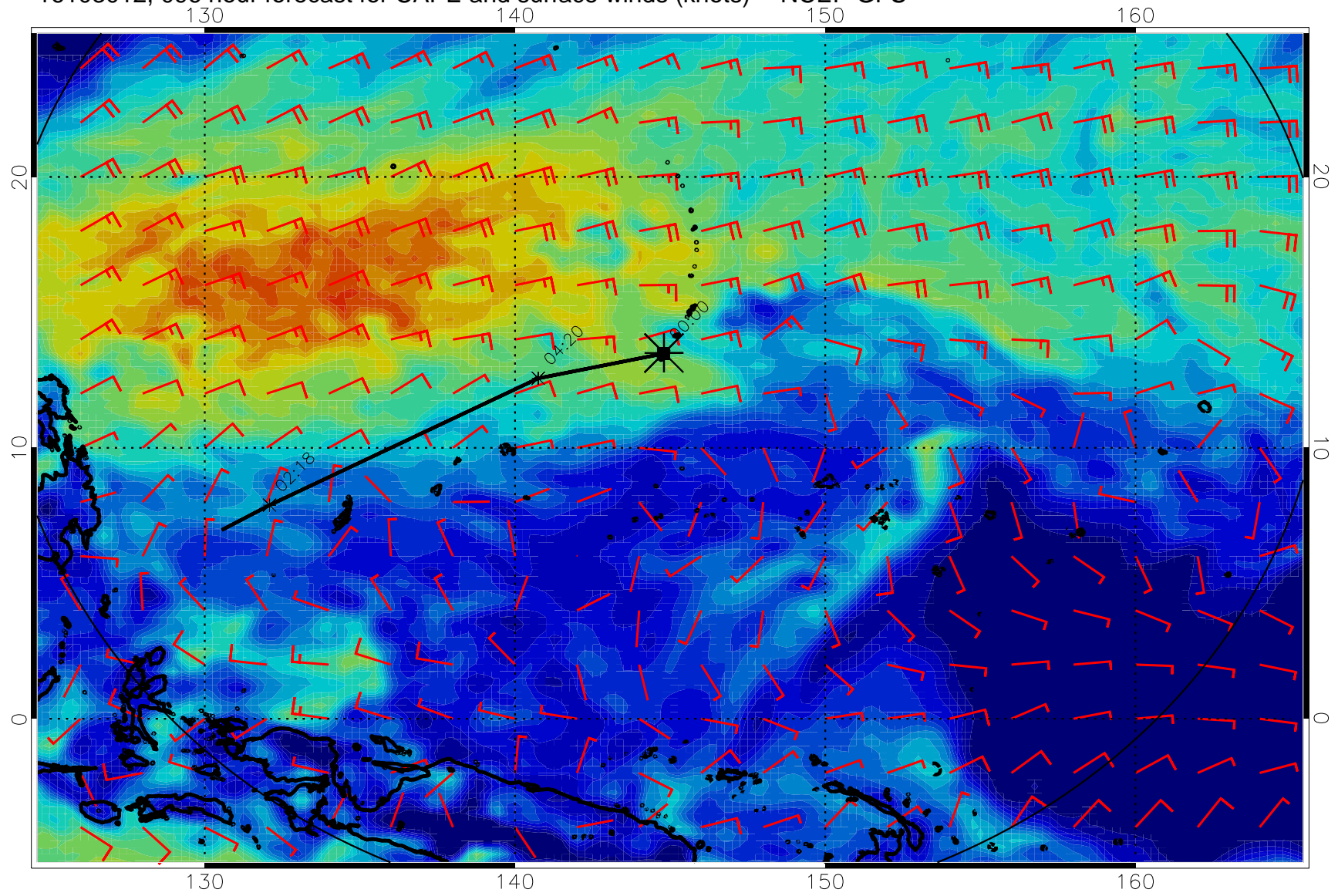
16103012, 096 hour forecast for CAPE and surface winds (knots) -- NCEP GFS
