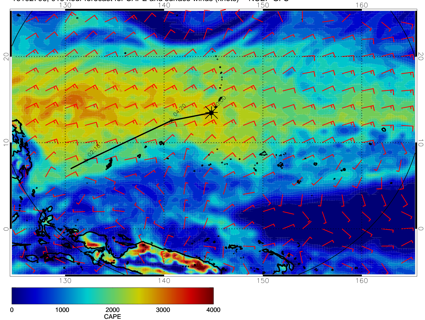
16102706, 018 hour forecast for CAPE and surface winds (knots) -- NCEP GFS
