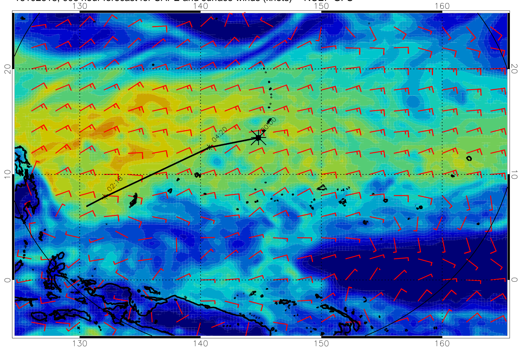
16102618, 006 hour forecast for CAPE and surface winds (knots) -- NCEP GFS
