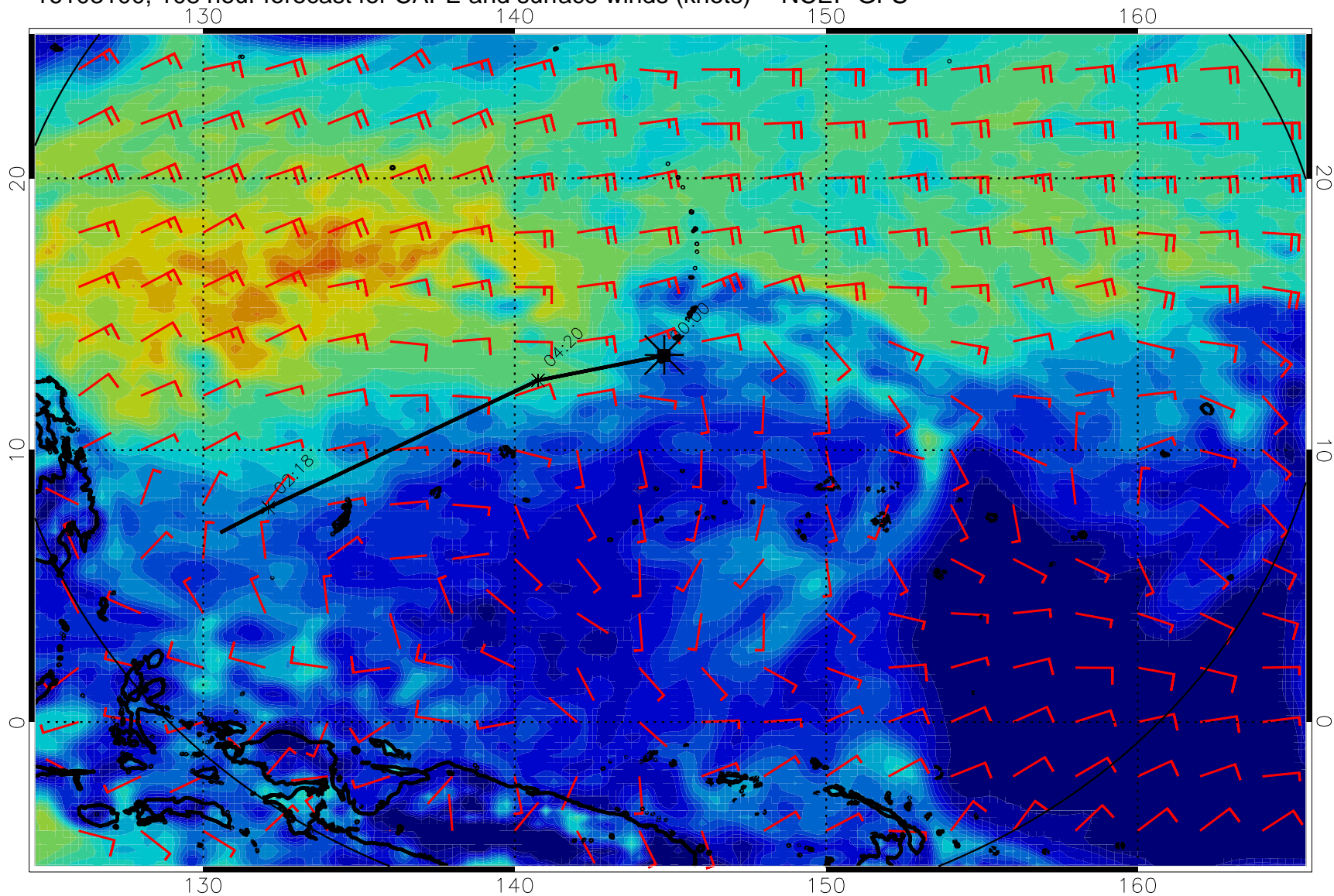
16103100, 108 hour forecast for CAPE and surface winds (knots) -- NCEP GFS
