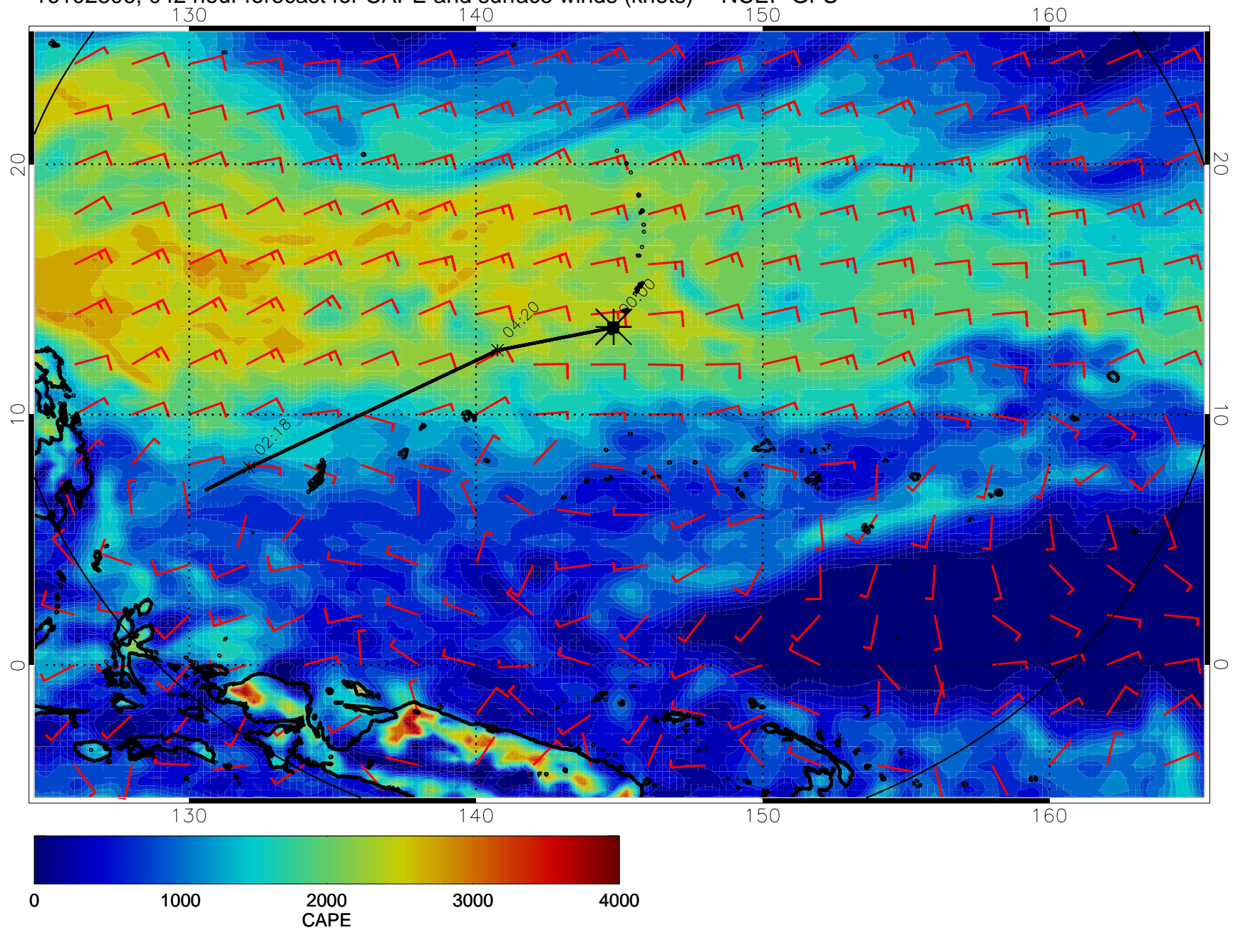
16102806, 042 hour forecast for CAPE and surface winds (knots) -- NCEP GFS
