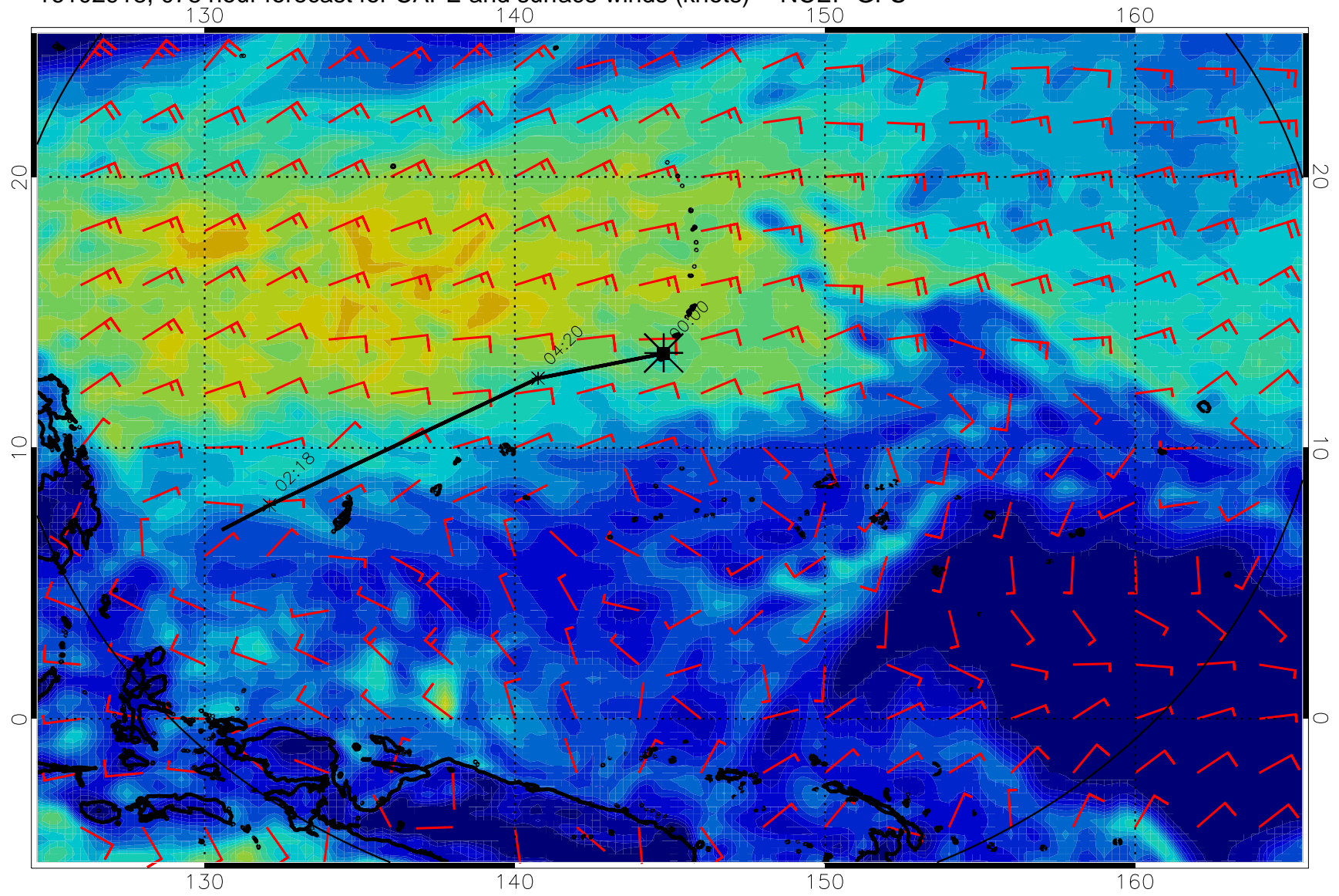
16102918, 078 hour forecast for CAPE and surface winds (knots) -- NCEP GFS
