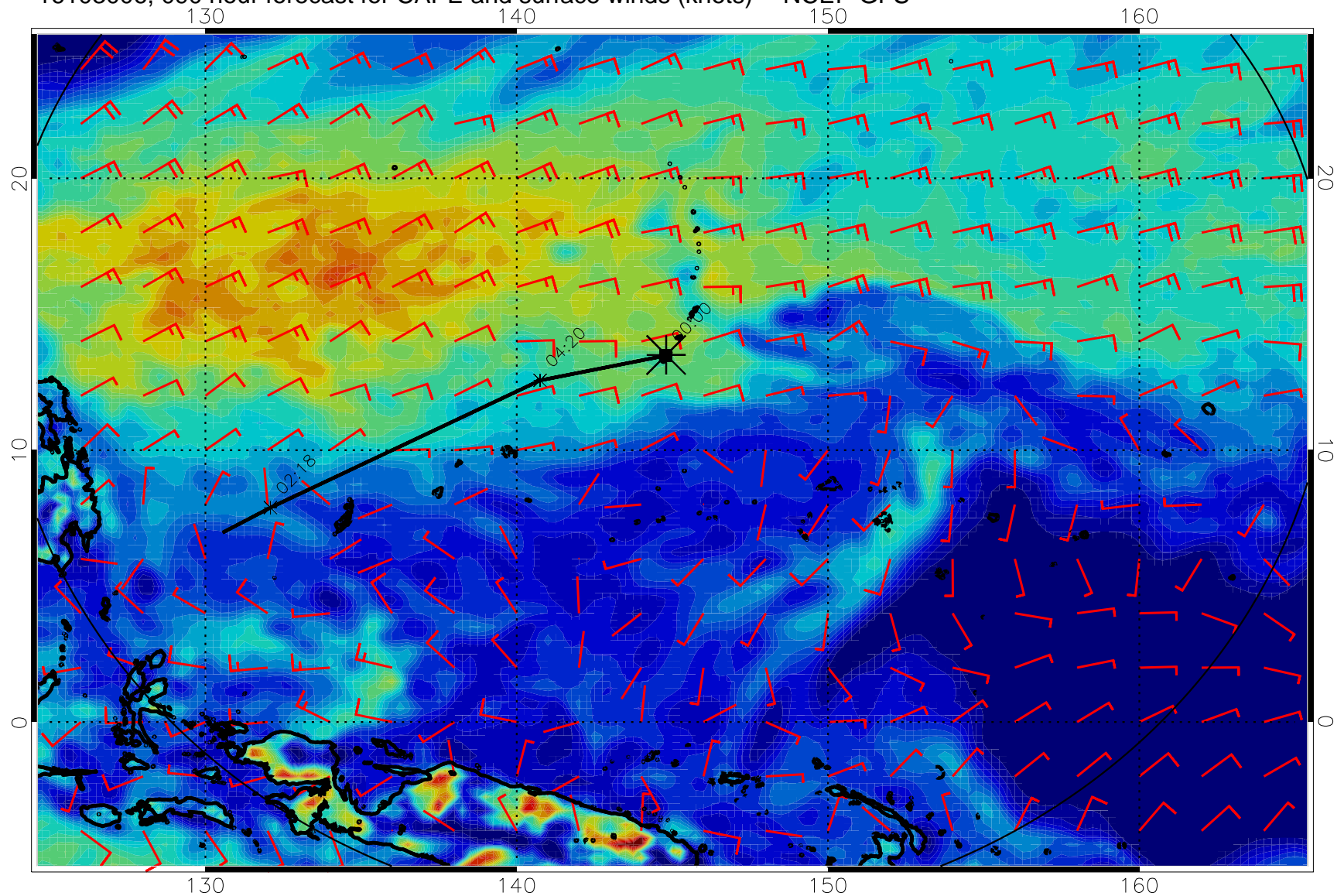
16103006, 090 hour forecast for CAPE and surface winds (knots) -- NCEP GFS
