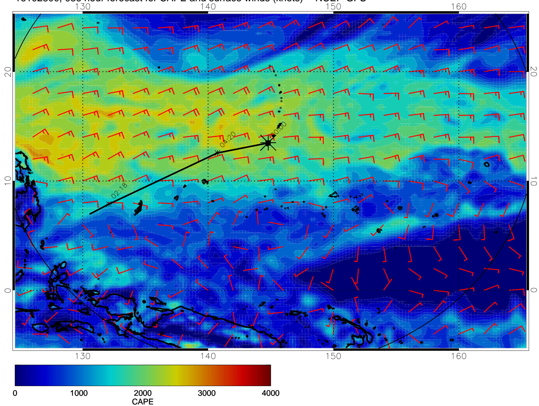
16102800, 036 hour forecast for CAPE and surface winds (knots) -- NCEP GFS
