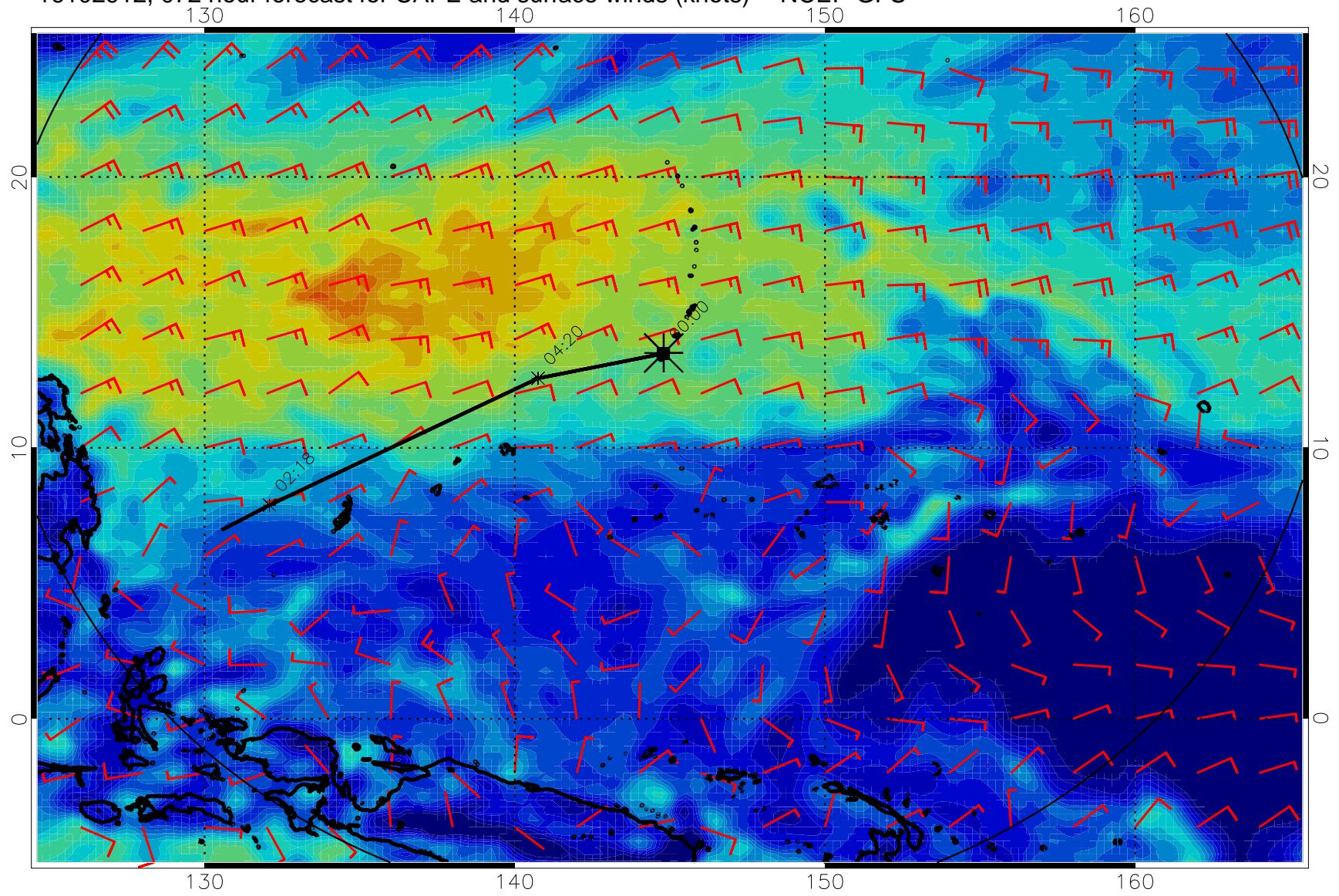
16102912, 072 hour forecast for CAPE and surface winds (knots) -- NCEP GFS
