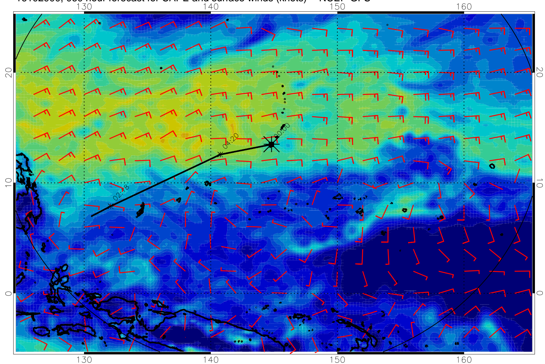
16102900, 060 hour forecast for CAPE and surface winds (knots) -- NCEP GFS
