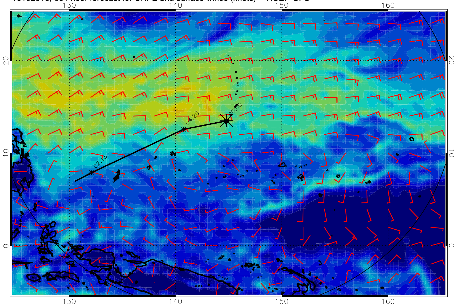
16102818, 054 hour forecast for CAPE and surface winds (knots) -- NCEP GFS
