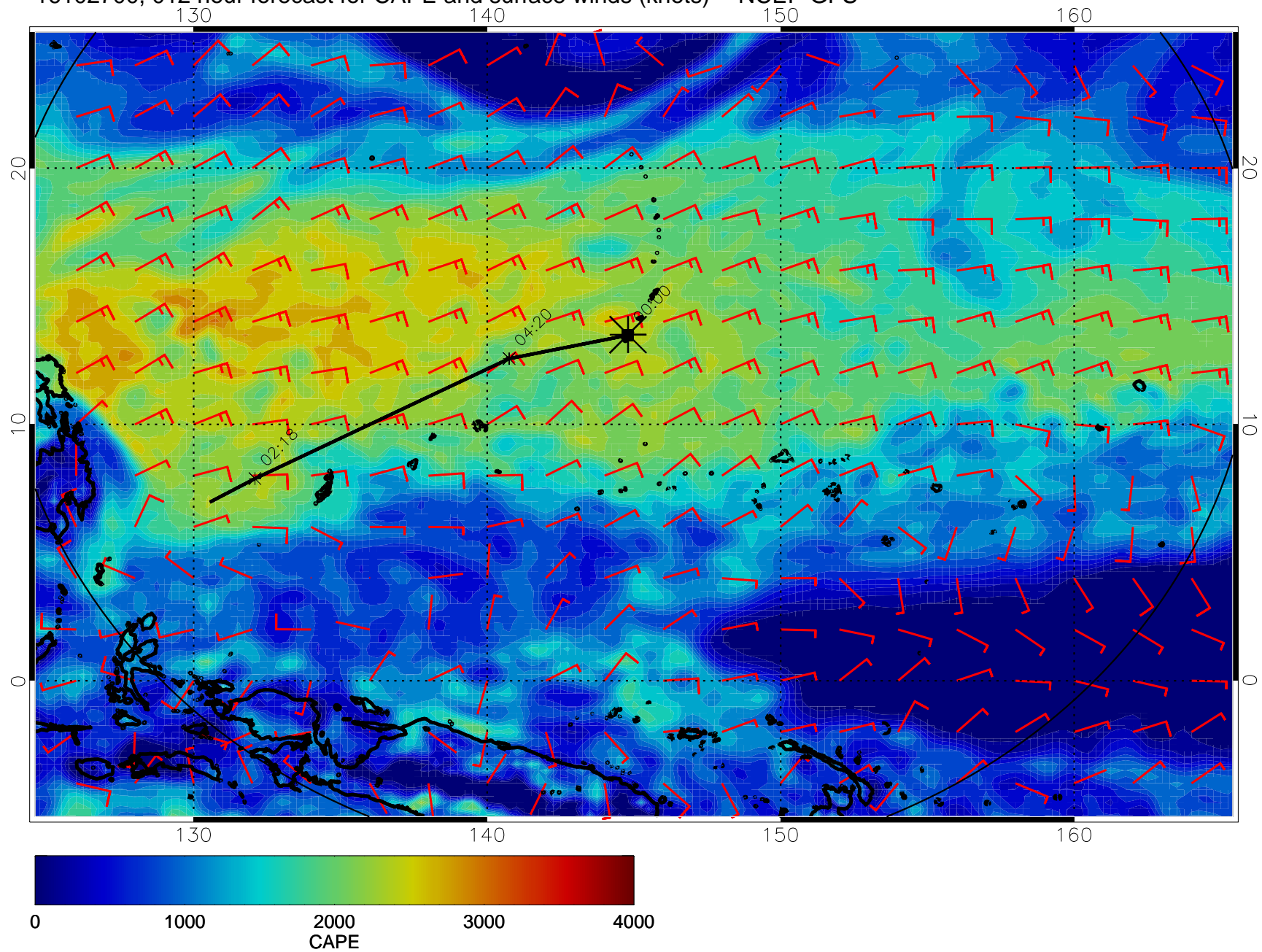
16102700, 012 hour forecast for CAPE and surface winds (knots) -- NCEP GFS
