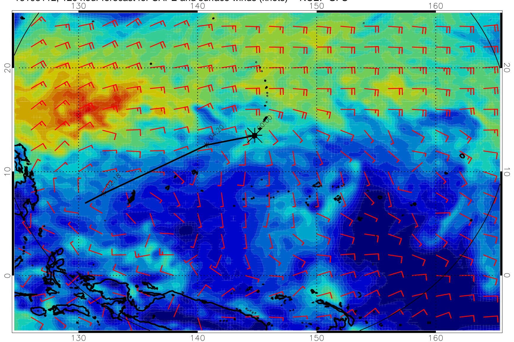
16103112, 120 hour forecast for CAPE and surface winds (knots) -- NCEP GFS
