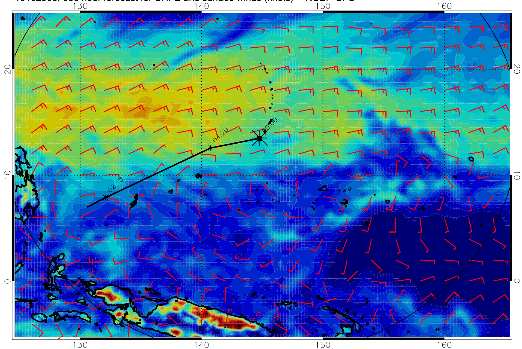
16102906, 066 hour forecast for CAPE and surface winds (knots) -- NCEP GFS
