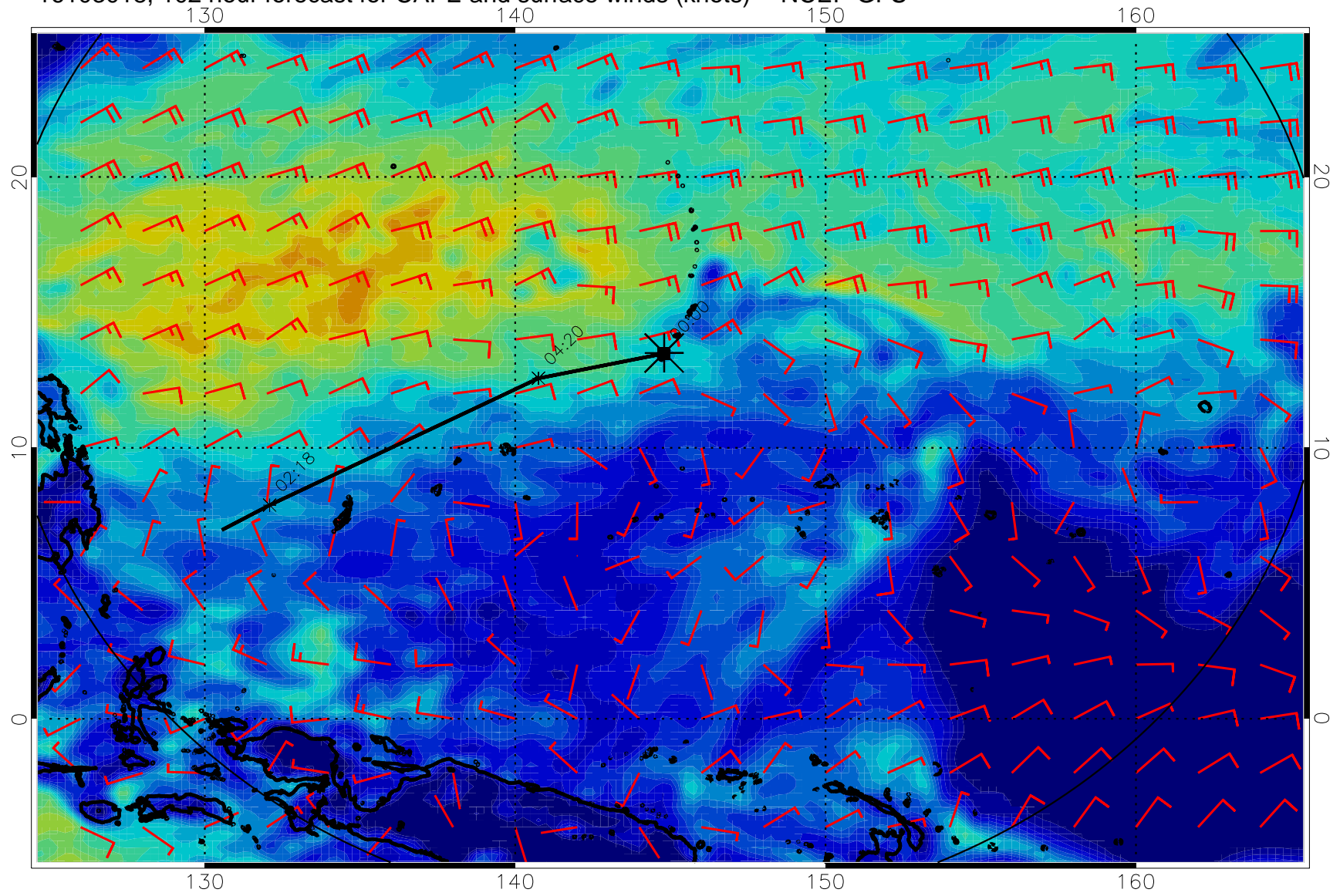
16103018, 102 hour forecast for CAPE and surface winds (knots) -- NCEP GFS
