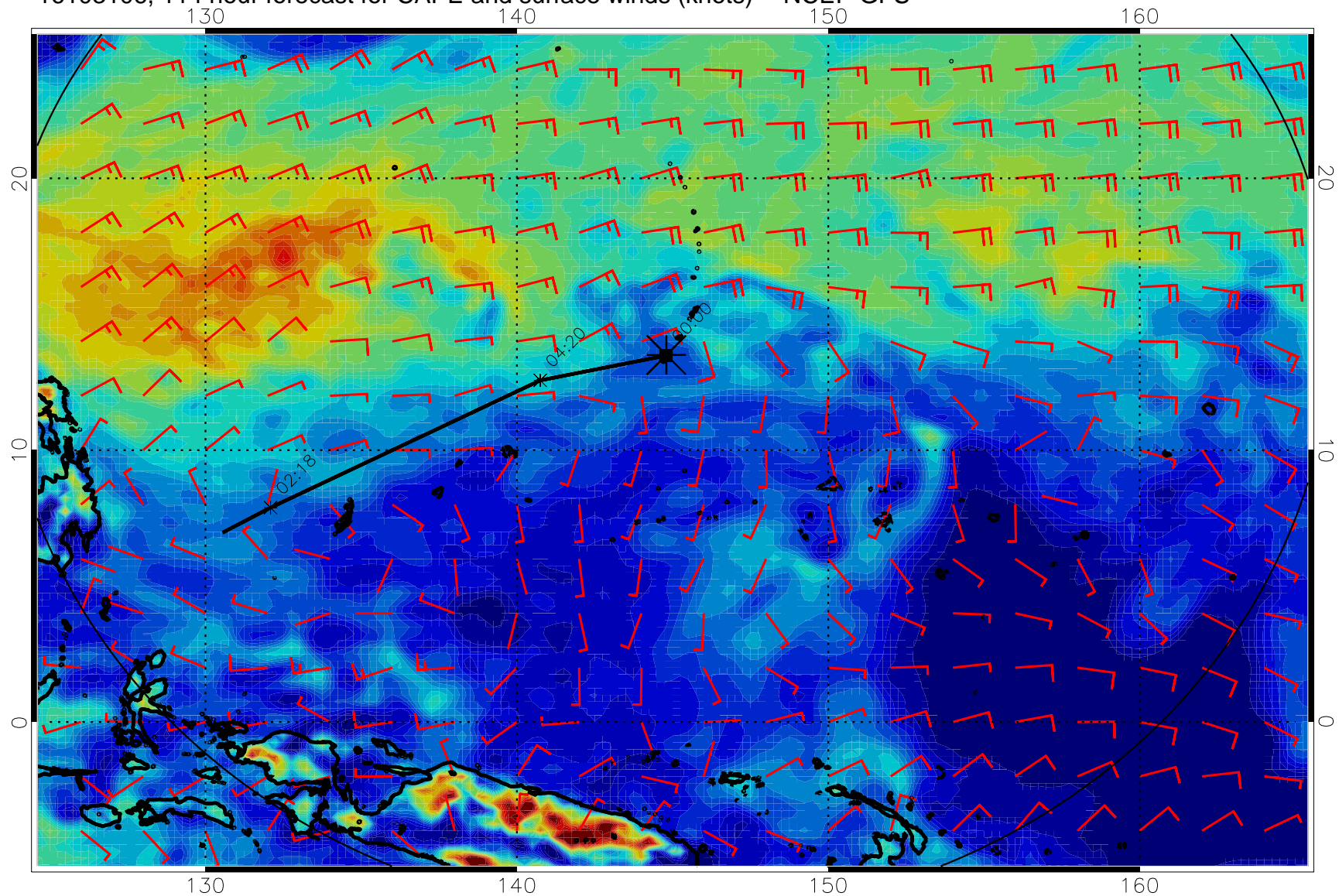
16103106, 114 hour forecast for CAPE and surface winds (knots) -- NCEP GFS
