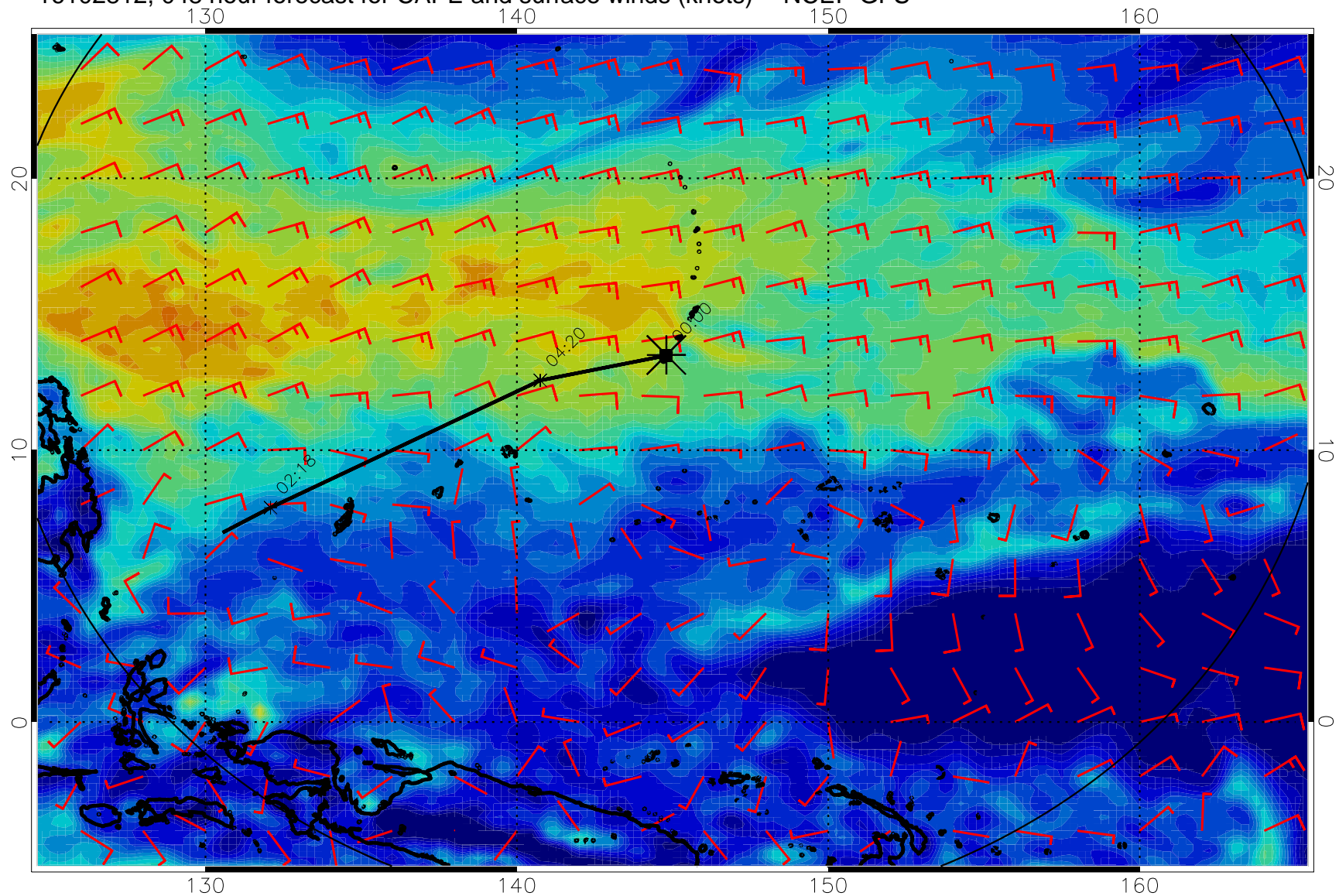
16102812, 048 hour forecast for CAPE and surface winds (knots) -- NCEP GFS
