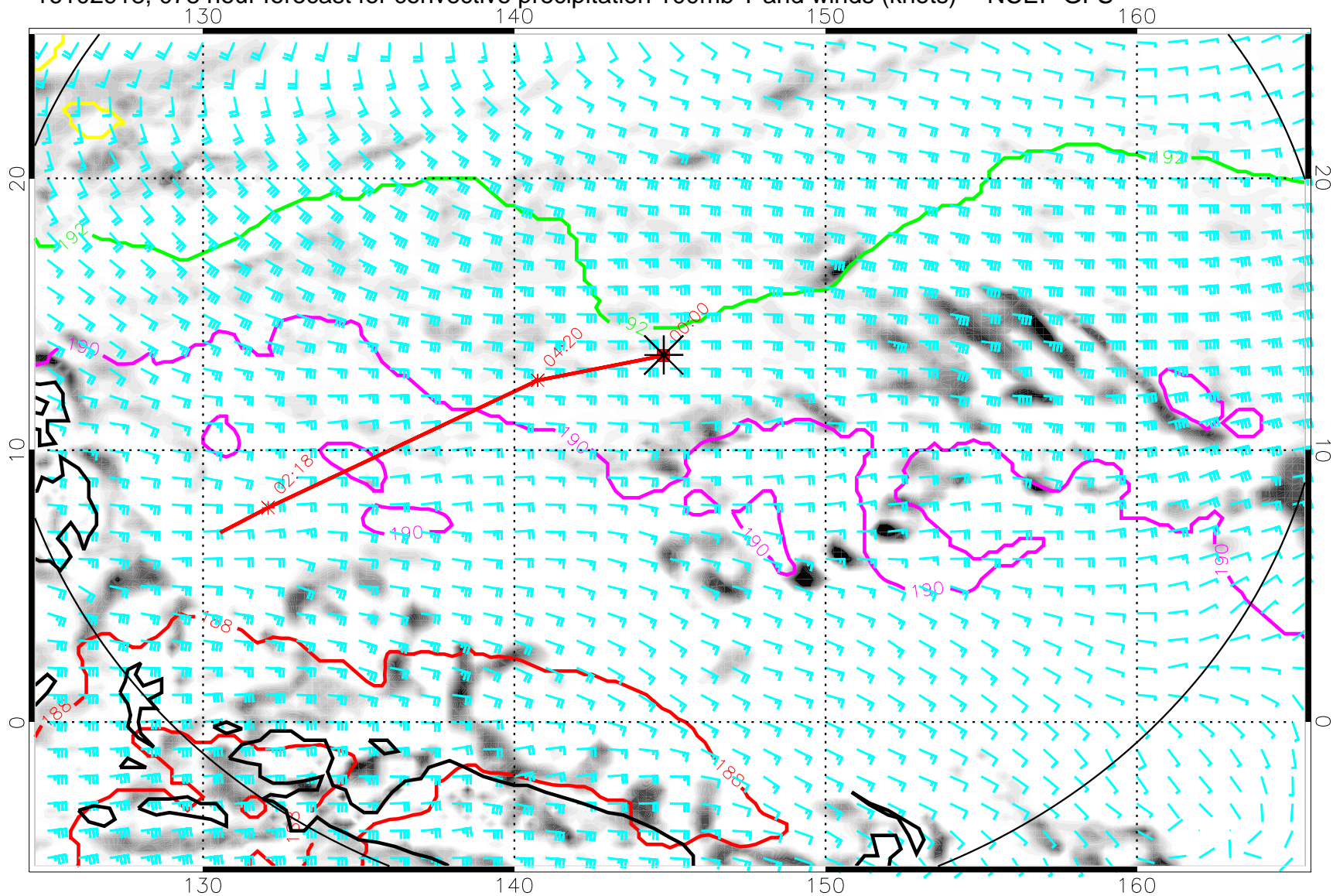
16102918, 078 hour forecast for convective precipitation 100mb T and winds (knots) -- NCEP GFS
