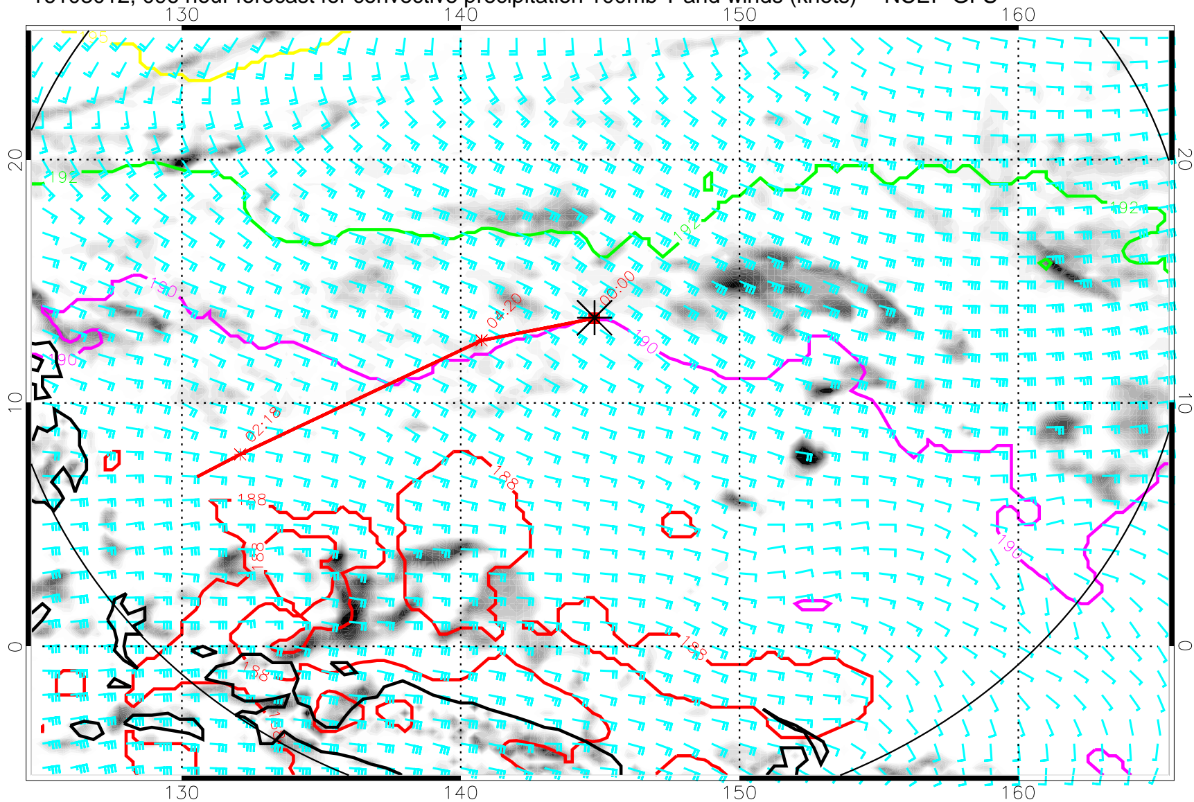
16103012, 096 hour forecast for convective precipitation 100mb T and winds (knots) -- NCEP GFS
