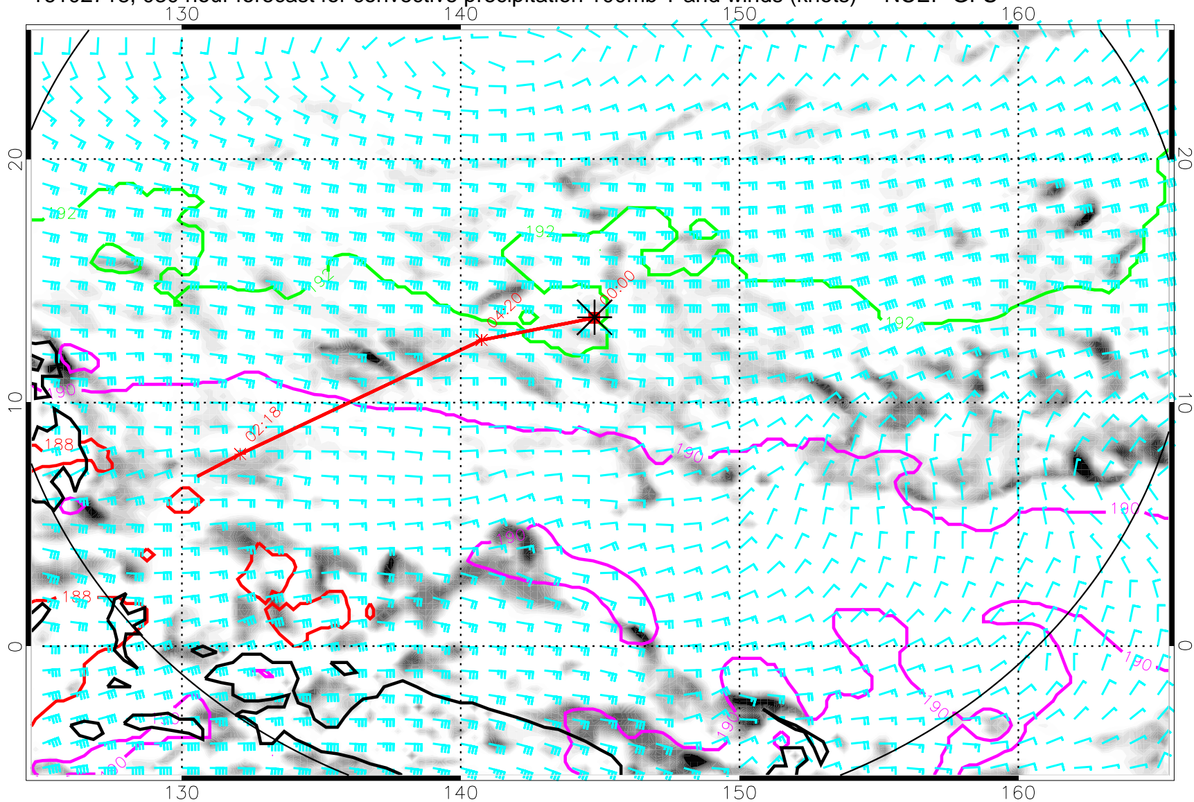
16102718, 030 hour forecast for convective precipitation 100mb T and winds (knots) -- NCEP GFS
