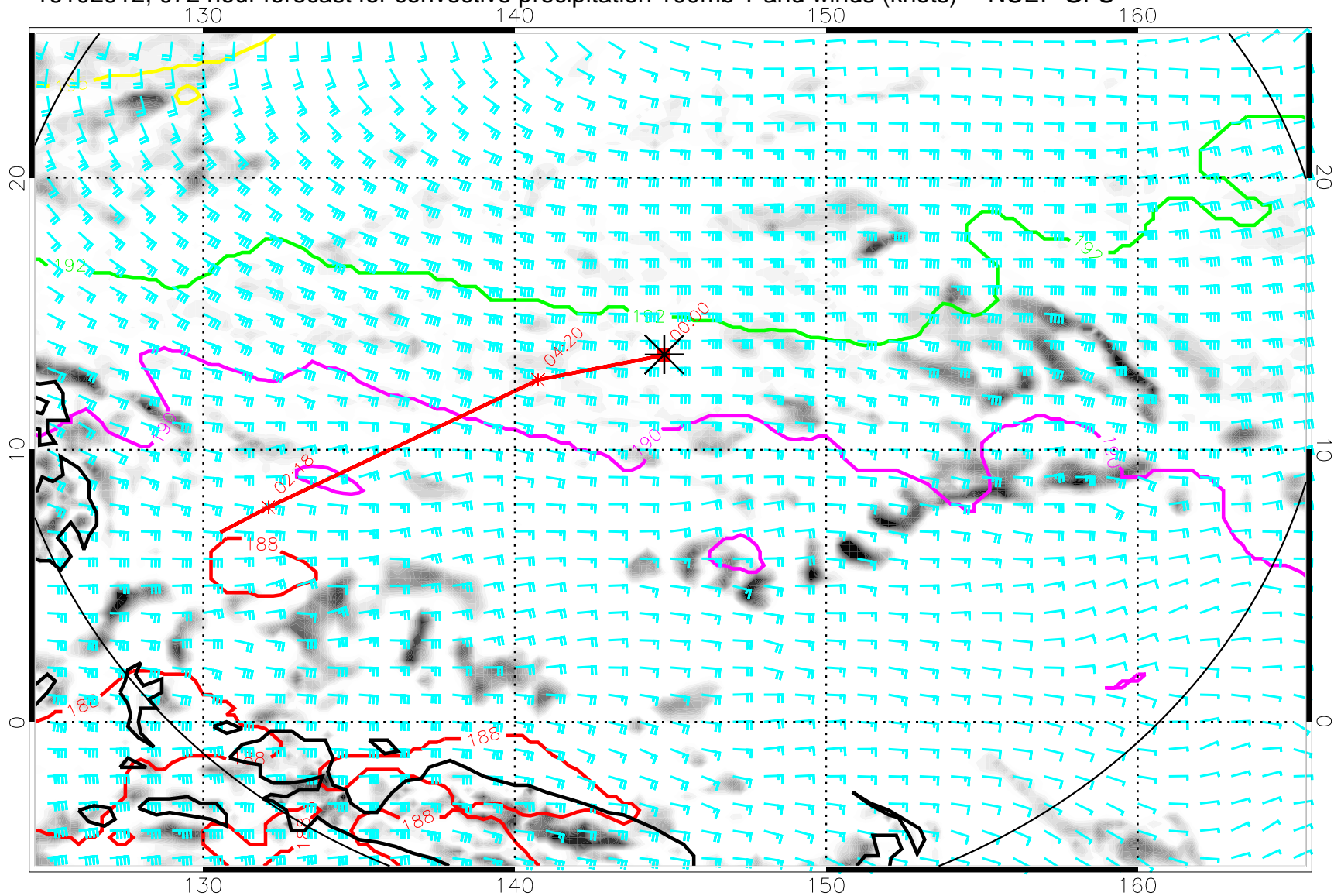
16102912, 072 hour forecast for convective precipitation 100mb T and winds (knots) -- NCEP GFS
