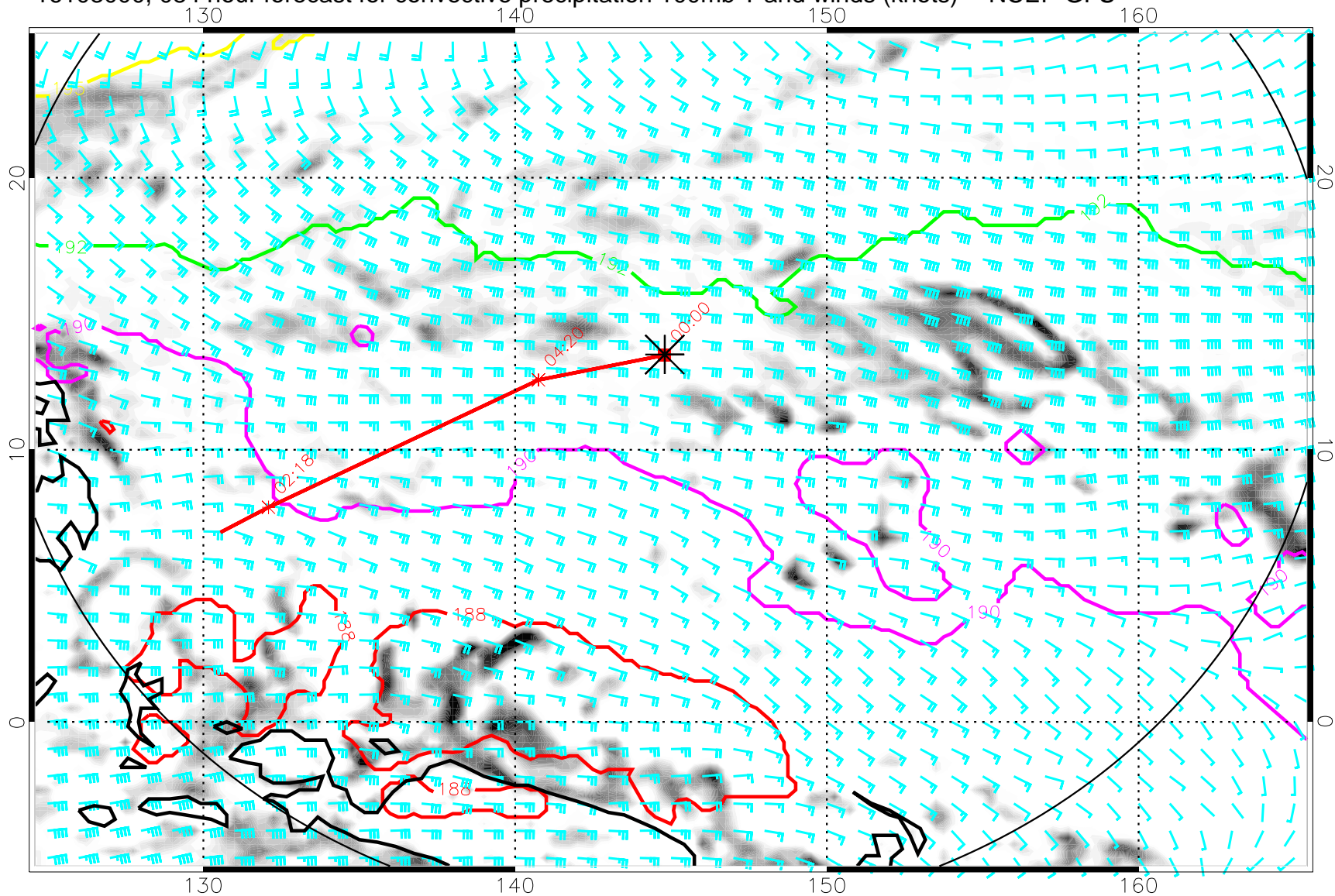
16103000, 084 hour forecast for convective precipitation 100mb T and winds (knots) -- NCEP GFS
