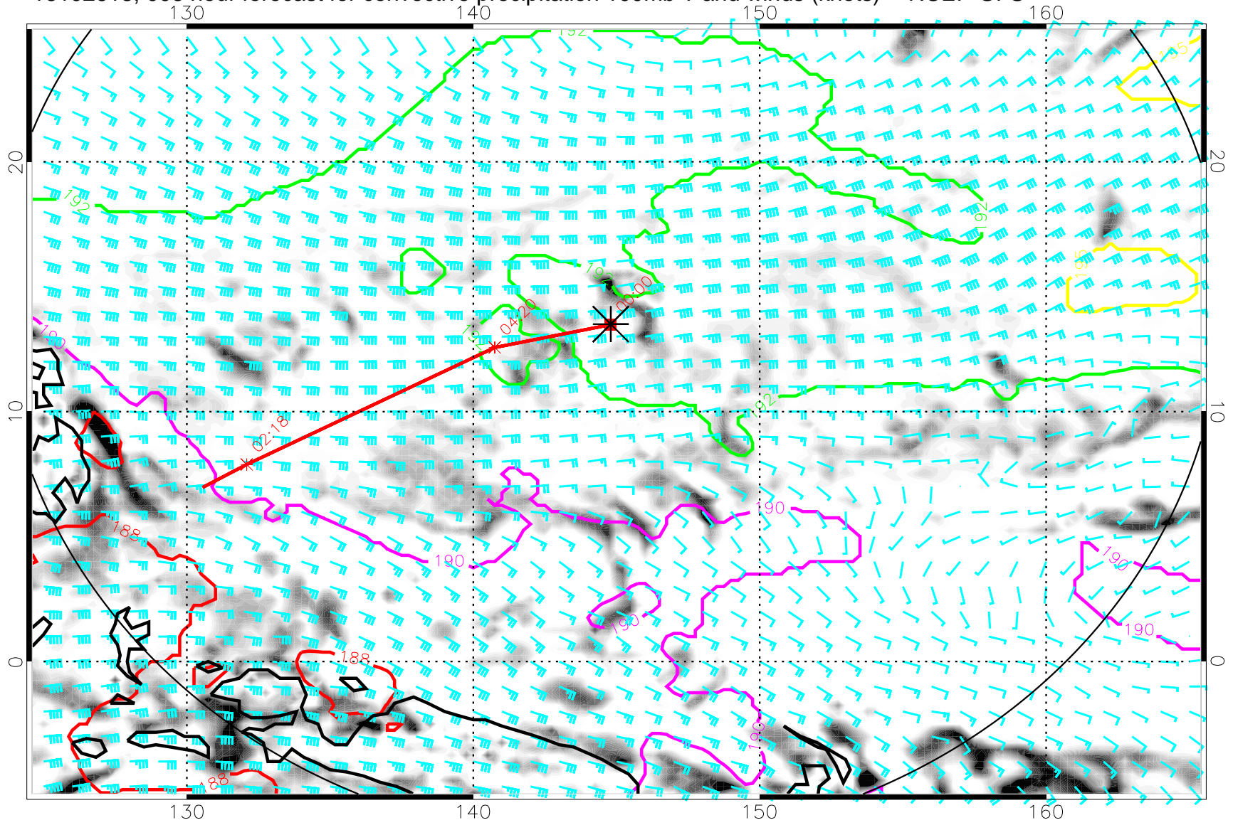
16102618, 006 hour forecast for convective precipitation 100mb T and winds (knots) -- NCEP GFS
