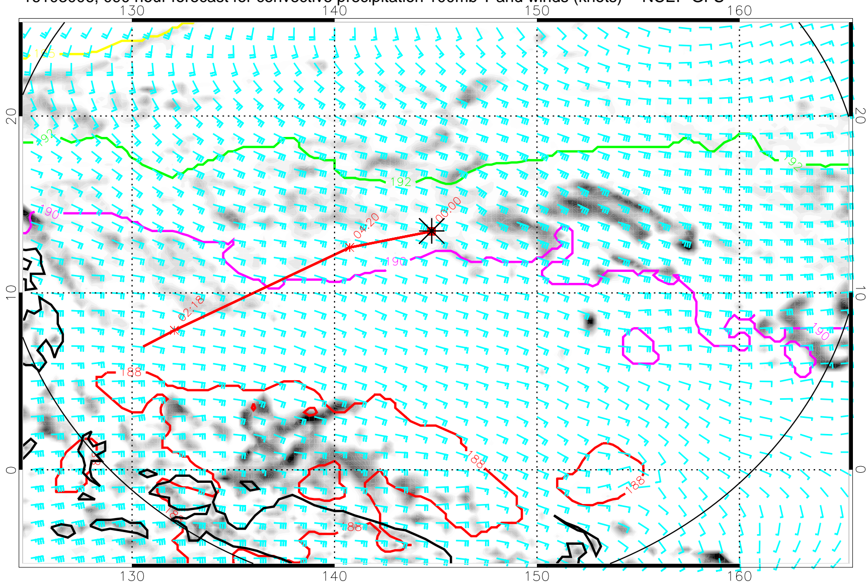
16103006, 090 hour forecast for convective precipitation 100mb T and winds (knots) -- NCEP GFS
