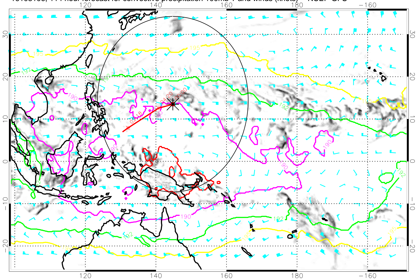
16103106, 114 hour forecast for convective precipitation 100mb T and winds (knots) -- NCEP GFS
