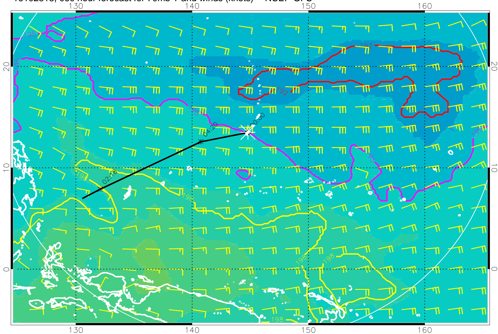
16102818, 060 hour forecast for 70mb T and winds (knots) -- NCEP GFS
