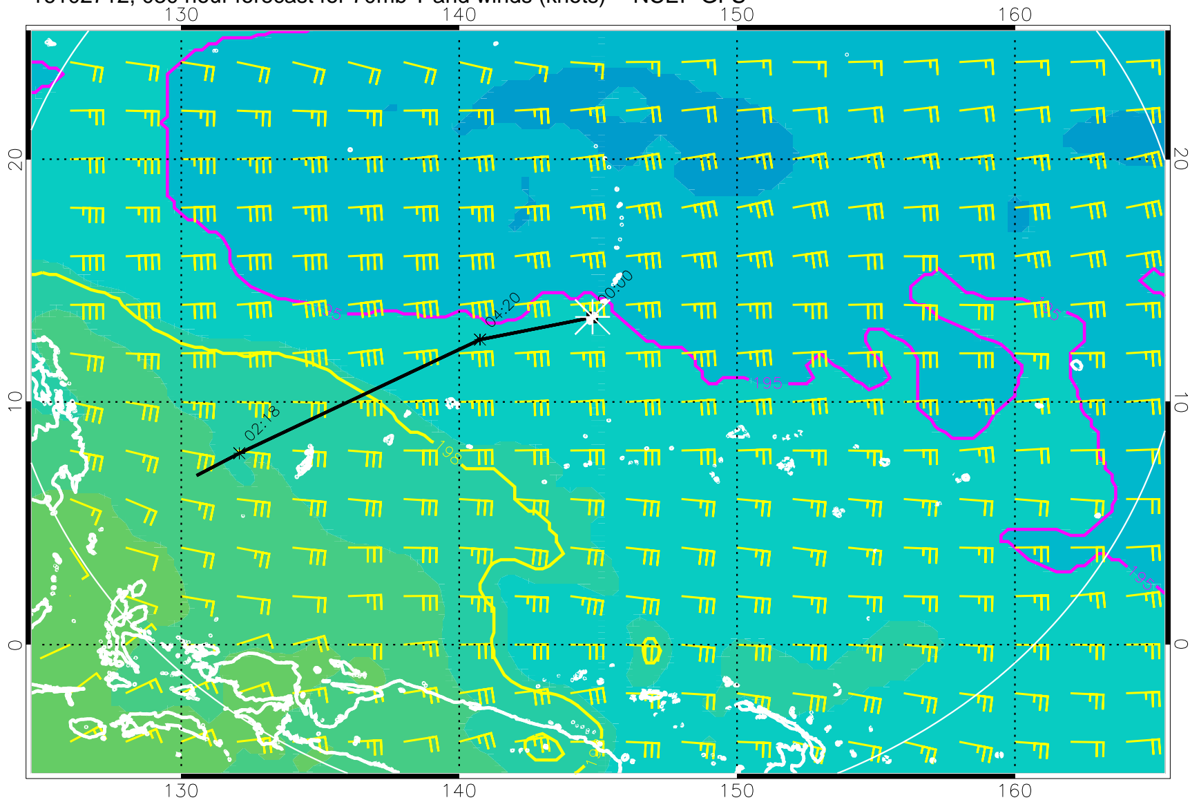
16102712, 030 hour forecast for 70mb T and winds (knots) -- NCEP GFS
