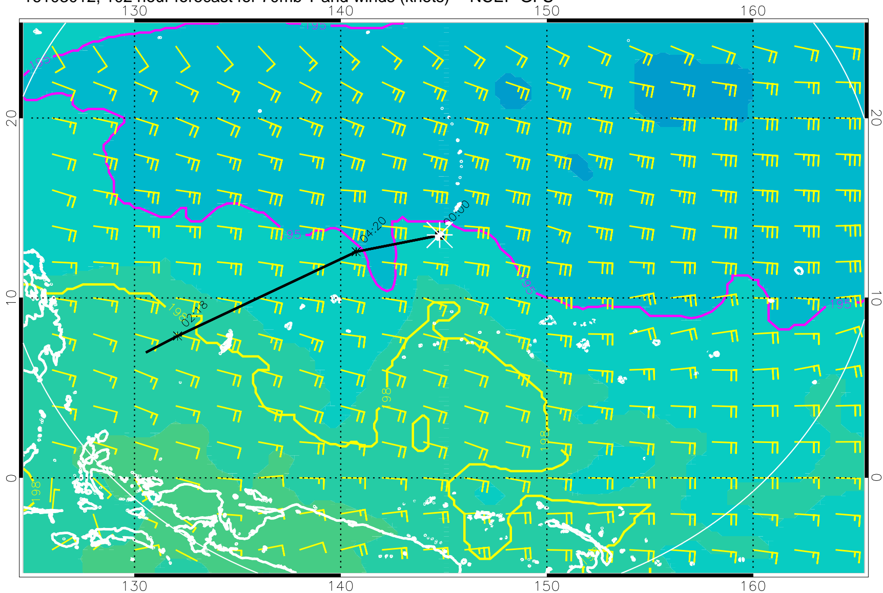
16103012, 102 hour forecast for 70mb T and winds (knots) -- NCEP GFS
