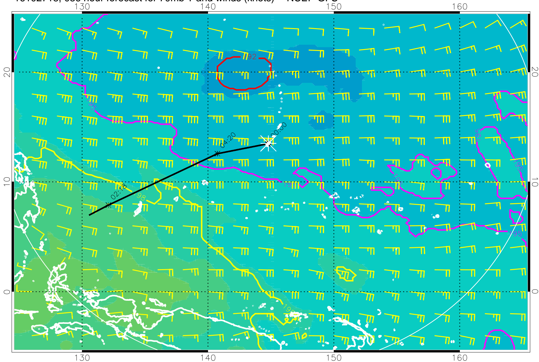
16102718, 036 hour forecast for 70mb T and winds (knots) -- NCEP GFS
