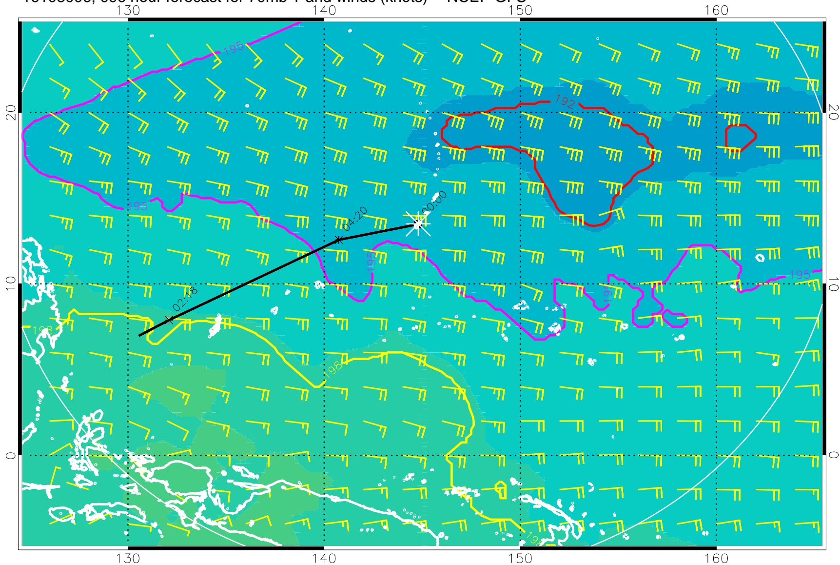
16103006, 096 hour forecast for 70mb T and winds (knots) -- NCEP GFS
