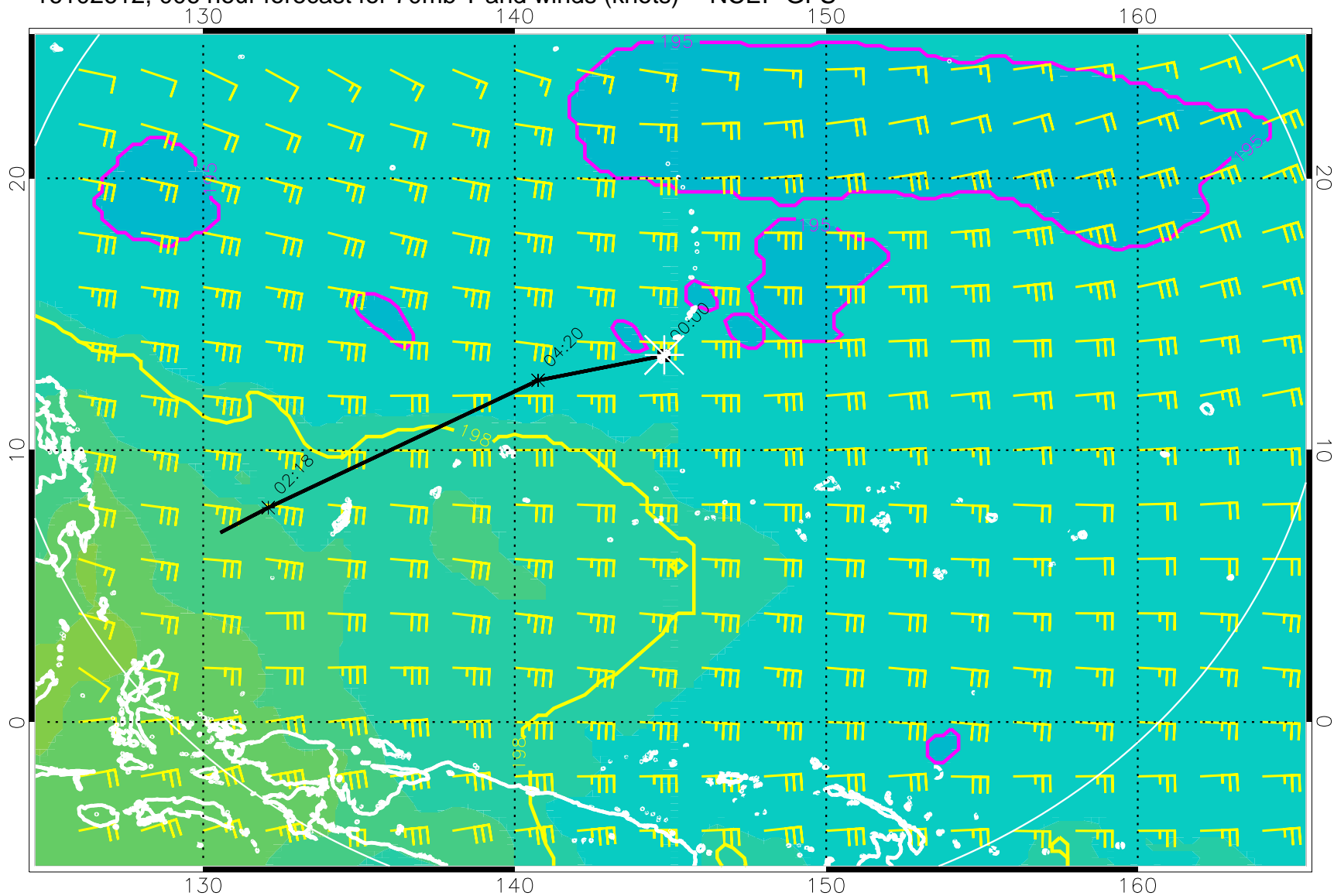
16102612, 006 hour forecast for 70mb T and winds (knots) -- NCEP GFS
