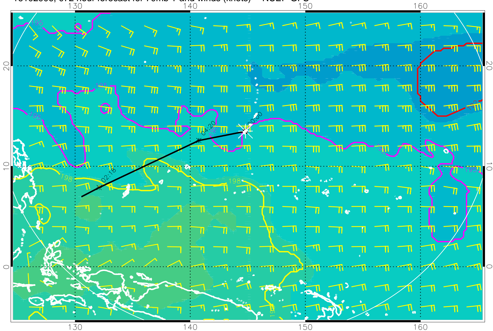
16102906, 072 hour forecast for 70mb T and winds (knots) -- NCEP GFS
