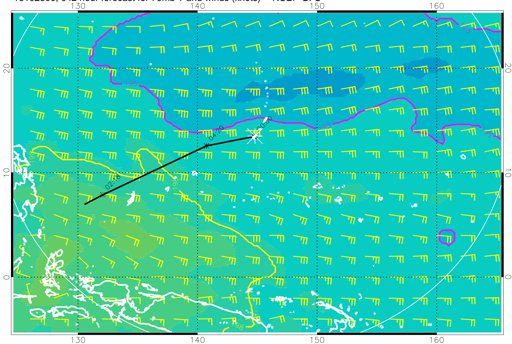
16102800, 042 hour forecast for 70mb T and winds (knots) -- NCEP GFS
