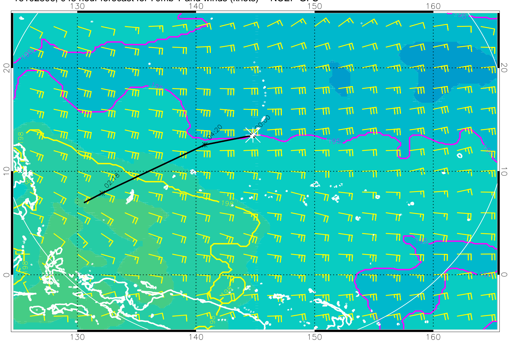
16102806, 048 hour forecast for 70mb T and winds (knots) -- NCEP GFS
