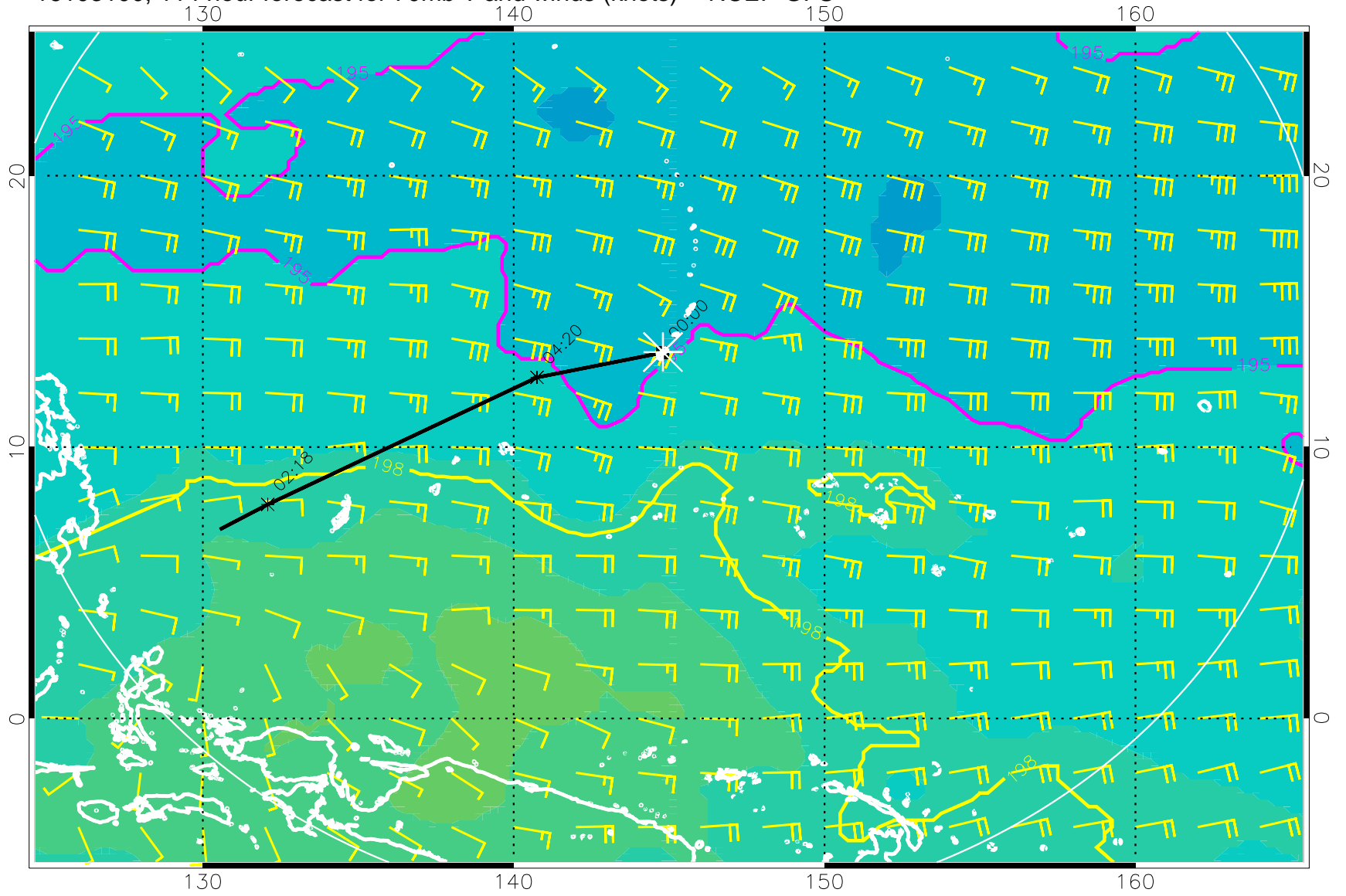
16103100, 114 hour forecast for 70mb T and winds (knots) -- NCEP GFS
