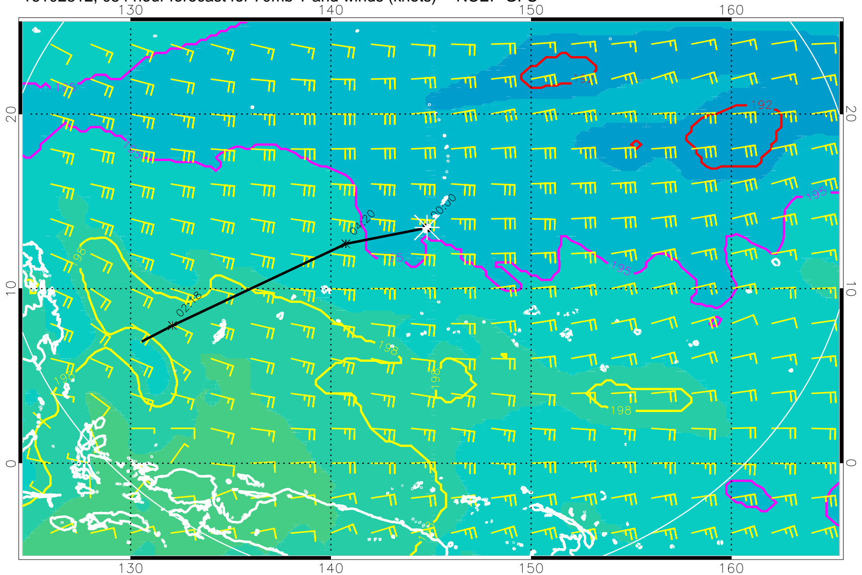
16102812, 054 hour forecast for 70mb T and winds (knots) -- NCEP GFS
