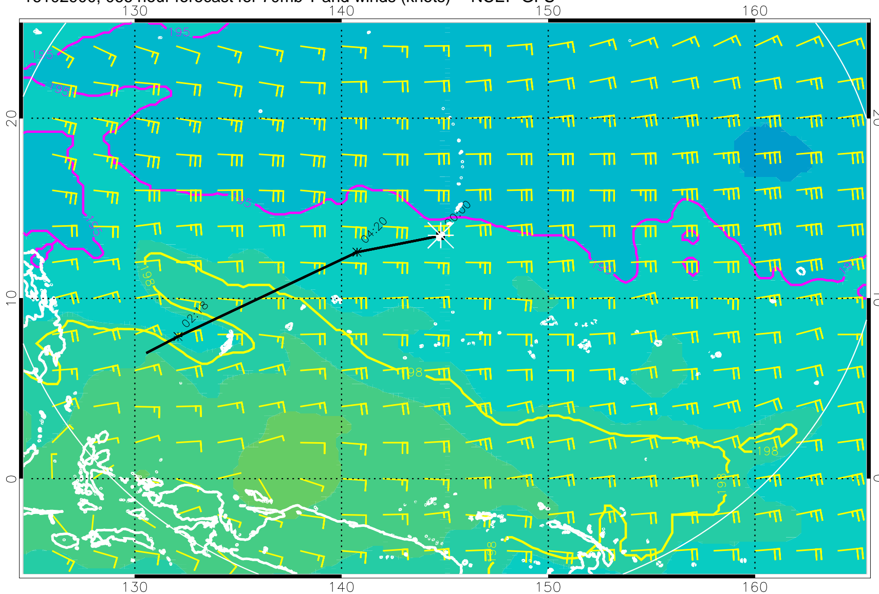
16102900, 066 hour forecast for 70mb T and winds (knots) -- NCEP GFS
