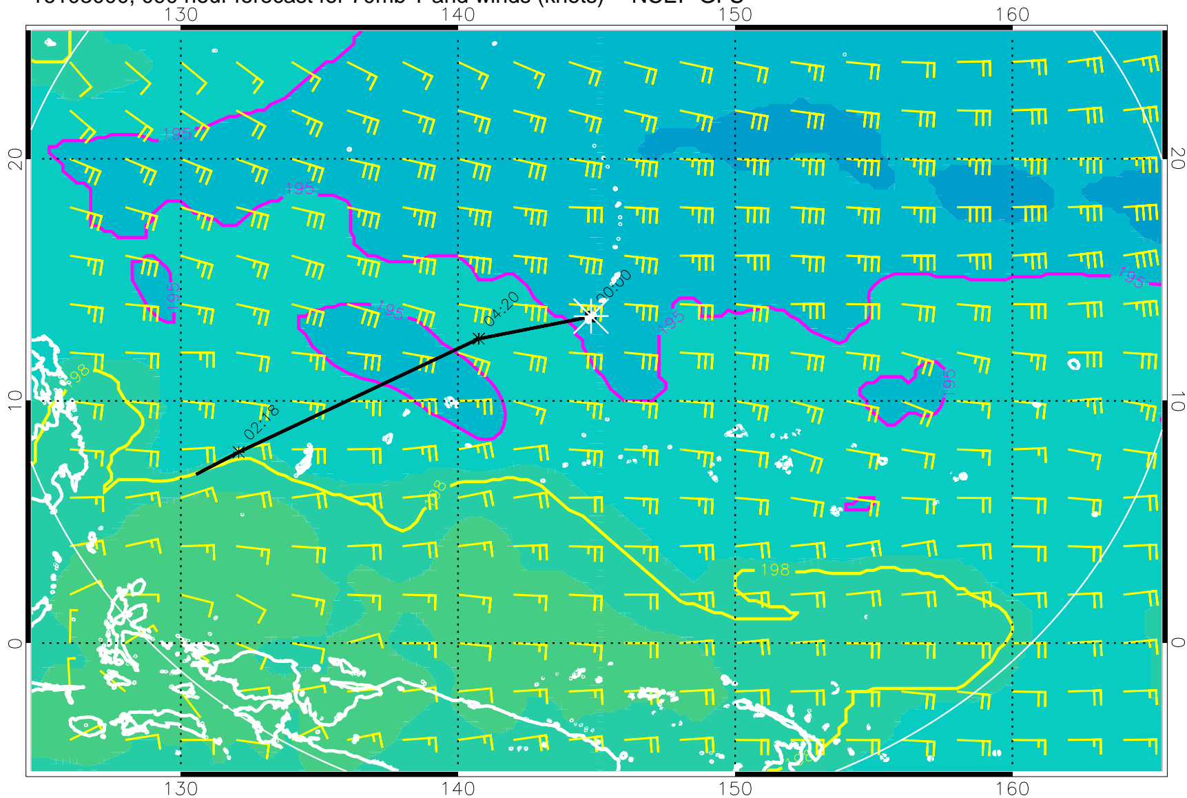
16103000, 090 hour forecast for 70mb T and winds (knots) -- NCEP GFS
