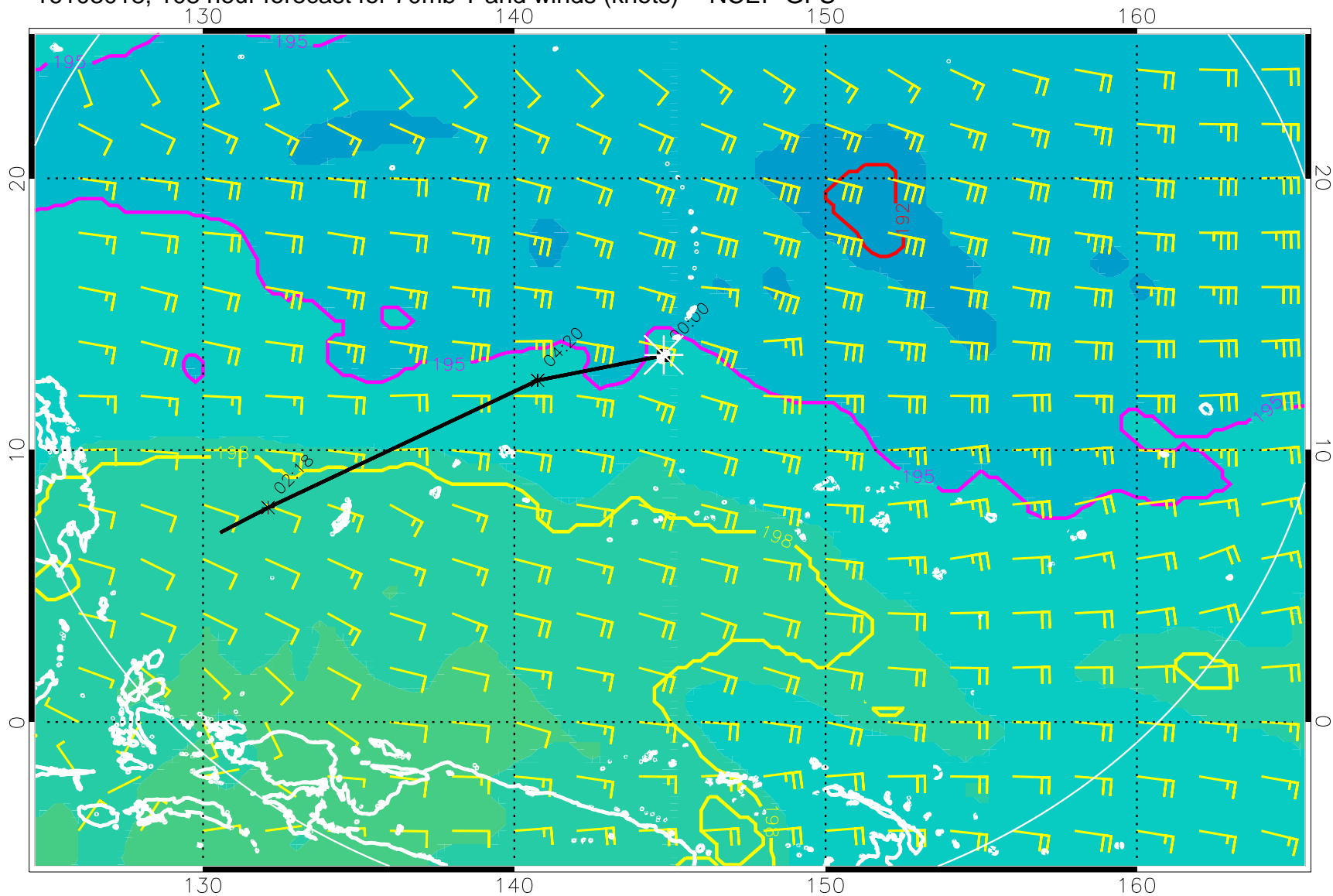
16103018, 108 hour forecast for 70mb T and winds (knots) -- NCEP GFS
