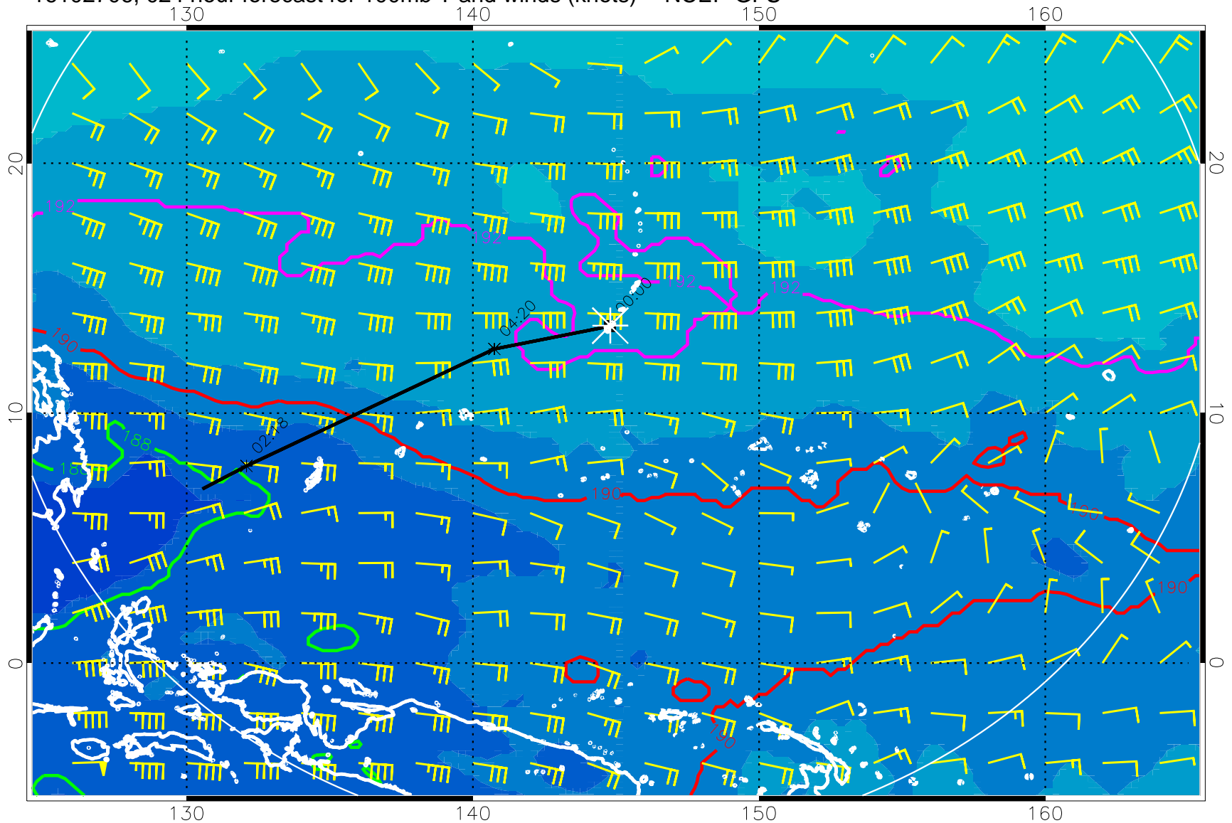
16102706, 024 hour forecast for 100mb T and winds (knots) -- NCEP GFS
