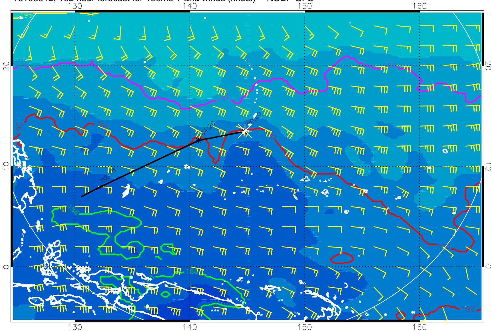
16103012, 102 hour forecast for 100mb T and winds (knots) -- NCEP GFS
