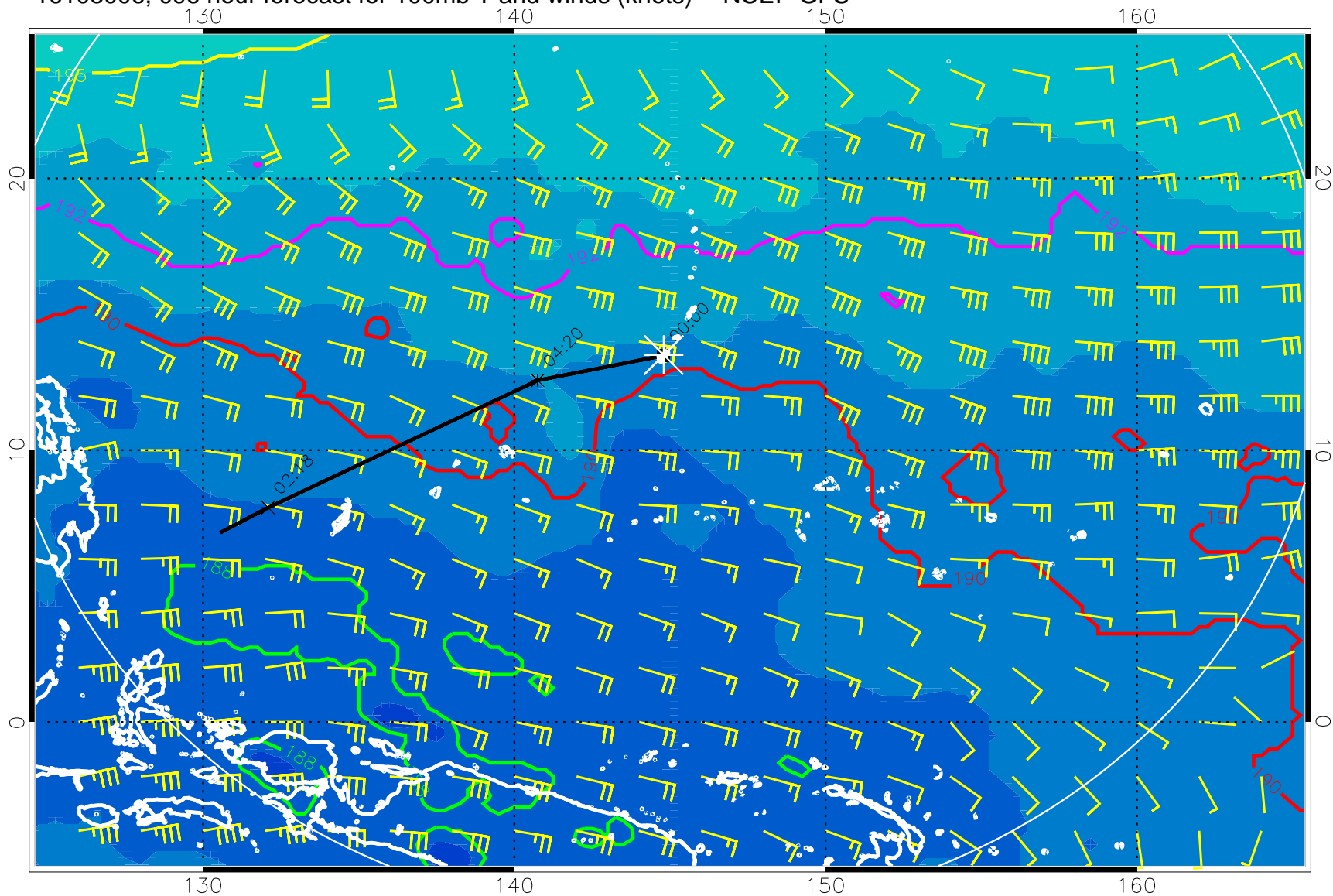
16103006, 096 hour forecast for 100mb T and winds (knots) -- NCEP GFS
