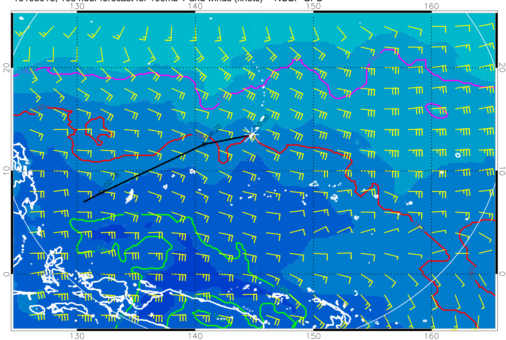
16103018, 108 hour forecast for 100mb T and winds (knots) -- NCEP GFS
