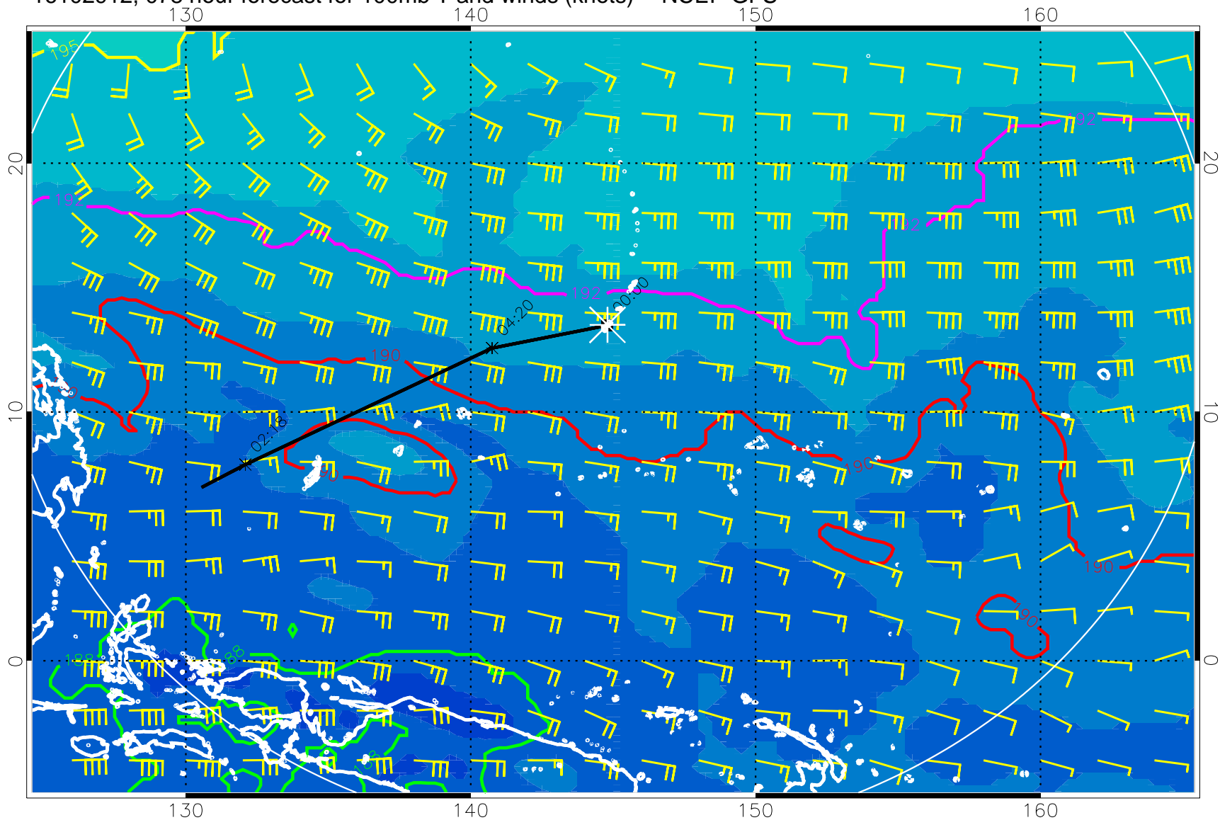
16102912, 078 hour forecast for 100mb T and winds (knots) -- NCEP GFS
