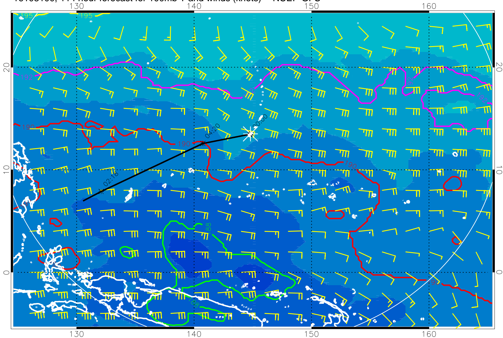
16103100, 114 hour forecast for 100mb T and winds (knots) -- NCEP GFS
