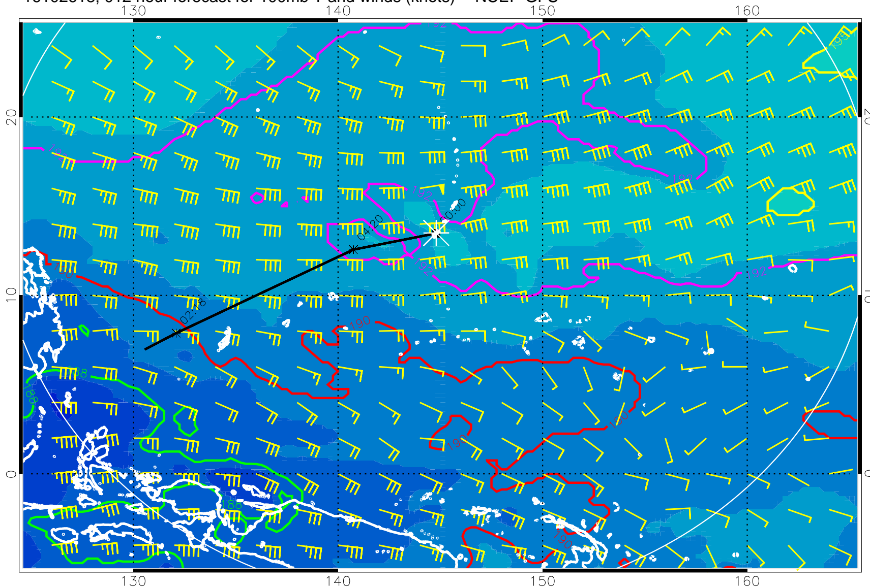
16102618, 012 hour forecast for 100mb T and winds (knots) -- NCEP GFS
