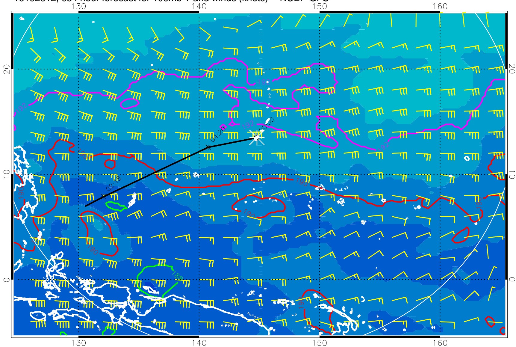
16102812, 054 hour forecast for 100mb T and winds (knots) -- NCEP GFS
