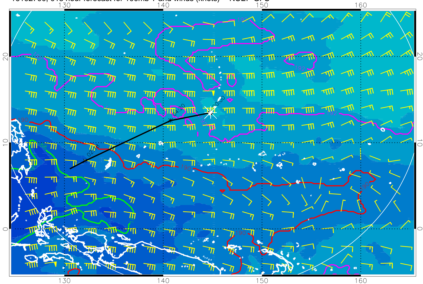
16102700, 018 hour forecast for 100mb T and winds (knots) -- NCEP GFS
