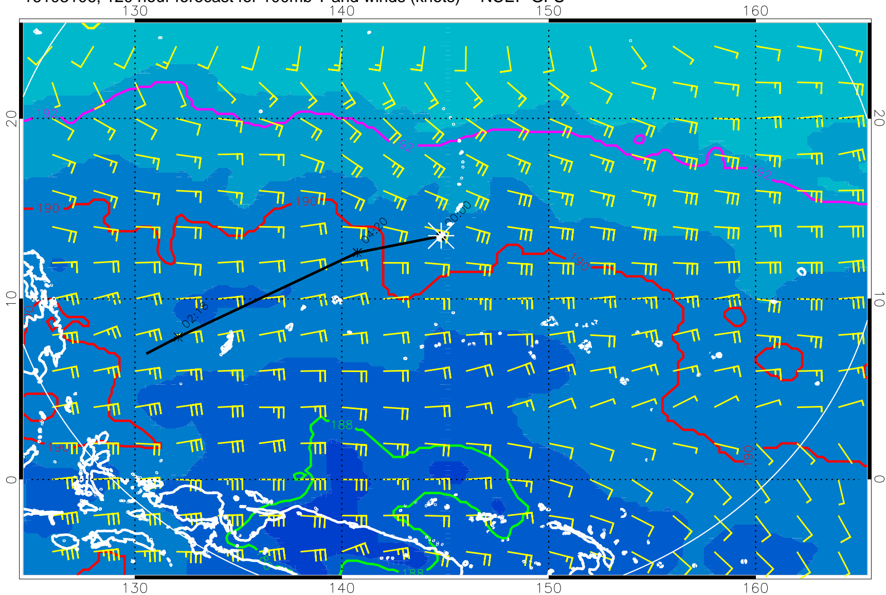
16103106, 120 hour forecast for 100mb T and winds (knots) -- NCEP GFS
