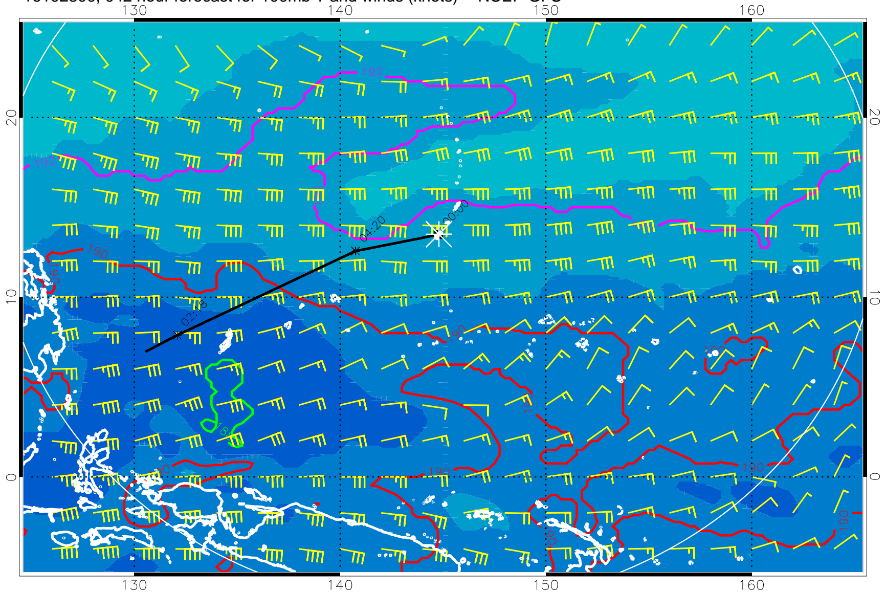
16102800, 042 hour forecast for 100mb T and winds (knots) -- NCEP GFS
