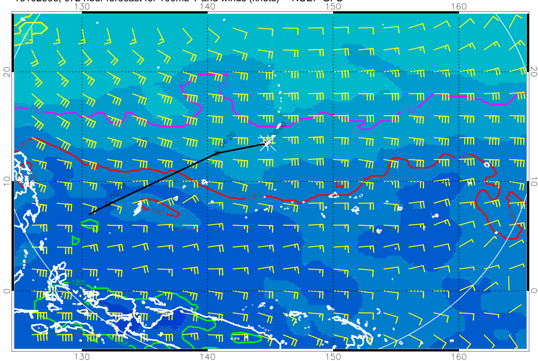
16102906, 072 hour forecast for 100mb T and winds (knots) -- NCEP GFS
