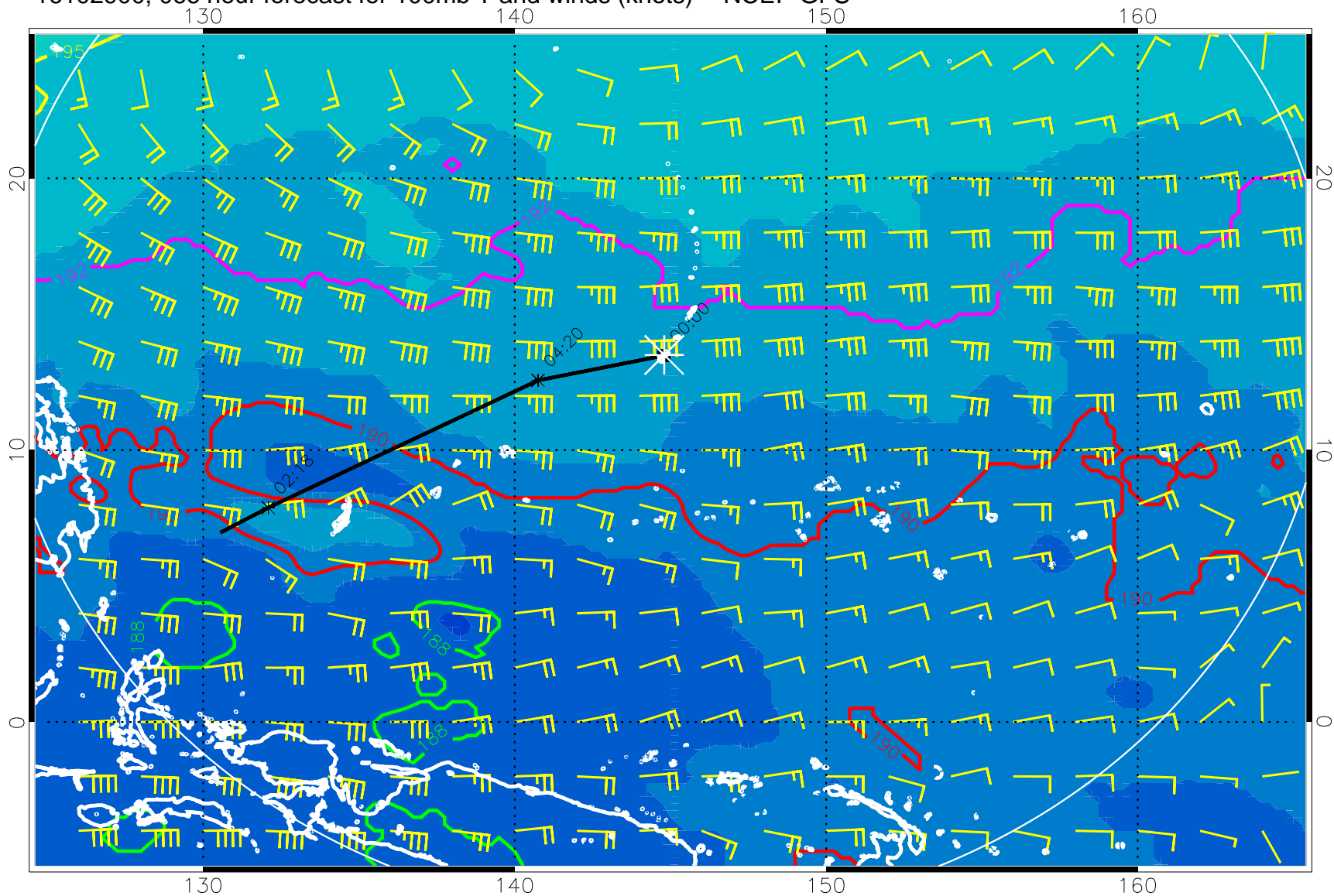
16102900, 066 hour forecast for 100mb T and winds (knots) -- NCEP GFS
