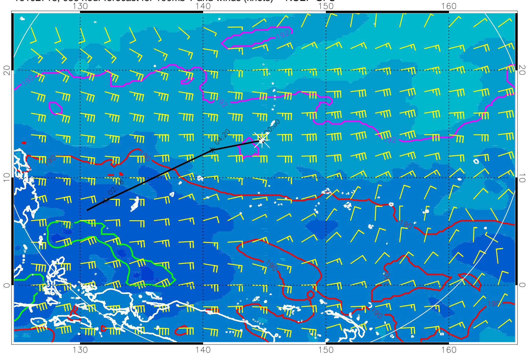
16102718, 036 hour forecast for 100mb T and winds (knots) -- NCEP GFS
