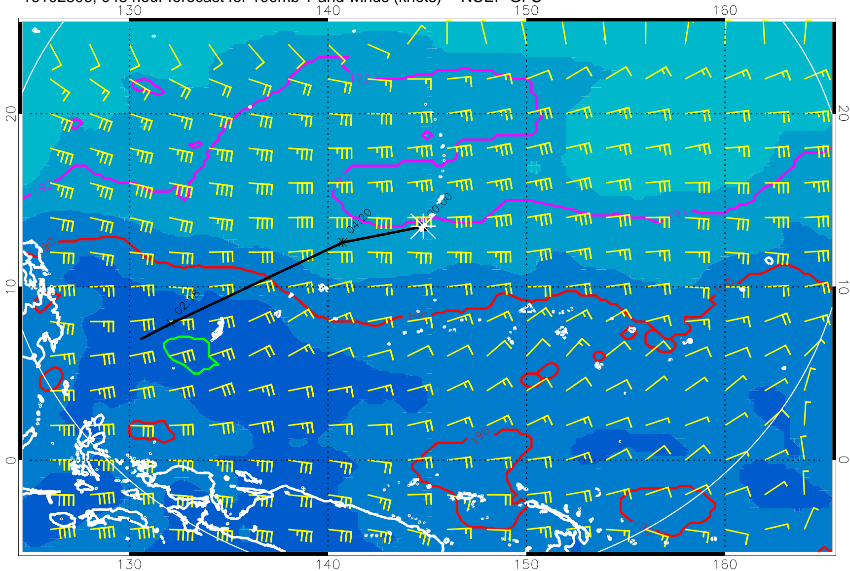
16102806, 048 hour forecast for 100mb T and winds (knots) -- NCEP GFS
