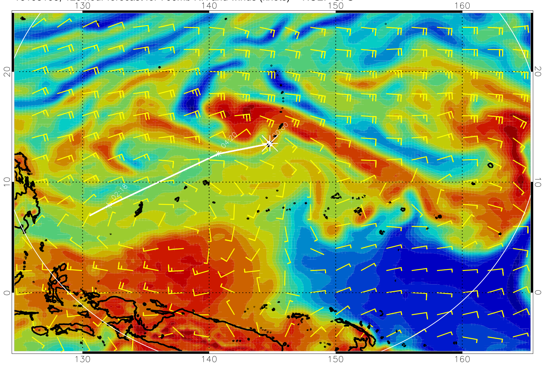
16103106, 120 hour forecast for 700mb RH and winds (knots) -- NCEP GFS
