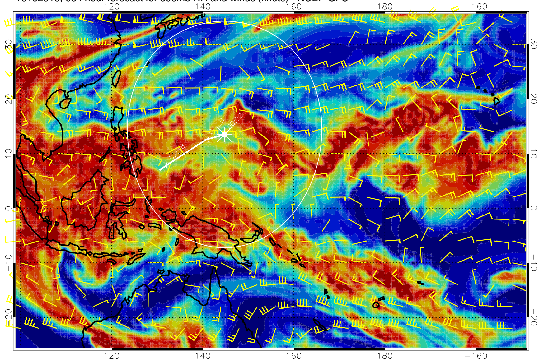
16102918, 084 hour forecast for 500mb RH and winds (knots) - NCEP GFS
