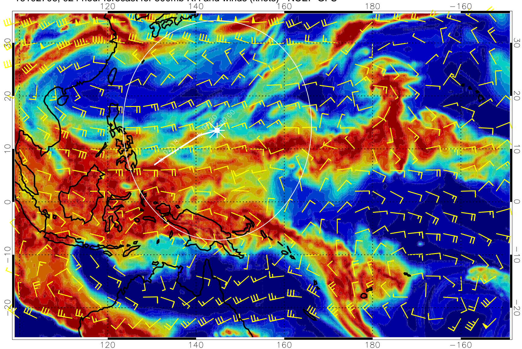
16102706, 024 hour forecast for 500mb RH and winds (knots) - NCEP GFS
