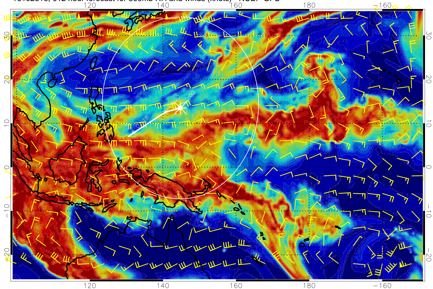
16102618, 012 hour forecast for 500mb RH and winds (knots) - NCEP GFS
