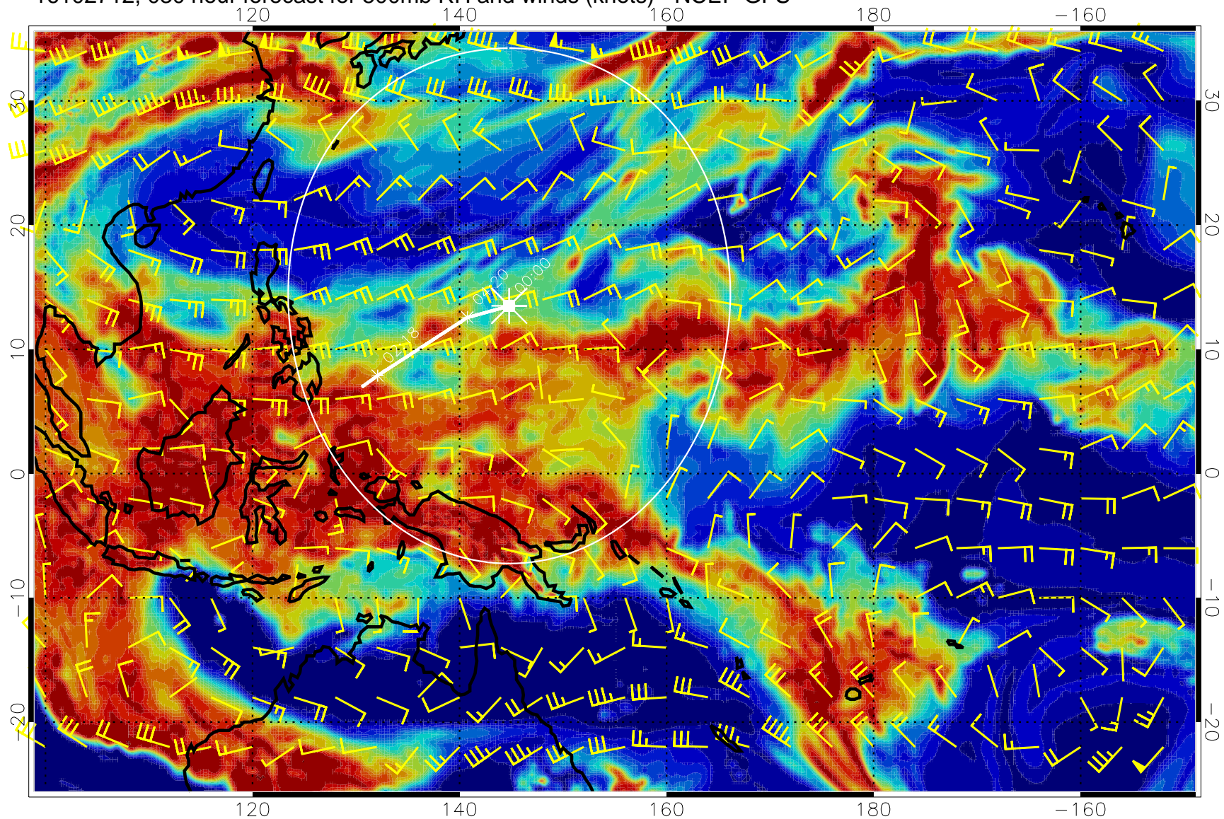
16102712, 030 hour forecast for 500mb RH and winds (knots) - NCEP GFS
