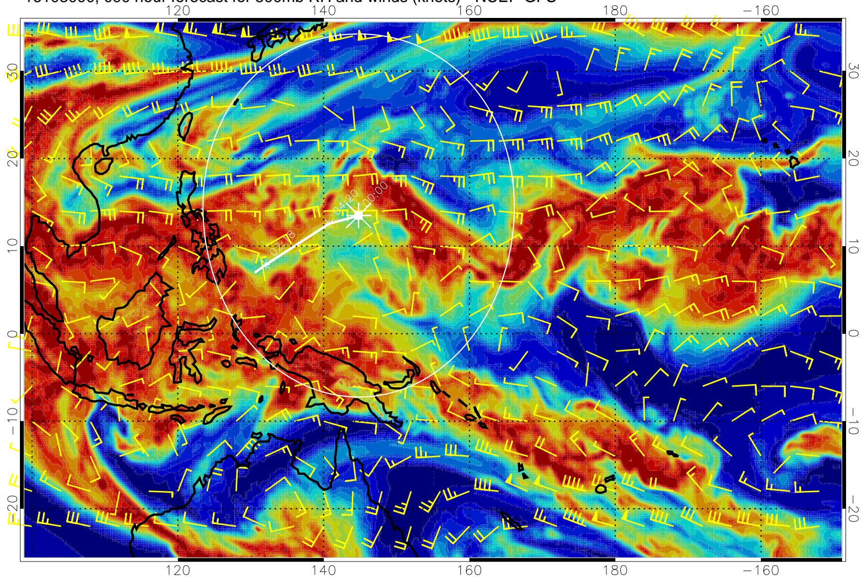
16103000, 090 hour forecast for 500mb RH and winds (knots) - NCEP GFS
