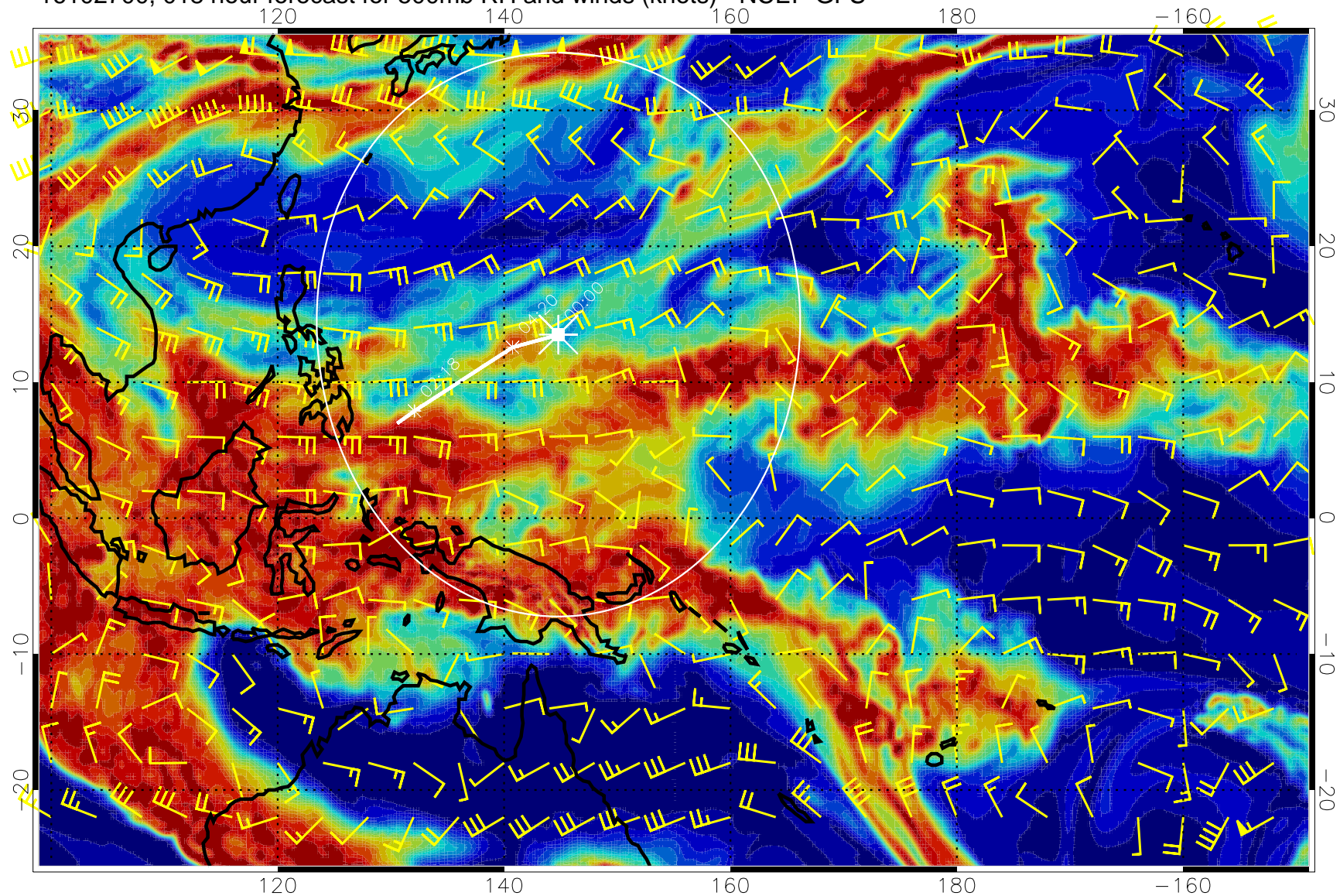
16102700, 018 hour forecast for 500mb RH and winds (knots) - NCEP GFS
