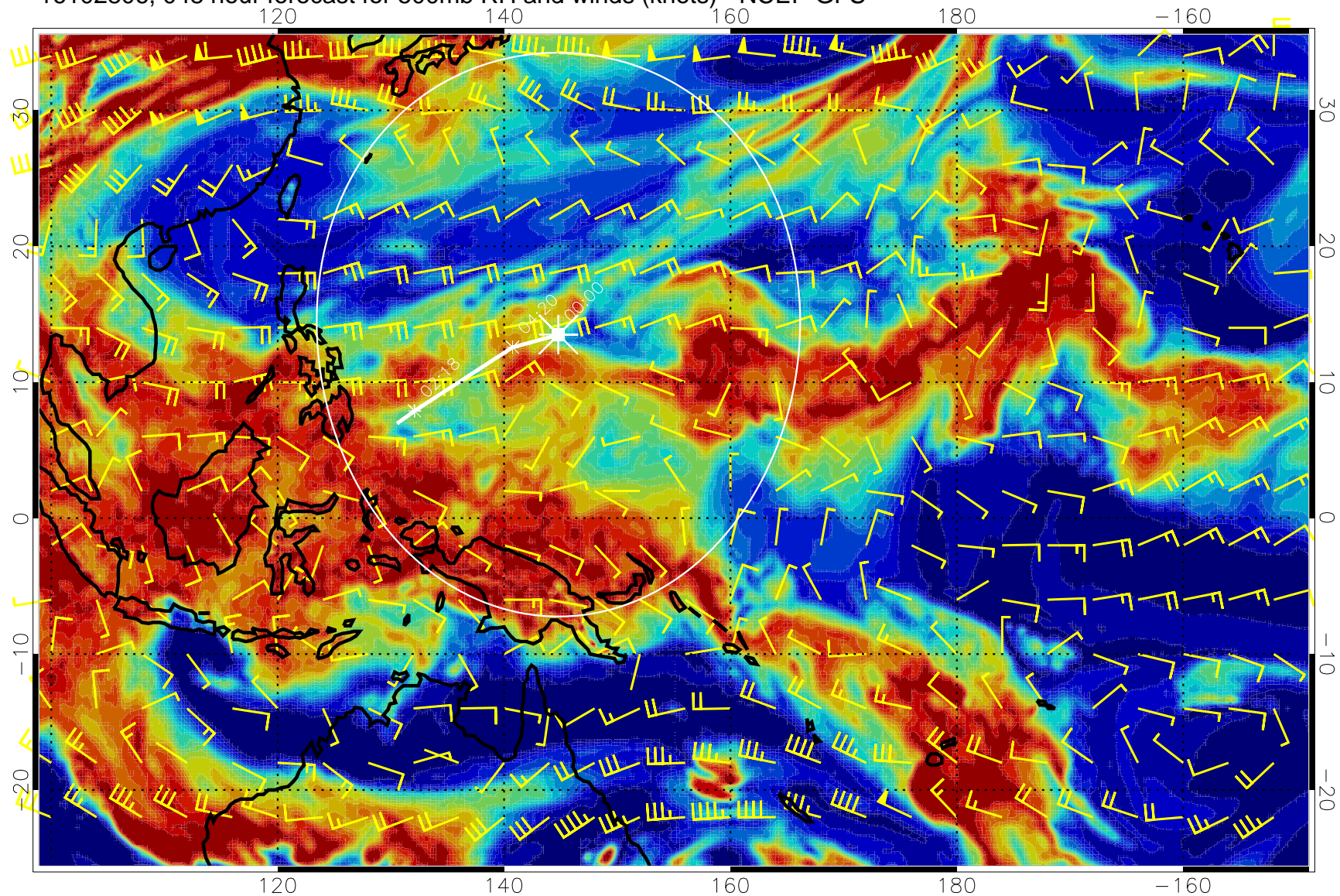
16102806, 048 hour forecast for 500mb RH and winds (knots) - NCEP GFS
