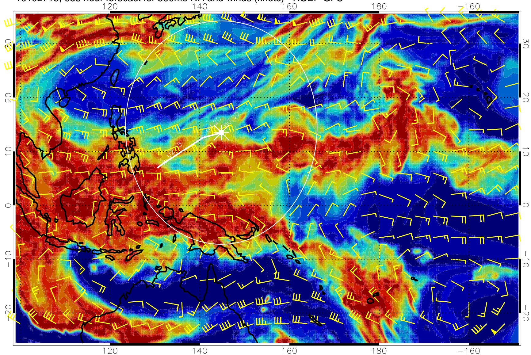
16102718, 036 hour forecast for 500mb RH and winds (knots) - NCEP GFS
