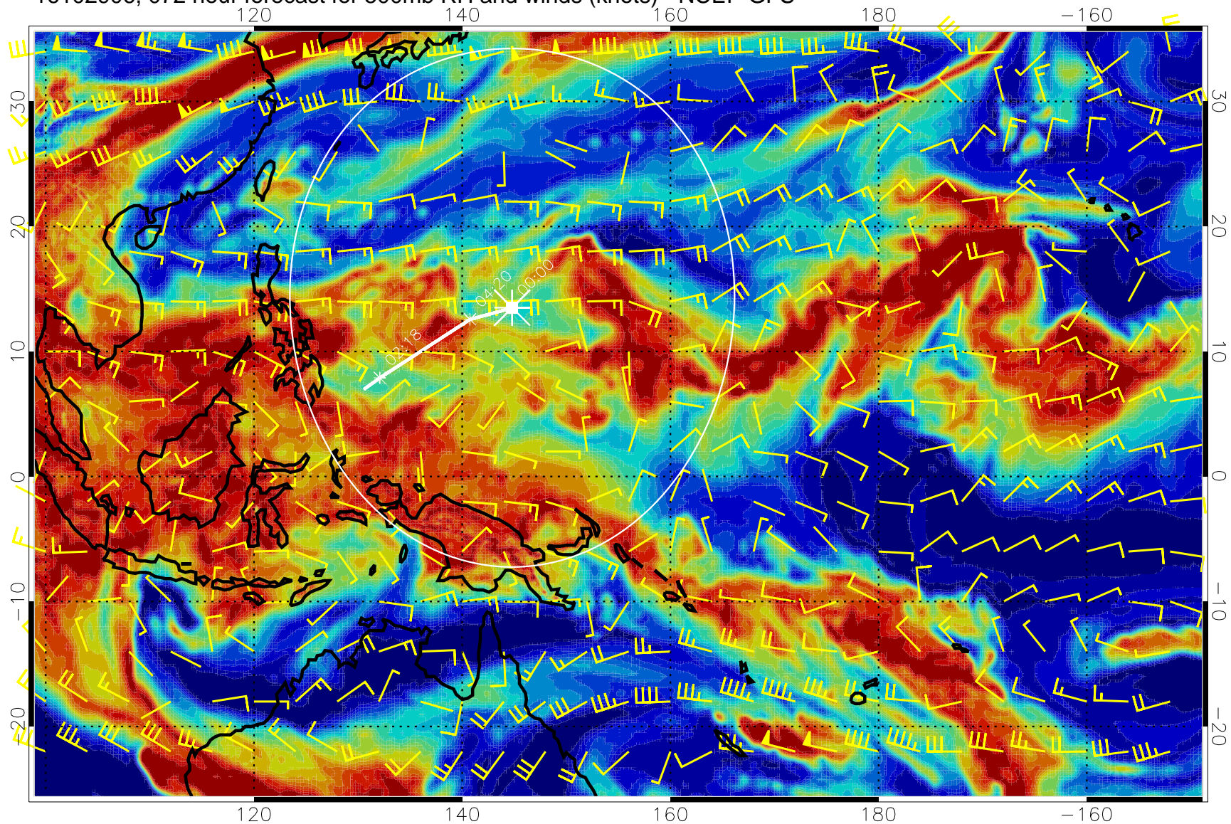
16102906, 072 hour forecast for 500mb RH and winds (knots) - NCEP GFS
