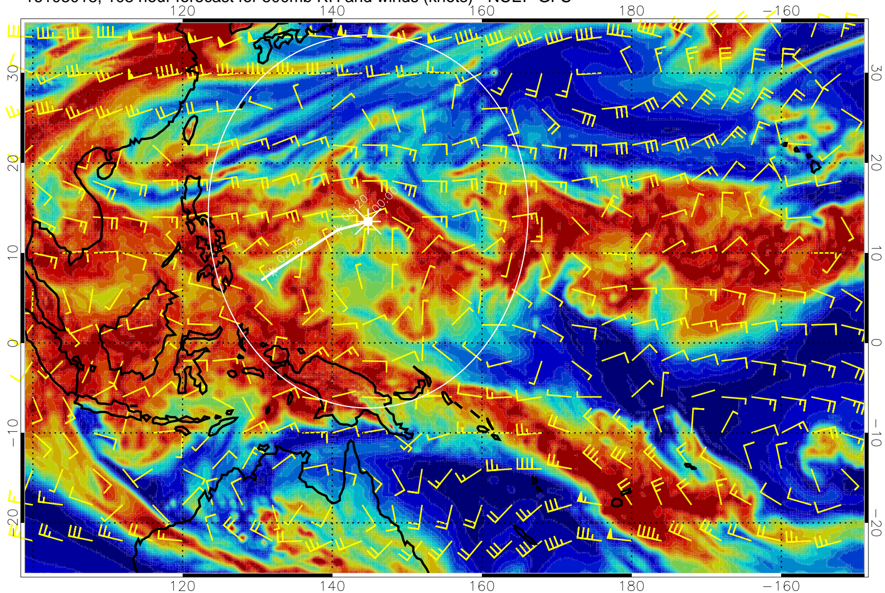
16103018, 108 hour forecast for 500mb RH and winds (knots) - NCEP GFS
