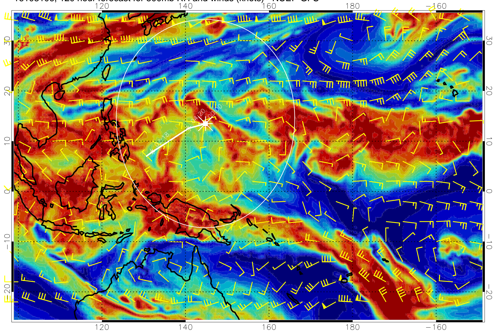
16103106, 120 hour forecast for 500mb RH and winds (knots) - NCEP GFS
