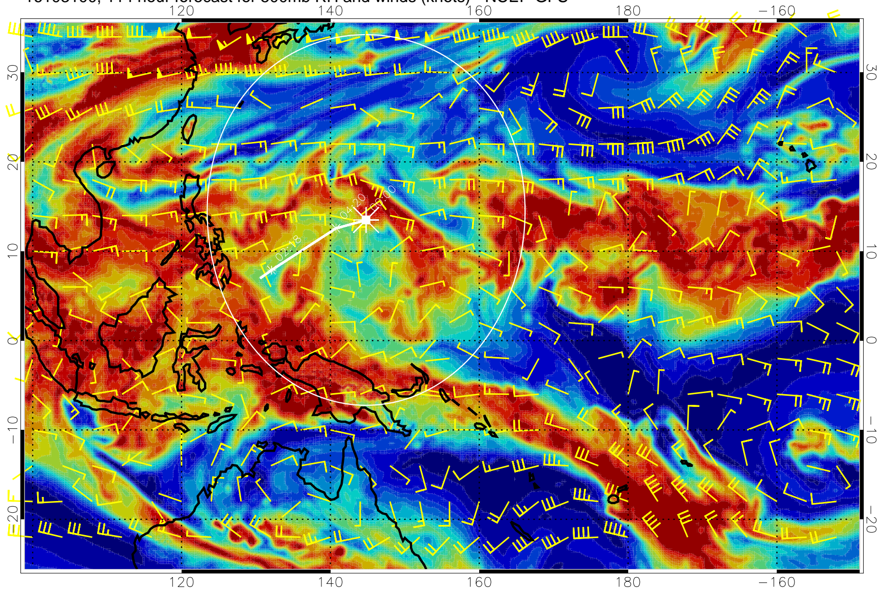
16103100, 114 hour forecast for 500mb RH and winds (knots) - NCEP GFS
