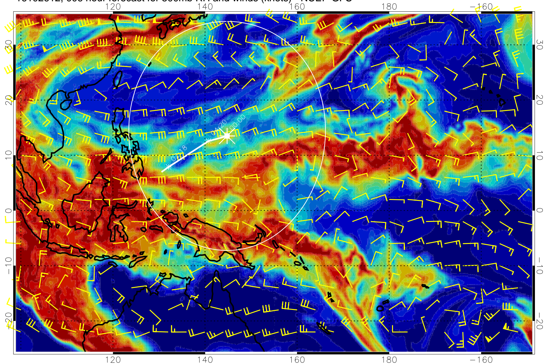
16102612, 006 hour forecast for 500mb RH and winds (knots) - NCEP GFS
