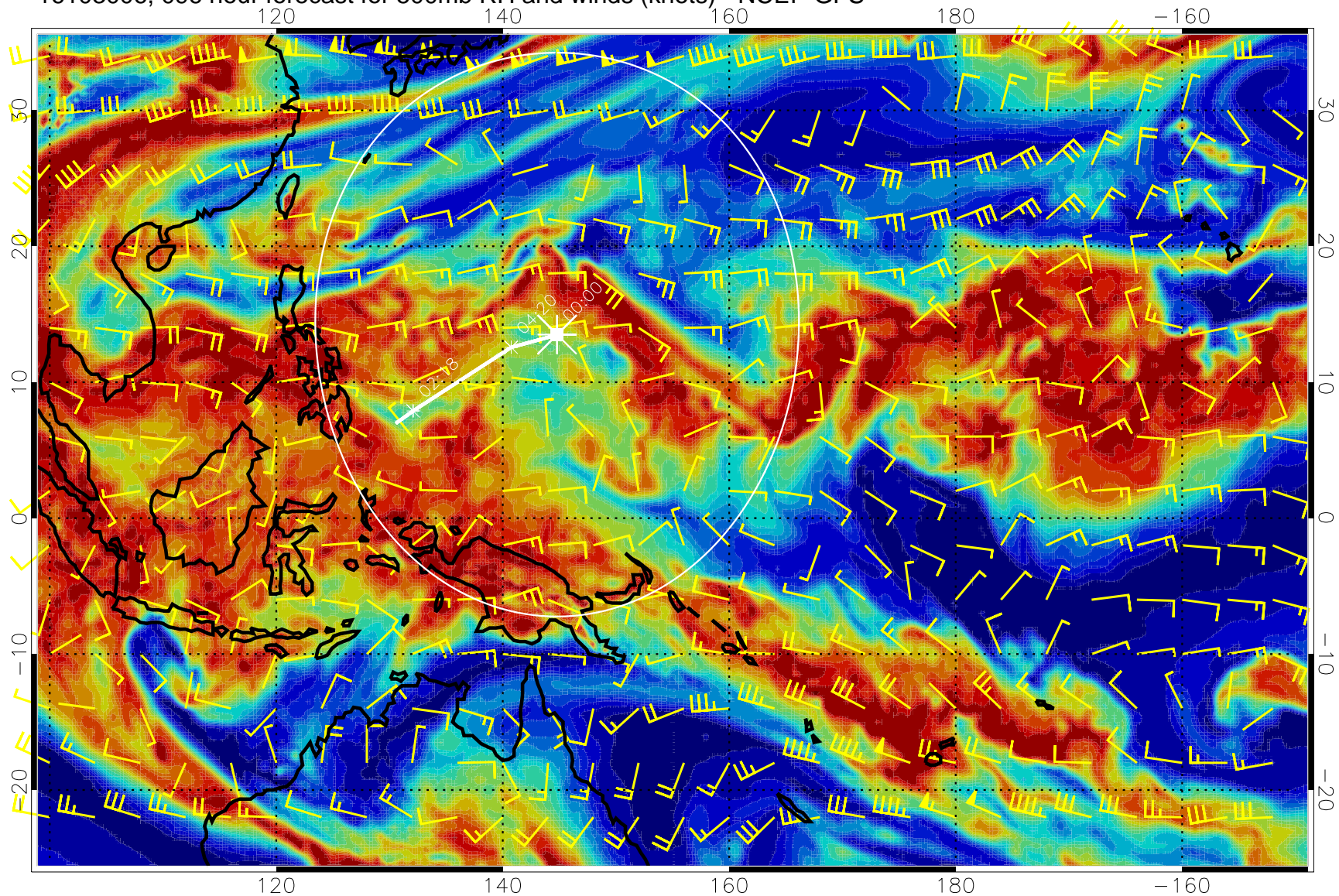
16103006, 096 hour forecast for 500mb RH and winds (knots) - NCEP GFS
