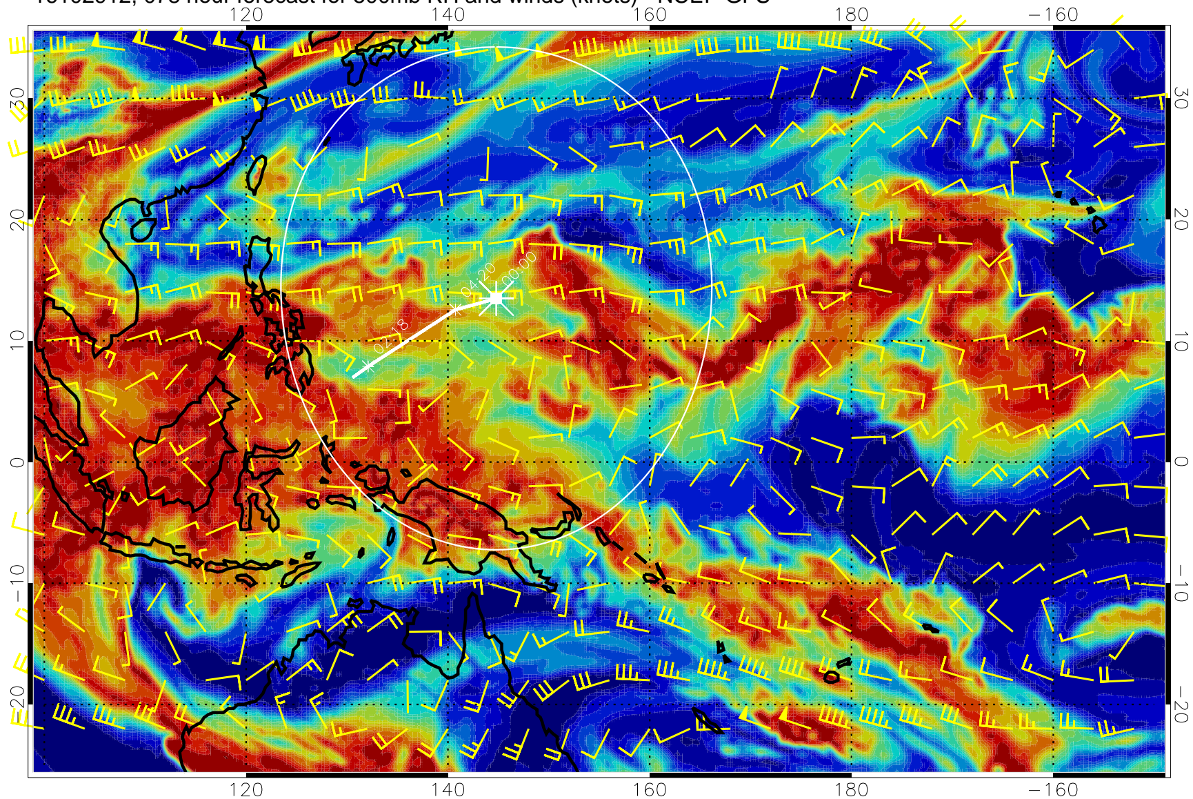
16102912, 078 hour forecast for 500mb RH and winds (knots) - NCEP GFS
