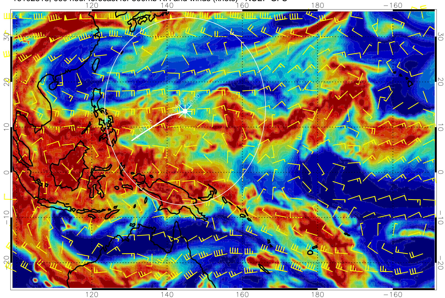
16102818, 060 hour forecast for 500mb RH and winds (knots) - NCEP GFS
