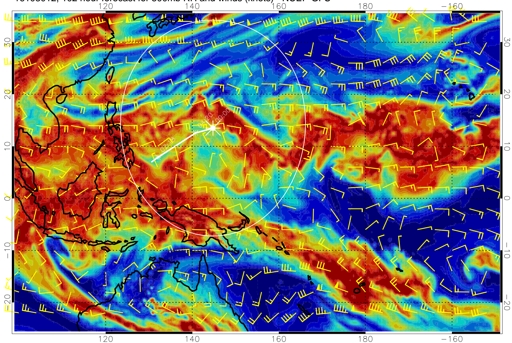
16103012, 102 hour forecast for 500mb RH and winds (knots) - NCEP GFS
